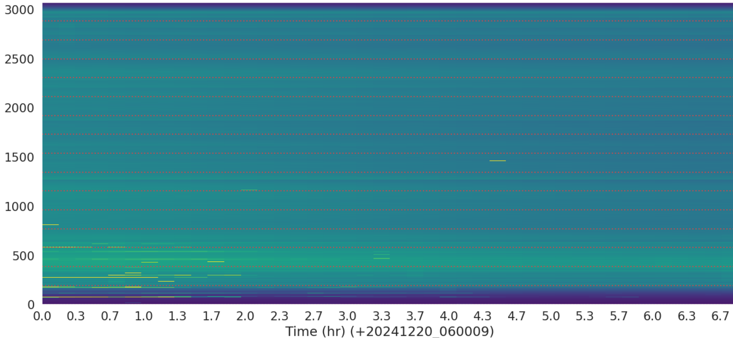
LWA347 - Correlator# 255 - XX - FLAGS: Good
