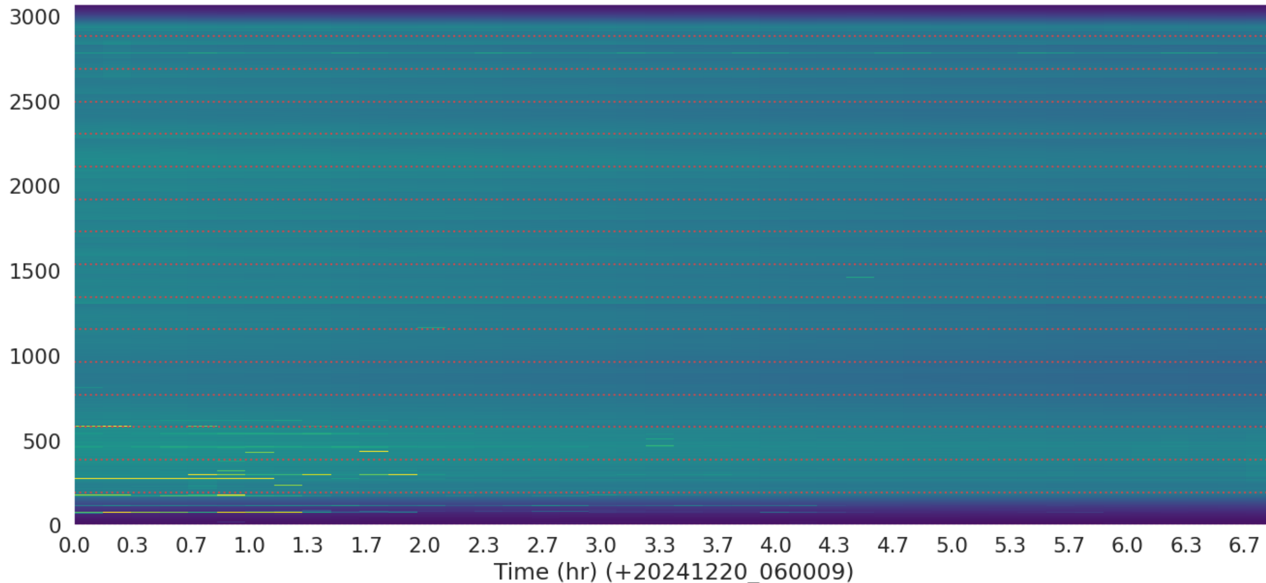
LWA149 - Correlator# 216 - XX - FLAGS: Good
