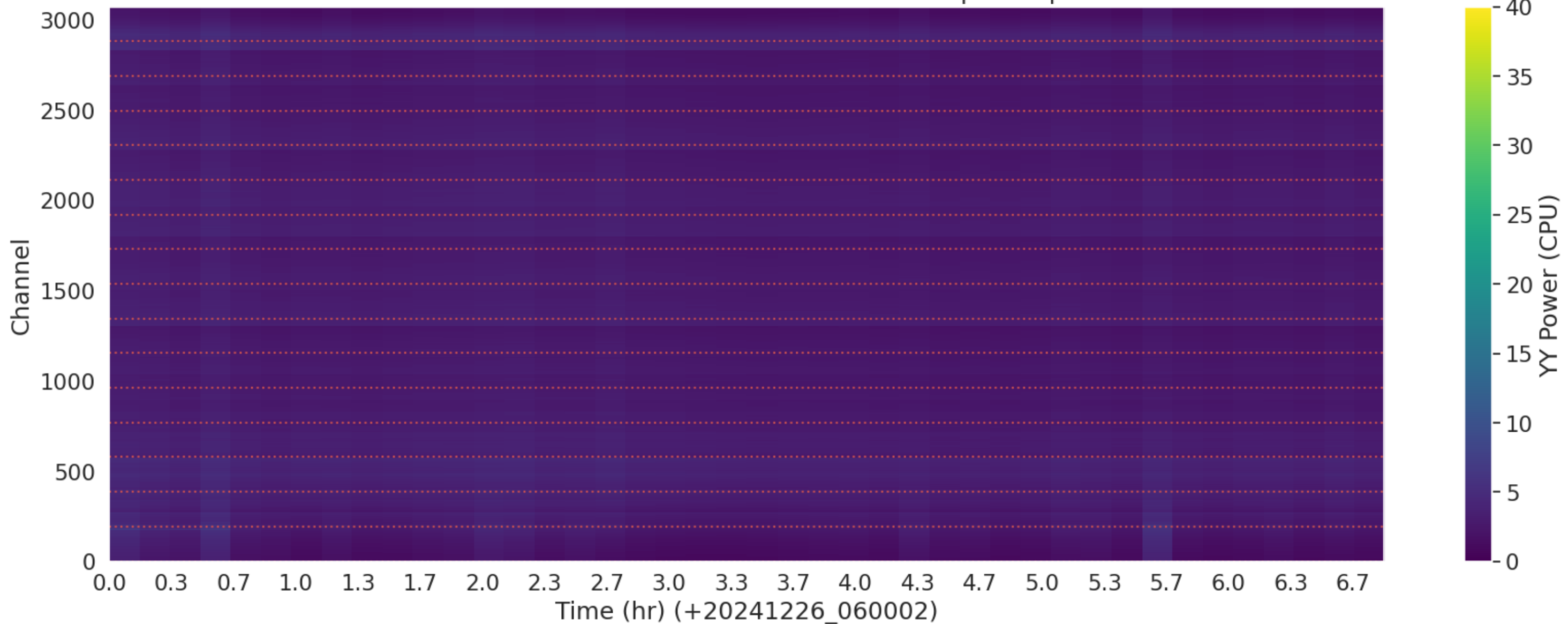
LWA244 - Correlator# 338 - YY - FLAGS: BadSpecShape
