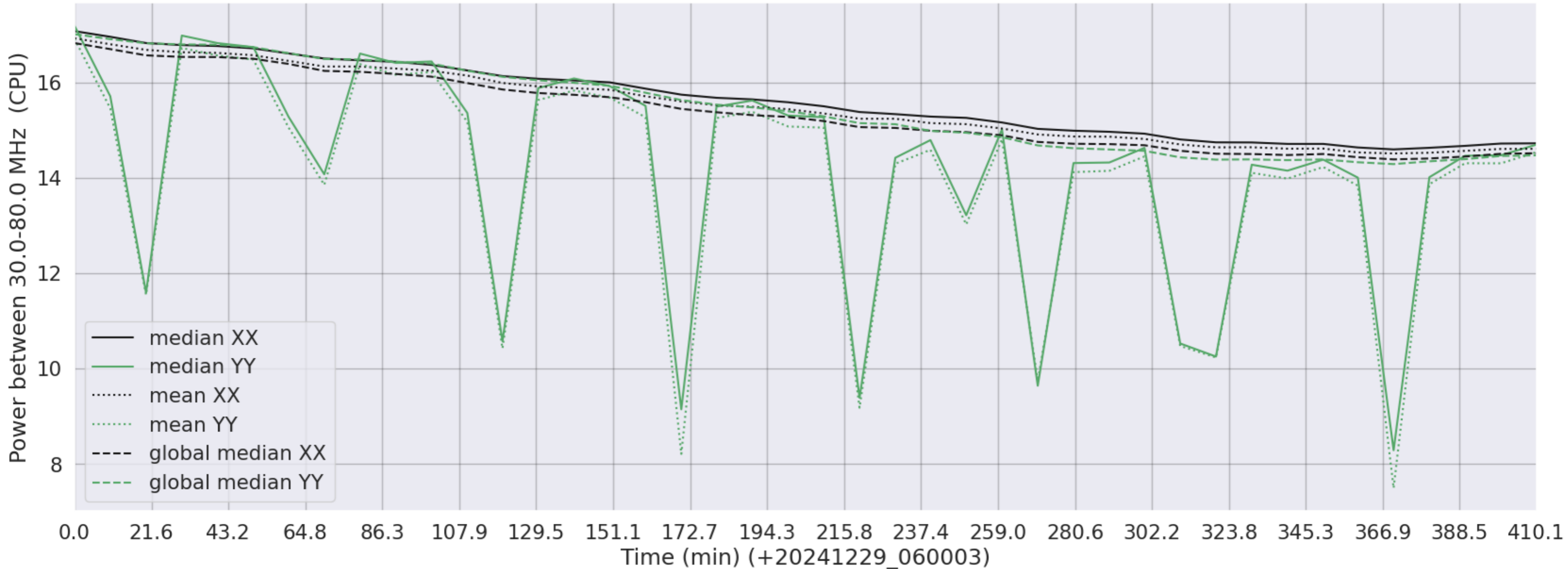
LWA120 - Correlator# 208 - XX FLAGS:Good - YY FLAGS:HighTimeVar
