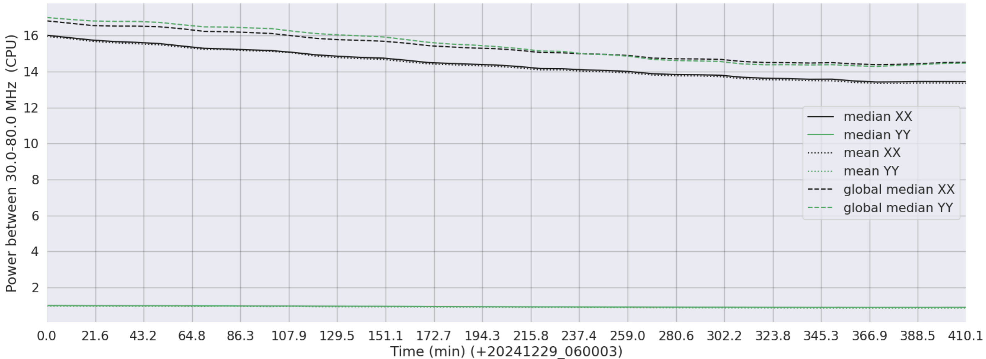
LWA280 - Correlator# 041 - XX FLAGS:Good - YY FLAGS:LowPower
