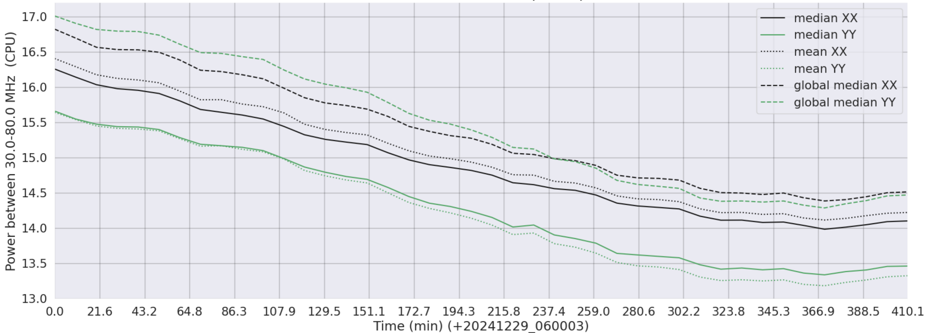
LWA143 - Correlator# 210 - XX FLAGS:BadSpecShape - YY FLAGS:Good
