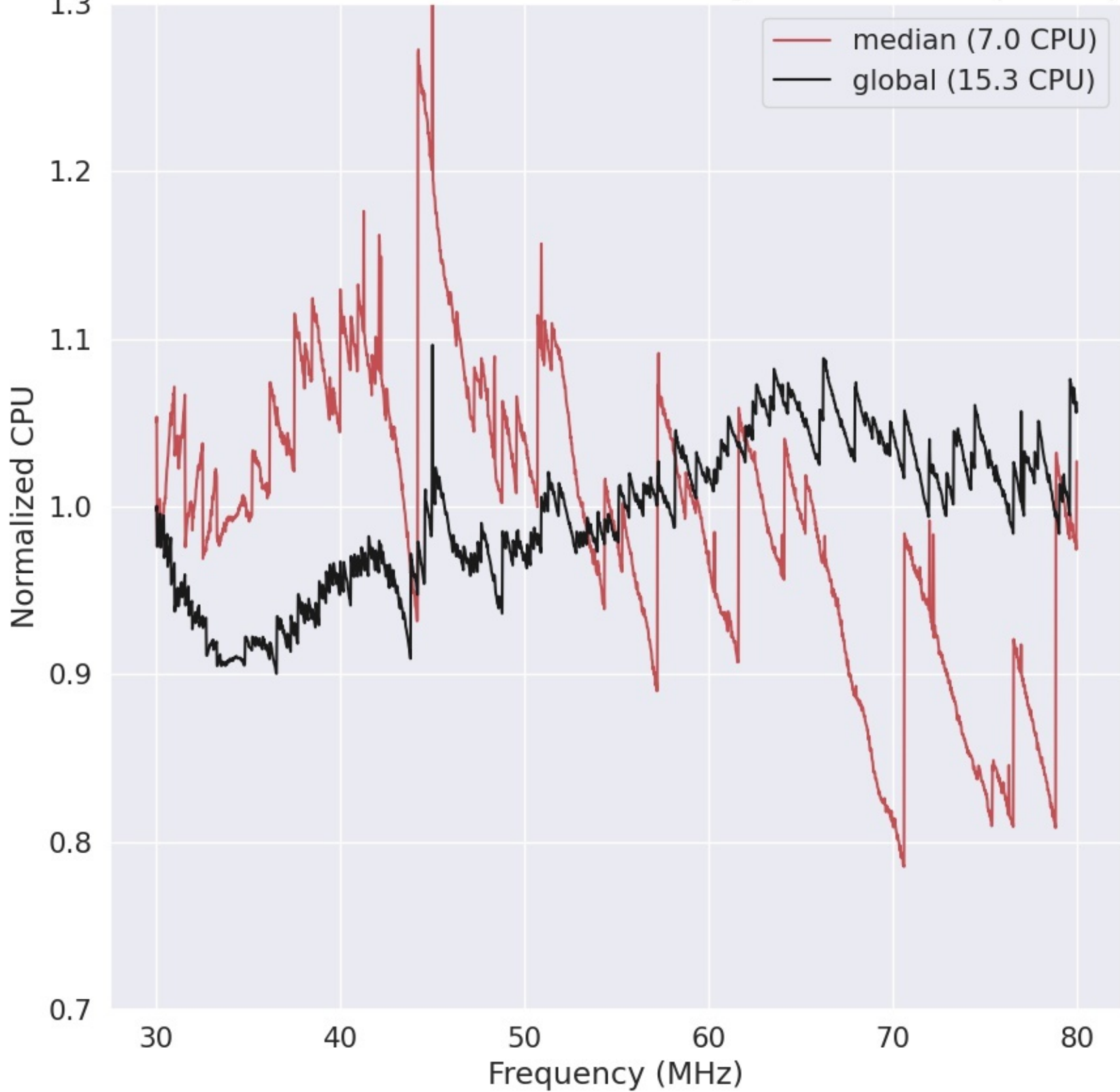
LWA124 - Correlator# 224 - XX - FLAGS:HighTimeVar+BadSpecShape
