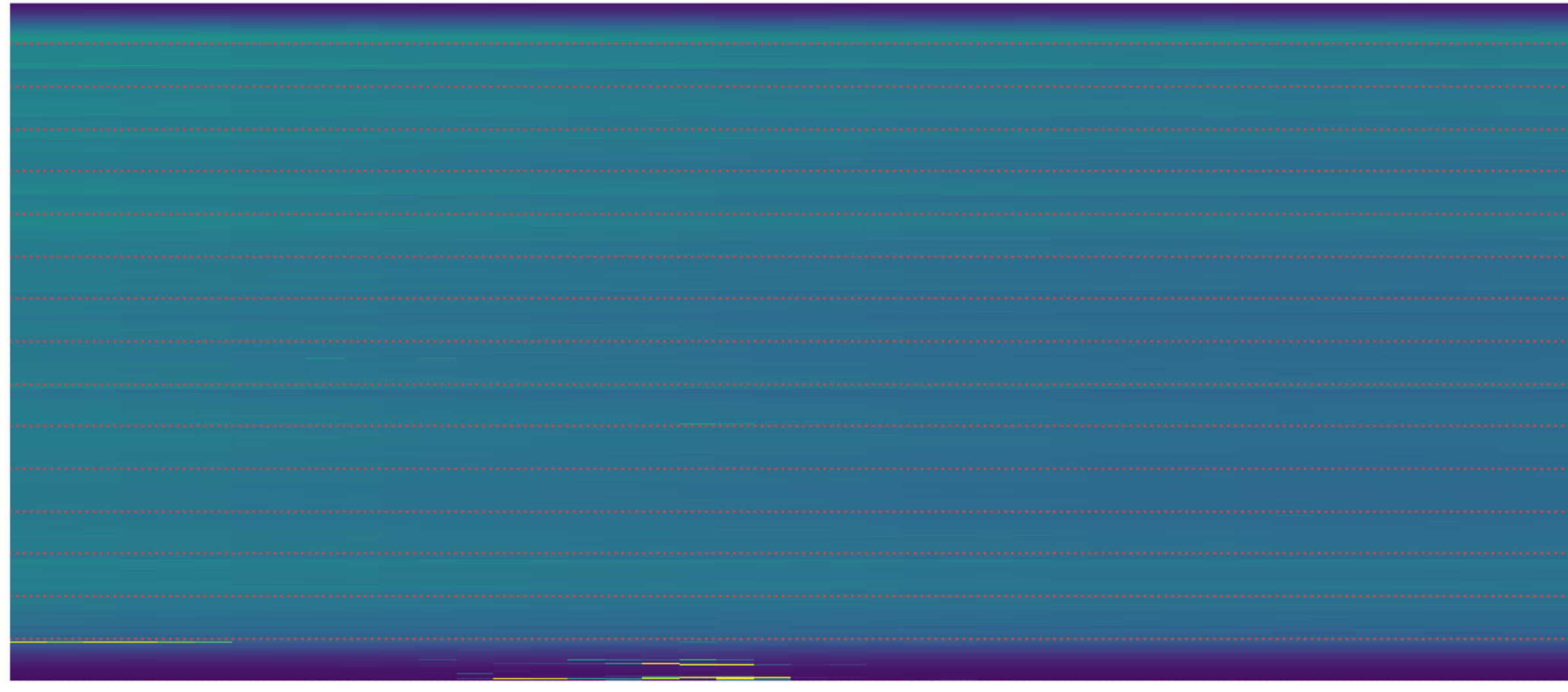
LWA173 - Correlator# 290 - XX - FLAGS: Good
