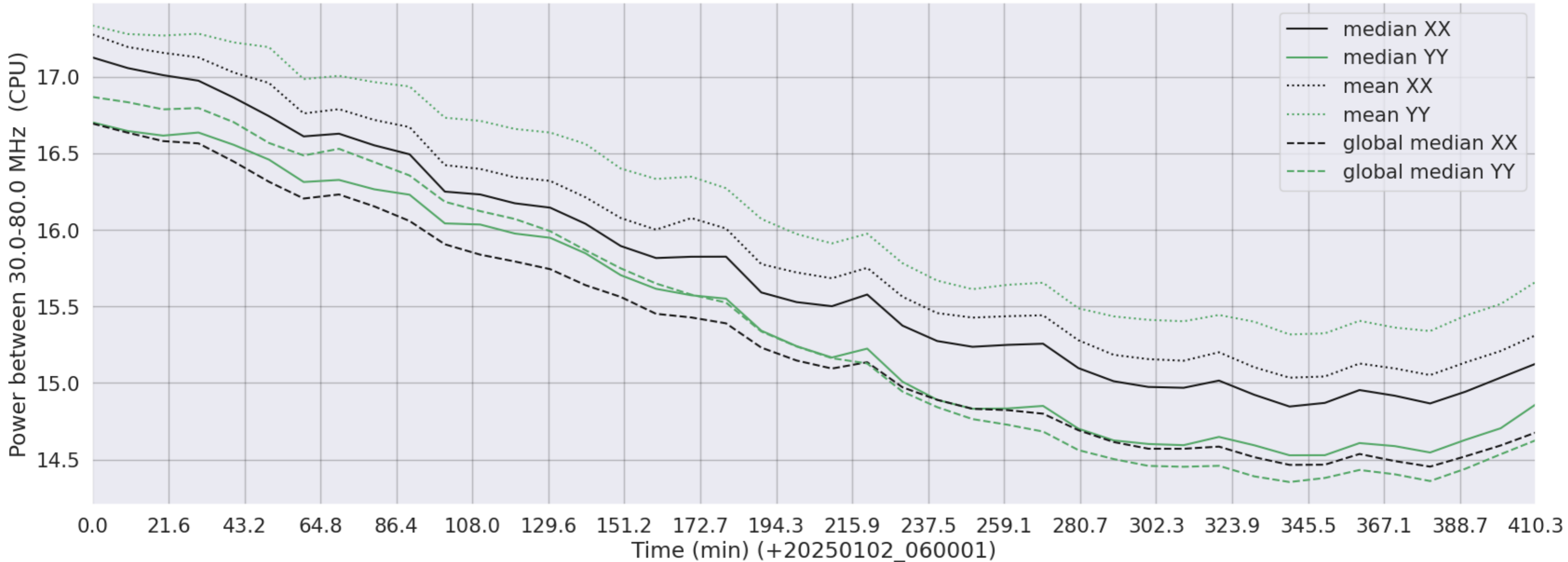
LWA336 - Correlator# 056 - XX FLAGS:Good - YY FLAGS:BadSpecShape
