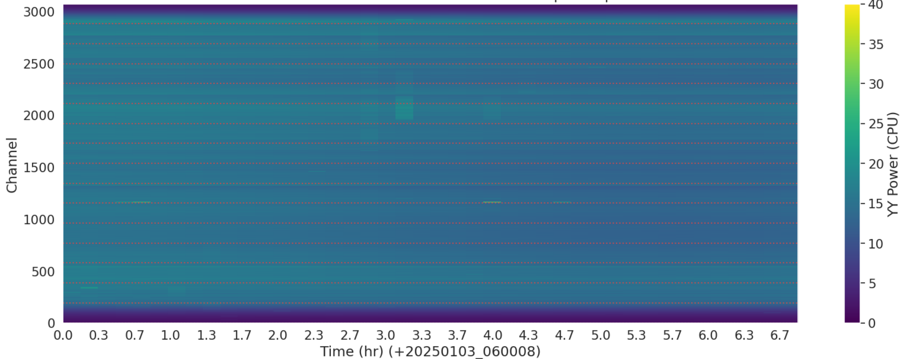
LWA012 - Correlator# 074 - YY - FLAGS: BadSpecShape
