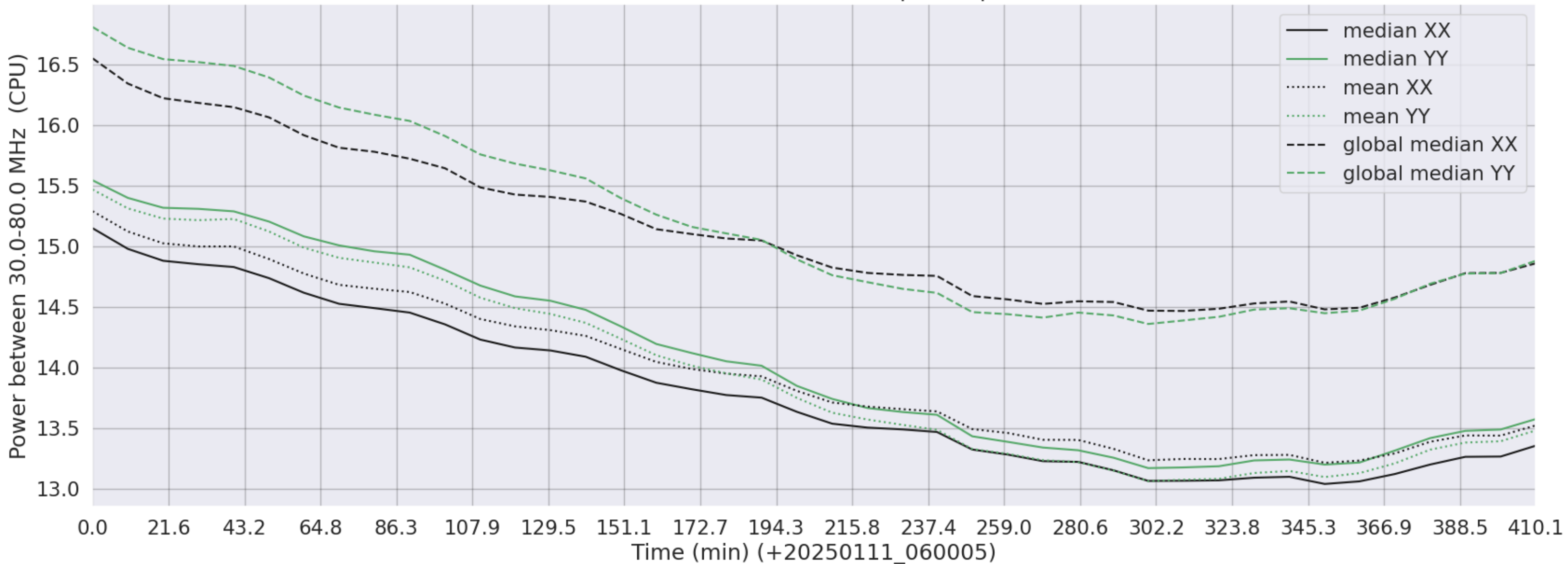
LWA021 - Correlator# 105 - XX FLAGS:BadSpecShape - YY FLAGS:Good
