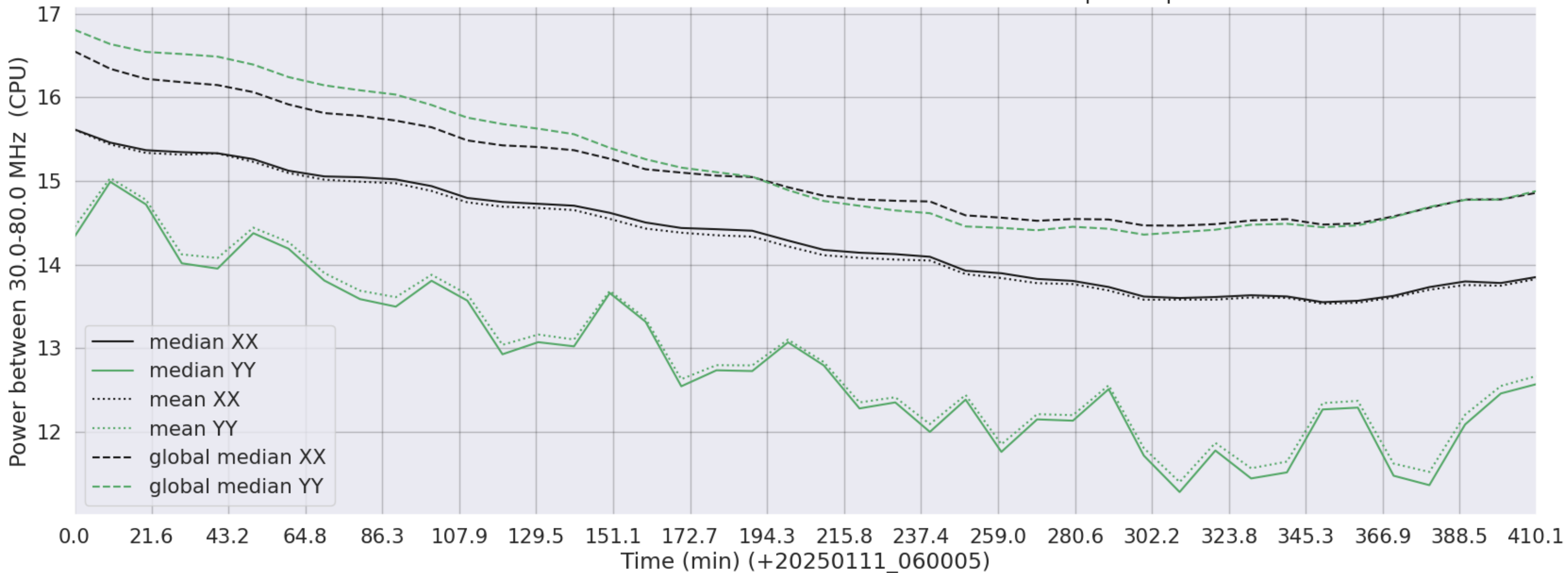
LWA011 - Correlator# 072 - XX FLAGS:Good - YY FLAGS:BadSpecShape
