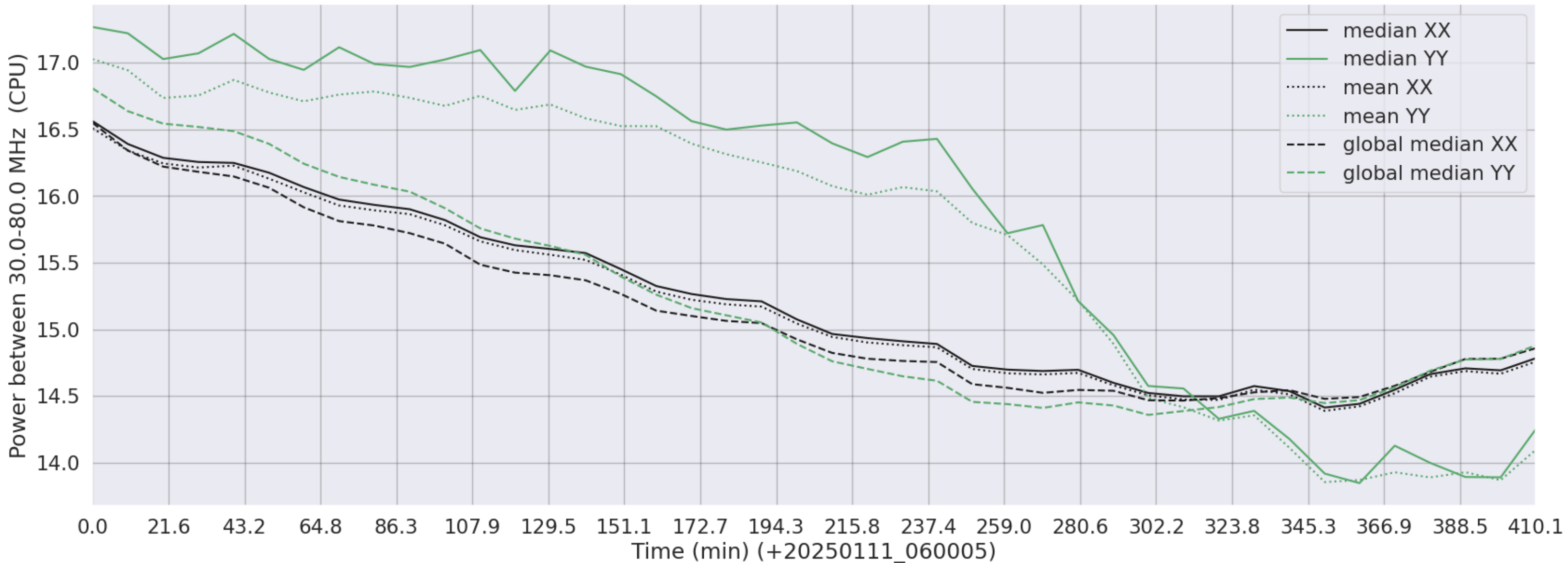
LWA282 - Correlator# 010 - XX FLAGS:Good - YY FLAGS:Good
