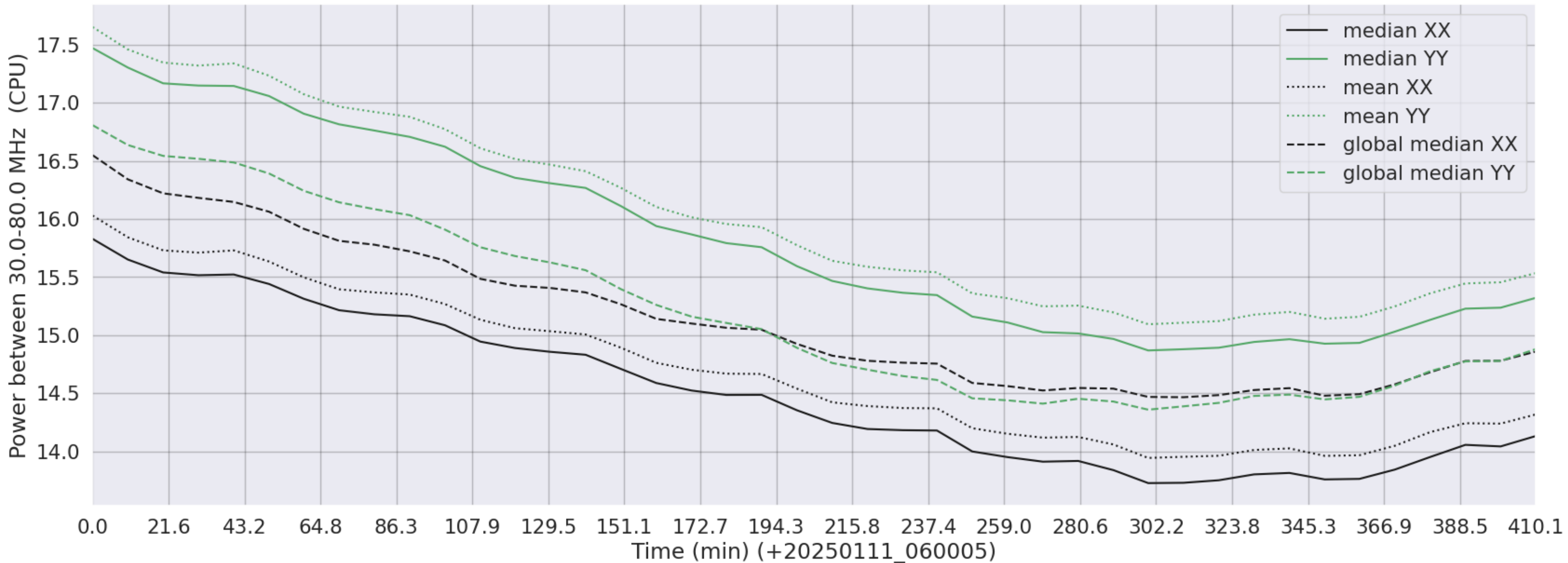
LWA239 - Correlator# 313 - XX FLAGS:Good - YY FLAGS:Good
