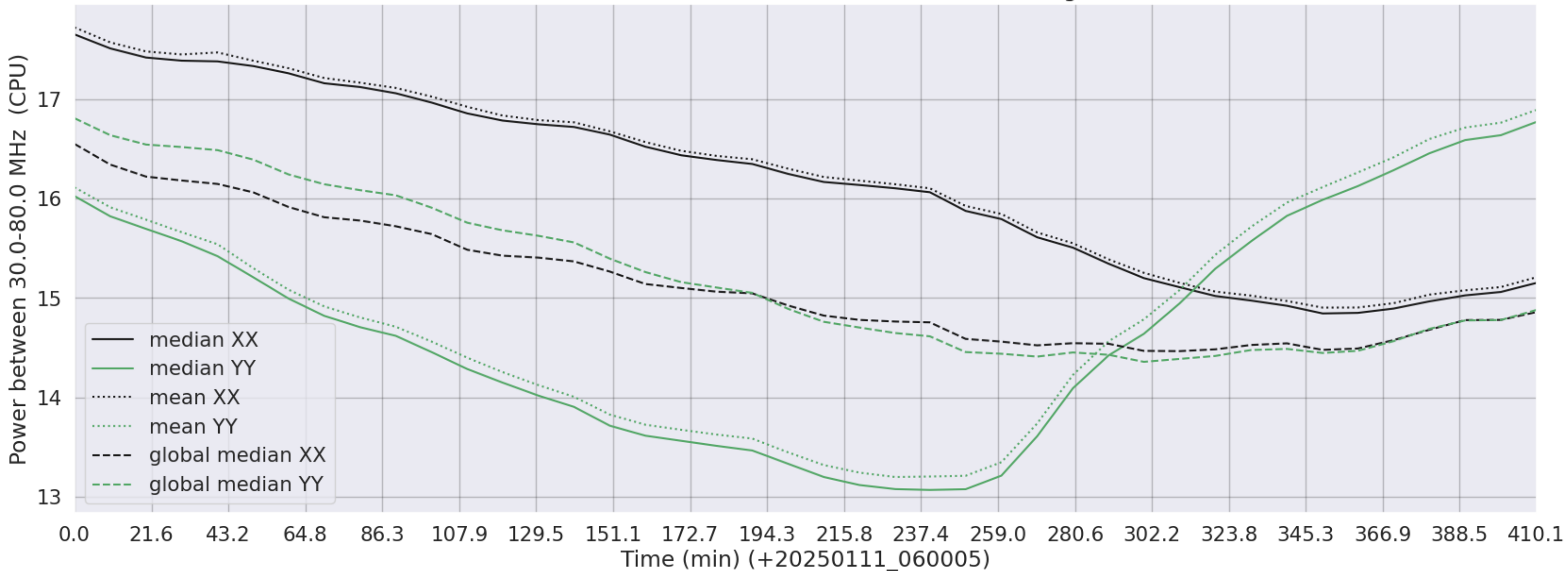
LWA347 - Correlator# 255 - XX FLAGS:Good - YY FLAGS:HighTimeVar
