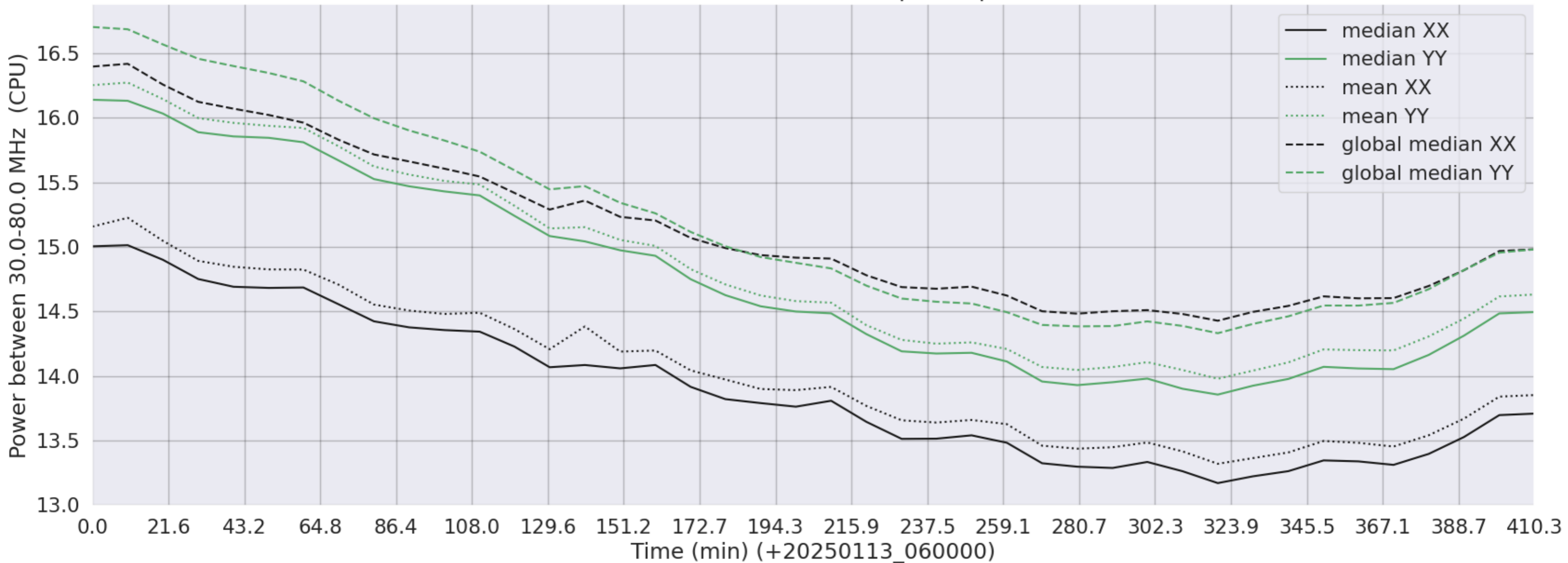
LWA042 - Correlator# 078 - XX FLAGS:BadSpecShape - YY FLAGS:Good
