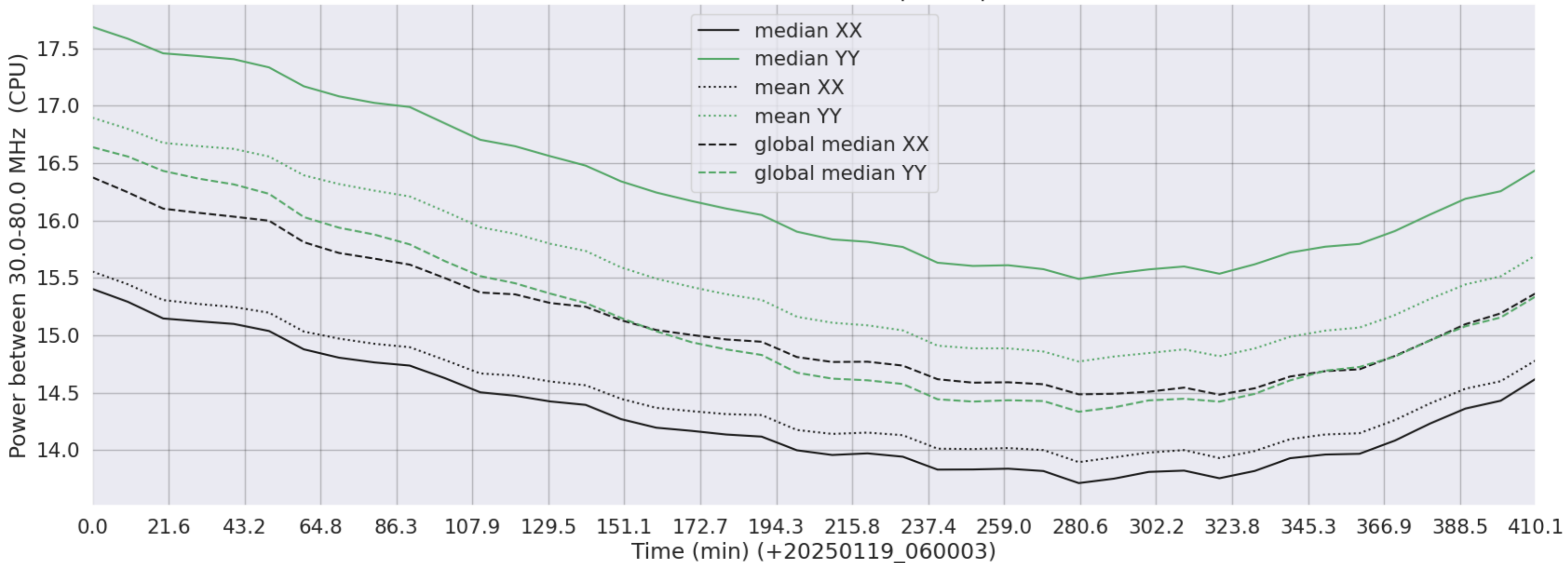
LWA205 - Correlator# 297 - XX FLAGS:BadSpecShape - YY FLAGS:Good
