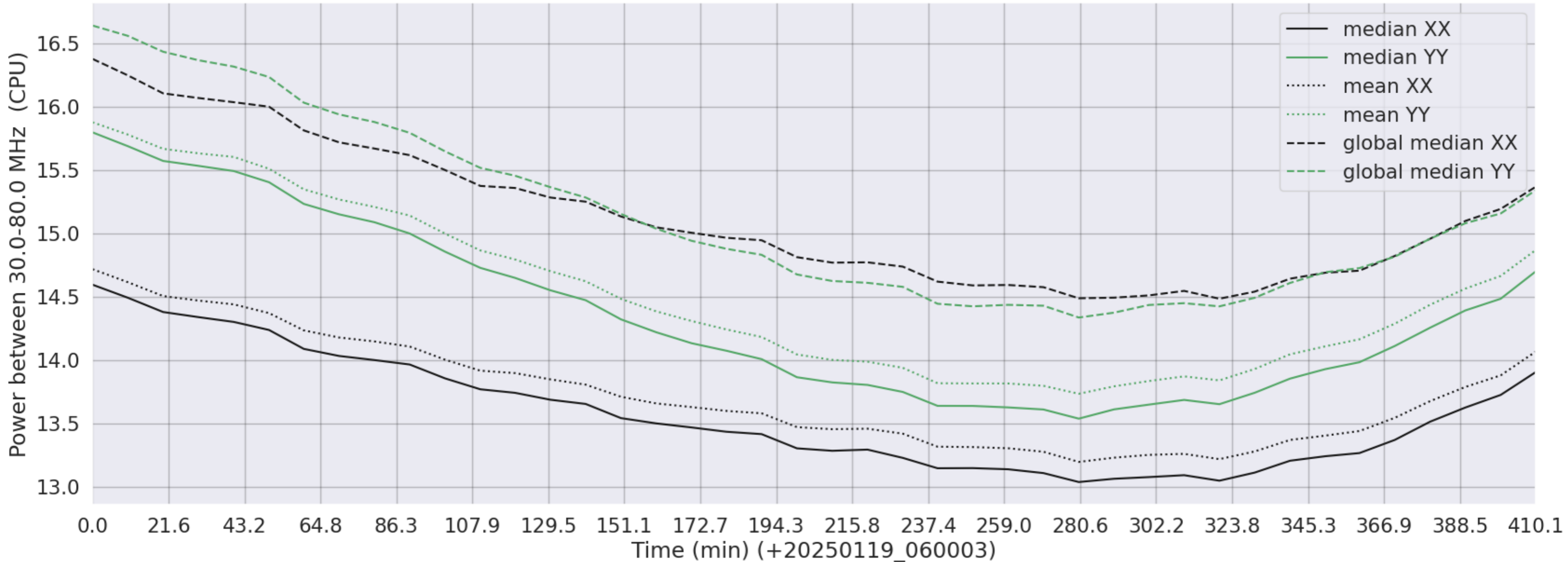
LWA047 - Correlator# 085 - XX FLAGS:BadSpecShape - YY FLAGS:BadSpecShape
