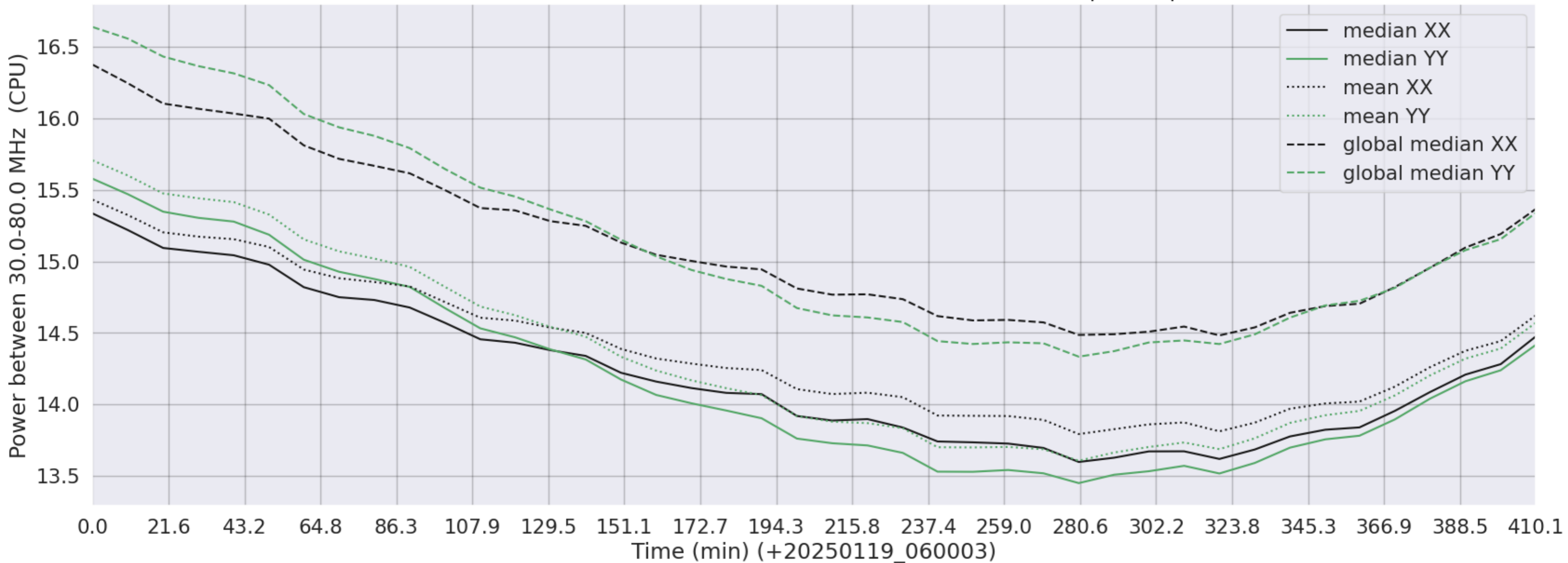
LWA012 - Correlator# 074 - XX FLAGS:Good - YY FLAGS:BadSpecShape
