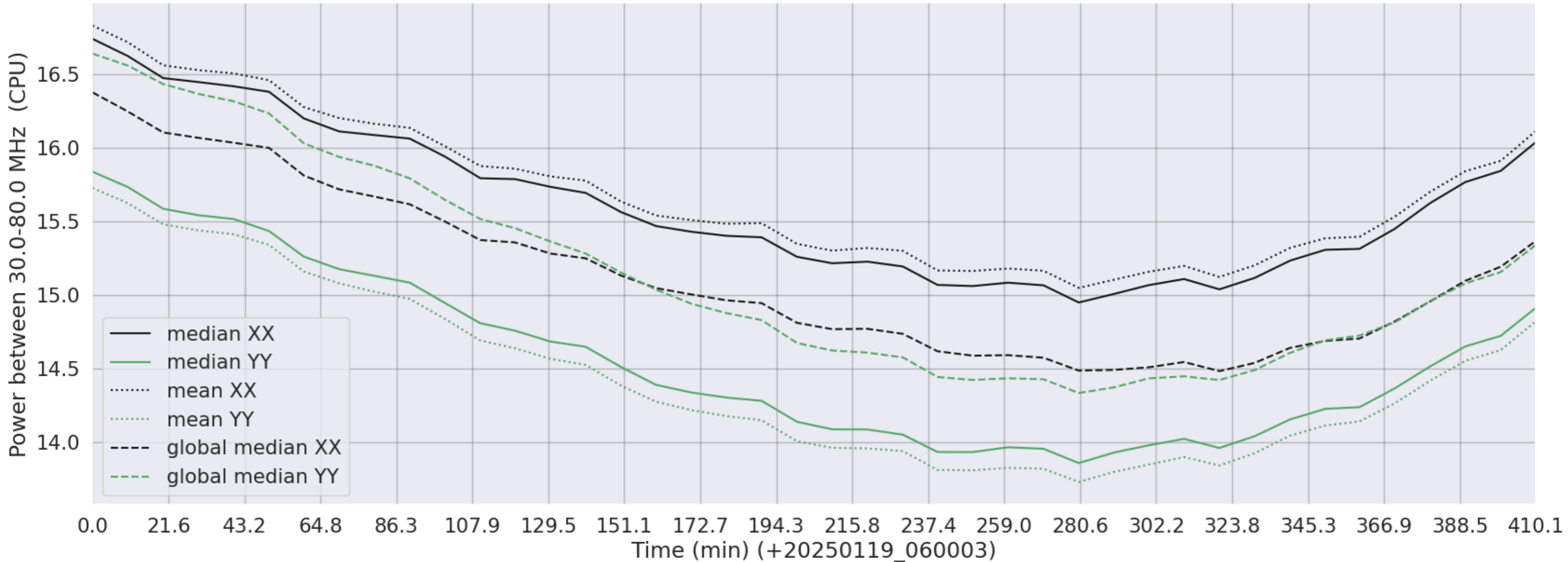
LWA240 - Correlator# 312 - XX FLAGS:Good - YY FLAGS:BadSpecShape
