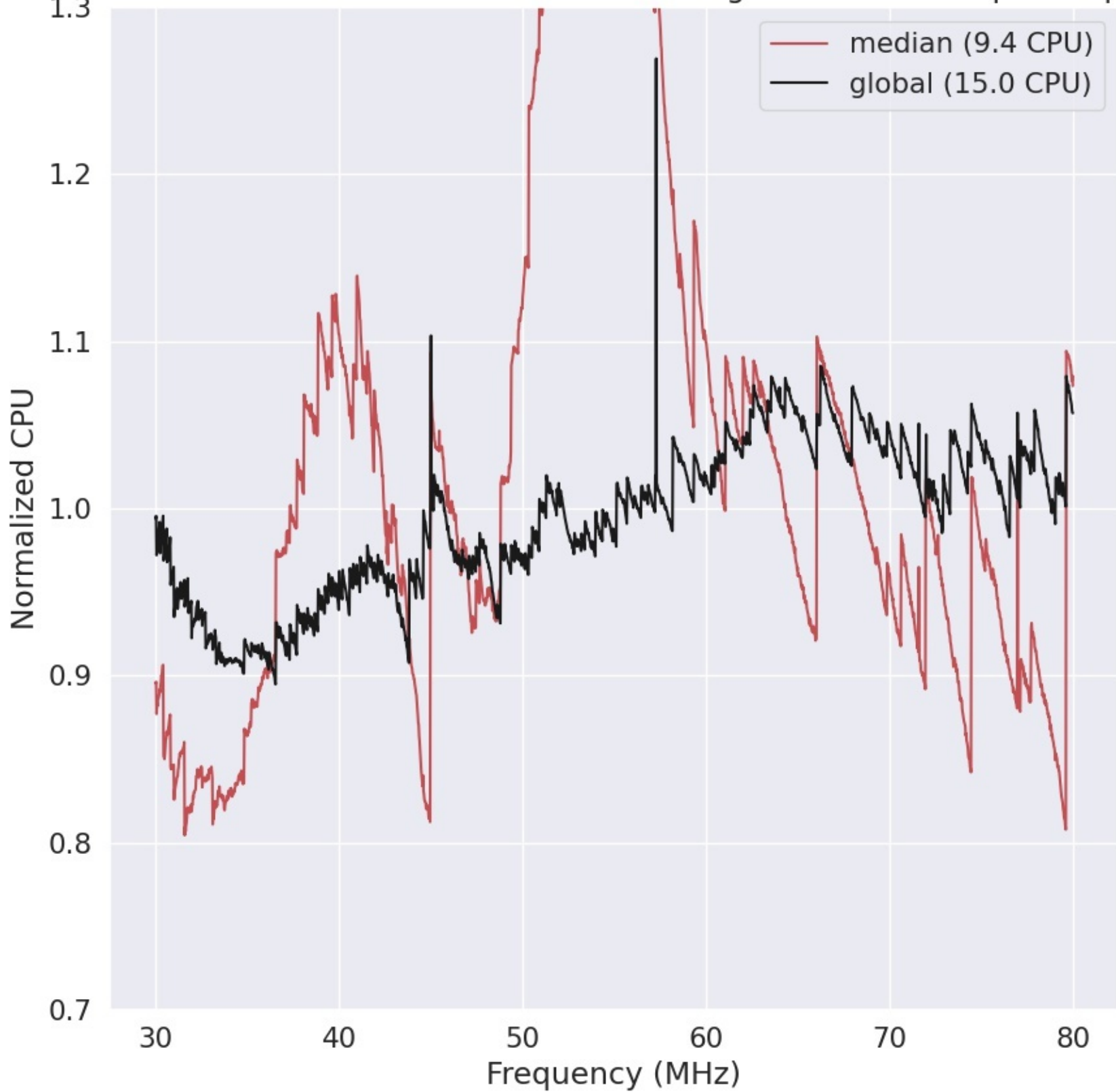
LWA105 - Correlator# 178 - XX - FLAGS:HighTimeVar+BadSpecShape
