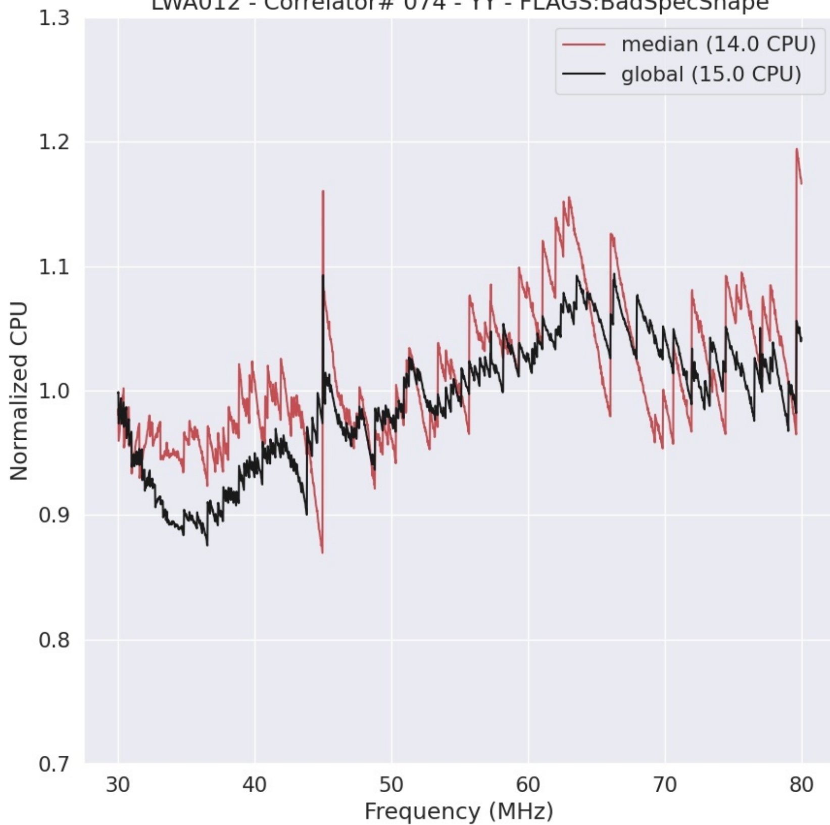
LWA012 - Correlator# 074 - YY - FLAGS:BadSpecShape
