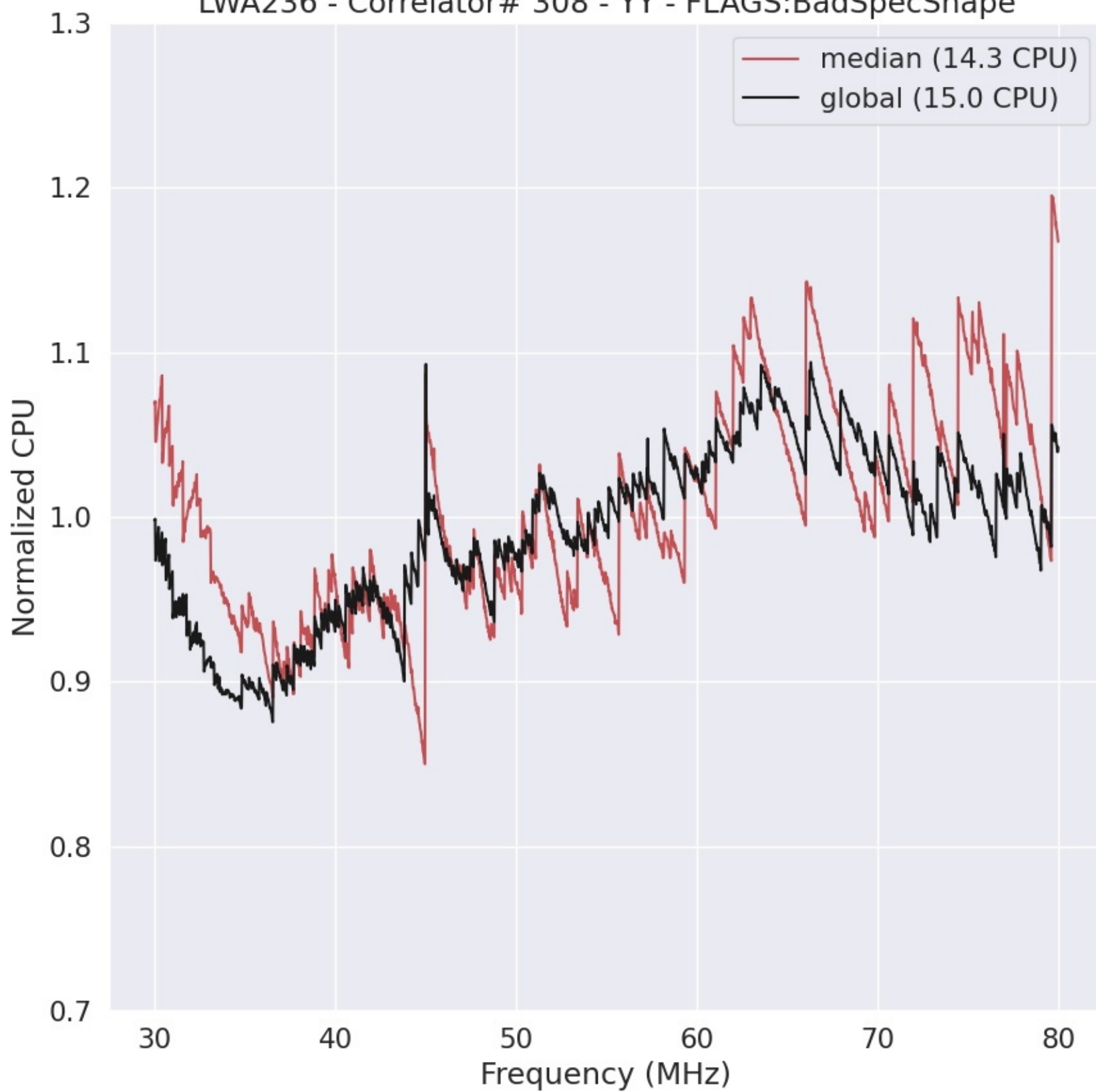
LWA236 - Correlator# 308 - YY - FLAGS:BadSpecShape
