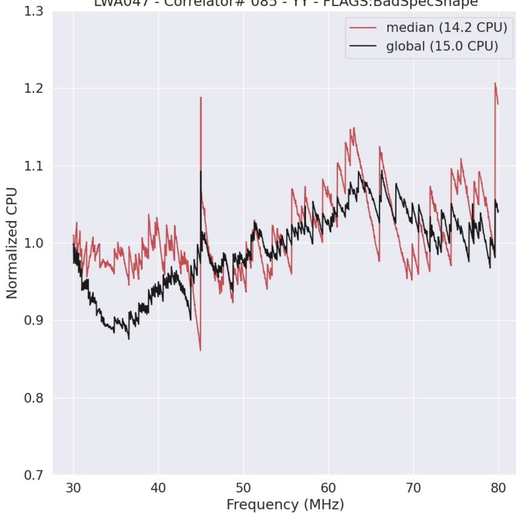
LWA047 - Correlator# 085 - YY - FLAGS:BadSpecShape
