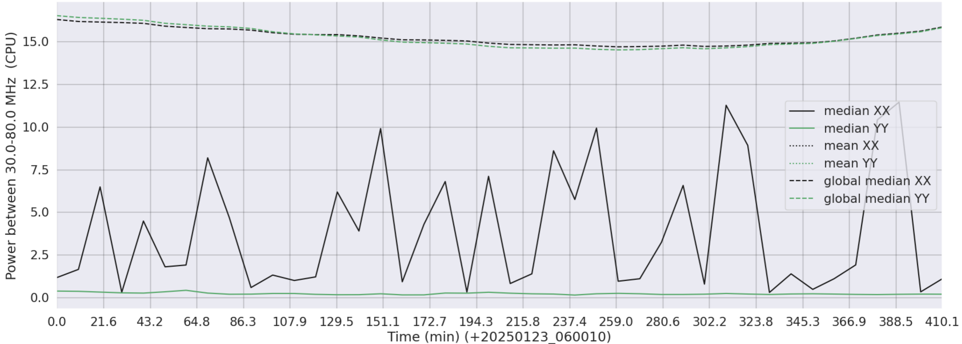
LWA124 - Correlator# 224 - XX FLAGS:HighTimeVar - YY FLAGS:LowPower
