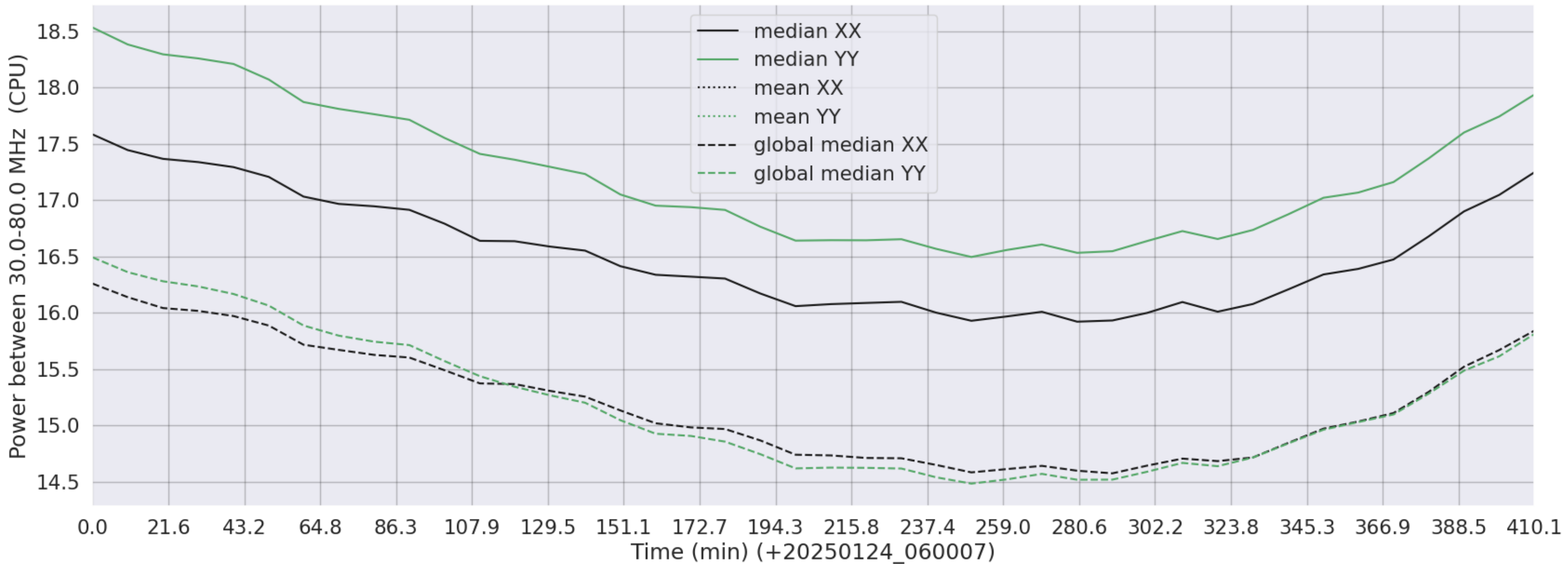
LWA165 - Correlator# 266 - XX FLAGS:Good - YY FLAGS:Good
