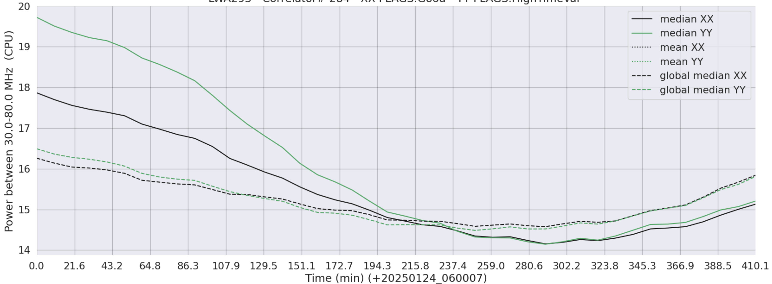
LWA293 - Correlator# 284 - XX FLAGS:Good - YY FLAGS:HighTimeVar
