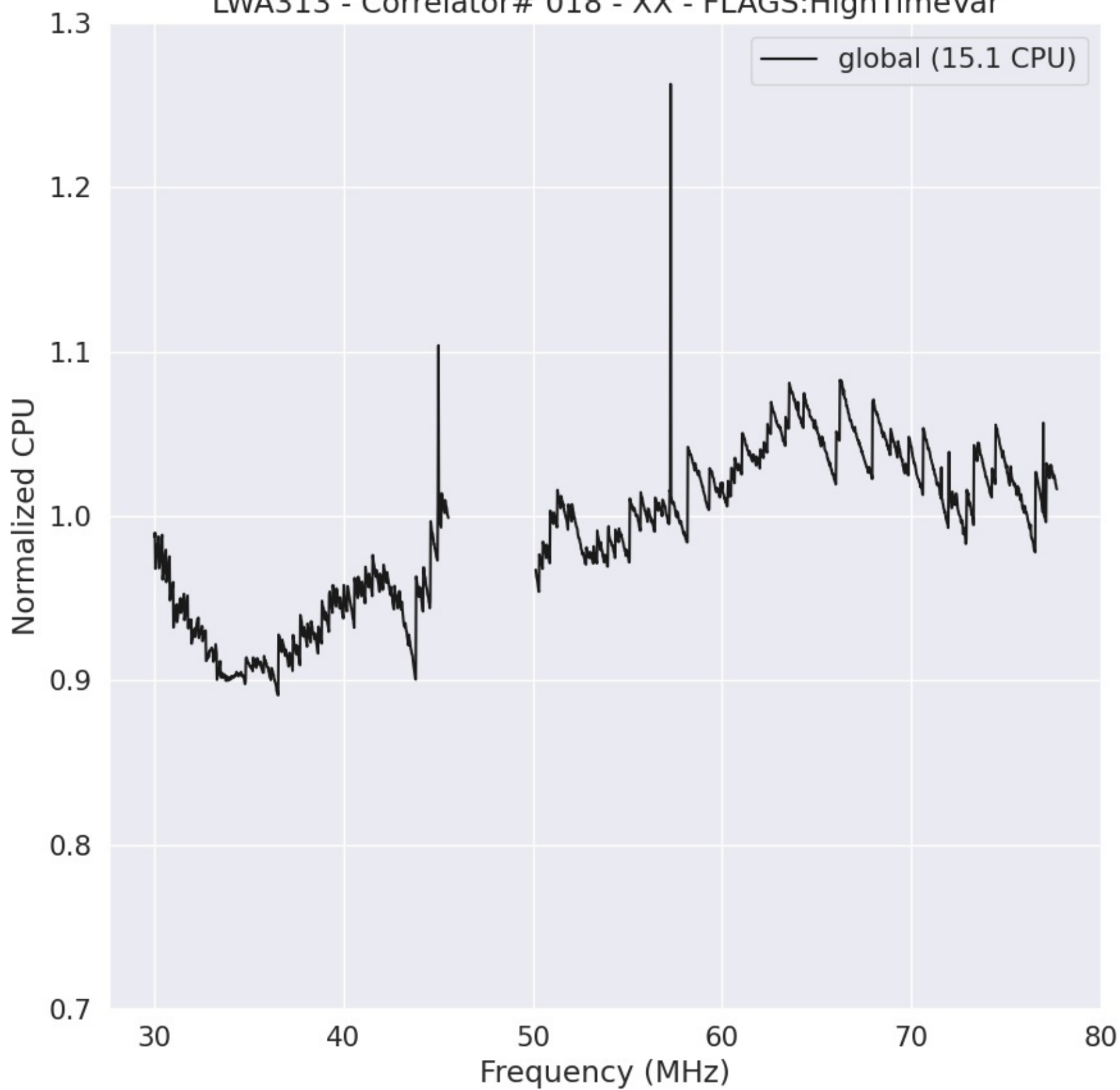
LWA313 - Correlator# 018 - XX - FLAGS:HighTimeVar
