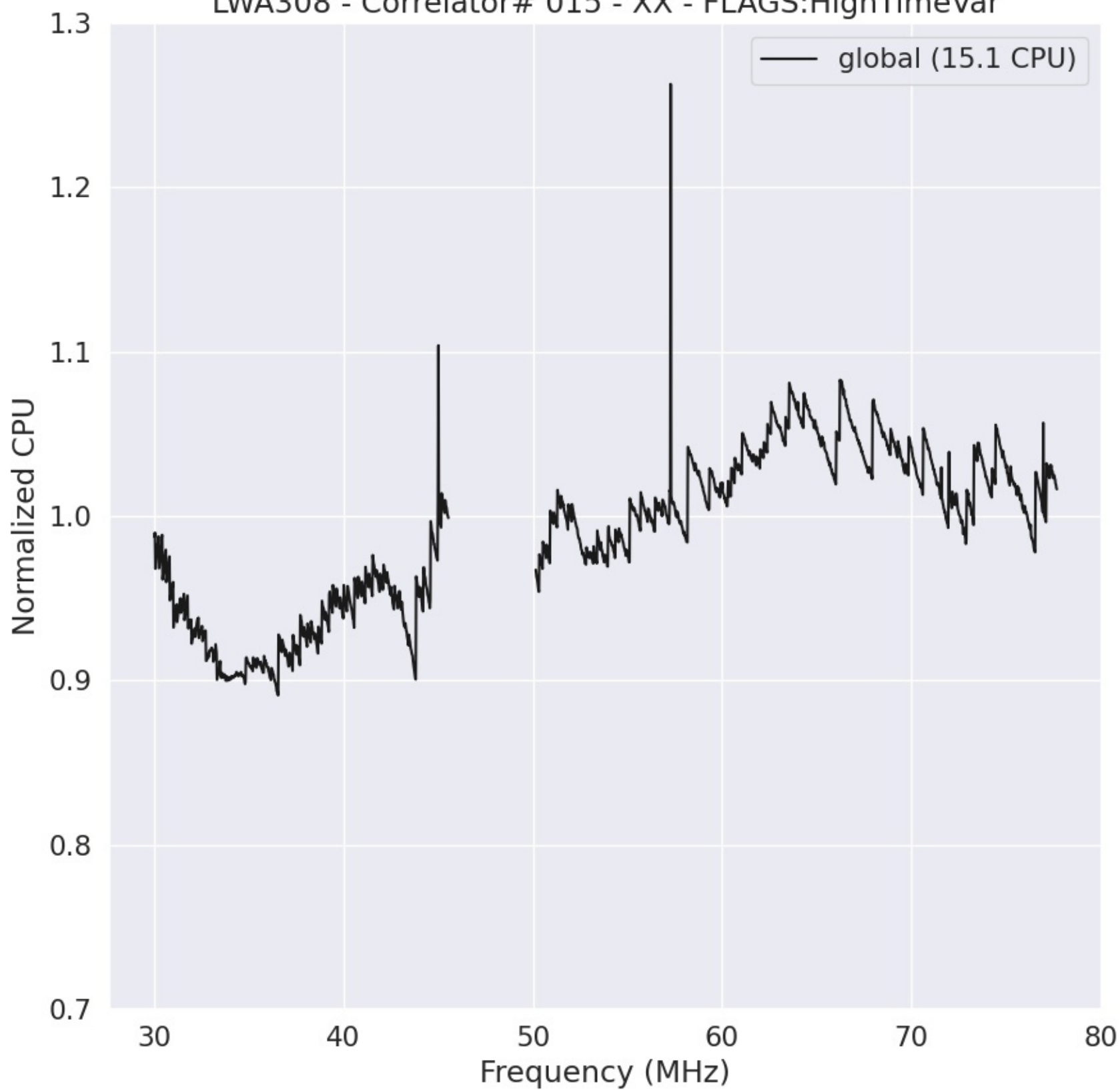
LWA308 - Correlator# 015 - XX - FLAGS:HighTimeVar
