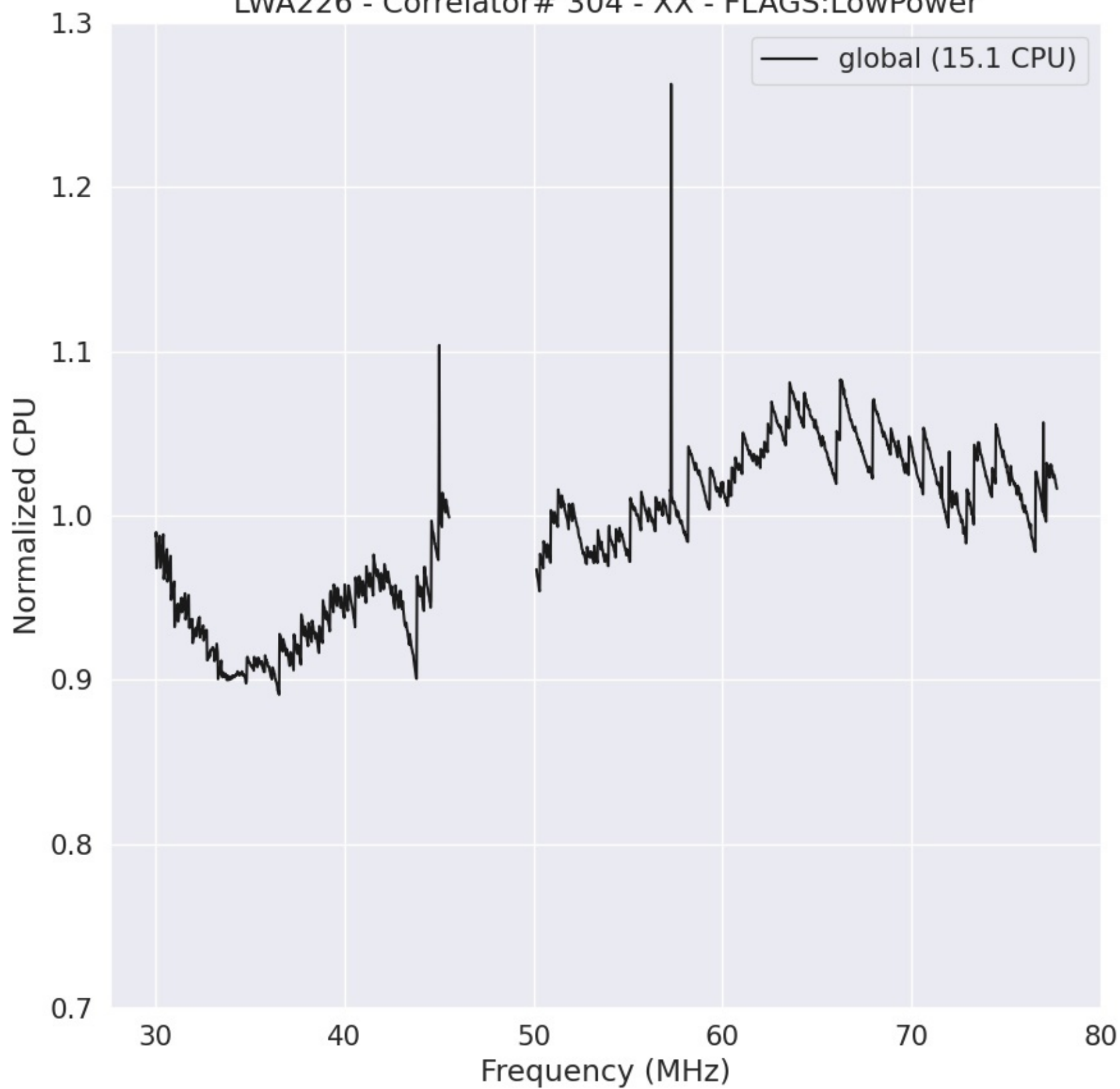
LWA226 - Correlator# 304 - XX - FLAGS:LowPower
