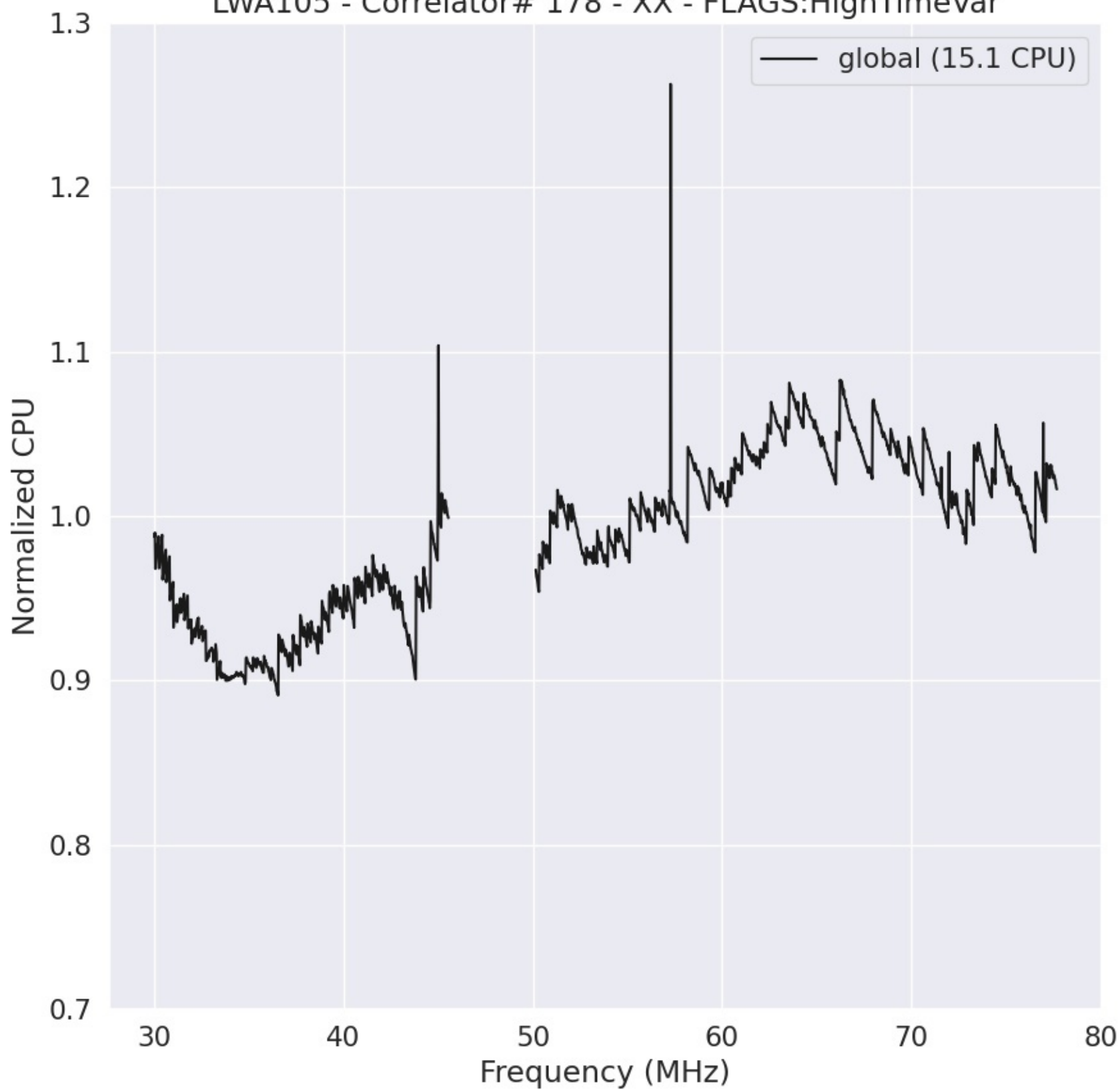
LWA105 - Correlator# 178 - XX - FLAGS:HighTimeVar
