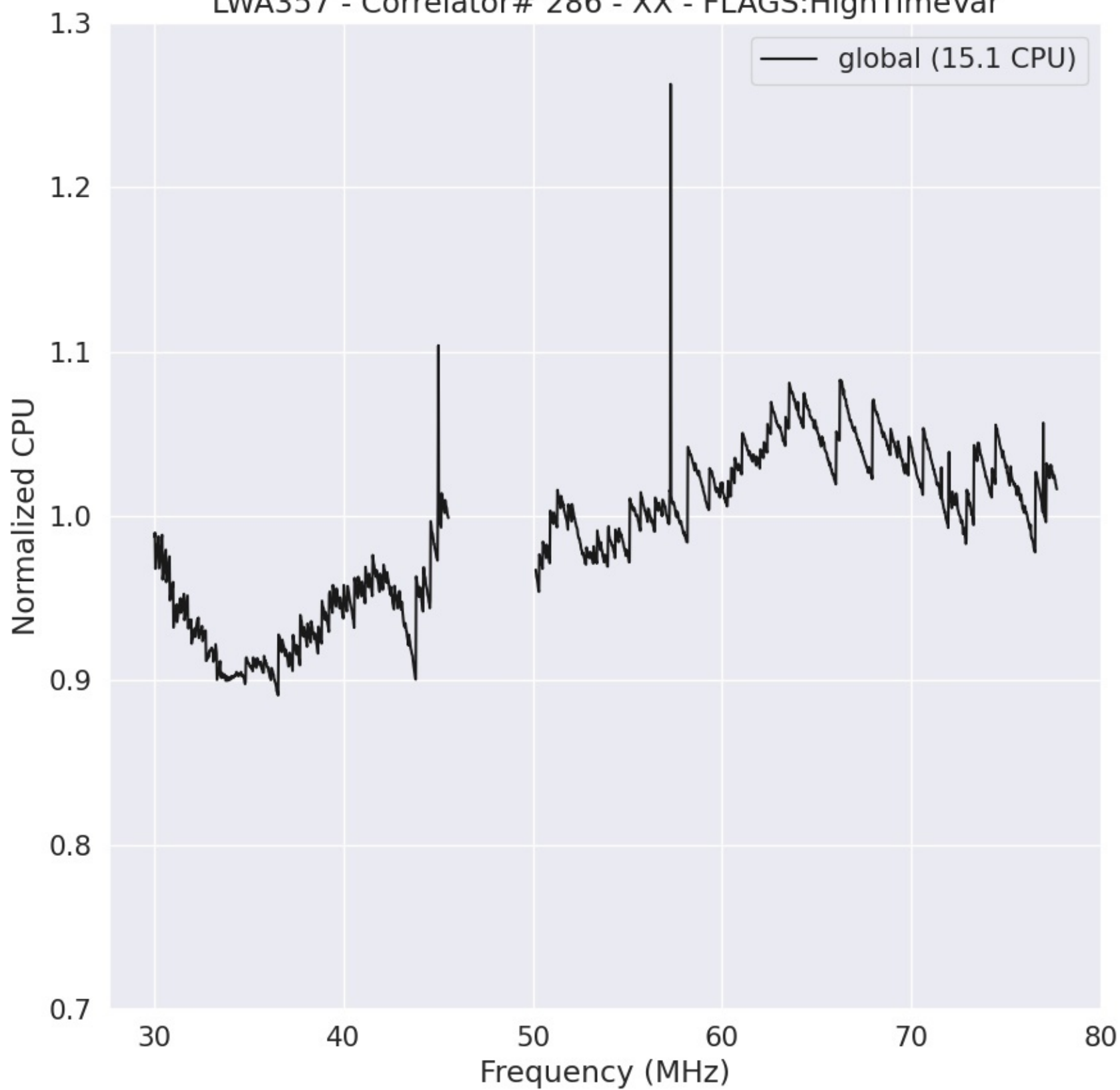
LWA357 - Correlator# 286 - XX - FLAGS:HighTimeVar
