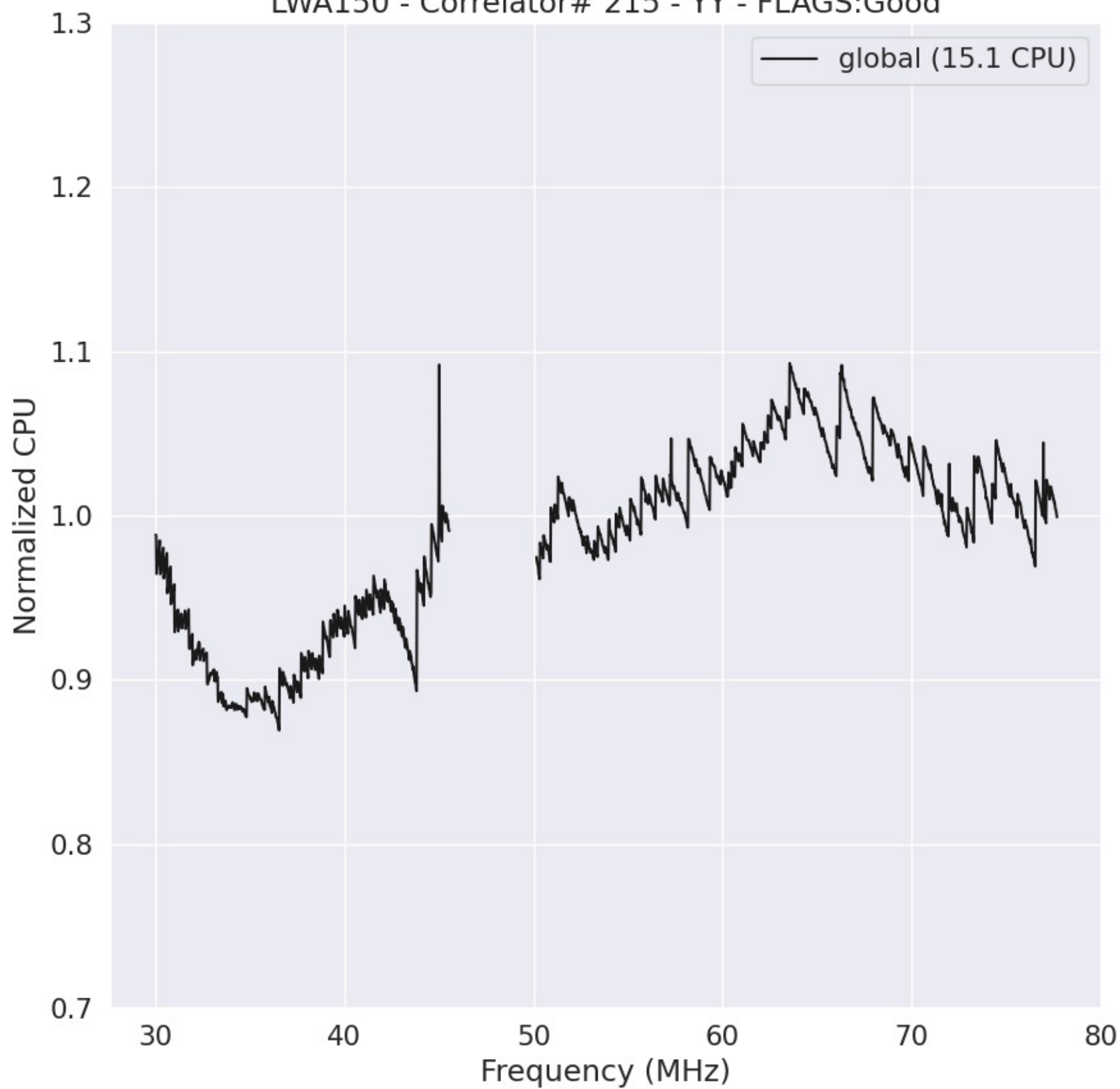
LWA150 - Correlator# 215 - YY - FLAGS:Good
