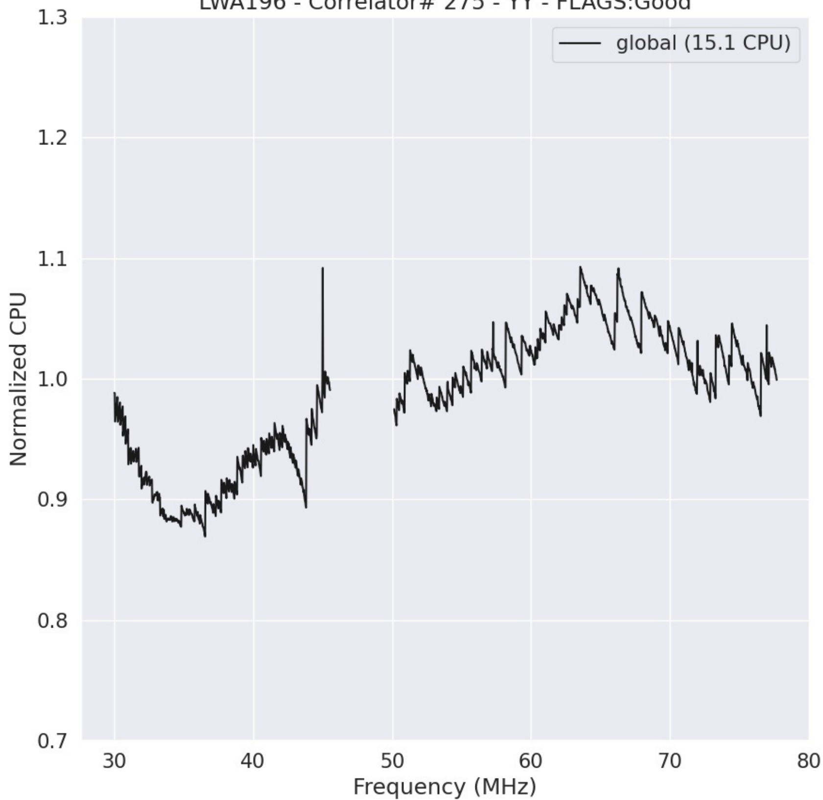
LWA196 - Correlator# 275 - YY - FLAGS:Good
