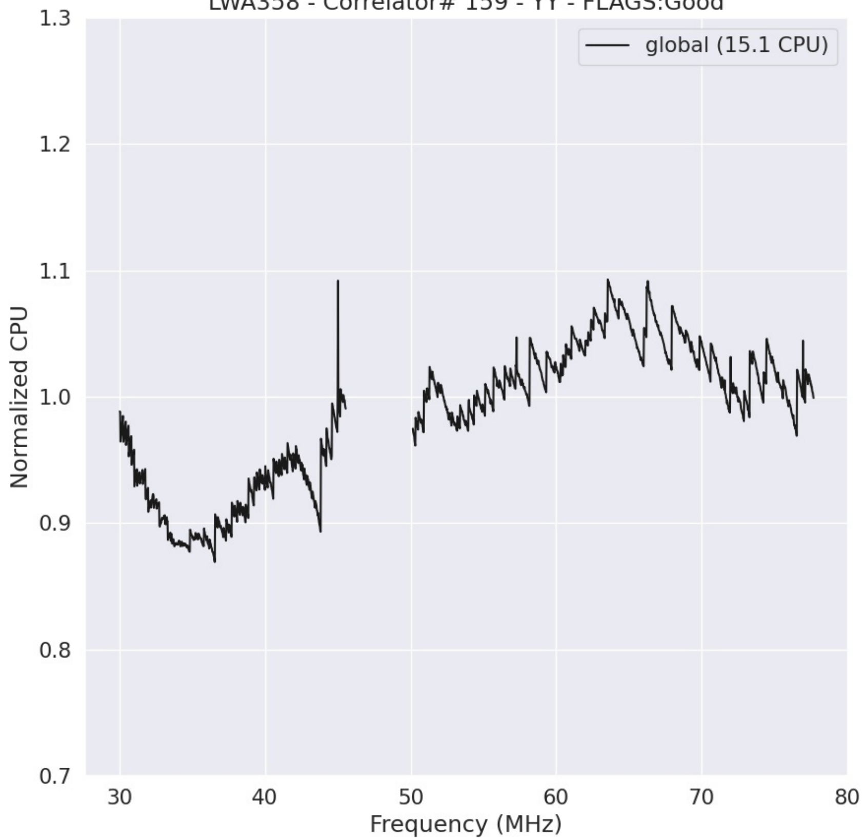
LWA358 - Correlator# 159 - YY - FLAGS:Good
