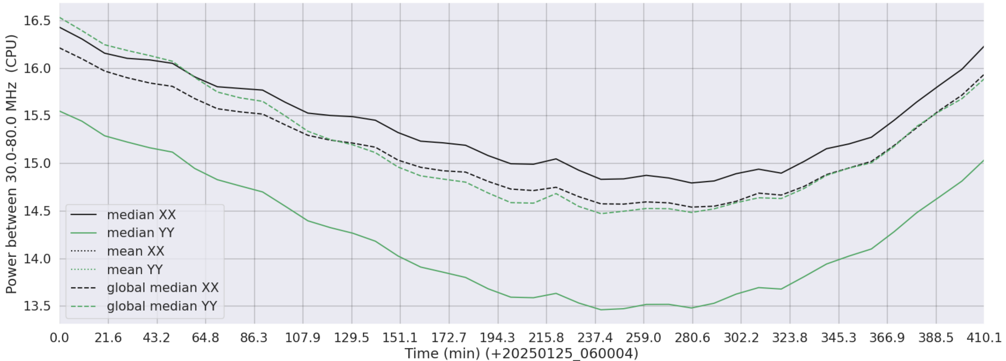
LWA022 - Correlator# 104 - XX FLAGS:Good - YY FLAGS:Good
