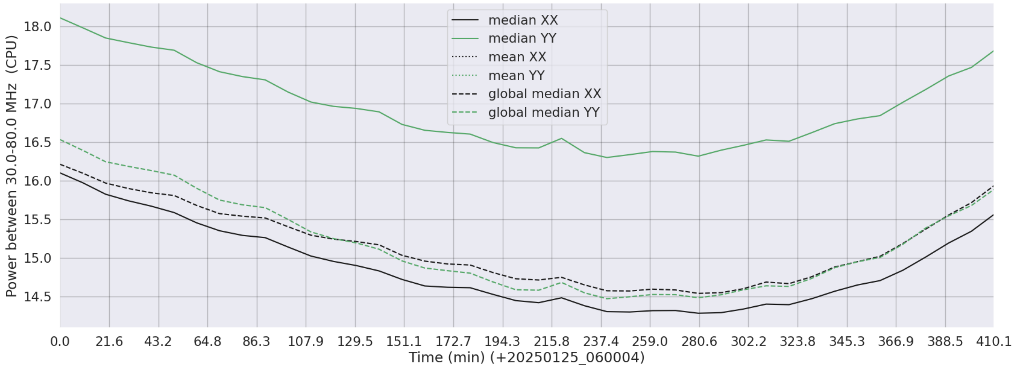
LWA344 - Correlator# 061 - XX FLAGS:Good - YY FLAGS:Good
