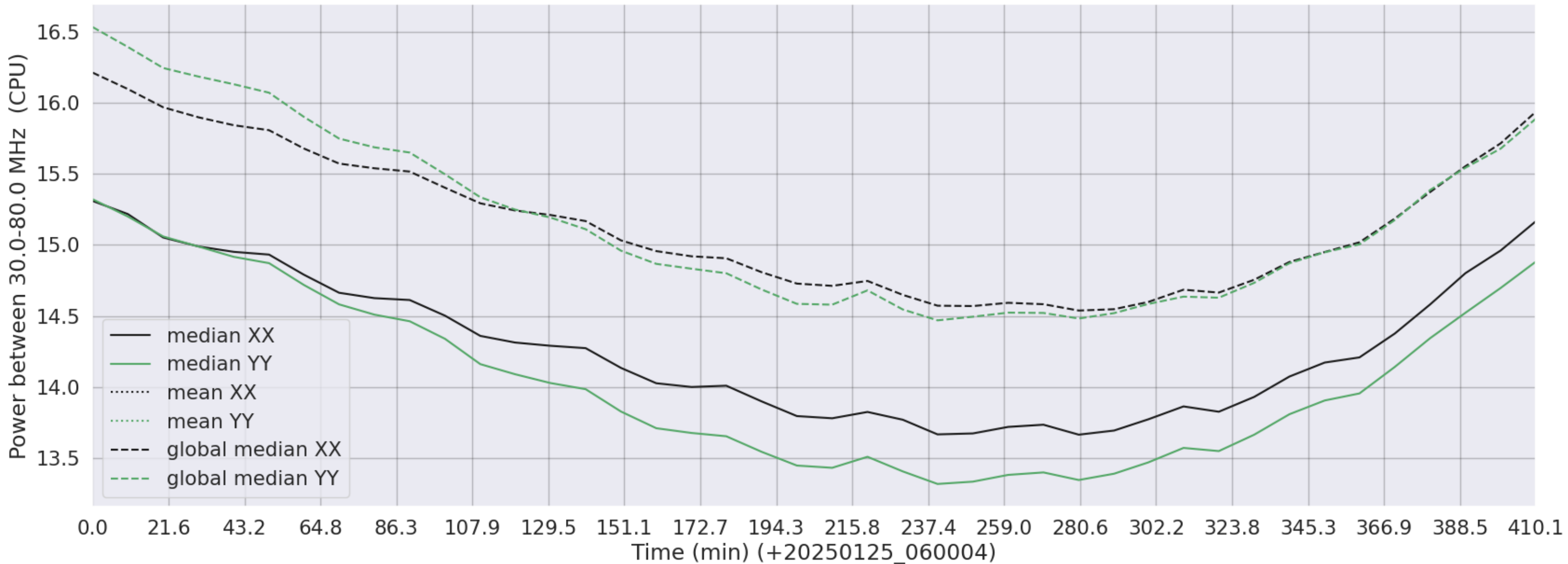
LWA251 - Correlator# 344 - XX FLAGS:Good - YY FLAGS:Good
