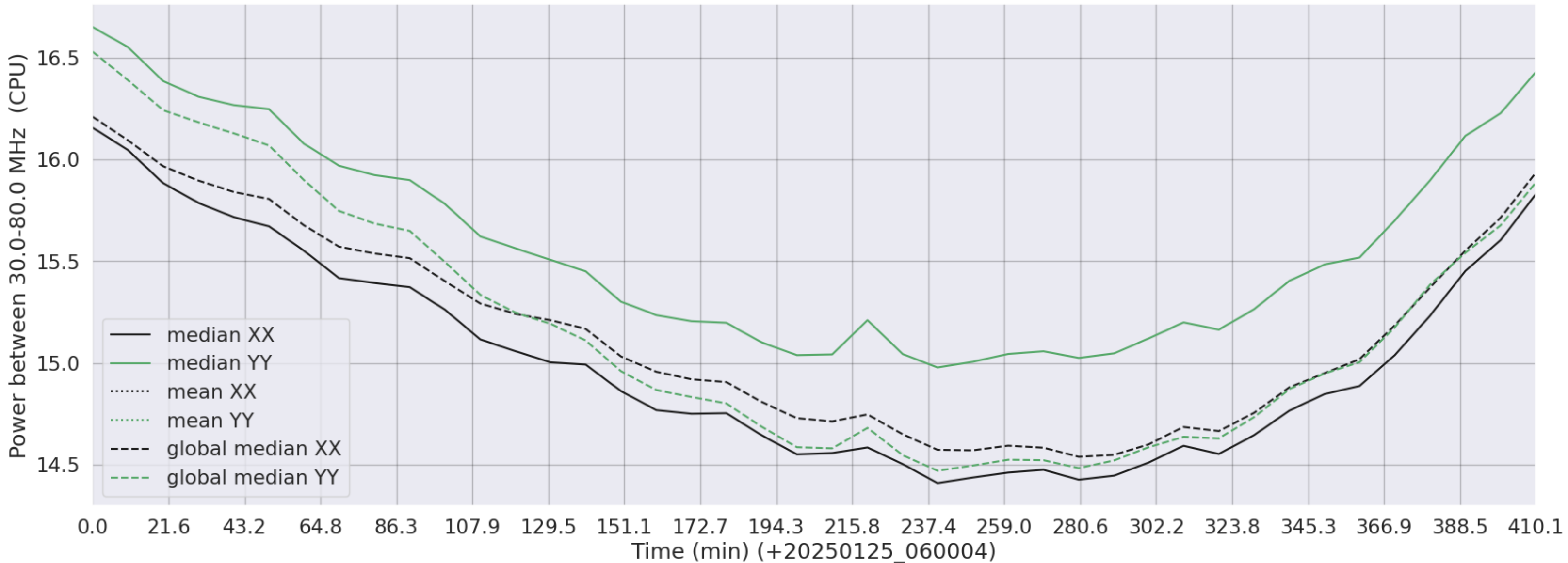
LWA257 - Correlator# 032 - XX FLAGS:Good - YY FLAGS:Good
