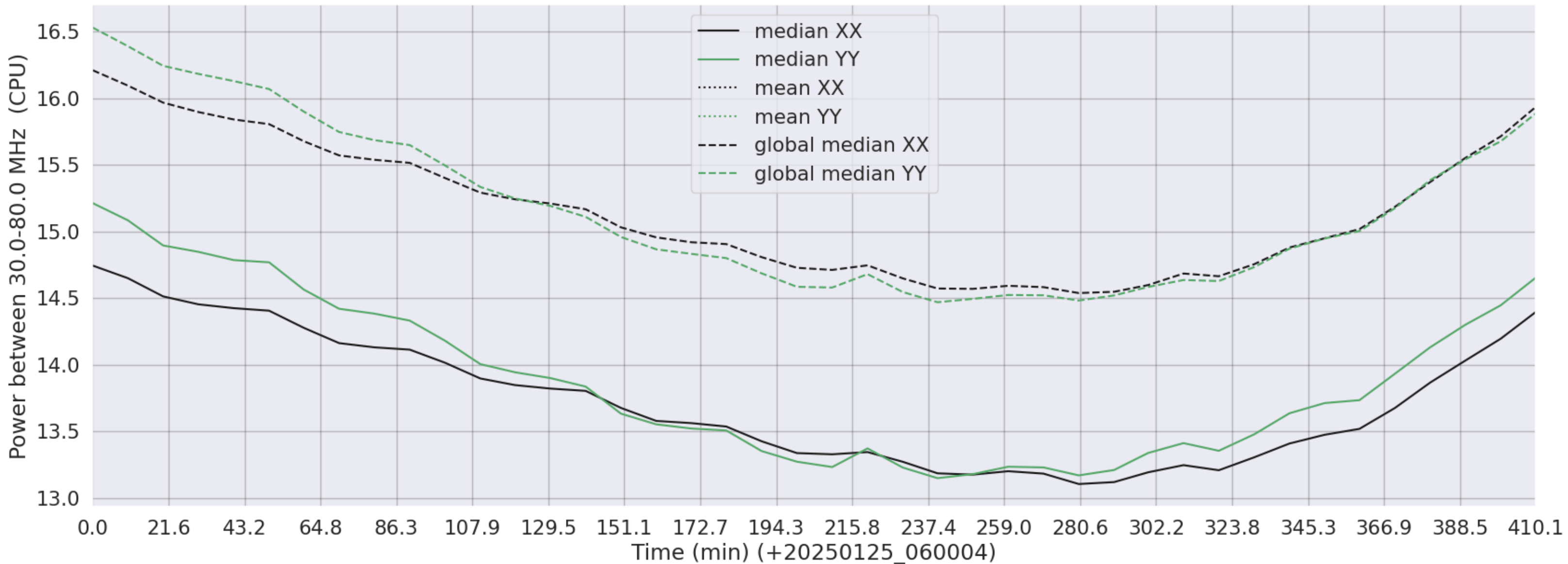
LWA127 - Correlator# 225 - XX FLAGS:Good - YY FLAGS:Good
