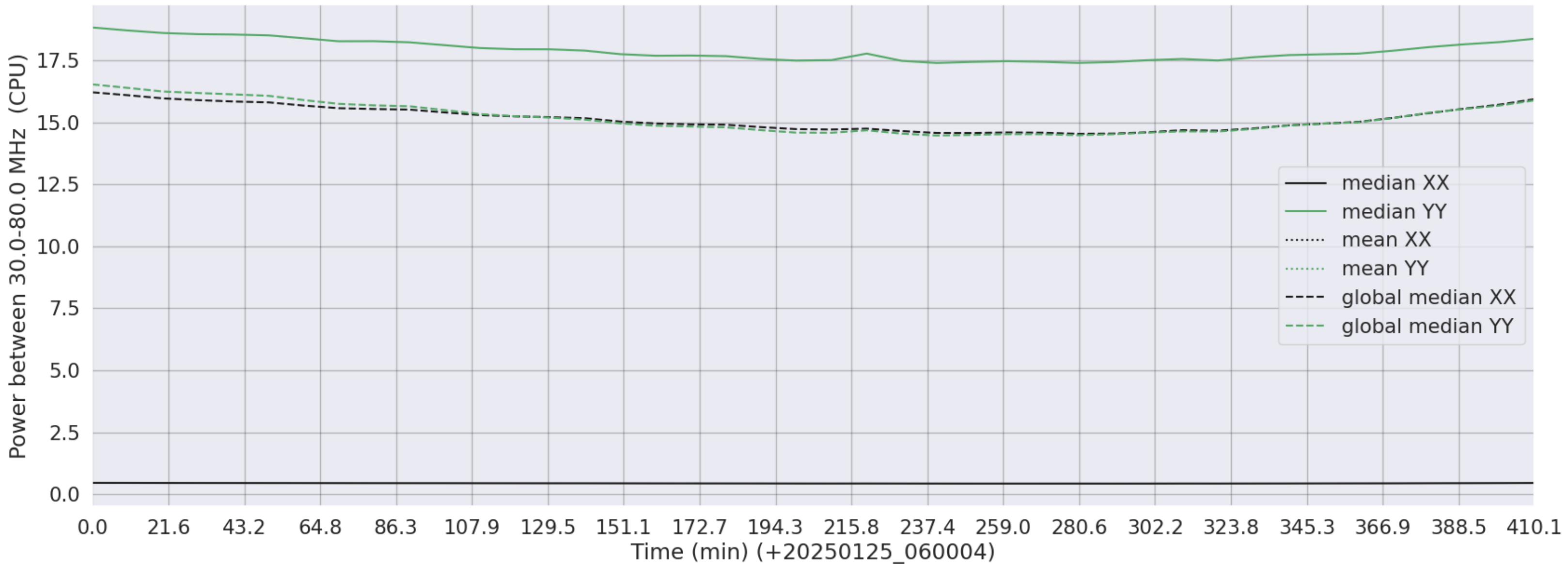
LWA069 - Correlator# 169 - XX FLAGS:LowPower - YY FLAGS:Good
