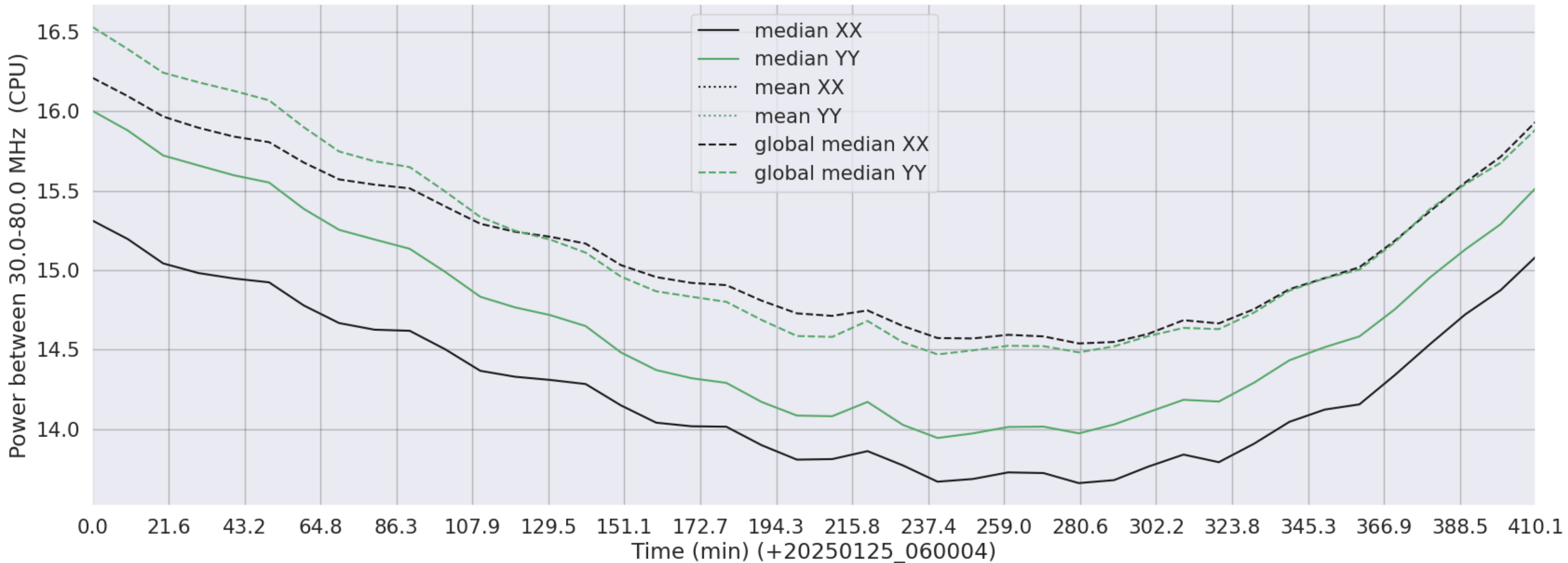
LWA214 - Correlator# 328 - XX FLAGS:Good - YY FLAGS:Good
