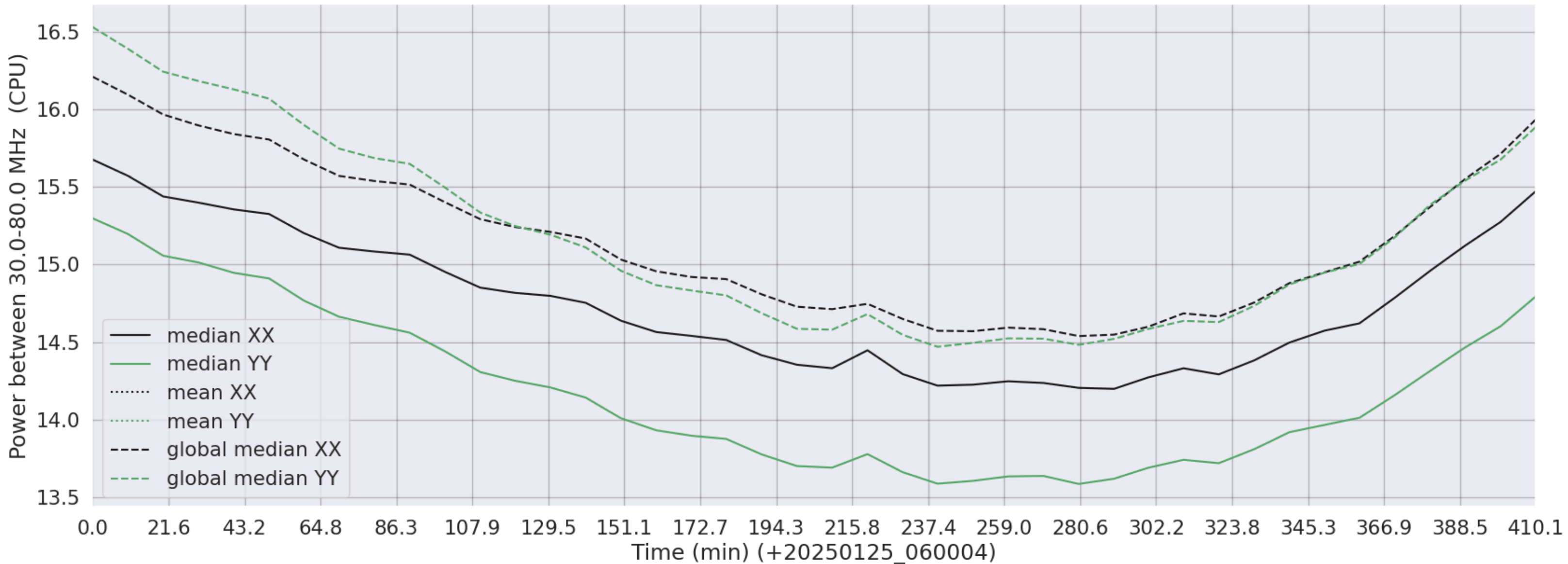
LWA143 - Correlator# 210 - XX FLAGS:Good - YY FLAGS:Good
