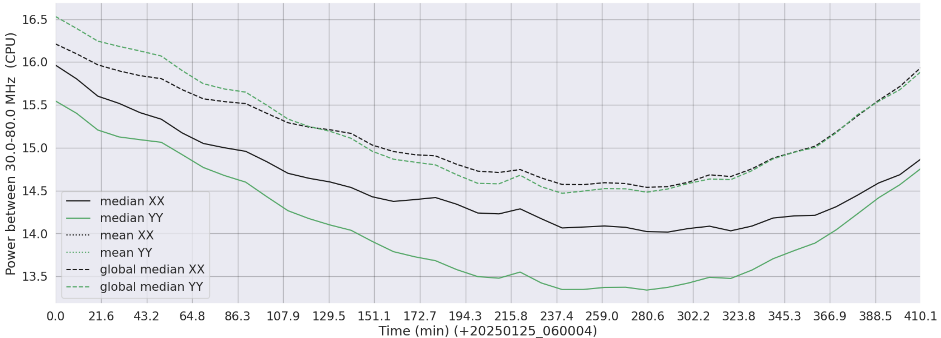
LWA285 - Correlator# 013 - XX FLAGS:Good - YY FLAGS:Good
