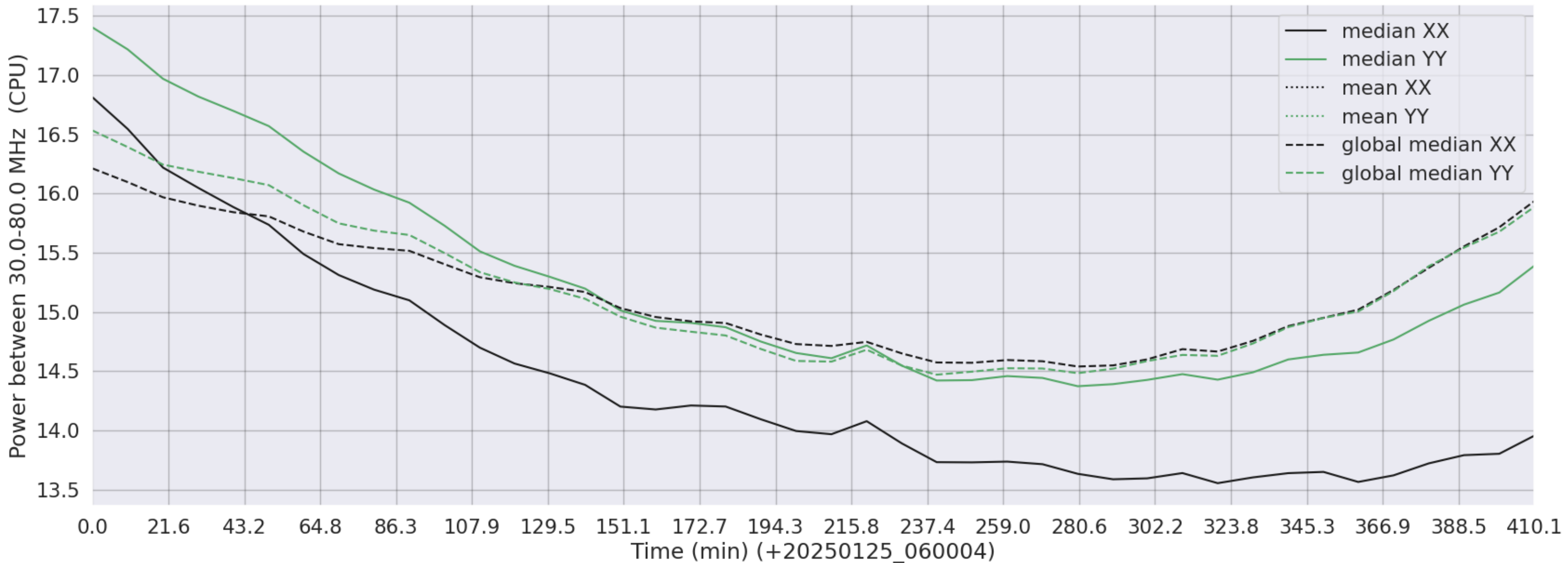
LWA313 - Correlator# 018 - XX FLAGS:Good - YY FLAGS:Good
