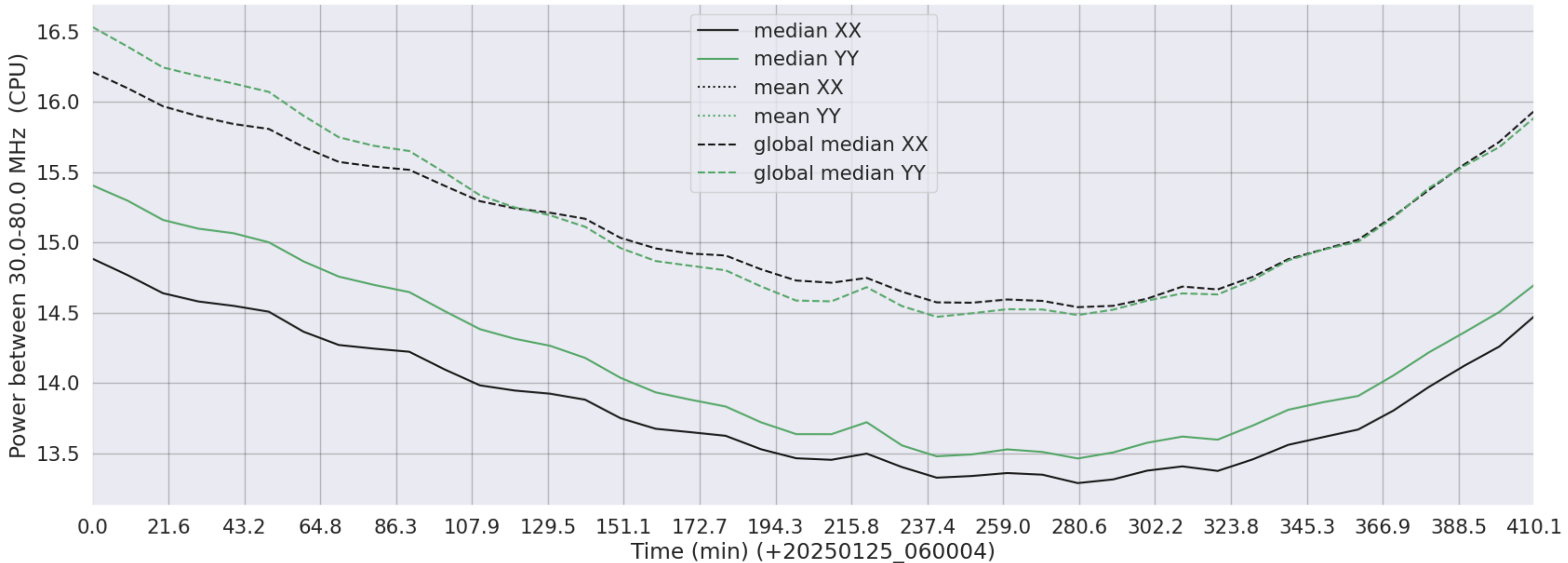
LWA021 - Correlator# 105 - XX FLAGS:Good - YY FLAGS:Good
