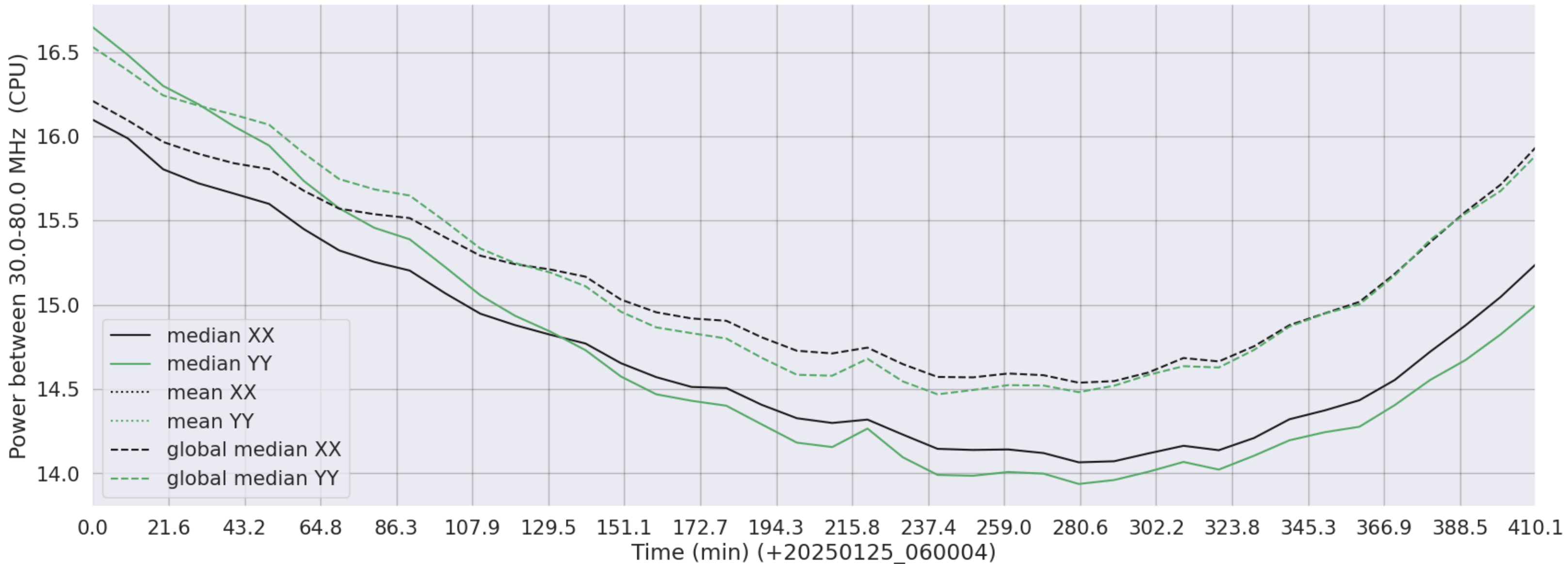
LWA262 - Correlator# 123 - XX FLAGS:Good - YY FLAGS:Good
