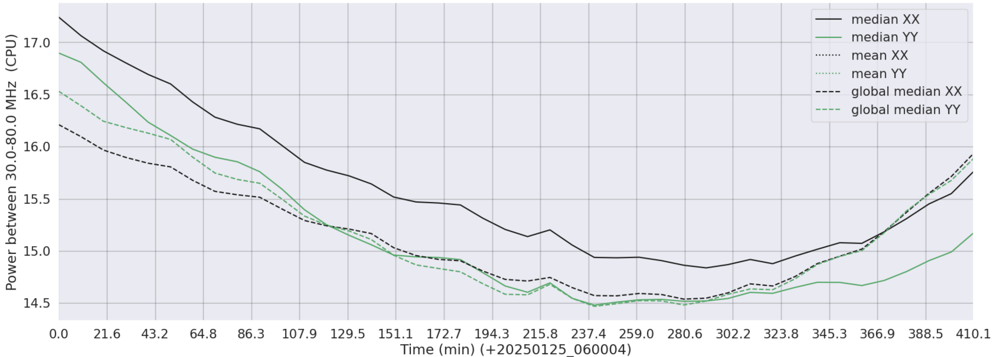
LWA297 - Correlator# 314 - XX FLAGS:Good - YY FLAGS:Good
