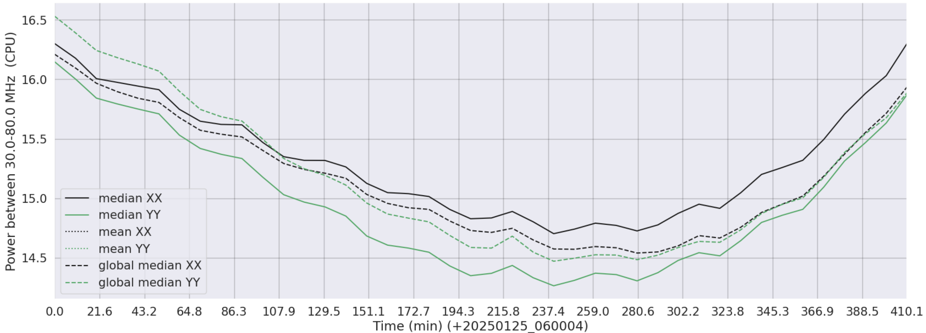
LWA080 - Correlator# 119 - XX FLAGS:Good - YY FLAGS:Good
