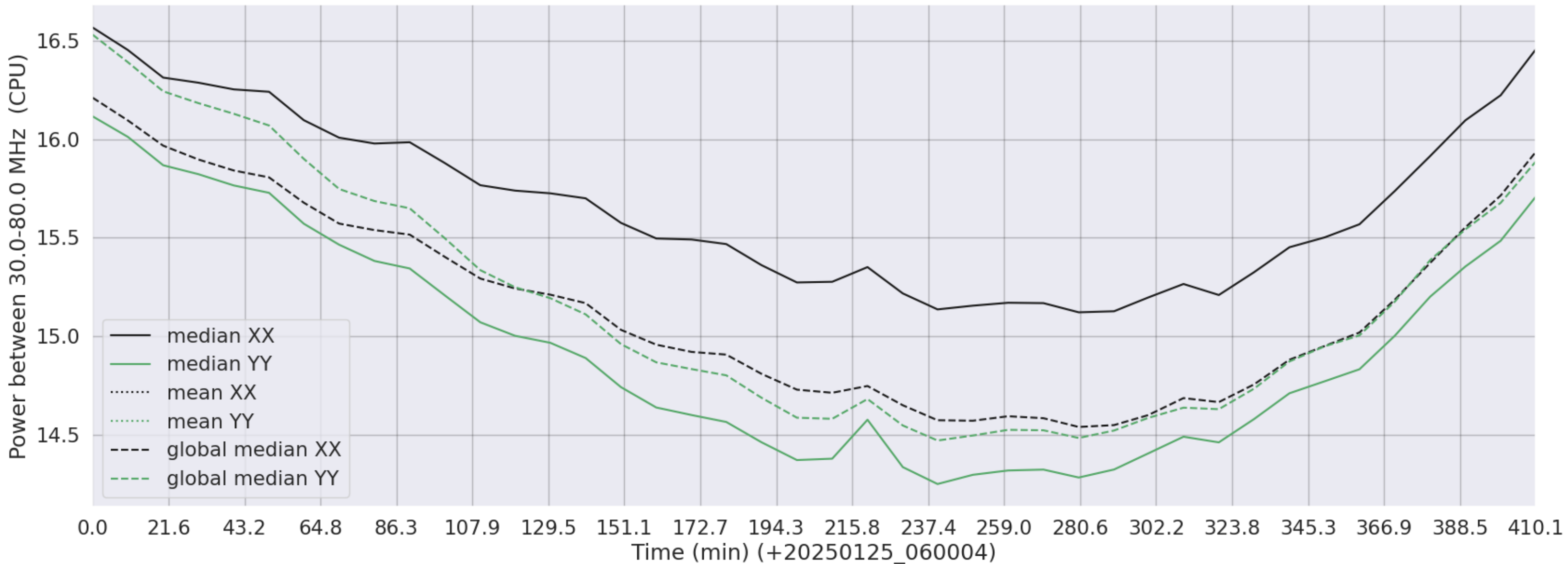
LWA008 - Correlator# 075 - XX FLAGS:Good - YY FLAGS:Good
