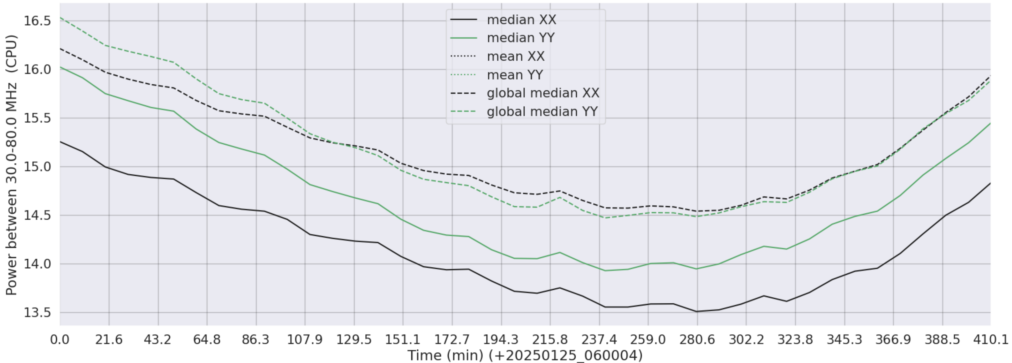
LWA026 - Correlator# 108 - XX FLAGS:Good - YY FLAGS:Good
