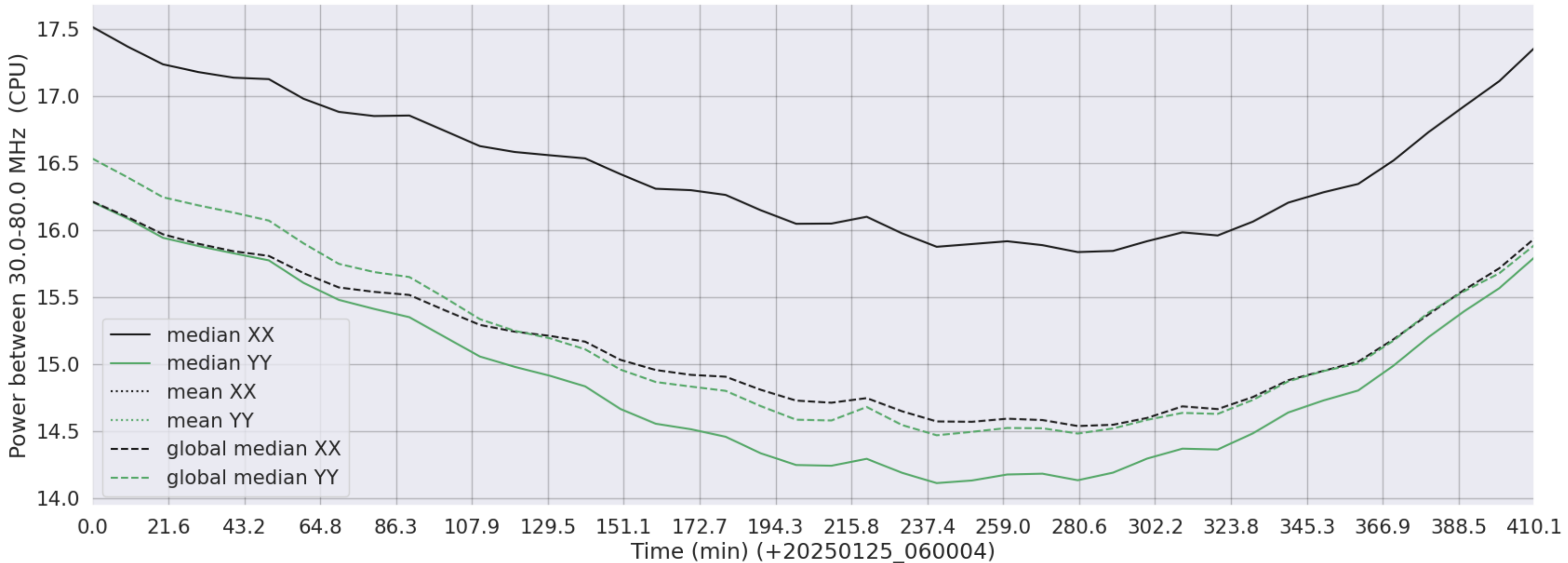
LWA150 - Correlator# 215 - XX FLAGS:Good - YY FLAGS:Good
