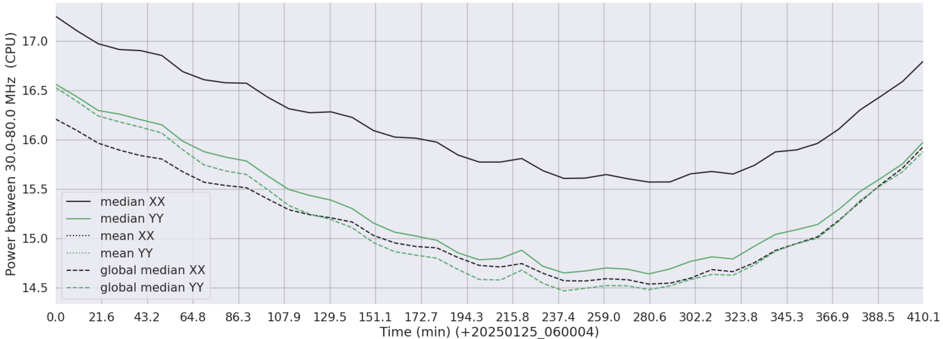
LWA013 - Correlator# 096 - XX FLAGS:Good - YY FLAGS:Good
