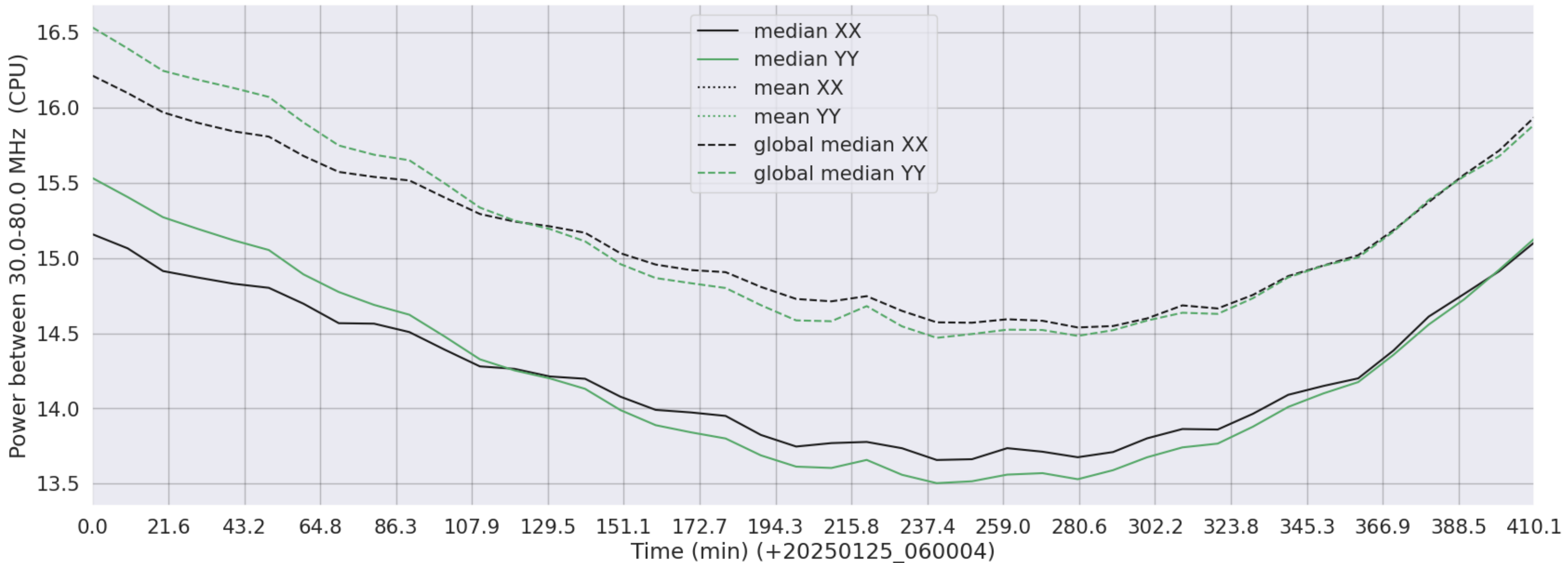
LWA159 - Correlator# 236 - XX FLAGS:Good - YY FLAGS:Good
