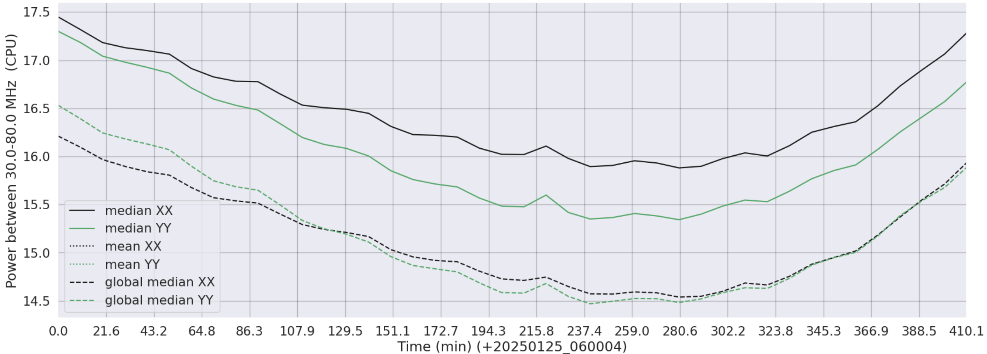
LWA204 - Correlator# 294 - XX FLAGS:Good - YY FLAGS:Good
