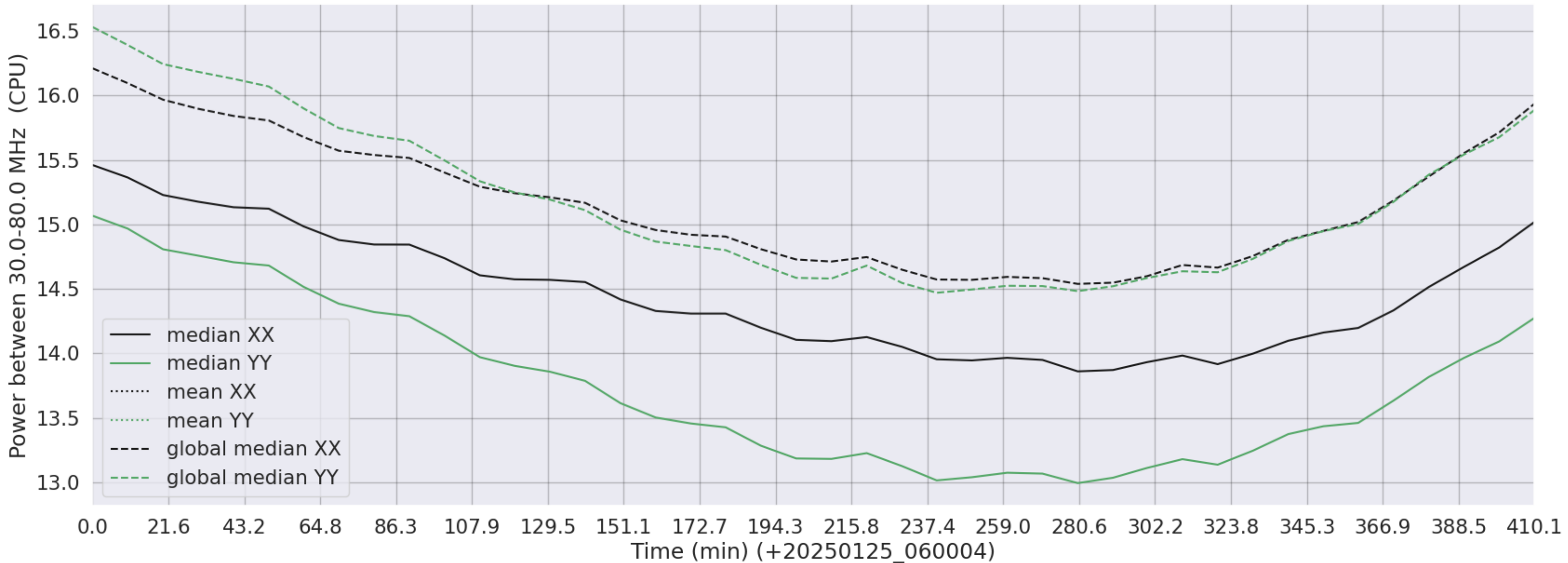
LWA027 - Correlator# 111 - XX FLAGS:Good - YY FLAGS:Good
