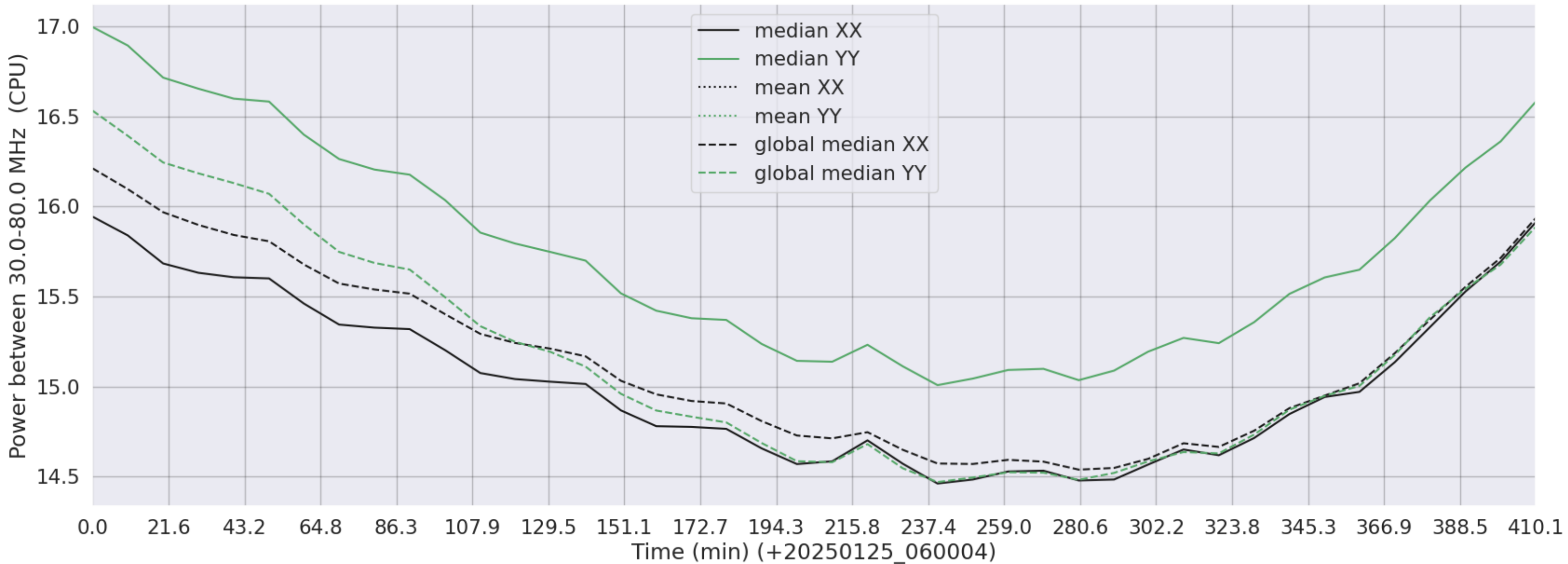
LWA210 - Correlator# 300 - XX FLAGS:Good - YY FLAGS:Good
