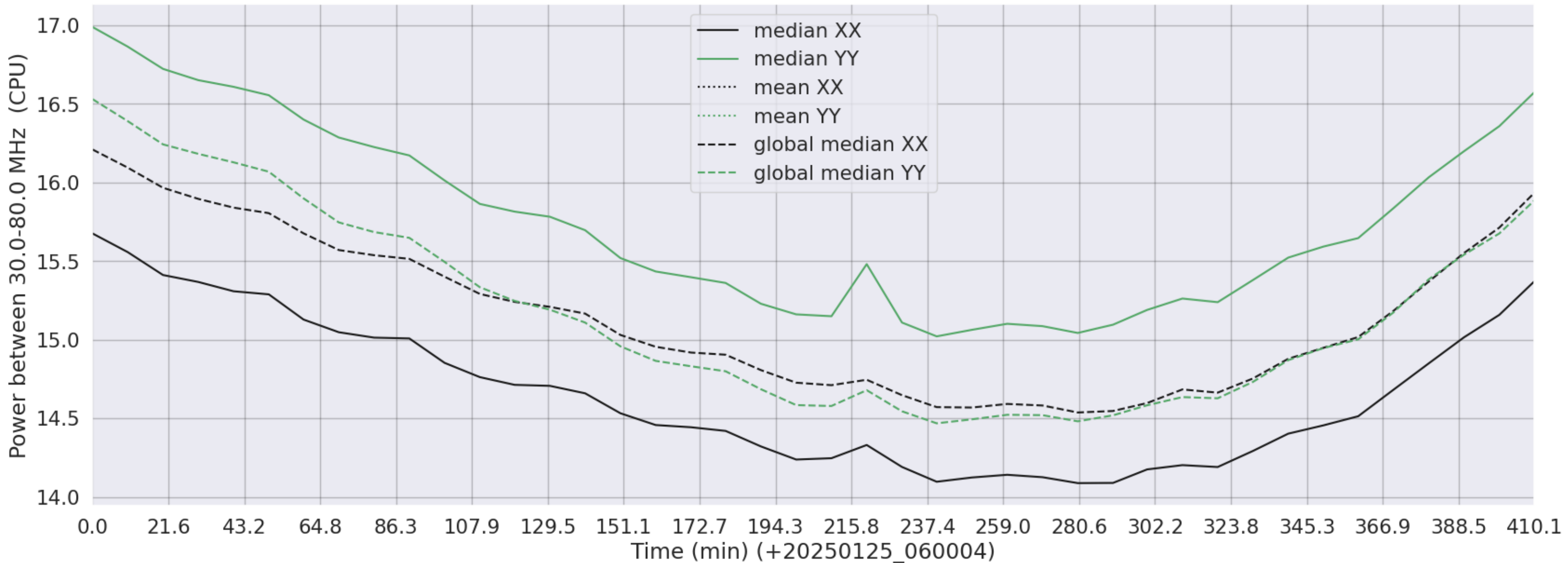
LWA200 - Correlator# 276 - XX FLAGS:Good - YY FLAGS:Good
