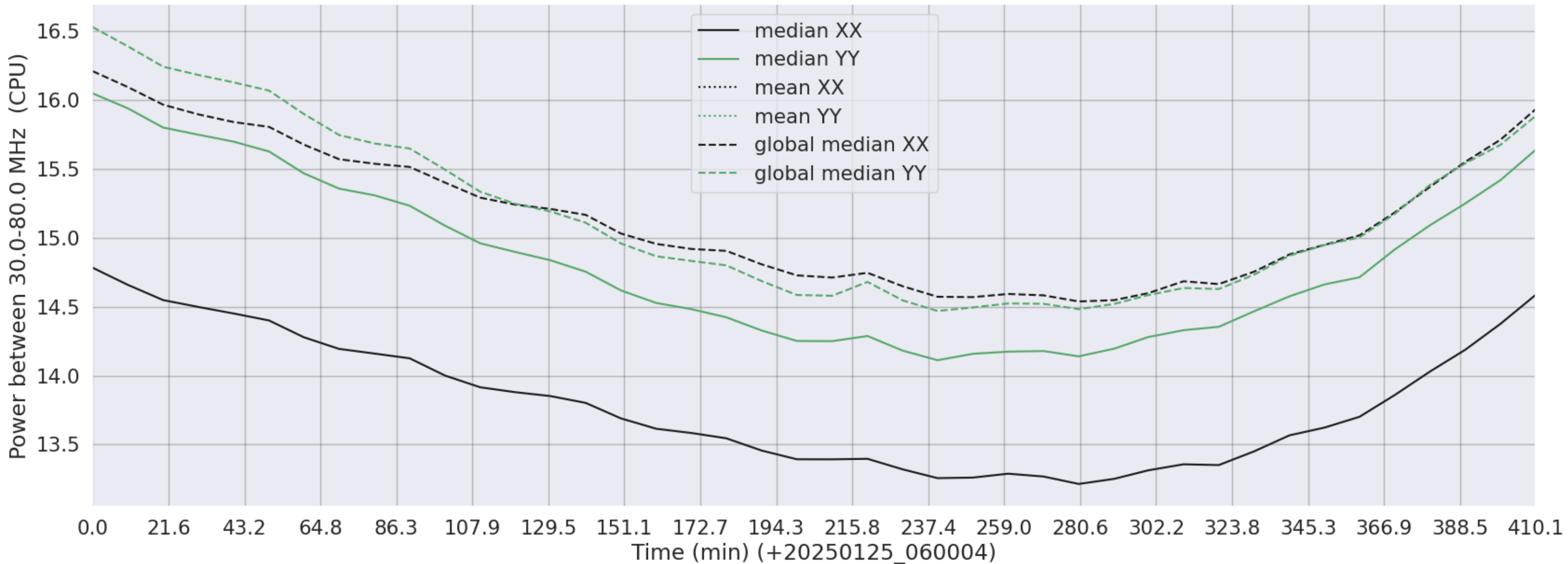
LWA211 - Correlator# 327 - XX FLAGS:Good - YY FLAGS:Good
