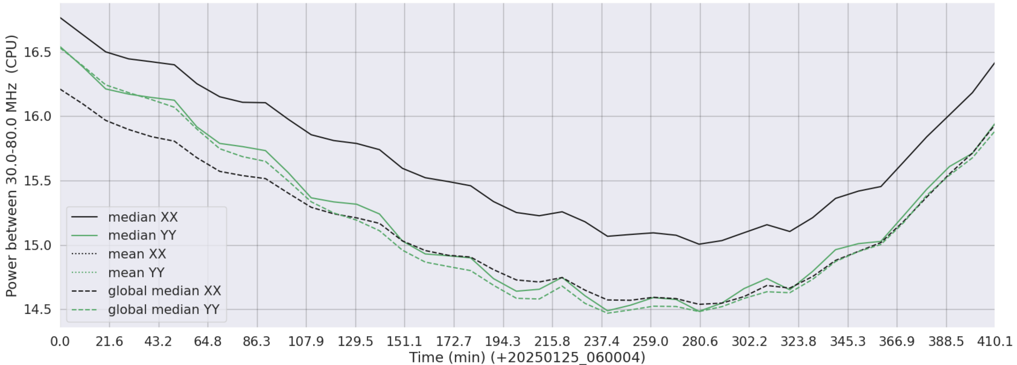
LWA149 - Correlator# 216 - XX FLAGS:Good - YY FLAGS:Good
