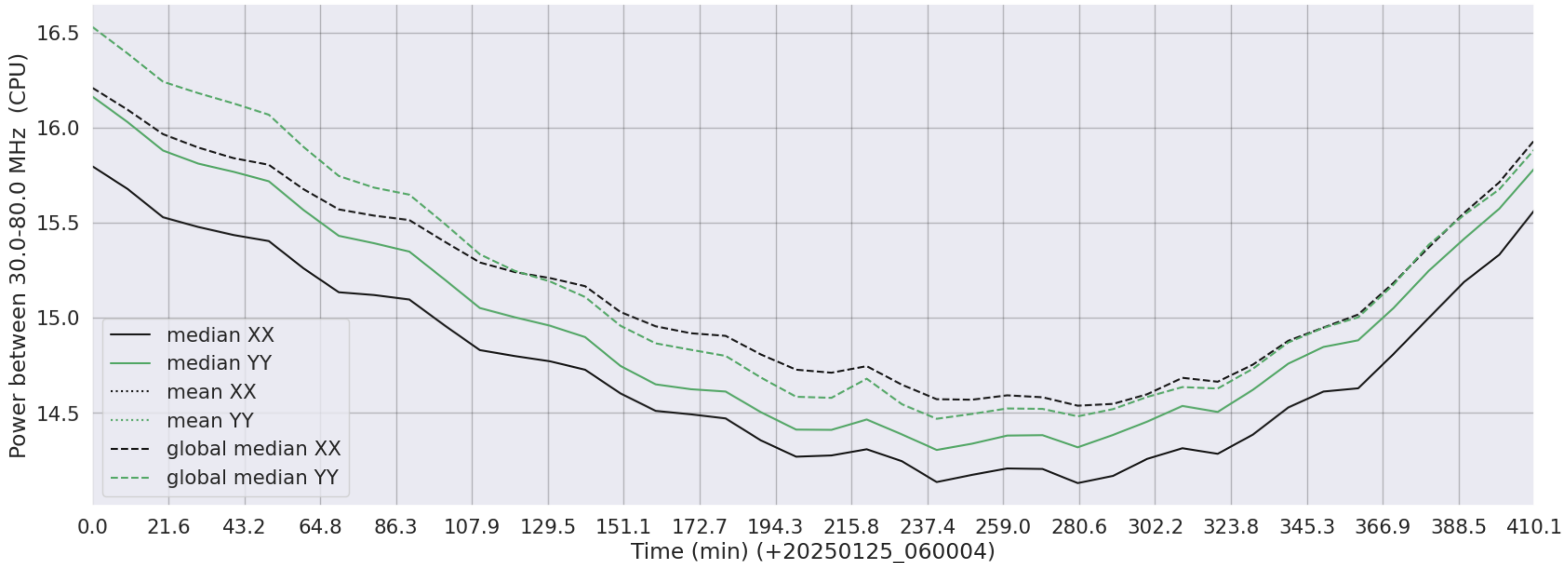
LWA084 - Correlator# 120 - XX FLAGS:Good - YY FLAGS:Good
