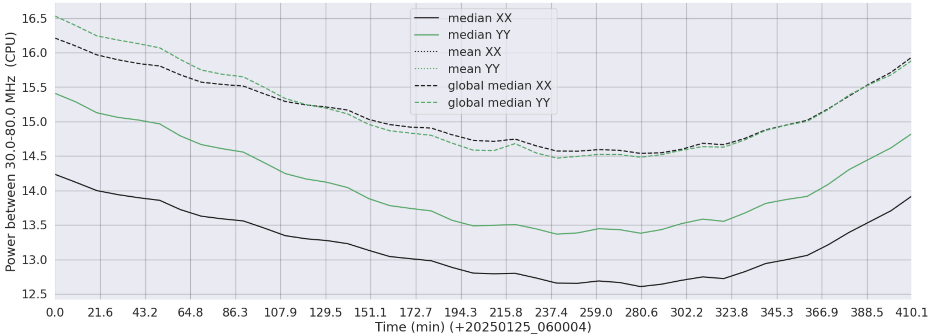
LWA060 - Correlator# 133 - XX FLAGS:Good - YY FLAGS:Good
