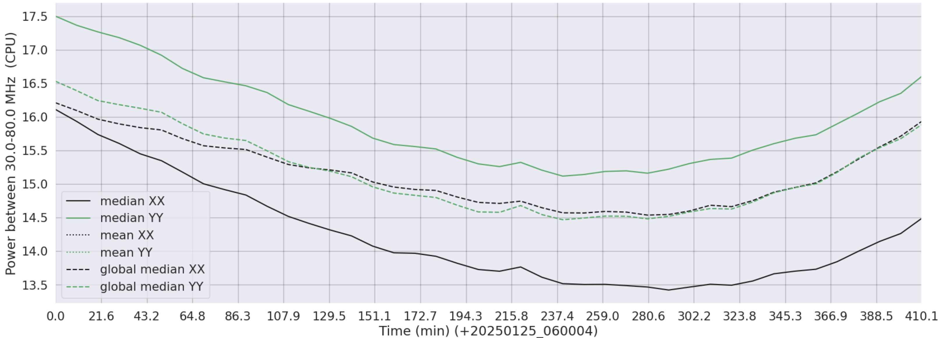
LWA314 - Correlator# 021 - XX FLAGS:Good - YY FLAGS:Good
