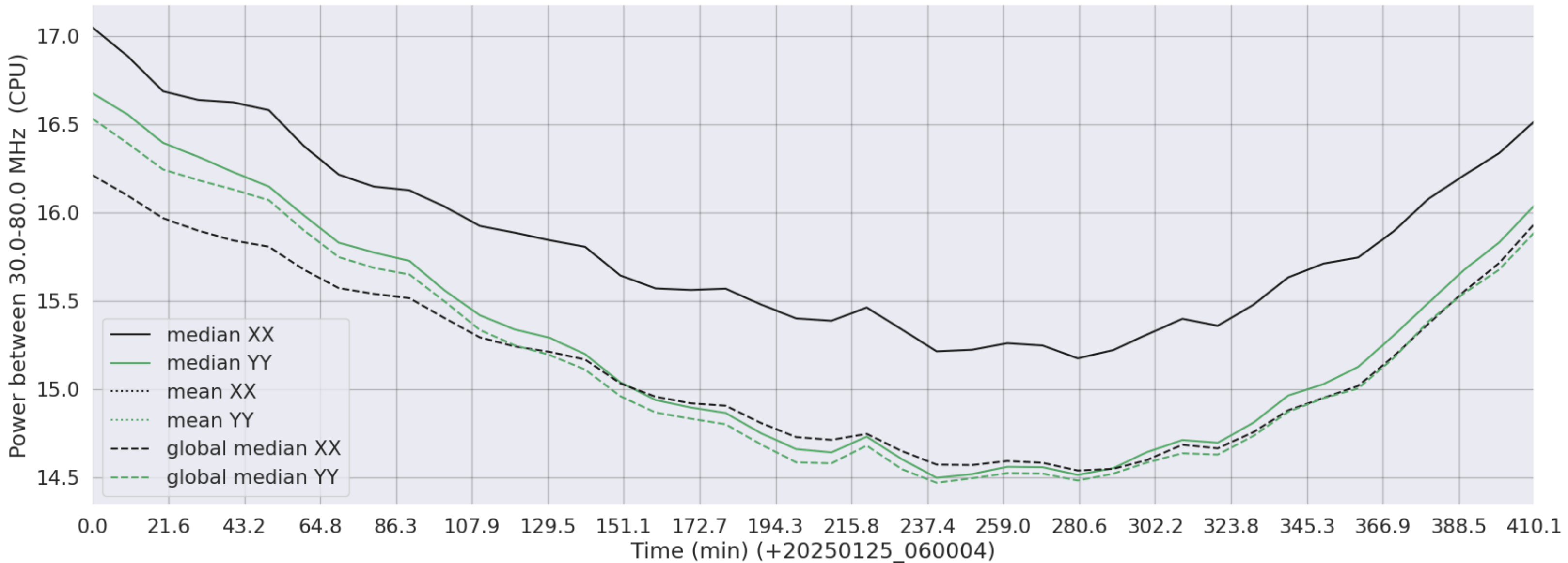
LWA324 - Correlator# 122 - XX FLAGS:Good - YY FLAGS:Good
