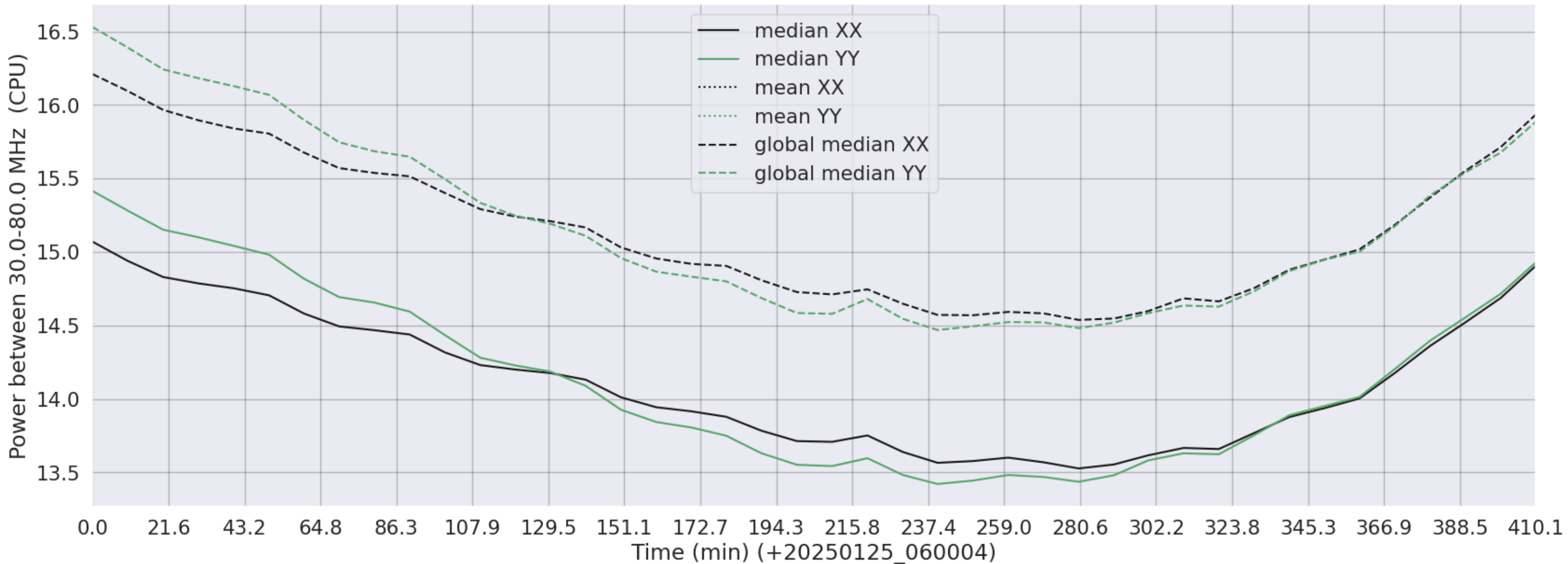
LWA212 - Correlator# 326 - XX FLAGS:Good - YY FLAGS:Good
