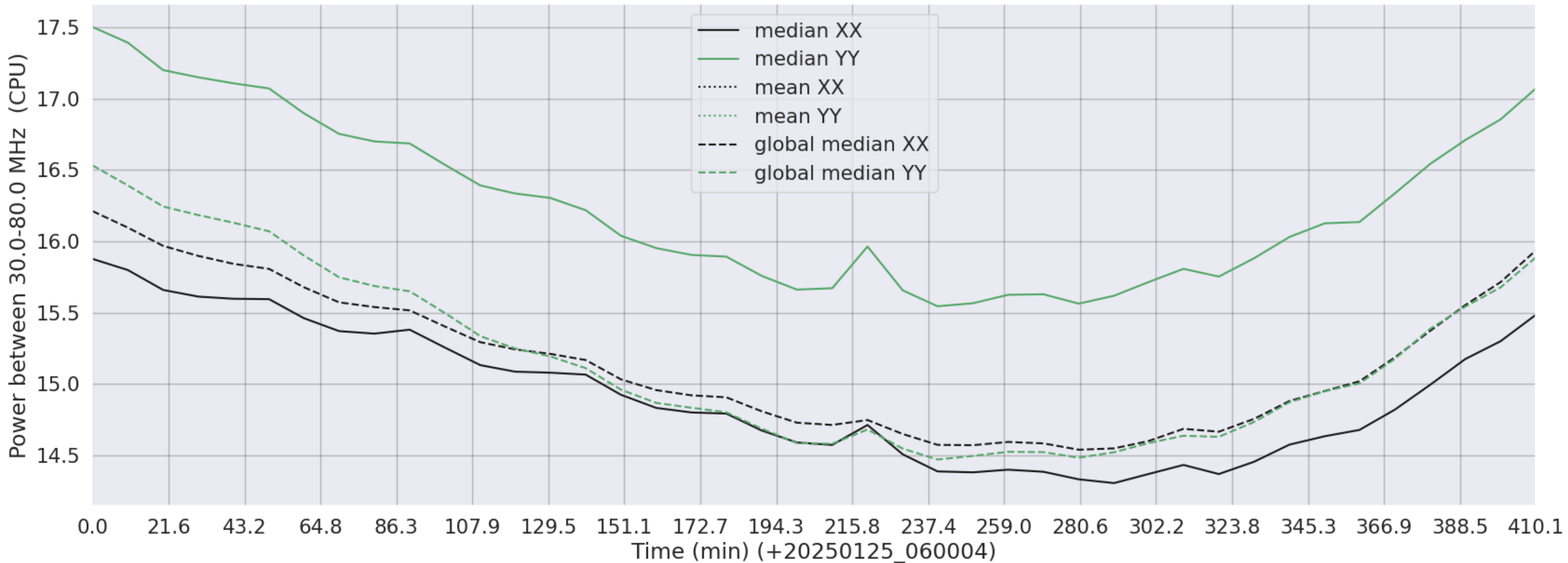
LWA070 - Correlator# 168 - XX FLAGS:Good - YY FLAGS:Good
