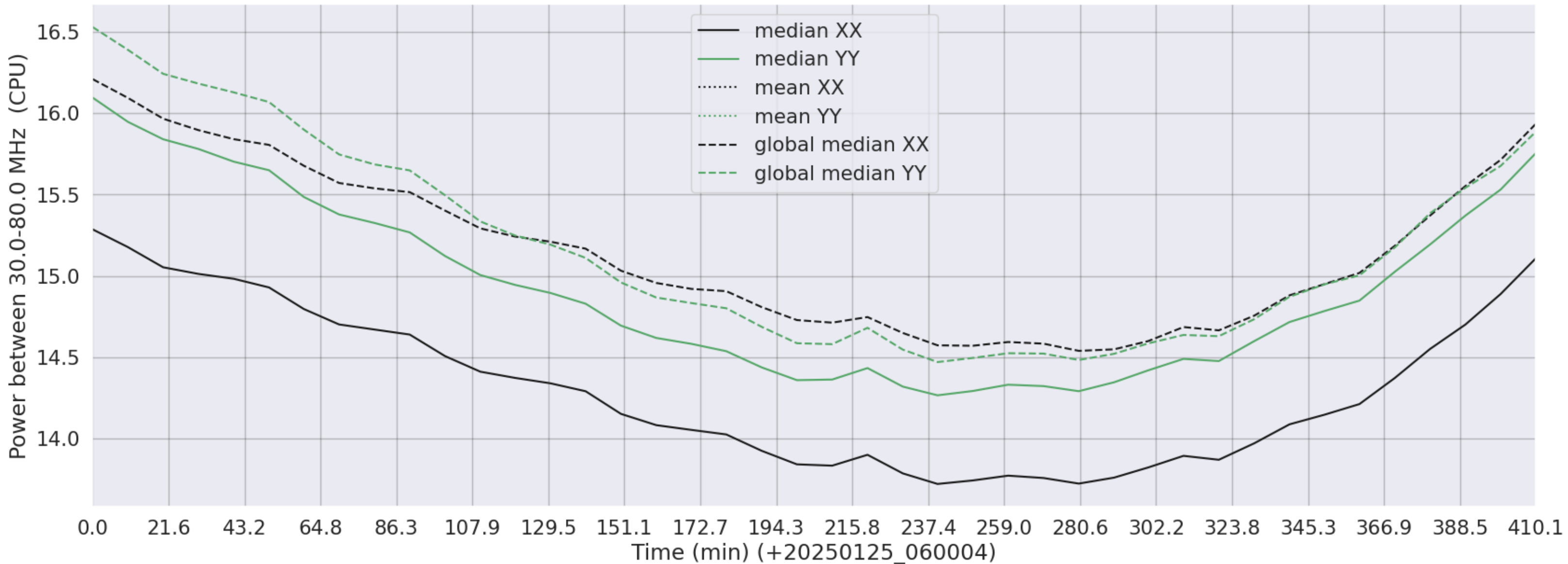
LWA079 - Correlator# 195 - XX FLAGS:Good - YY FLAGS:Good
