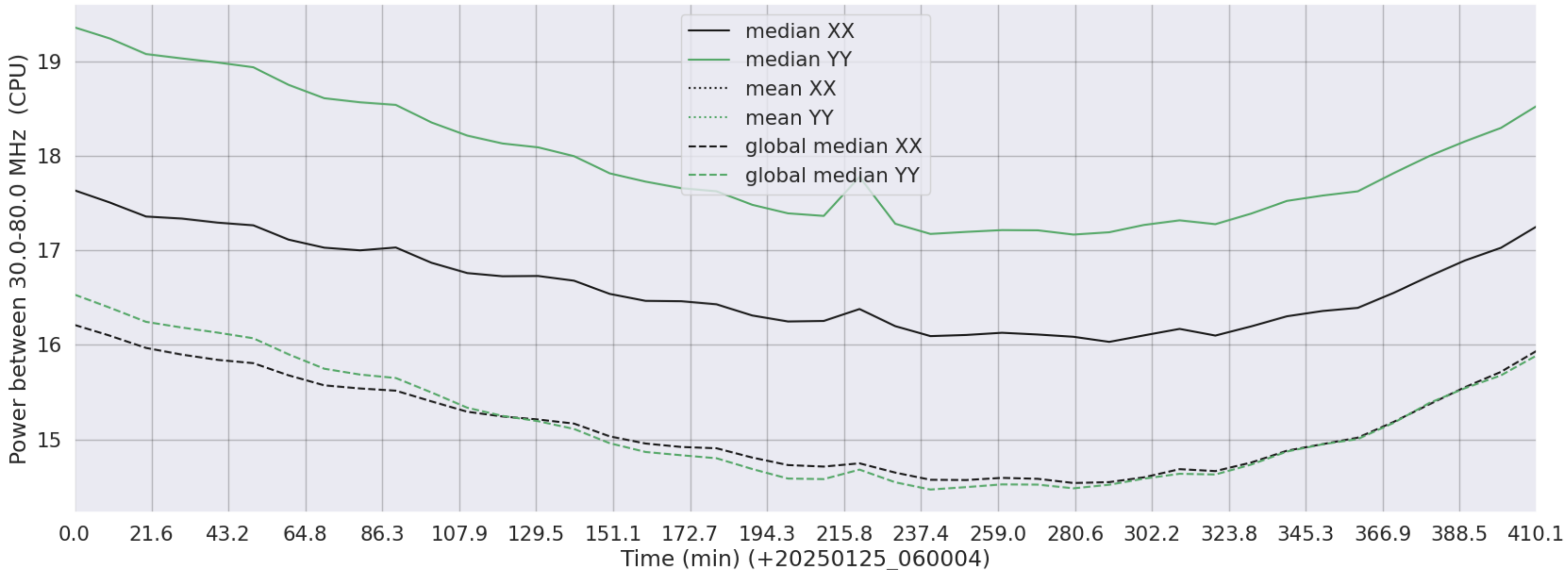
LWA003 - Correlator# 067 - XX FLAGS:Good - YY FLAGS:Good
