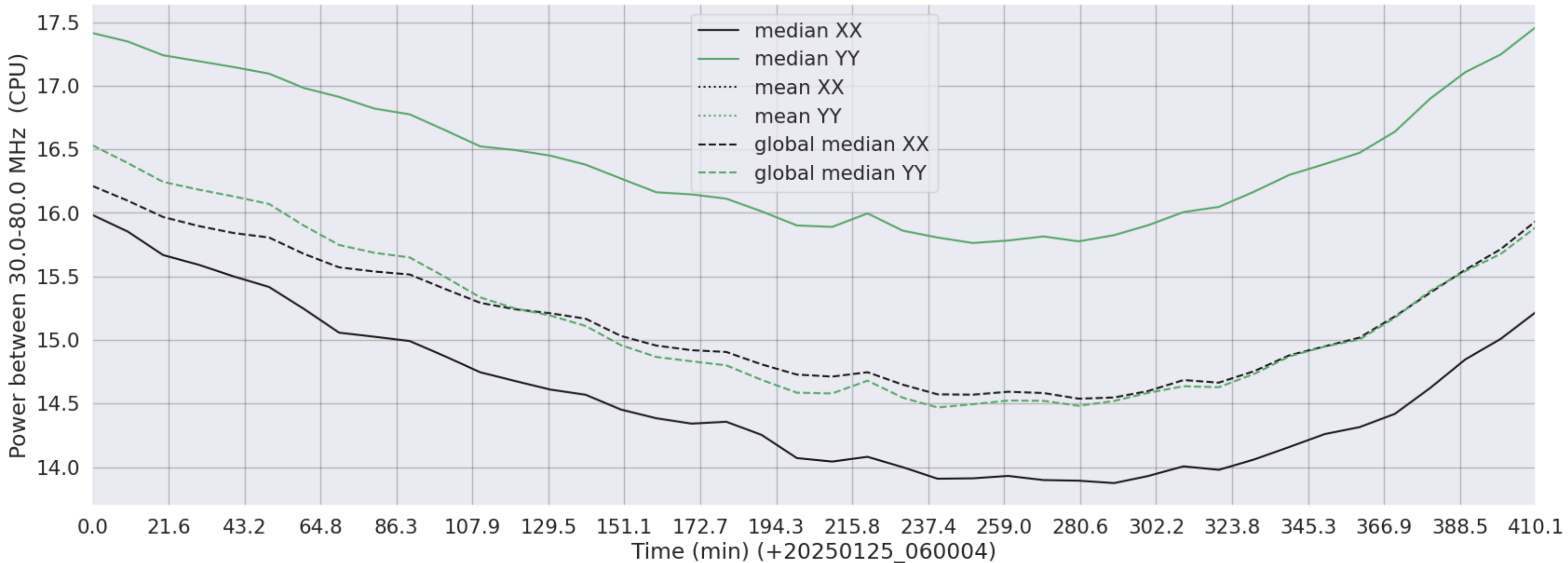
LWA364 - Correlator# 127 - XX FLAGS:Good - YY FLAGS:Good
