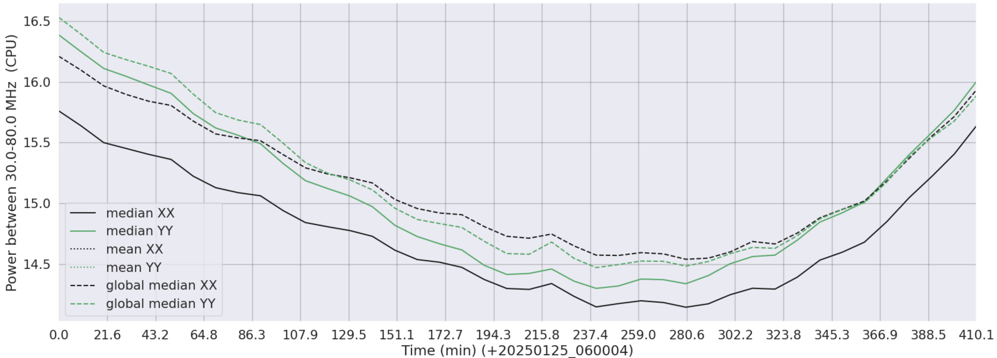
LWA024 - Correlator# 106 - XX FLAGS:Good - YY FLAGS:Good
