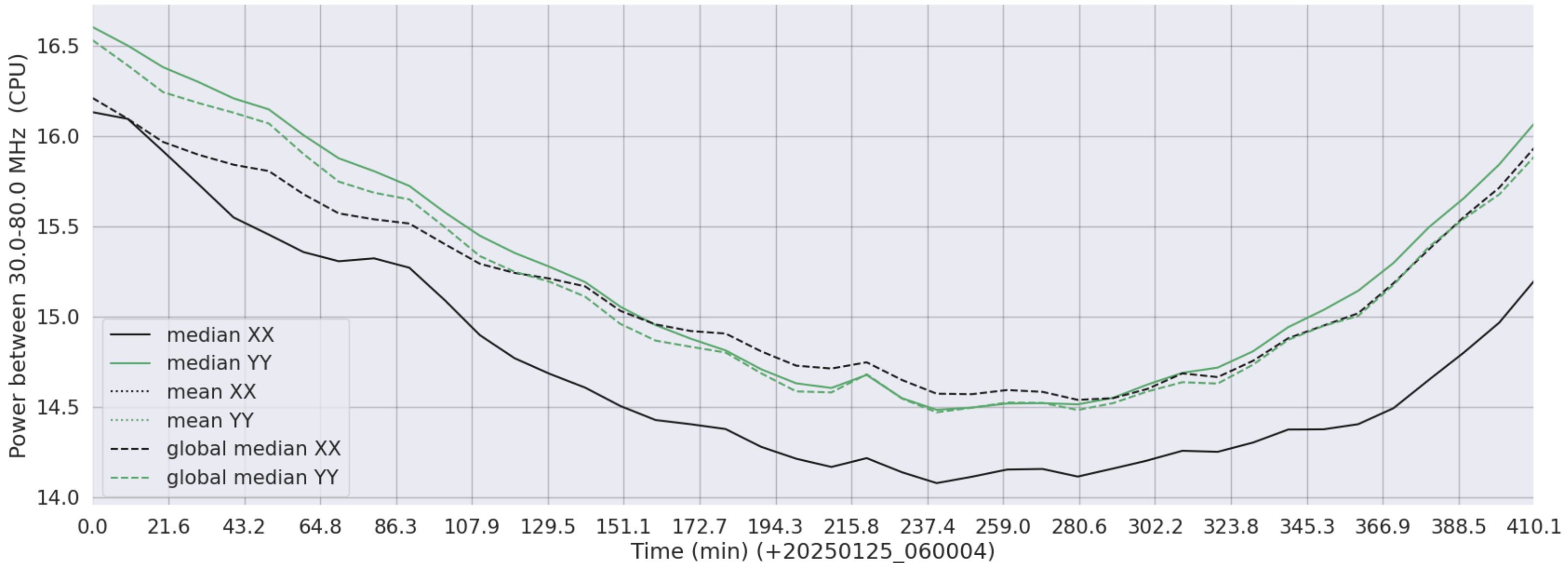
LWA346 - Correlator# 316 - XX FLAGS:Good - YY FLAGS:Good
