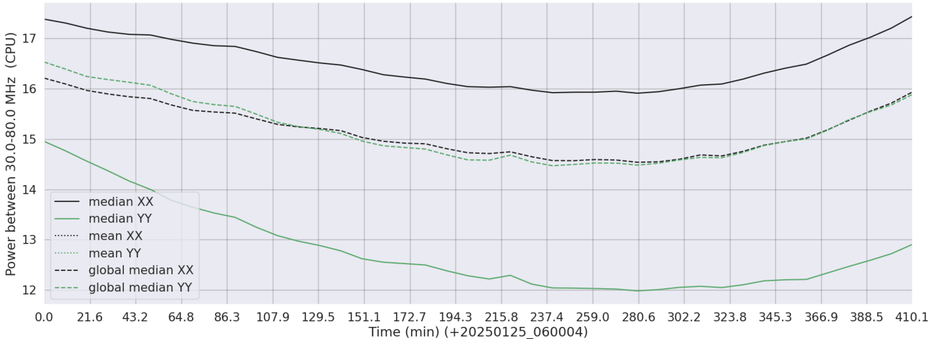
LWA347 - Correlator# 255 - XX FLAGS:Good - YY FLAGS:Good
