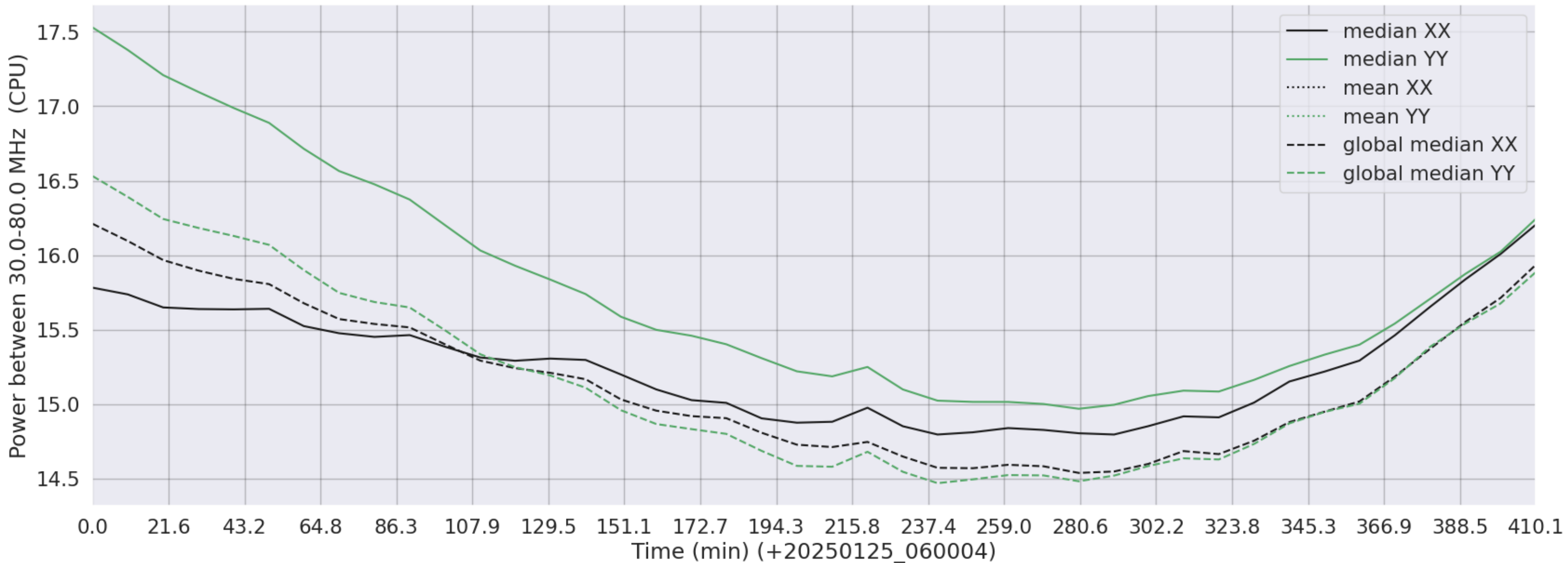
LWA306 - Correlator# 053 - XX FLAGS:Good - YY FLAGS:Good
