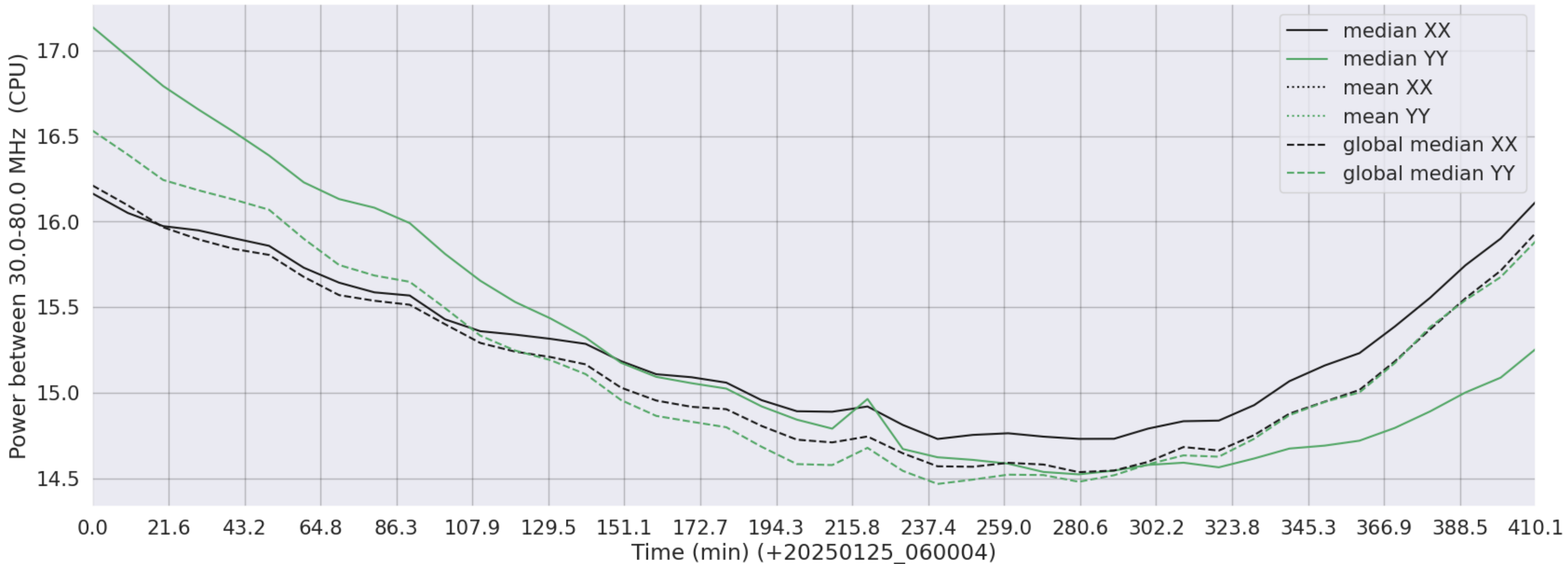
LWA290 - Correlator# 285 - XX FLAGS:Good - YY FLAGS:Good
