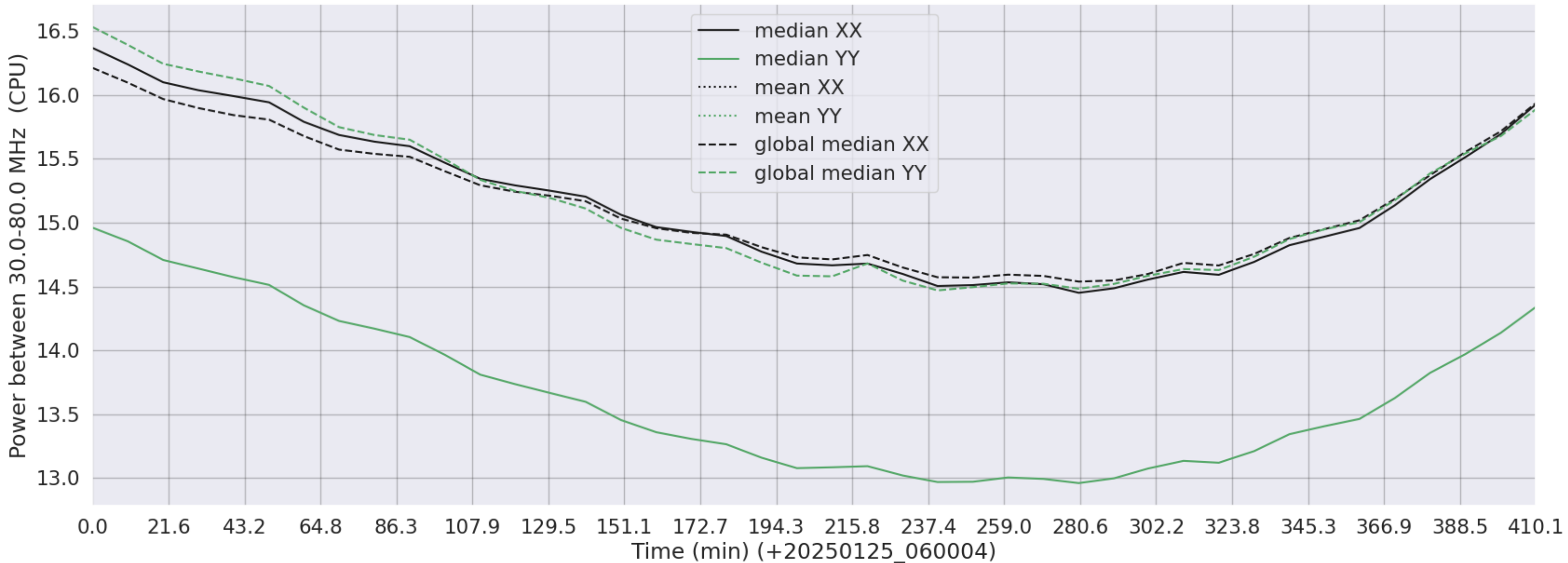
LWA059 - Correlator# 136 - XX FLAGS:Good - YY FLAGS:Good
