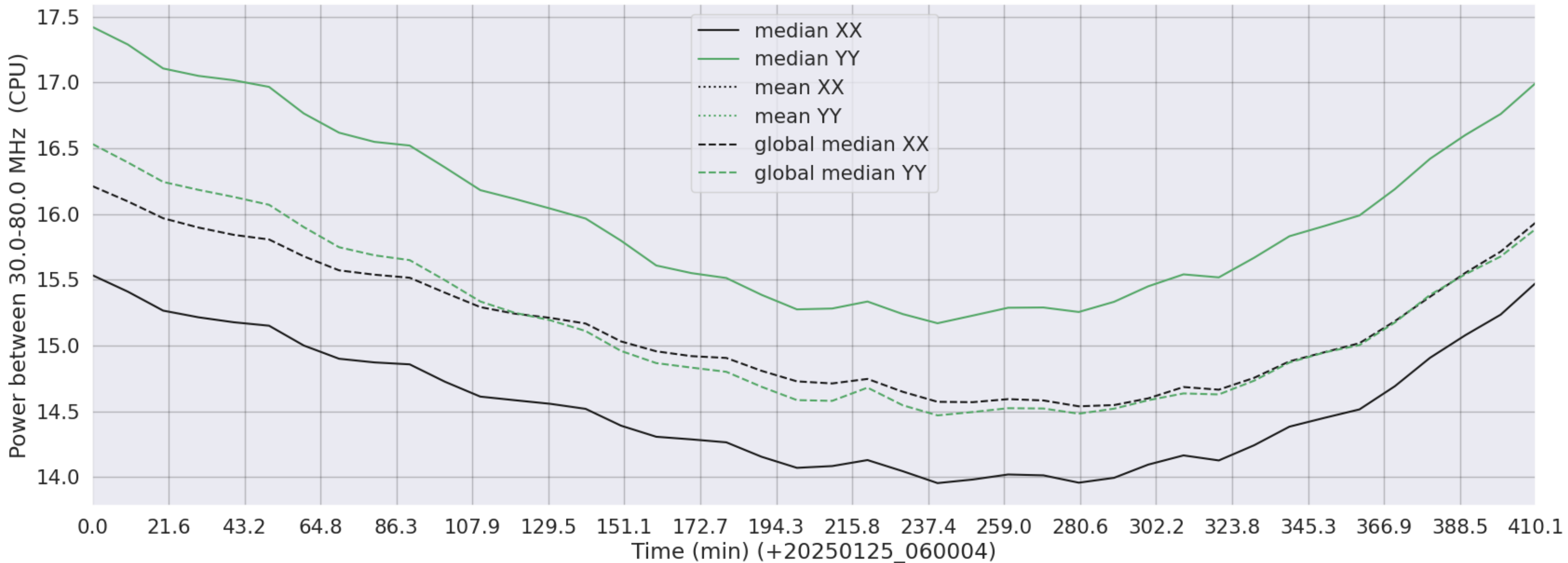
LWA046 - Correlator# 082 - XX FLAGS:Good - YY FLAGS:Good
