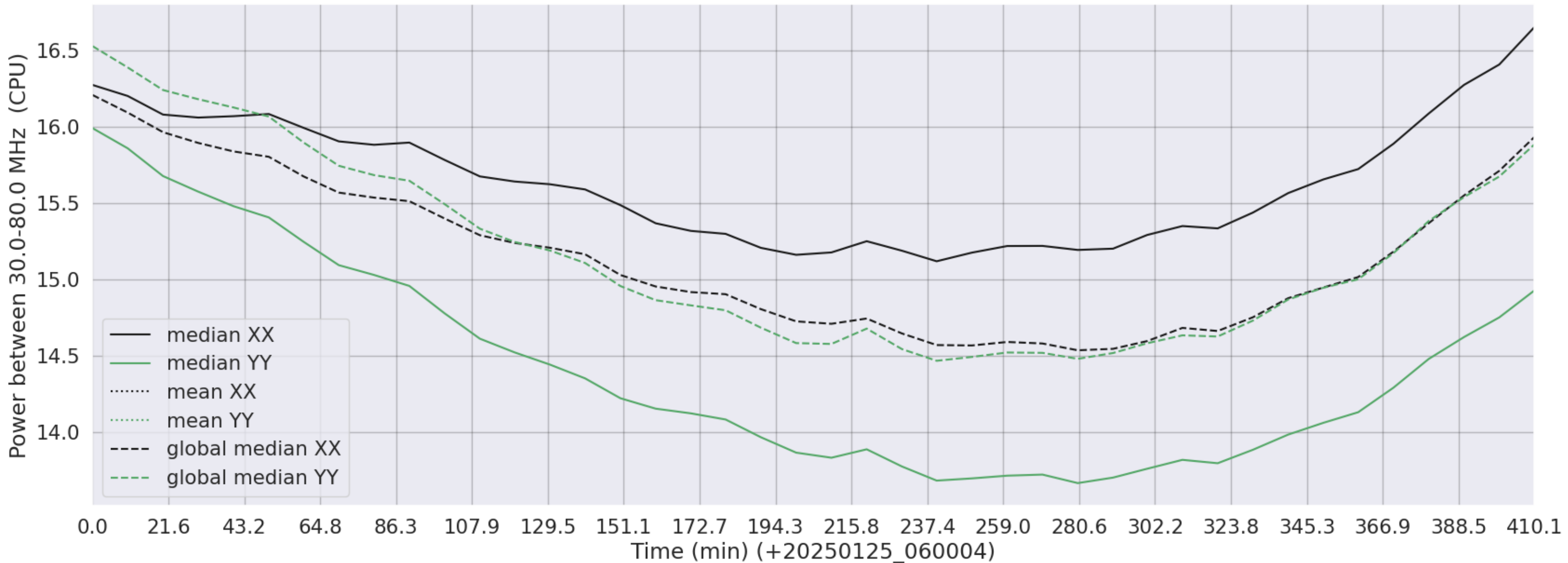
LWA353 - Correlator# 031 - XX FLAGS:Good - YY FLAGS:Good
