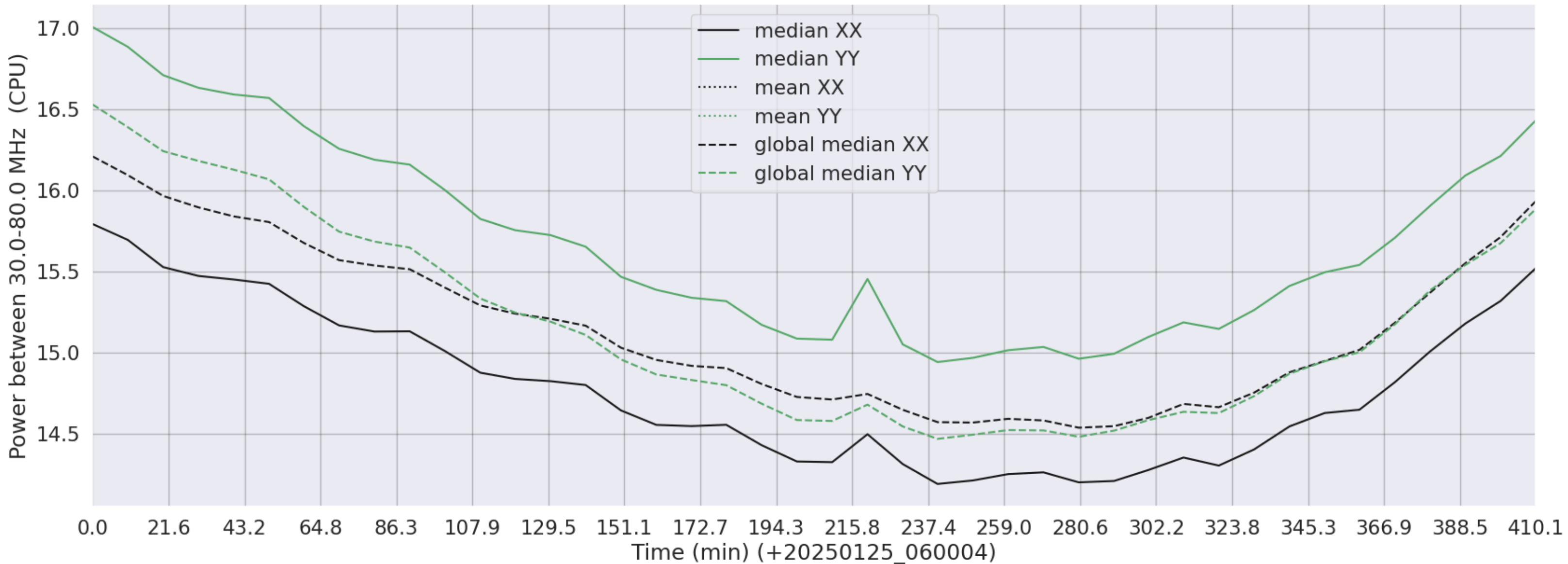
LWA201 - Correlator# 279 - XX FLAGS:Good - YY FLAGS:Good
