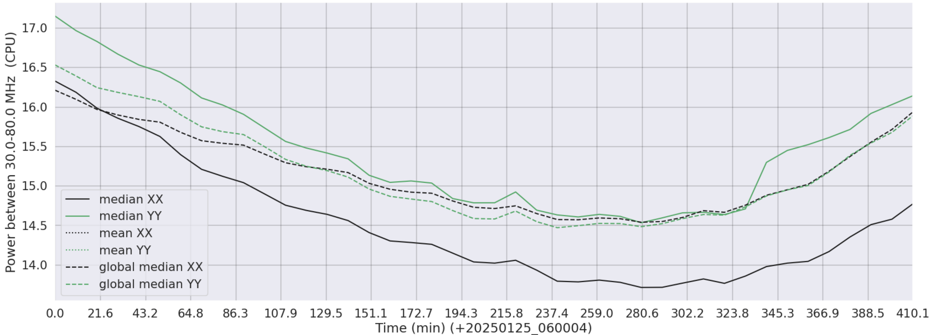
LWA362 - Correlator# 030 - XX FLAGS:Good - YY FLAGS:Good
