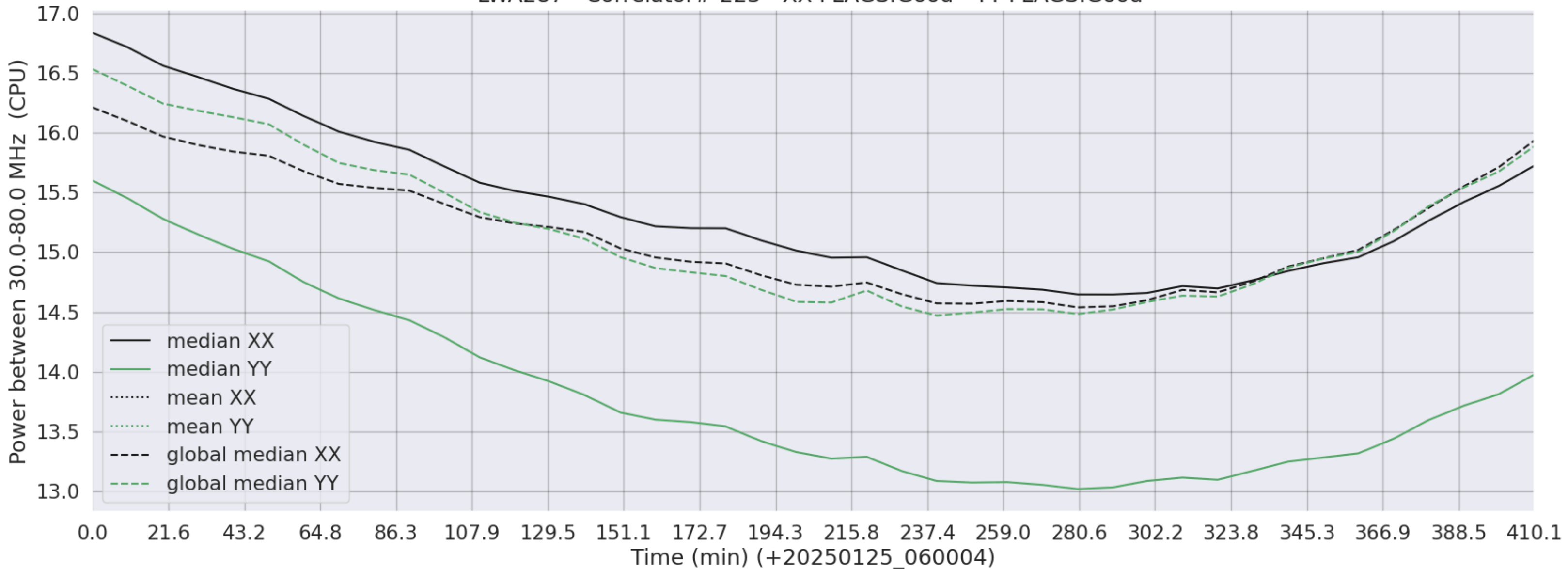
LWA287 - Correlator# 223 - XX FLAGS:Good - YY FLAGS:Good
