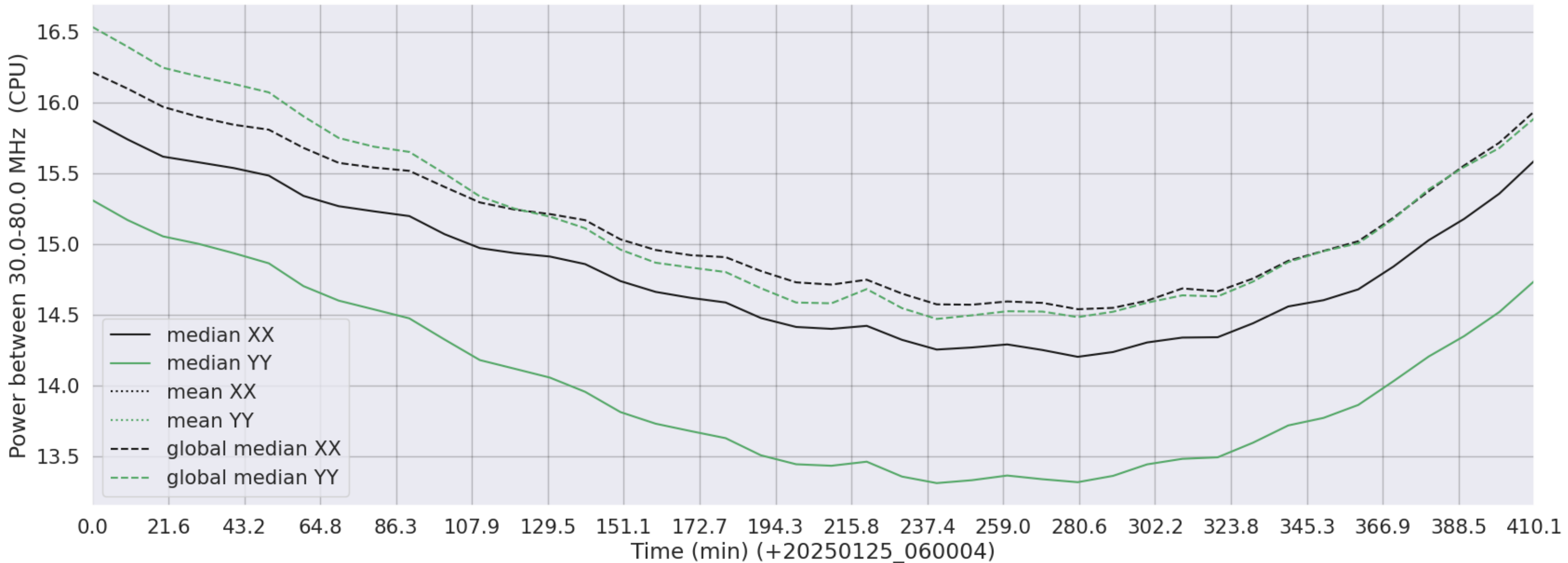
LWA192 - Correlator# 247 - XX FLAGS:Good - YY FLAGS:Good
