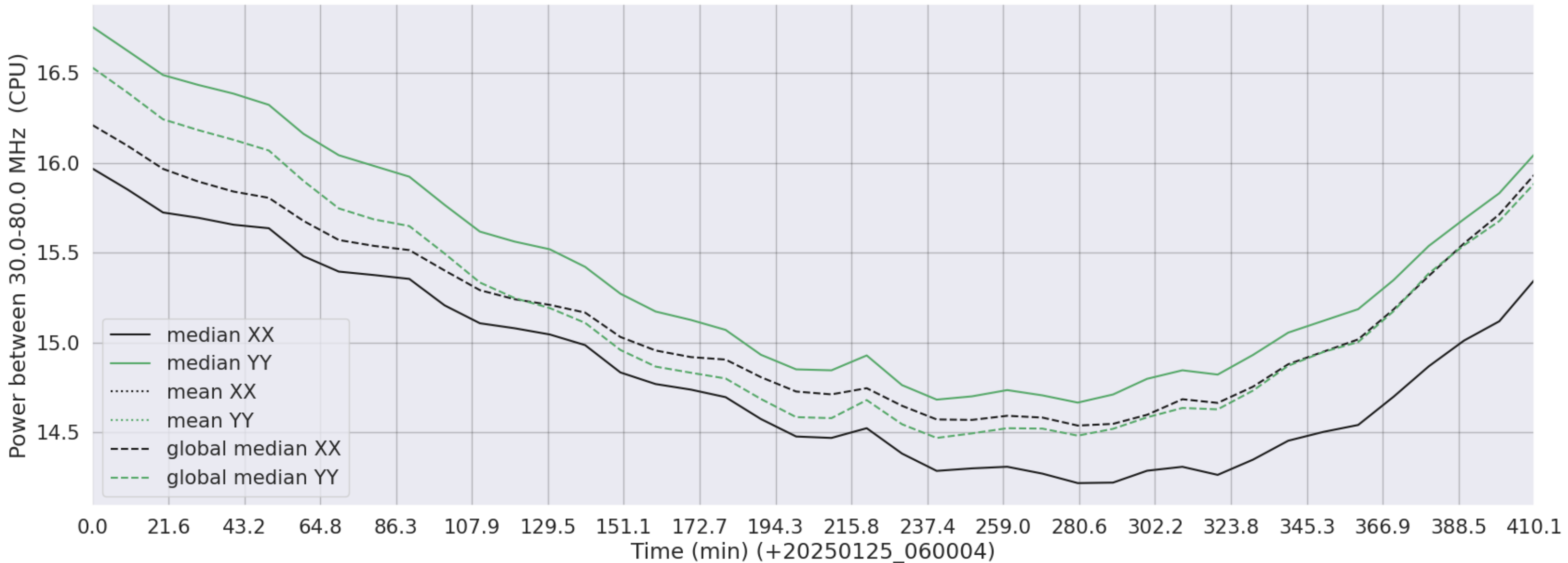
LWA016 - Correlator# 097 - XX FLAGS:Good - YY FLAGS:Good
