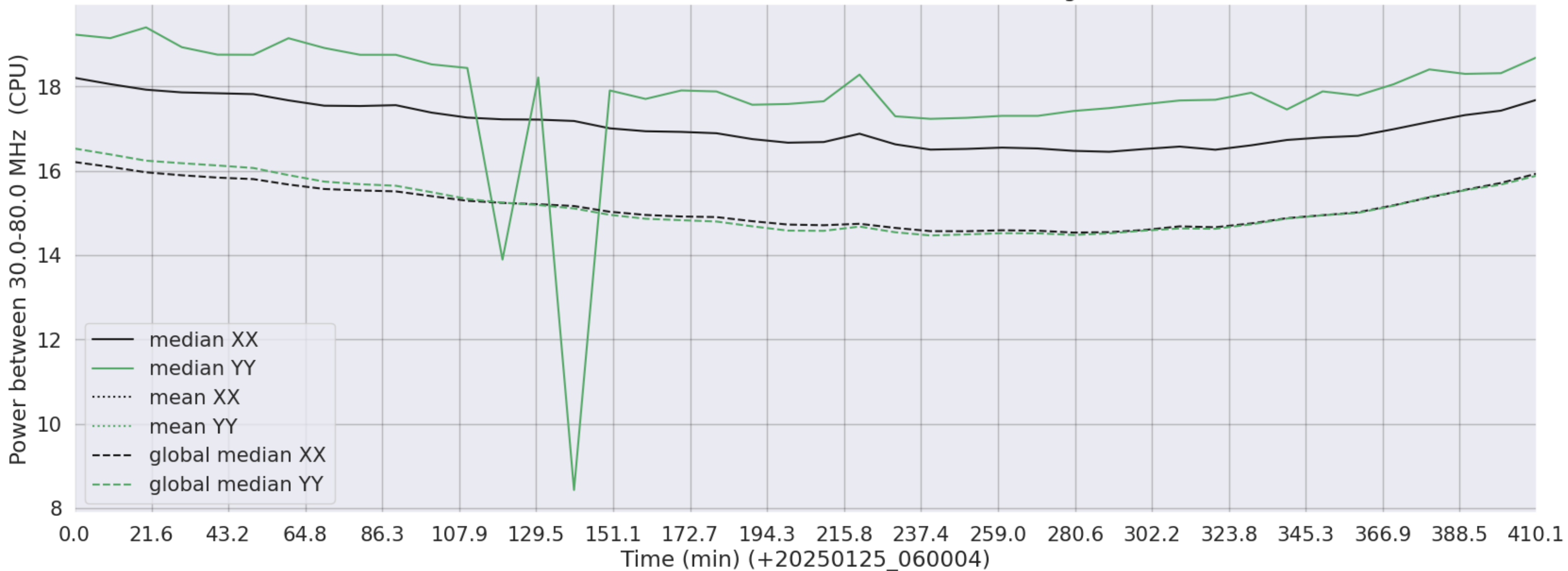
LWA065 - Correlator# 165 - XX FLAGS:Good - YY FLAGS:HighTimeVar
