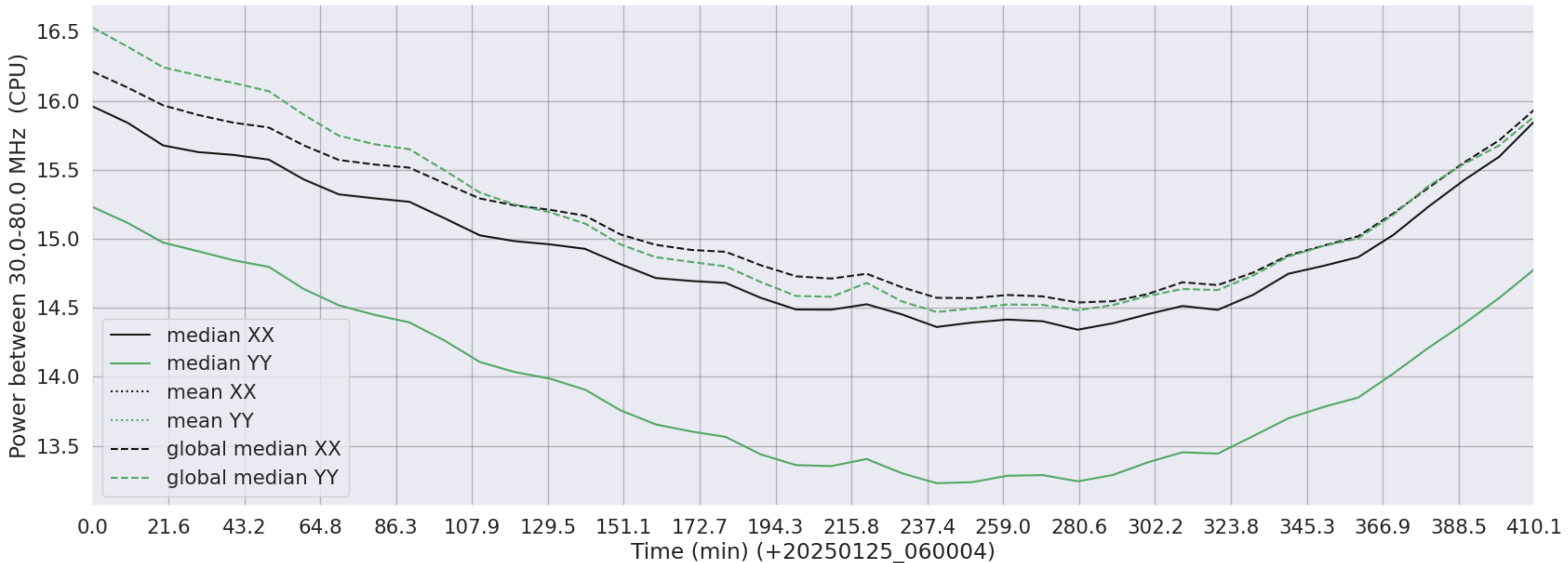
LWA092 - Correlator# 149 - XX FLAGS:Good - YY FLAGS:Good
