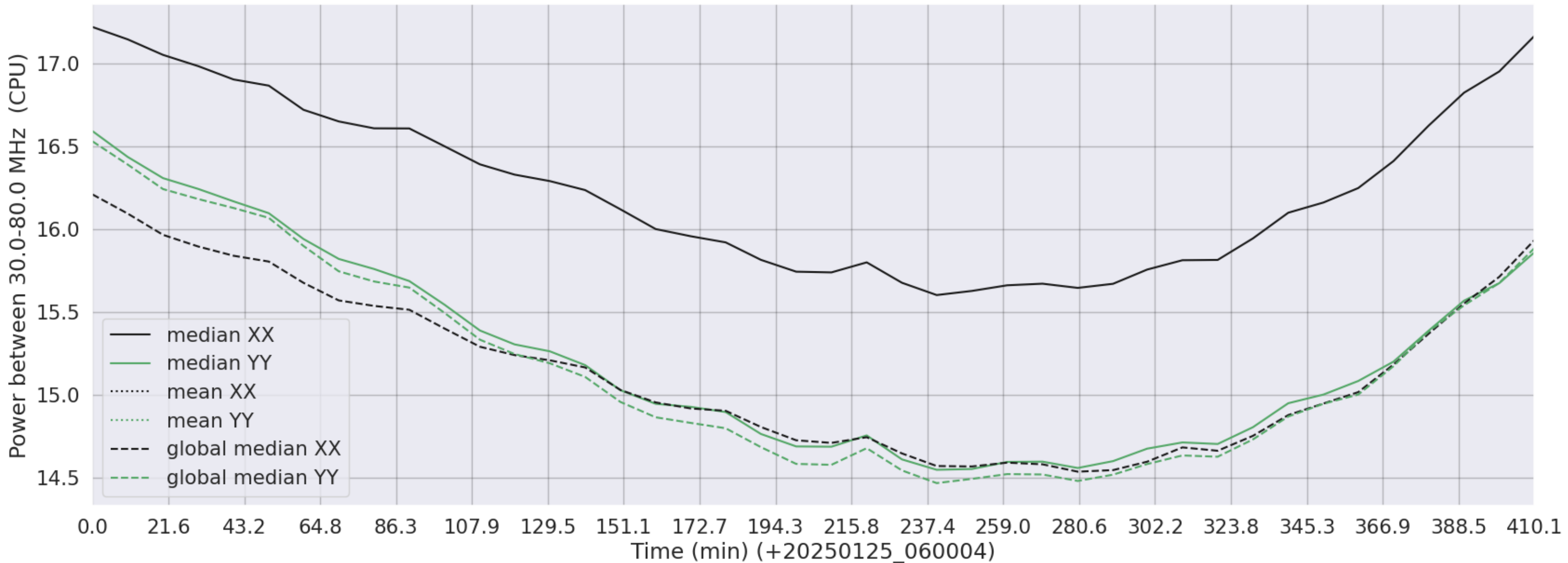
LWA327 - Correlator# 023 - XX FLAGS:Good - YY FLAGS:Good
