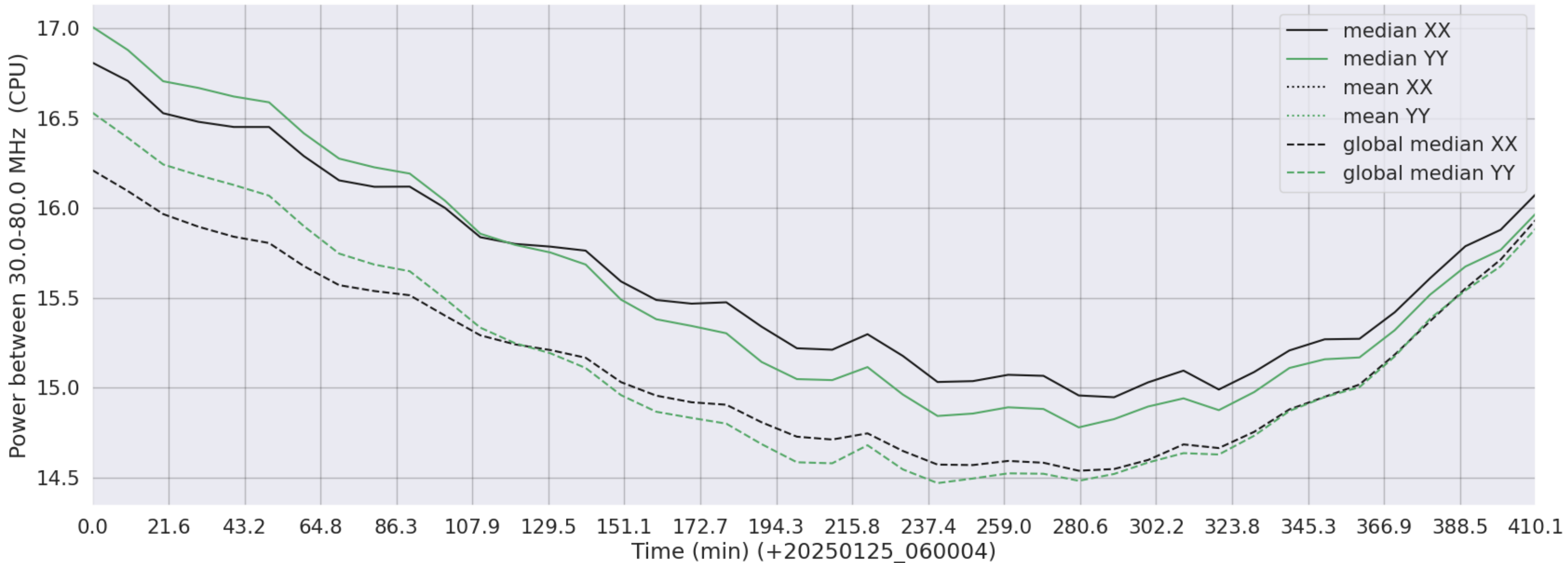
LWA018 - Correlator# 100 - XX FLAGS:Good - YY FLAGS:Good
