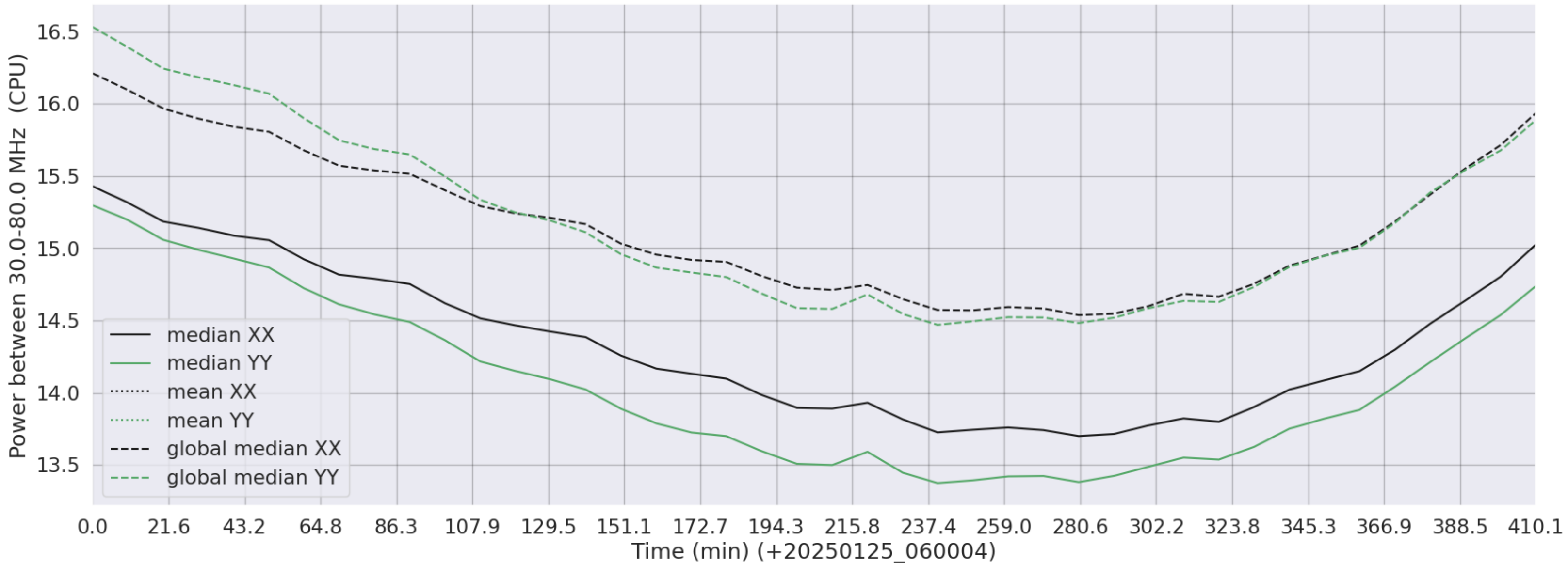
LWA058 - Correlator# 137 - XX FLAGS:Good - YY FLAGS:Good
