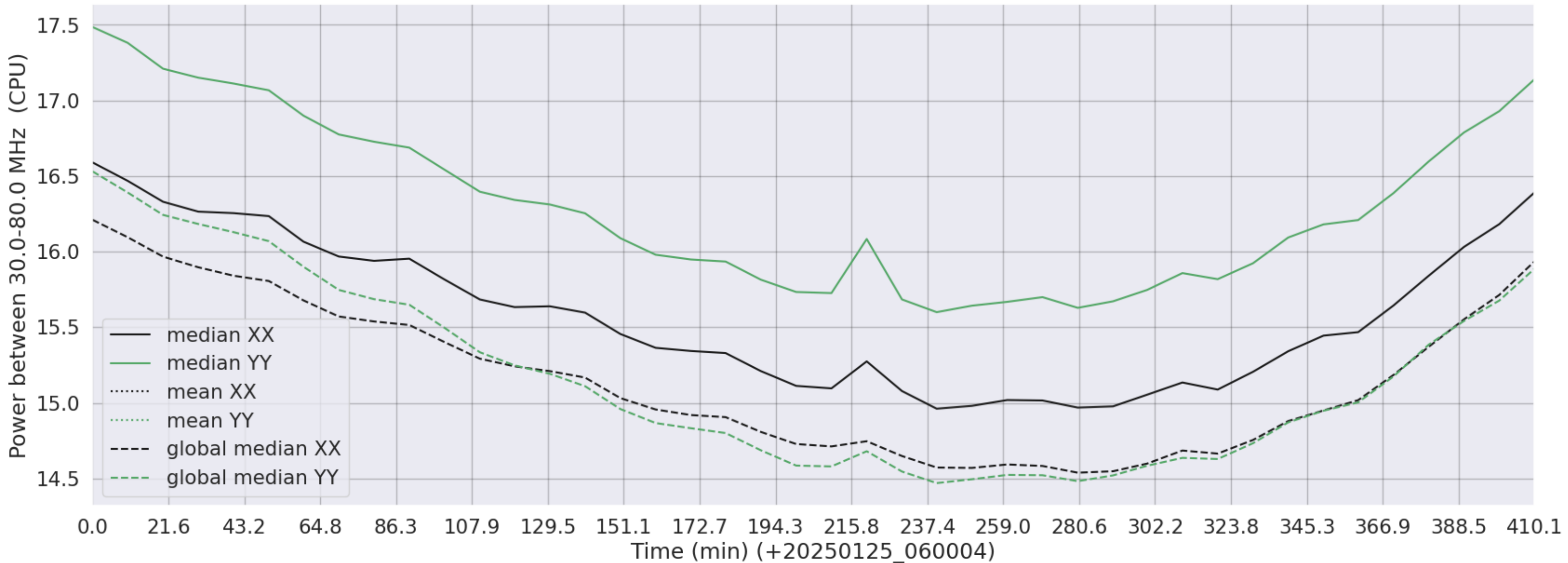
LWA196 - Correlator# 275 - XX FLAGS:Good - YY FLAGS:Good
