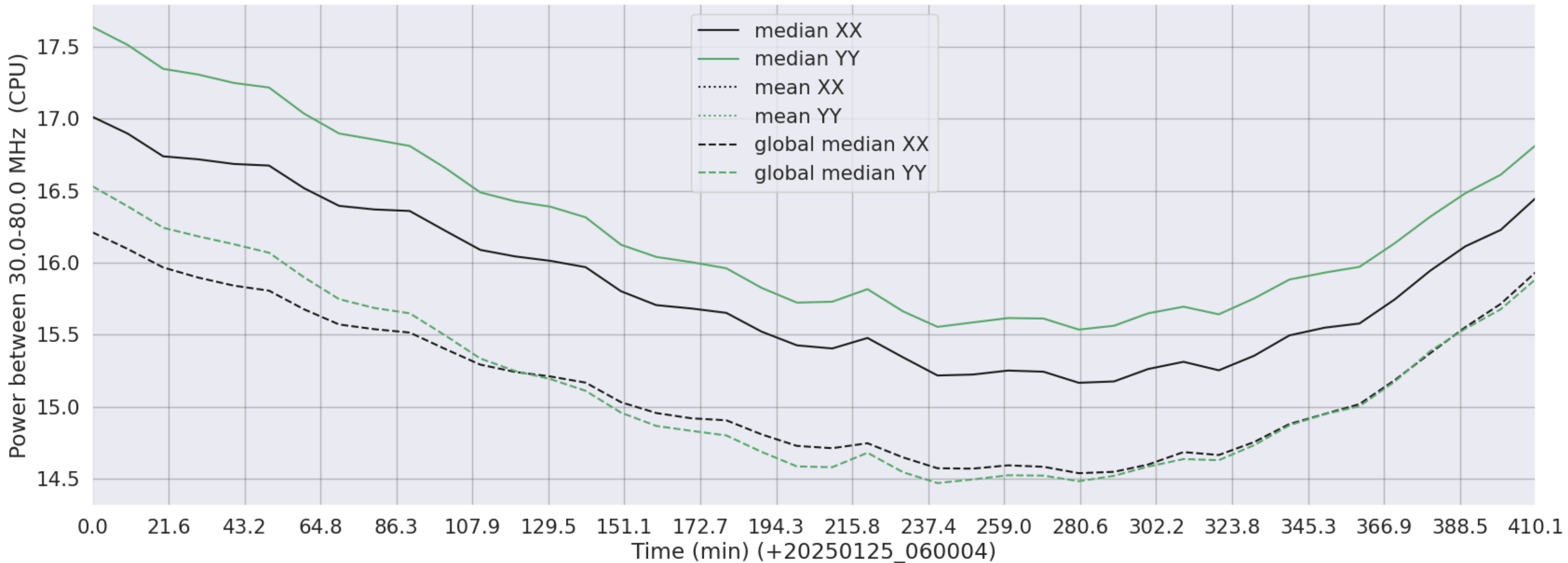
LWA077 - Correlator# 088 - XX FLAGS:Good - YY FLAGS:Good
