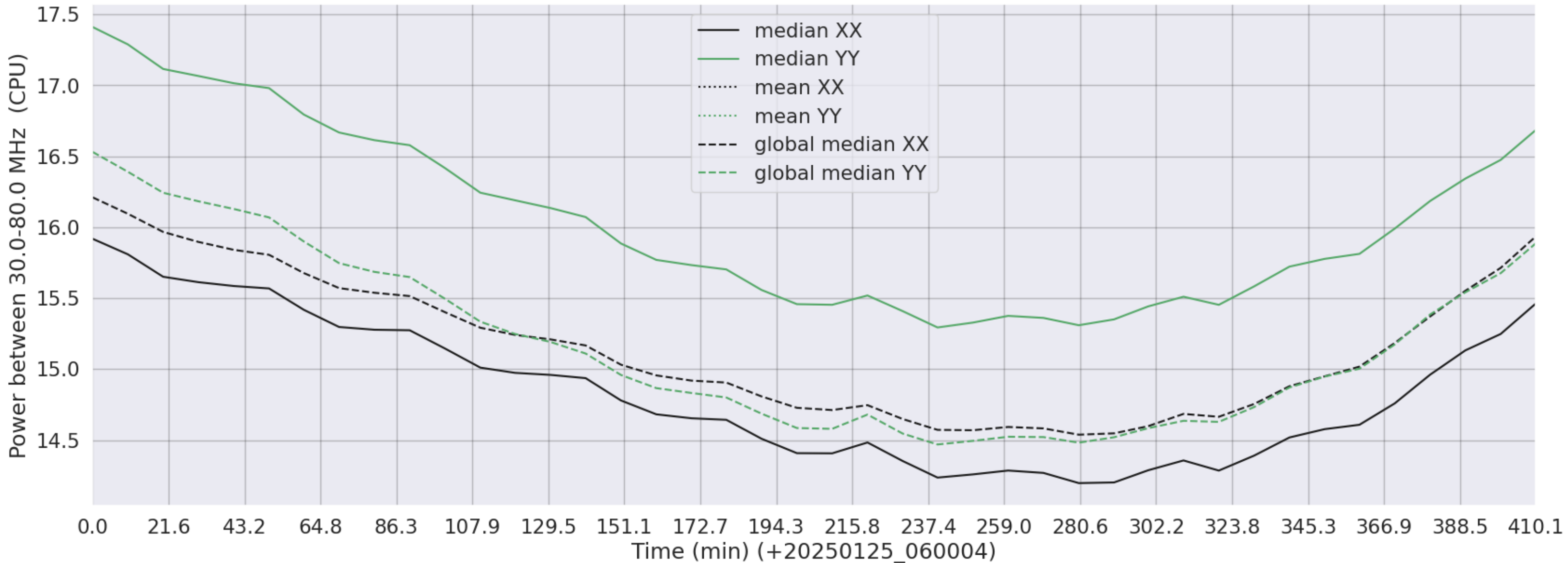
LWA075 - Correlator# 089 - XX FLAGS:Good - YY FLAGS:Good
