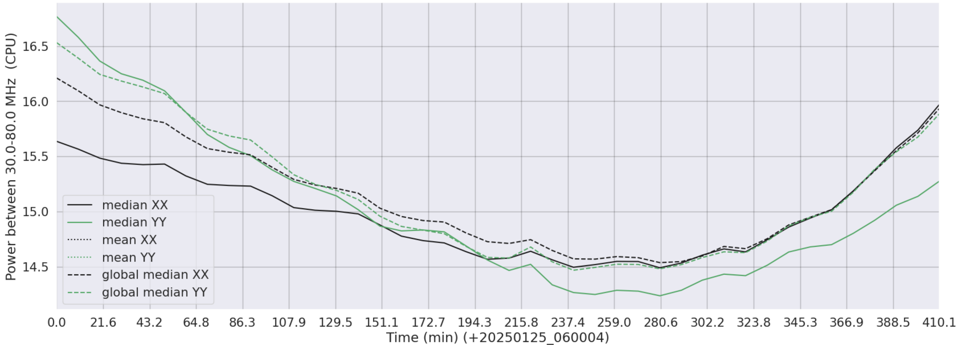
LWA271 - Correlator# 004 - XX FLAGS:Good - YY FLAGS:Good
