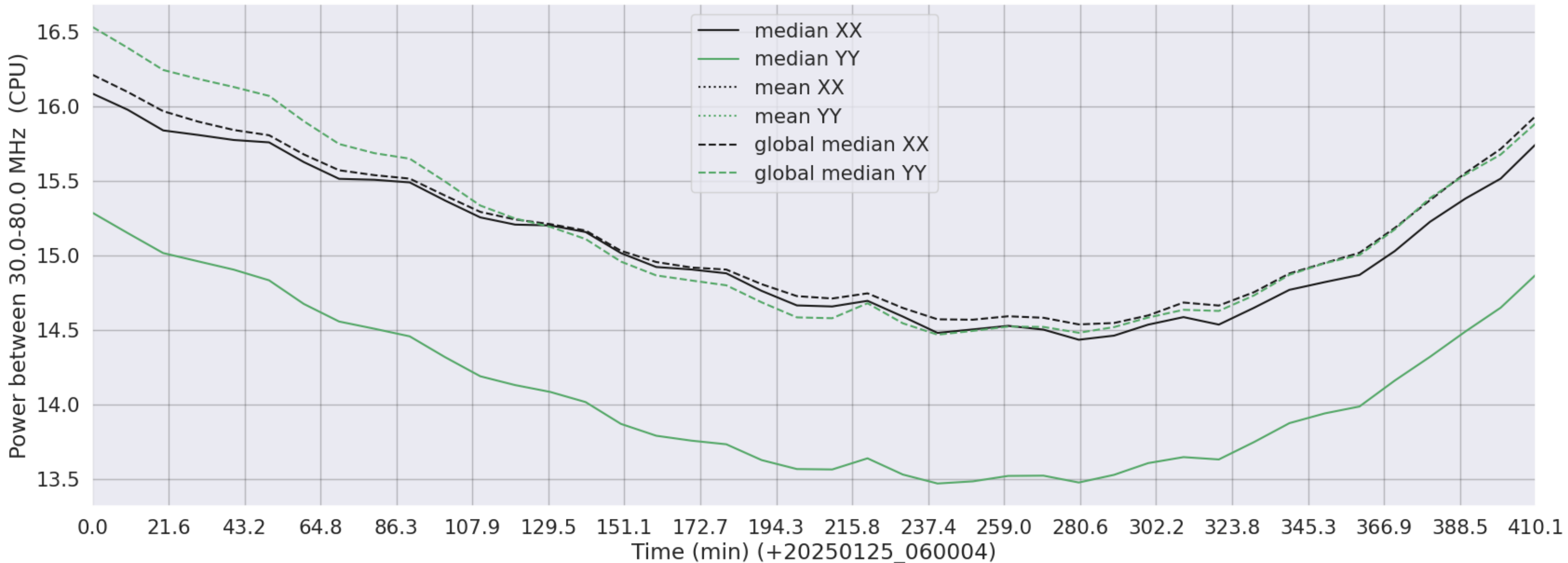
LWA114 - Correlator# 202 - XX FLAGS:Good - YY FLAGS:Good
