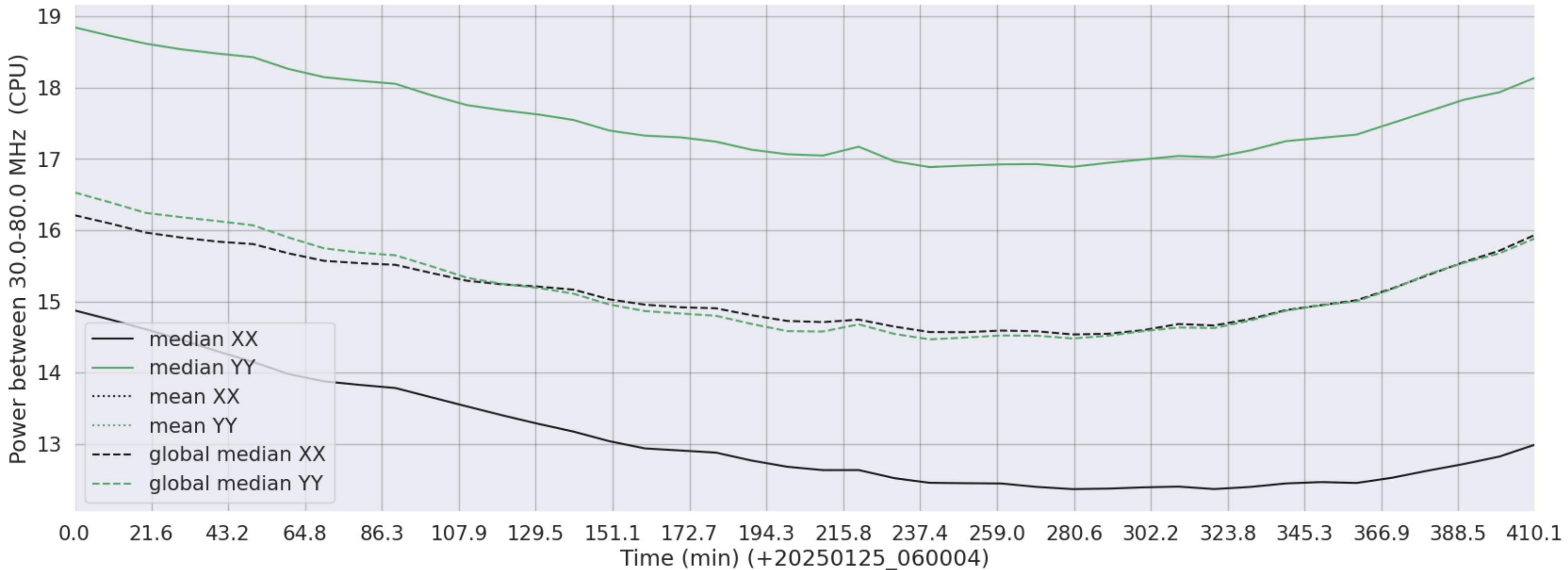
LWA342 - Correlator# 317 - XX FLAGS:Good - YY FLAGS:Good
