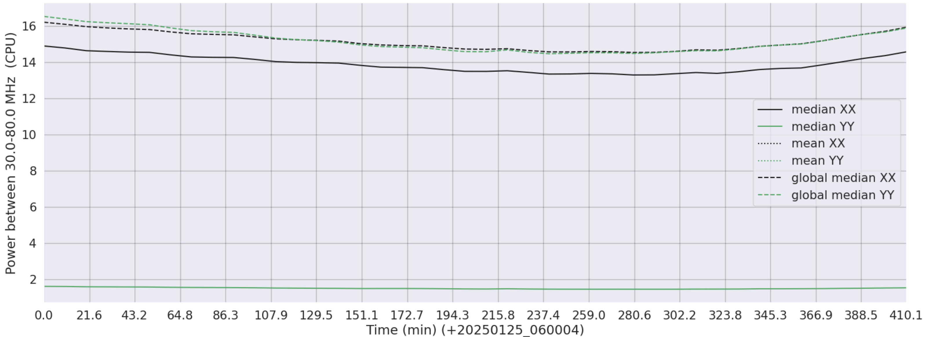
LWA186 - Correlator# 243 - XX FLAGS:Good - YY FLAGS:LowPower
