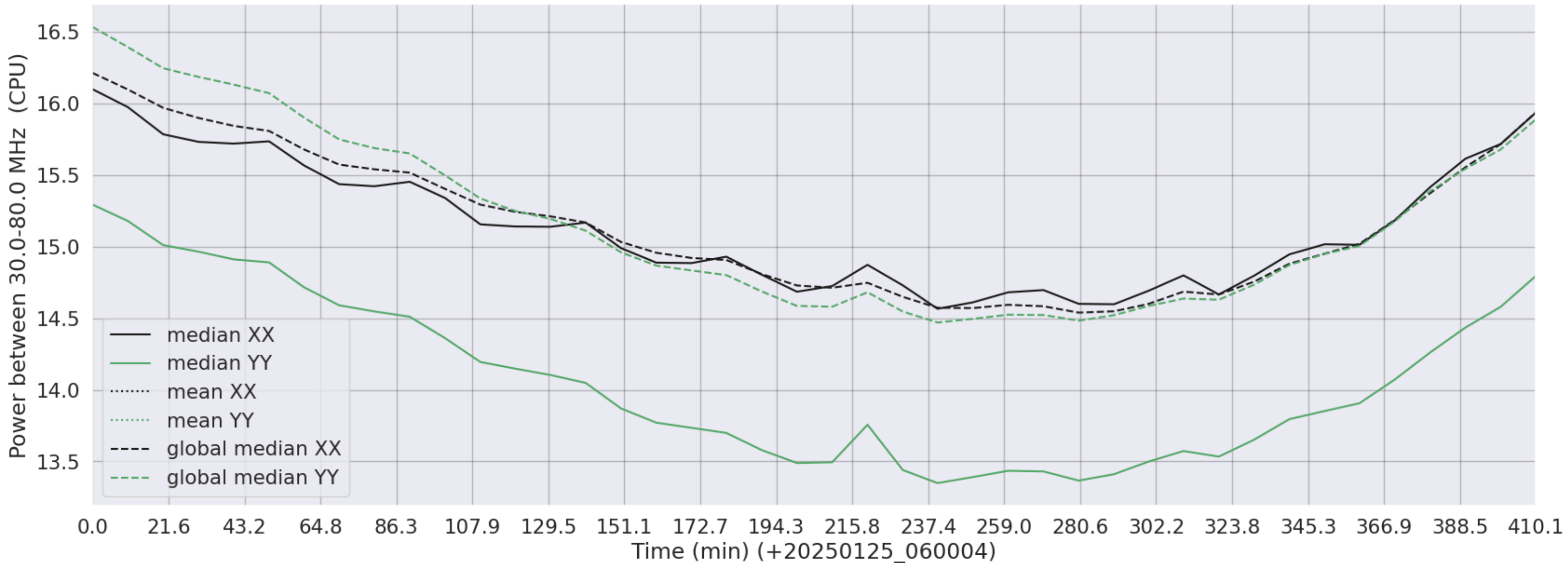
LWA255 - Correlator# 033 - XX FLAGS:Good - YY FLAGS:Good
