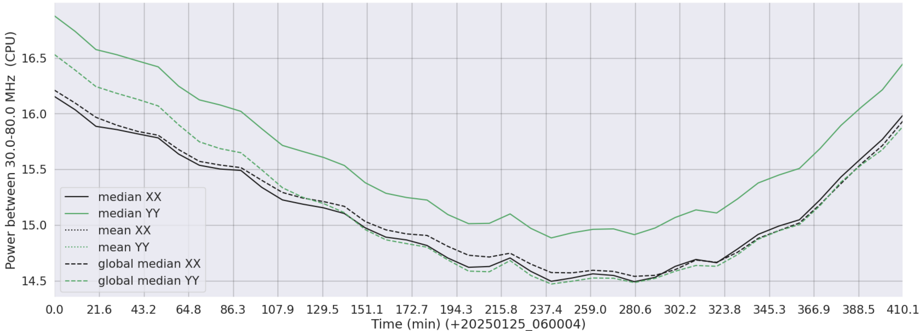
LWA048 - Correlator# 113 - XX FLAGS:Good - YY FLAGS:Good
