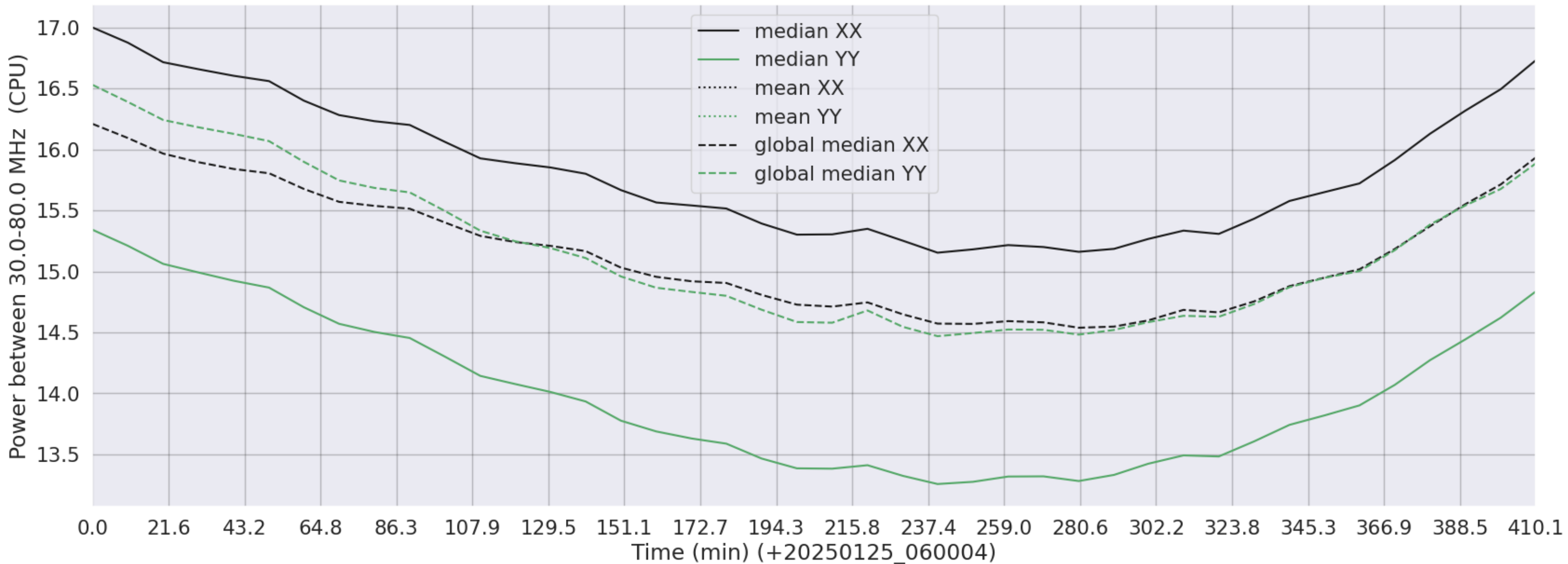
LWA221 - Correlator# 334 - XX FLAGS:Good - YY FLAGS:Good
