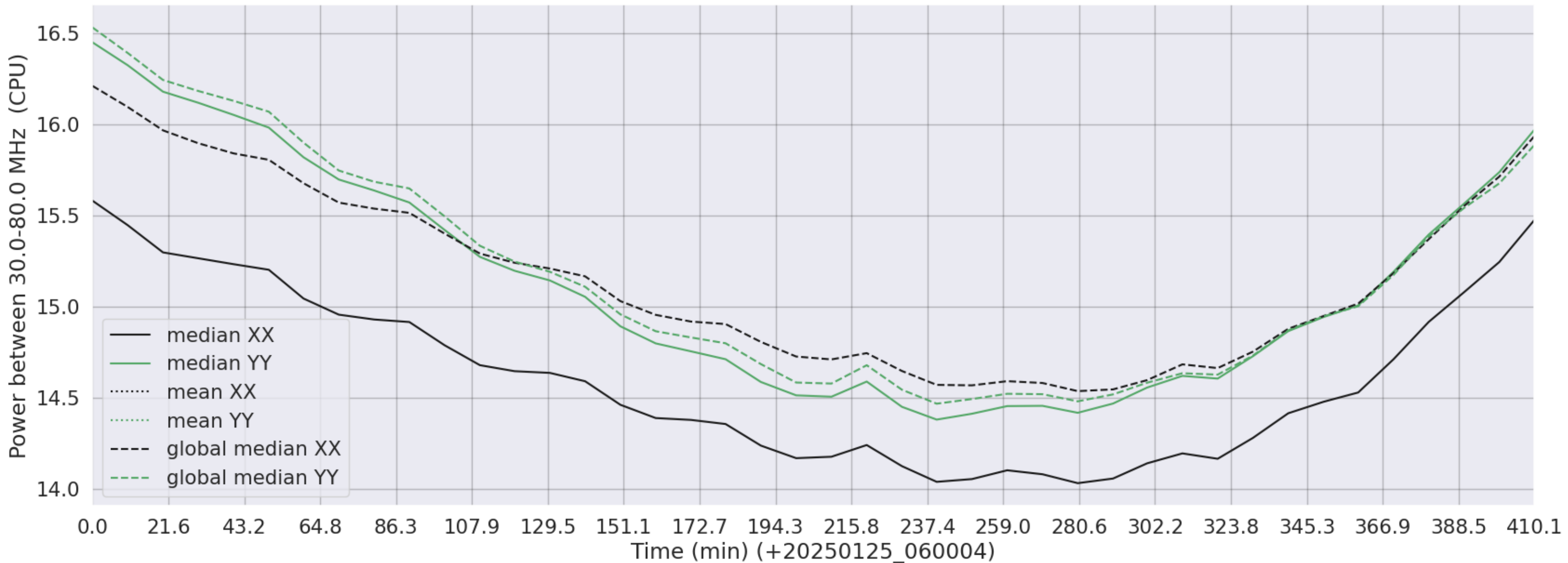
LWA179 - Correlator# 323 - XX FLAGS:Good - YY FLAGS:Good
