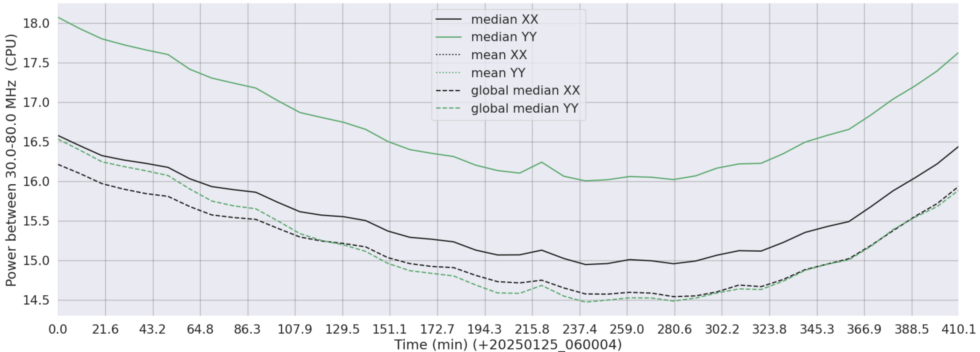
LWA234 - Correlator# 289 - XX FLAGS:Good - YY FLAGS:Good
