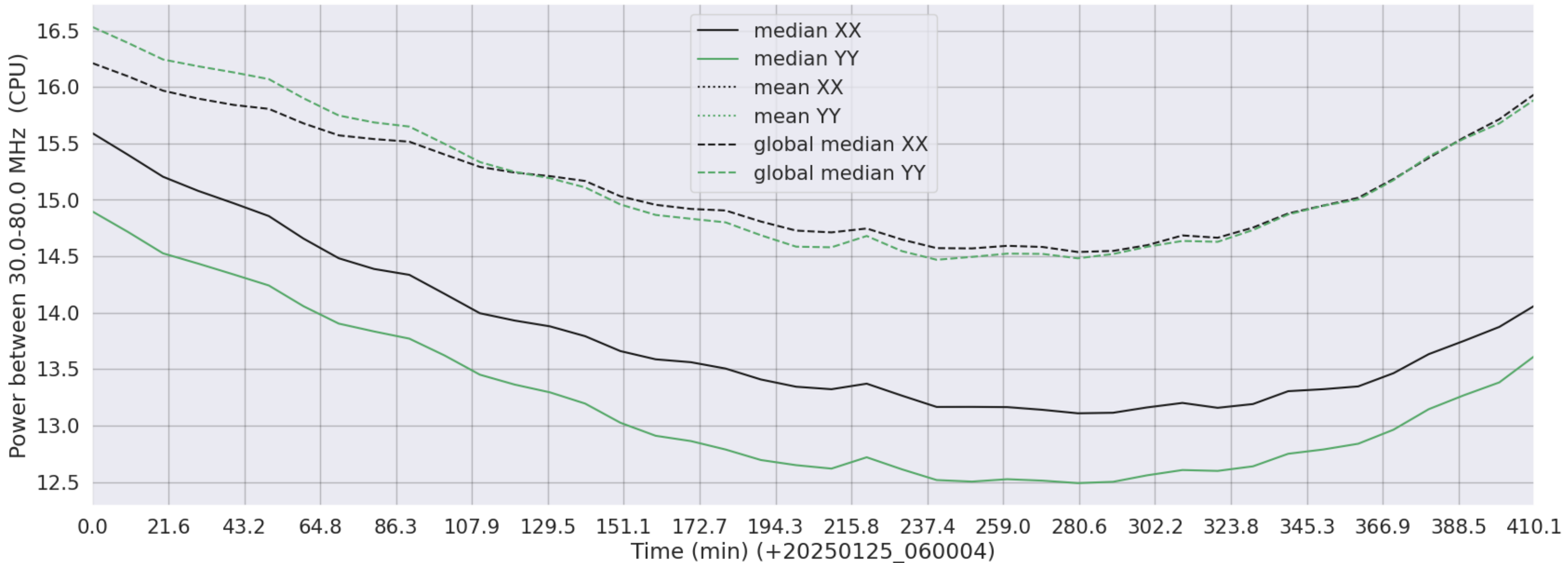
LWA360 - Correlator# 062 - XX FLAGS:Good - YY FLAGS:Good
