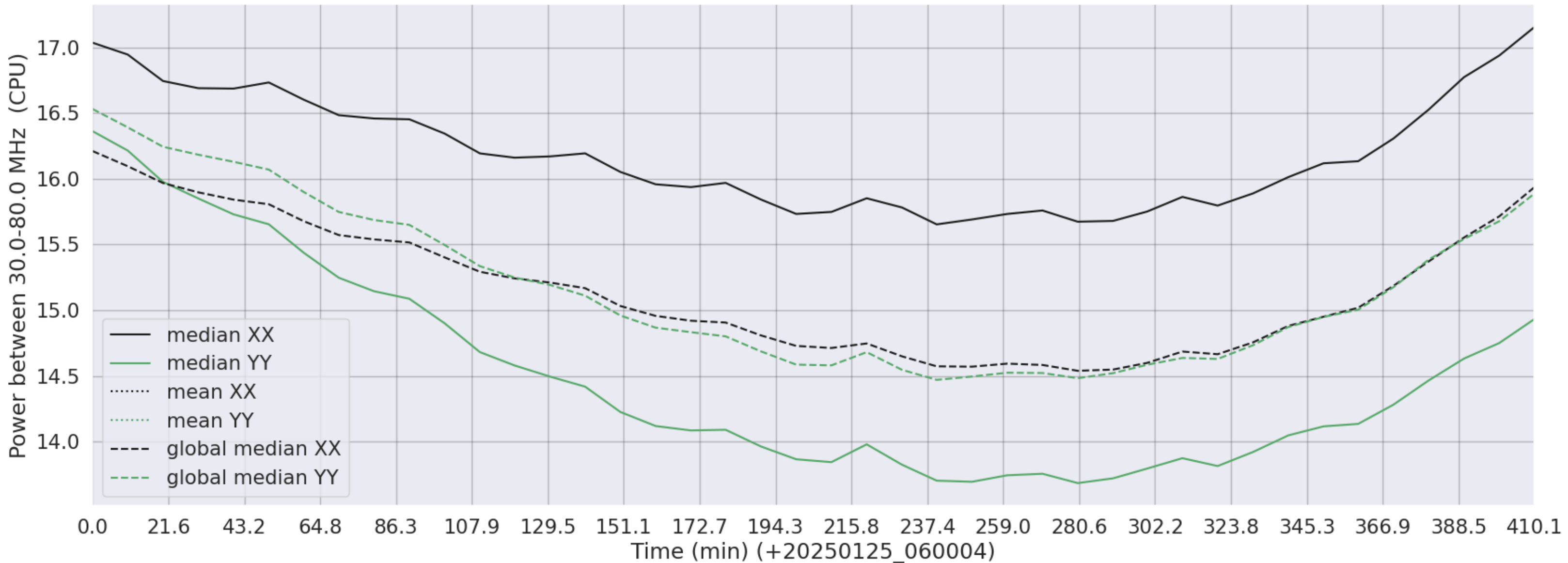
LWA361 - Correlator# 158 - XX FLAGS:Good - YY FLAGS:Good
