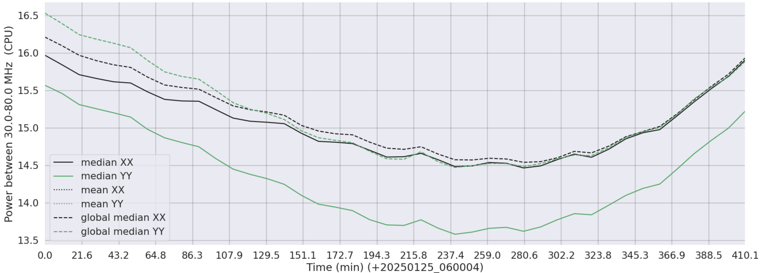
LWA215 - Correlator# 331 - XX FLAGS:Good - YY FLAGS:Good
