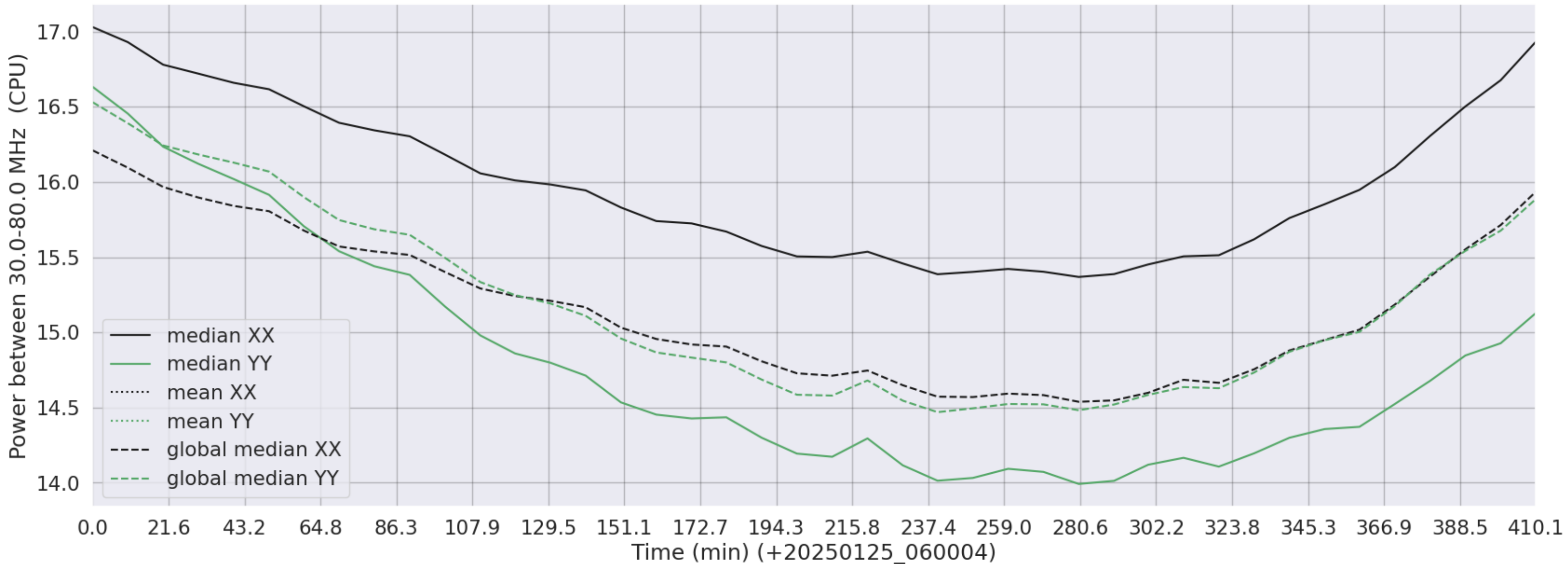
LWA355 - Correlator# 222 - XX FLAGS:Good - YY FLAGS:Good
