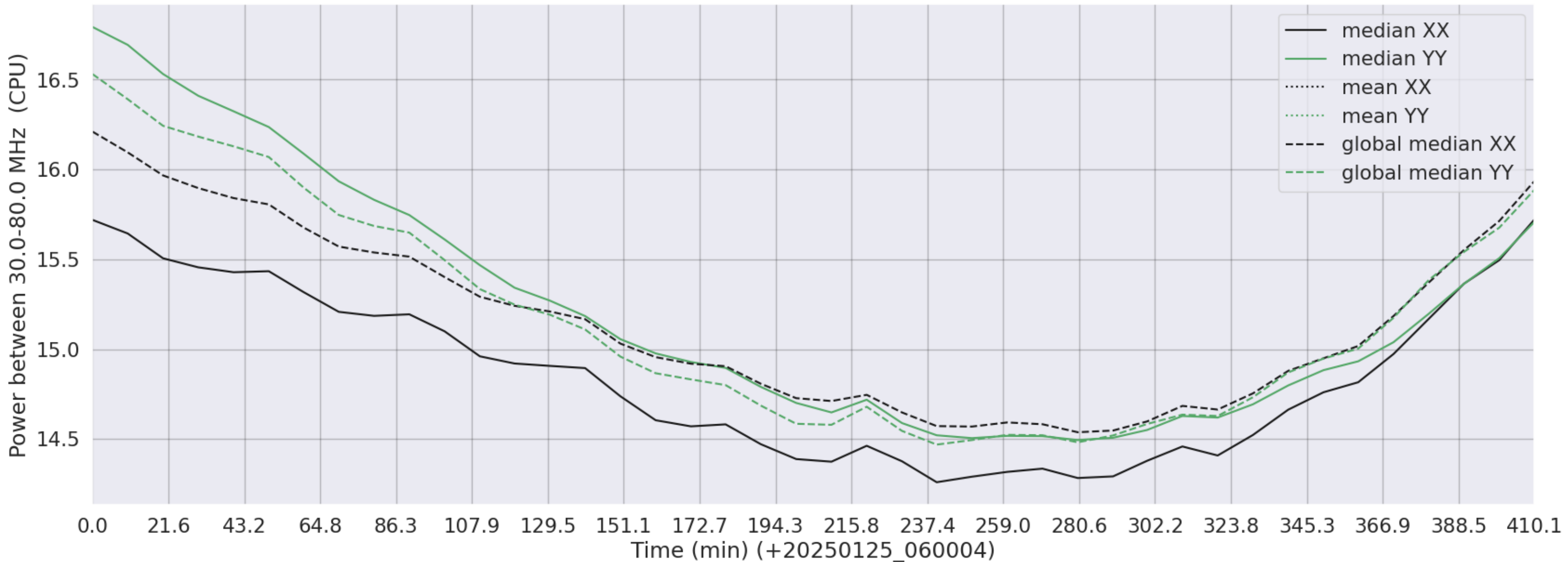
LWA261 - Correlator# 346 - XX FLAGS:Good - YY FLAGS:Good
