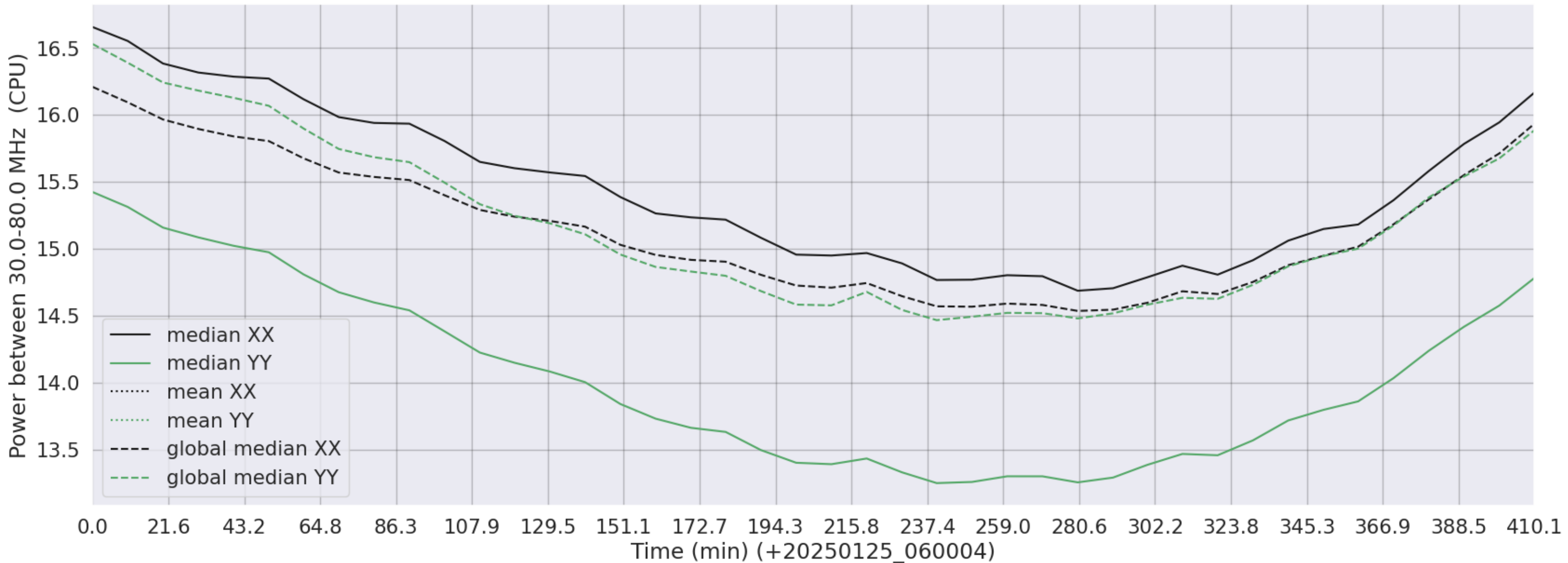
LWA062 - Correlator# 138 - XX FLAGS:Good - YY FLAGS:Good
