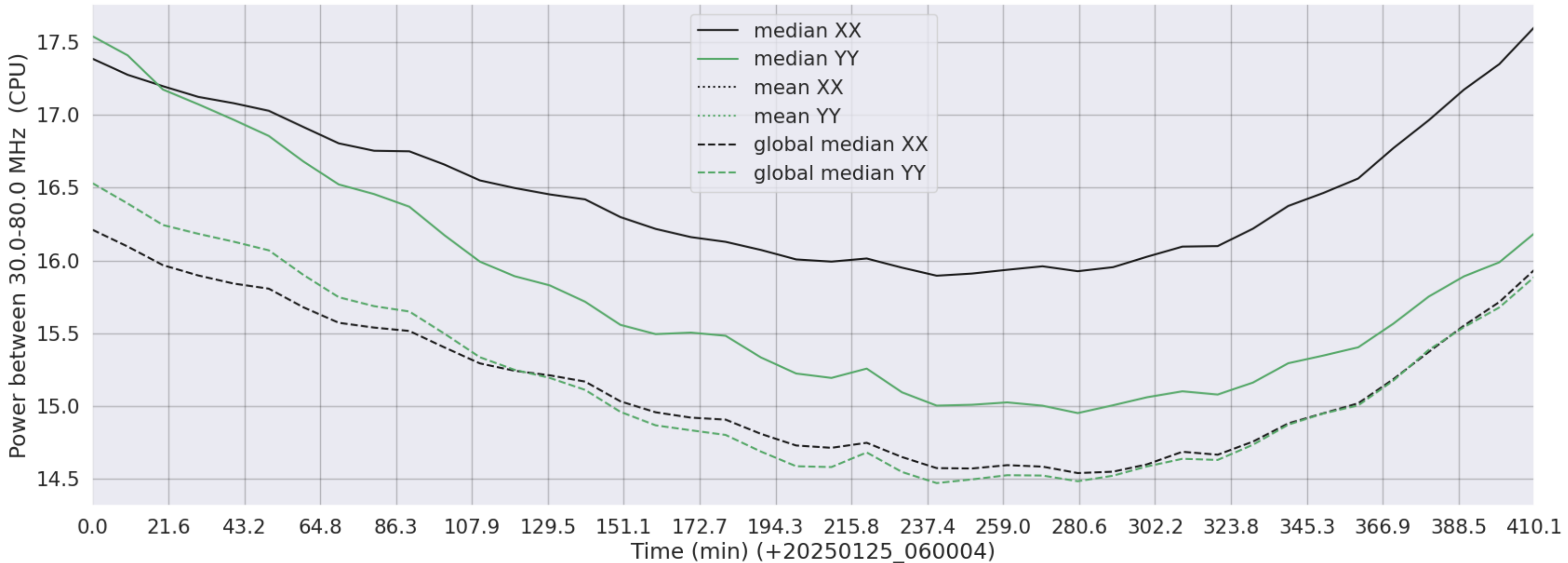
LWA319 - Correlator# 190 - XX FLAGS:Good - YY FLAGS:Good
