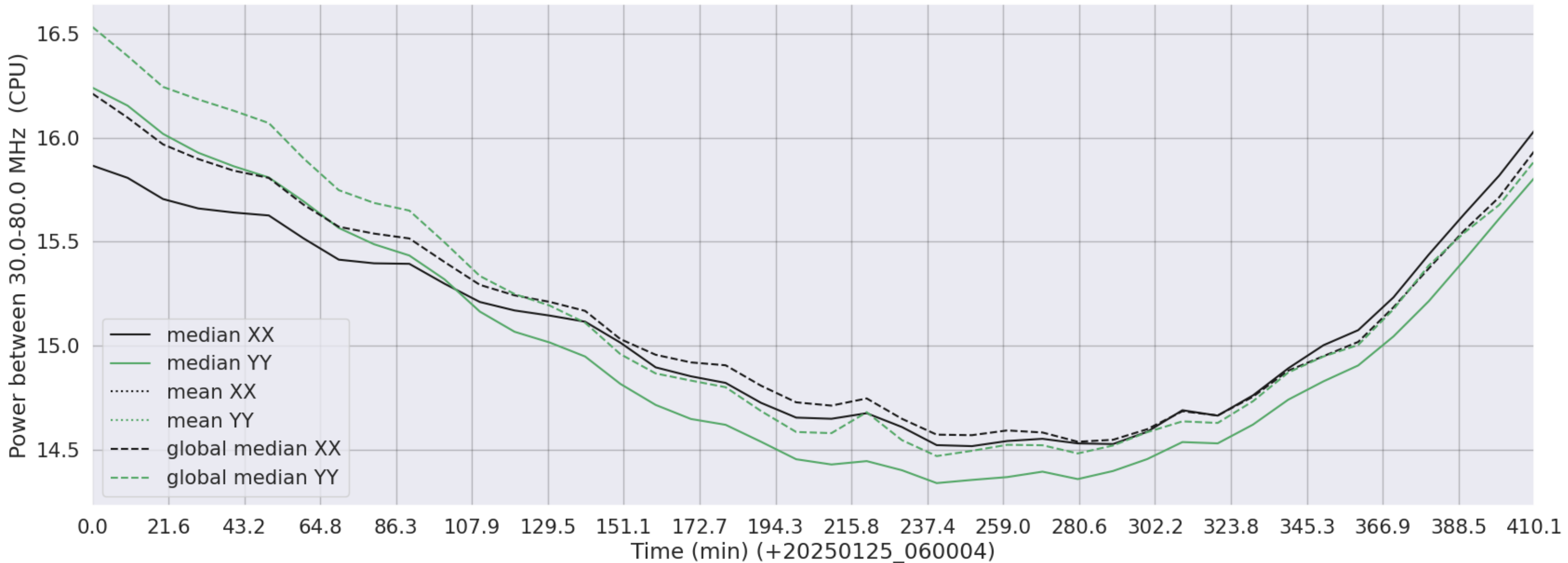
LWA307 - Correlator# 012 - XX FLAGS:Good - YY FLAGS:Good
