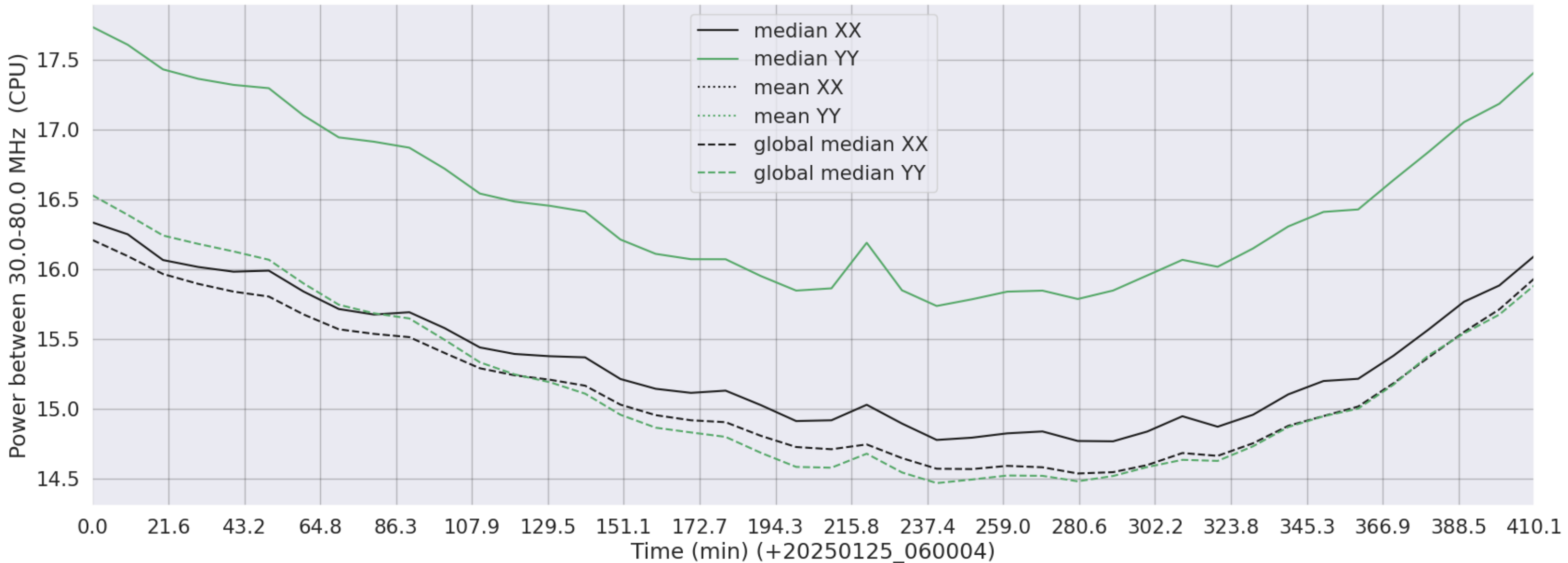
LWA134 - Correlator# 184 - XX FLAGS:Good - YY FLAGS:Good
