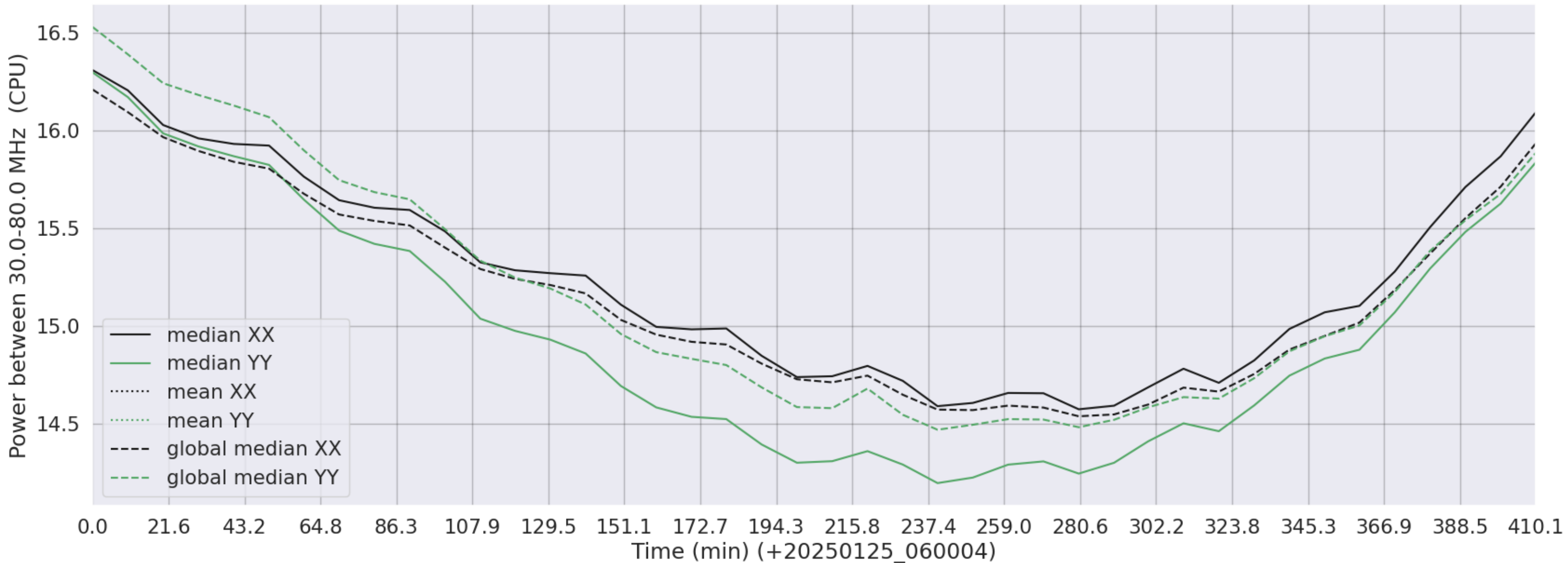
LWA184 - Correlator# 241 - XX FLAGS:Good - YY FLAGS:Good
