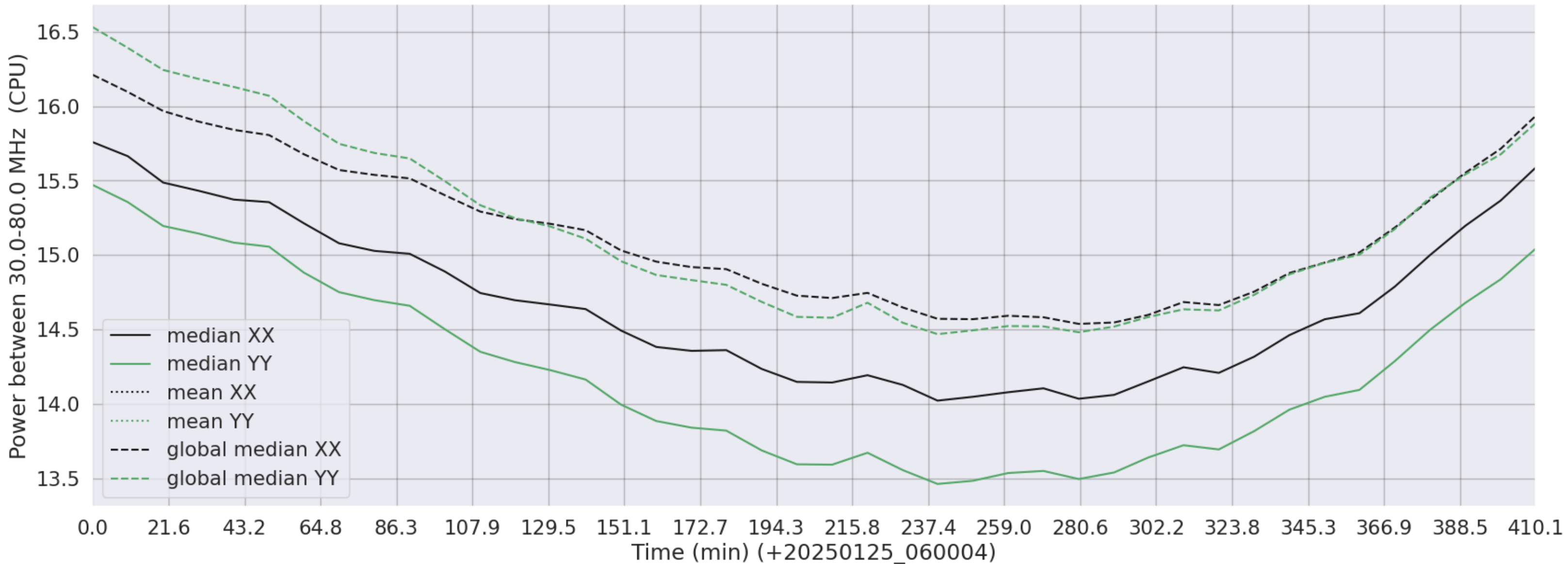
LWA247 - Correlator# 321 - XX FLAGS:Good - YY FLAGS:Good
