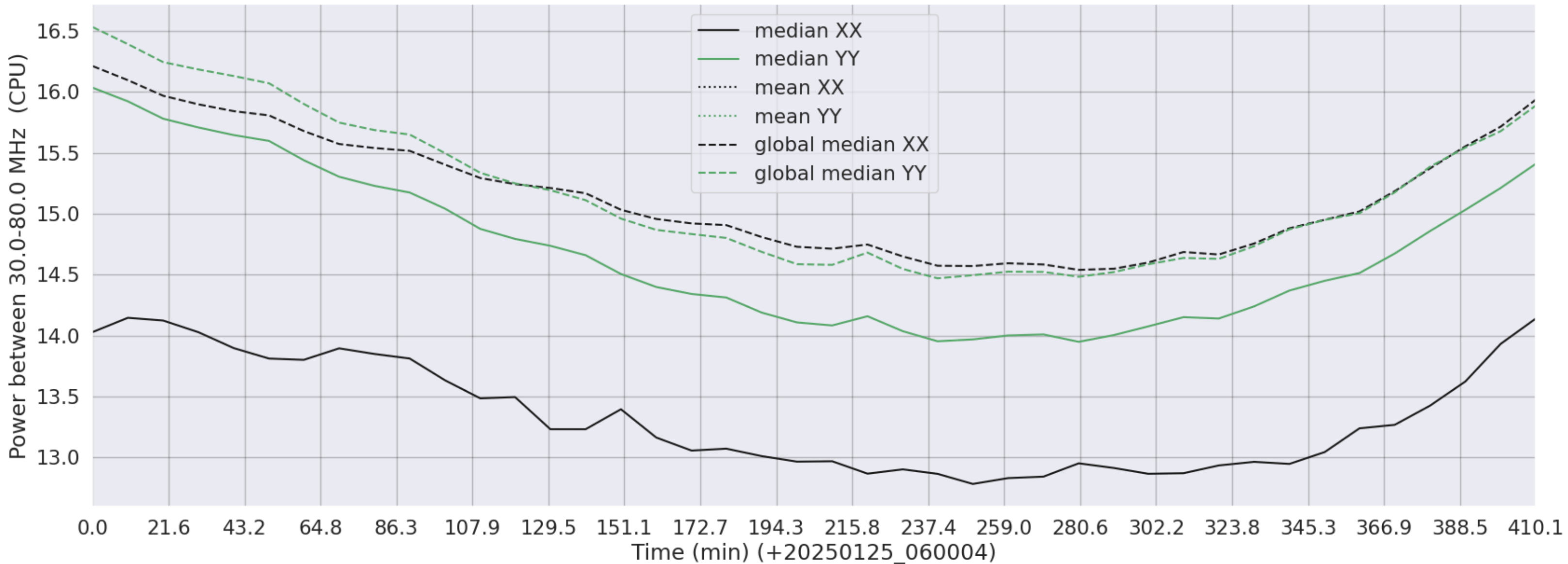
LWA224 - Correlator# 248 - XX FLAGS:Good - YY FLAGS:Good
