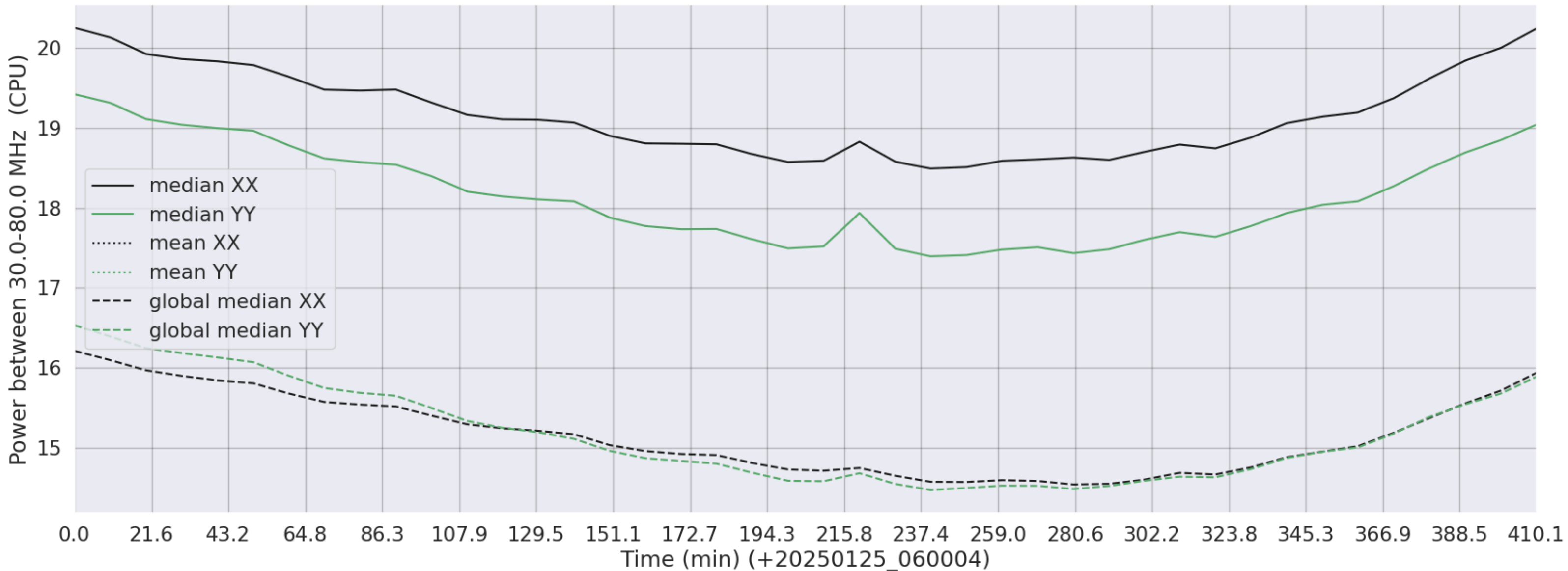
LWA225 - Correlator# 281 - XX FLAGS:Good - YY FLAGS:Good
