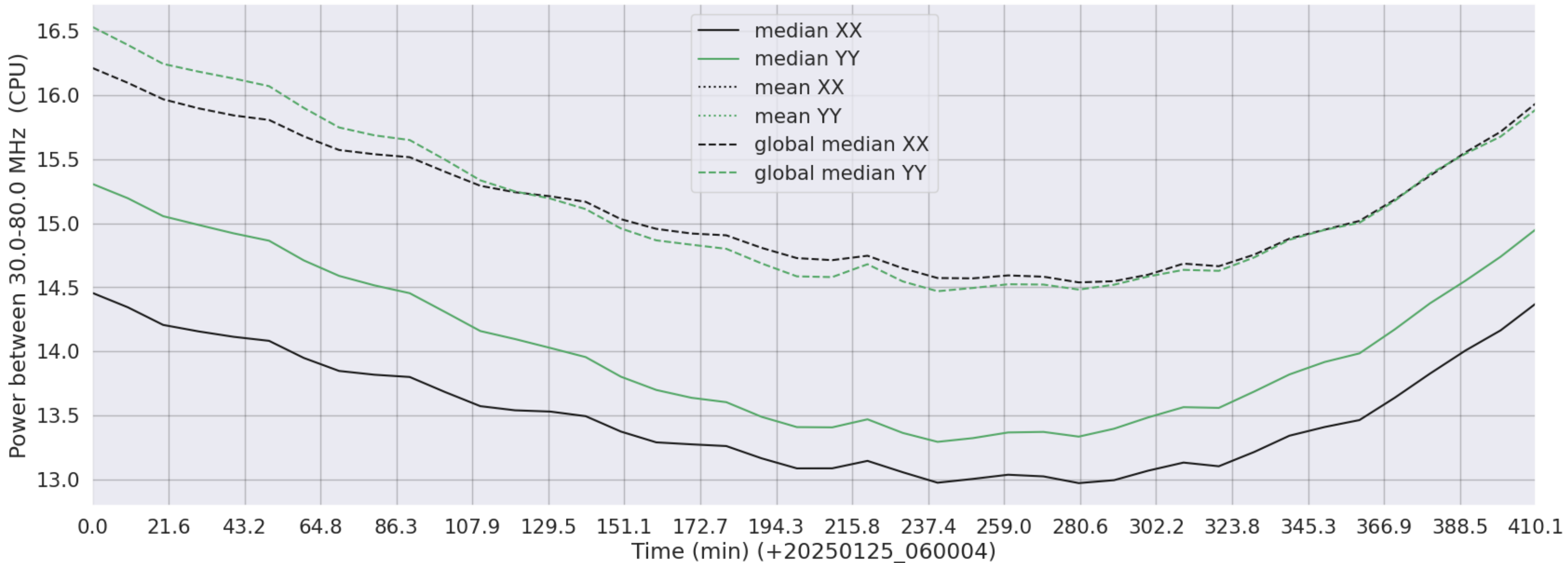
LWA218 - Correlator# 332 - XX FLAGS:Good - YY FLAGS:Good
