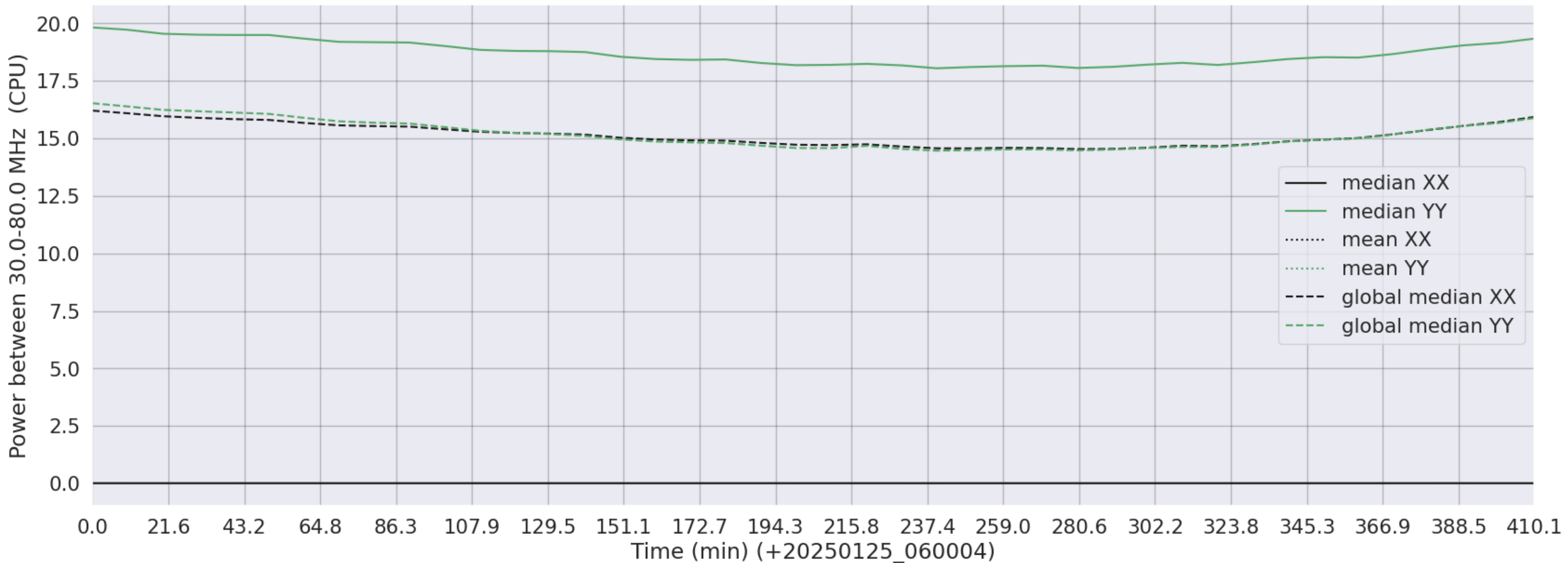
LWA209 - Correlator# 301 - XX FLAGS:LowPower - YY FLAGS:Good
