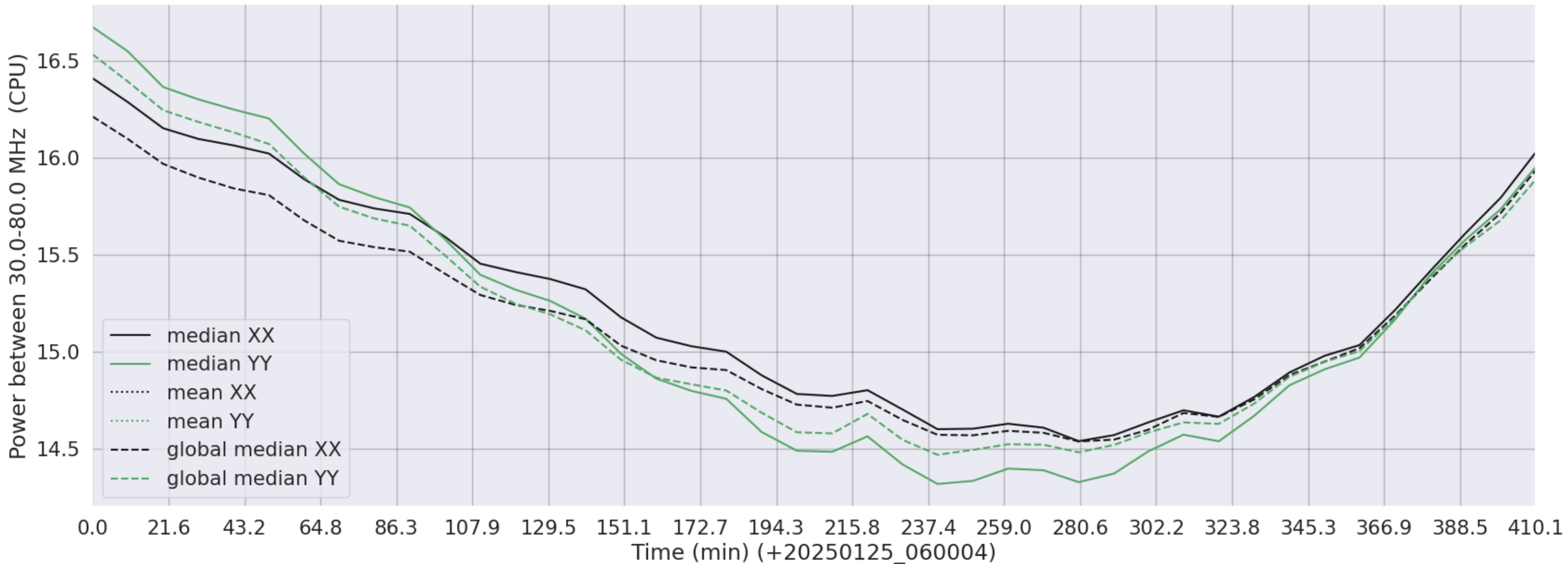
LWA185 - Correlator# 240 - XX FLAGS:Good - YY FLAGS:Good
