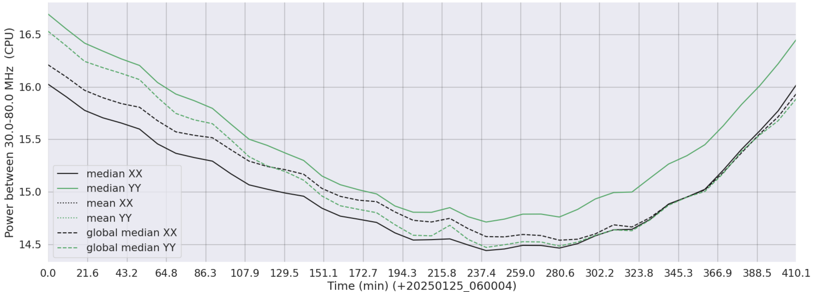
LWA089 - Correlator# 144 - XX FLAGS:Good - YY FLAGS:Good
