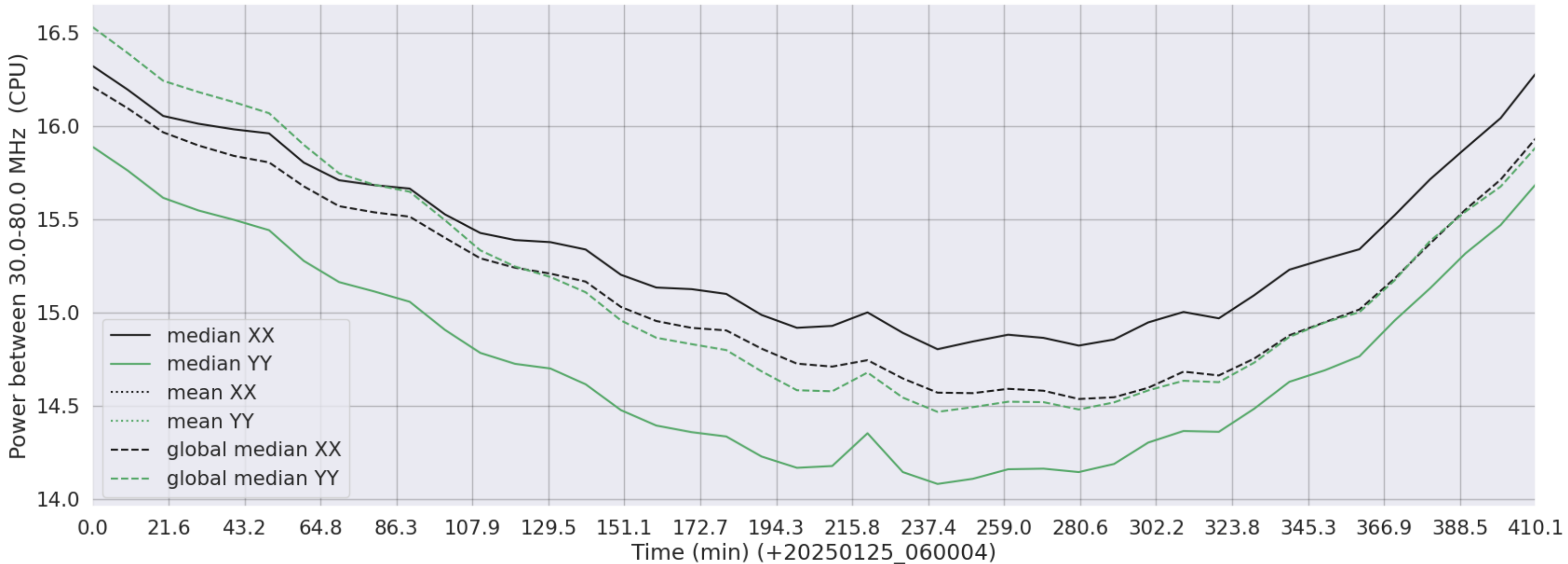
LWA167 - Correlator# 268 - XX FLAGS:Good - YY FLAGS:Good
