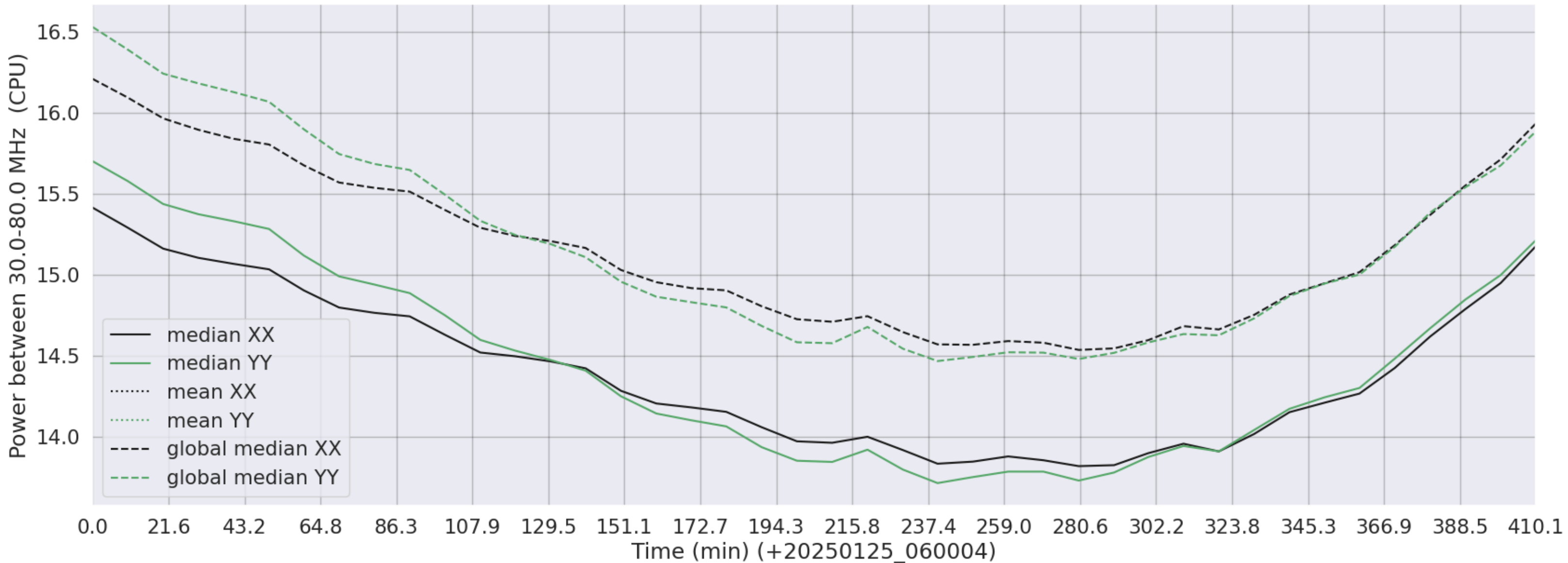
LWA045 - Correlator# 083 - XX FLAGS:Good - YY FLAGS:Good
