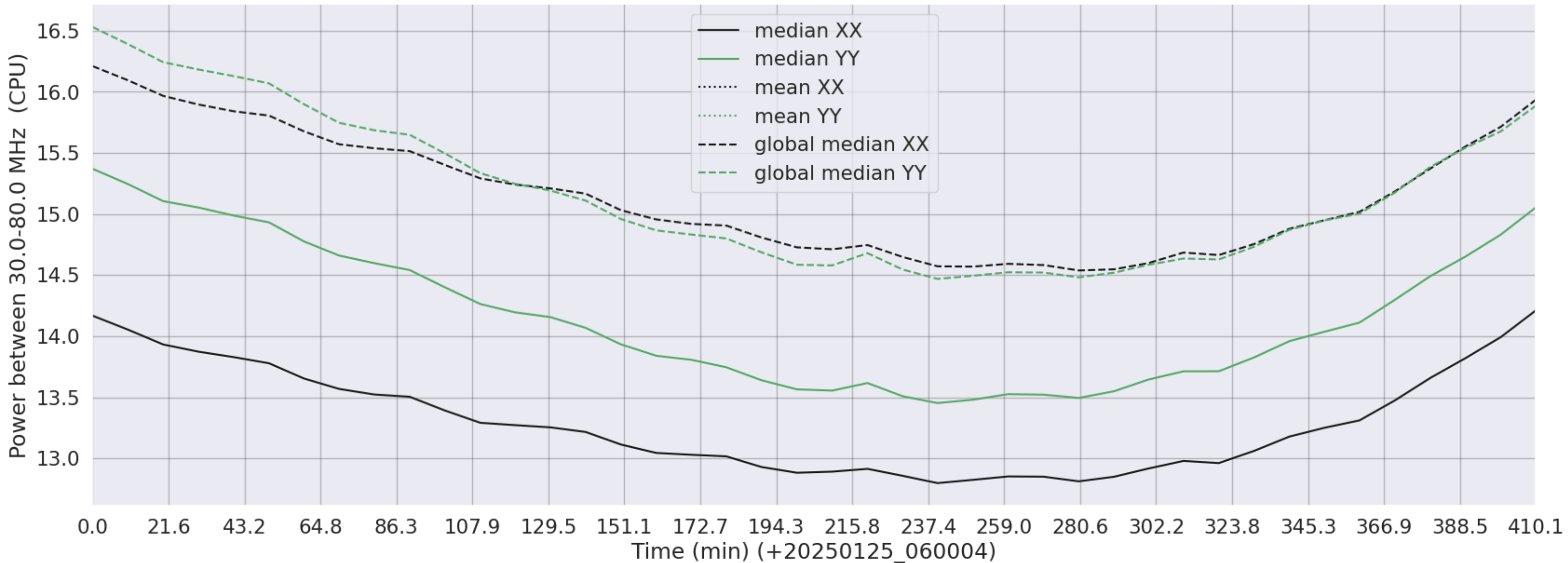
LWA181 - Correlator# 231 - XX FLAGS:Good - YY FLAGS:Good
