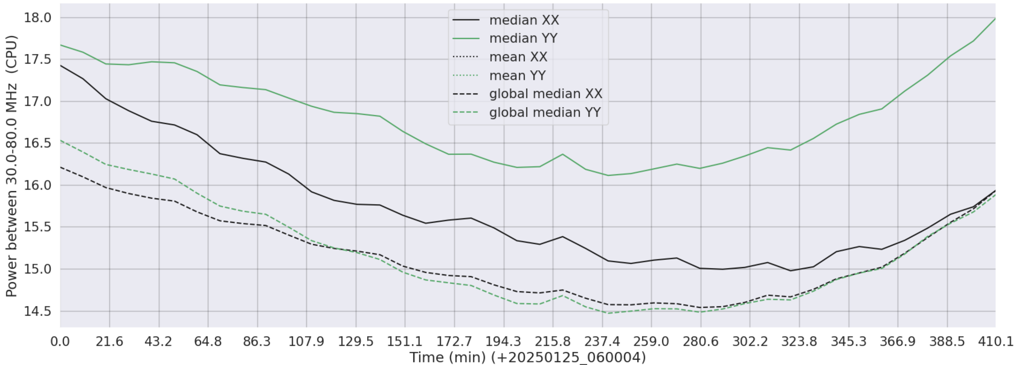
LWA310 - Correlator# 017 - XX FLAGS:Good - YY FLAGS:Good
