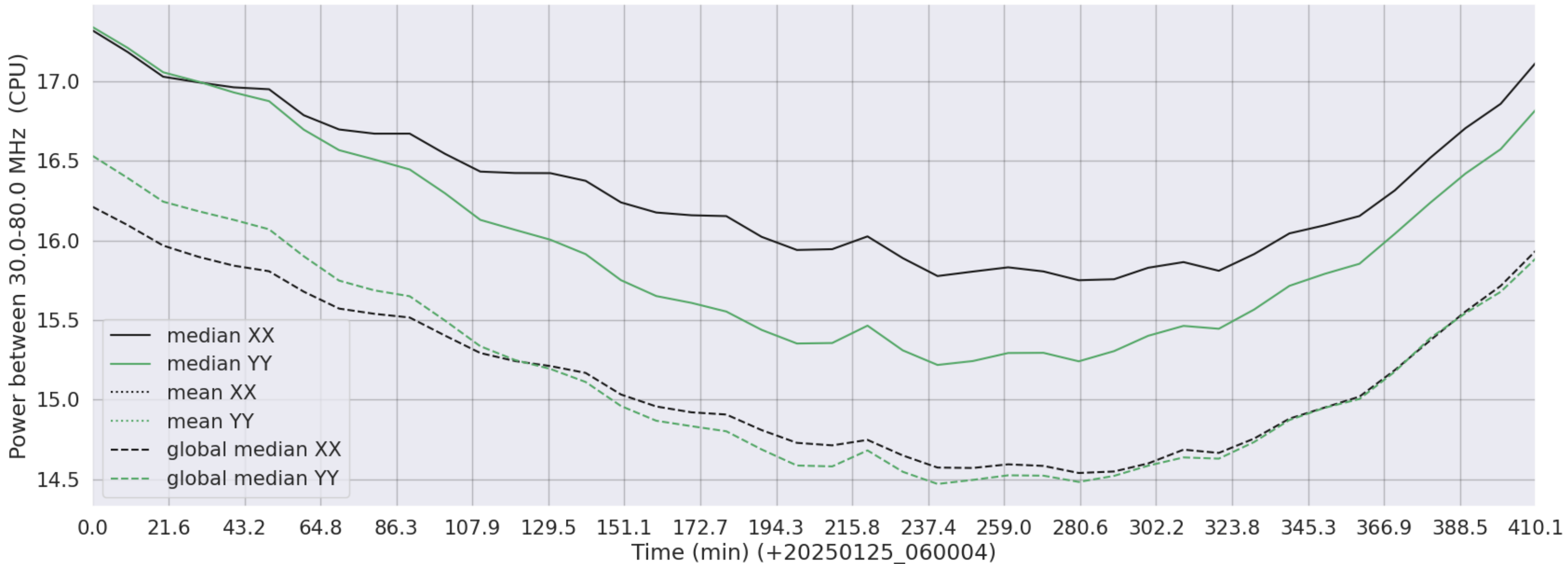
LWA020 - Correlator# 102 - XX FLAGS:Good - YY FLAGS:Good
