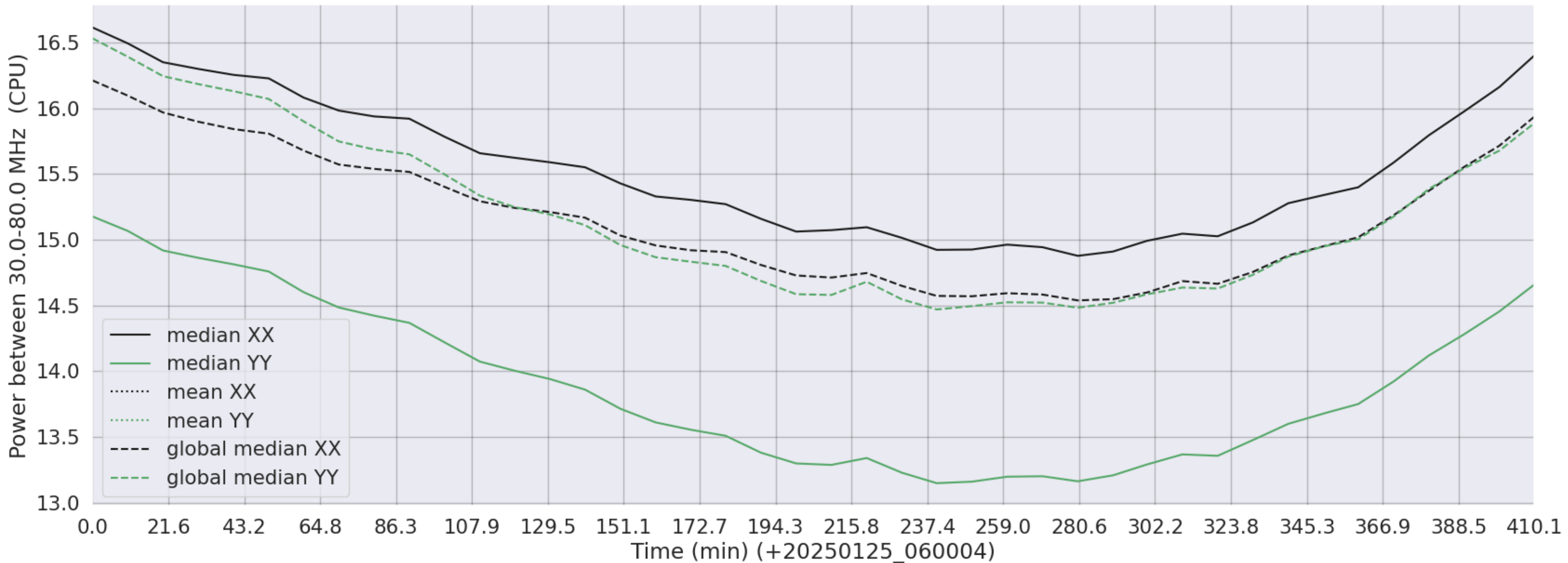
LWA093 - Correlator# 148 - XX FLAGS:Good - YY FLAGS:Good
