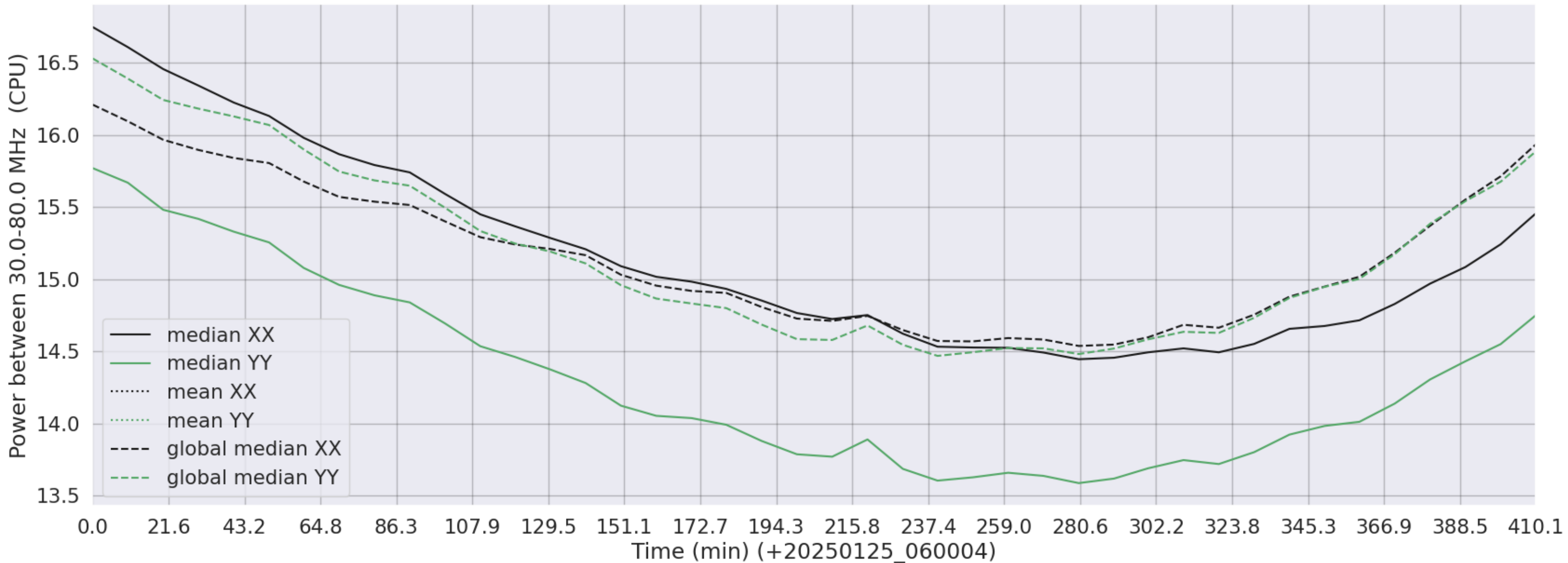
LWA274 - Correlator# 091 - XX FLAGS:Good - YY FLAGS:Good
