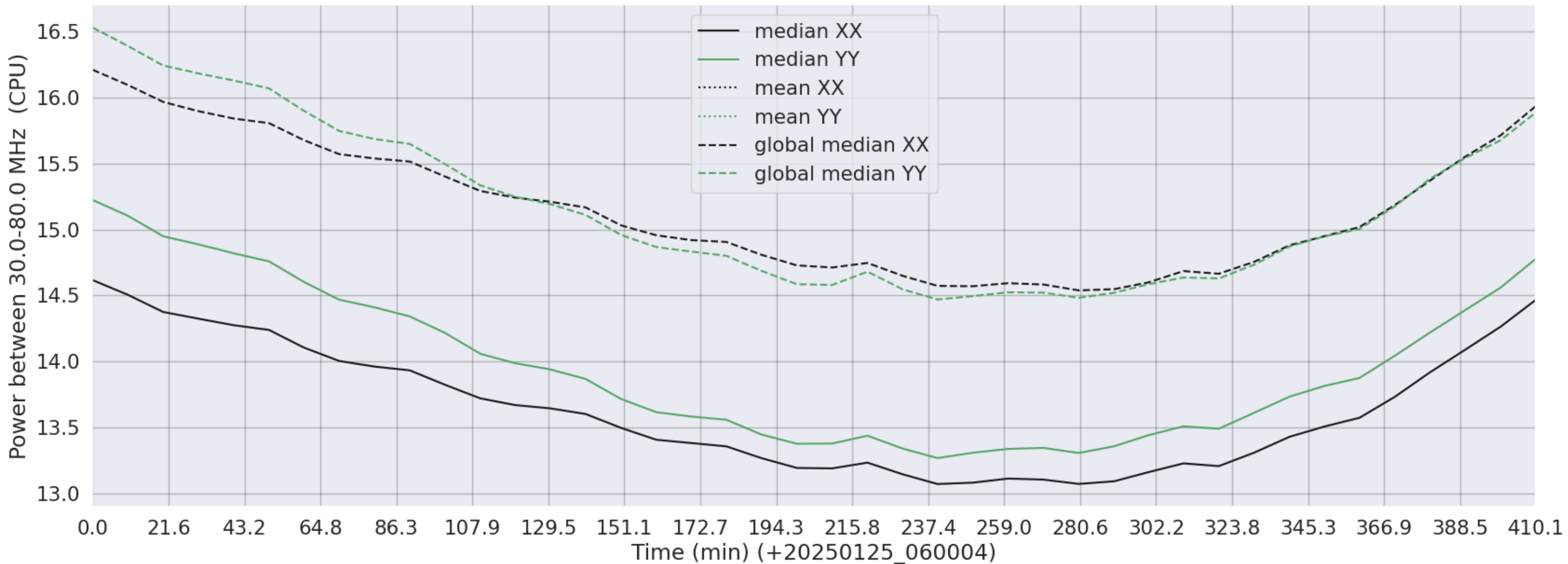
LWA217 - Correlator# 333 - XX FLAGS:Good - YY FLAGS:Good
