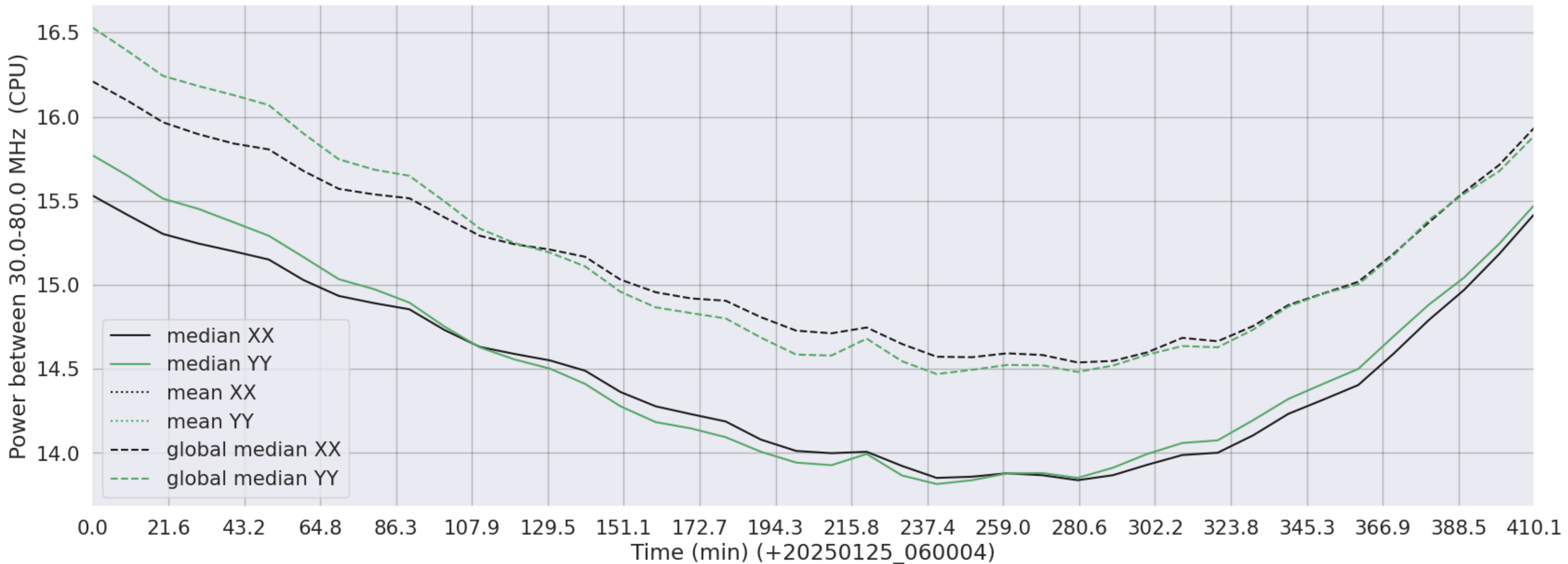
LWA248 - Correlator# 343 - XX FLAGS:Good - YY FLAGS:Good
