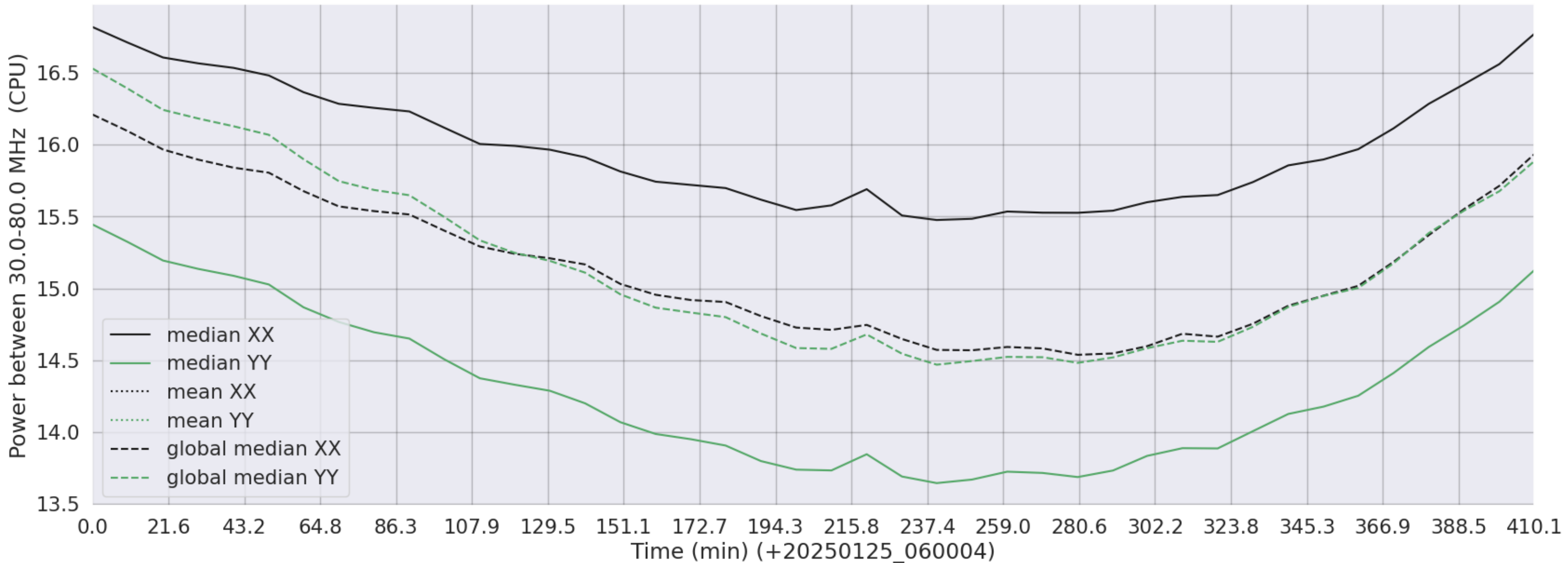
LWA107 - Correlator# 197 - XX FLAGS:Good - YY FLAGS:Good
