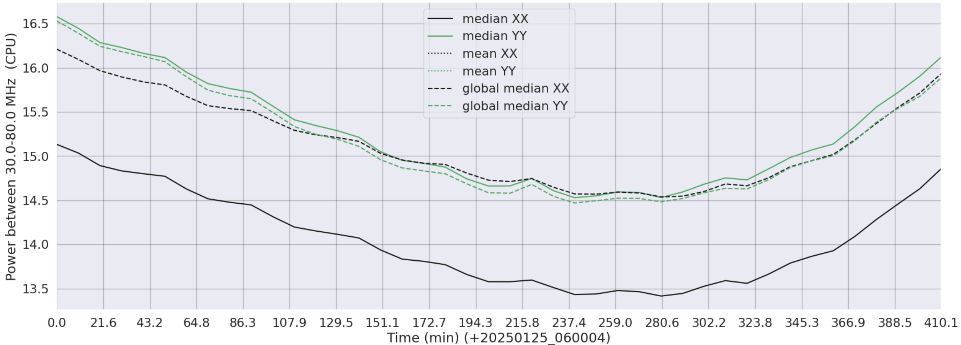
LWA182 - Correlator# 238 - XX FLAGS:Good - YY FLAGS:Good
