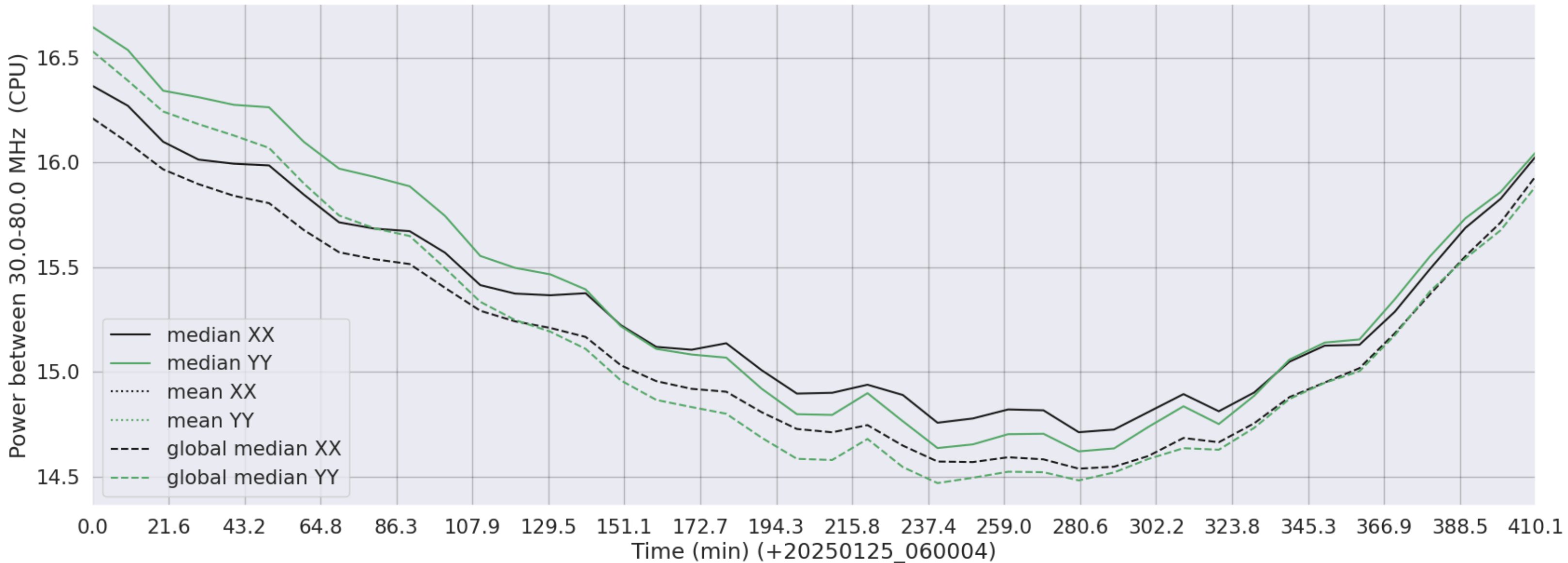
LWA116 - Correlator# 204 - XX FLAGS:Good - YY FLAGS:Good
