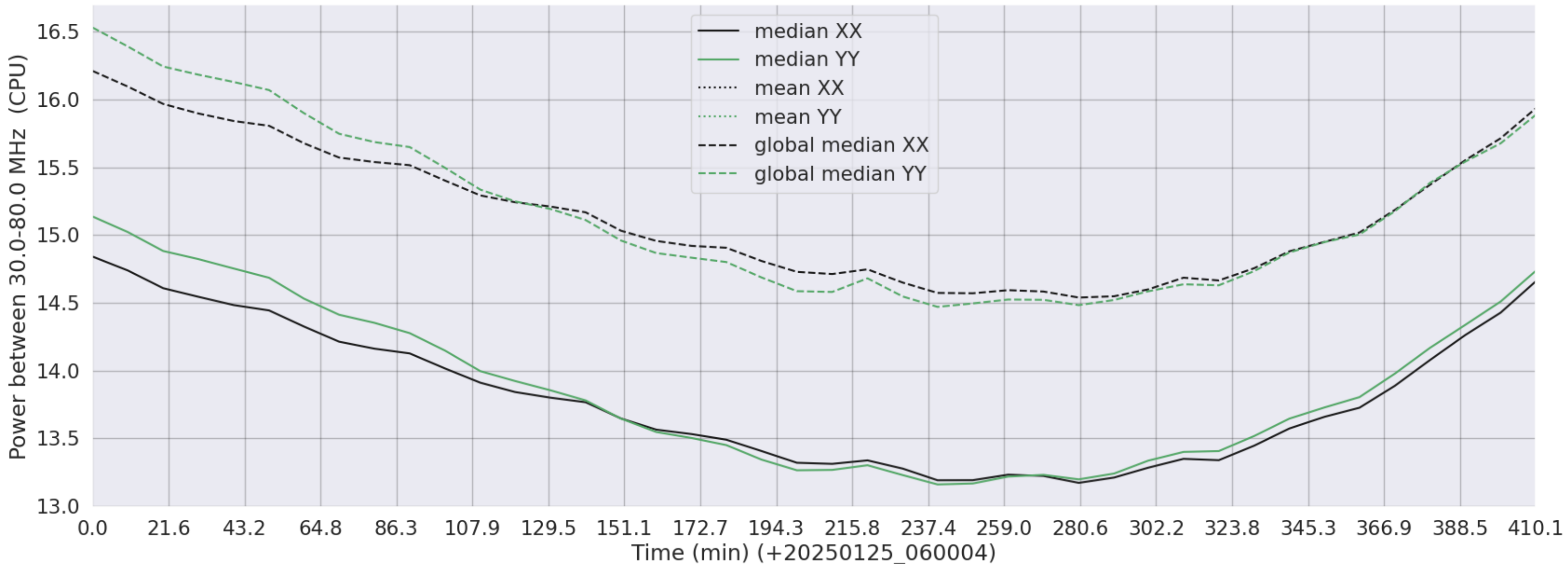
LWA122 - Correlator# 152 - XX FLAGS:Good - YY FLAGS:Good
