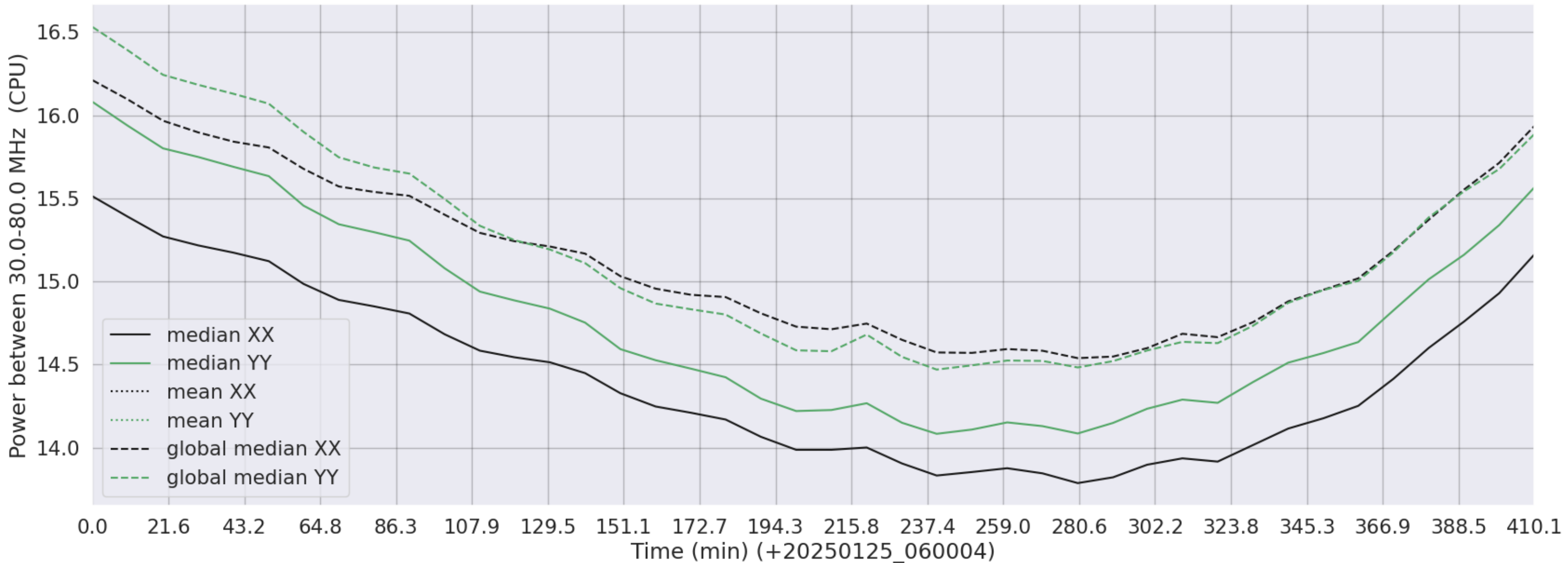
LWA030 - Correlator# 128 - XX FLAGS:Good - YY FLAGS:Good
