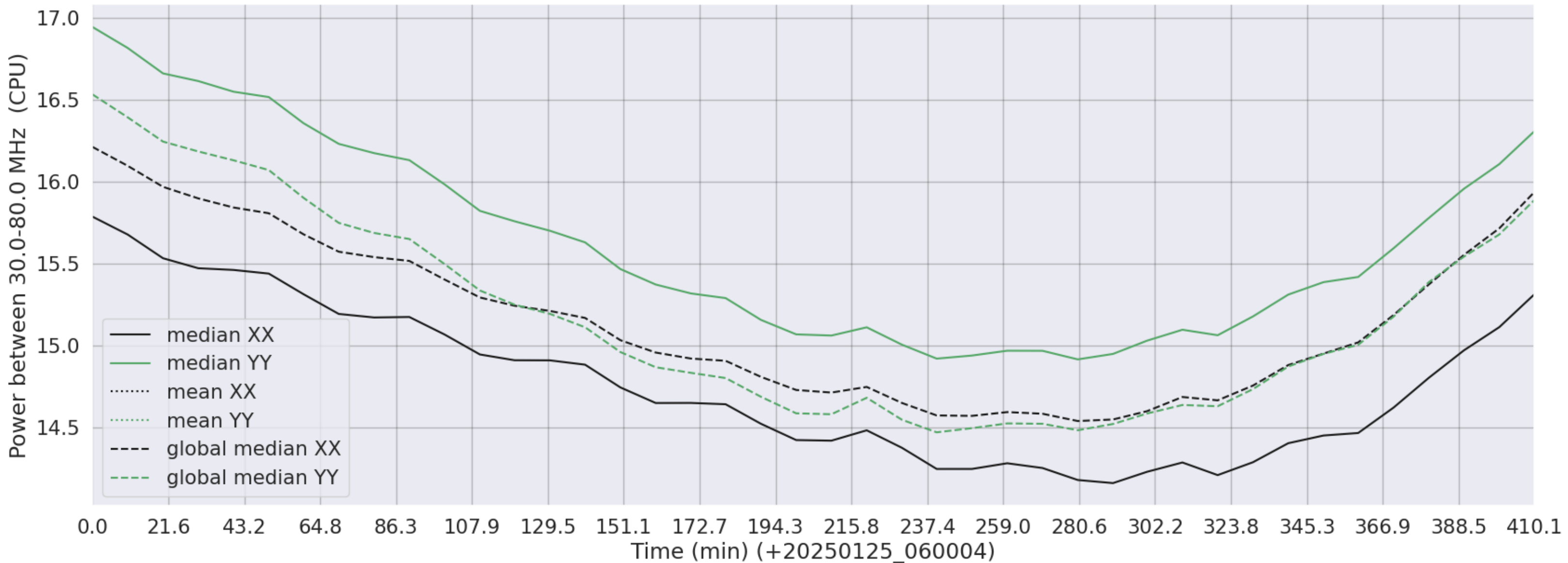
LWA118 - Correlator# 206 - XX FLAGS:Good - YY FLAGS:Good
