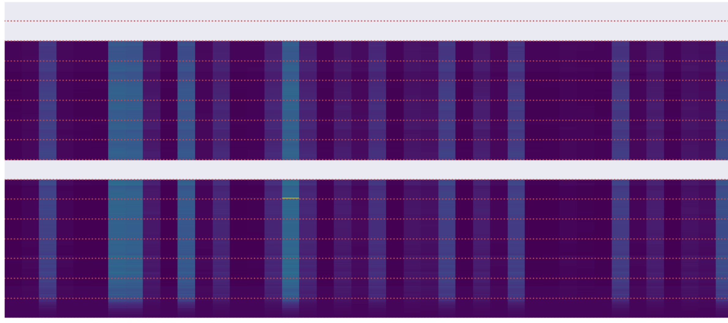
LWA124 - Correlator# 224 - XX - FLAGS: HighTimeVar
