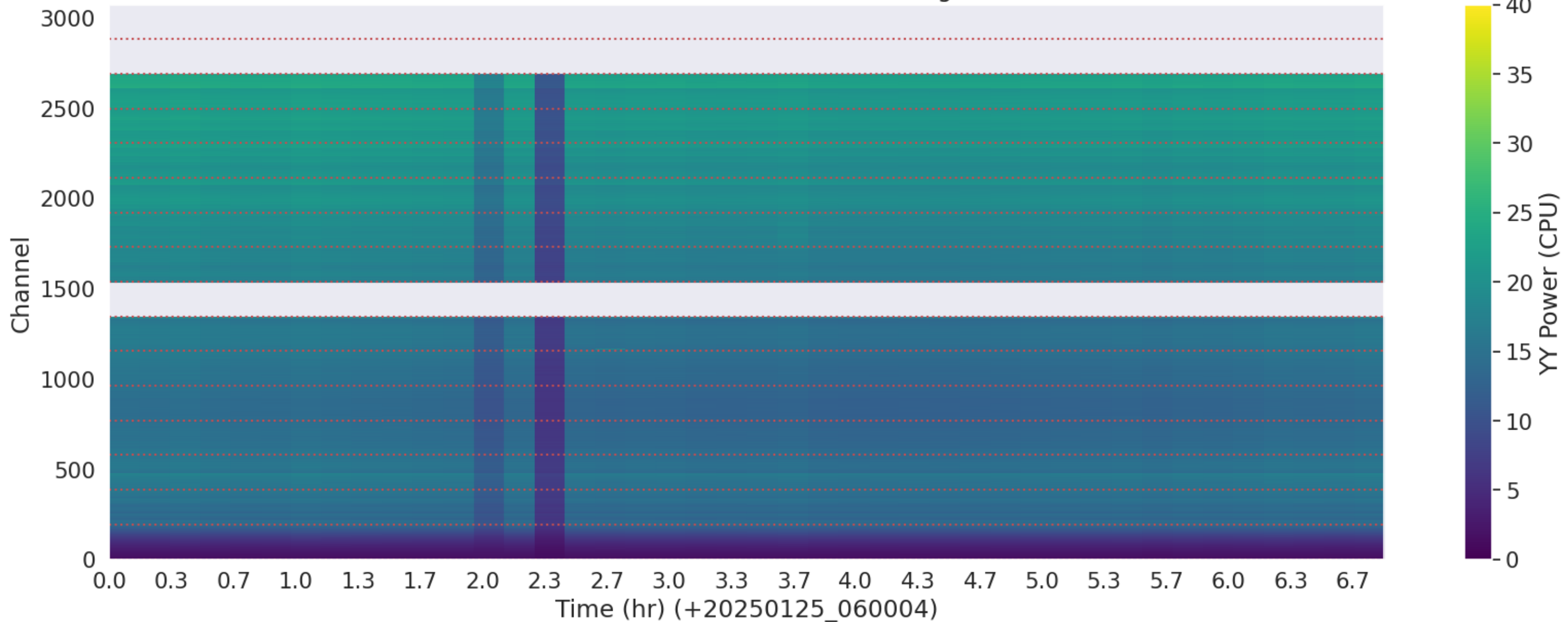
LWA065 - Correlator# 165 - YY - FLAGS: HighTimeVar
