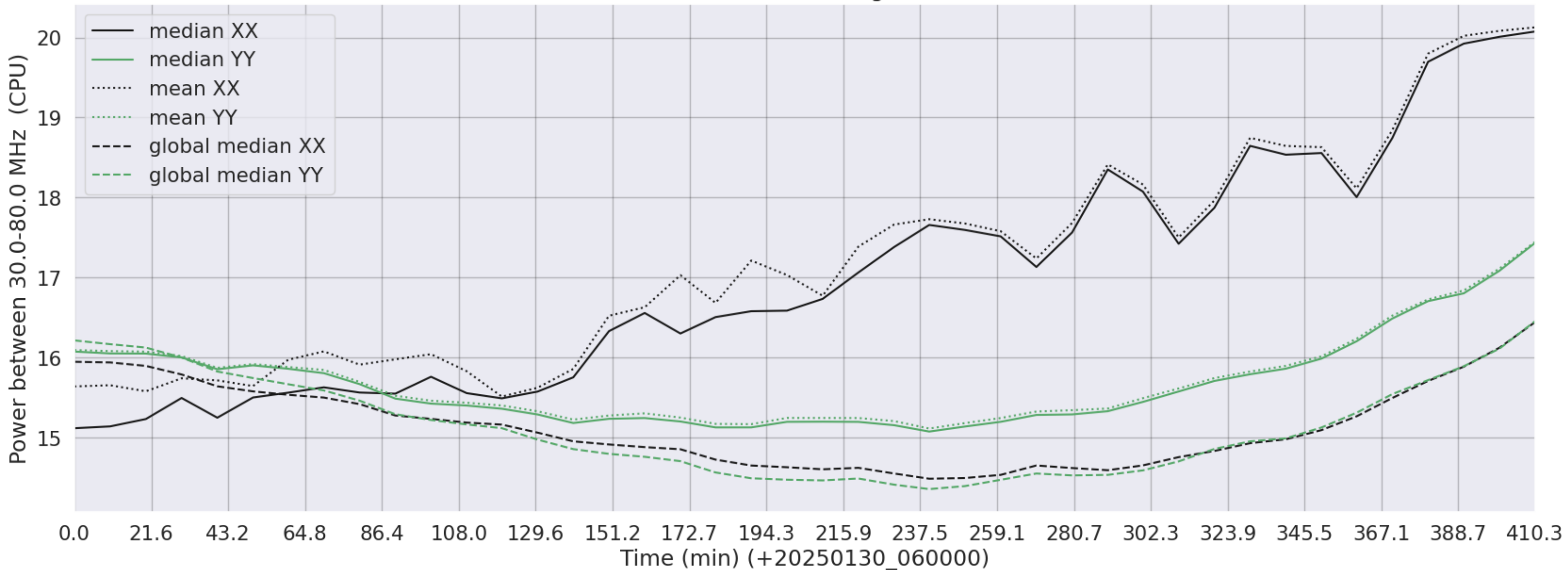
LWA272 - Correlator# 038 - XX FLAGS:HighTimeVar - YY FLAGS:Good
