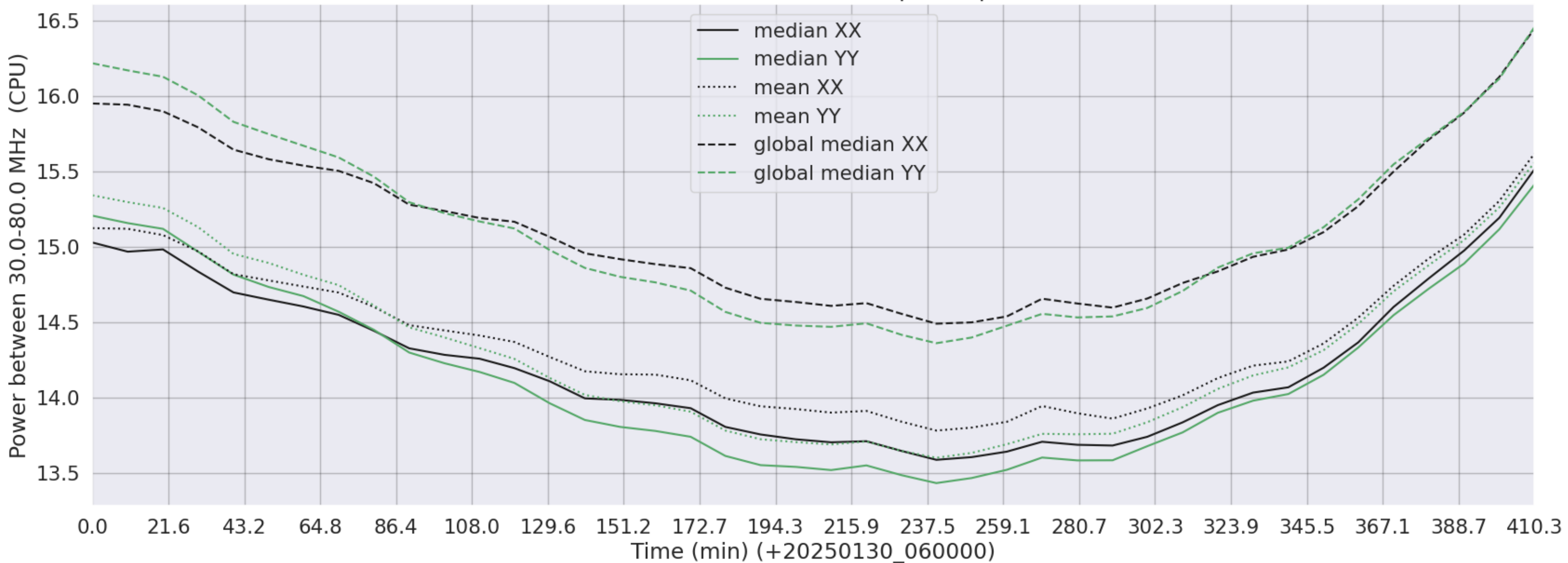
LWA012 - Correlator# 074 - XX FLAGS:BadSpecShape - YY FLAGS:Good
