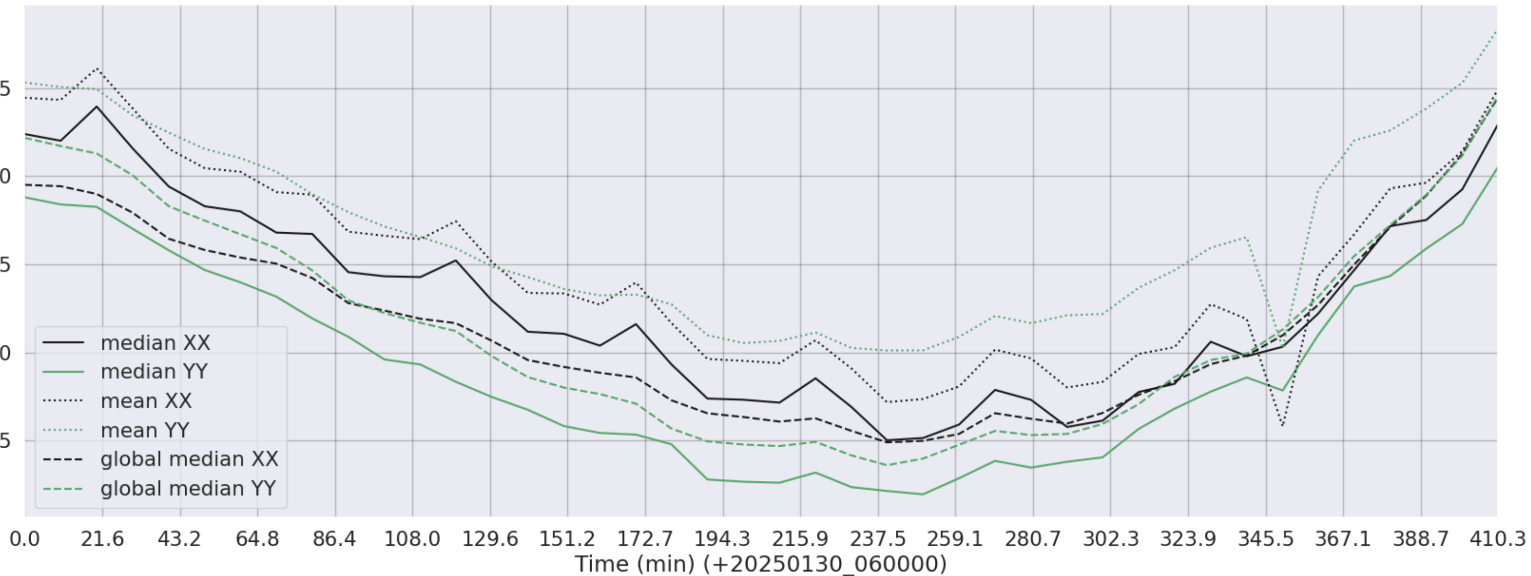
LWA336 - Correlator# 056 - XX FLAGS:Good - YY FLAGS:Good
