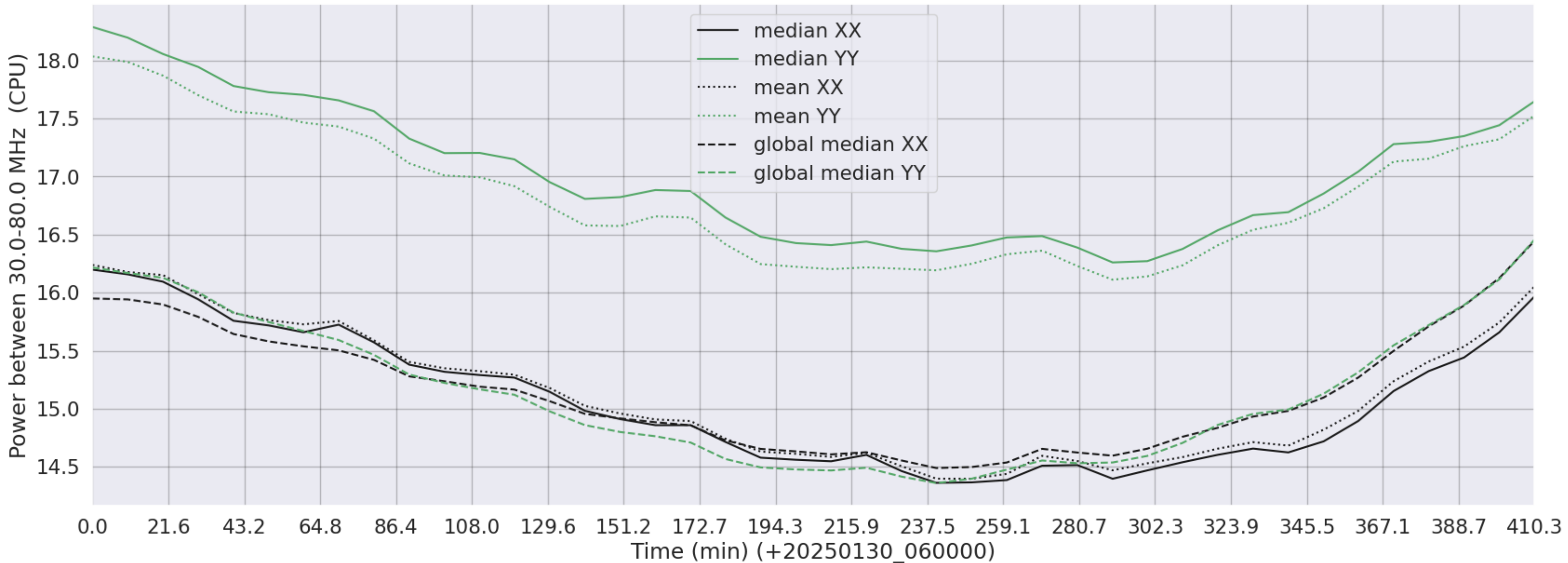
LWA302 - Correlator# 092 - XX FLAGS:Good - YY FLAGS:Good
