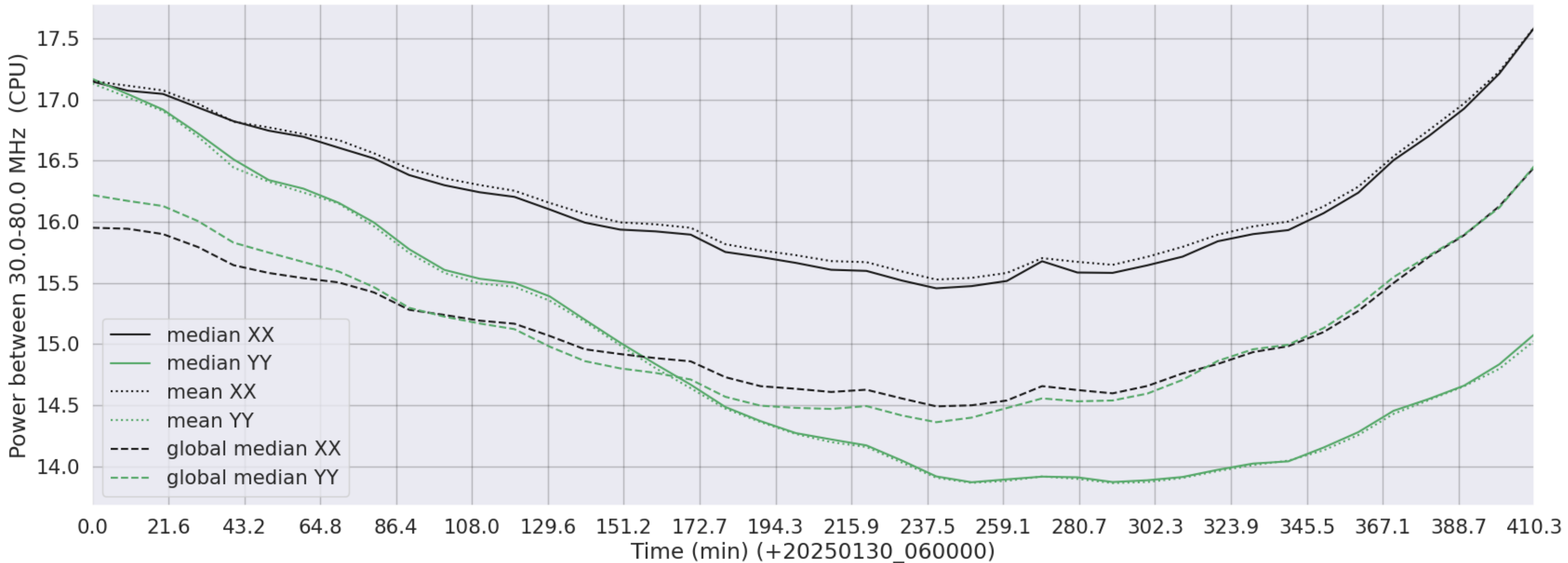
LWA359 - Correlator# 254 - XX FLAGS:Good - YY FLAGS:Good
