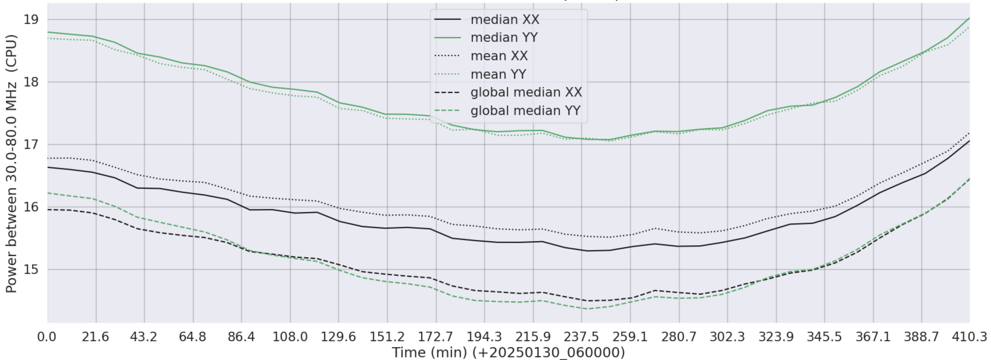
LWA097 - Correlator# 170 - XX FLAGS:BadSpecShape - YY FLAGS:Good
