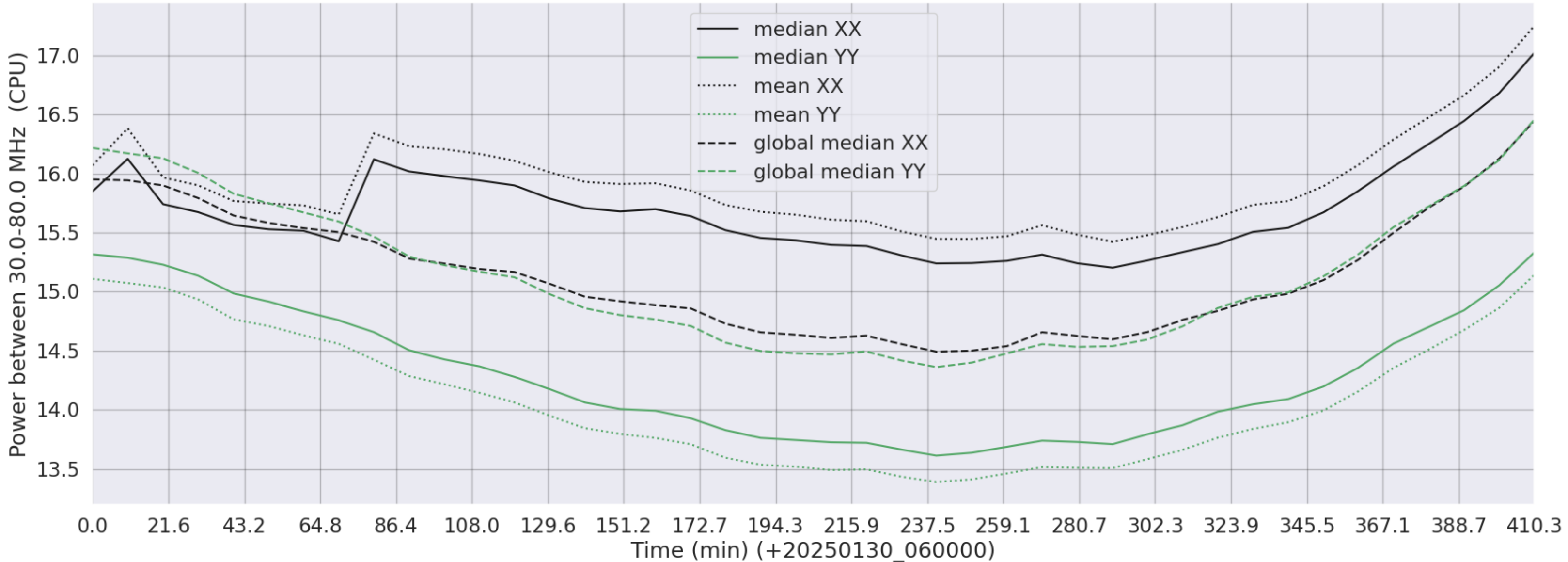
LWA071 - Correlator# 084 - XX FLAGS:Good - YY FLAGS:BadSpecShape
