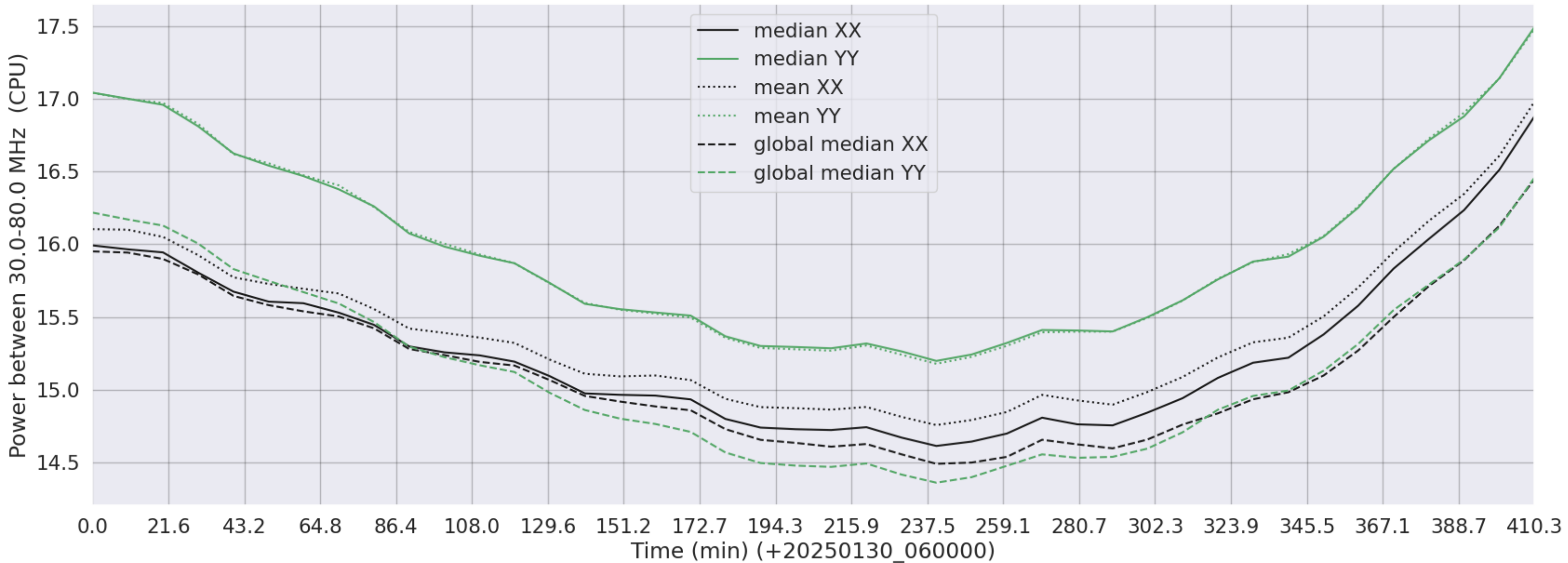
LWA044 - Correlator# 080 - XX FLAGS:Good - YY FLAGS:Good
