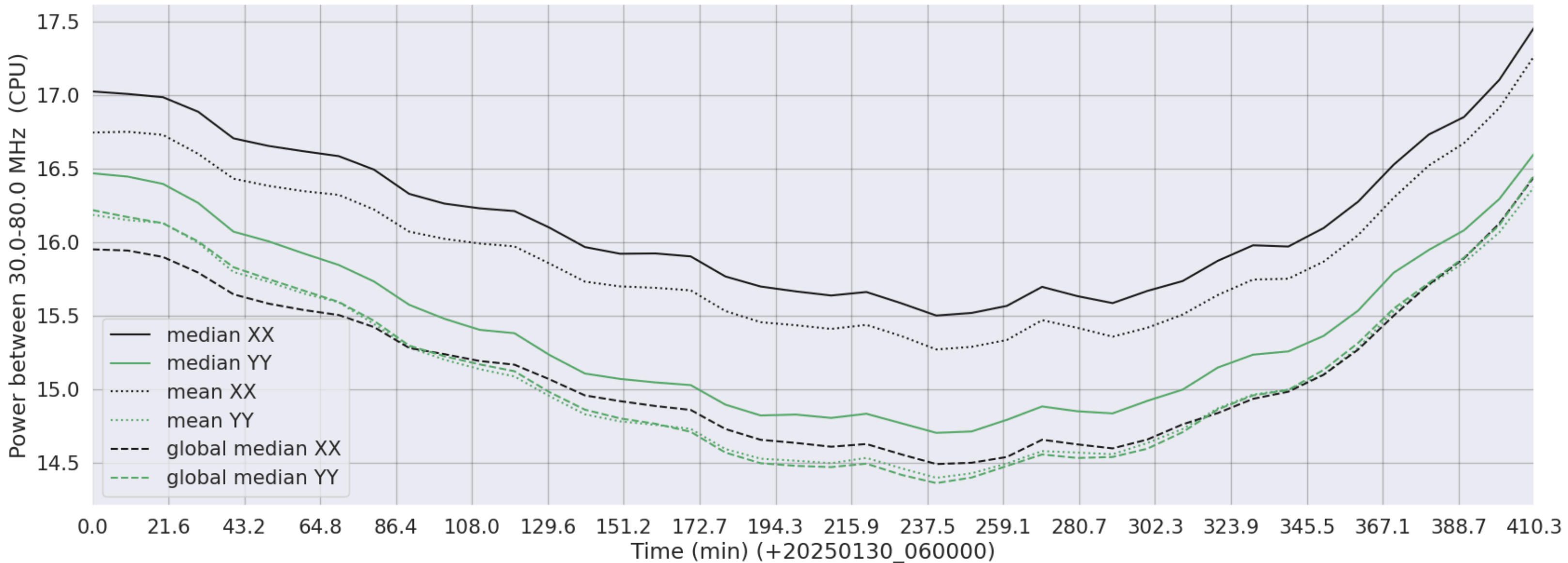
LWA108 - Correlator# 196 - XX FLAGS:Good - YY FLAGS:Good
