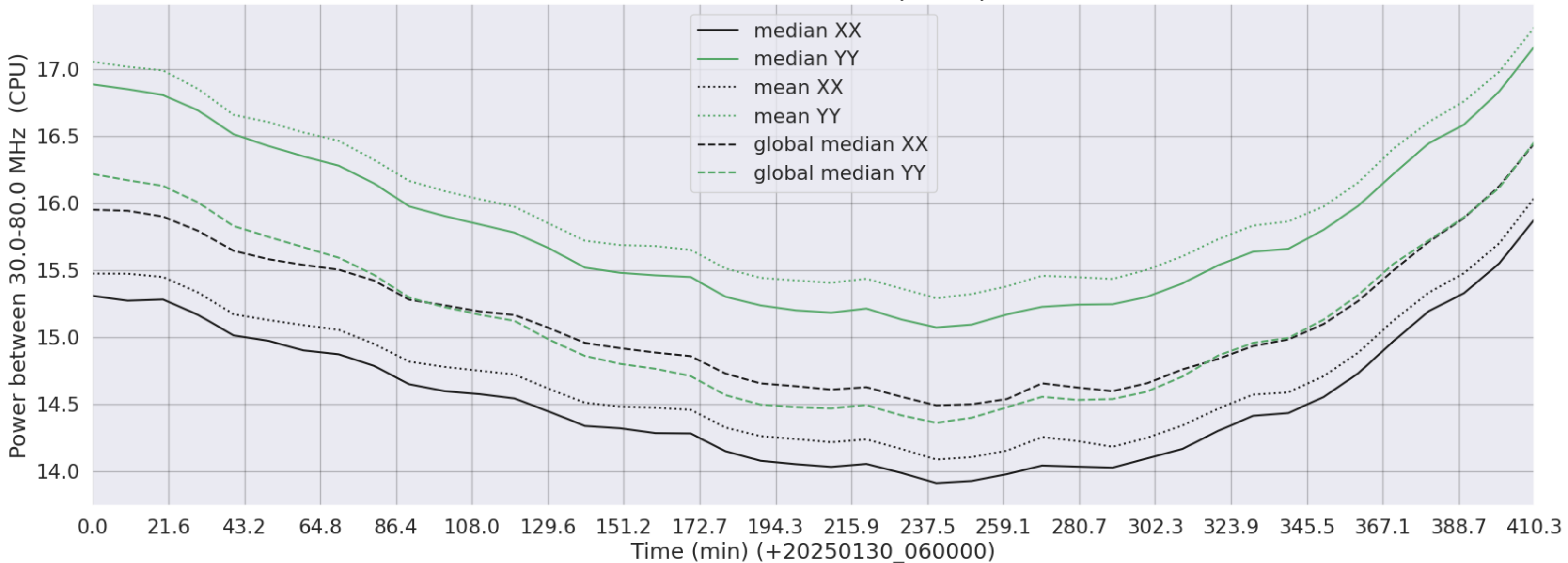
LWA239 - Correlator# 313 - XX FLAGS:BadSpecShape - YY FLAGS:Good
