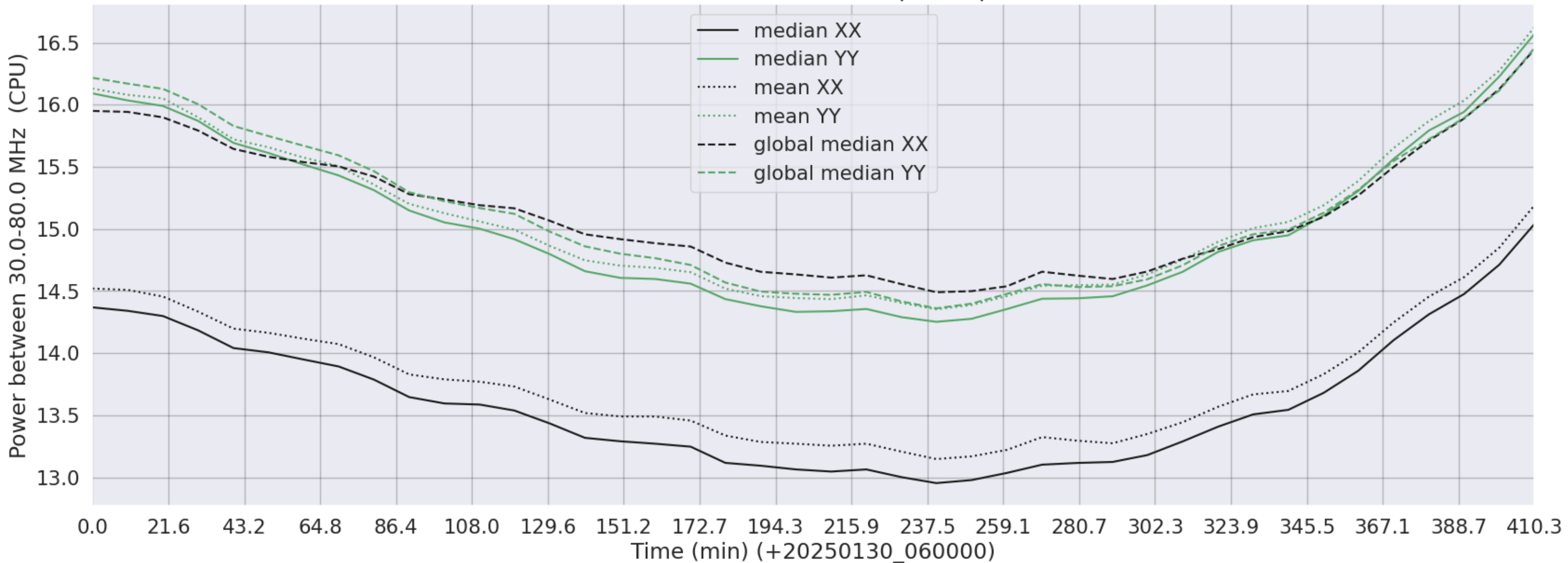
LWA245 - Correlator# 341 - XX FLAGS:BadSpecShape - YY FLAGS:Good
