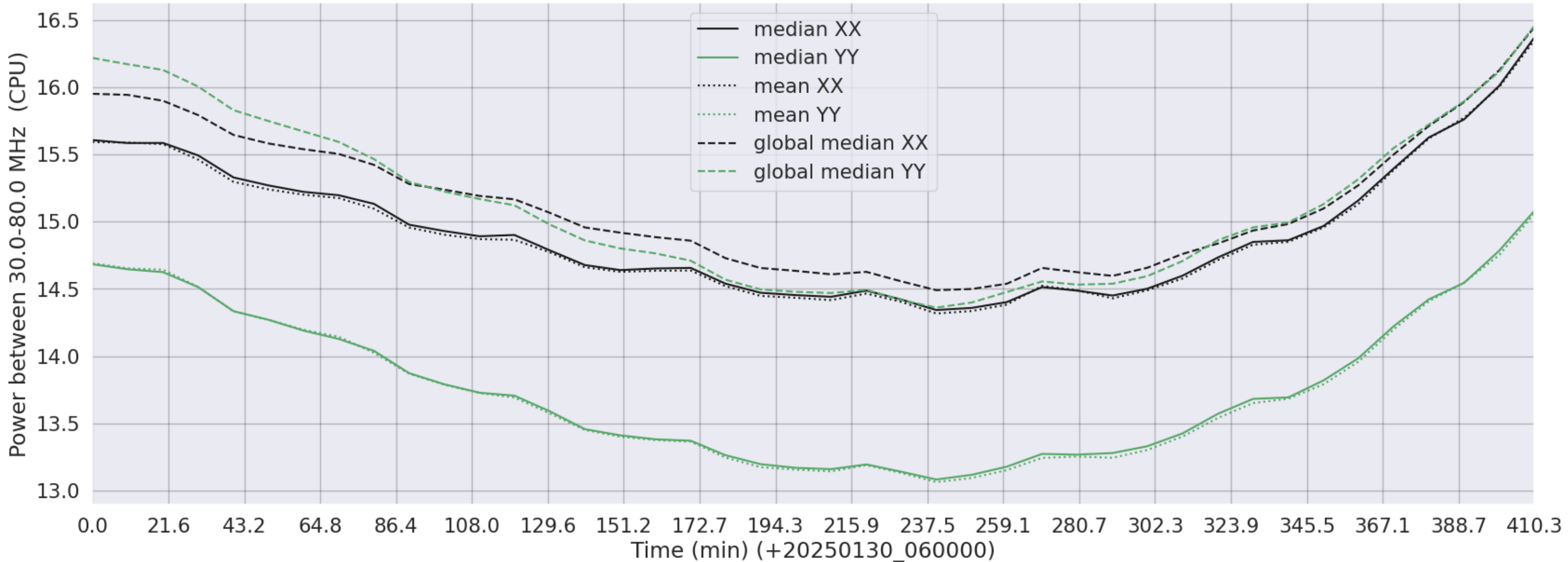
LWA208 - Correlator# 298 - XX FLAGS:Good - YY FLAGS:BadSpecShape
