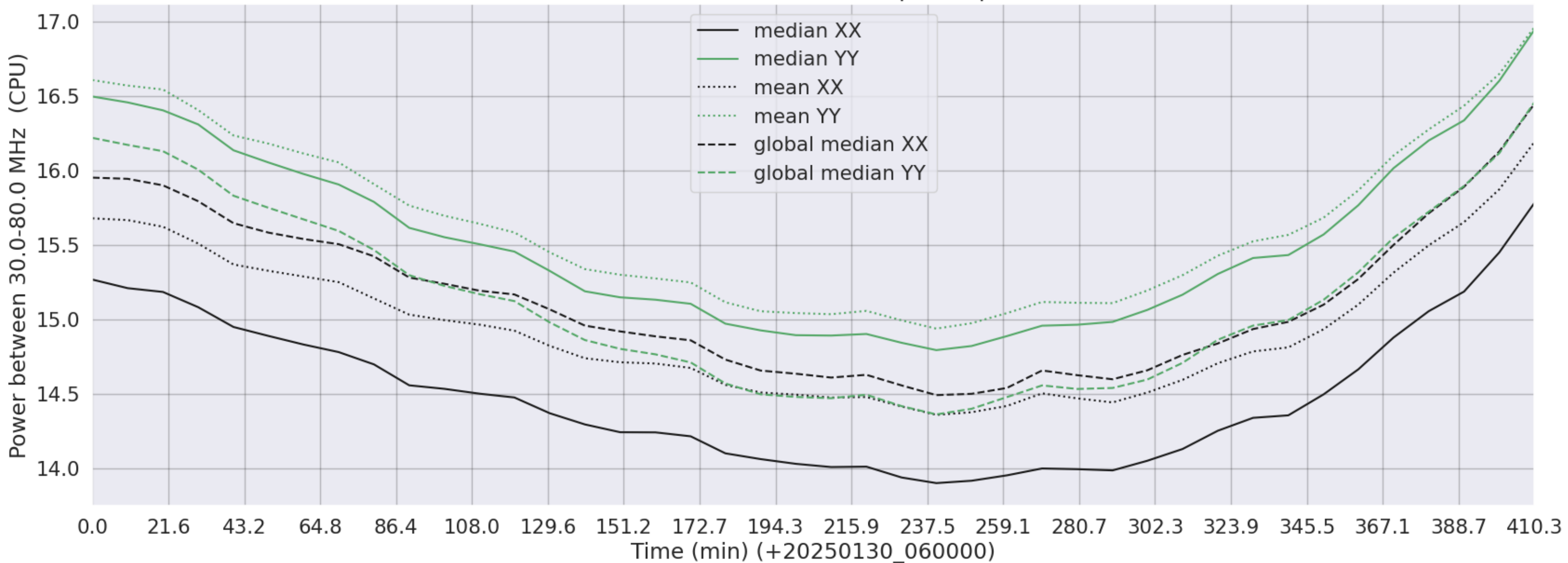
LWA200 - Correlator# 276 - XX FLAGS:BadSpecShape - YY FLAGS:Good
