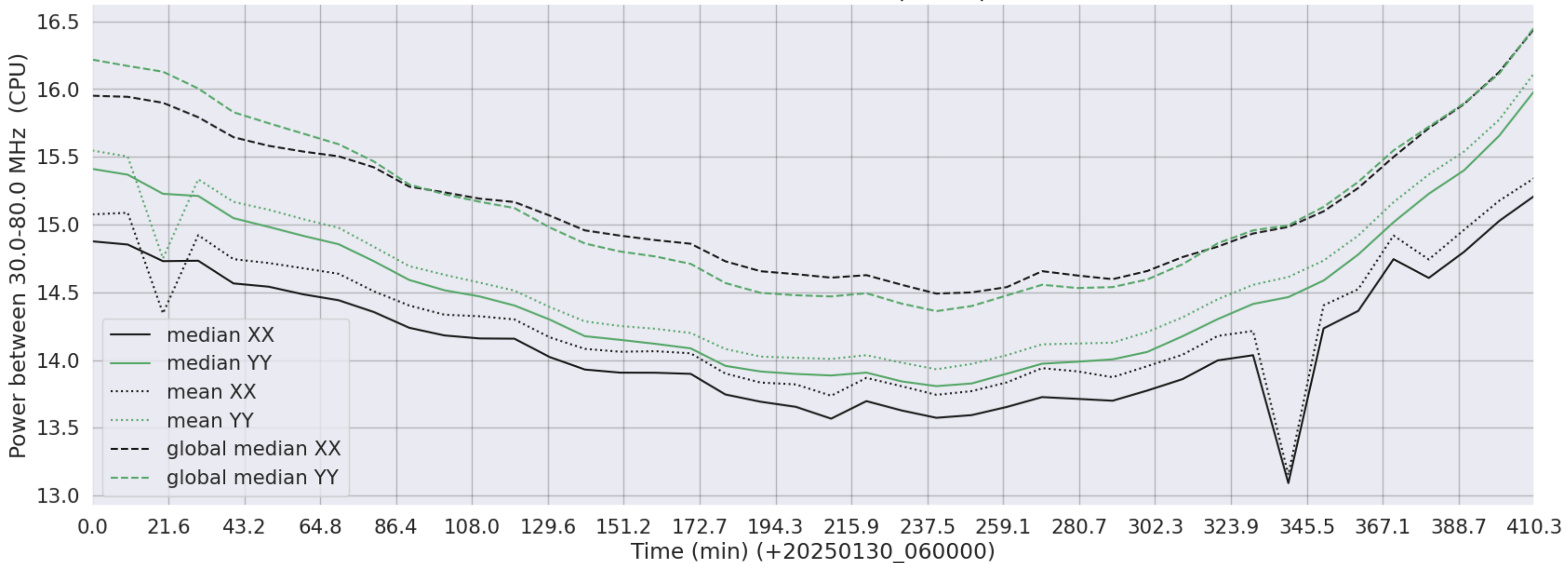
LWA243 - Correlator# 330 - XX FLAGS:BadSpecShape - YY FLAGS:Good
