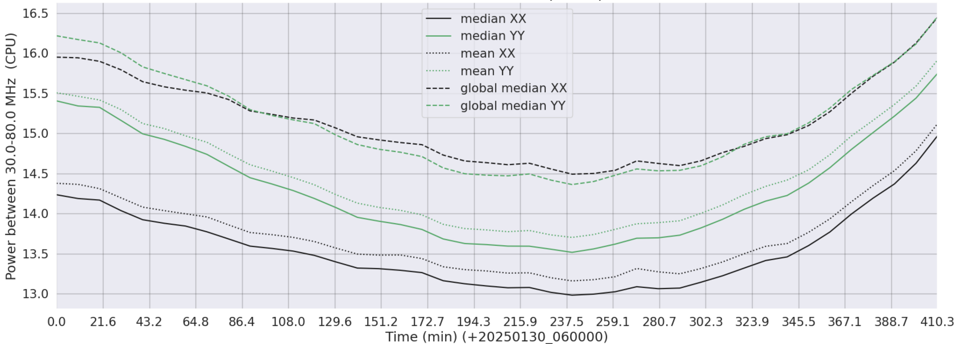
LWA047 - Correlator# 085 - XX FLAGS:BadSpecShape - YY FLAGS:Good
