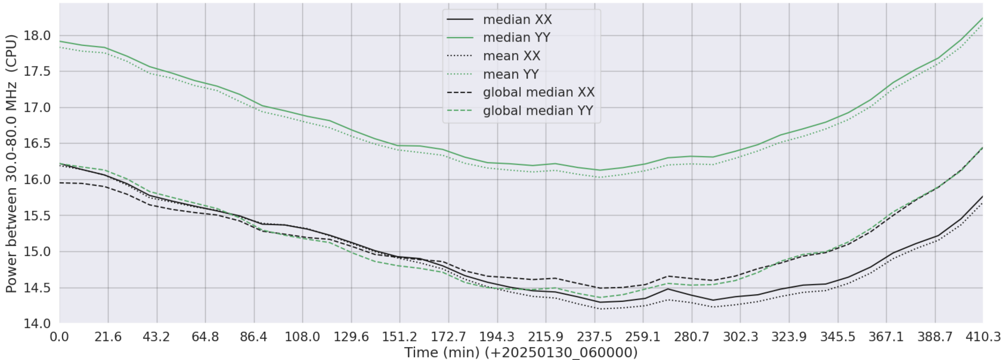
LWA276 - Correlator# 006 - XX FLAGS:Good - YY FLAGS:Good
