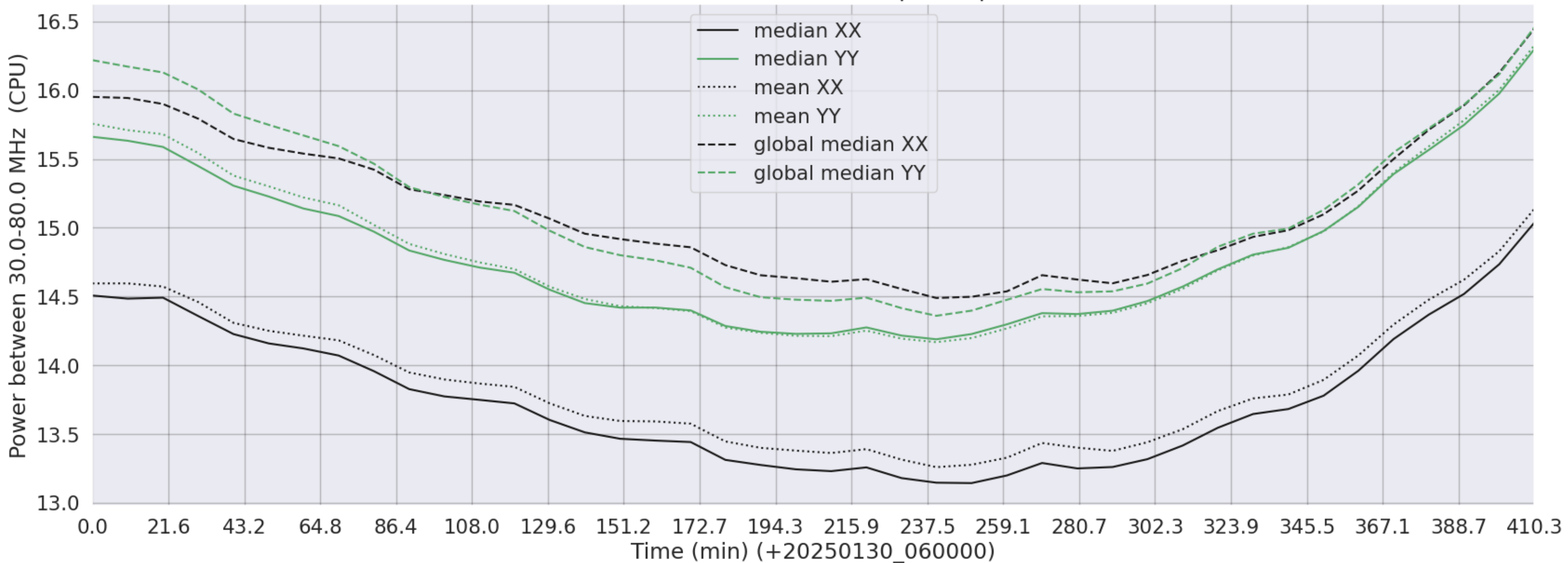
LWA072 - Correlator# 171 - XX FLAGS:BadSpecShape - YY FLAGS:Good
