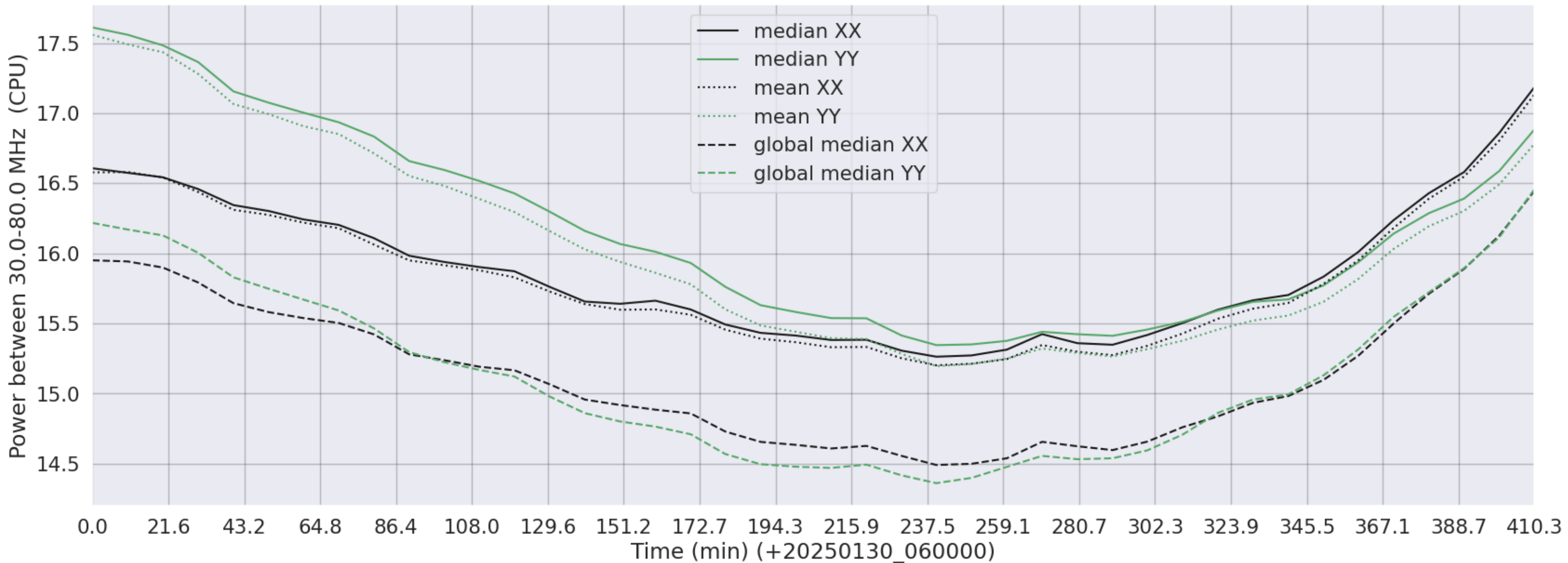
LWA266 - Correlator# 000 - XX FLAGS:Good - YY FLAGS:Good
