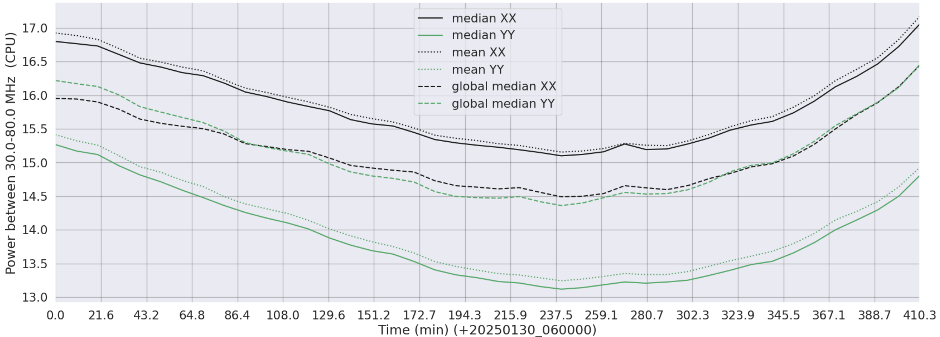
LWA350 - Correlator# 319 - XX FLAGS:Good - YY FLAGS:Good
