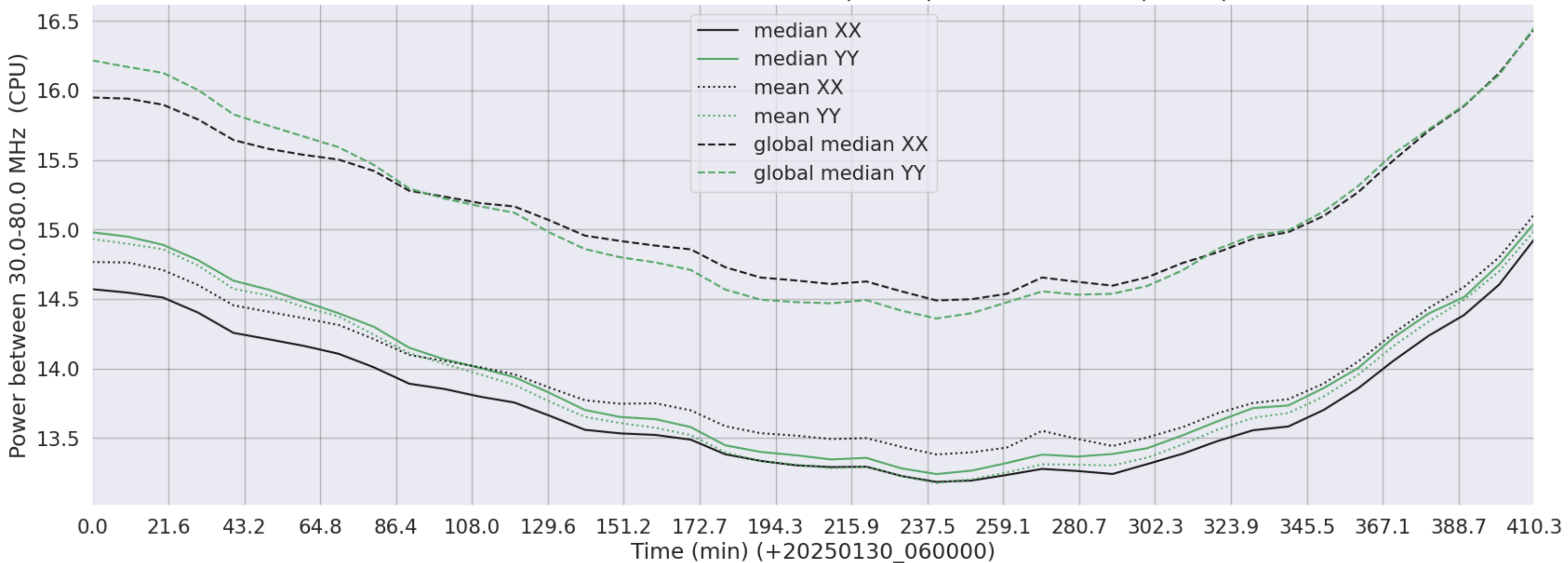
LWA021 - Correlator# 105 - XX FLAGS:BadSpecShape - YY FLAGS:BadSpecShape
