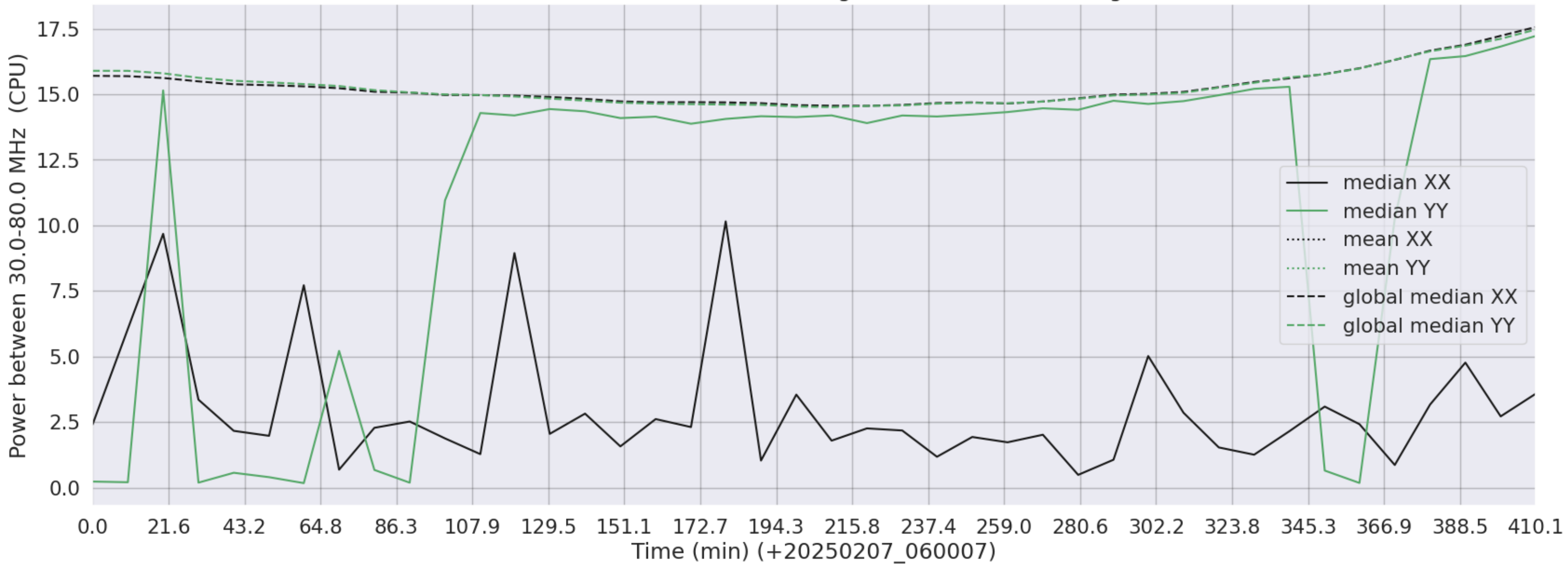
LWA124 - Correlator# 224 - XX FLAGS:HighTimeVar - YY FLAGS:HighTimeVar
