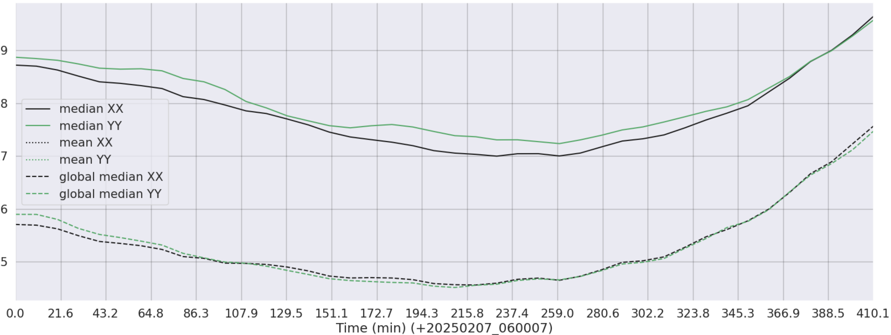
LWA297 - Correlator# 314 - XX FLAGS:Good - YY FLAGS:Good
