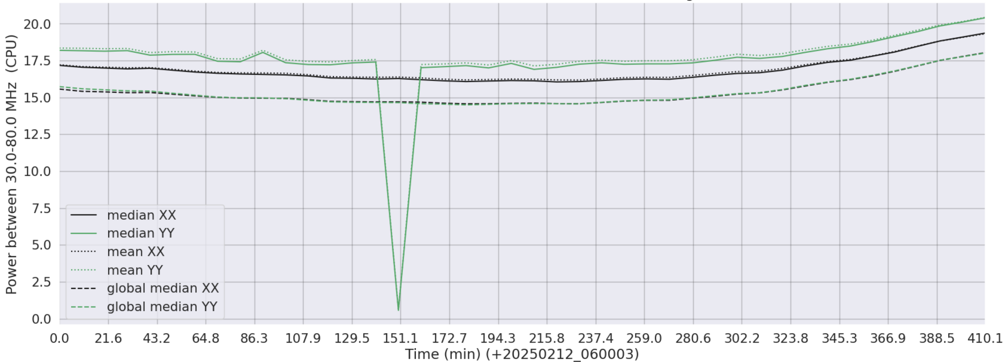
LWA065 - Correlator# 165 - XX FLAGS:Good - YY FLAGS:HighTimeVar
