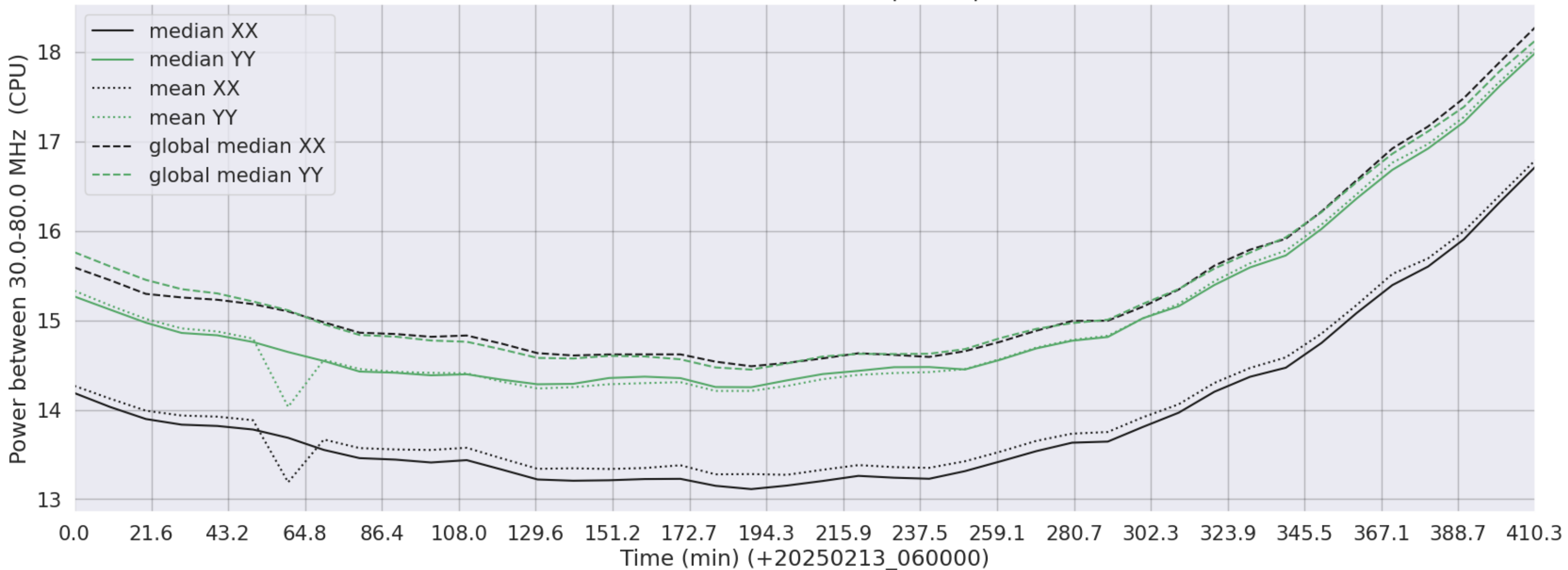
LWA072 - Correlator# 171 - XX FLAGS:BadSpecShape - YY FLAGS:Good
