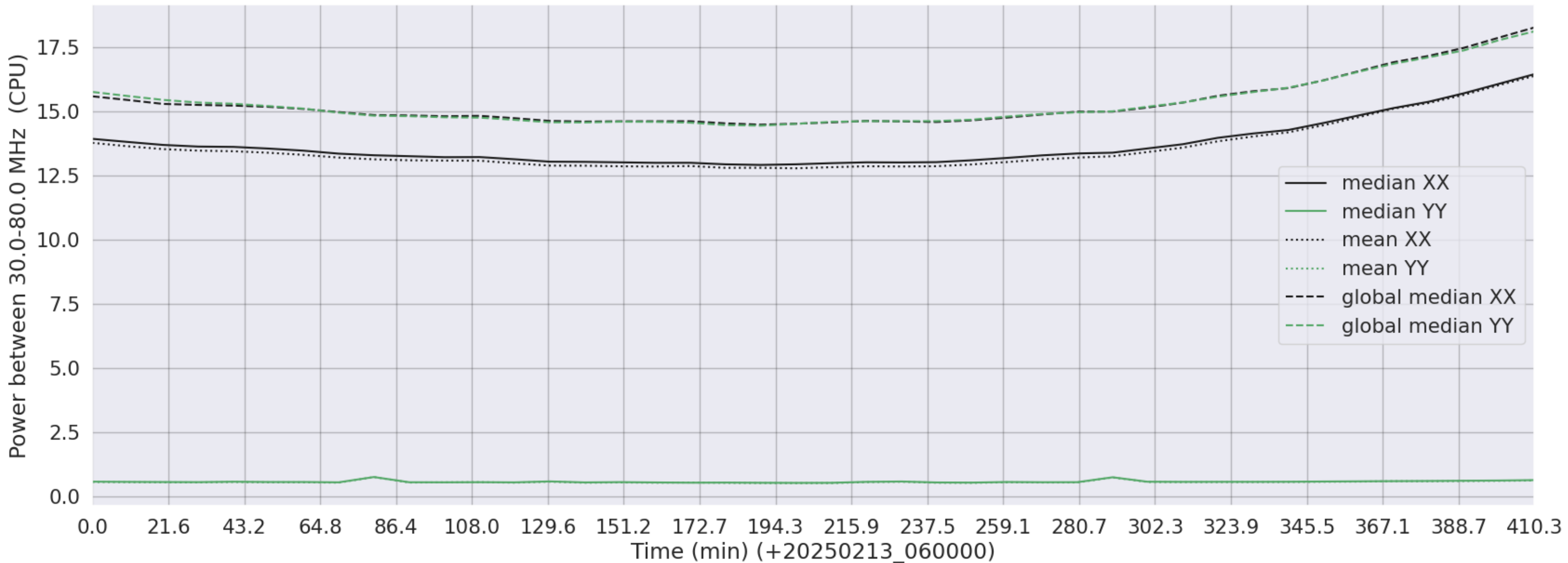
LWA190 - Correlator# 244 - XX FLAGS:Good - YY FLAGS:LowPower
