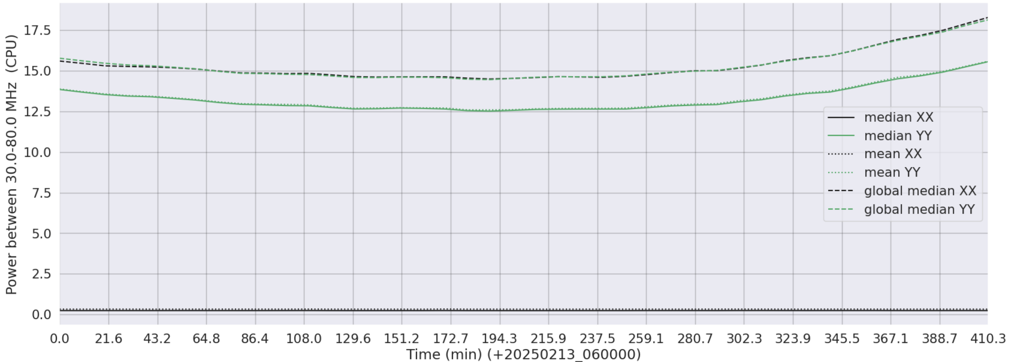
LWA110 - Correlator# 198 - XX FLAGS:LowPower - YY FLAGS:Good
