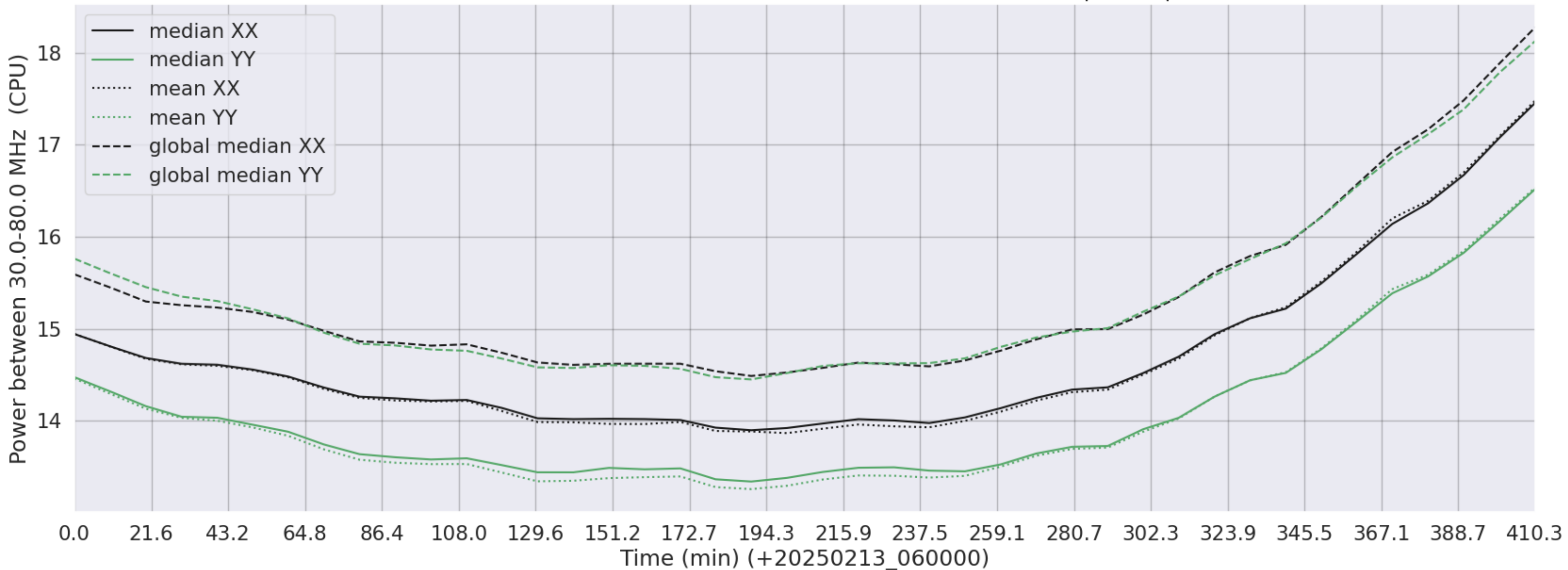
LWA139 - Correlator# 187 - XX FLAGS:Good - YY FLAGS:BadSpecShape
