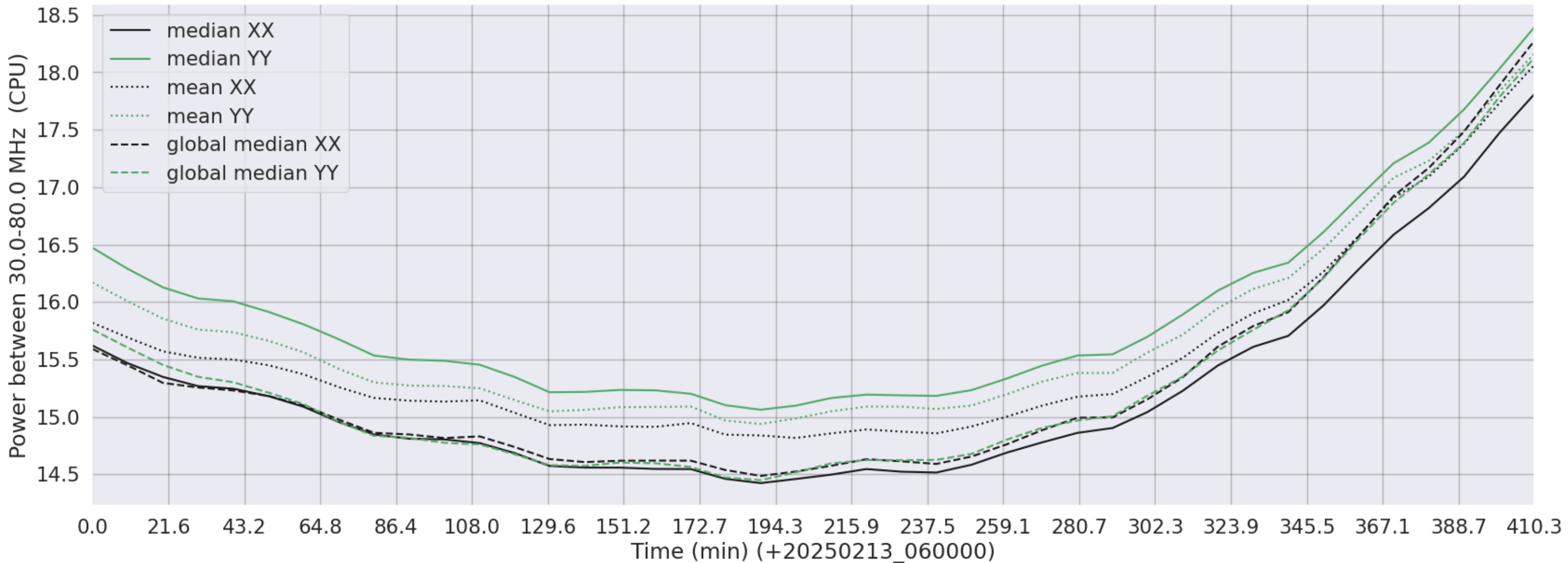
LWA163 - Correlator# 264 - XX FLAGS:Good - YY FLAGS:Good
