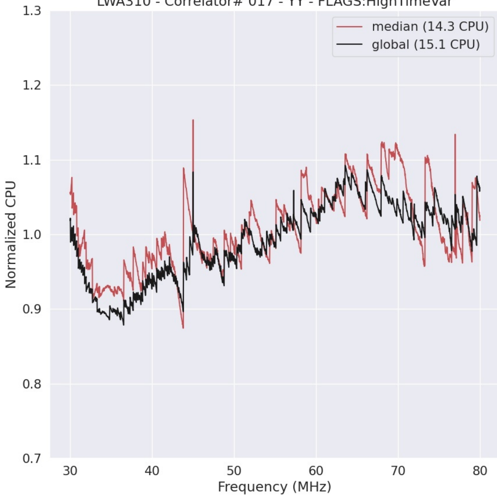
LWA310 - Correlator# 017 - YY - FLAGS:HighTimeVar
