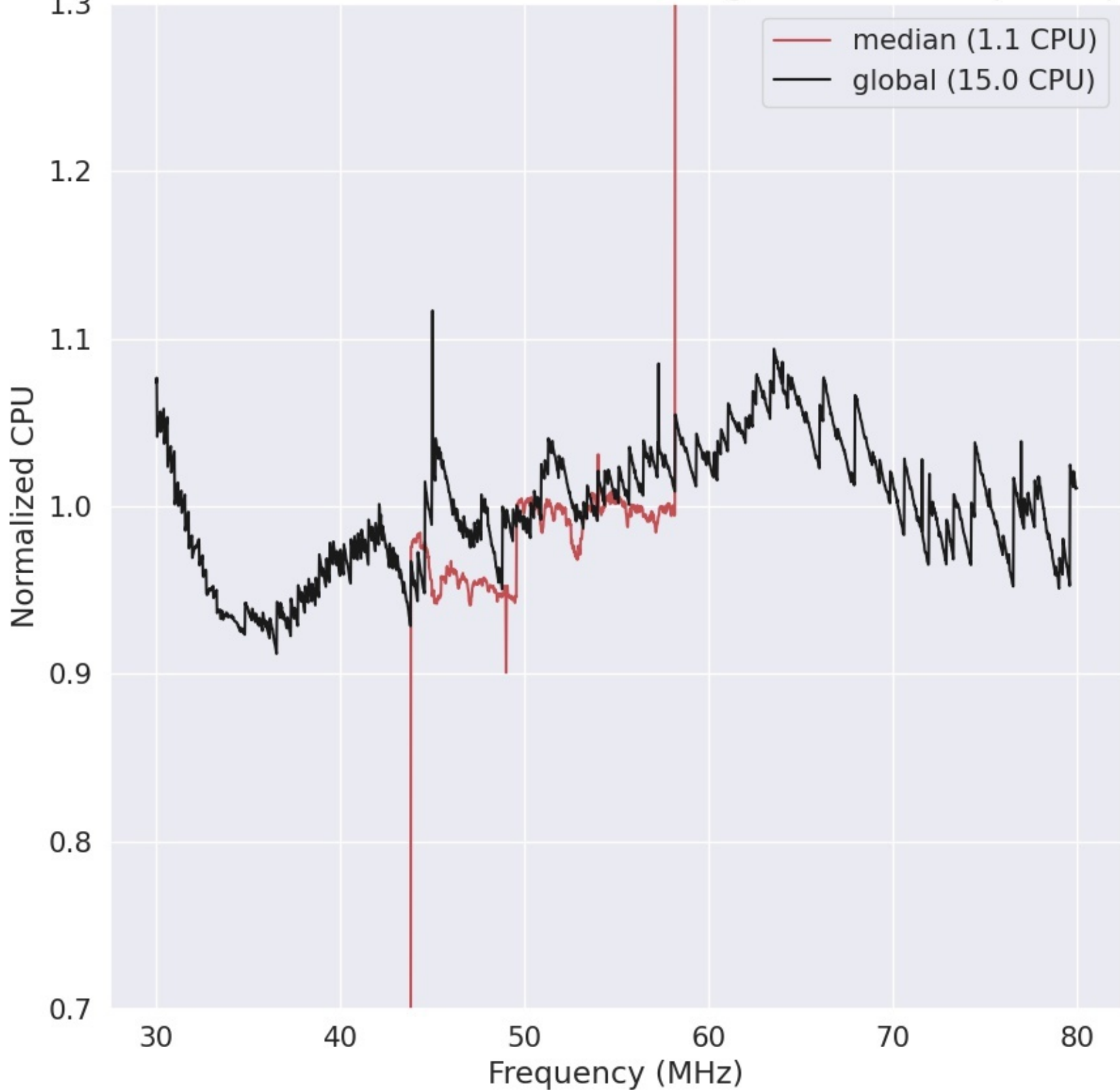
LWA288 - Correlator# 042 - YY - FLAGS:HighTimeVar+BadSpecShape
