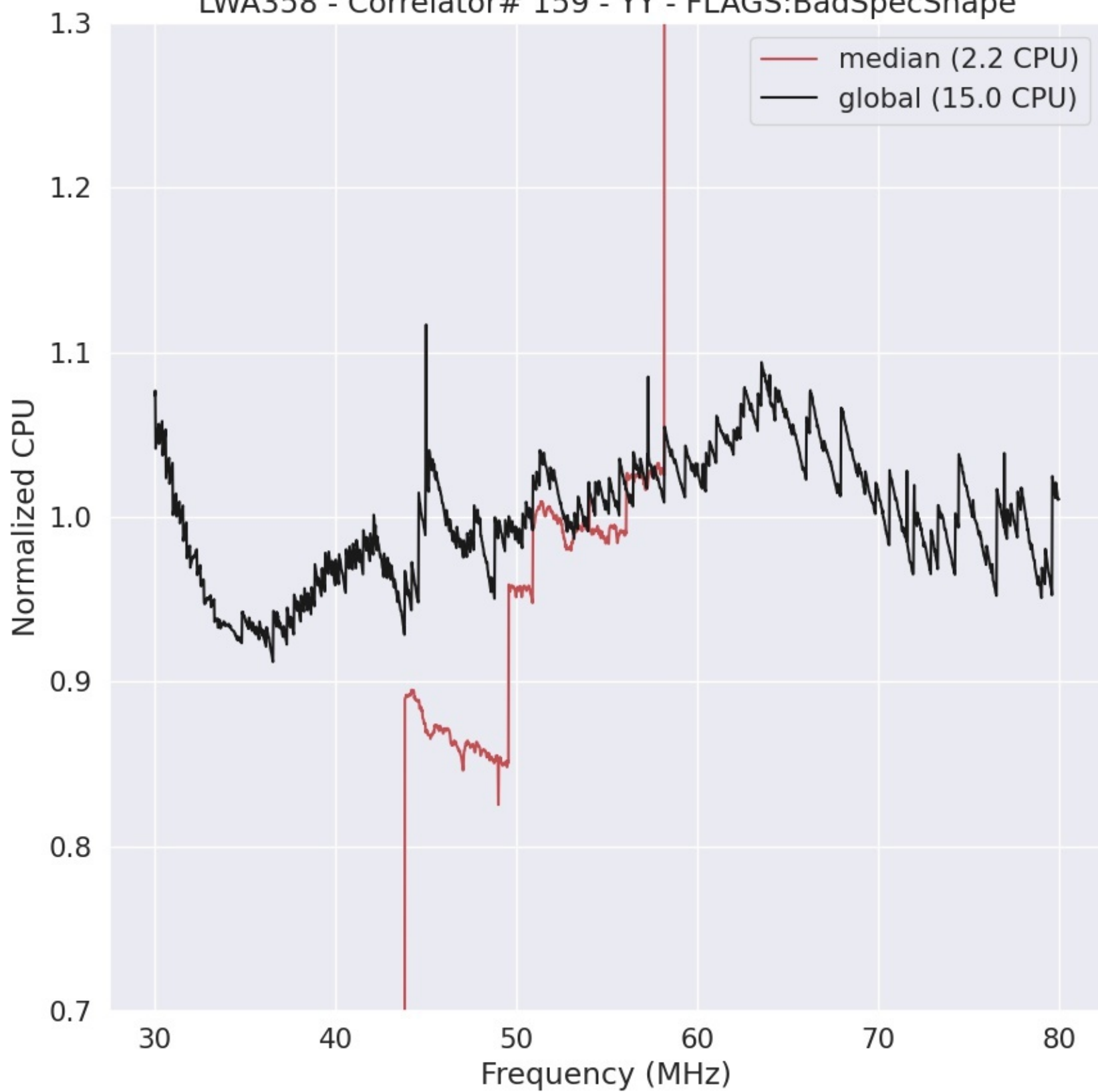
LWA358 - Correlator# 159 - YY - FLAGS:BadSpecShape
