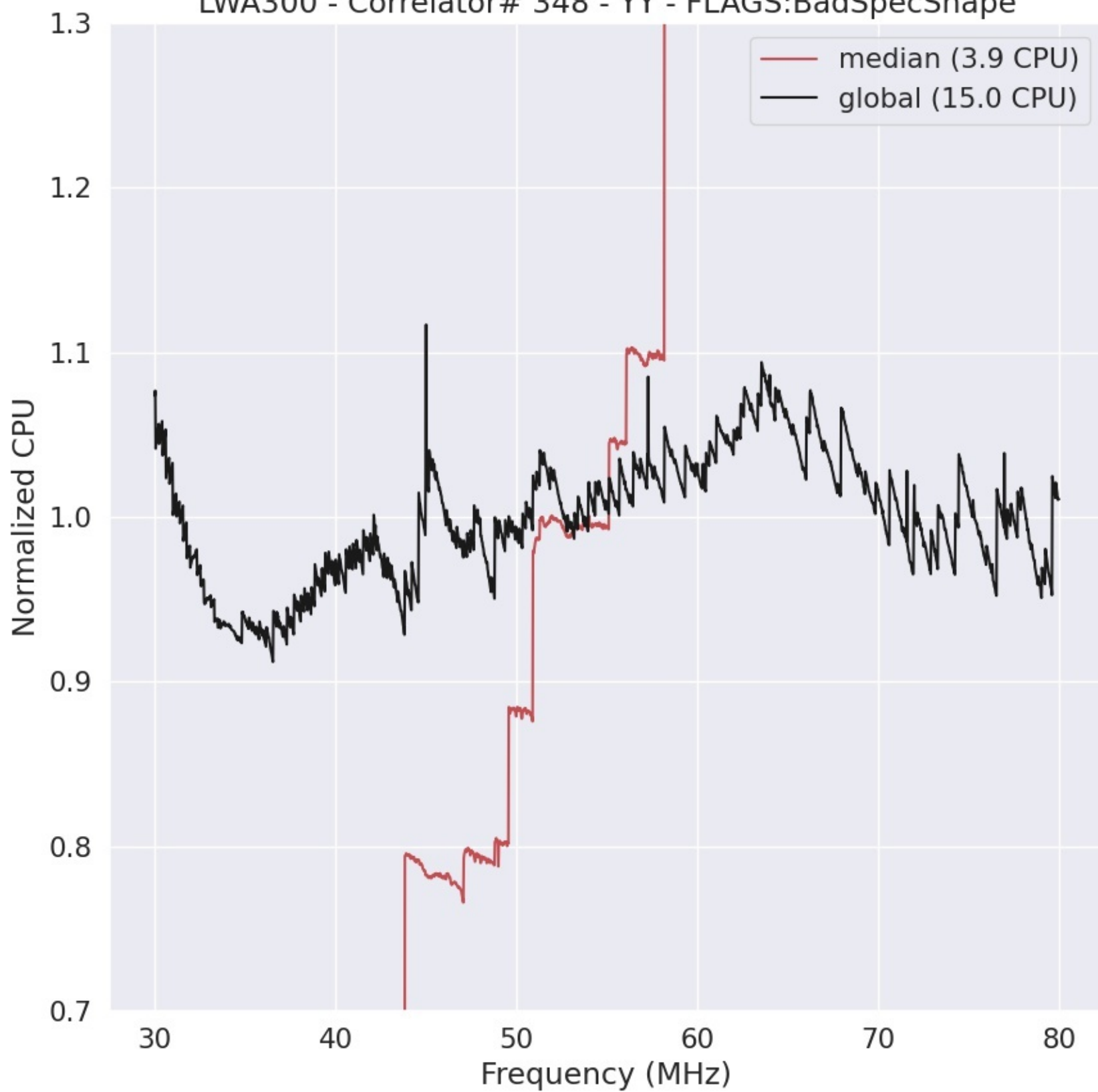
LWA300 - Correlator# 348 - YY - FLAGS:BadSpecShape
