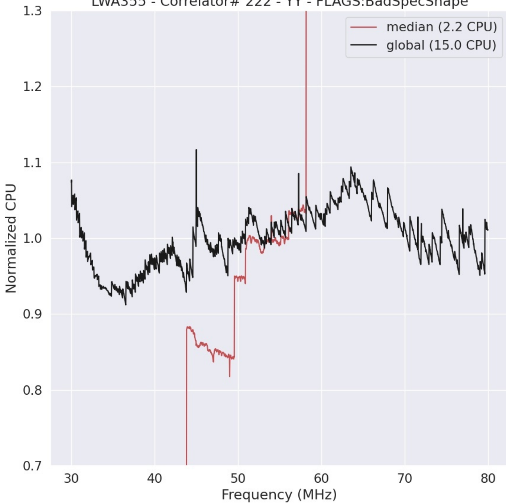
LWA355 - Correlator# 222 - YY - FLAGS:BadSpecShape
