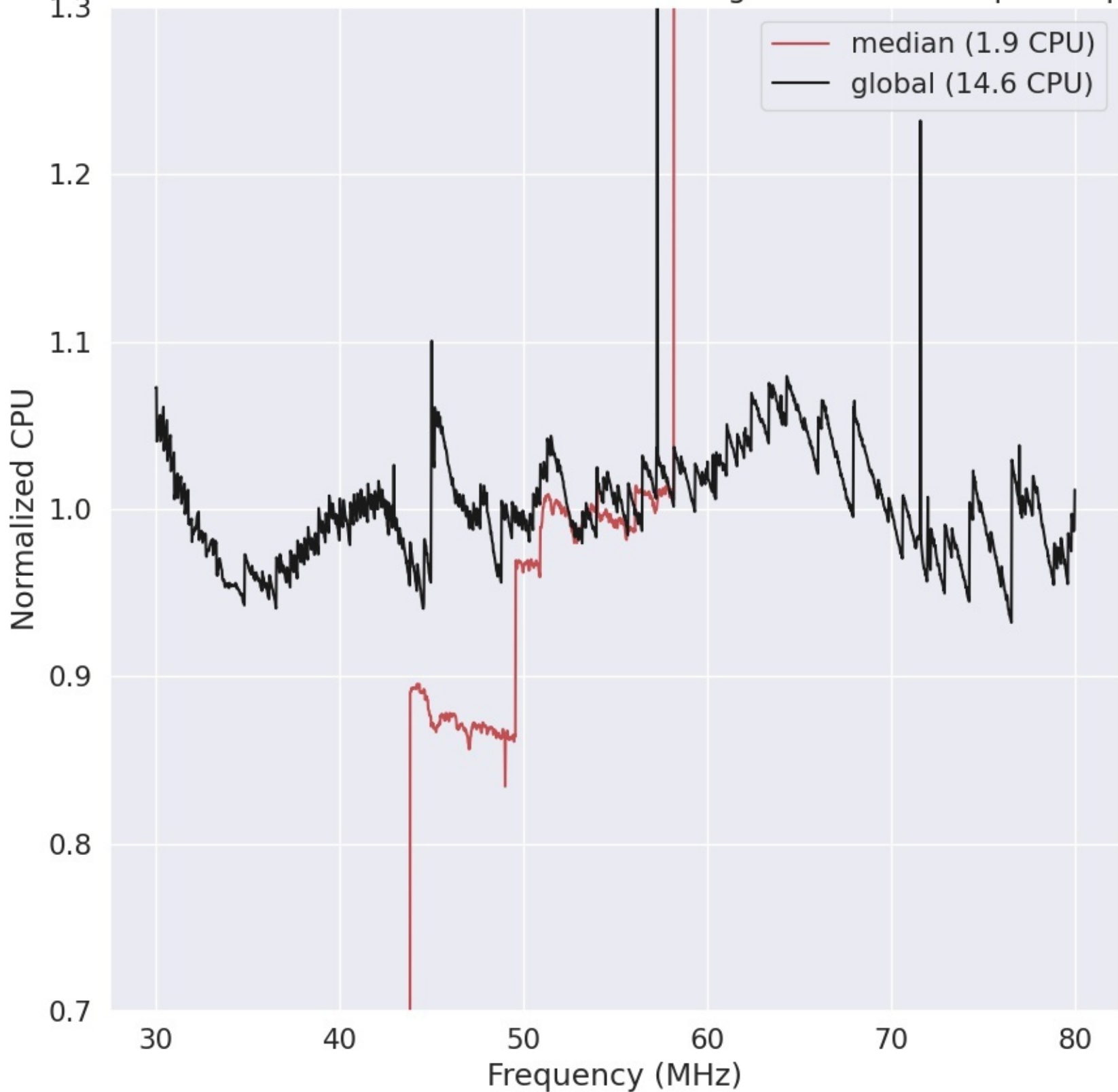
LWA320 - Correlator# 054 - XX - FLAGS:HighTimeVar+BadSpecShape
