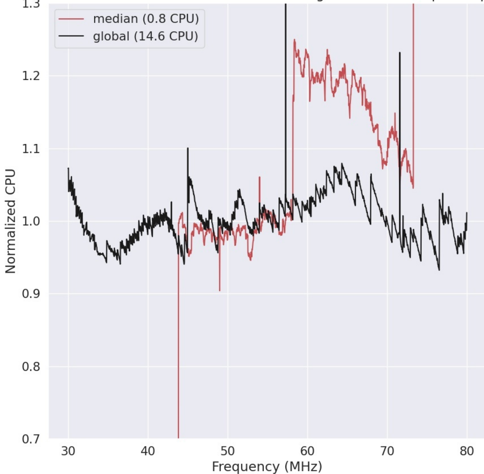
LWA260 - Correlator# 034 - XX - FLAGS:HighTimeVar+BadSpecShape
