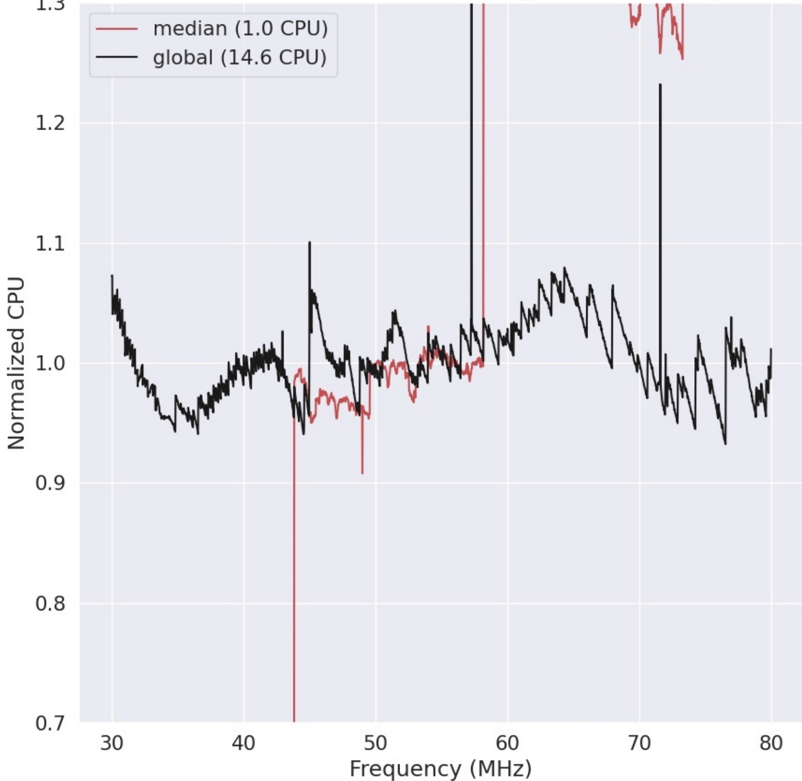
LWA296 - Correlator# 046 - XX - FLAGS:HighTimeVar+BadSpecShape
