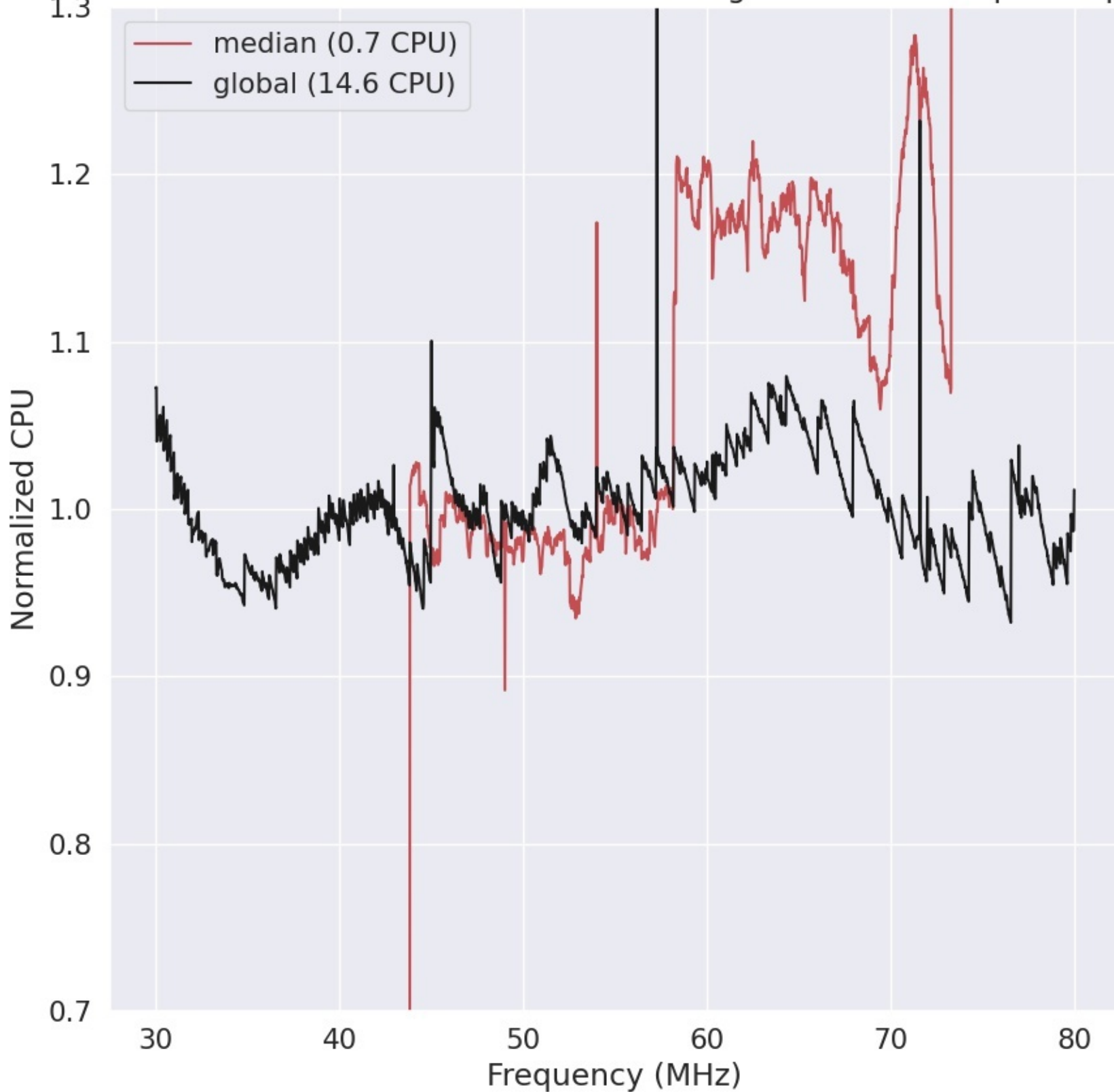
LWA322 - Correlator# 251 - XX - FLAGS:HighTimeVar+BadSpecShape
