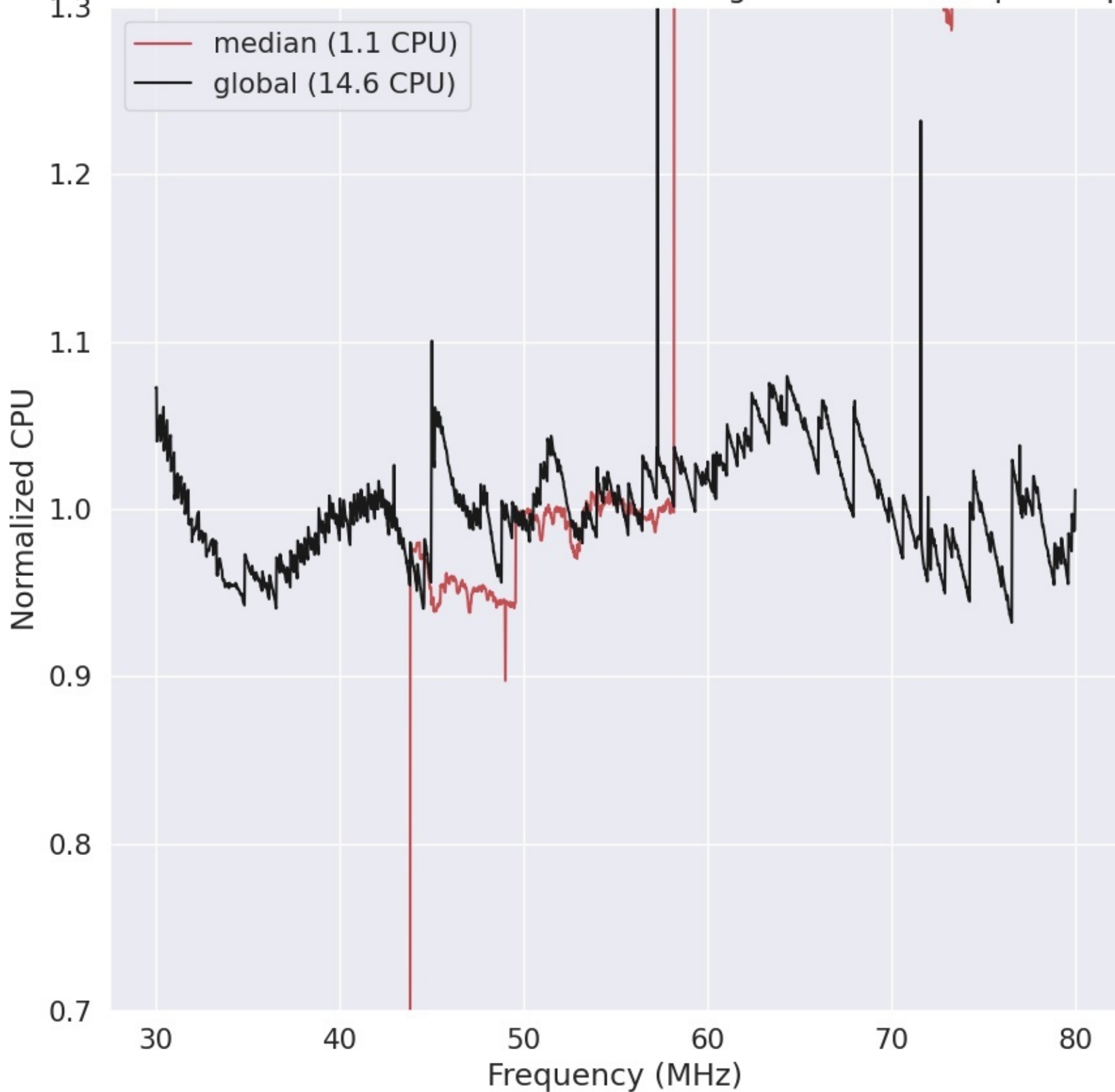
LWA341 - Correlator# 029 - XX - FLAGS:HighTimeVar+BadSpecShape
