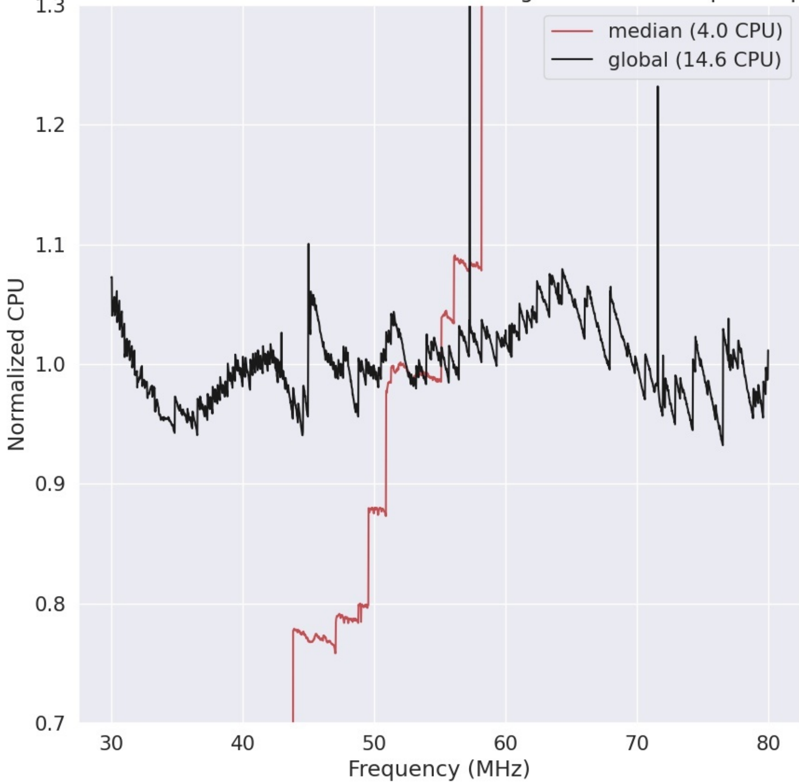
LWA321 - Correlator# 020 - XX - FLAGS:HighTimeVar+BadSpecShape
