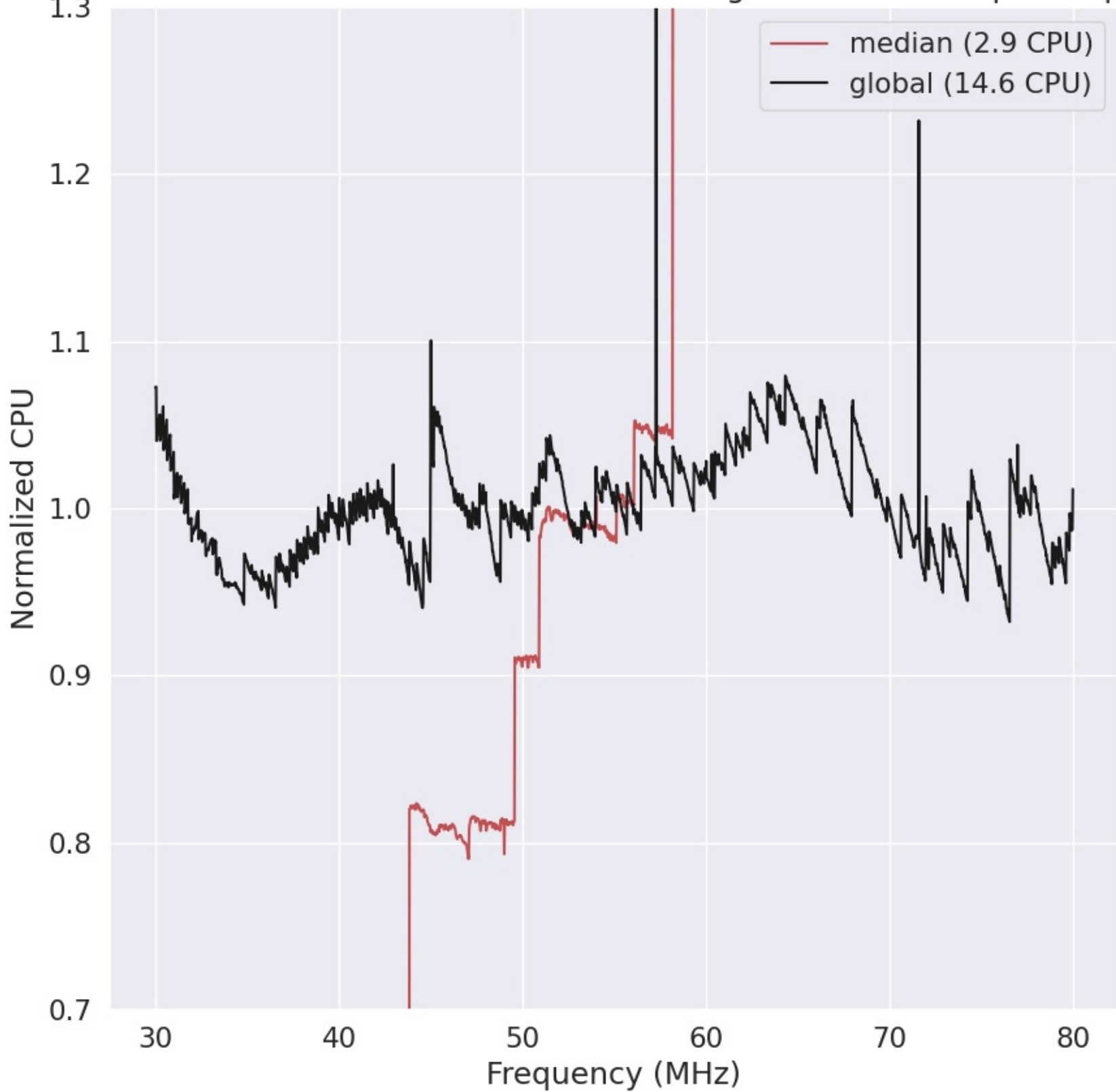
LWA283 - Correlator# 040 - XX - FLAGS:HighTimeVar+BadSpecShape
