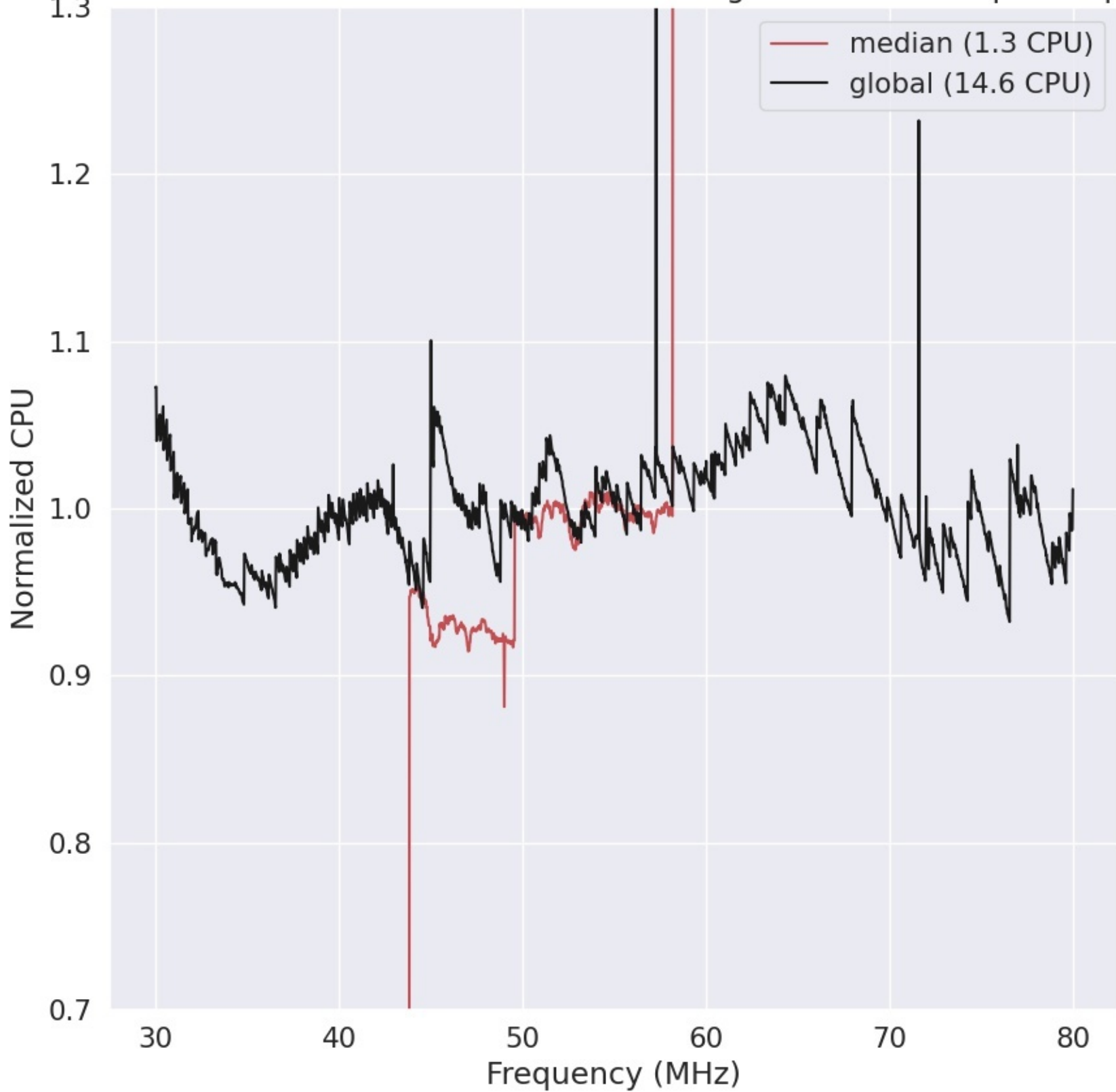
LWA259 - Correlator# 001 - XX - FLAGS:HighTimeVar+BadSpecShape
