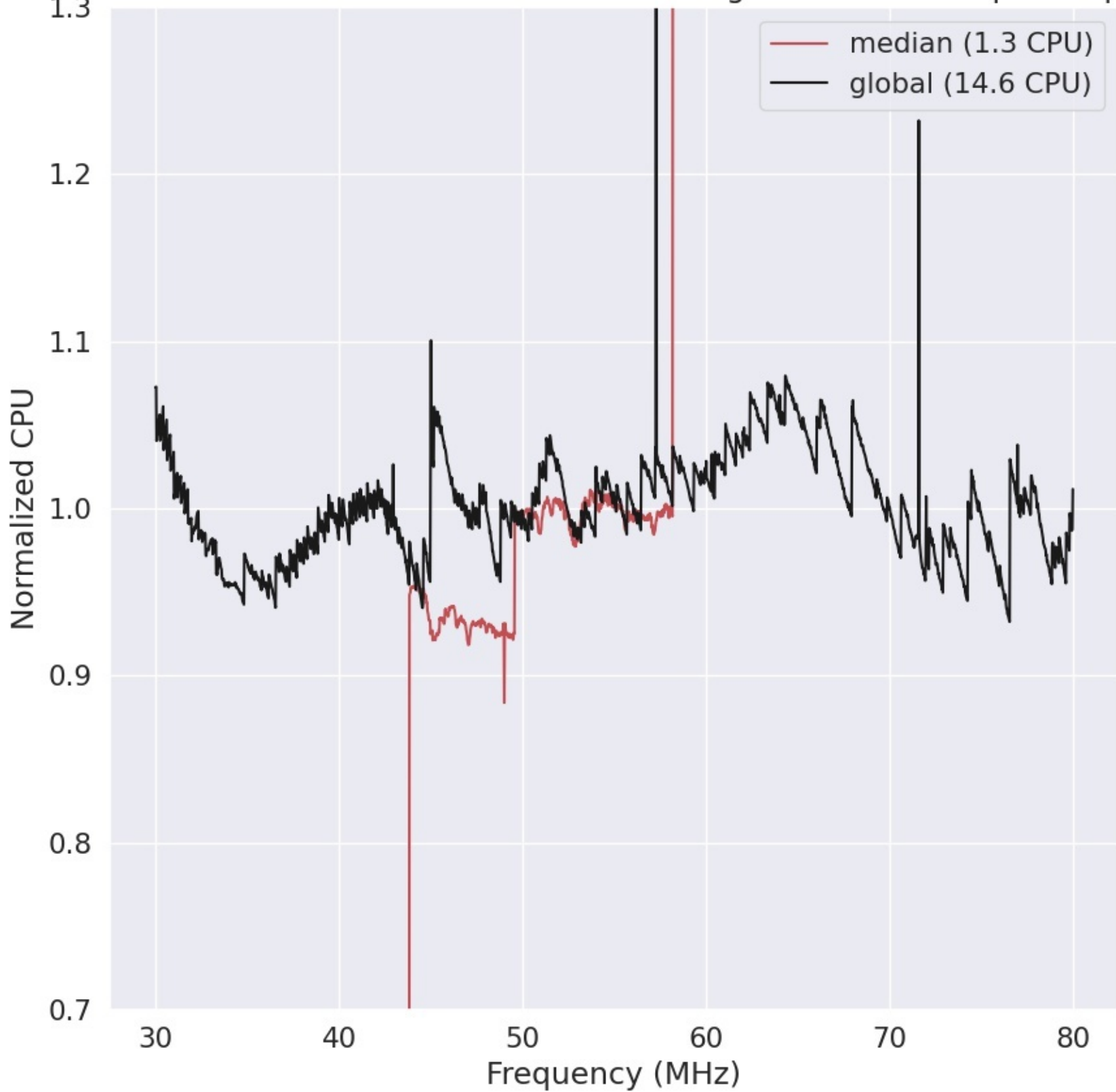
LWA258 - Correlator# 035 - XX - FLAGS:HighTimeVar+BadSpecShape
