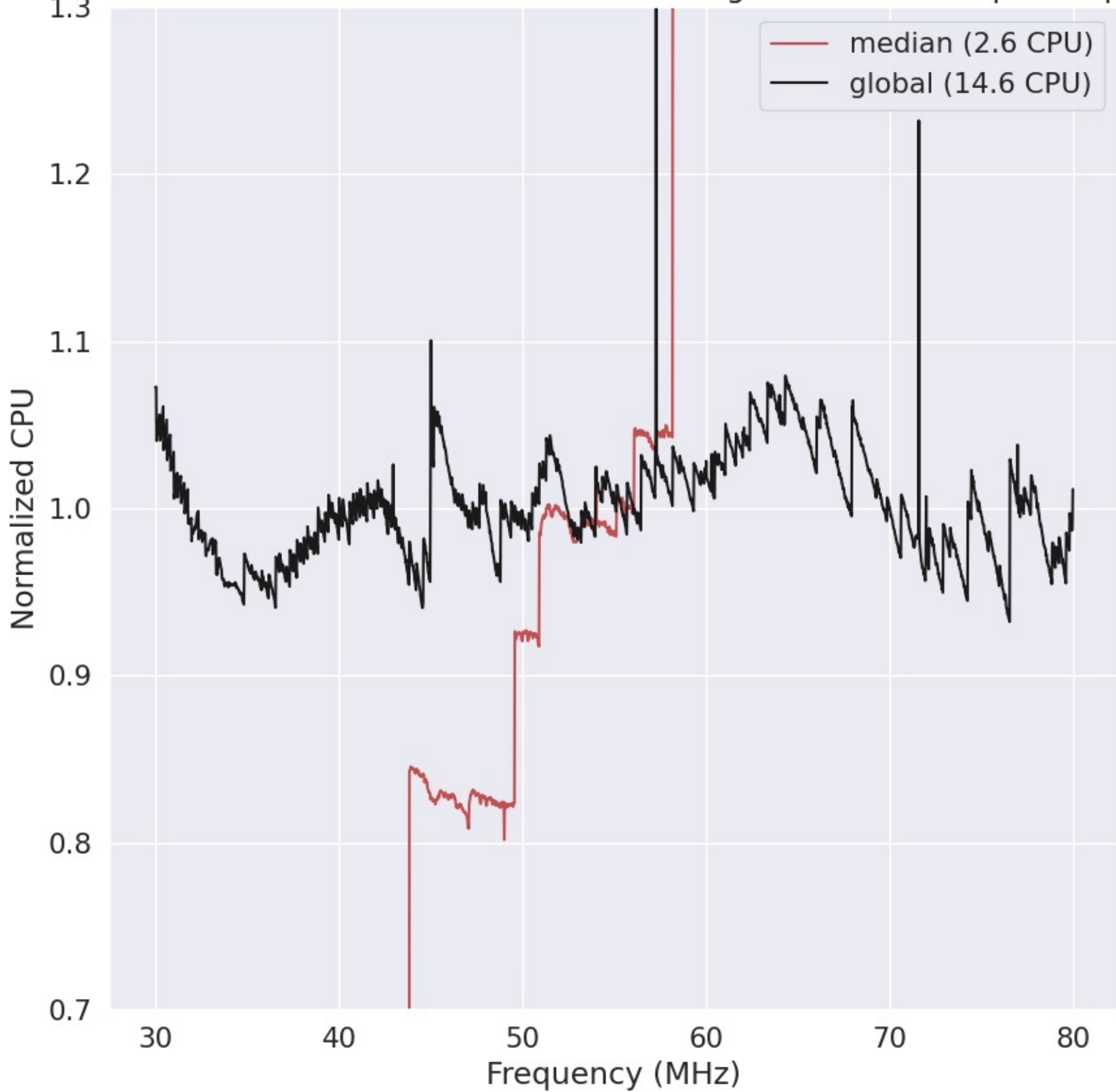
LWA316 - Correlator# 155 - XX - FLAGS:HighTimeVar+BadSpecShape
