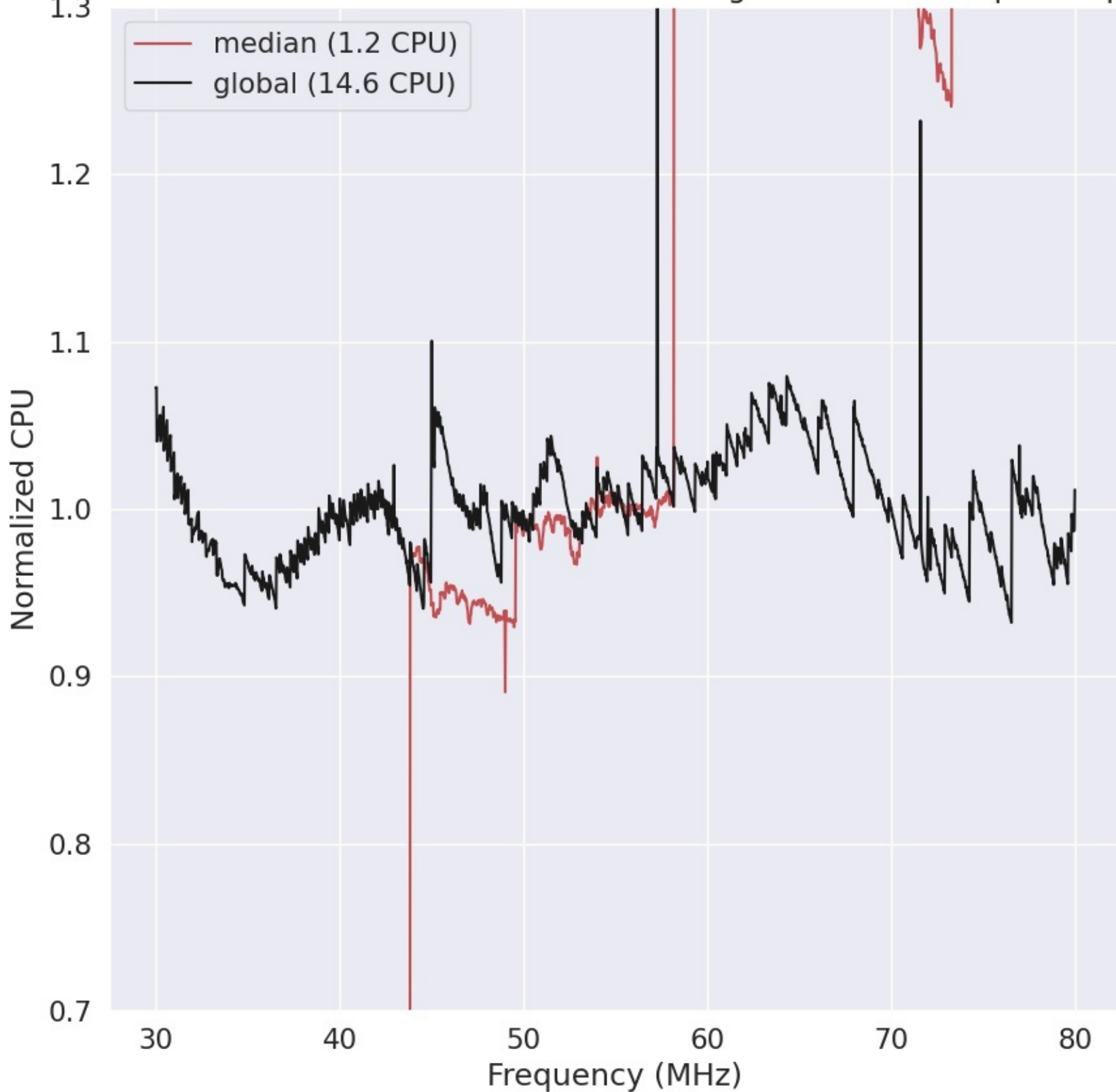
LWA272 - Correlator# 038 - XX - FLAGS:HighTimeVar+BadSpecShape
