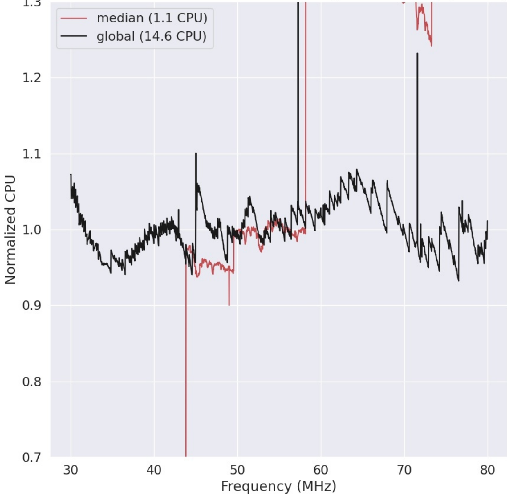
LWA282 - Correlator# 010 - XX - FLAGS:HighTimeVar+BadSpecShape
