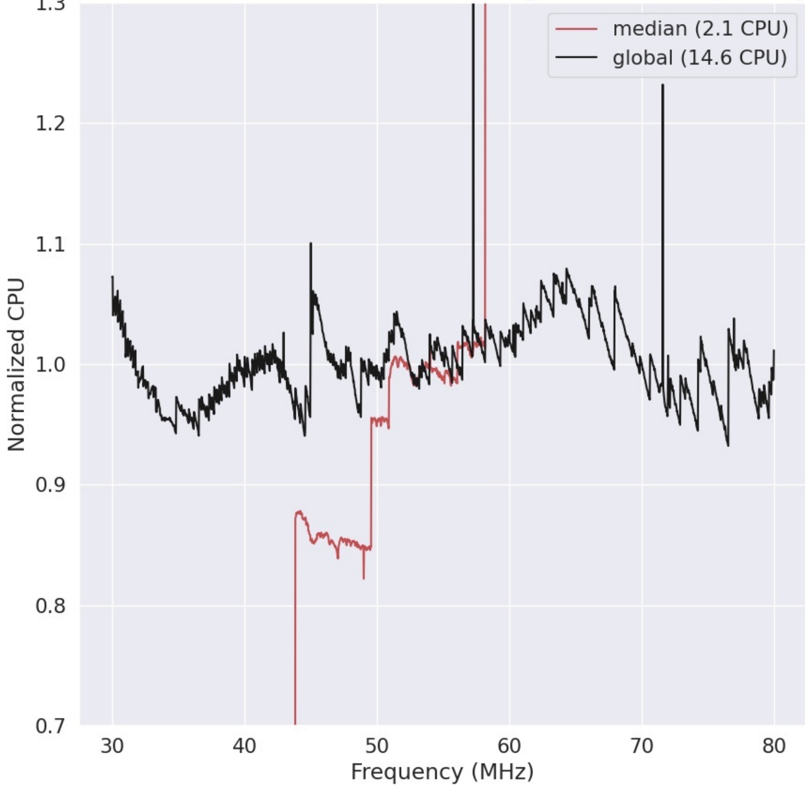
LWA276 - Correlator# 006 - XX - FLAGS:HighTimeVar+BadSpecShape
