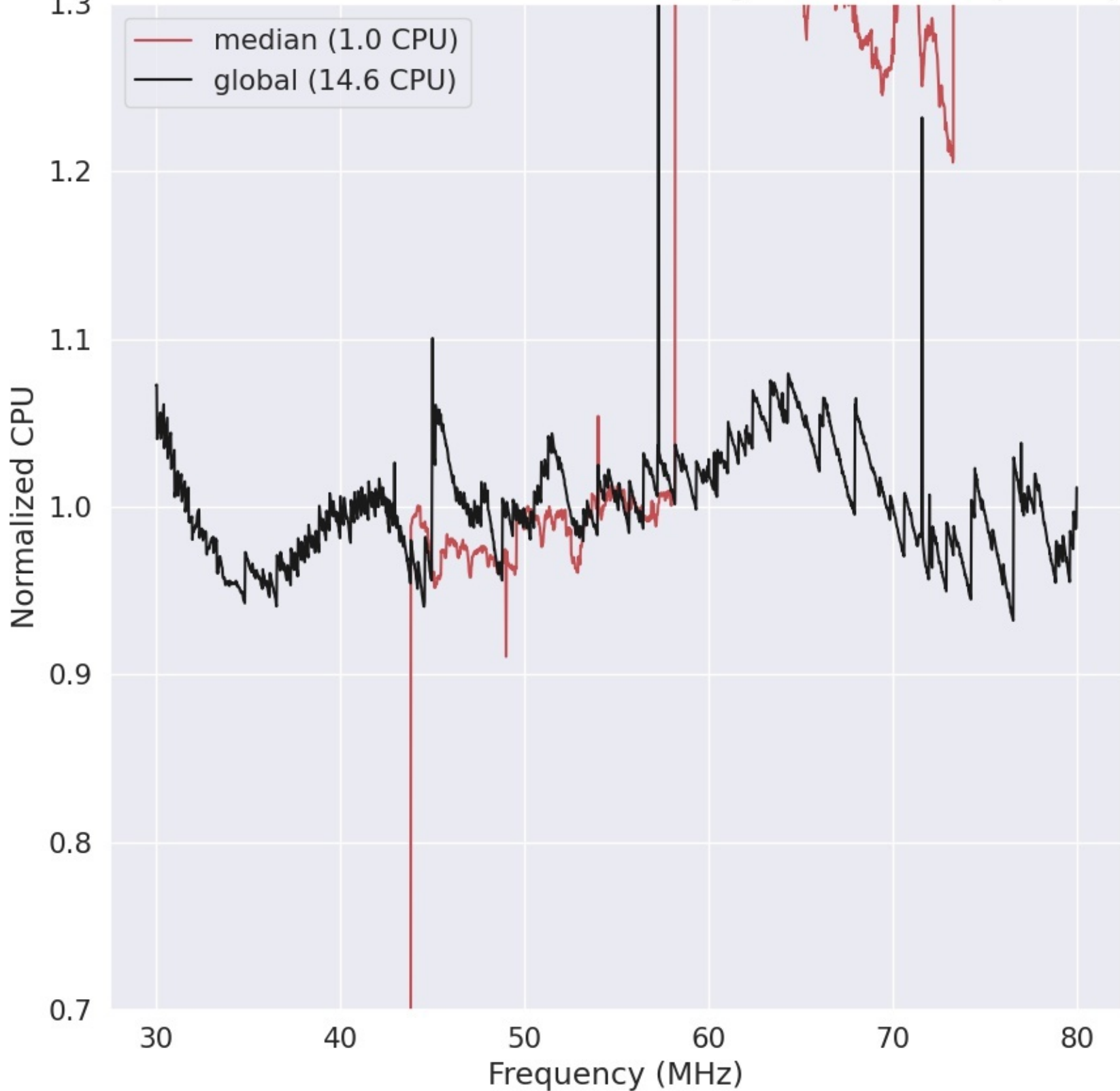
LWA257 - Correlator# 032 - XX - FLAGS:HighTimeVar+BadSpecShape
