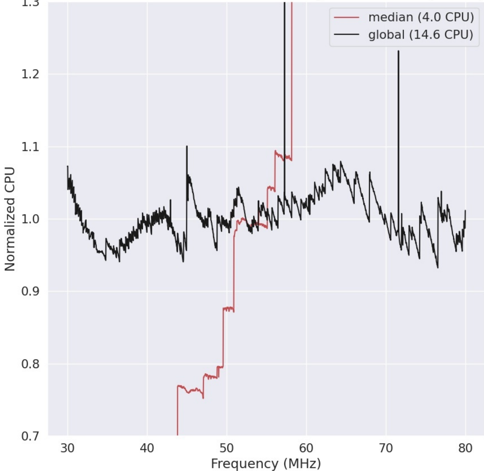
LWA277 - Correlator# 009 - XX - FLAGS:HighTimeVar+BadSpecShape
