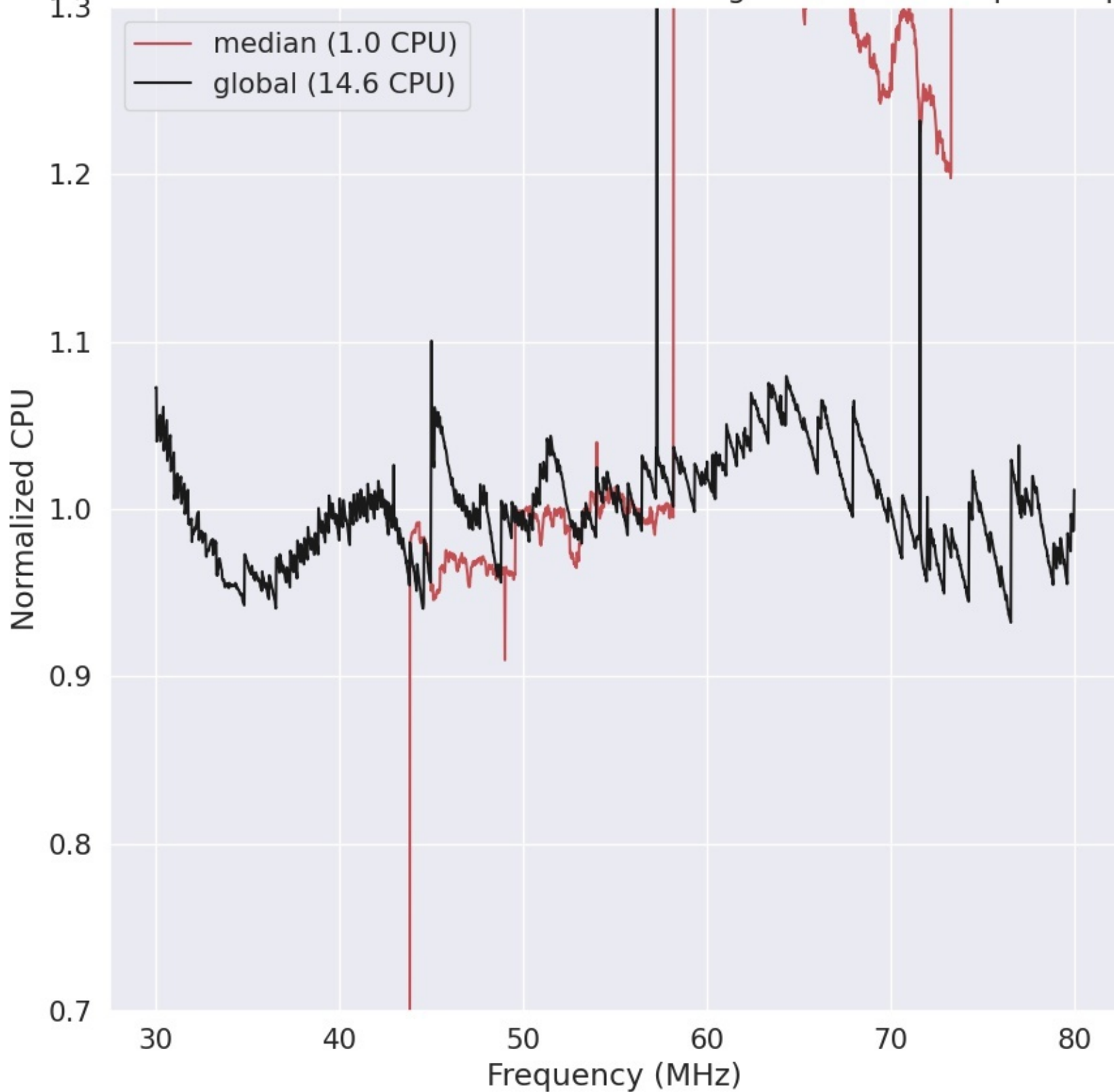
LWA289 - Correlator# 189 - XX - FLAGS:HighTimeVar+BadSpecShape
