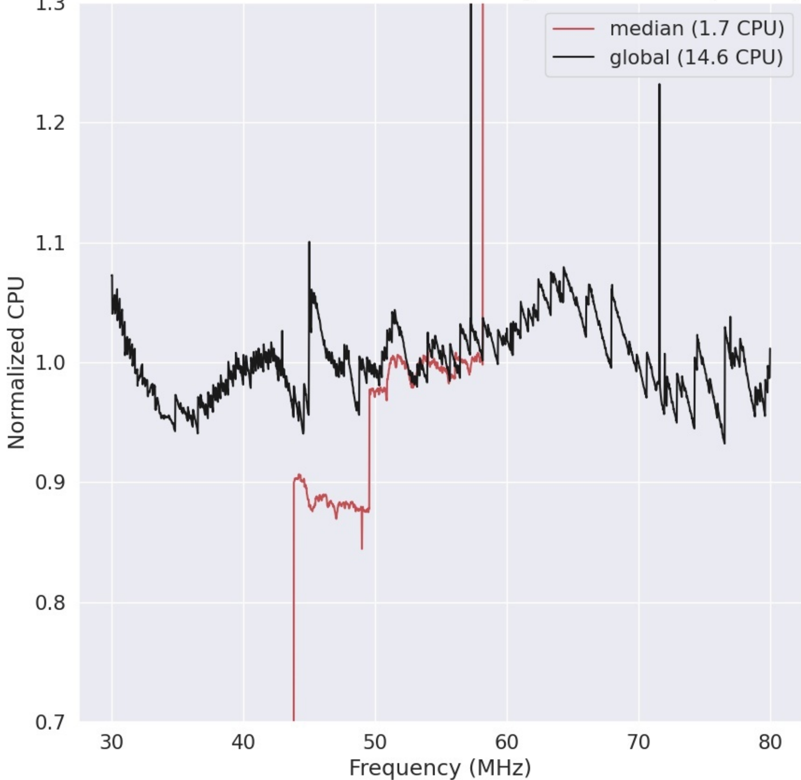
LWA285 - Correlator# 013 - XX - FLAGS:HighTimeVar+BadSpecShape
