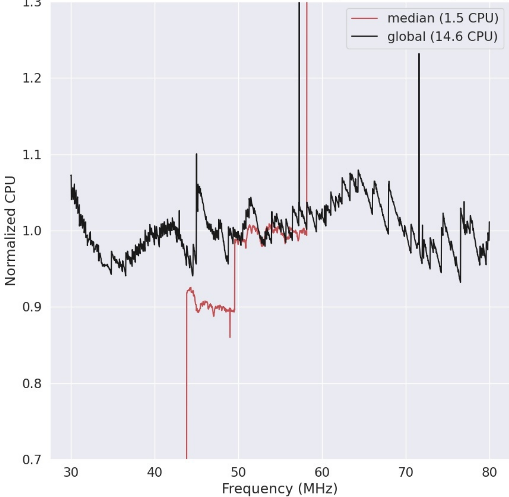
LWA327 - Correlator# 023 - XX - FLAGS:HighTimeVar+BadSpecShape
