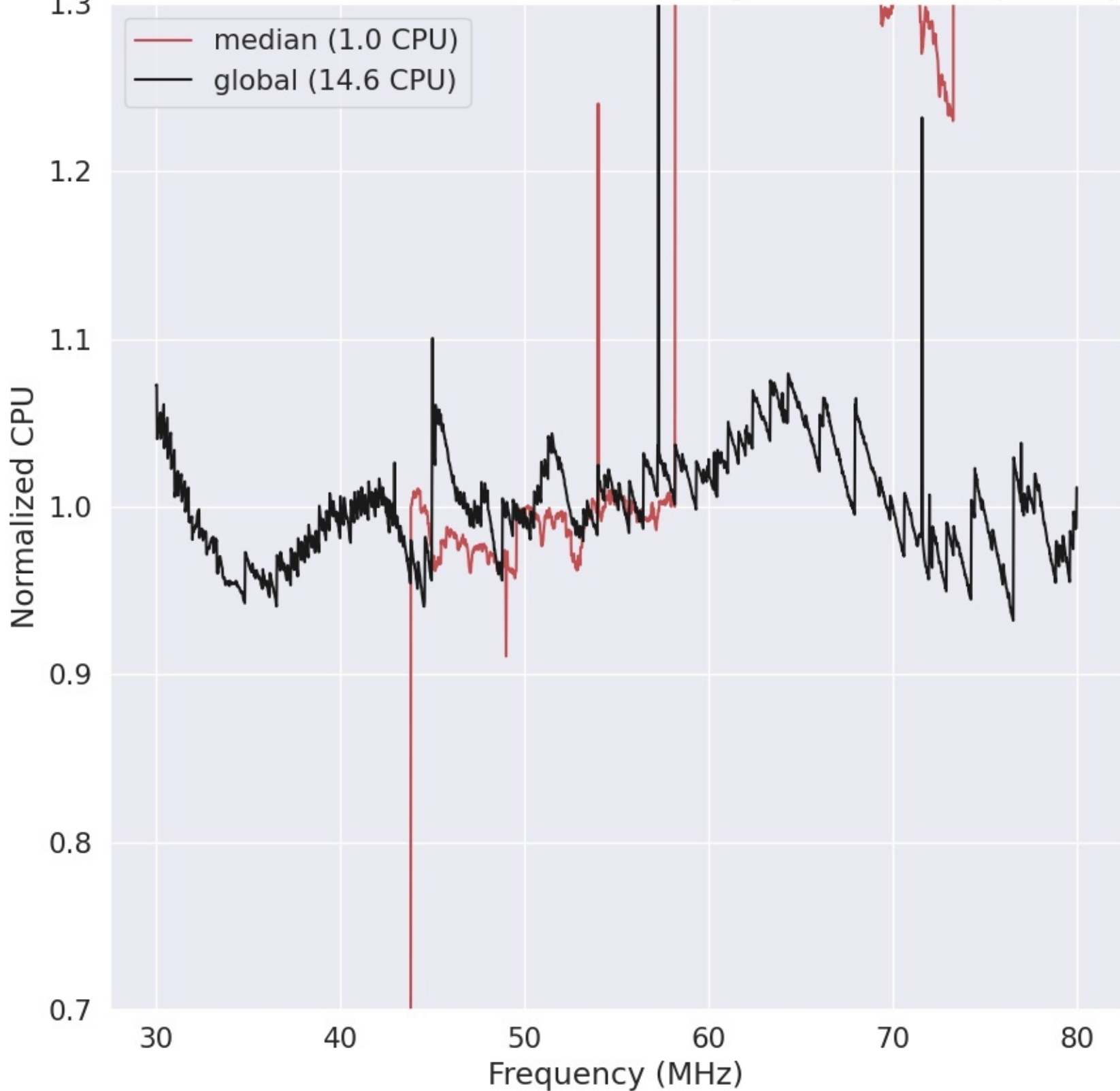
LWA347 - Correlator# 255 - XX - FLAGS:HighTimeVar+BadSpecShape
