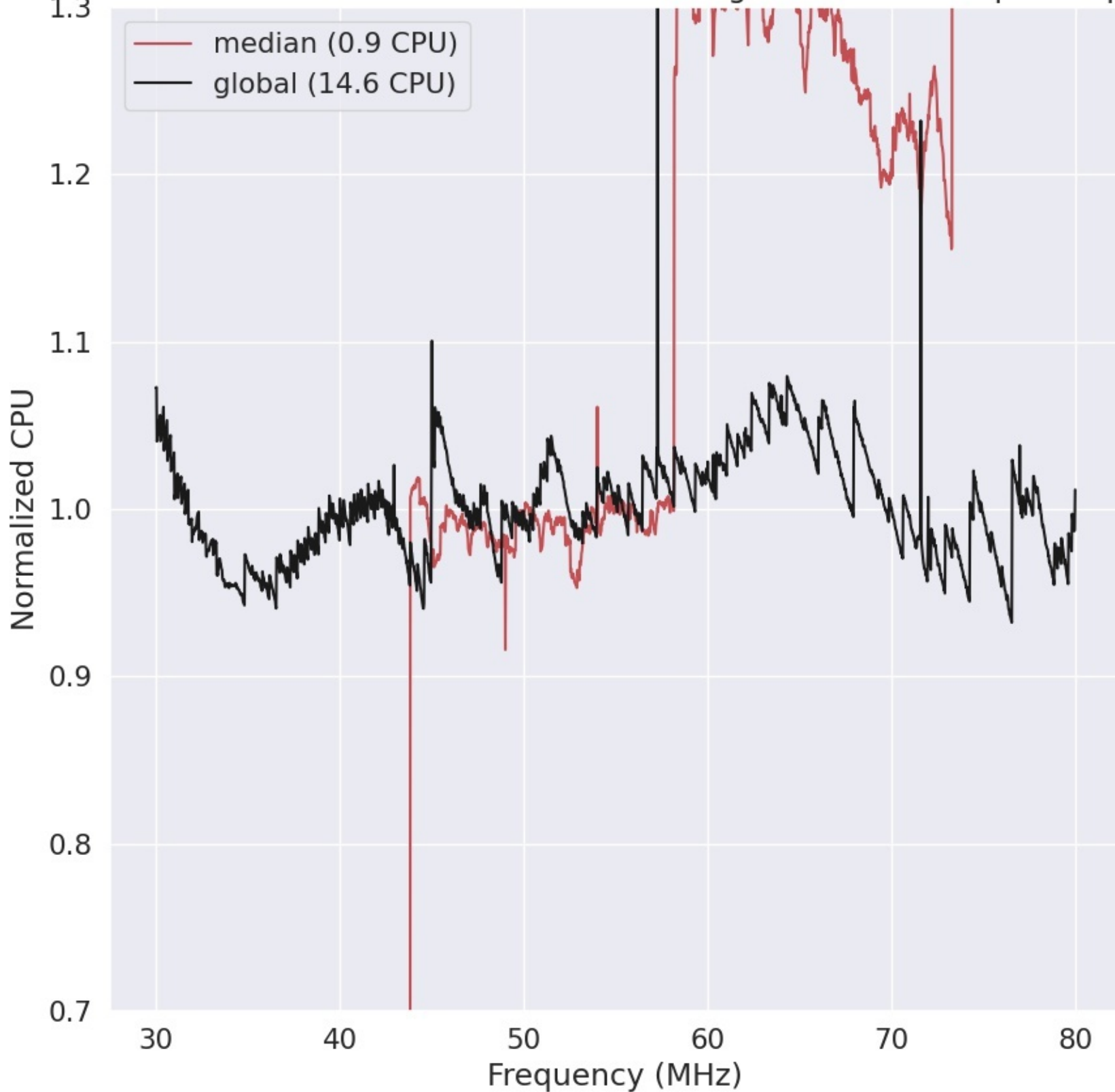
LWA325 - Correlator# 154 - XX - FLAGS:HighTimeVar+BadSpecShape
