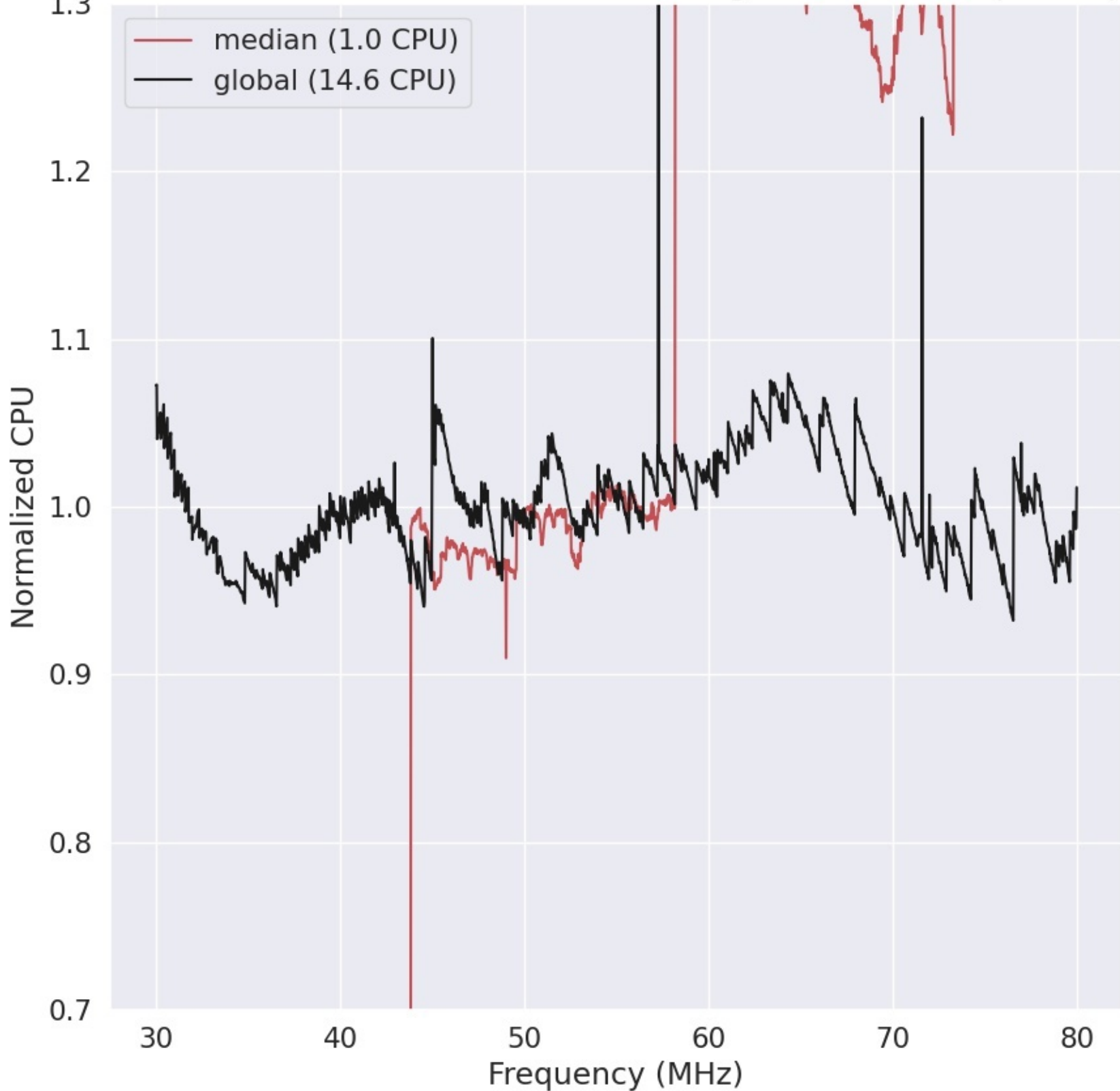
LWA280 - Correlator# 041 - XX - FLAGS:HighTimeVar+BadSpecShape
