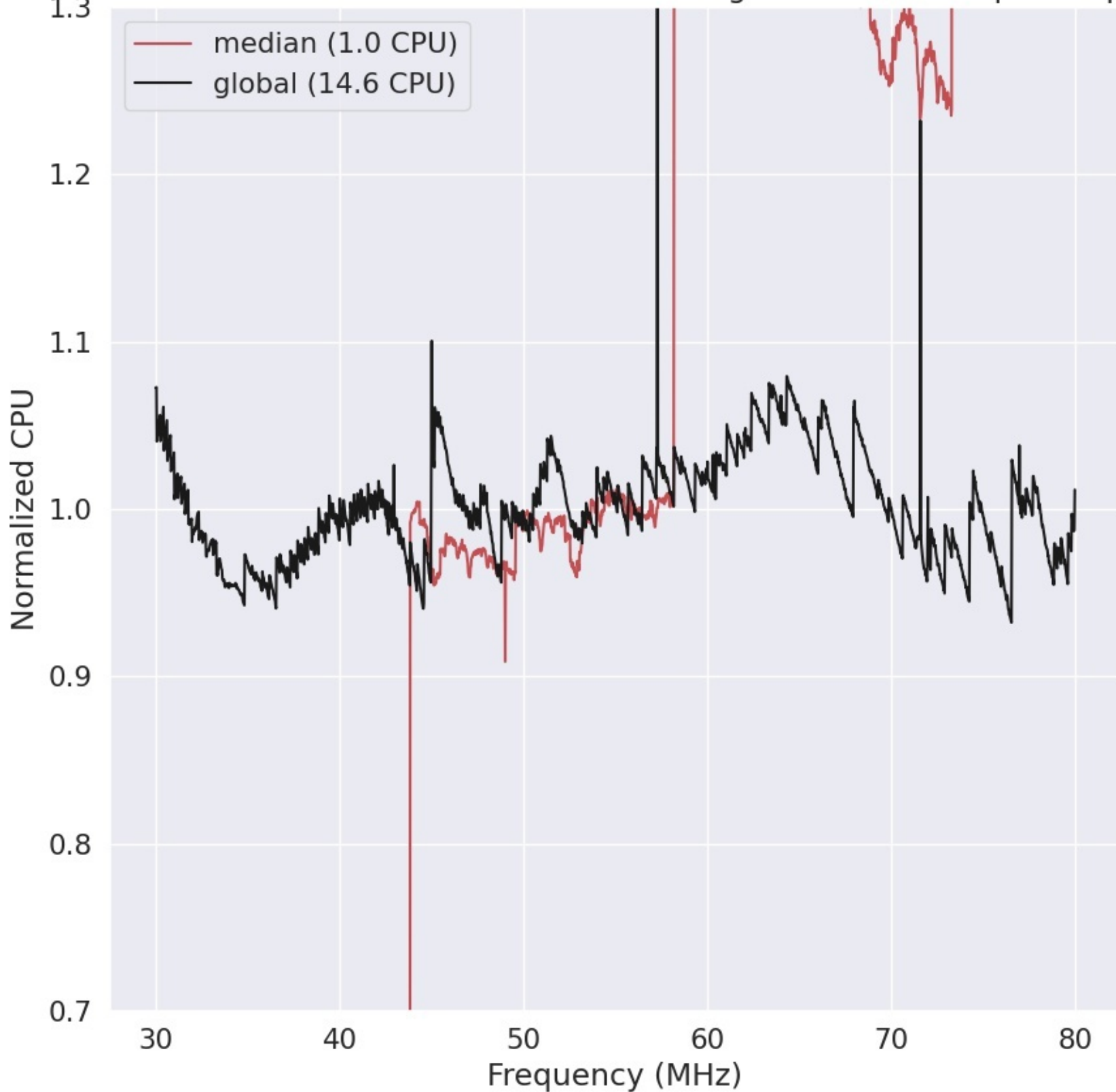
LWA332 - Correlator# 025 - XX - FLAGS:HighTimeVar+BadSpecShape
