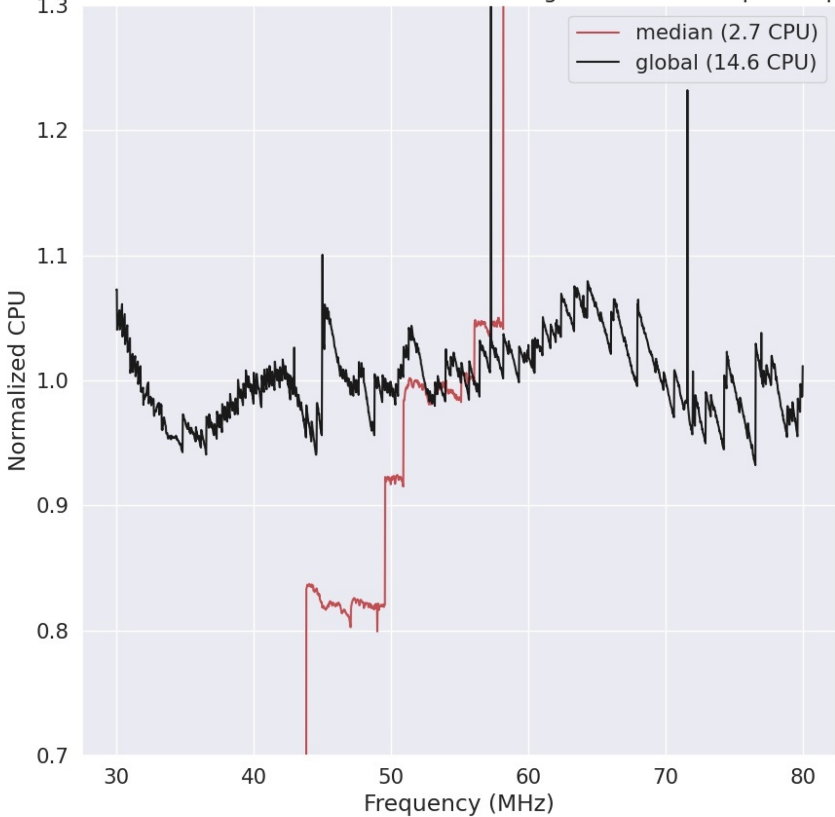
LWA335 - Correlator# 057 - XX - FLAGS:HighTimeVar+BadSpecShape
