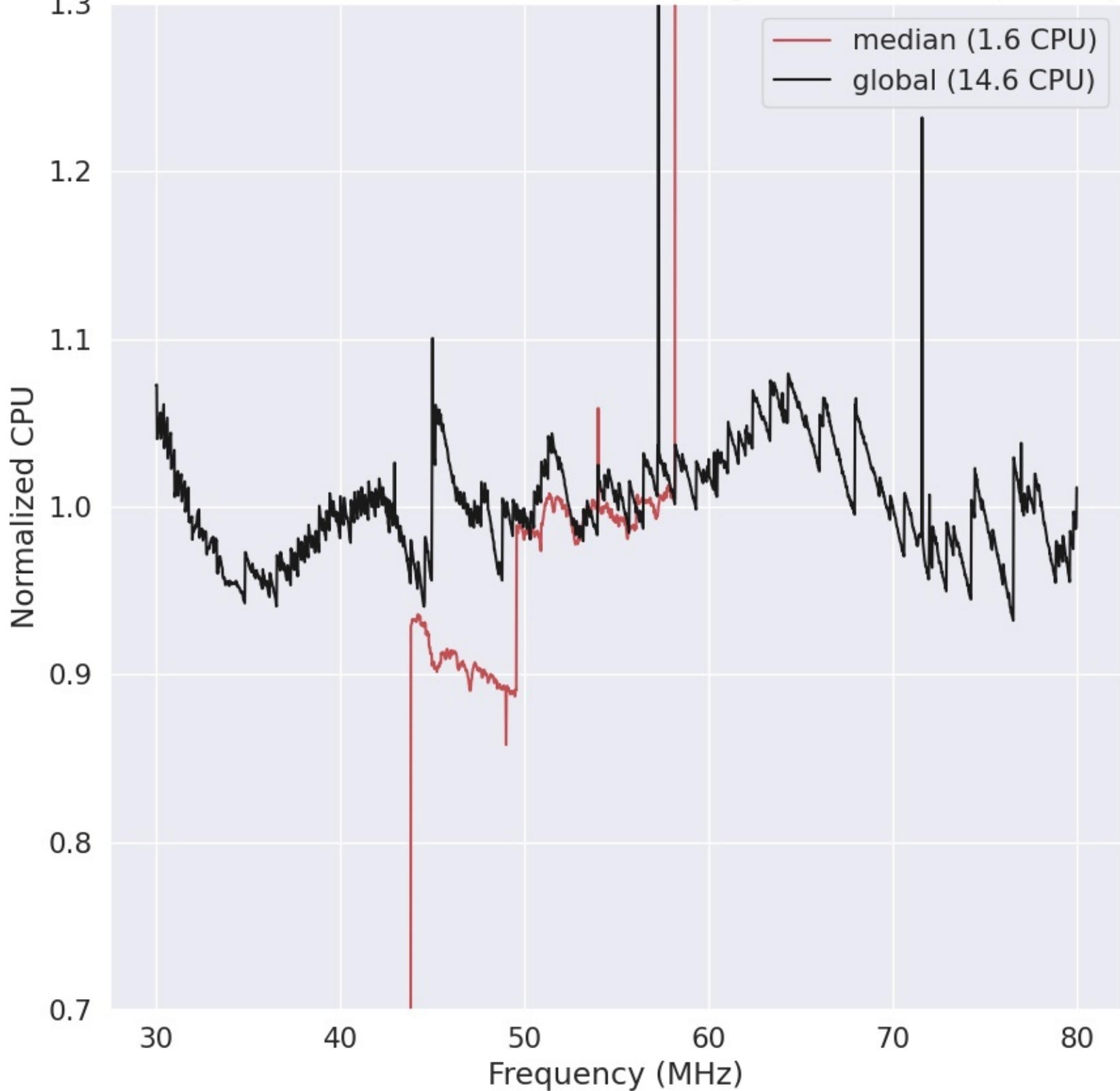
LWA328 - Correlator# 157 - XX - FLAGS:HighTimeVar+BadSpecShape
