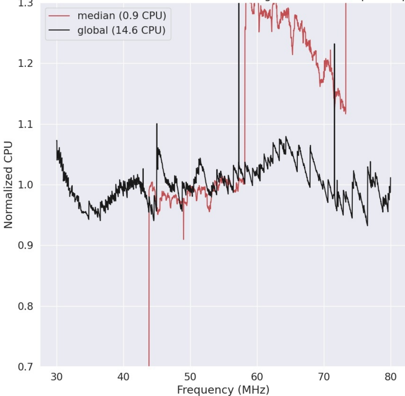
LWA308 - Correlator# 015 - XX - FLAGS:HighTimeVar+BadSpecShape
