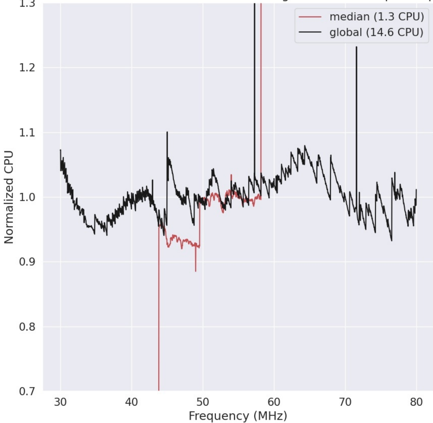
LWA309 - Correlator# 014 - XX - FLAGS:HighTimeVar+BadSpecShape
