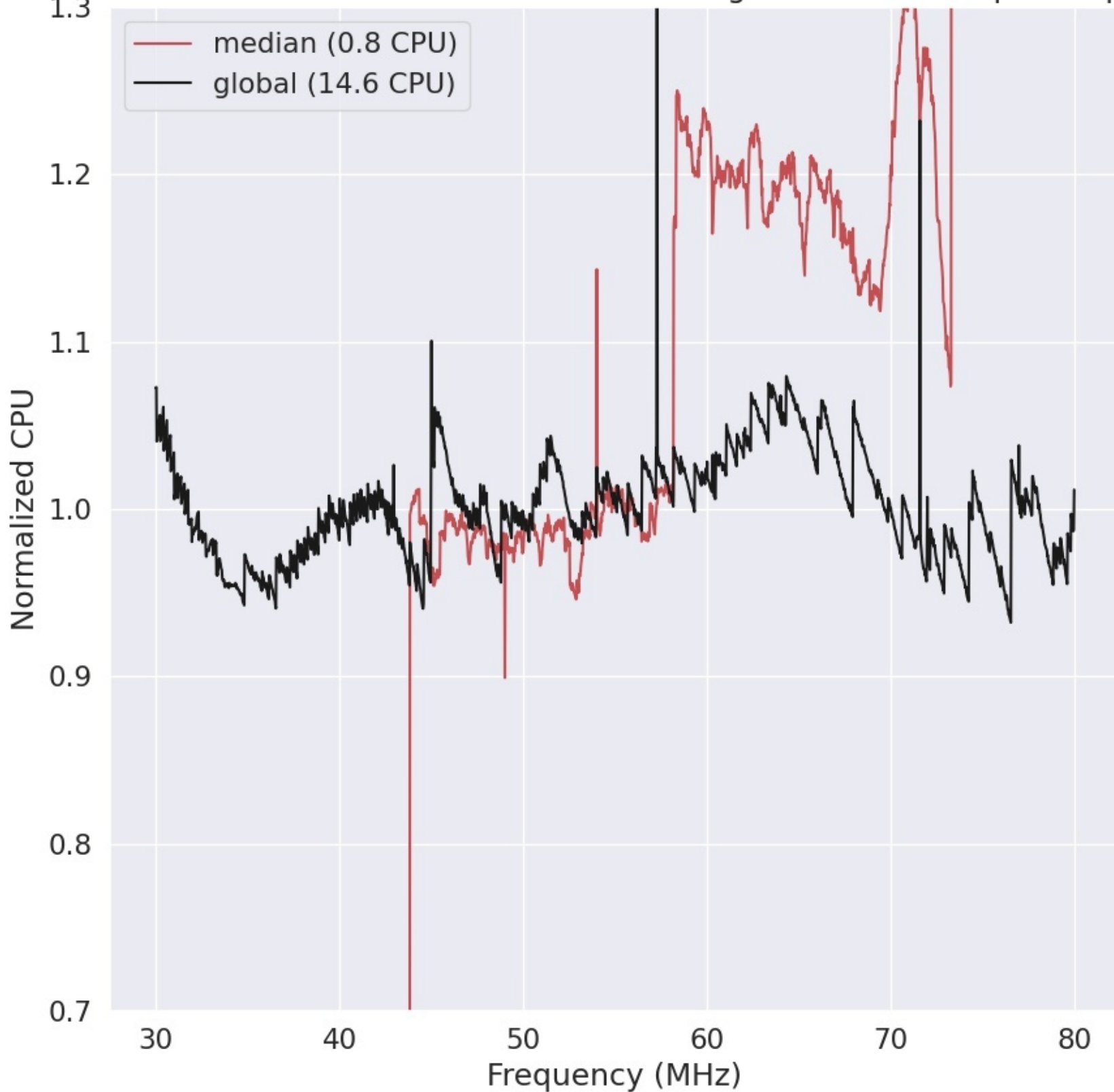
LWA295 - Correlator# 047 - XX - FLAGS:HighTimeVar+BadSpecShape
