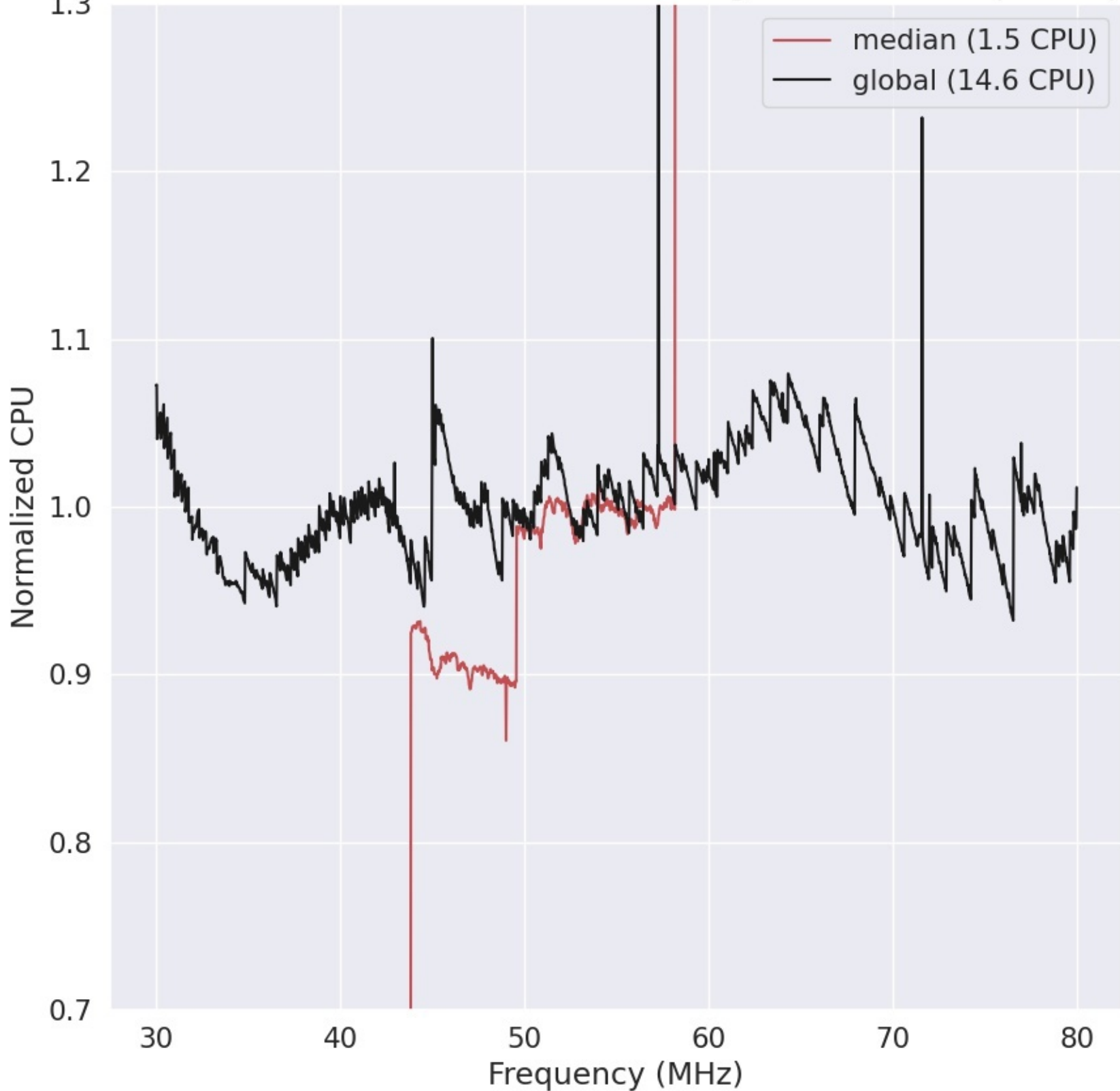
LWA291 - Correlator# 045 - XX - FLAGS:HighTimeVar+BadSpecShape
