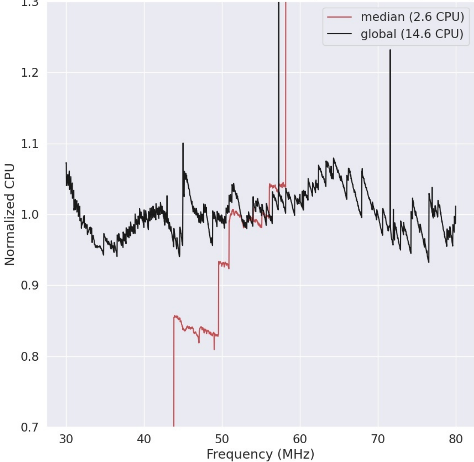
LWA275 - Correlator# 090 - XX - FLAGS:HighTimeVar+BadSpecShape
