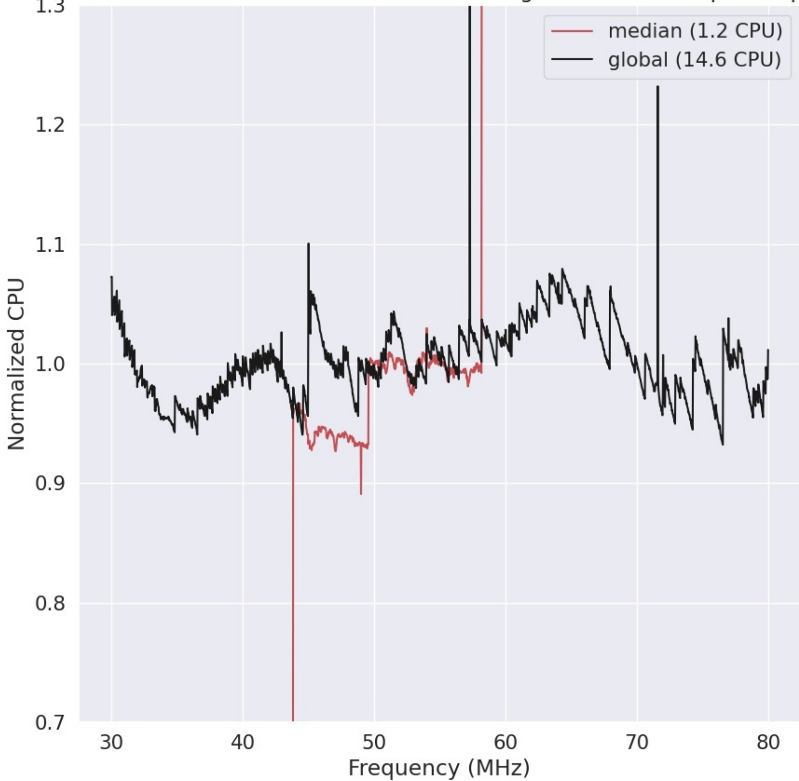
LWA336 - Correlator# 056 - XX - FLAGS:HighTimeVar+BadSpecShape
