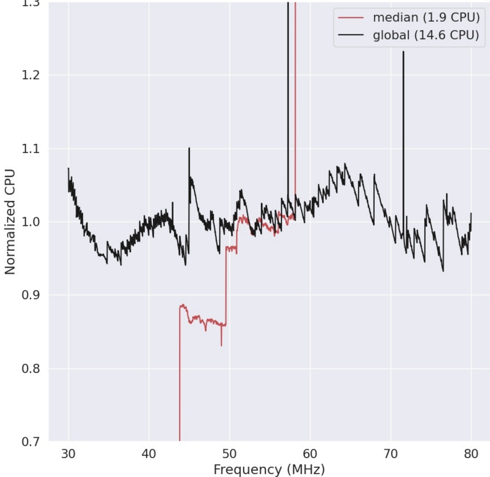
LWA279 - Correlator# 220 - XX - FLAGS:HighTimeVar+BadSpecShape
