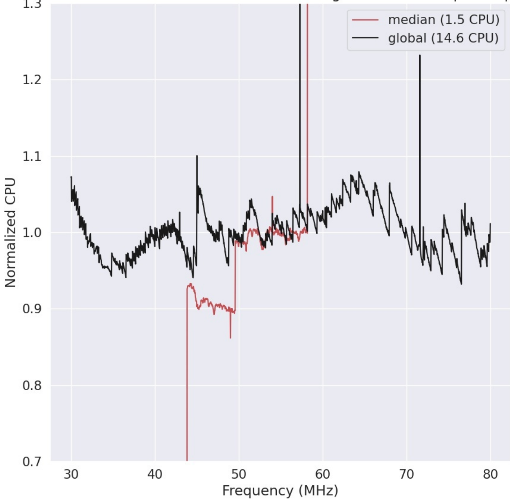
LWA298 - Correlator# 049 - XX - FLAGS:HighTimeVar+BadSpecShape
