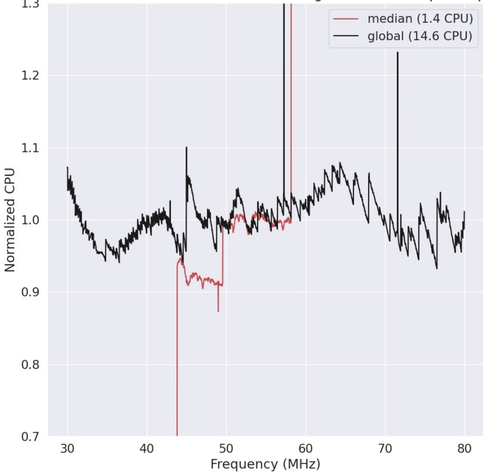
LWA292 - Correlator# 044 - XX - FLAGS:HighTimeVar+BadSpecShape
