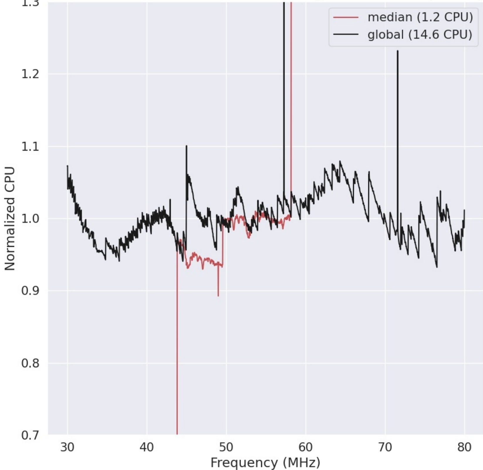
LWA353 - Correlator# 031 - XX - FLAGS:HighTimeVar+BadSpecShape
