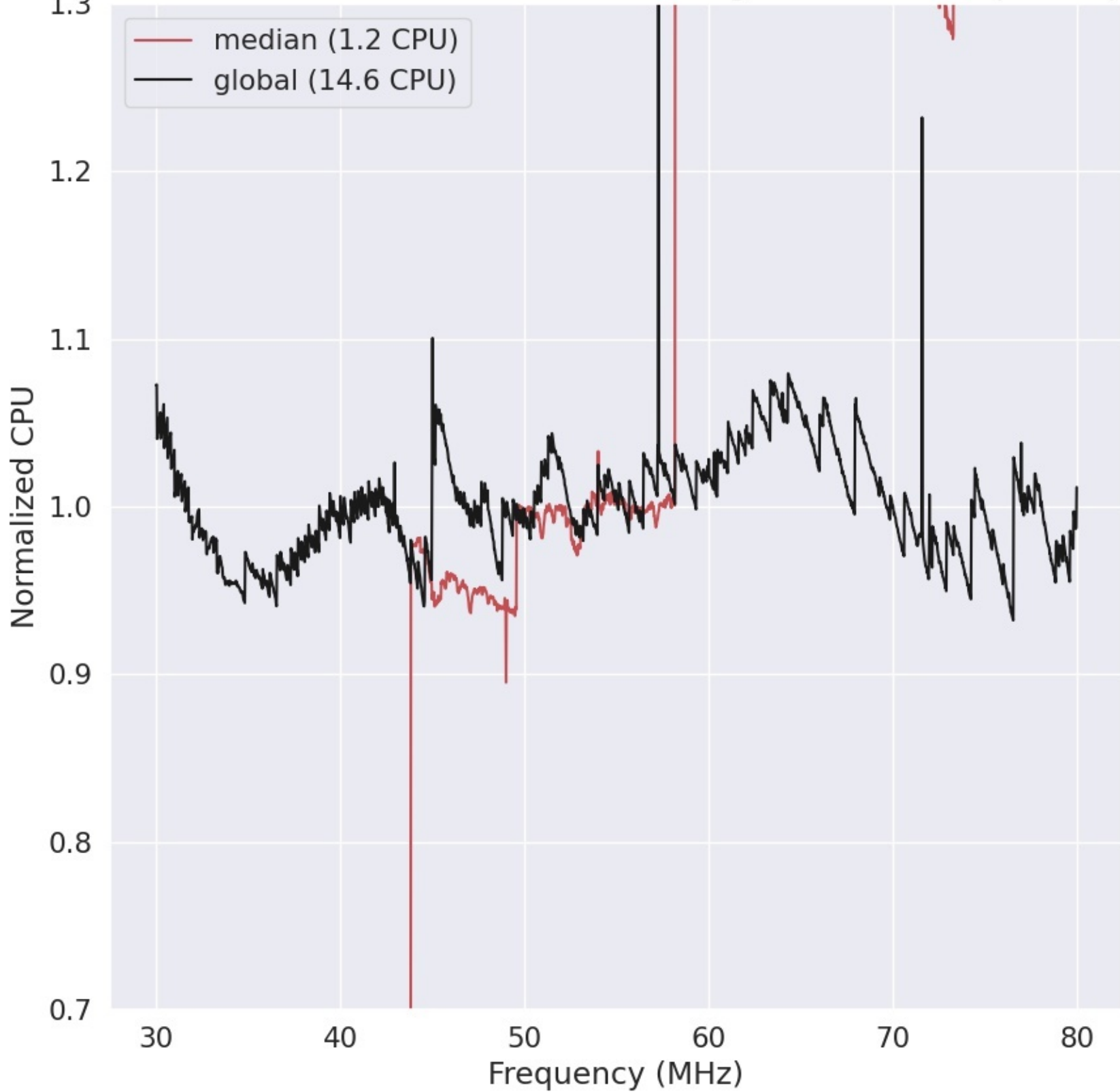
LWA290 - Correlator# 285 - XX - FLAGS:HighTimeVar+BadSpecShape
