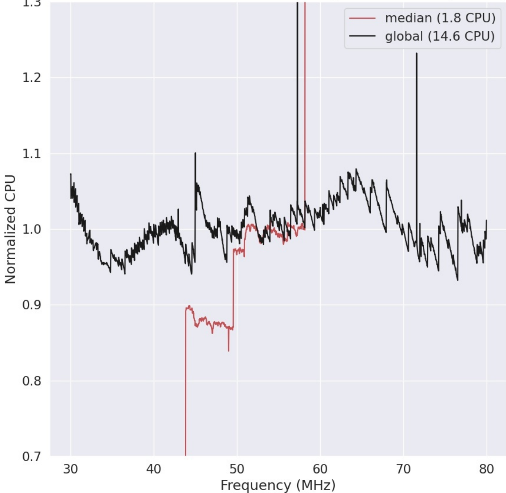
LWA351 - Correlator# 060 - XX - FLAGS:HighTimeVar+BadSpecShape
