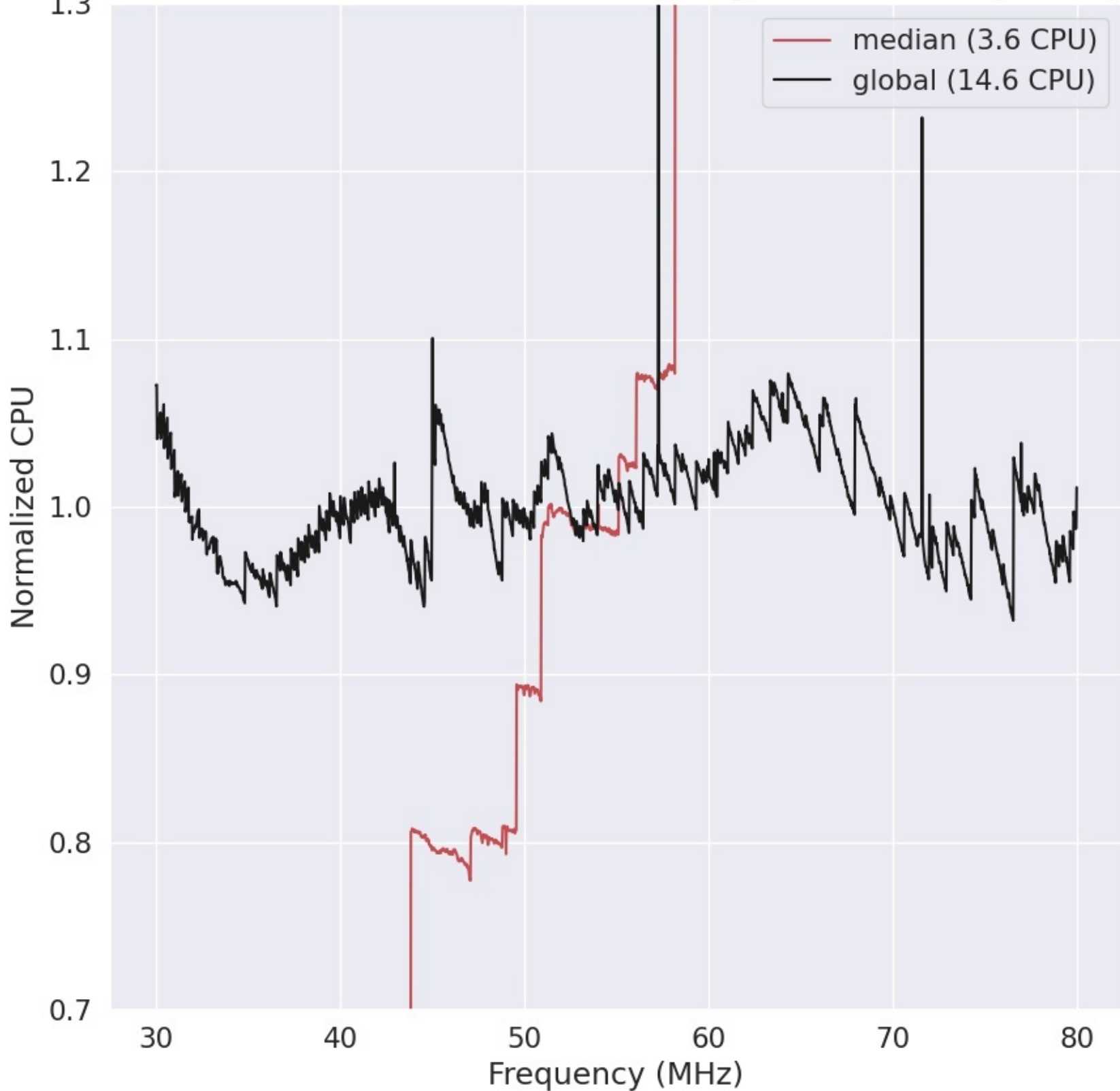
LWA286 - Correlator# 093 - XX - FLAGS:HighTimeVar+BadSpecShape
