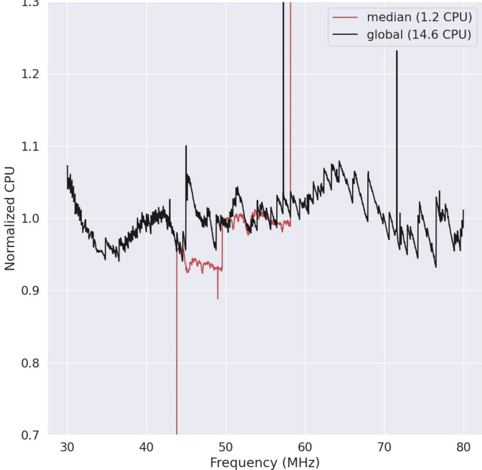
LWA343 - Correlator# 058 - XX - FLAGS:HighTimeVar+BadSpecShape
