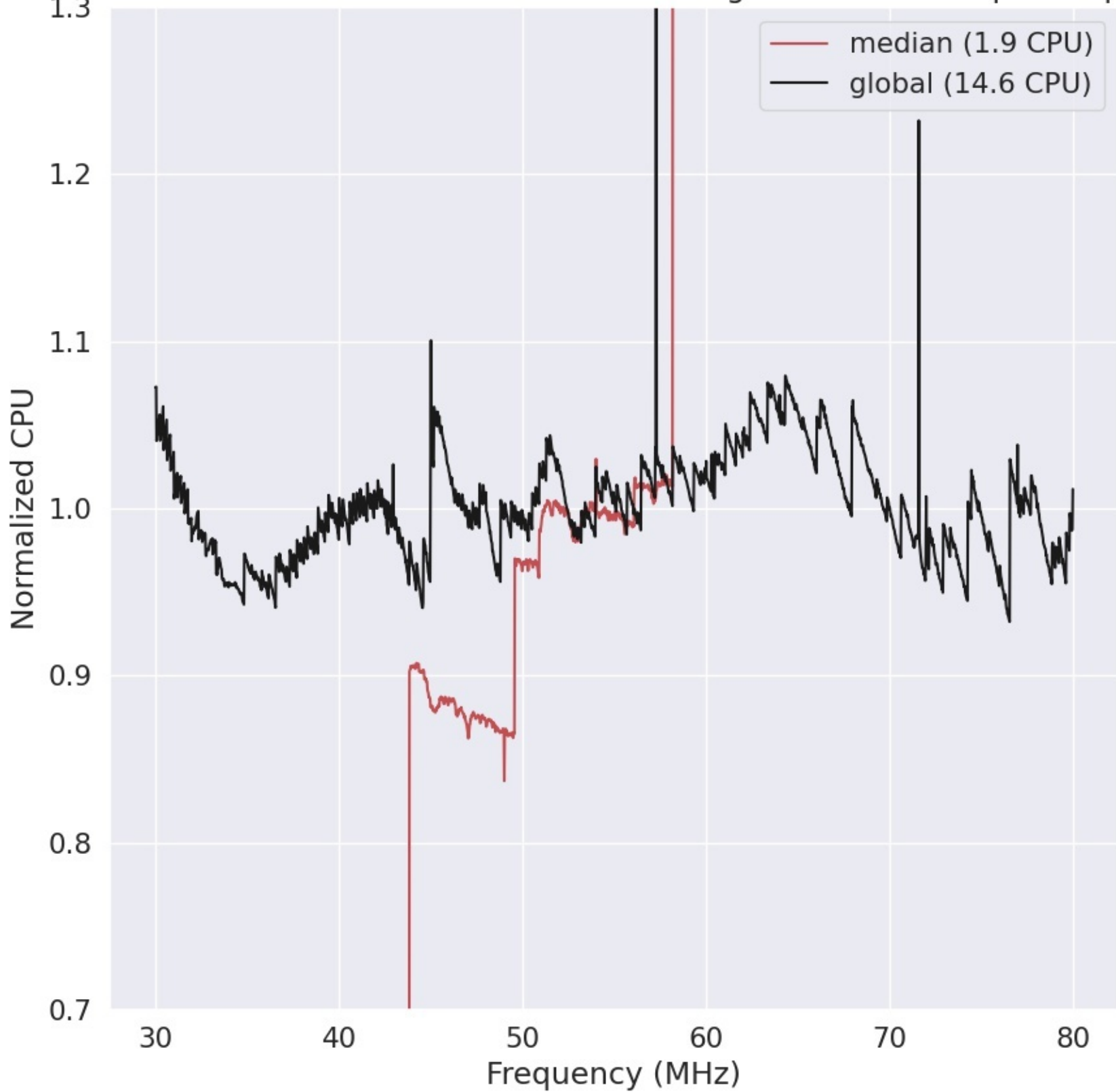
LWA297 - Correlator# 314 - XX - FLAGS:HighTimeVar+BadSpecShape
