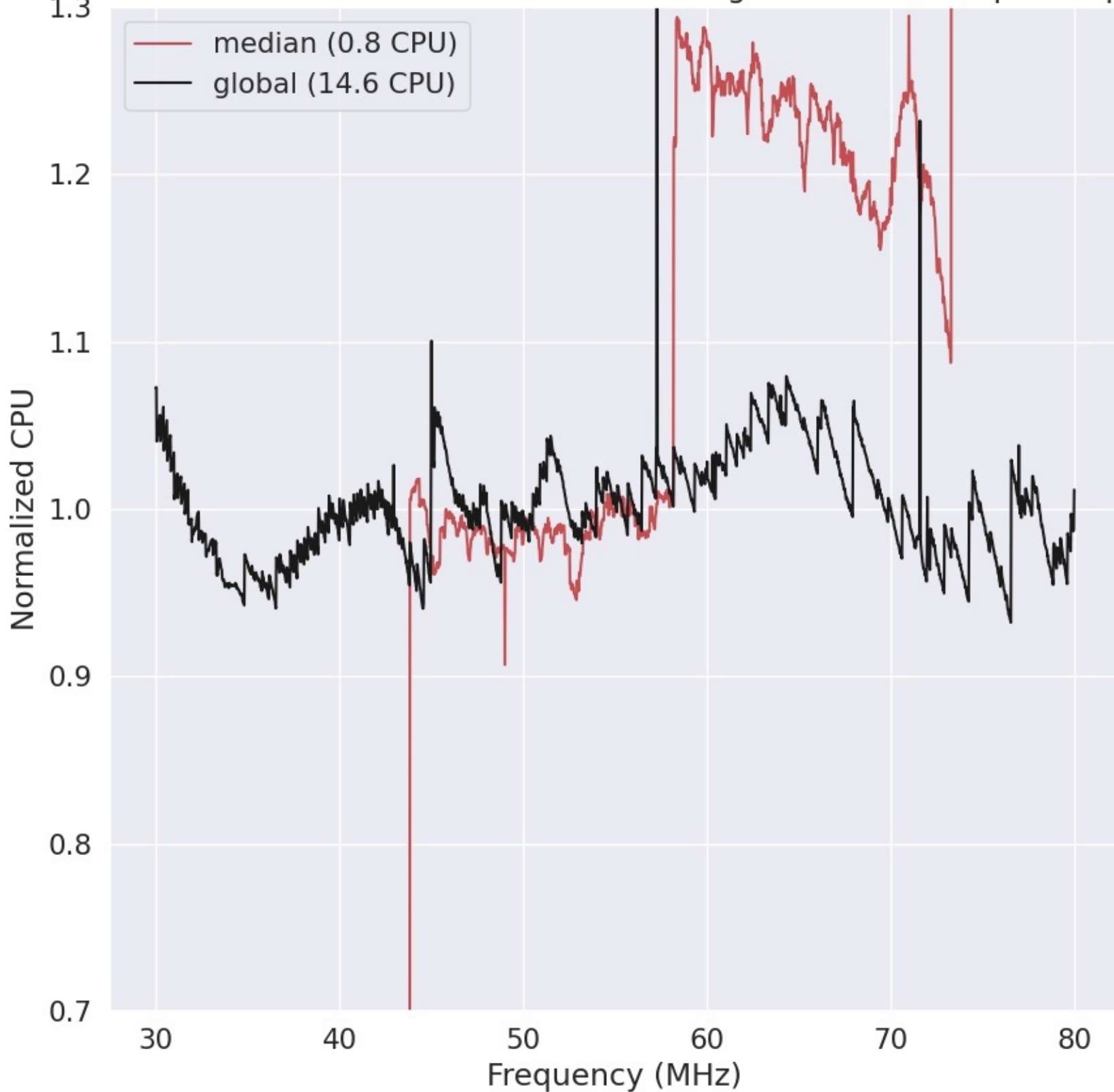
LWA267 - Correlator# 003 - XX - FLAGS:HighTimeVar+BadSpecShape
