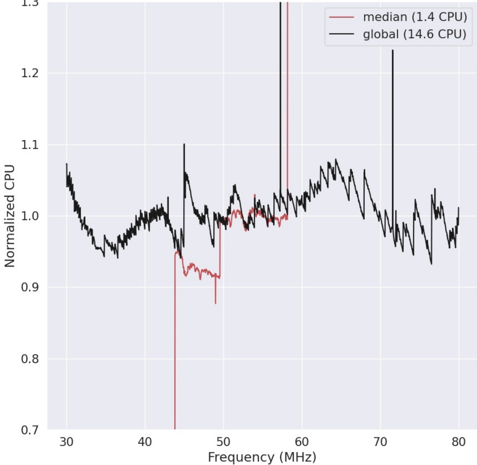
LWA266 - Correlator# 000 - XX - FLAGS:HighTimeVar+BadSpecShape
