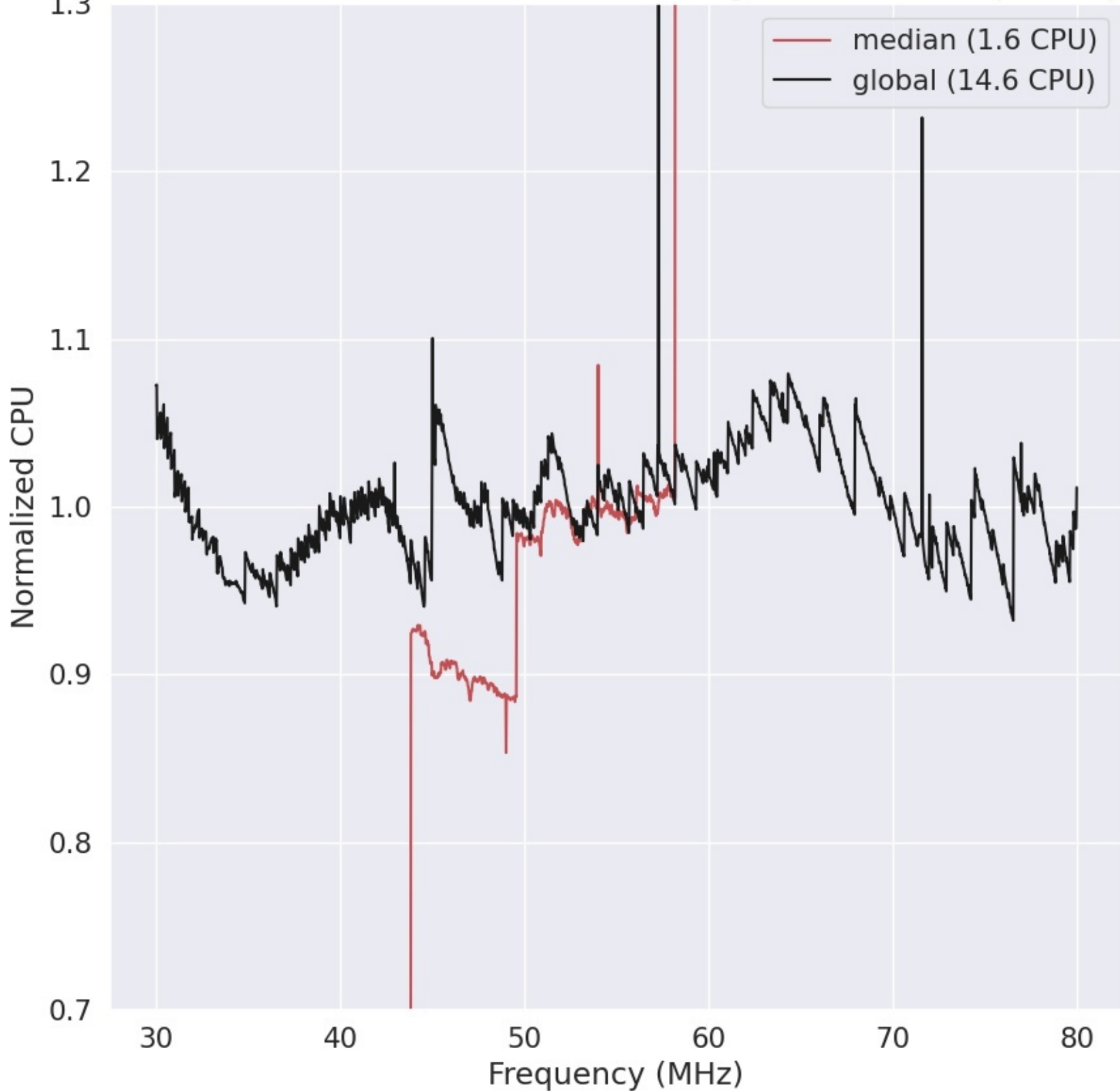
LWA342 - Correlator# 317 - XX - FLAGS:HighTimeVar+BadSpecShape
