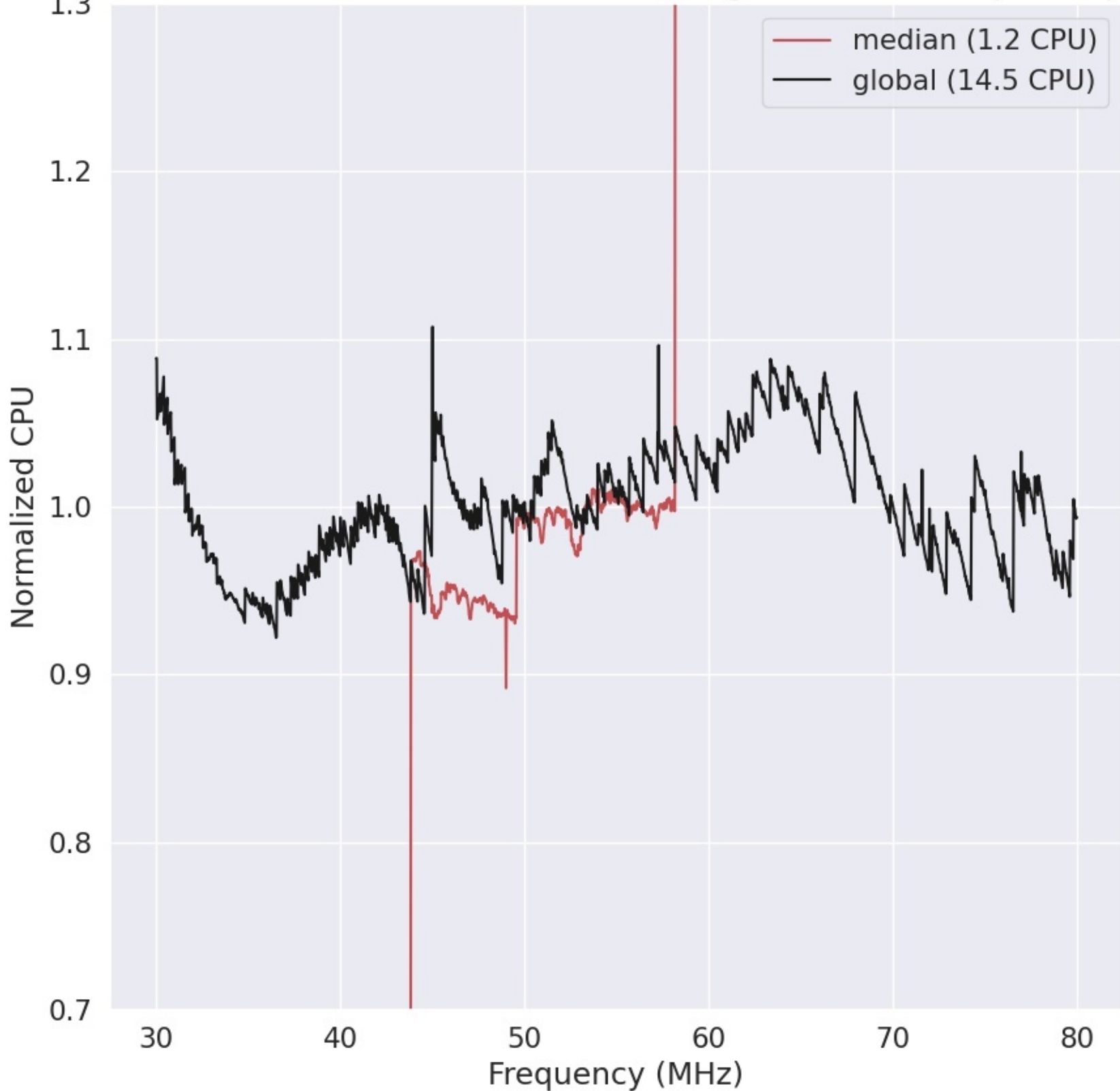
LWA310 - Correlator# 017 - YY - FLAGS:HighTimeVar+BadSpecShape
