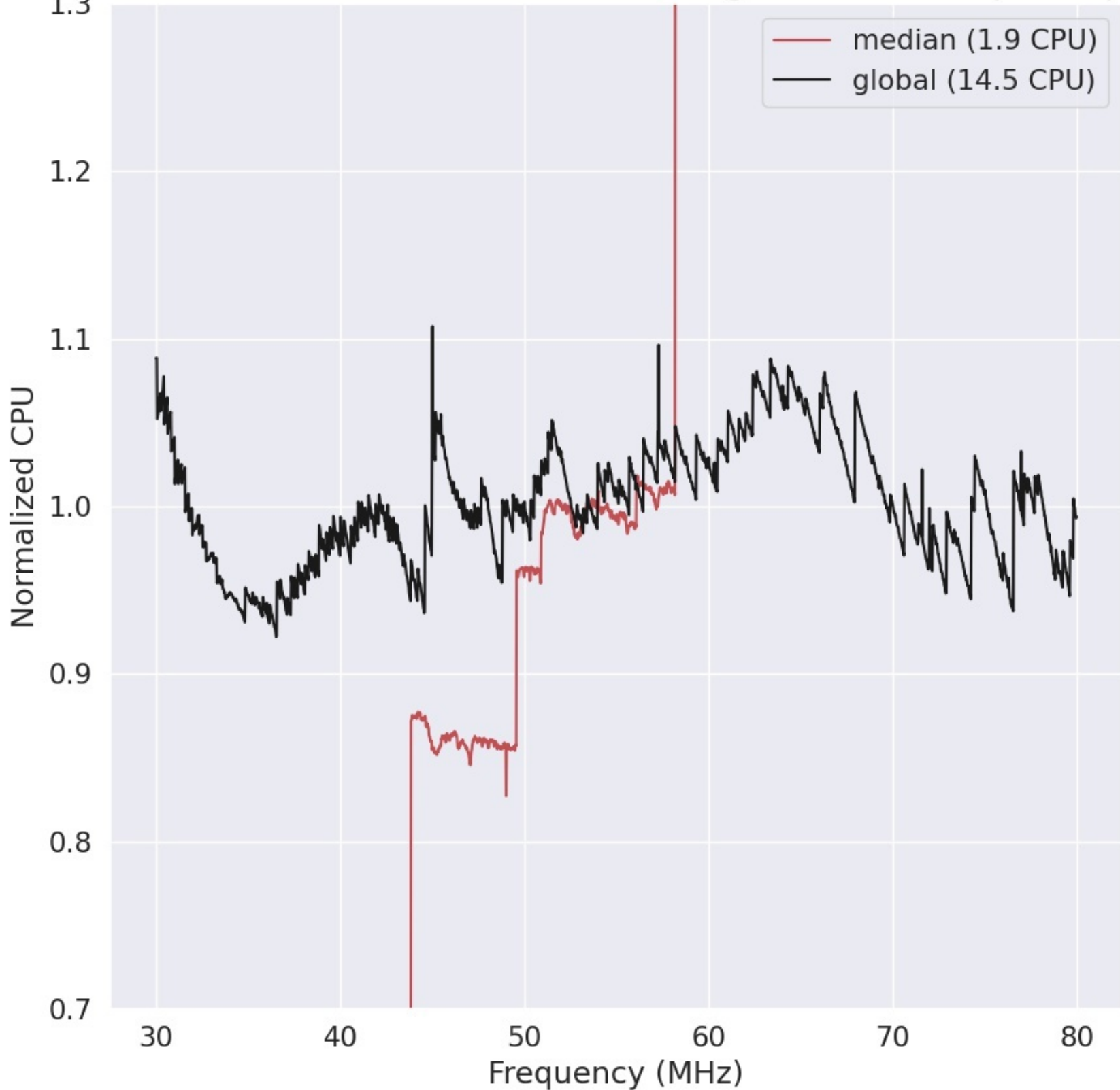
LWA291 - Correlator# 045 - YY - FLAGS:HighTimeVar+BadSpecShape
