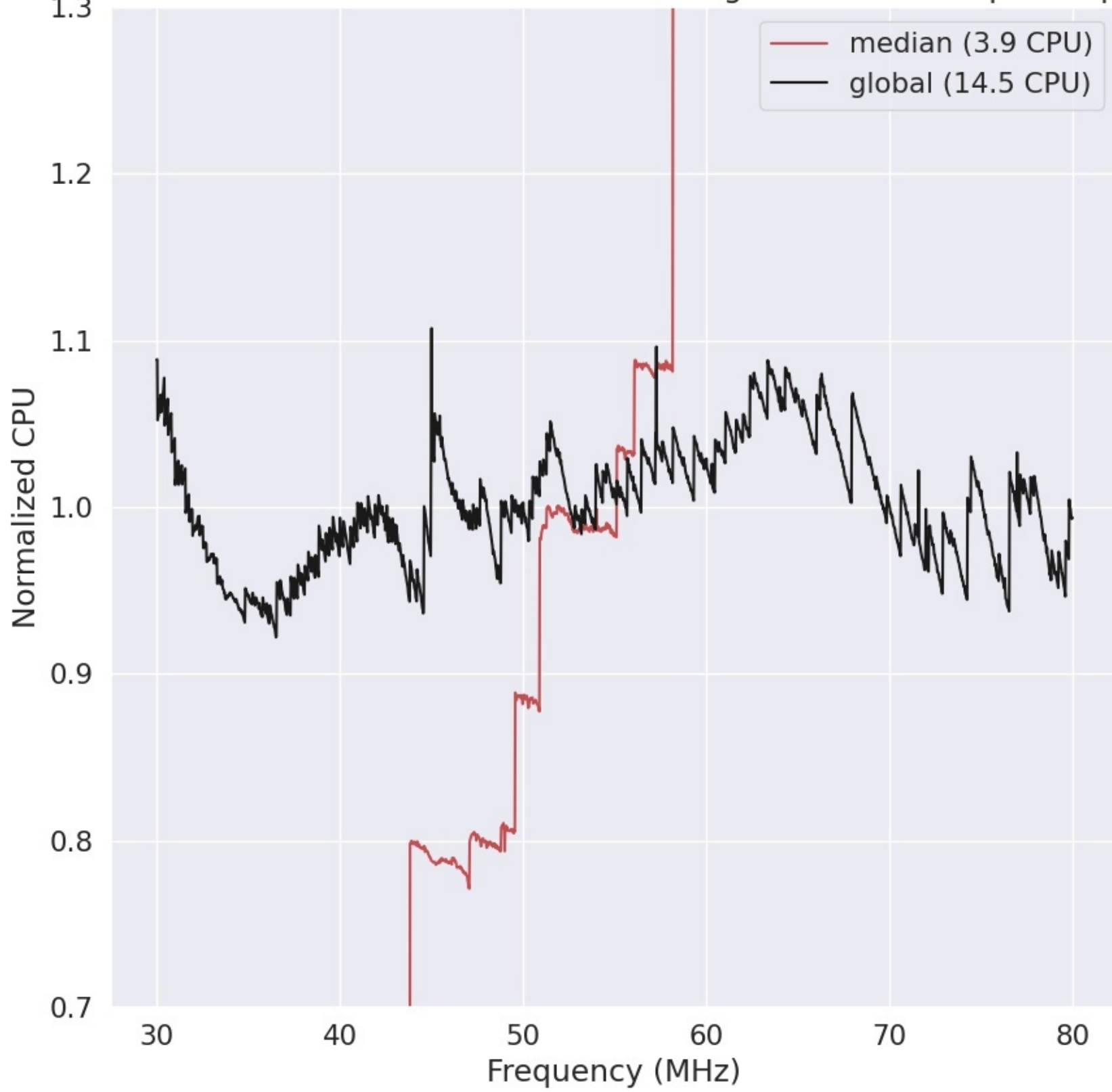
LWA326 - Correlator# 250 - YY - FLAGS:HighTimeVar+BadSpecShape
