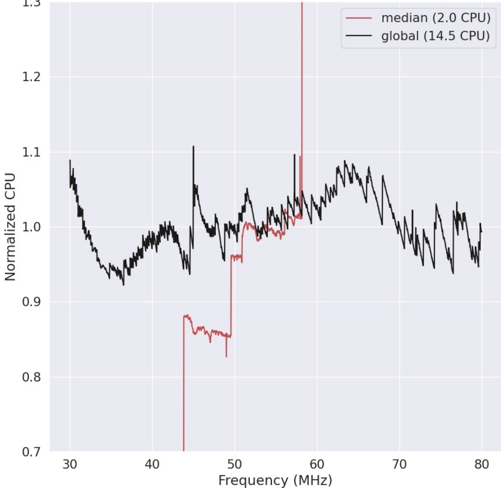
LWA257 - Correlator# 032 - YY - FLAGS:HighTimeVar+BadSpecShape
