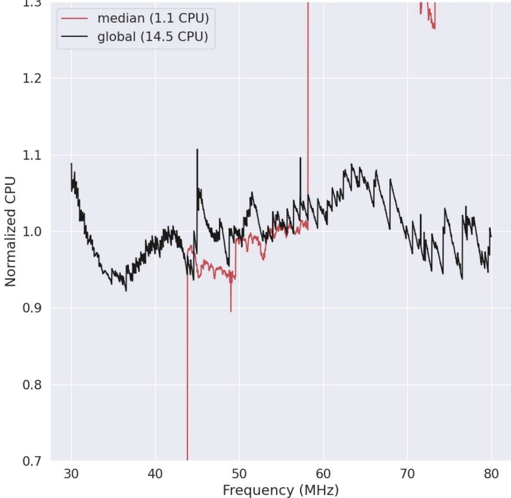
LWA309 - Correlator# 014 - YY - FLAGS:HighTimeVar+BadSpecShape
