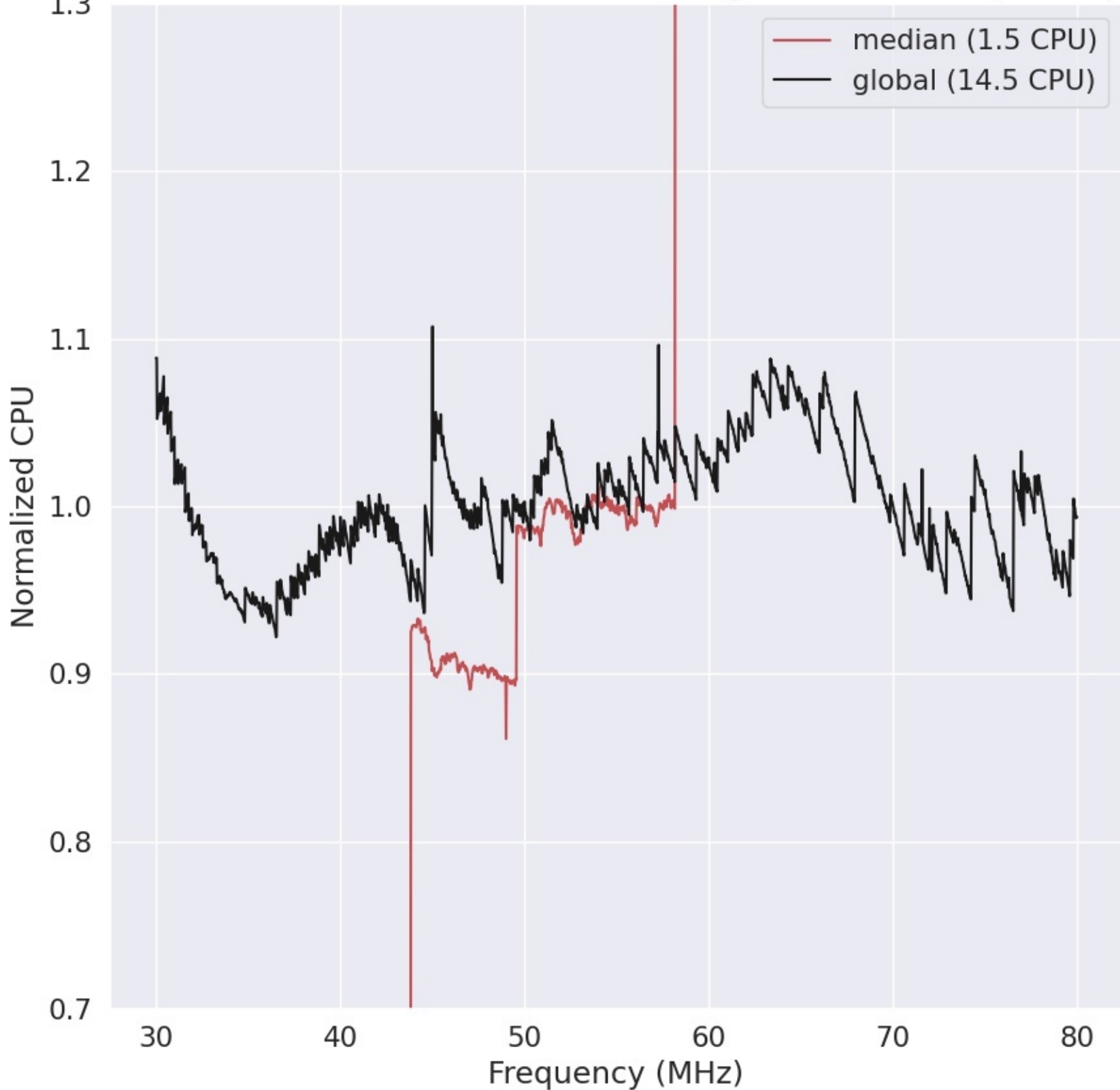
LWA339 - Correlator# 027 - YY - FLAGS:HighTimeVar+BadSpecShape
