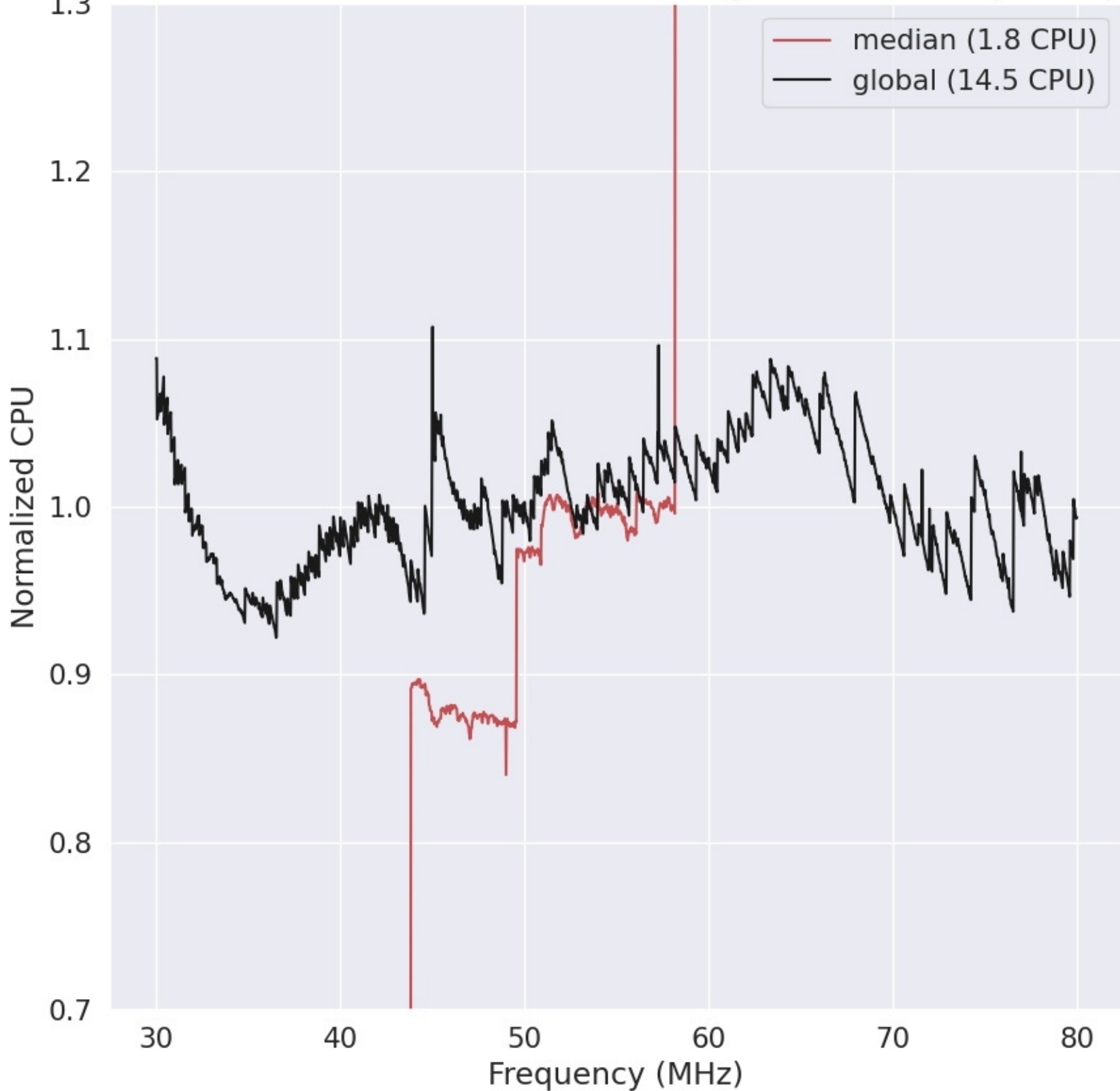
LWA343 - Correlator# 058 - YY - FLAGS:HighTimeVar+BadSpecShape
