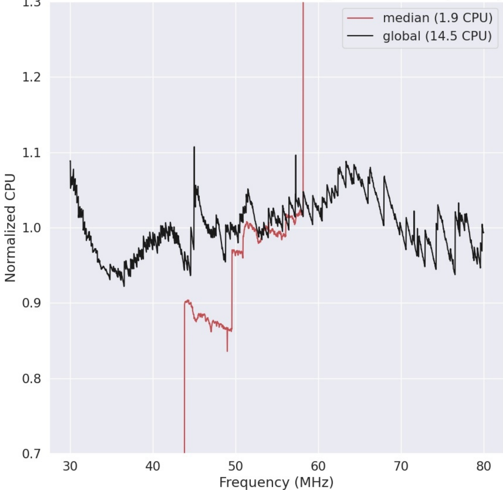
LWA332 - Correlator# 025 - YY - FLAGS:HighTimeVar+BadSpecShape
