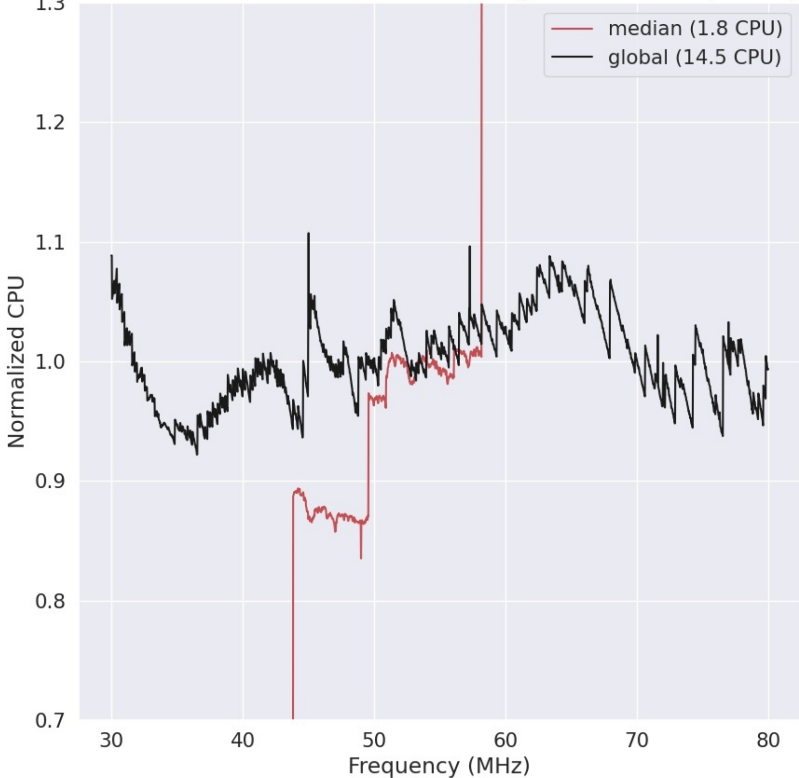
LWA327 - Correlator# 023 - YY - FLAGS:HighTimeVar+BadSpecShape
