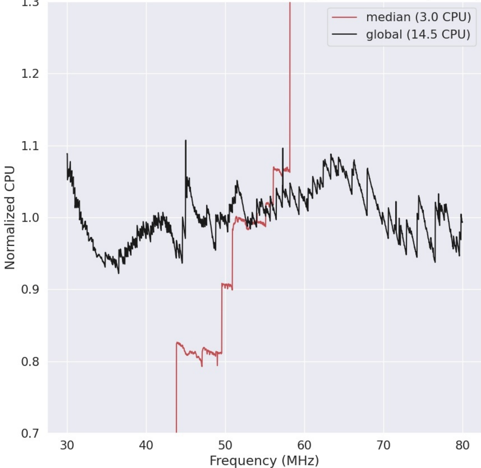
LWA342 - Correlator# 317 - YY - FLAGS:HighTimeVar+BadSpecShape
