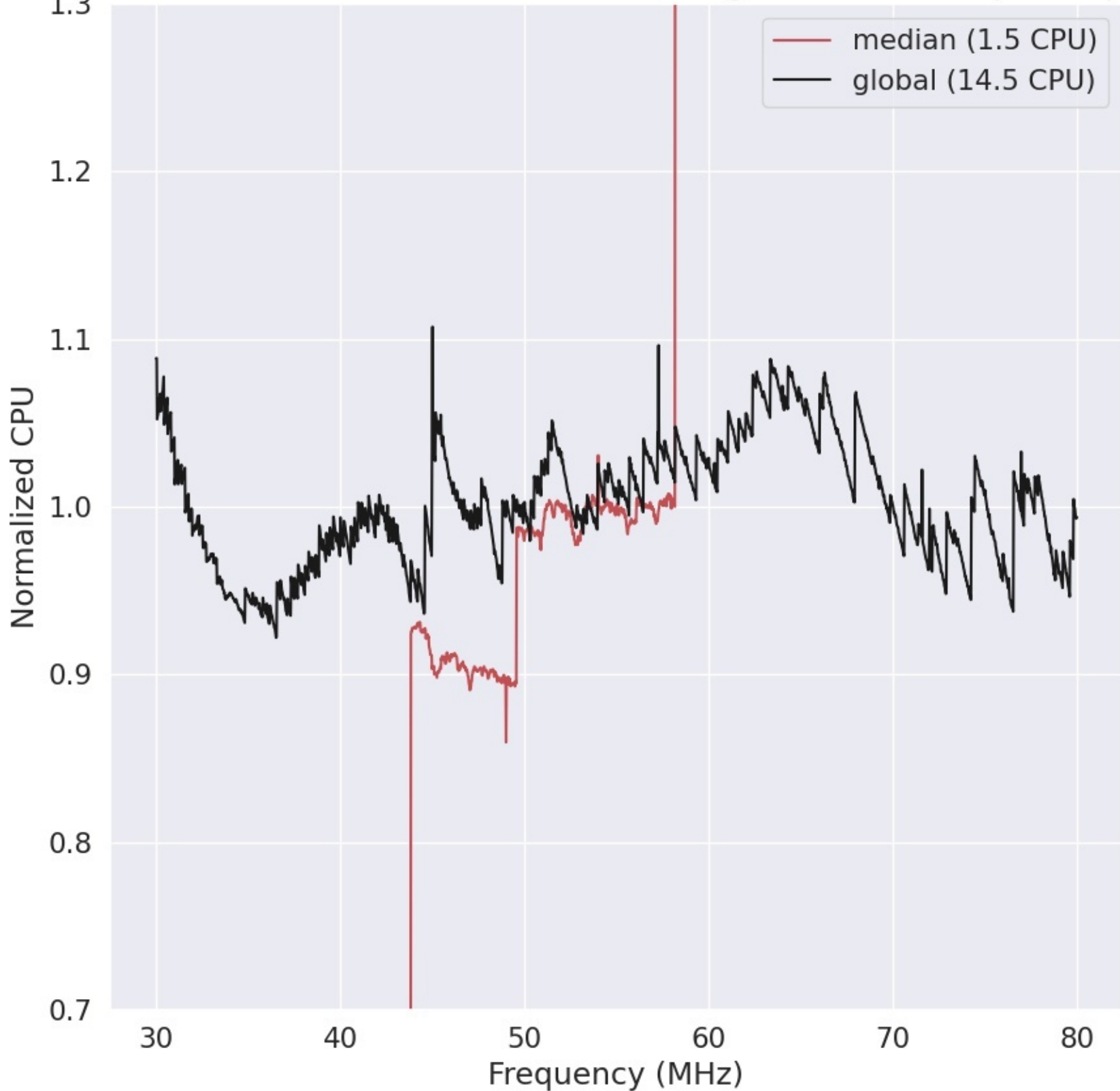
LWA298 - Correlator# 049 - YY - FLAGS:HighTimeVar+BadSpecShape
