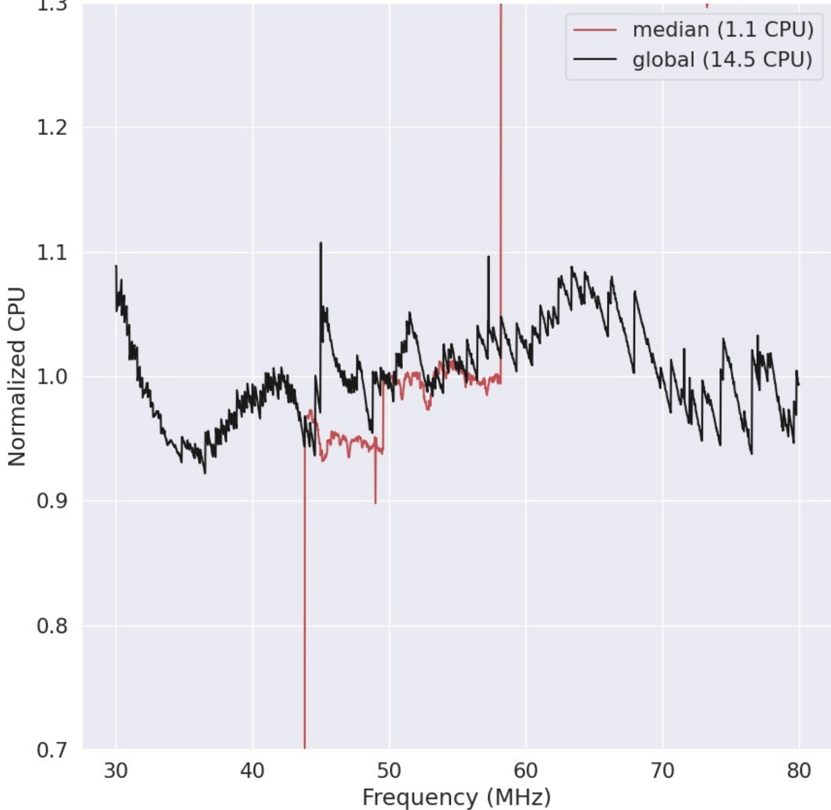
LWA258 - Correlator# 035 - YY - FLAGS:HighTimeVar+BadSpecShape
