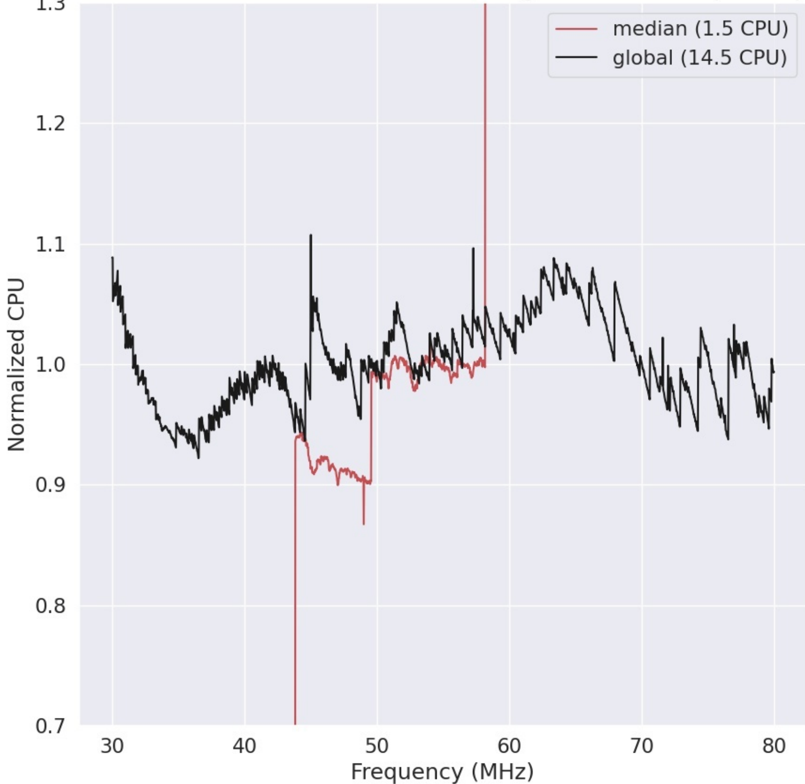
LWA268 - Correlator# 002 - YY - FLAGS:HighTimeVar+BadSpecShape
