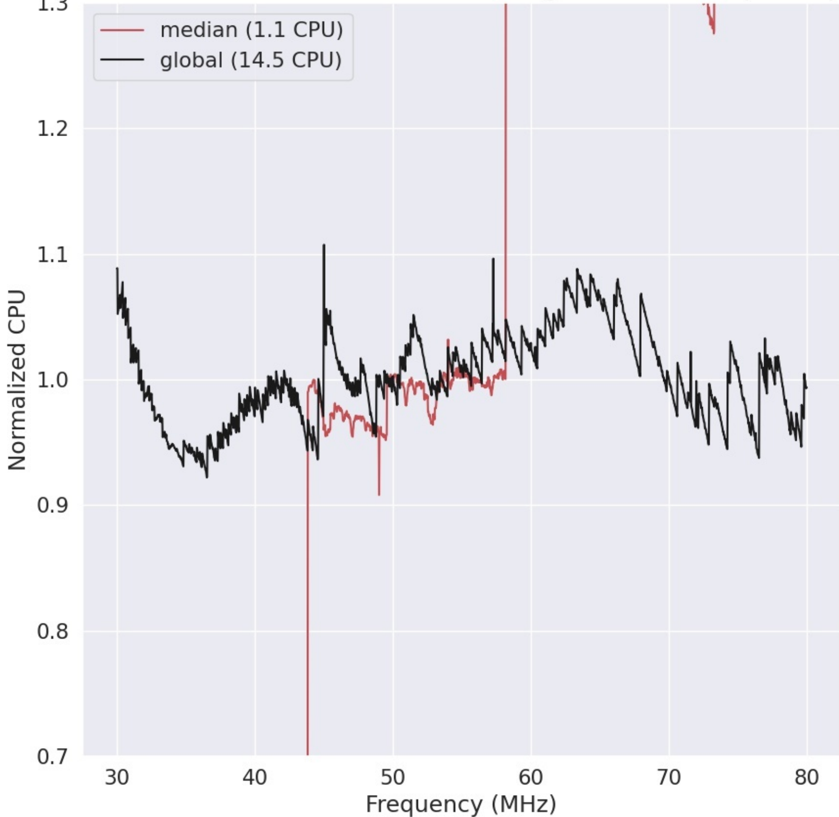
LWA316 - Correlator# 155 - YY - FLAGS:HighTimeVar+BadSpecShape
