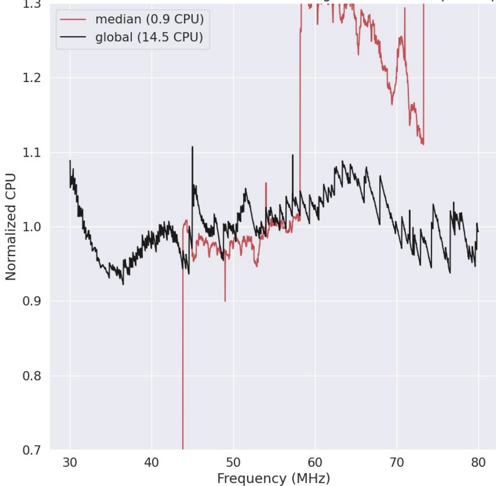
LWA285 - Correlator# 013 - YY - FLAGS:HighTimeVar+BadSpecShape
