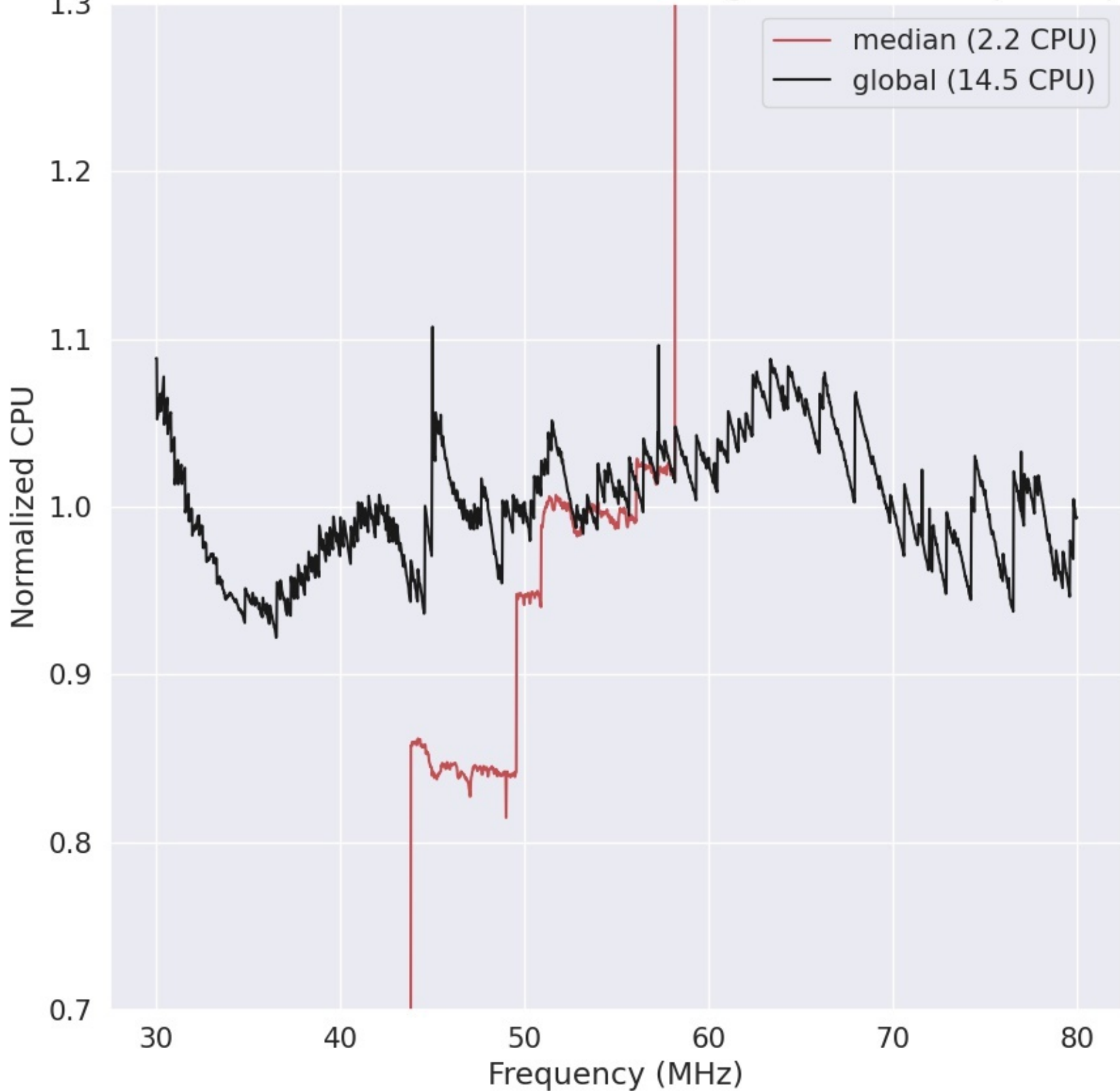
LWA279 - Correlator# 220 - YY - FLAGS:HighTimeVar+BadSpecShape
