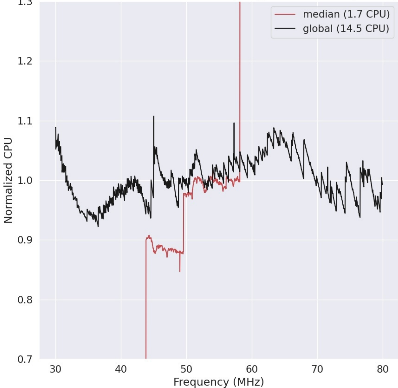
LWA289 - Correlator# 189 - YY - FLAGS:HighTimeVar+BadSpecShape
