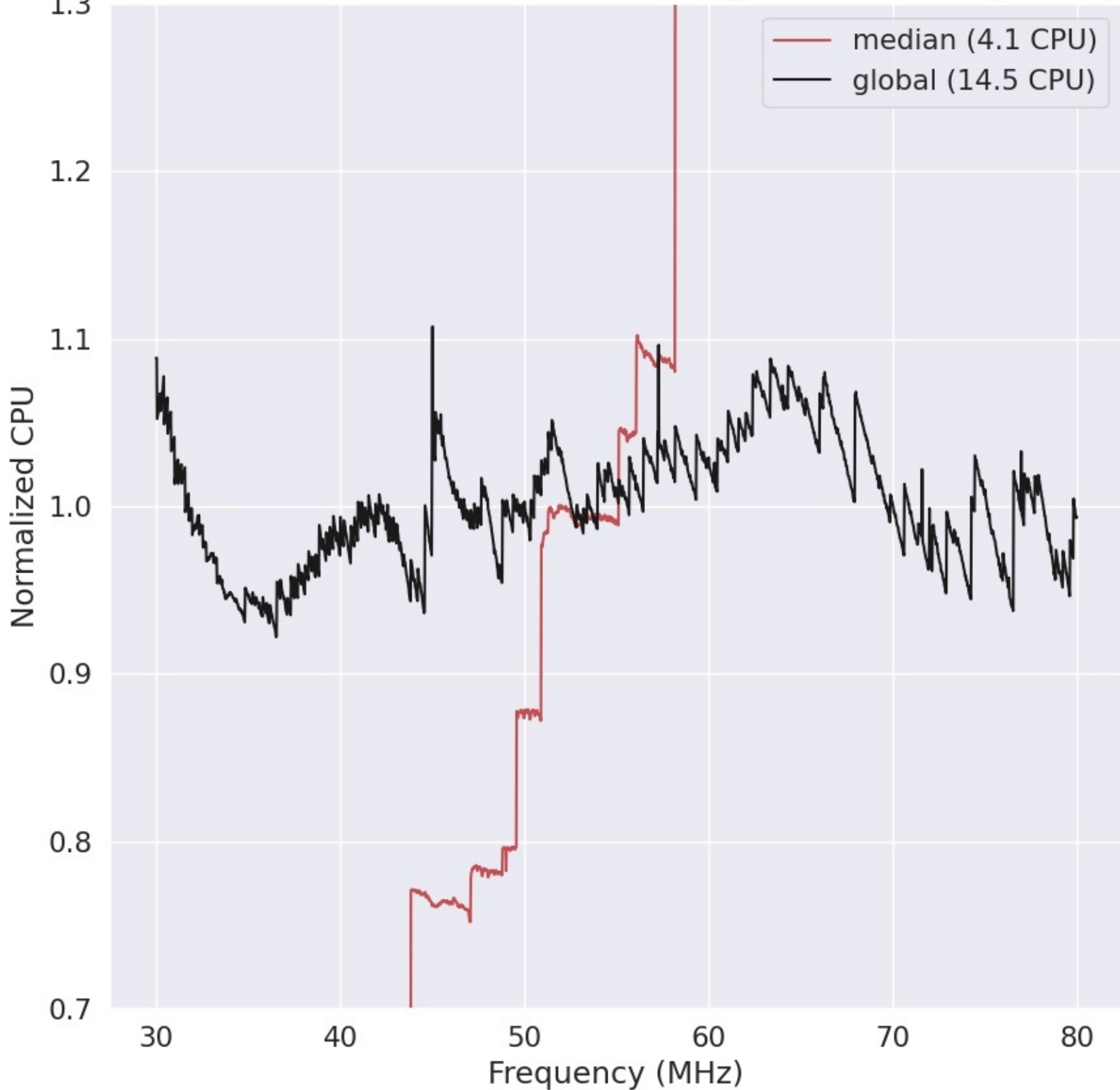
LWA354 - Correlator# 063 - YY - FLAGS:HighTimeVar+BadSpecShape
