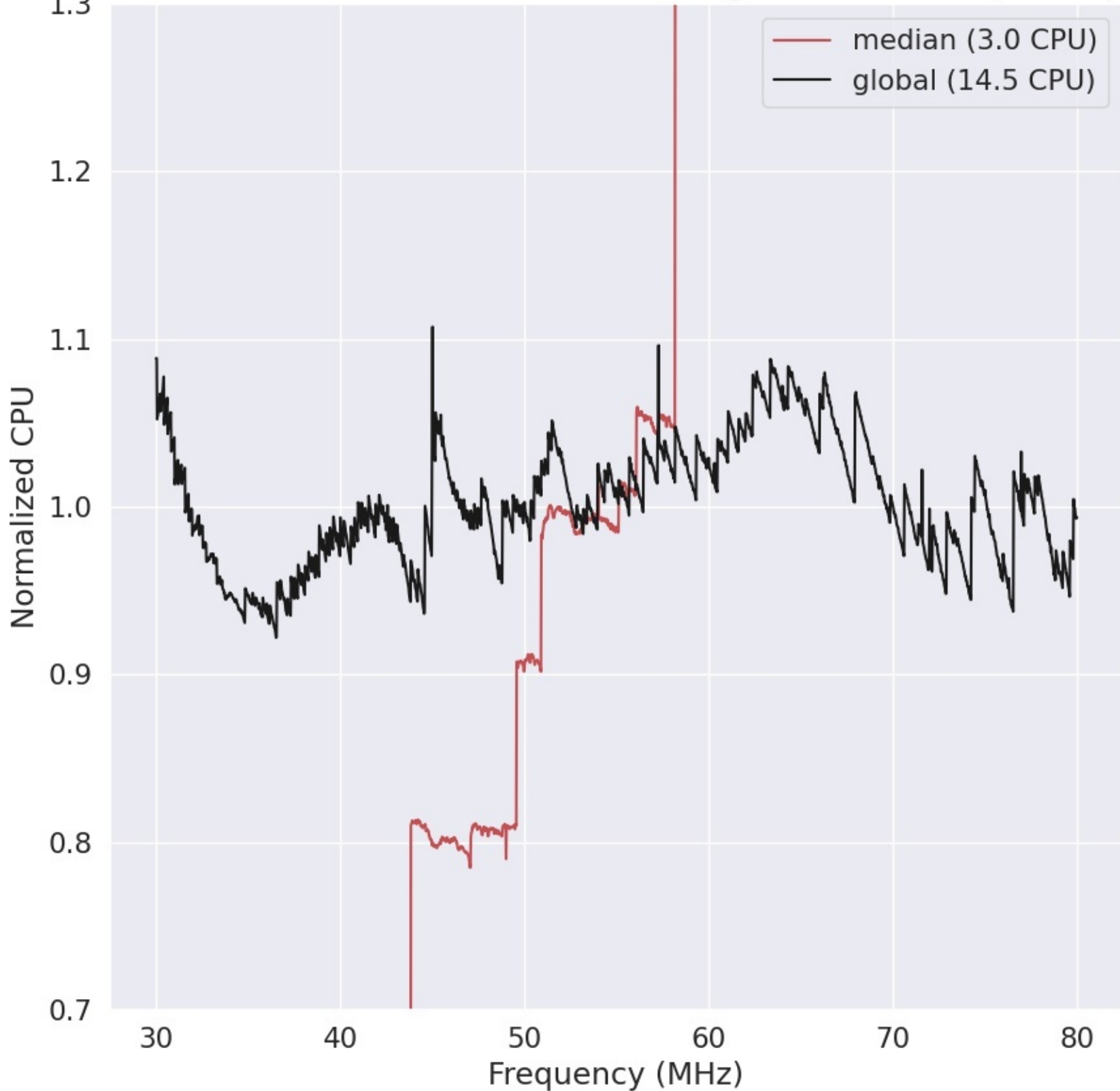
LWA344 - Correlator# 061 - YY - FLAGS:HighTimeVar+BadSpecShape
