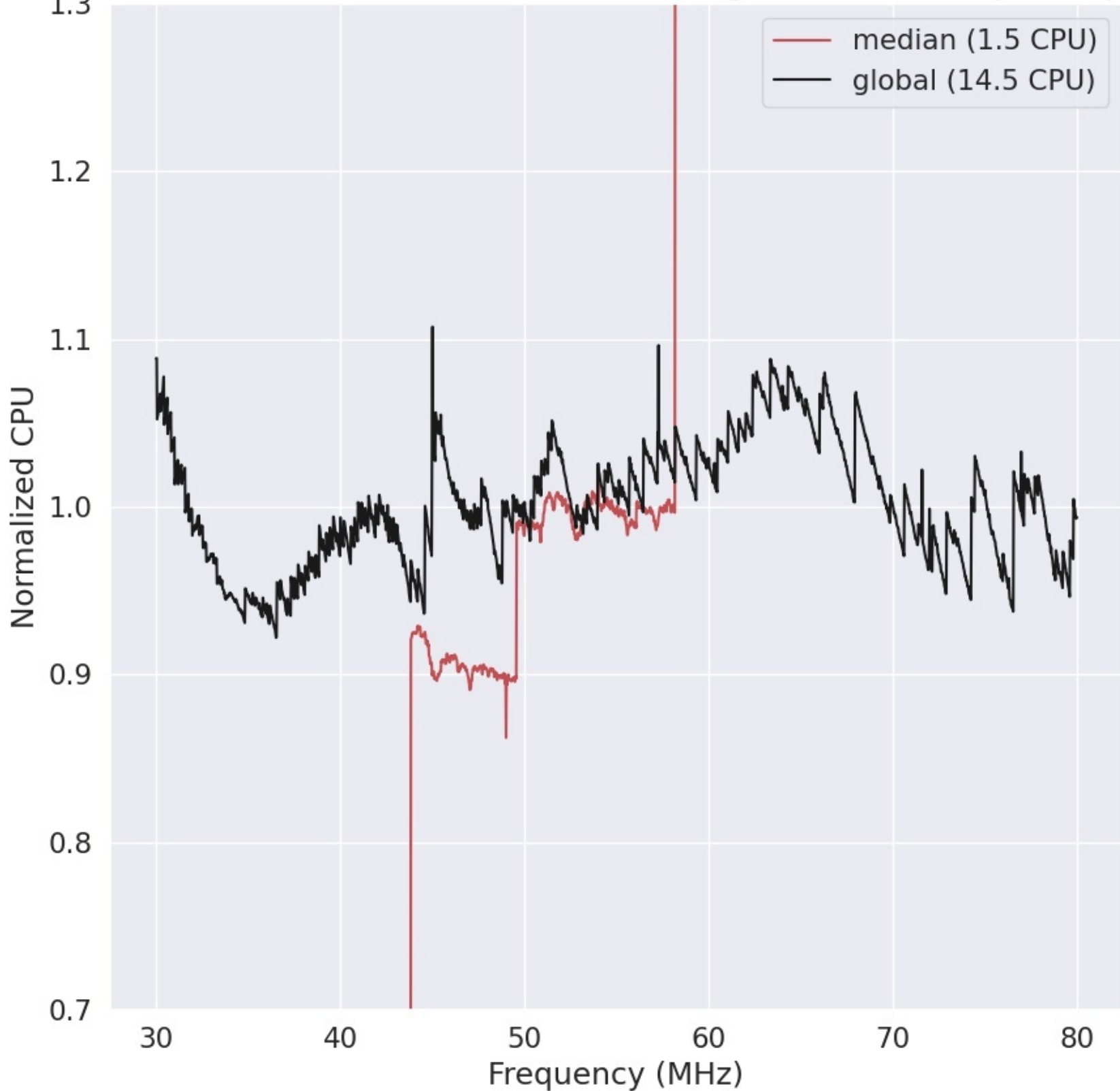
LWA320 - Correlator# 054 - YY - FLAGS:HighTimeVar+BadSpecShape
