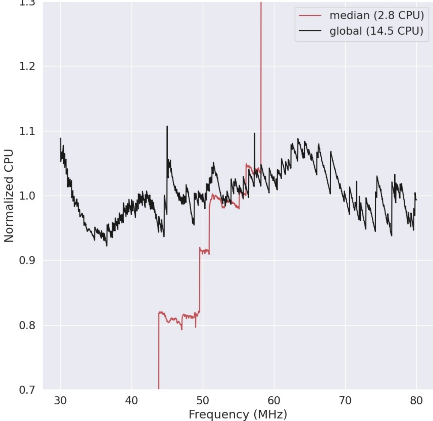
LWA321 - Correlator# 020 - YY - FLAGS:HighTimeVar+BadSpecShape
