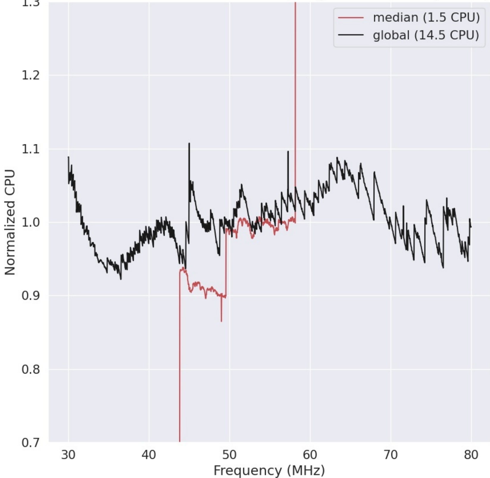
LWA313 - Correlator# 018 - YY - FLAGS:HighTimeVar+BadSpecShape
