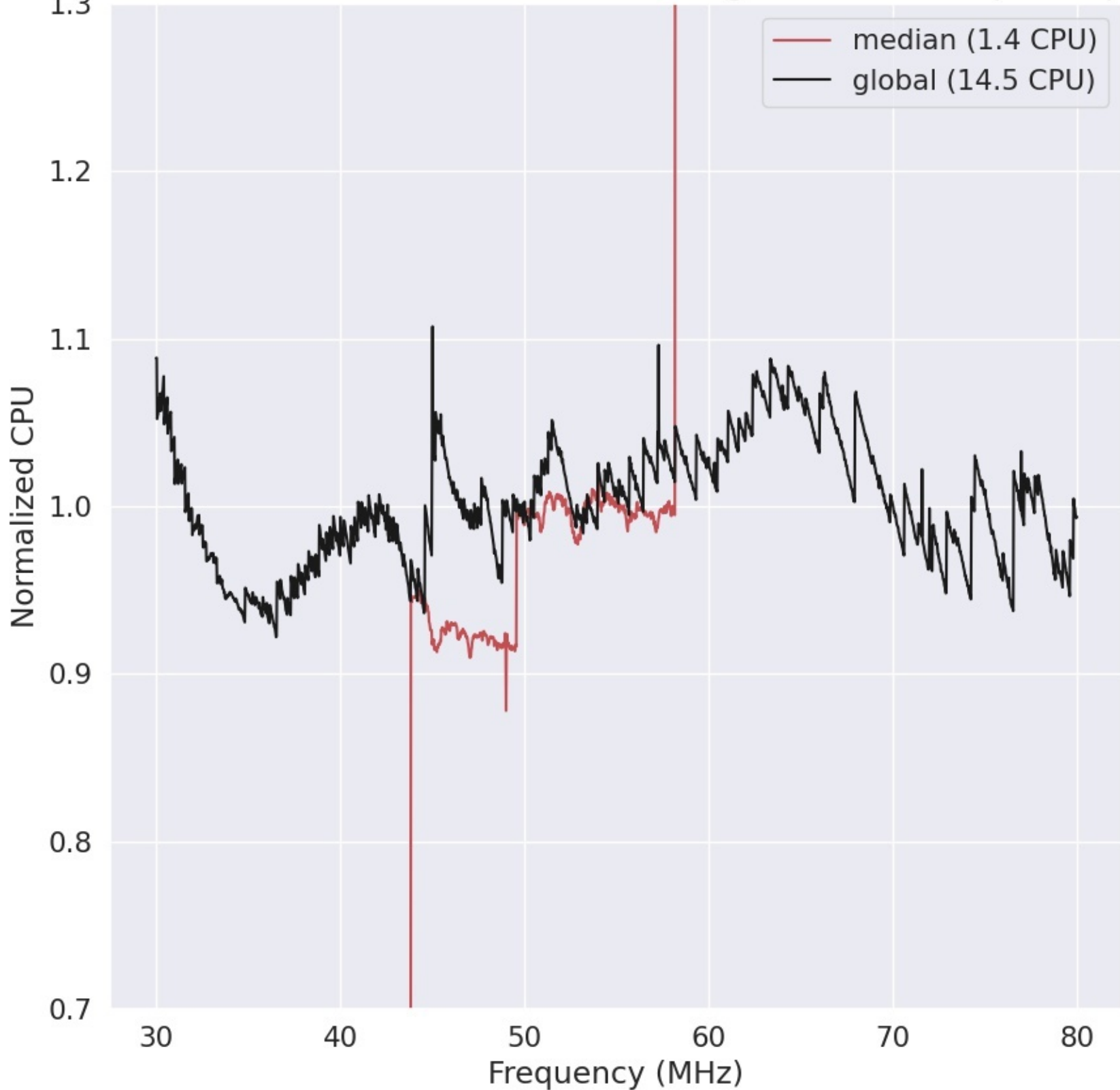
LWA272 - Correlator# 038 - YY - FLAGS:HighTimeVar+BadSpecShape
