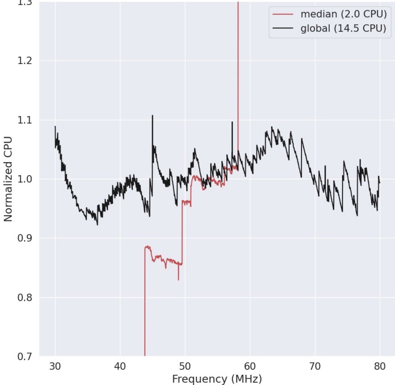
LWA259 - Correlator# 001 - YY - FLAGS:HighTimeVar+BadSpecShape
