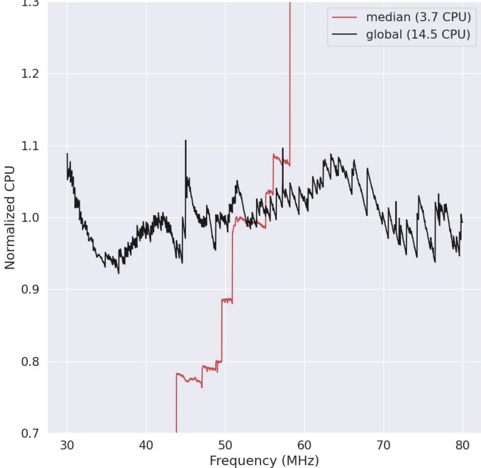
LWA269 - Correlator# 005 - YY - FLAGS:HighTimeVar+BadSpecShape
