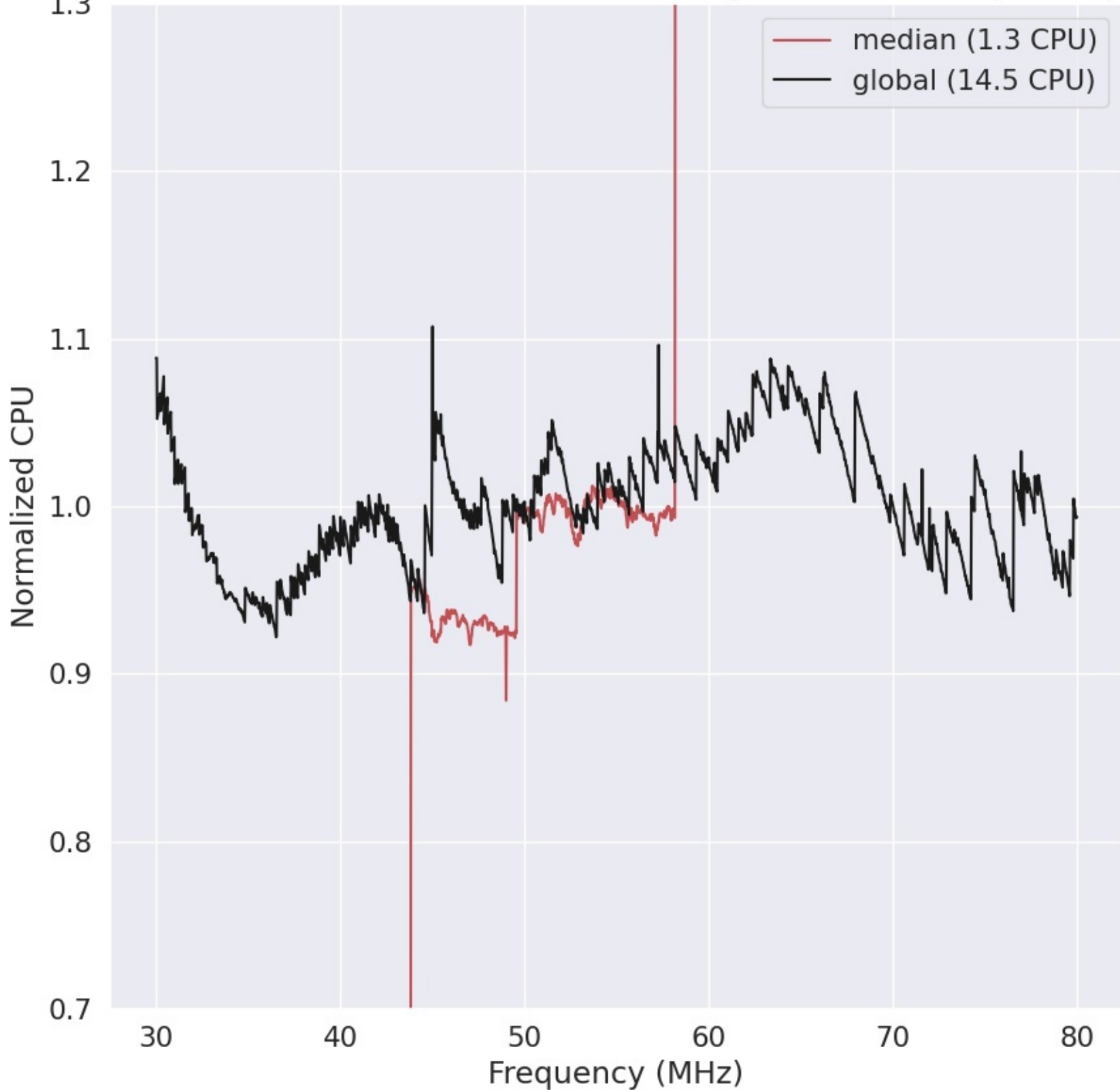
LWA282 - Correlator# 010 - YY - FLAGS:HighTimeVar+BadSpecShape
