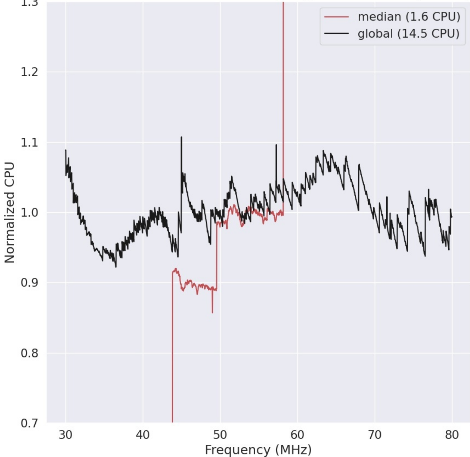
LWA330 - Correlator# 022 - YY - FLAGS:HighTimeVar+BadSpecShape
