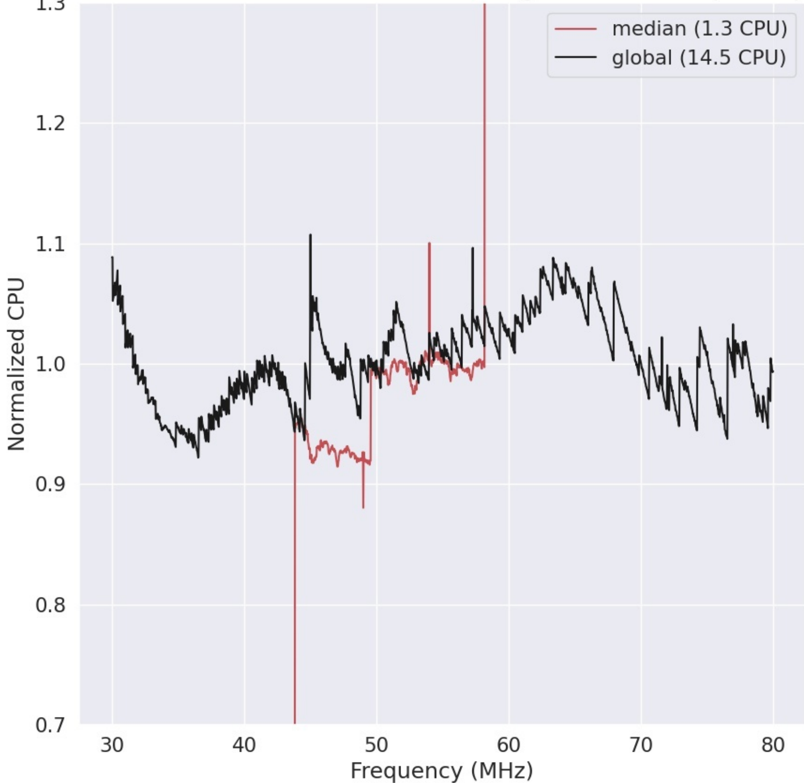
LWA270 - Correlator# 039 - YY - FLAGS:HighTimeVar+BadSpecShape
