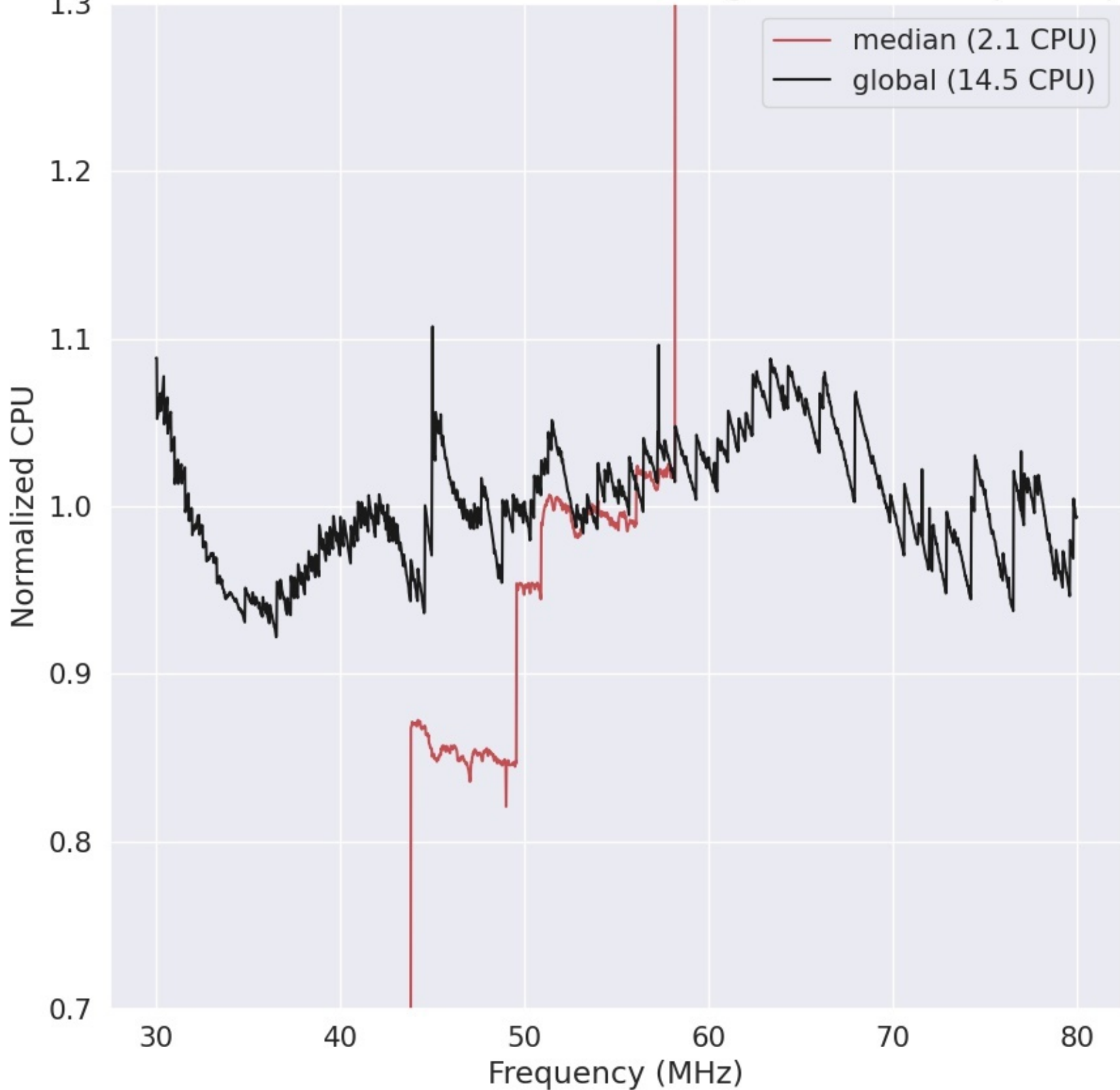
LWA276 - Correlator# 006 - YY - FLAGS:HighTimeVar+BadSpecShape
