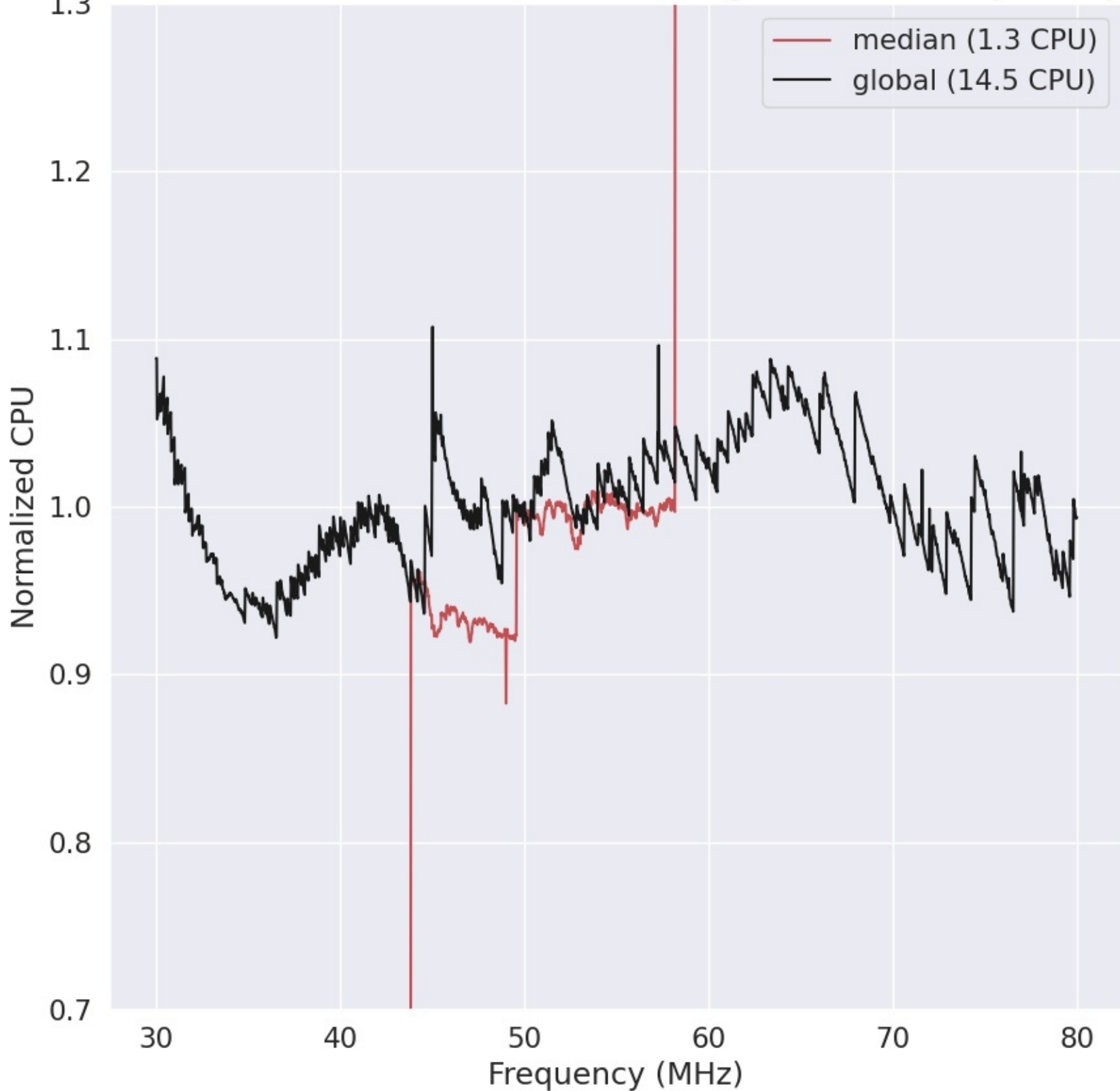
LWA267 - Correlator# 003 - YY - FLAGS:HighTimeVar+BadSpecShape
