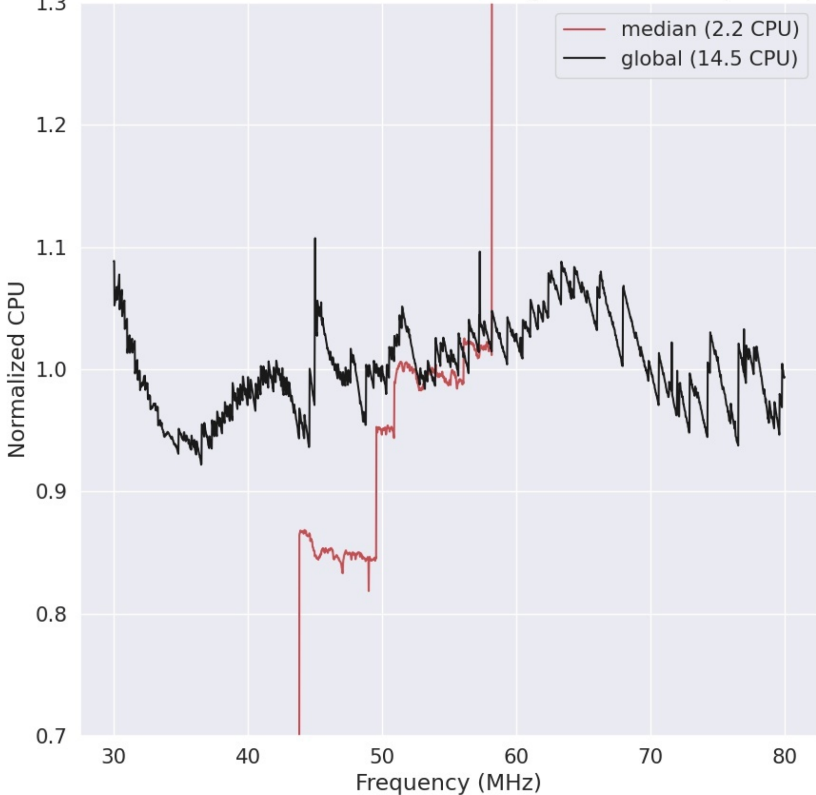
LWA319 - Correlator# 190 - YY - FLAGS:HighTimeVar+BadSpecShape
