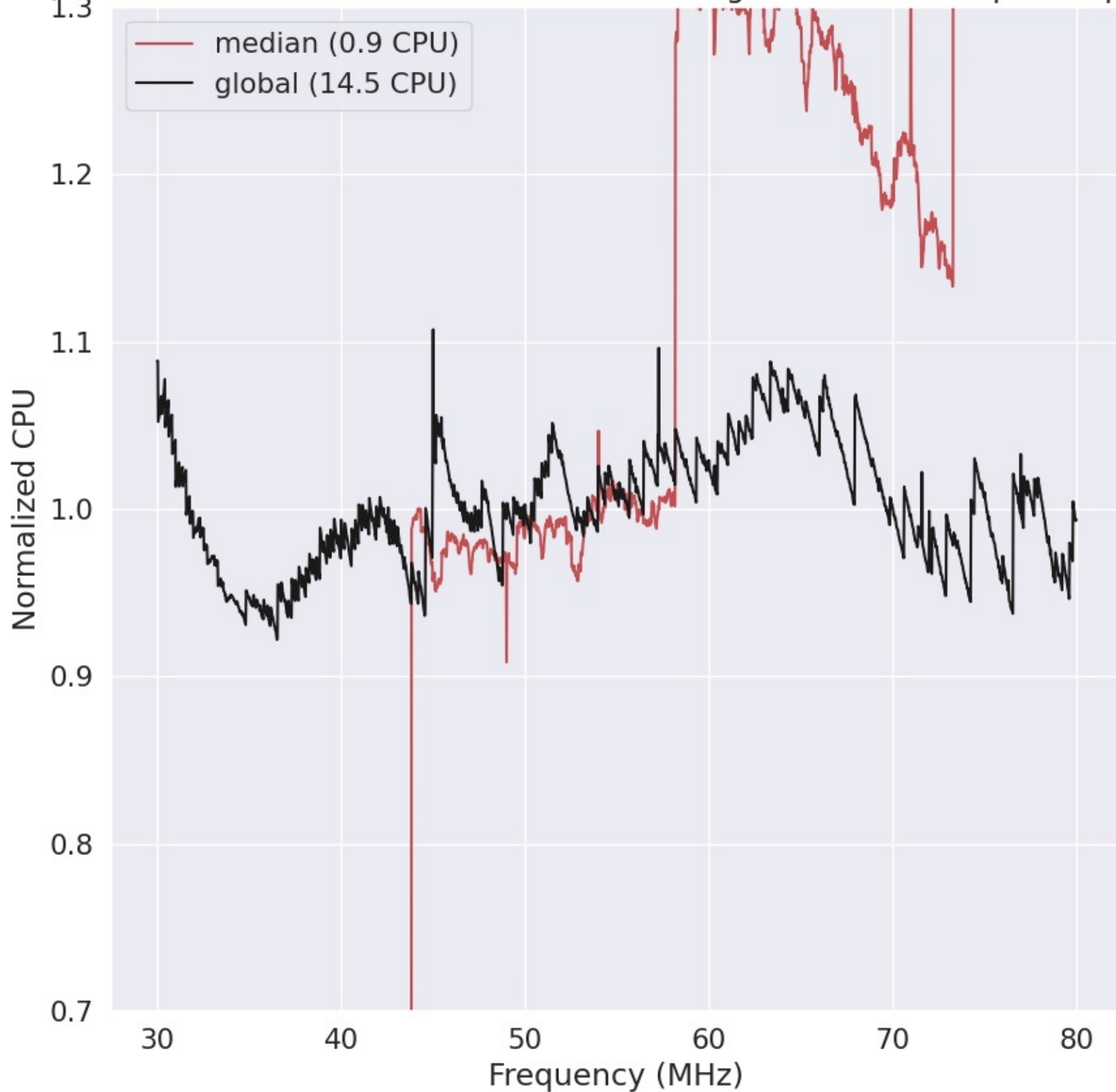
LWA273 - Correlator# 007 - YY - FLAGS:HighTimeVar+BadSpecShape
