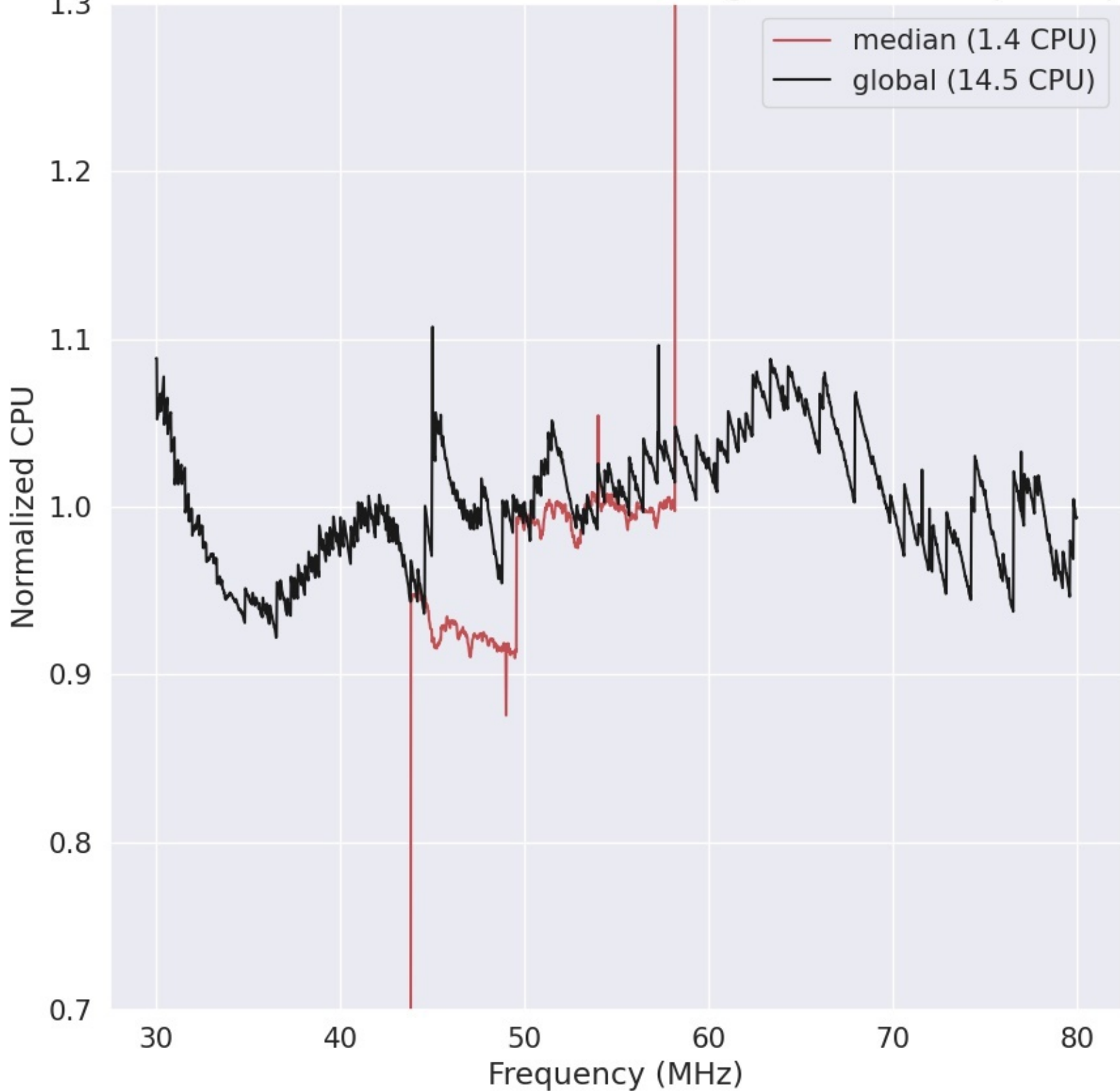
LWA295 - Correlator# 047 - YY - FLAGS:HighTimeVar+BadSpecShape
