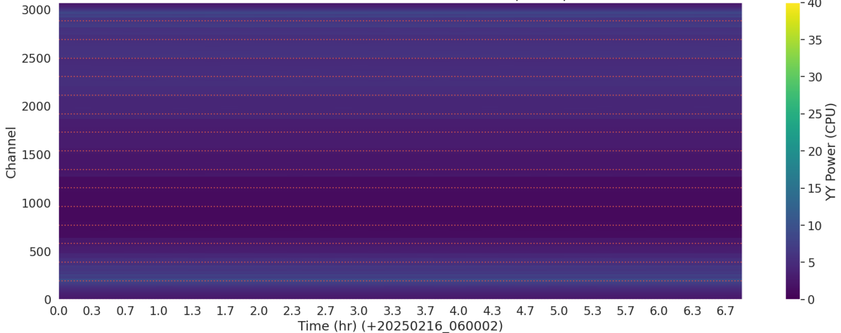
LWA342 - Correlator# 317 - YY - FLAGS: BadSpecShape
