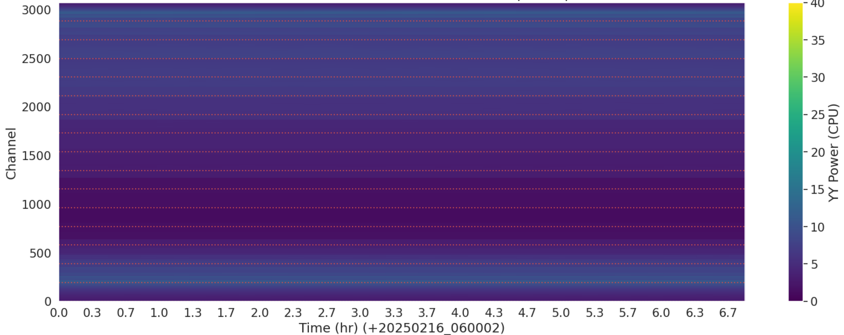
LWA335 - Correlator# 057 - YY - FLAGS: BadSpecShape
