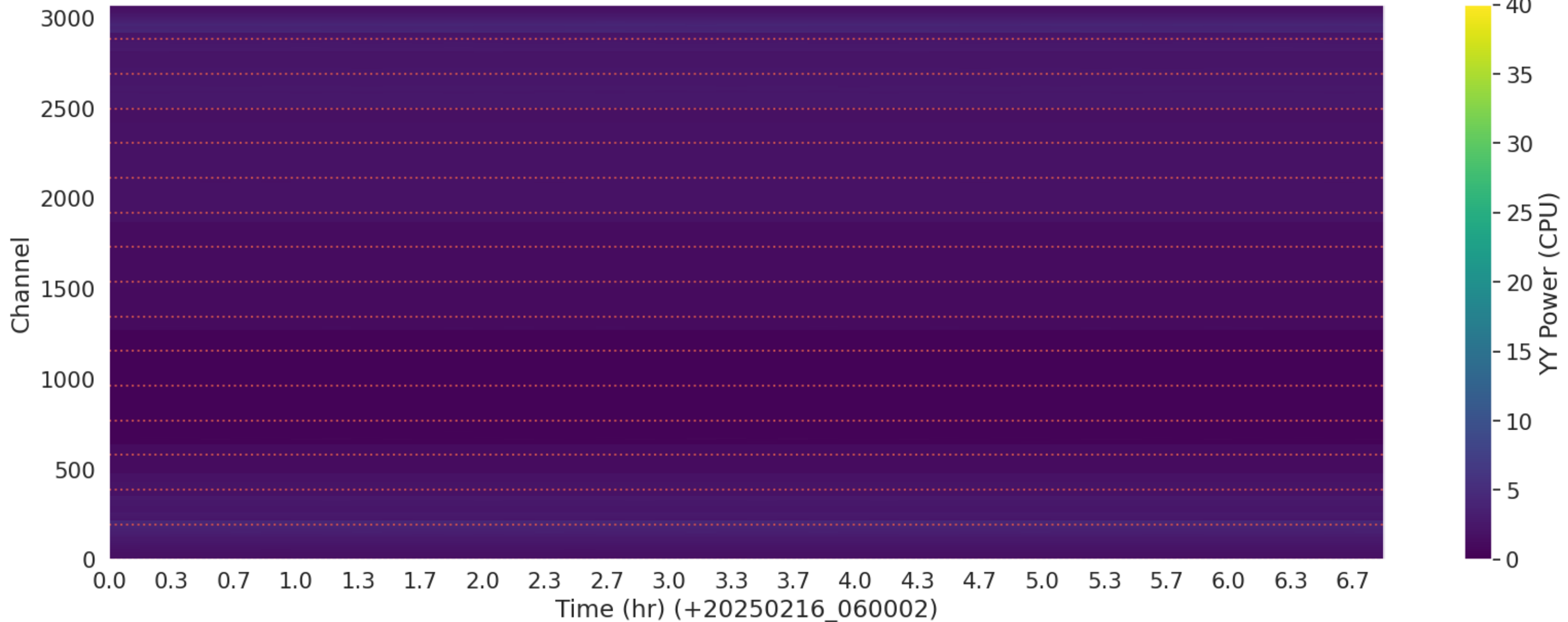
LWA270 - Correlator# 039 - YY - FLAGS: LowPower
