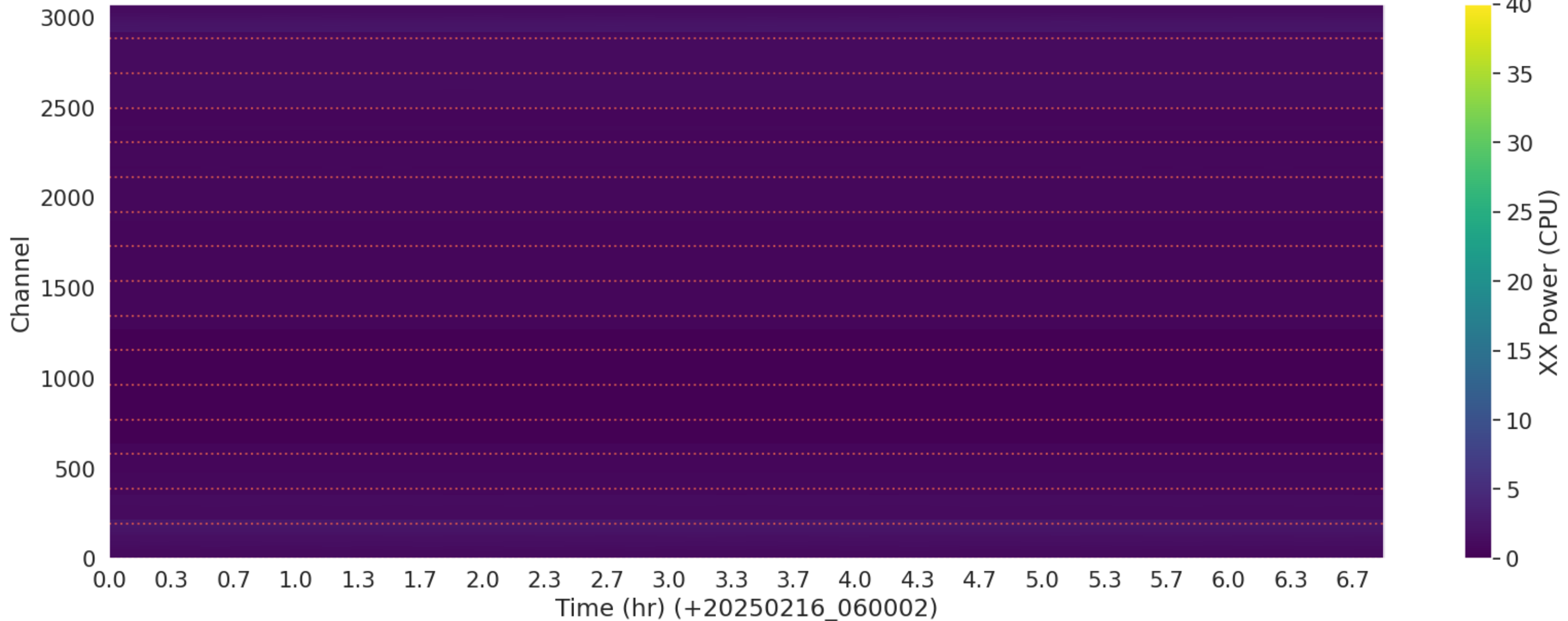
LWA281 - Correlator# 011 - XX - FLAGS: LowPower
