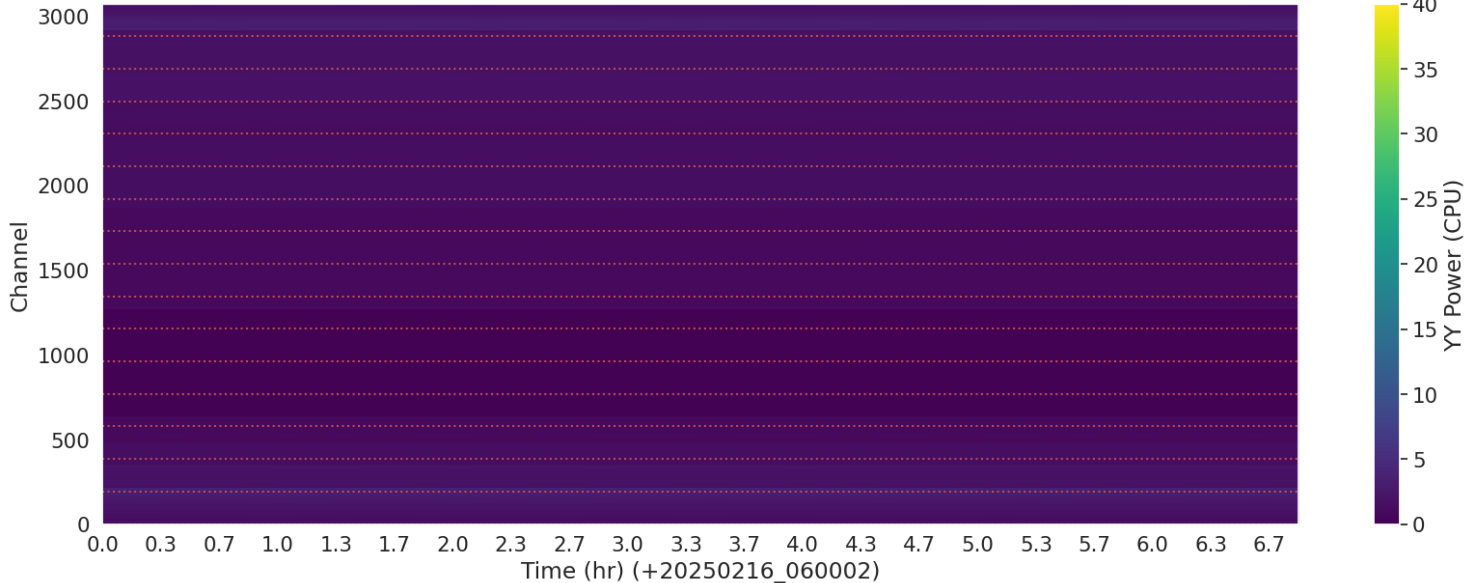
LWA353 - Correlator# 031 - YY - FLAGS: LowPower
