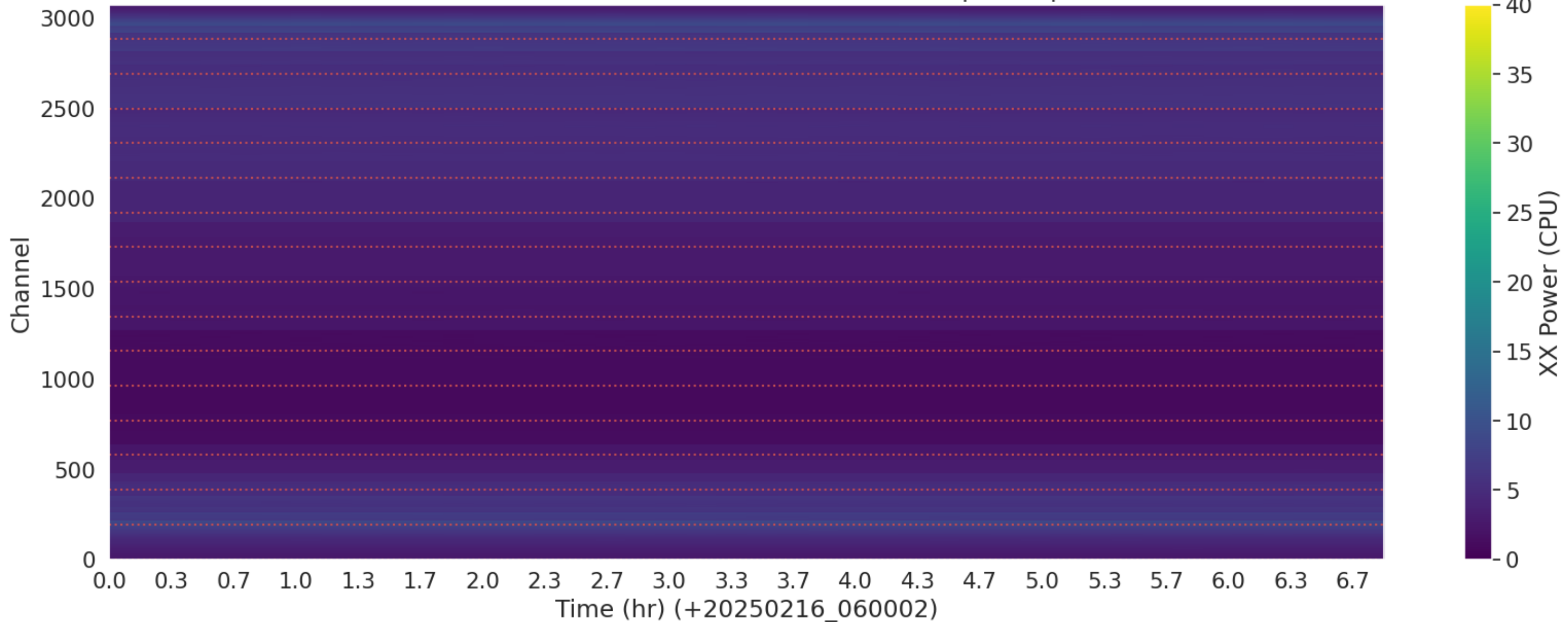
LWA283 - Correlator# 040 - XX - FLAGS: BadSpecShape
