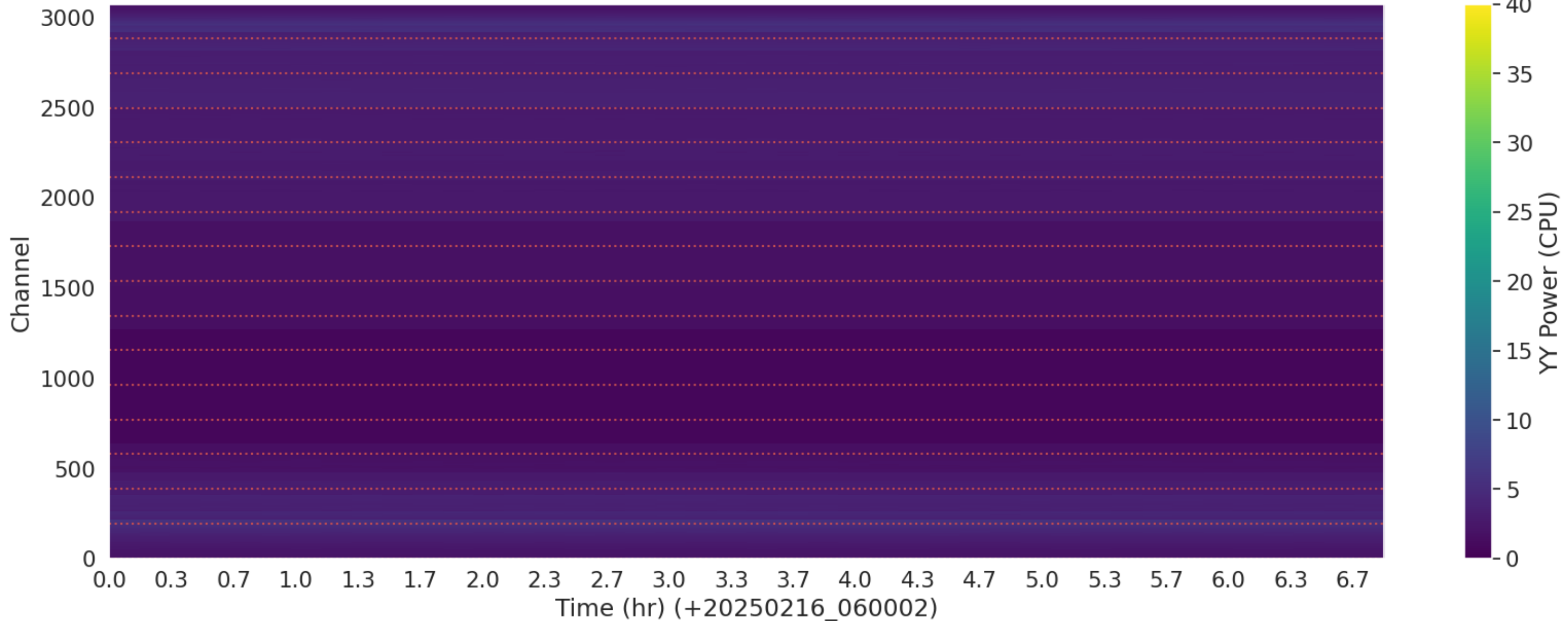
LWA327 - Correlator# 023 - YY - FLAGS: LowPower
