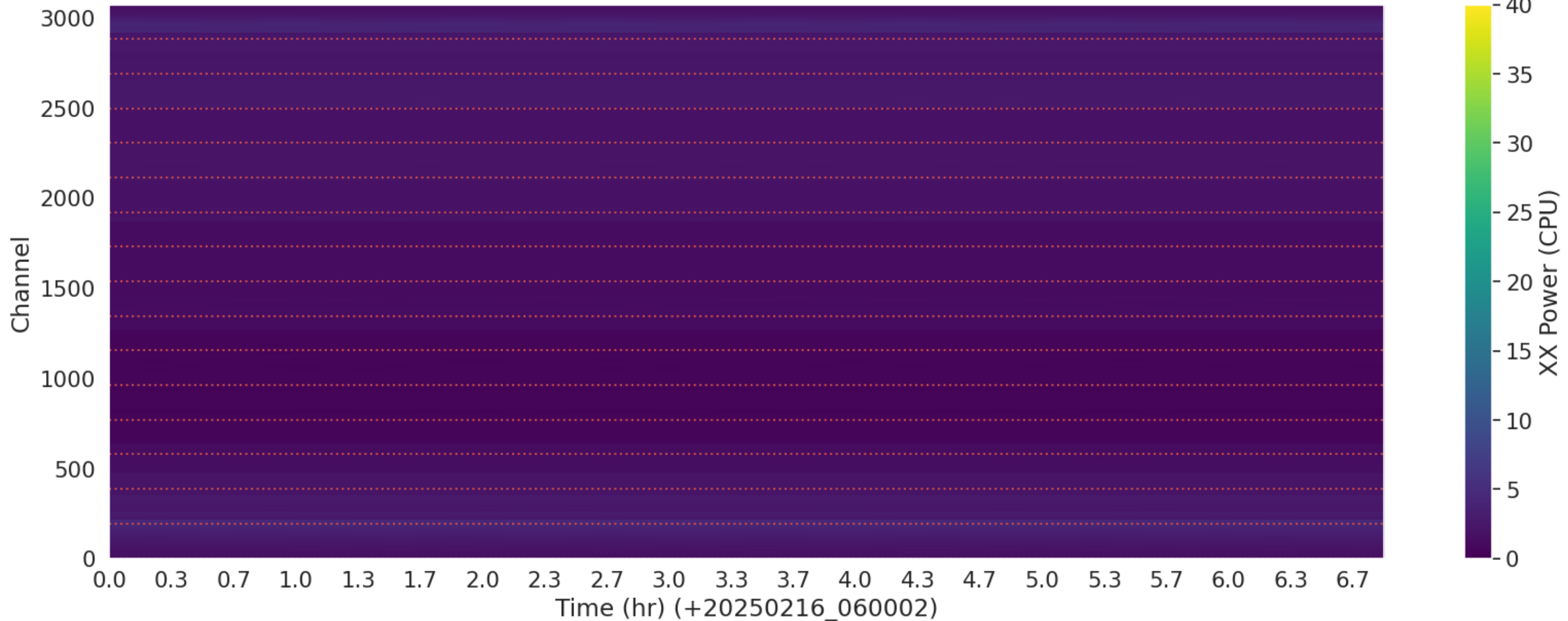
LWA266 - Correlator# 000 - XX - FLAGS: LowPower
