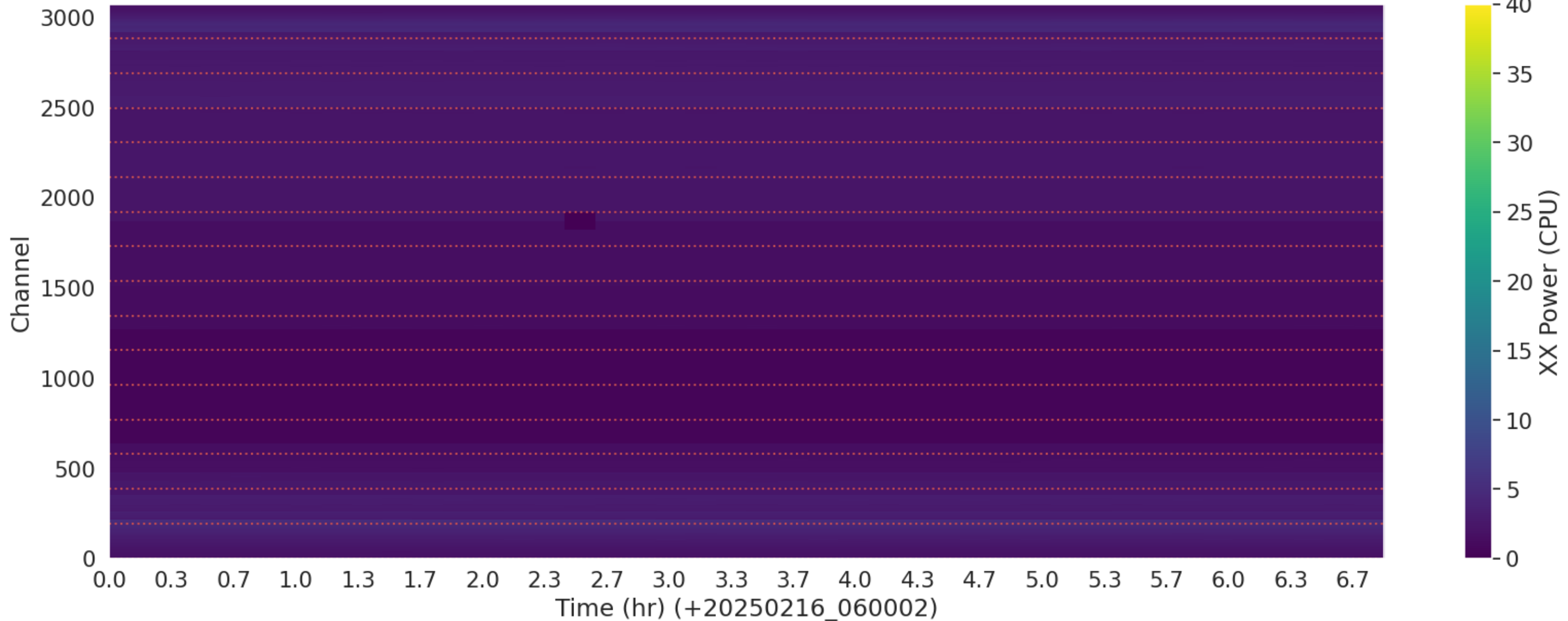
LWA298 - Correlator# 049 - XX - FLAGS: LowPower
