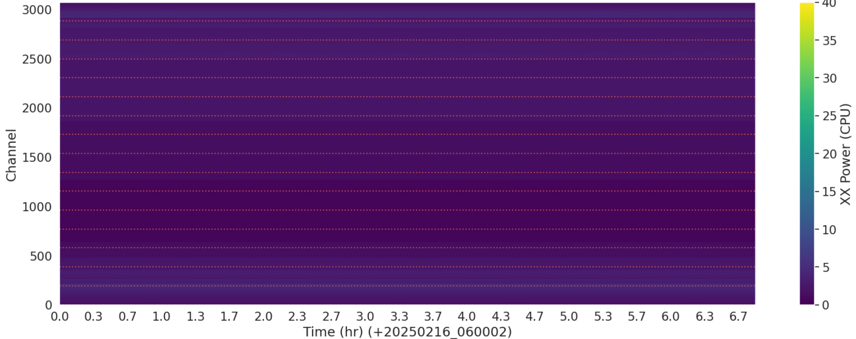
LWA334 - Correlator# 156 - XX - FLAGS: LowPower
