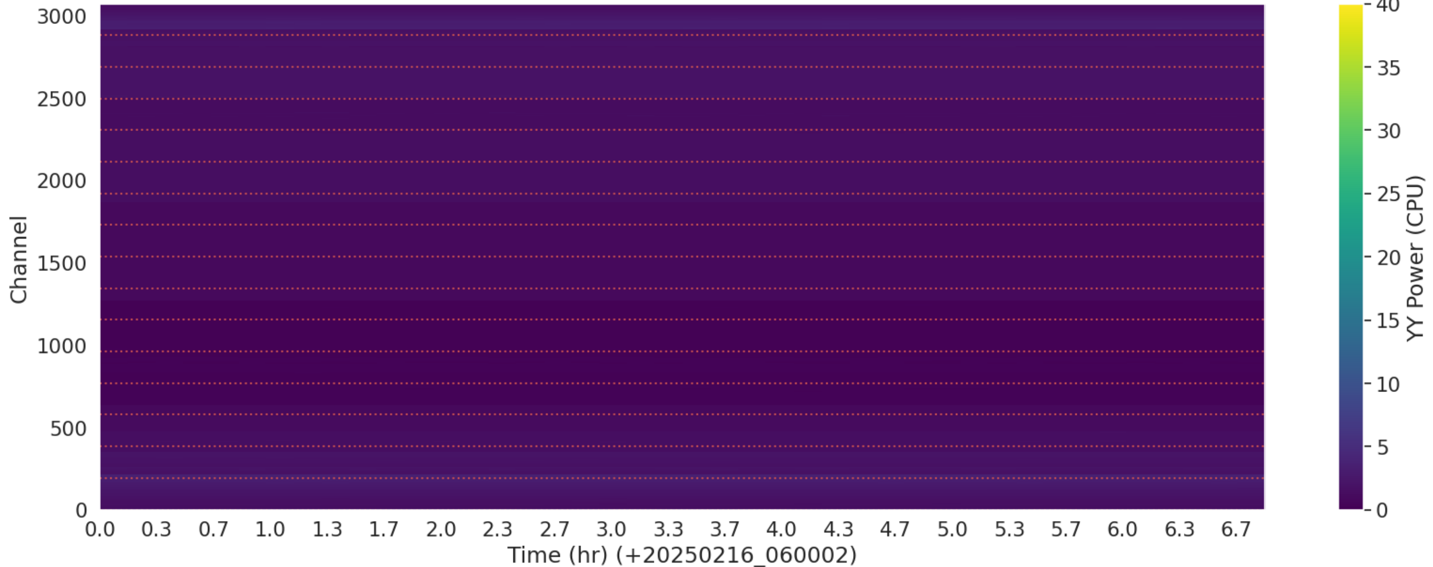
LWA314 - Correlator# 021 - YY - FLAGS: LowPower
