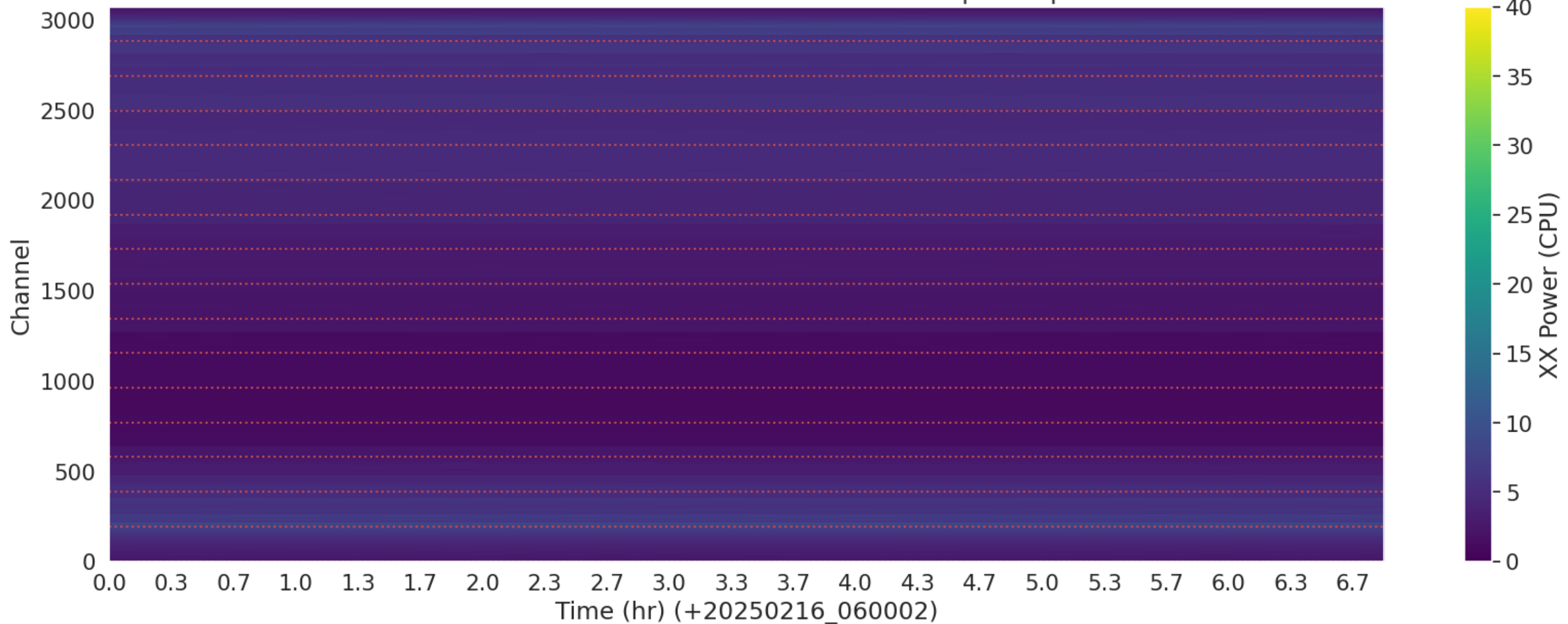
LWA264 - Correlator# 349 - XX - FLAGS: BadSpecShape
