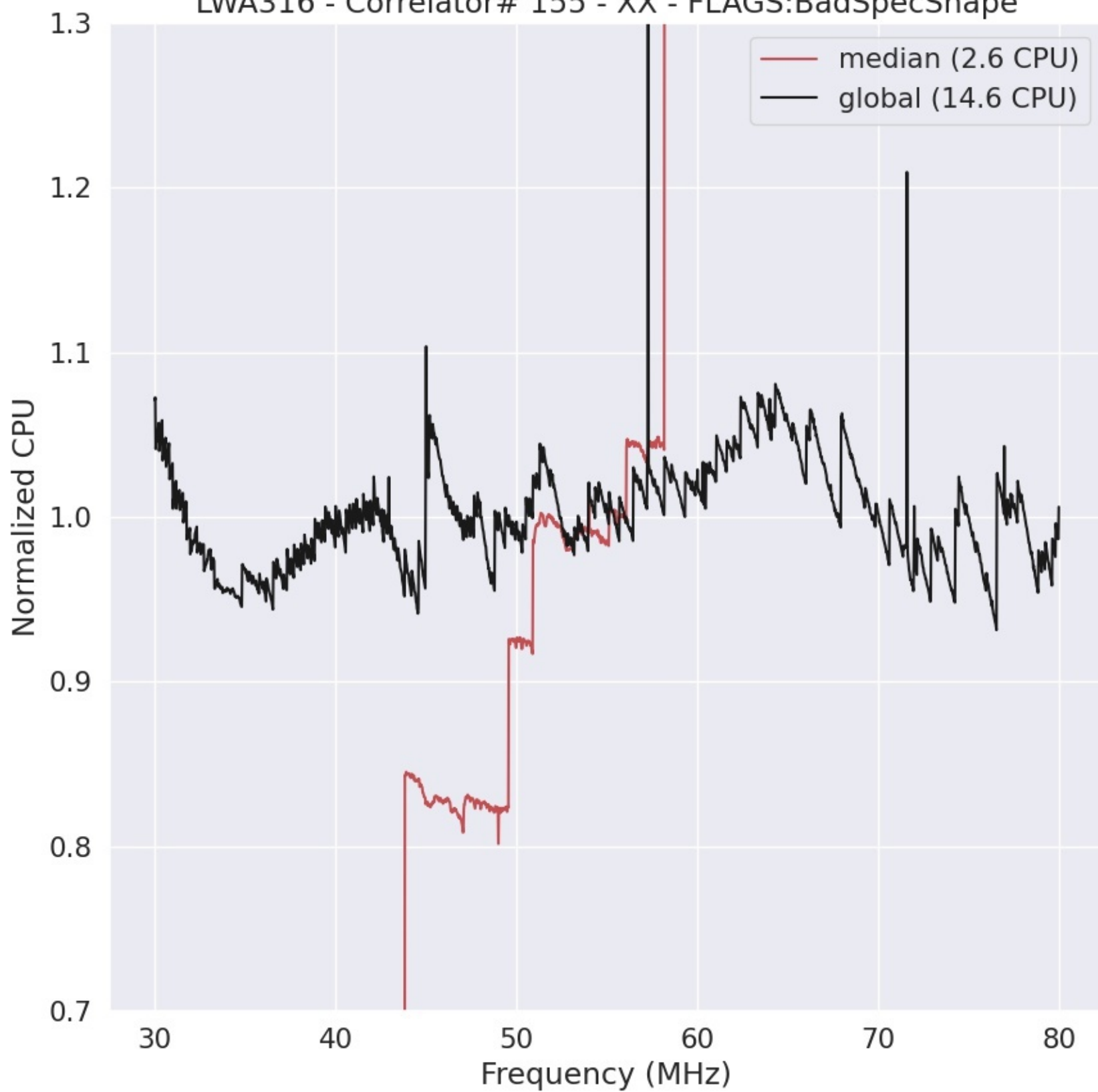
LWA316 - Correlator# 155 - XX - FLAGS:BadSpecShape
