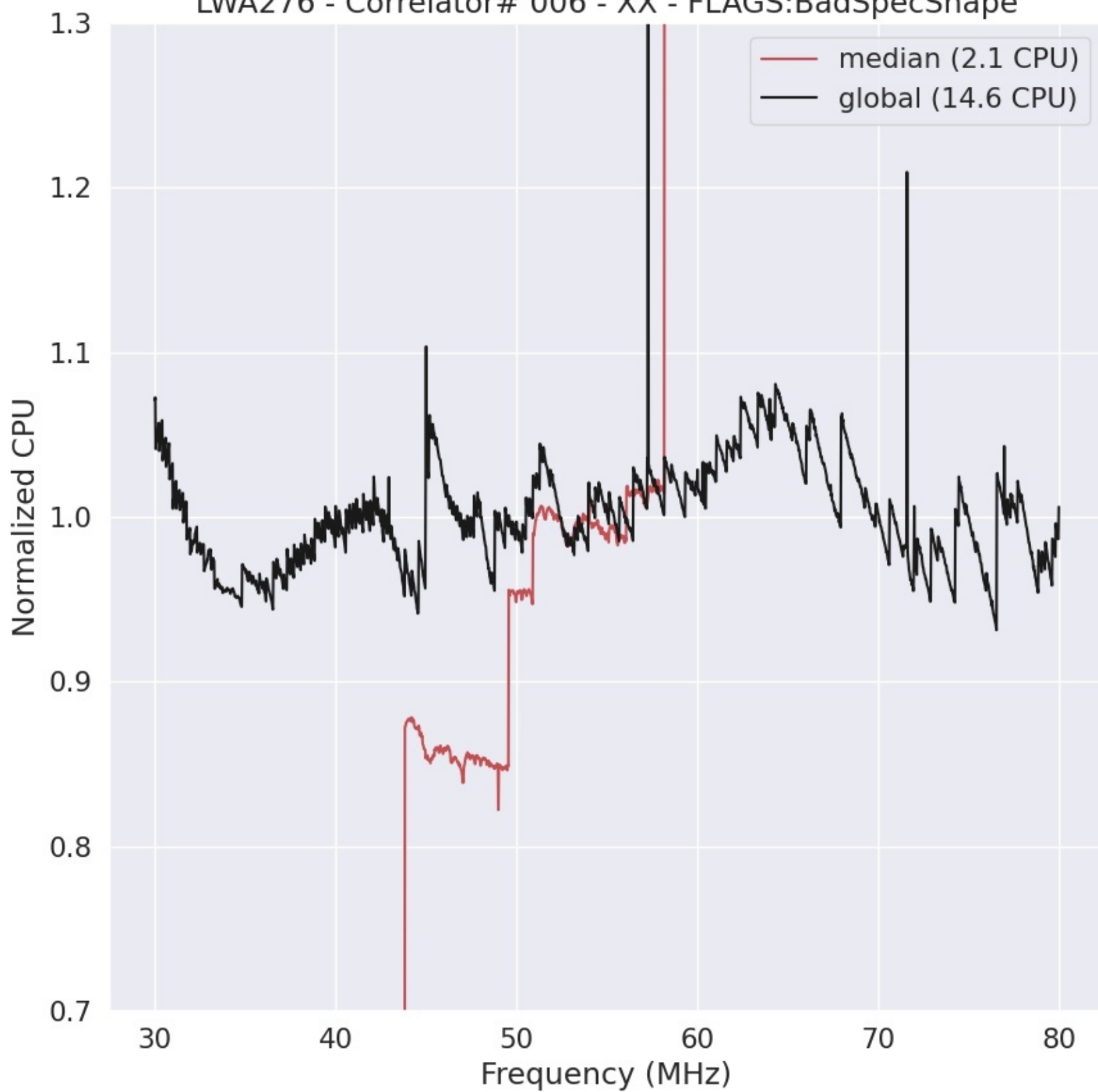
LWA276 - Correlator# 006 - XX - FLAGS:BadSpecShape
