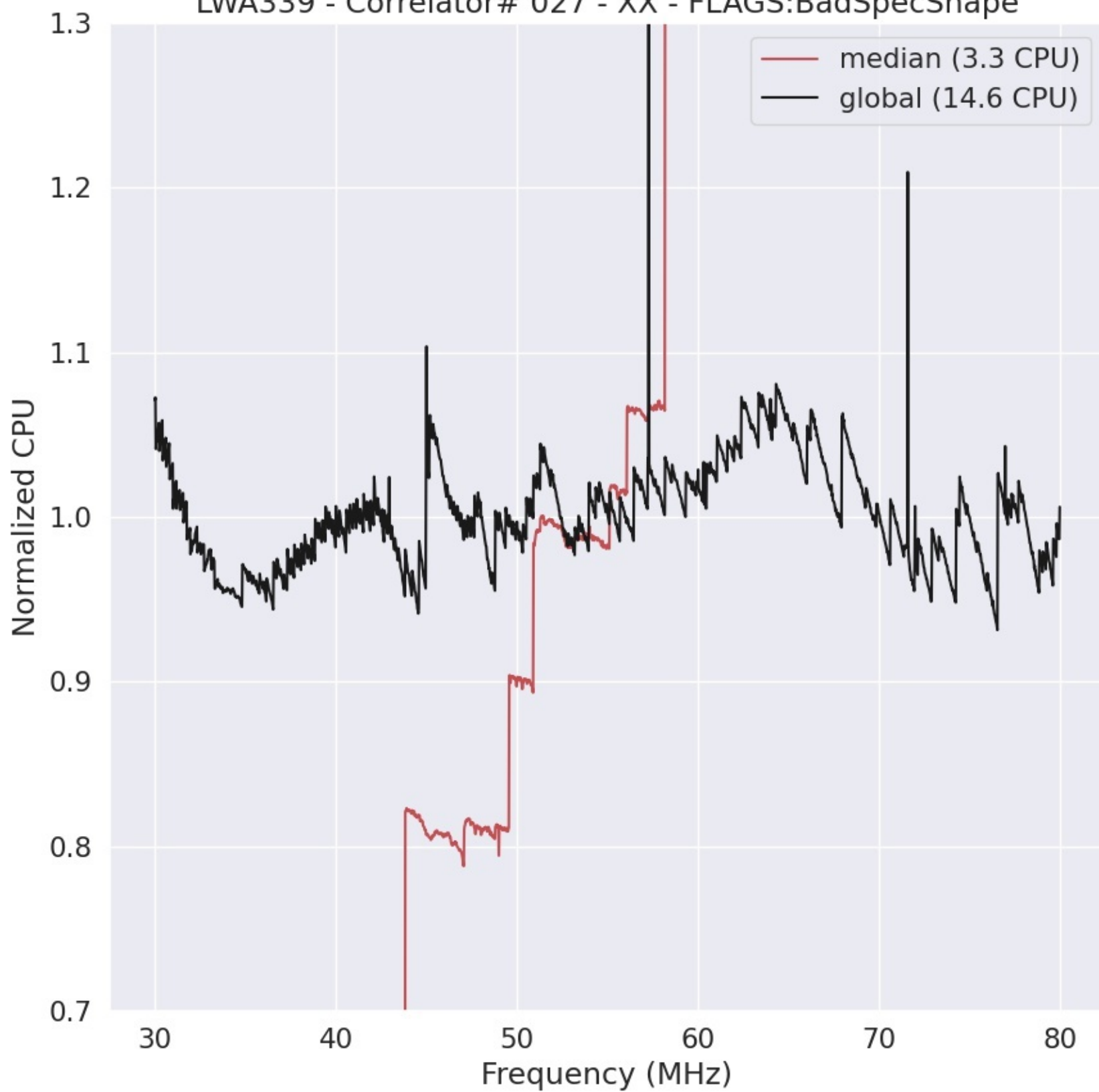
LWA339 - Correlator# 027 - XX - FLAGS:BadSpecShape
