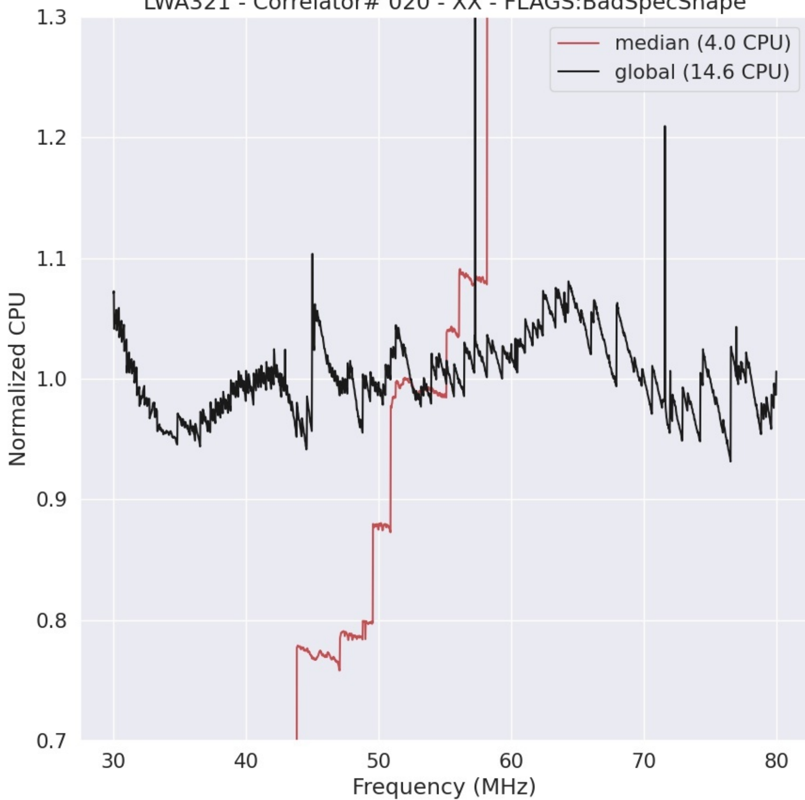
LWA321 - Correlator# 020 - XX - FLAGS:BadSpecShape
