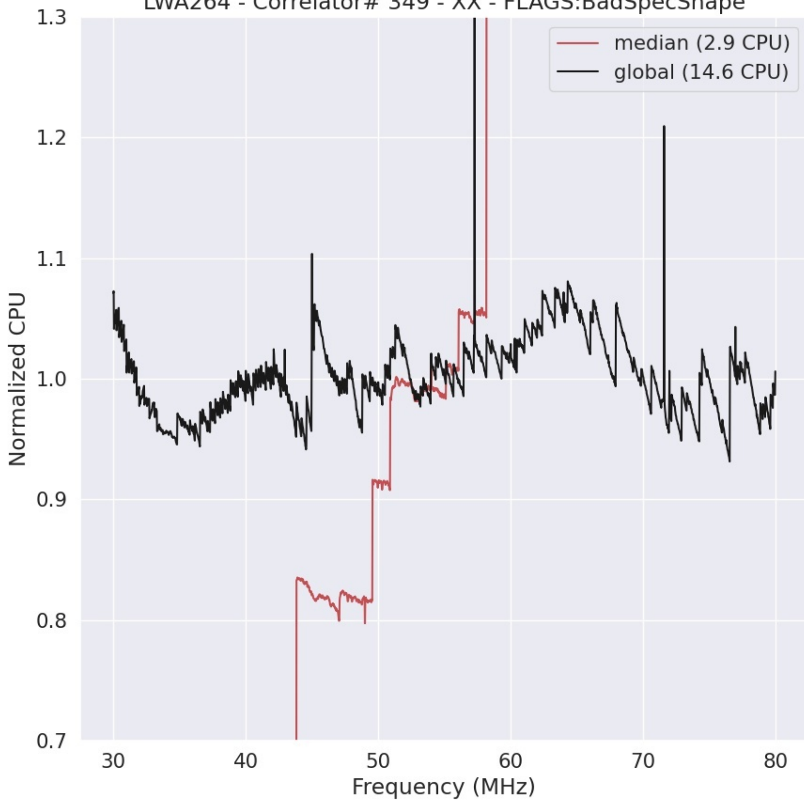
LWA264 - Correlator# 349 - XX - FLAGS:BadSpecShape
