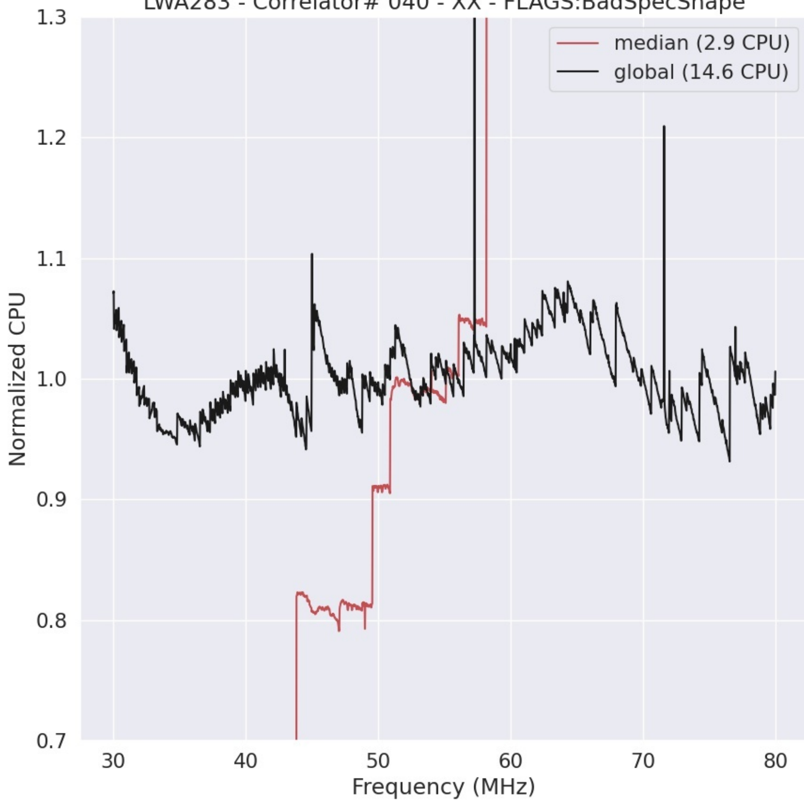
LWA283 - Correlator# 040 - XX - FLAGS:BadSpecShape
