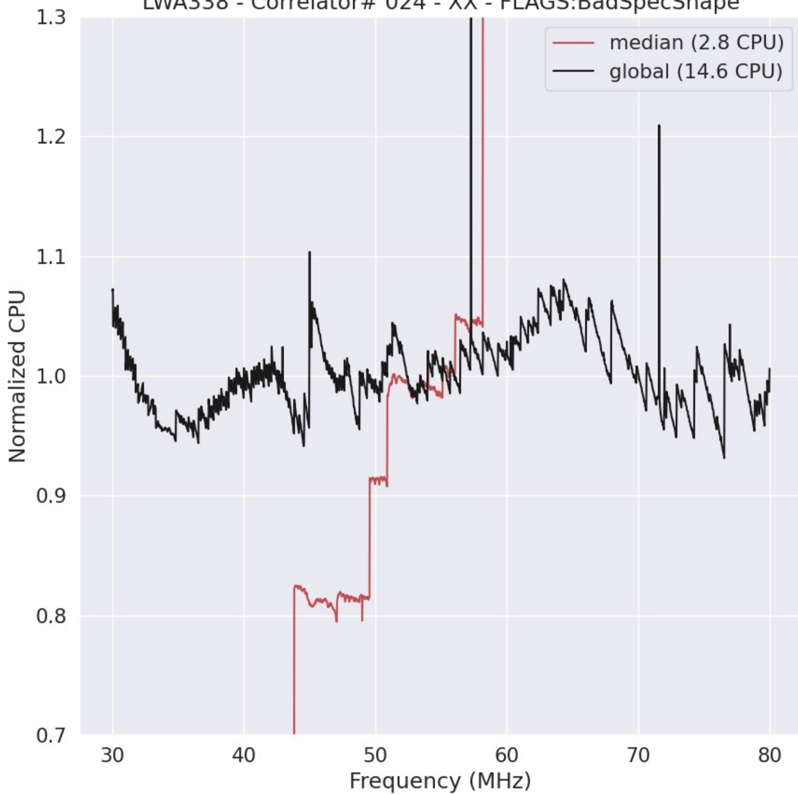
LWA338 - Correlator# 024 - XX - FLAGS:BadSpecShape
