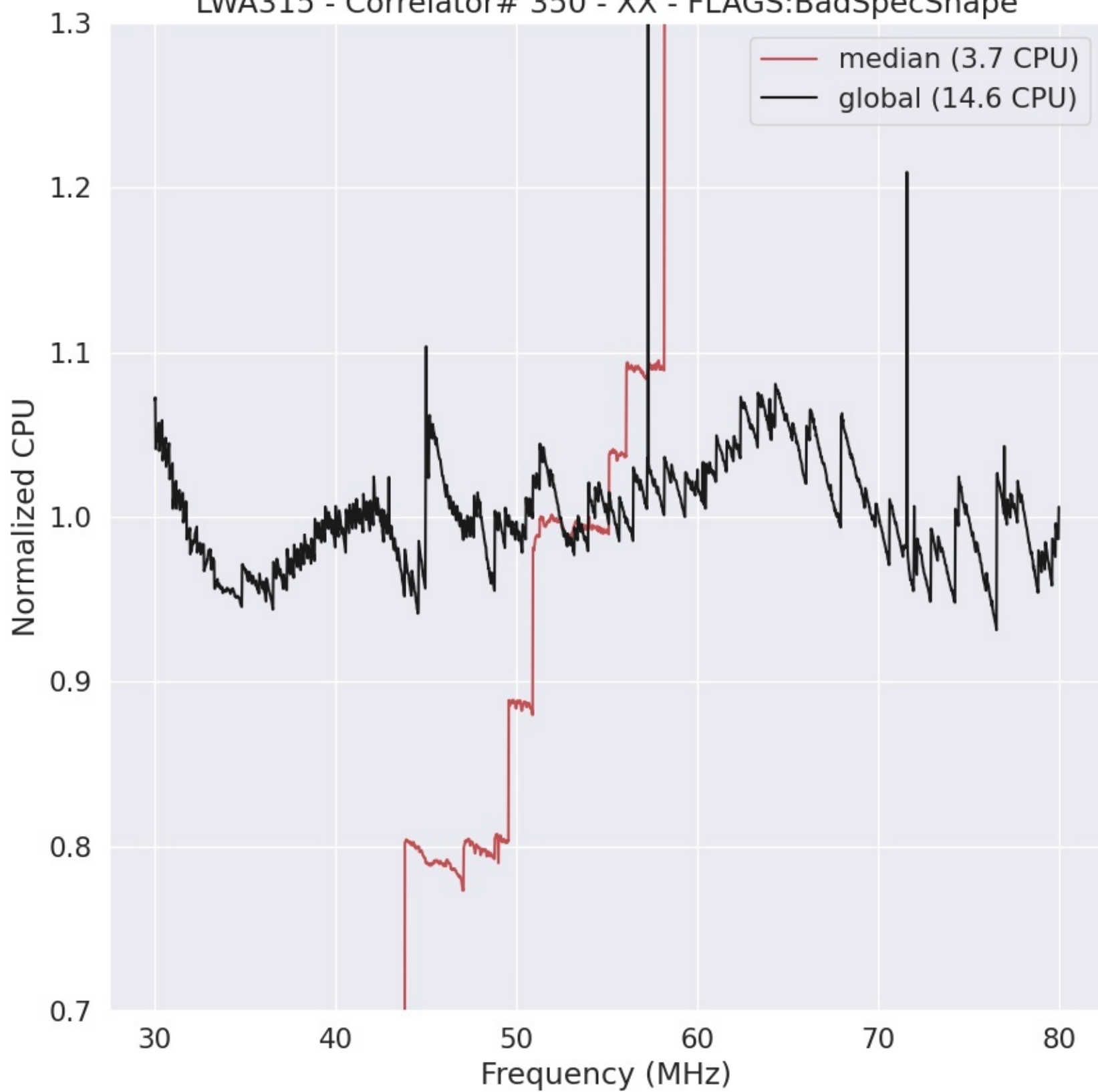
LWA315 - Correlator# 350 - XX - FLAGS:BadSpecShape
