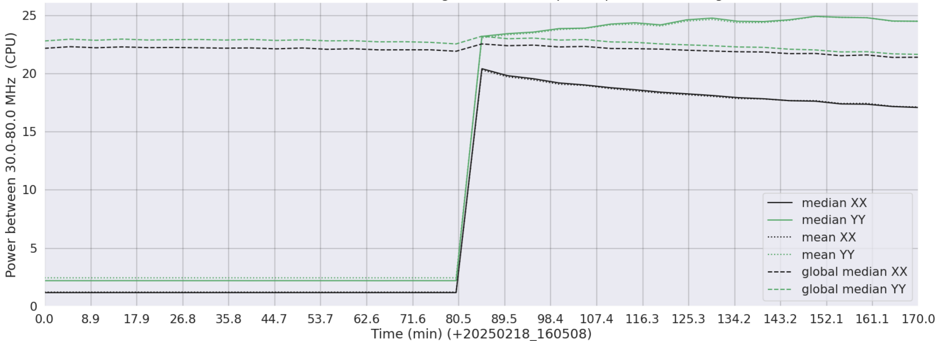
LWA271 - Correlator# 004 - XX FLAGS:HighTimeVar+BadSpecShape - YY FLAGS:HighTimeVar
