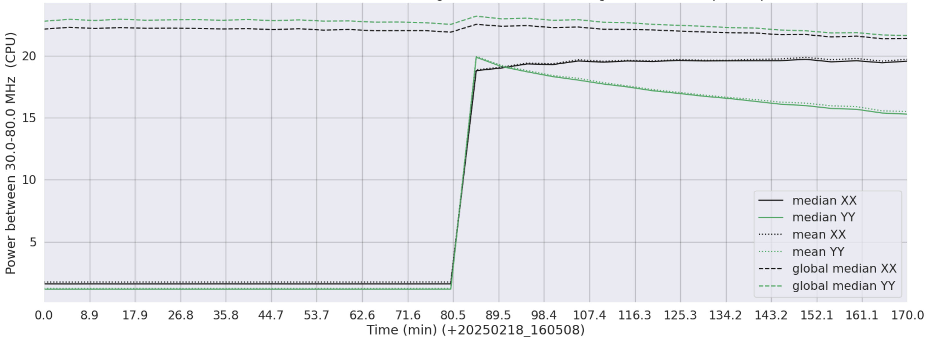
LWA310 - Correlator# 017 - XX FLAGS:HighTimeVar - YY FLAGS:HighTimeVar+BadSpecShape
