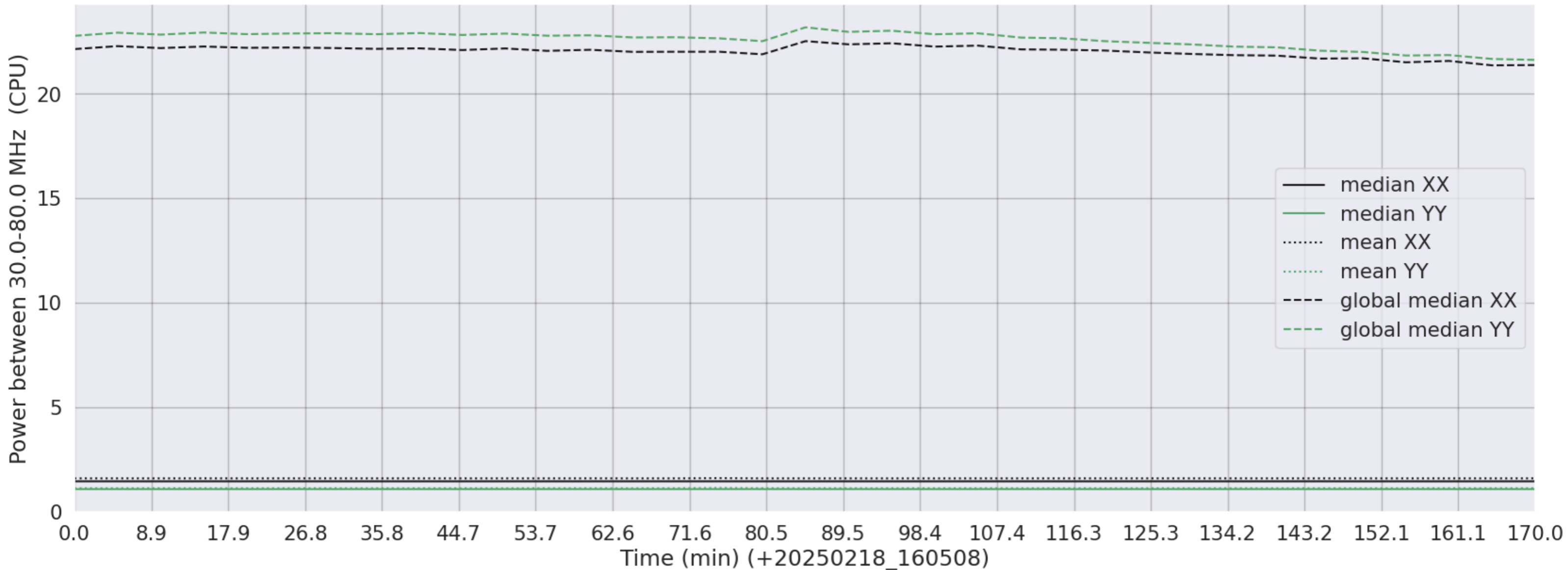
LWA324 - Correlator# 122 - XX FLAGS:LowPower - YY FLAGS:LowPower
