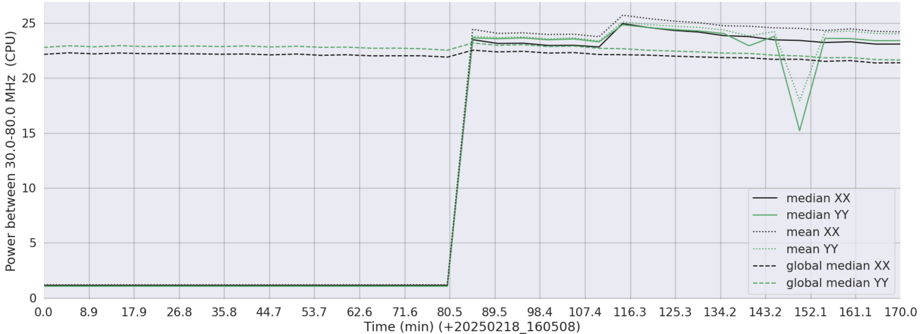
LWA341 - Correlator# 029 - XX FLAGS:HighTimeVar - YY FLAGS:HighTimeVar+BadSpecShape
