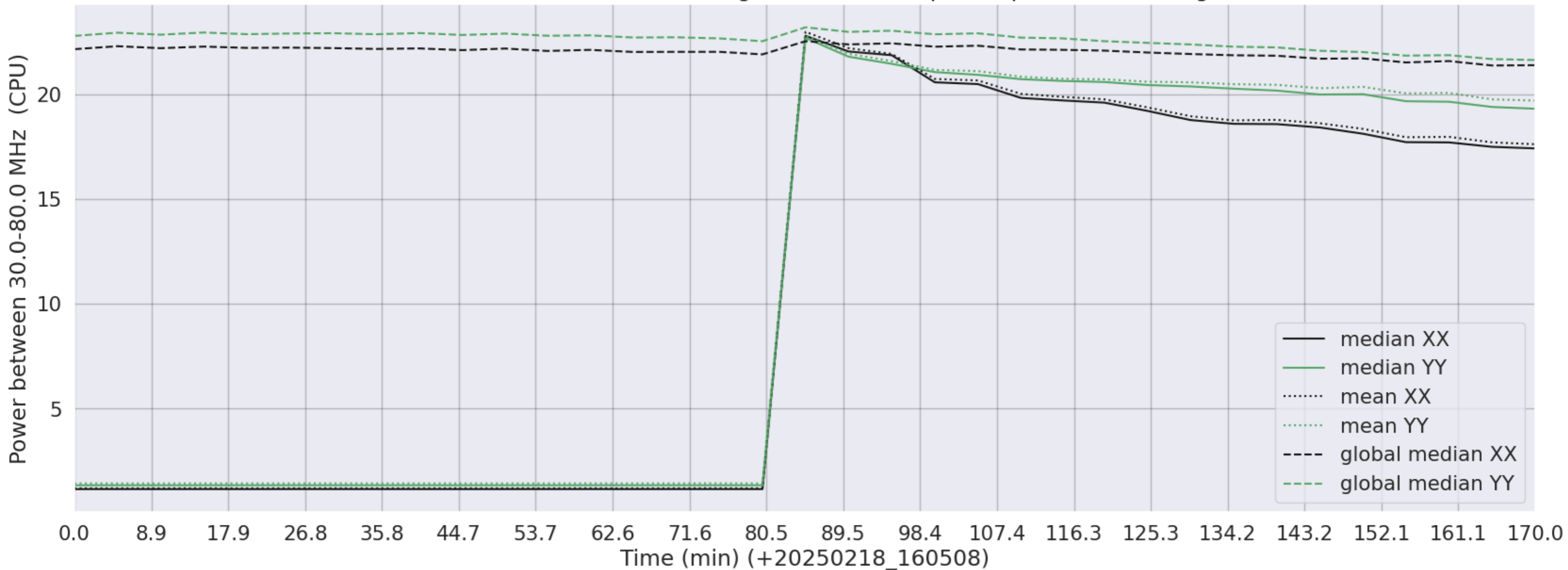
LWA272 - Correlator# 038 - XX FLAGS:HighTimeVar+BadSpecShape - YY FLAGS:HighTimeVar
