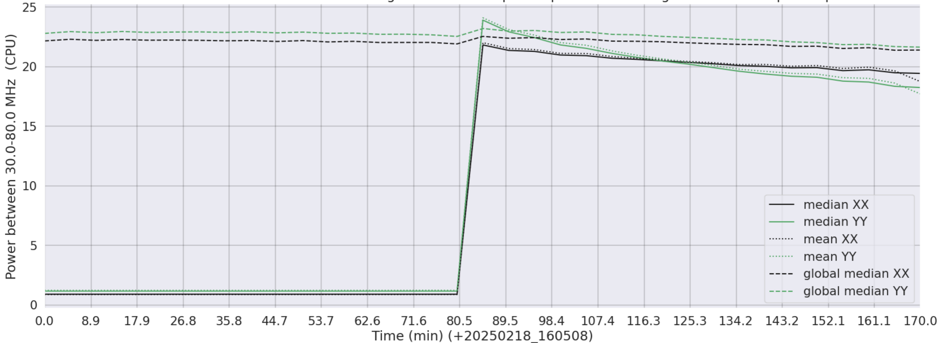
LWA325 - Correlator# 154 - XX FLAGS:HighTimeVar+BadSpecShape - YY FLAGS:HighTimeVar+BadSpecShape
