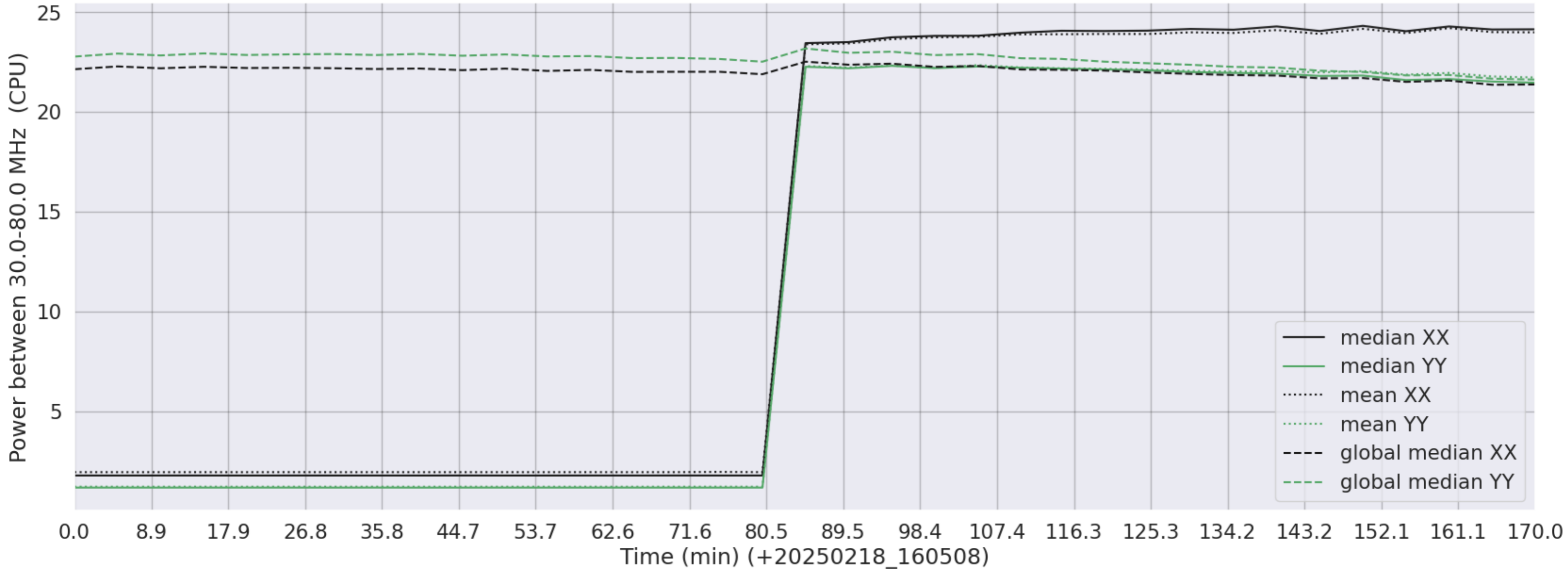
LWA351 - Correlator# 060 - XX FLAGS:HighTimeVar - YY FLAGS:HighTimeVar
