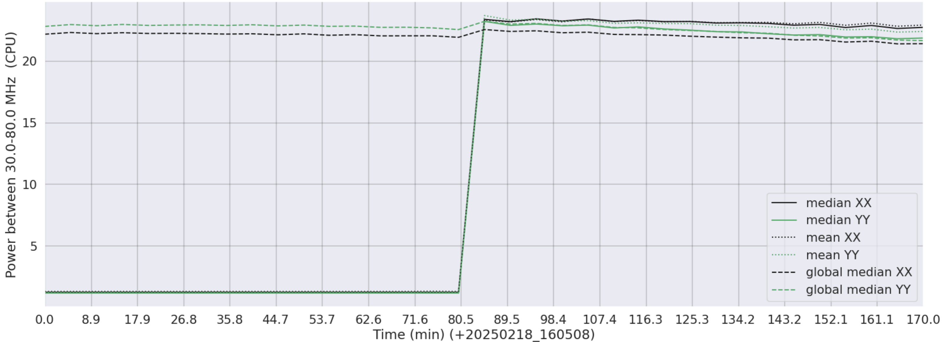
LWA336 - Correlator# 056 - XX FLAGS:HighTimeVar - YY FLAGS:HighTimeVar
