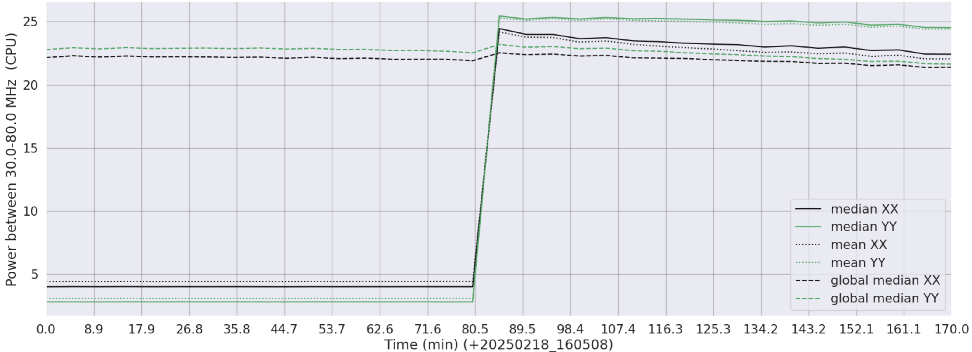
LWA321 - Correlator# 020 - XX FLAGS:HighTimeVar - YY FLAGS:HighTimeVar
