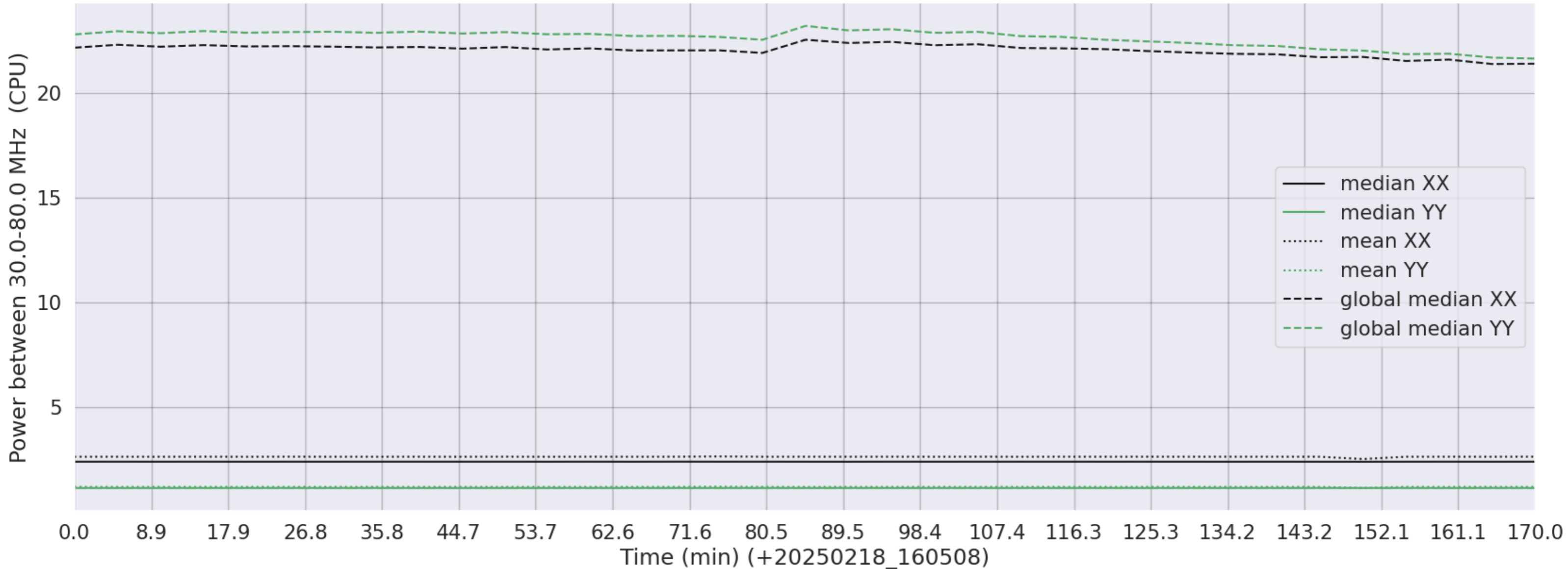
LWA288 - Correlator# 042 - XX FLAGS:BadSpecShape - YY FLAGS:LowPower
