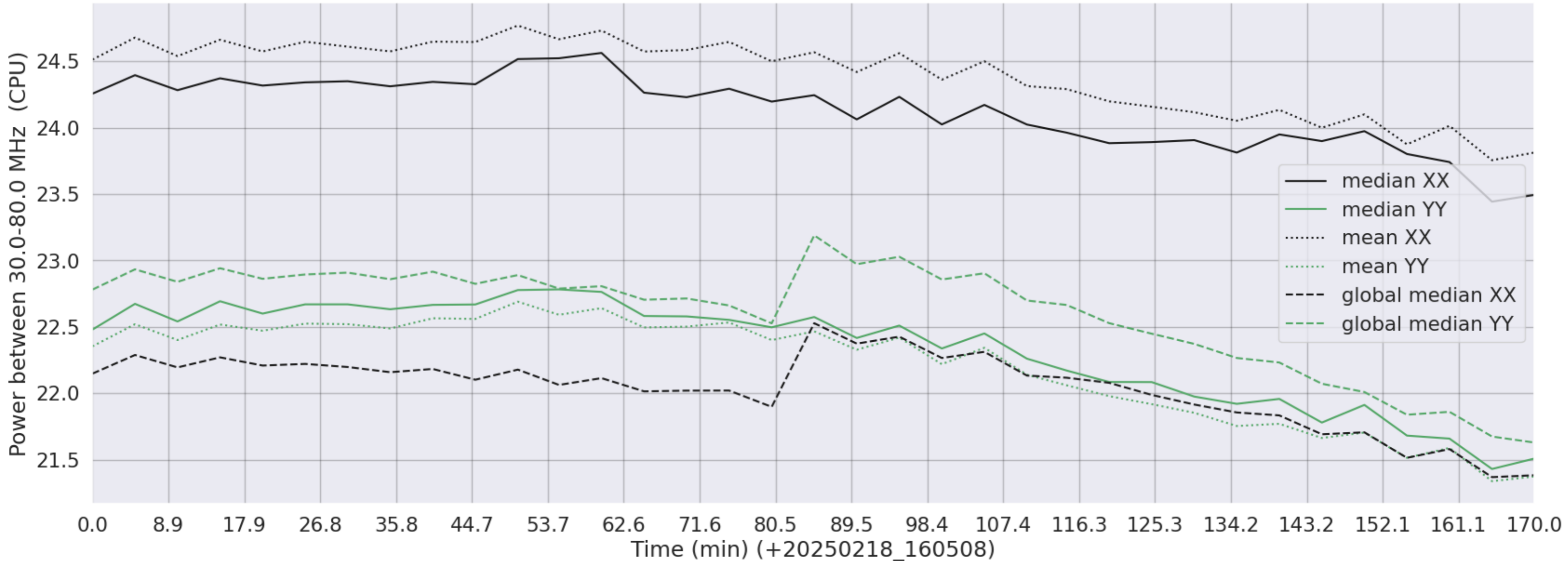
LWA194 - Correlator# 273 - XX FLAGS:Good - YY FLAGS:BadSpecShape
