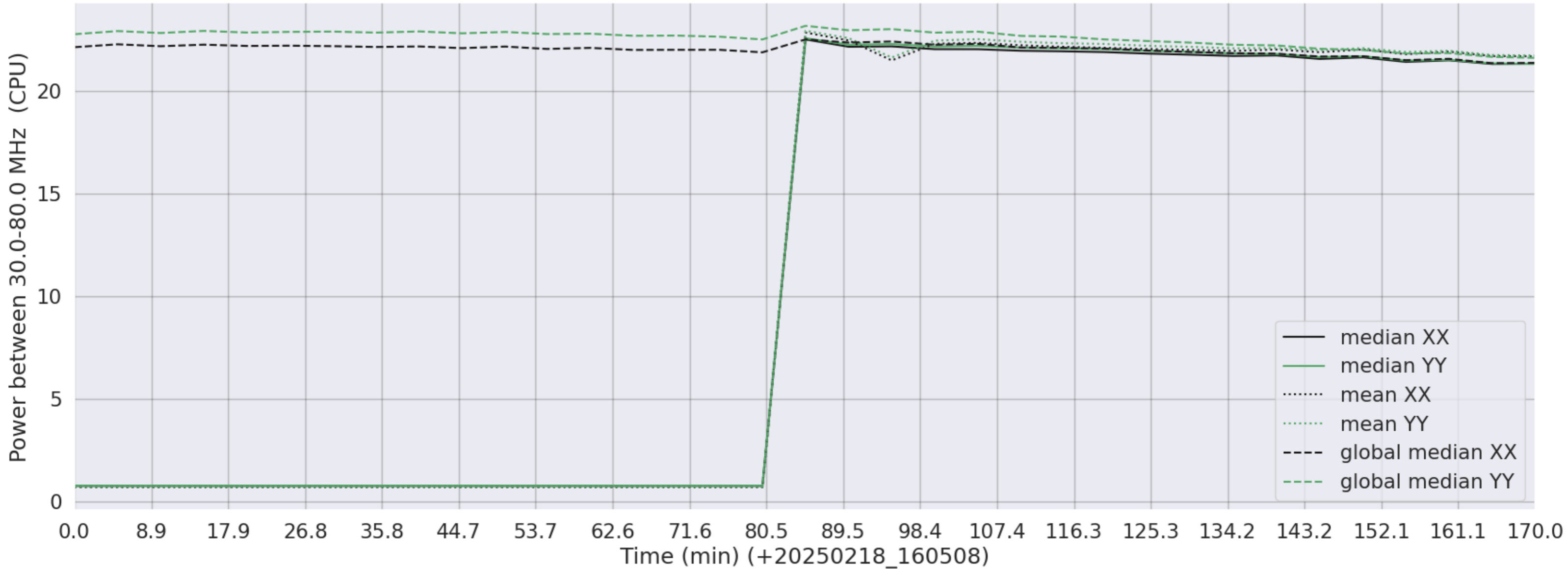
LWA260 - Correlator# 034 - XX FLAGS:HighTimeVar+BadSpecShape - YY FLAGS:HighTimeVar+BadSpecShape
