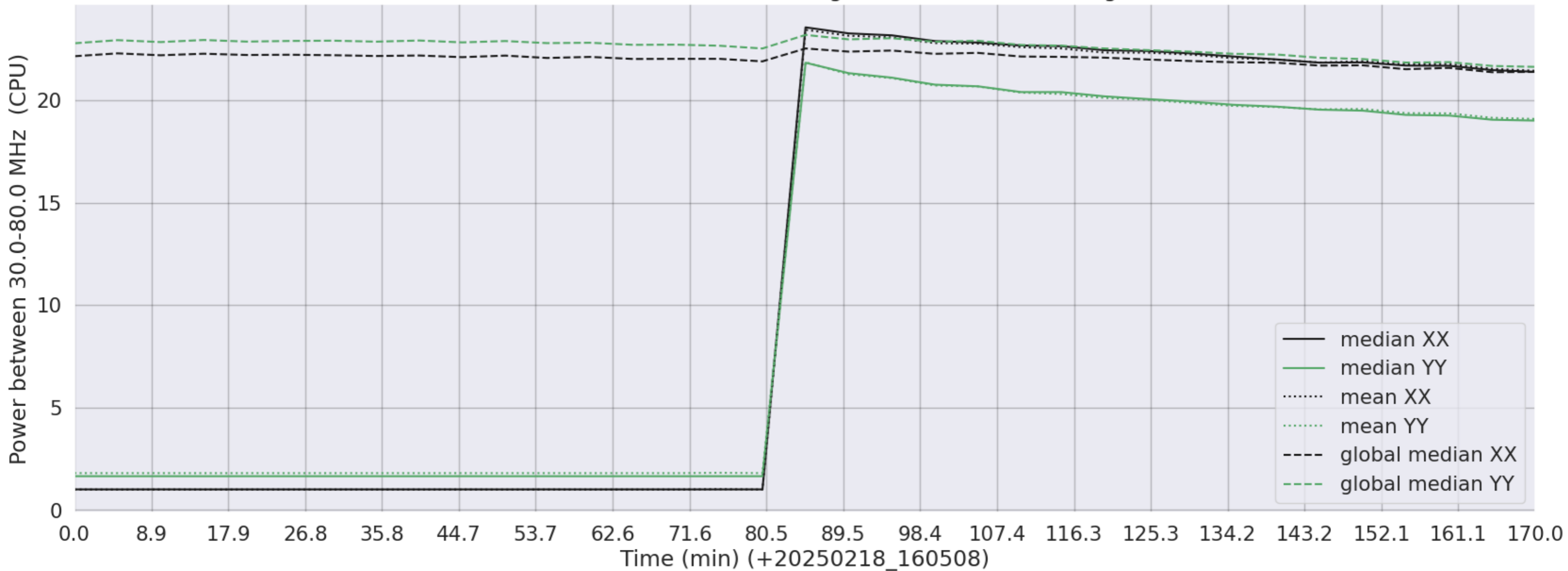
LWA289 - Correlator# 189 - XX FLAGS:HighTimeVar - YY FLAGS:HighTimeVar
