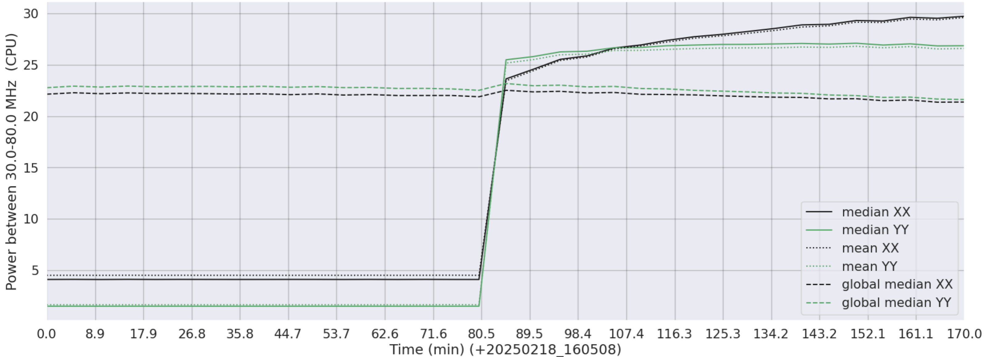
LWA313 - Correlator# 018 - XX FLAGS:HighTimeVar - YY FLAGS:HighTimeVar
