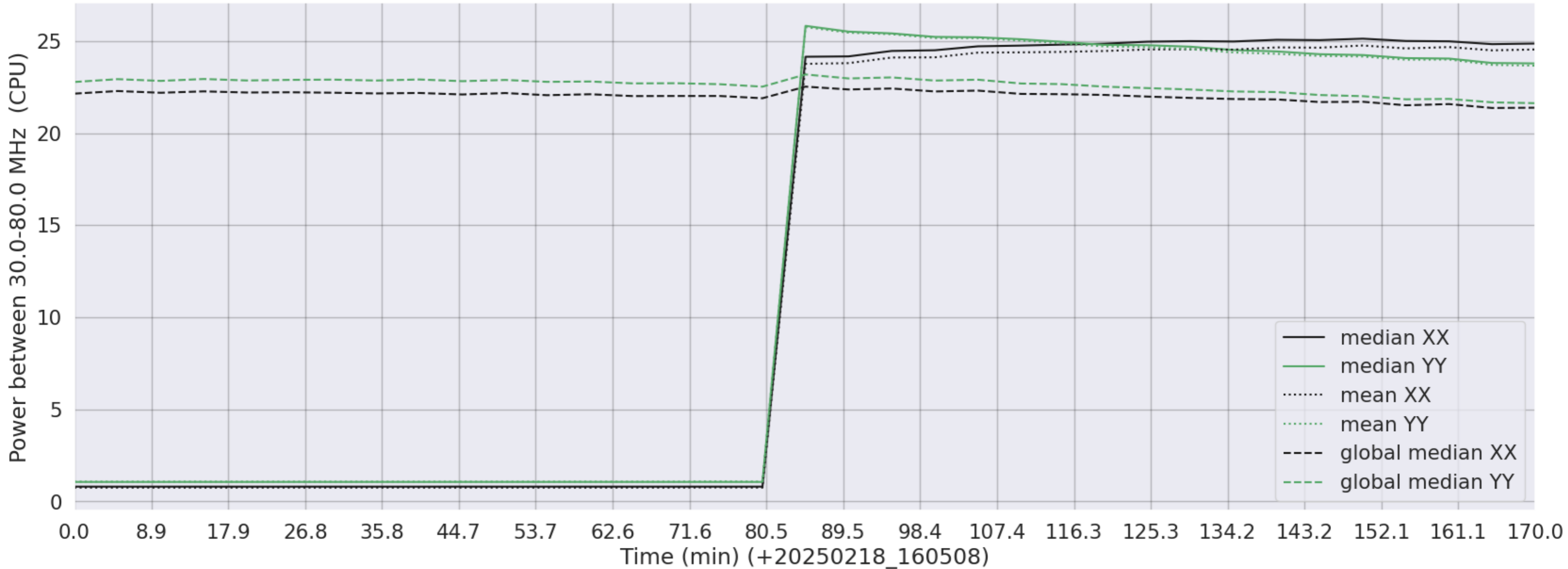
LWA314 - Correlator# 021 - XX FLAGS:HighTimeVar - YY FLAGS:HighTimeVar
