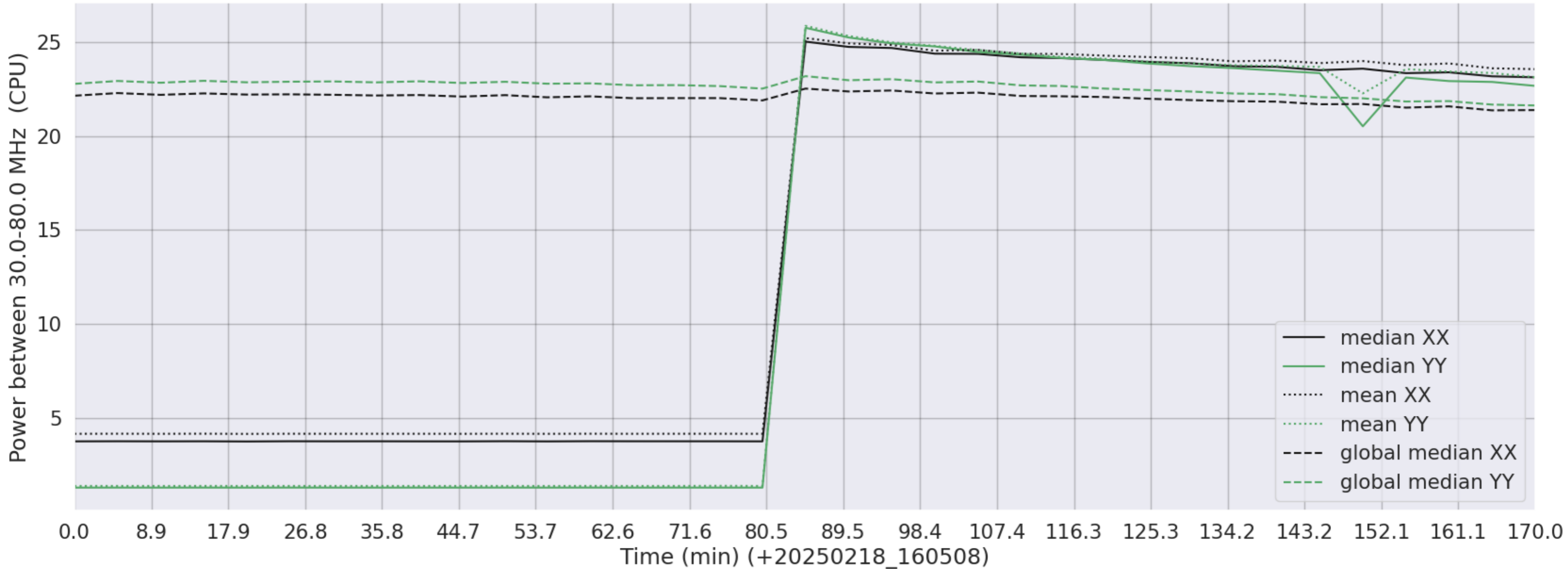
LWA315 - Correlator# 350 - XX FLAGS:HighTimeVar - YY FLAGS:HighTimeVar+BadSpecShape
