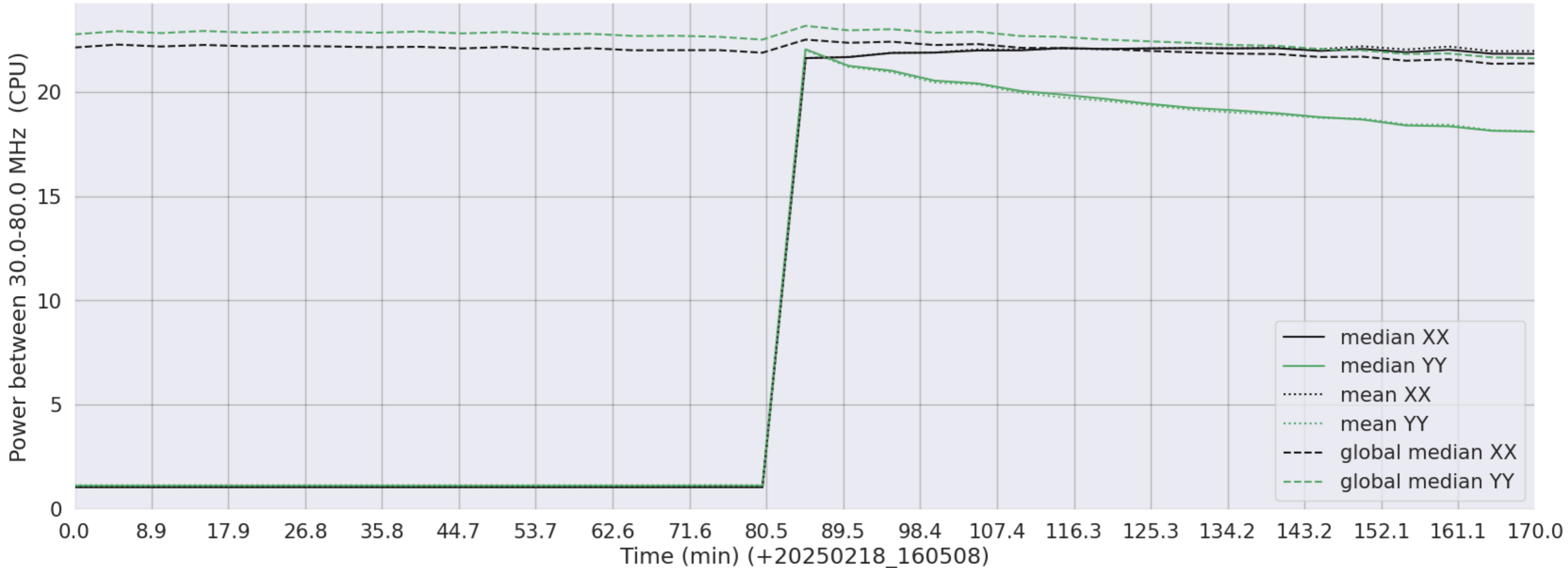
LWA296 - Correlator# 046 - XX FLAGS:HighTimeVar - YY FLAGS:HighTimeVar
