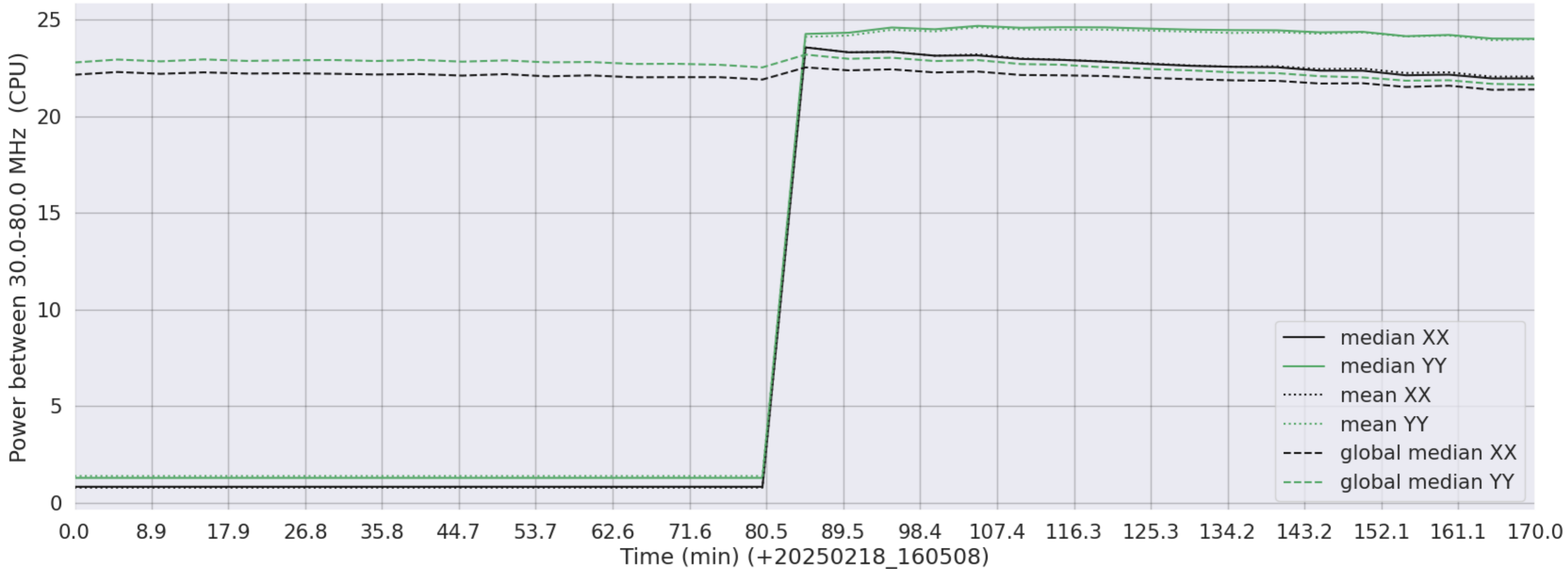
LWA267 - Correlator# 003 - XX FLAGS:HighTimeVar - YY FLAGS:HighTimeVar
