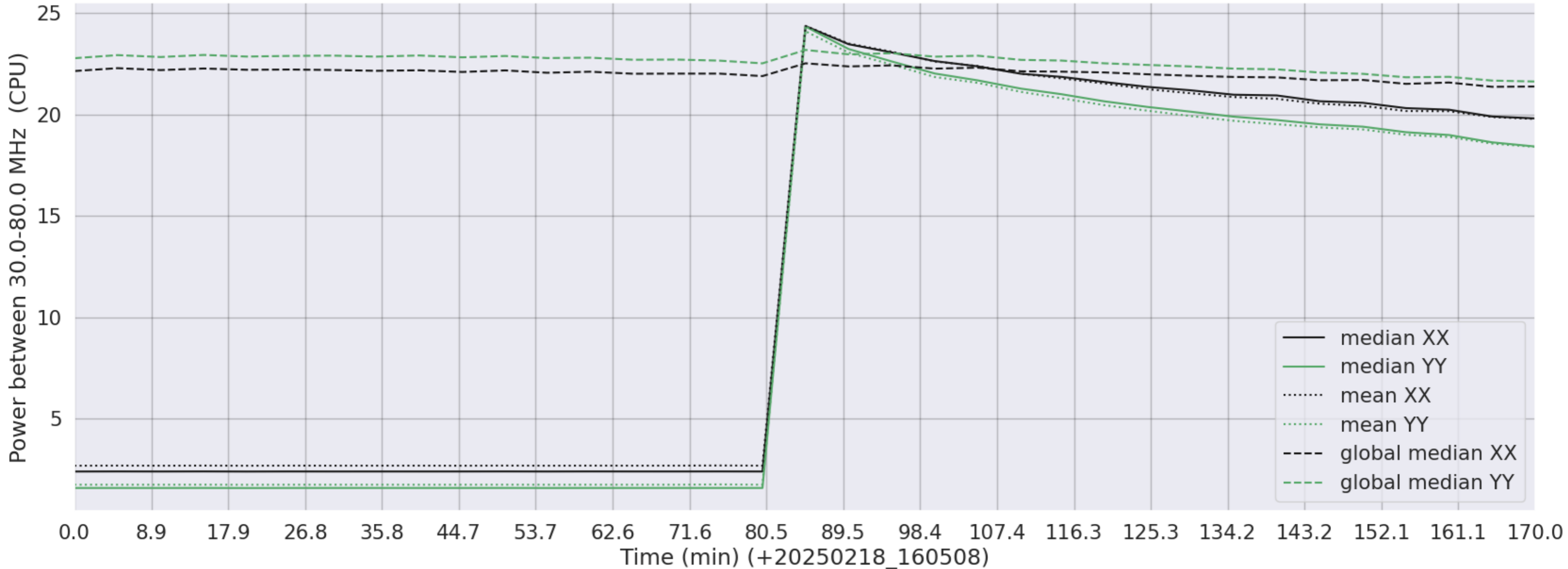
LWA333 - Correlator# 253 - XX FLAGS:HighTimeVar - YY FLAGS:HighTimeVar+BadSpecShape
