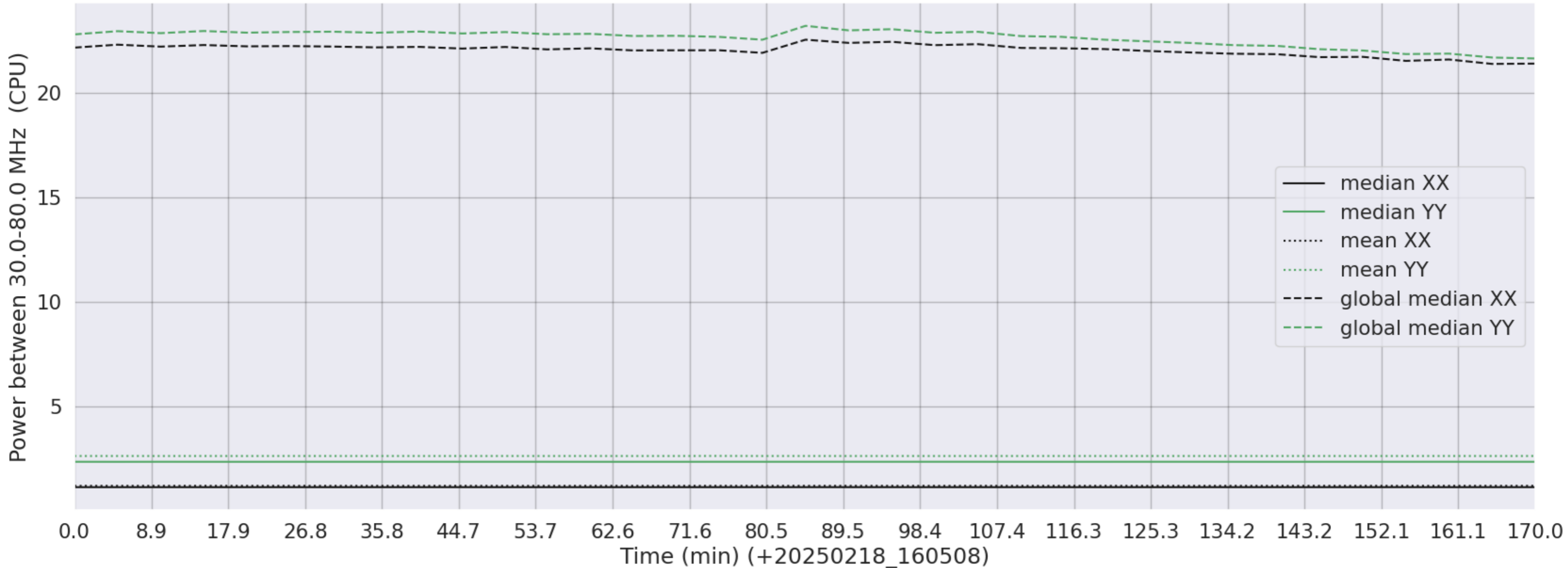
LWA323 - Correlator# 095 - XX FLAGS:LowPower - YY FLAGS:BadSpecShape
