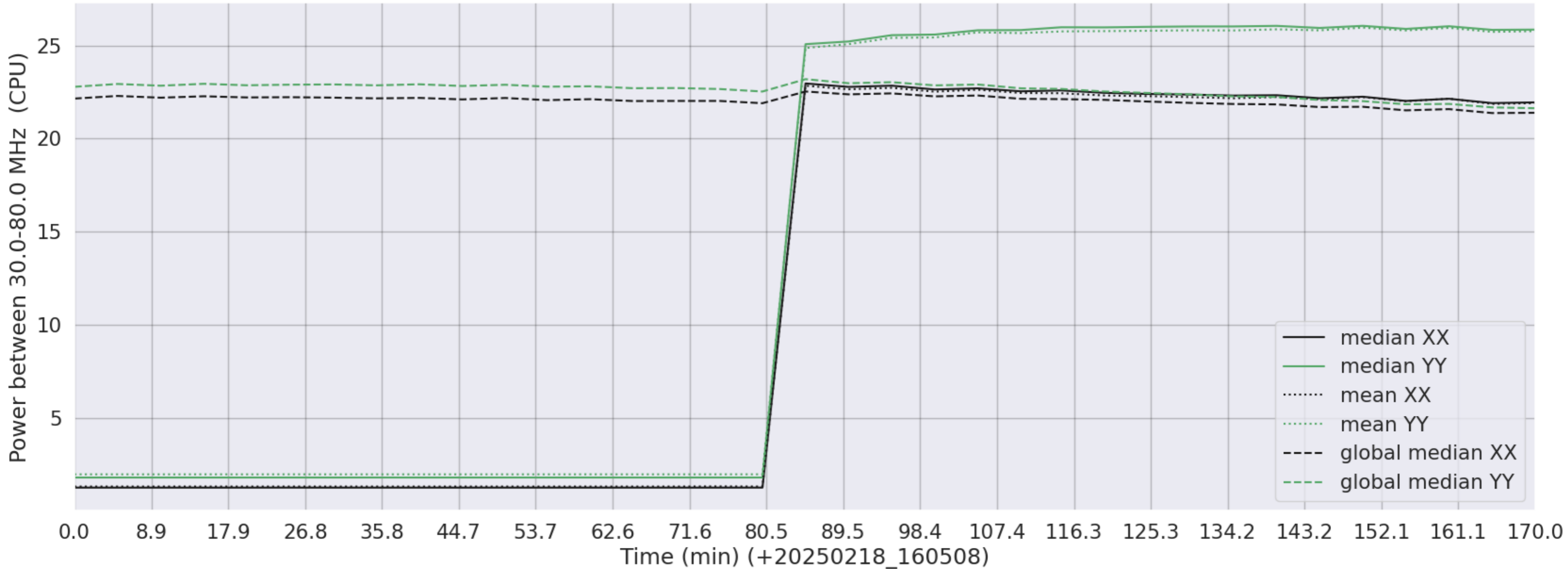
LWA343 - Correlator# 058 - XX FLAGS:HighTimeVar - YY FLAGS:HighTimeVar
