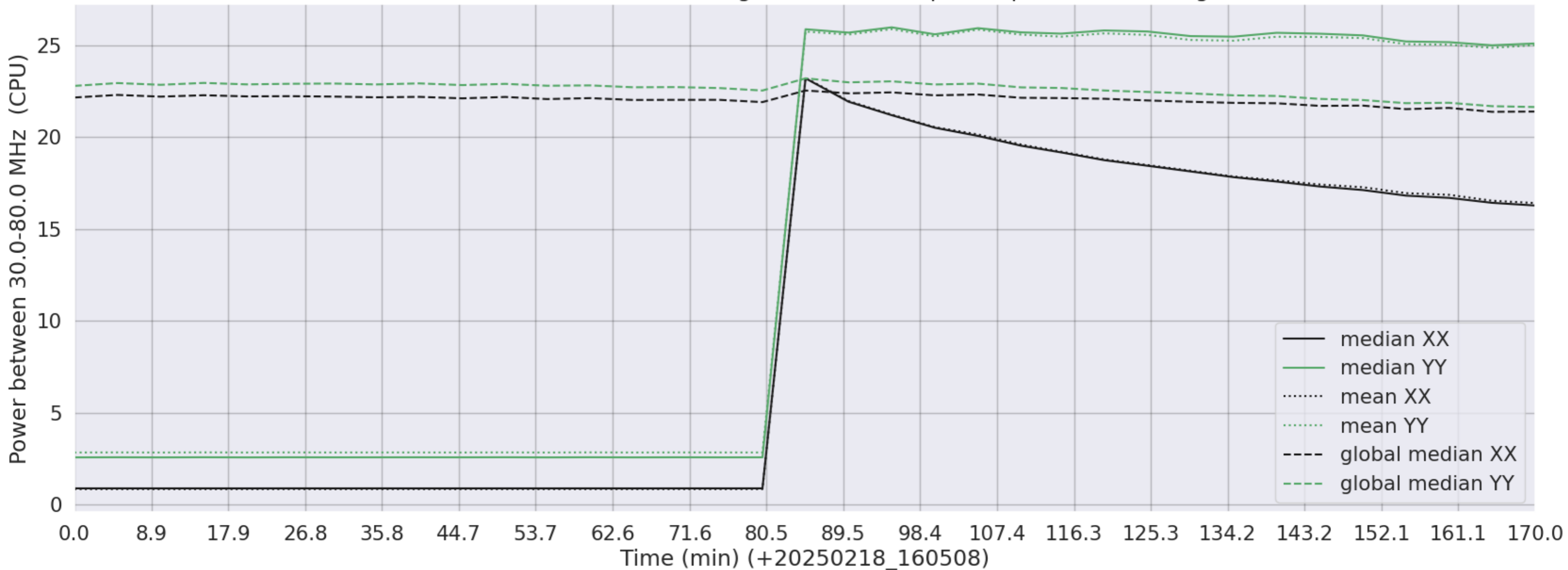
LWA308 - Correlator# 015 - XX FLAGS:HighTimeVar+BadSpecShape - YY FLAGS:HighTimeVar
