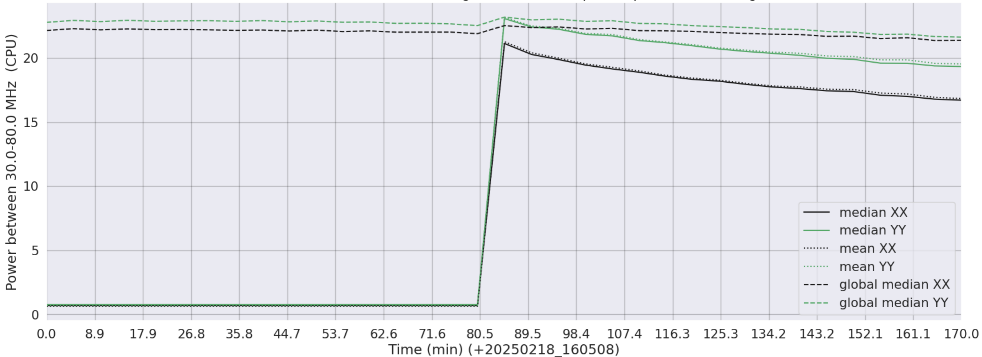
LWA281 - Correlator# 011 - XX FLAGS:HighTimeVar+BadSpecShape - YY FLAGS:HighTimeVar
