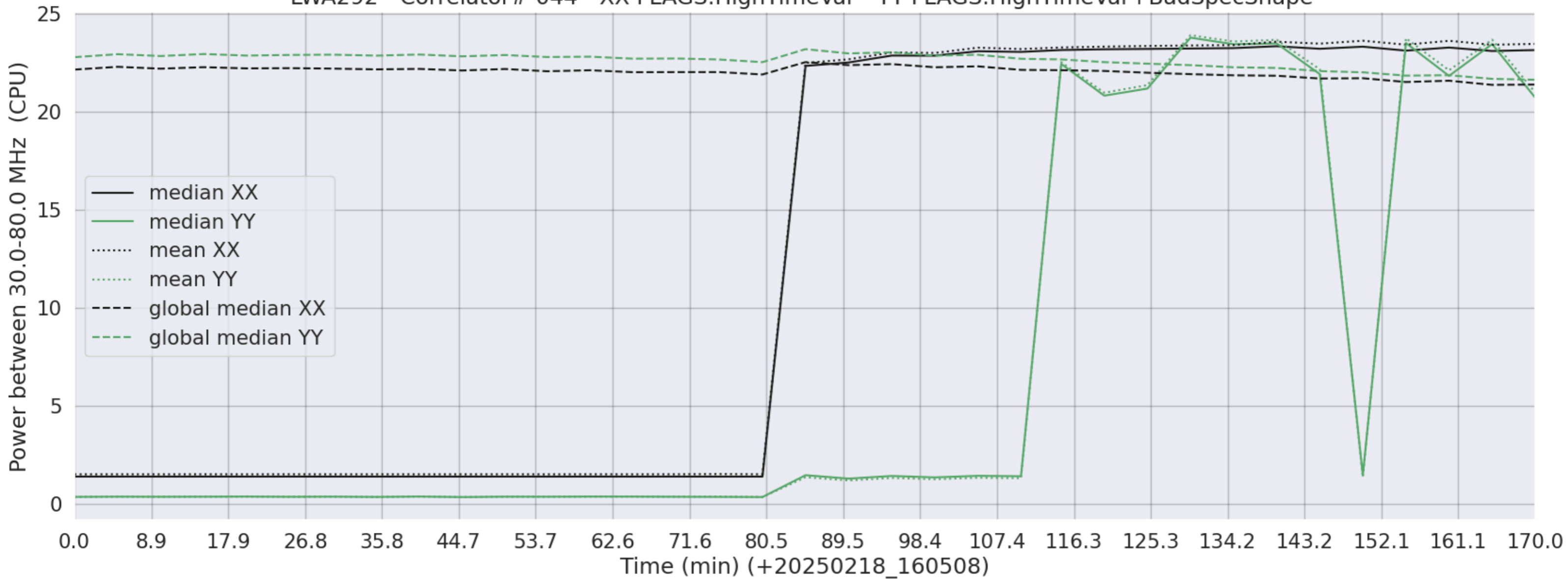
LWA292 - Correlator# 044 - XX FLAGS:HighTimeVar - YY FLAGS:HighTimeVar+BadSpecShape
