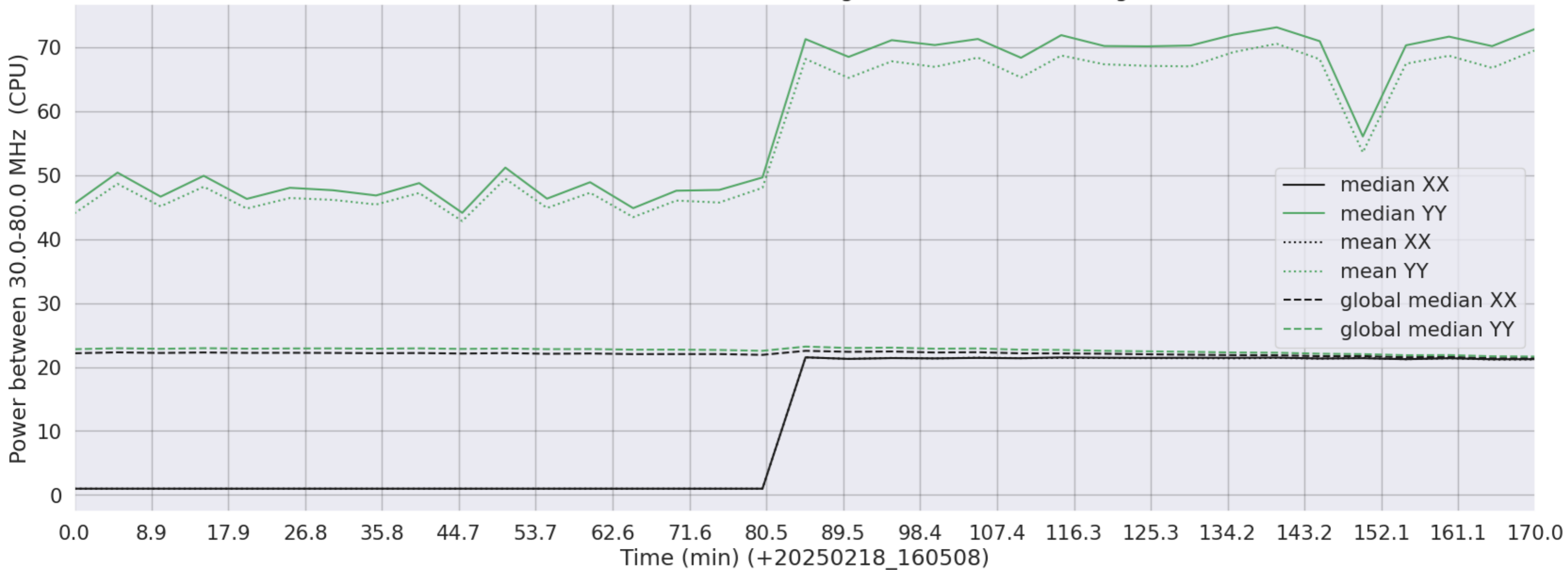
LWA280 - Correlator# 041 - XX FLAGS:HighTimeVar - YY FLAGS:HighPower
