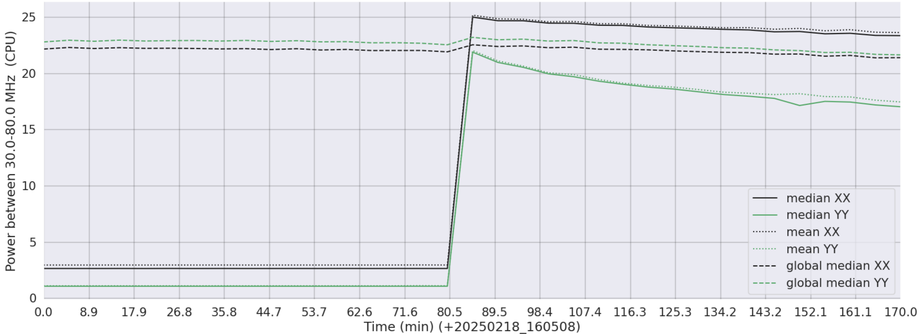
LWA316 - Correlator# 155 - XX FLAGS:HighTimeVar - YY FLAGS:HighTimeVar+BadSpecShape
