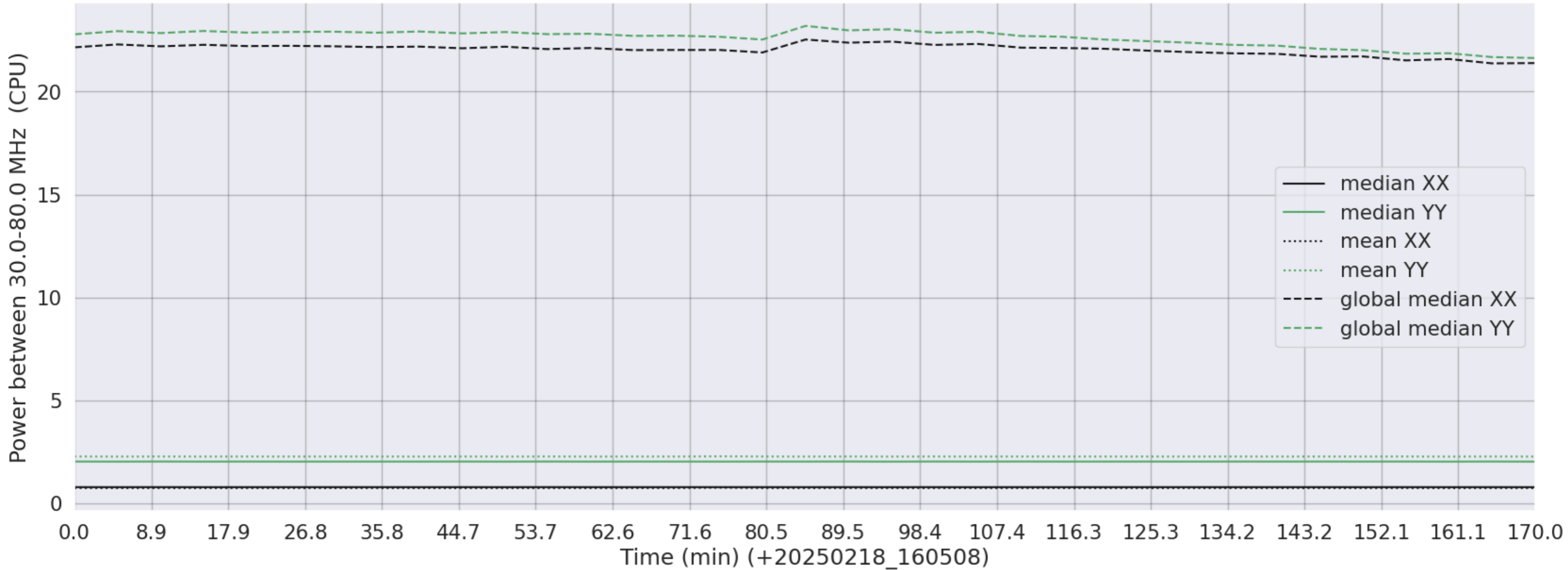
LWA348 - Correlator# 124 - XX FLAGS:LowPower - YY FLAGS:BadSpecShape
