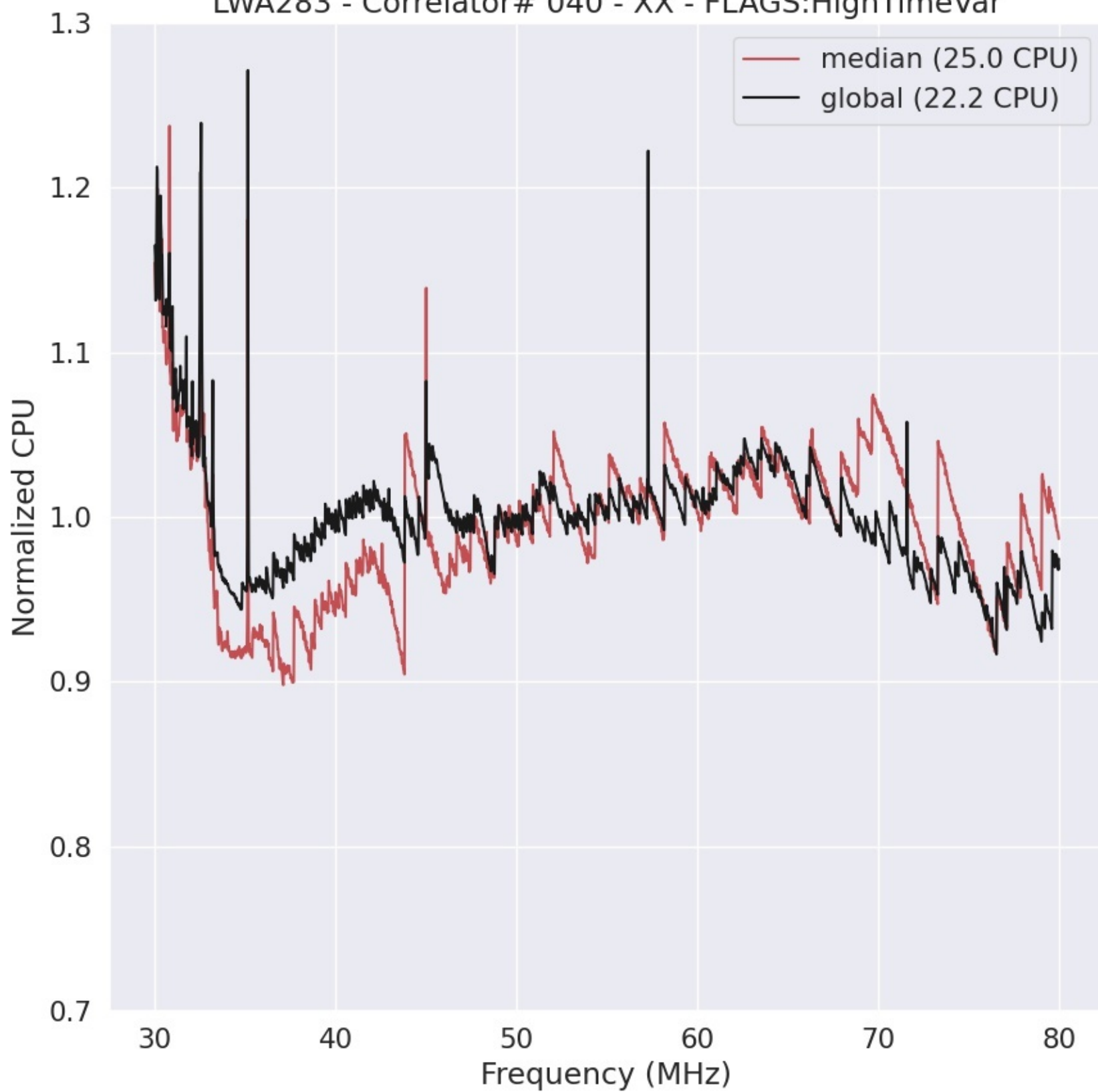
LWA283 - Correlator# 040 - XX - FLAGS:HighTimeVar
