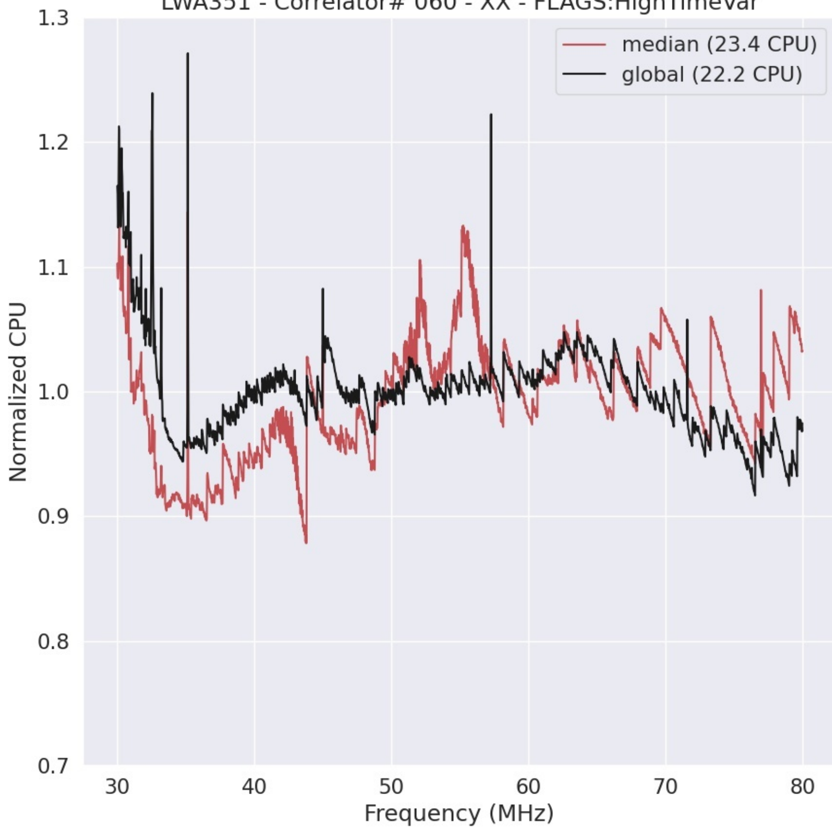
LWA351 - Correlator# 060 - XX - FLAGS:HighTimeVar
