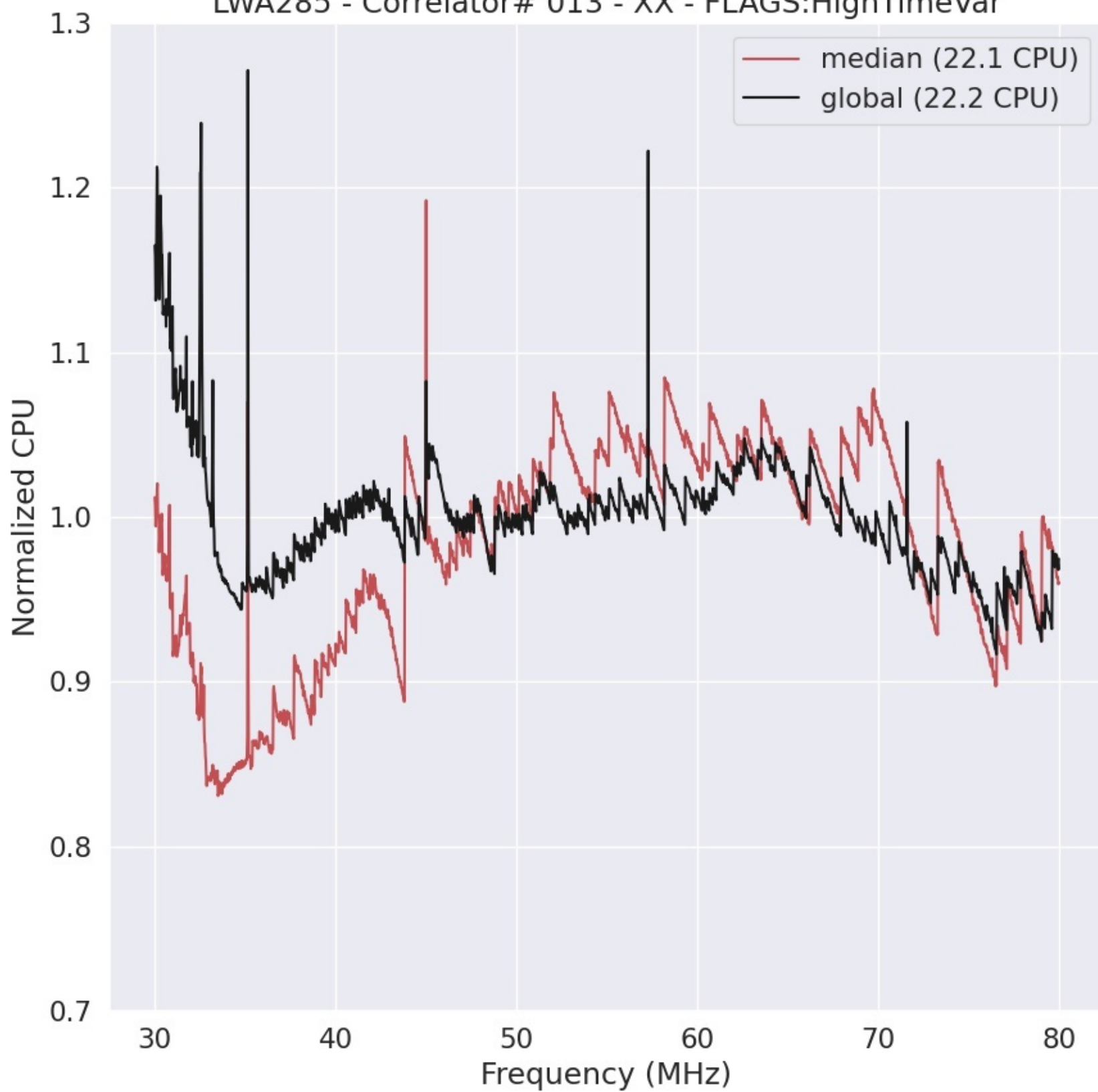
LWA285 - Correlator# 013 - XX - FLAGS:HighTimeVar
