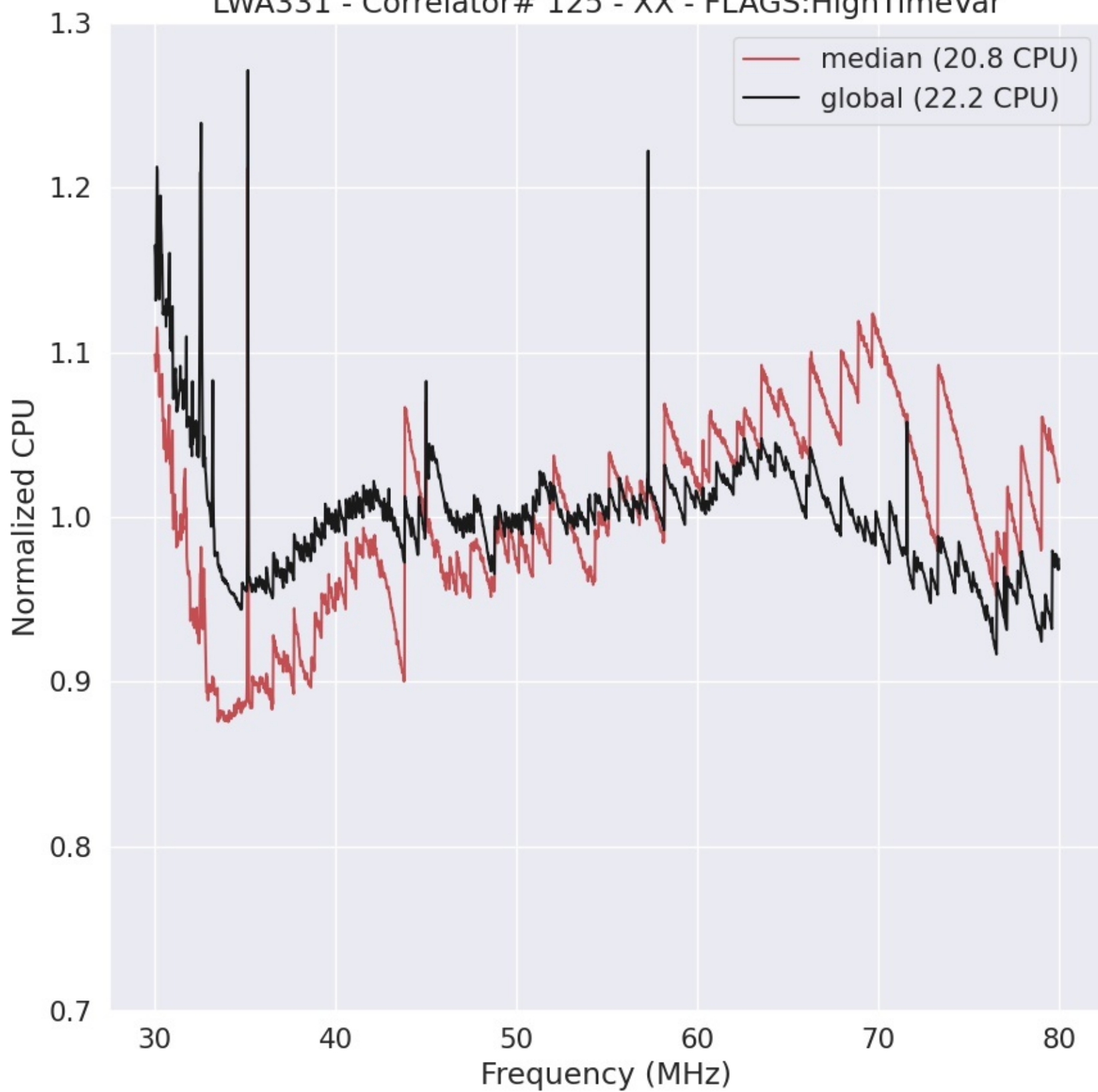
LWA331 - Correlator# 125 - XX - FLAGS:HighTimeVar
