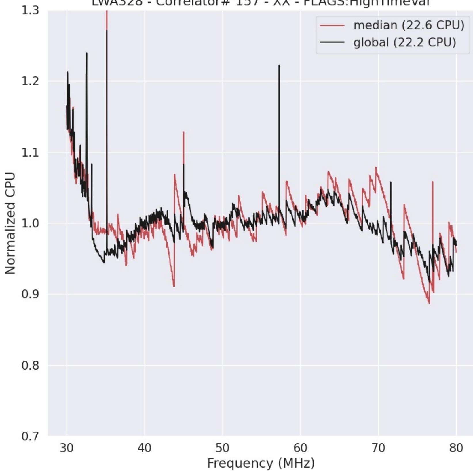
LWA328 - Correlator# 157 - XX - FLAGS:HighTimeVar
