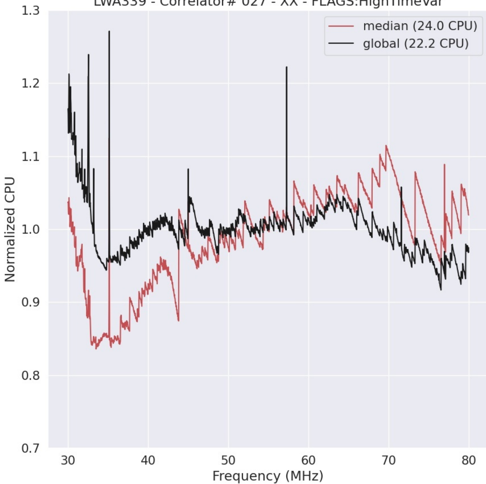
LWA339 - Correlator# 027 - XX - FLAGS:HighTimeVar
