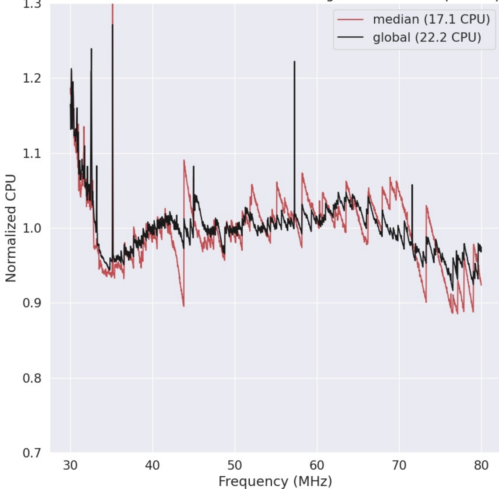
LWA271 - Correlator# 004 - XX - FLAGS:HighTimeVar+BadSpecShape
