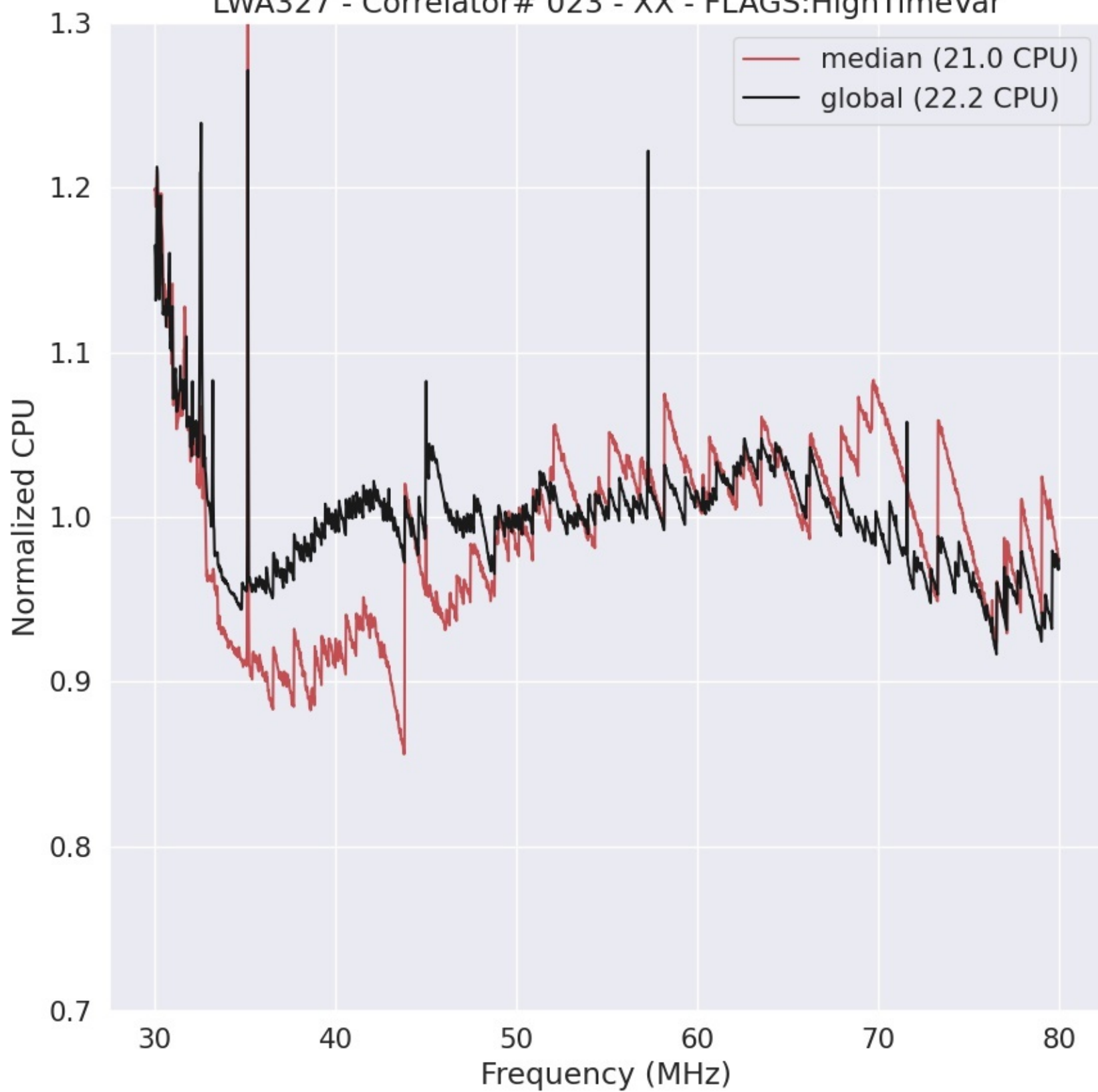
LWA327 - Correlator# 023 - XX - FLAGS:HighTimeVar
