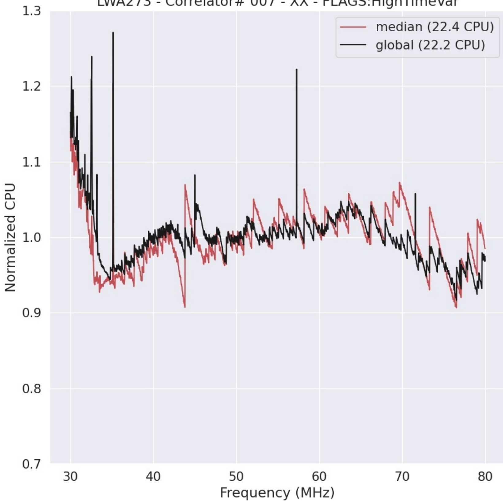
LWA273 - Correlator# 007 - XX - FLAGS:HighTimeVar
