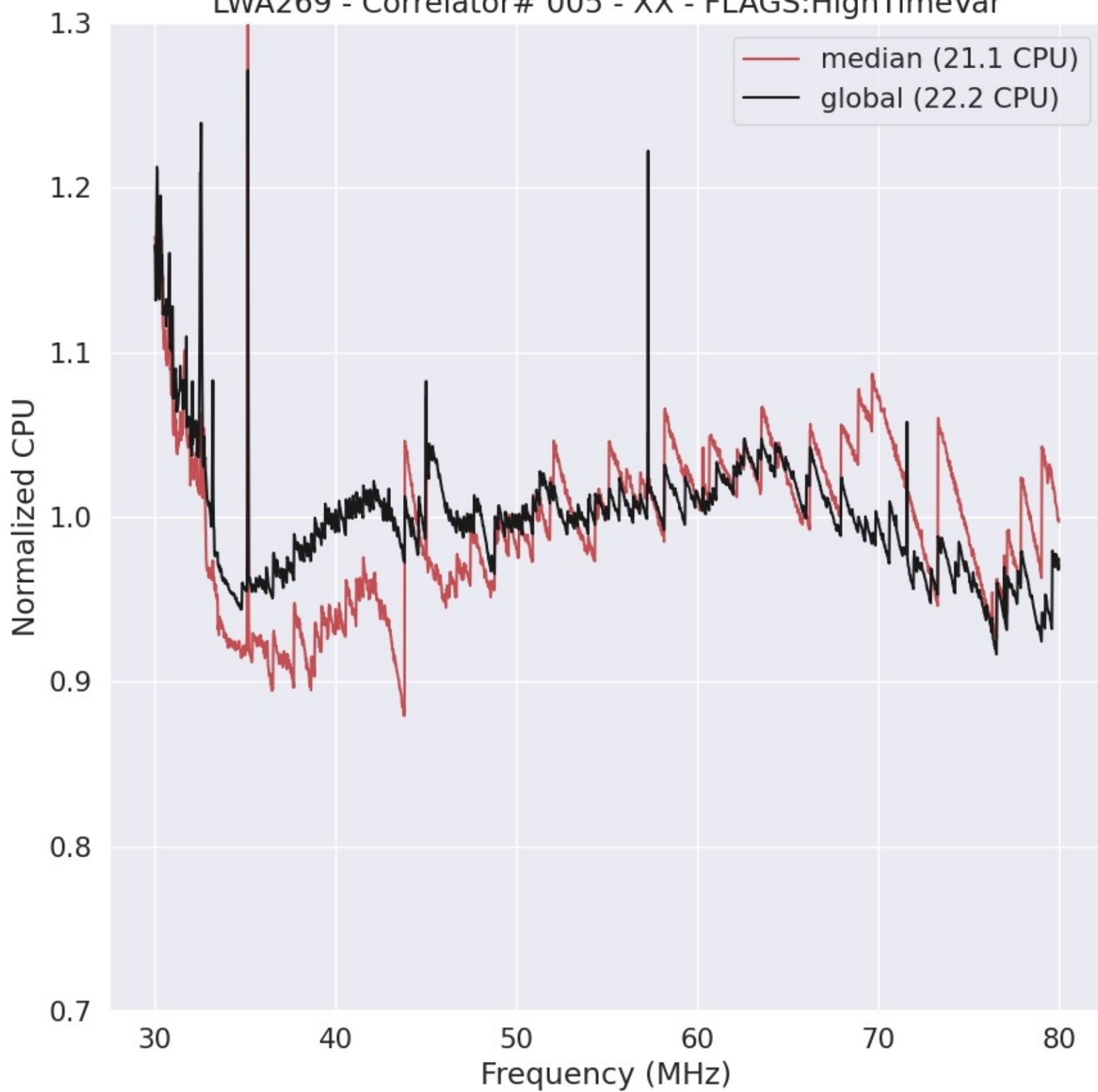
LWA269 - Correlator# 005 - XX - FLAGS:HighTimeVar
