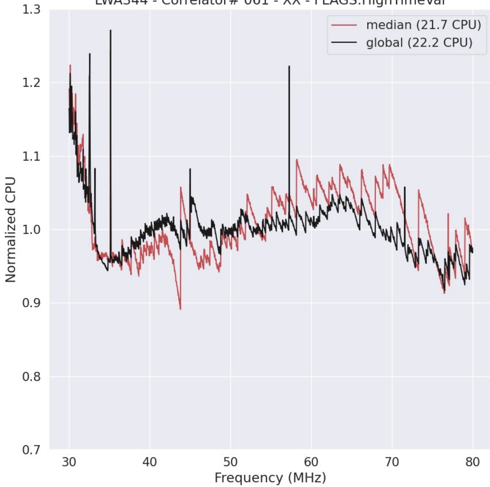
LWA344 - Correlator# 061 - XX - FLAGS:HighTimeVar
