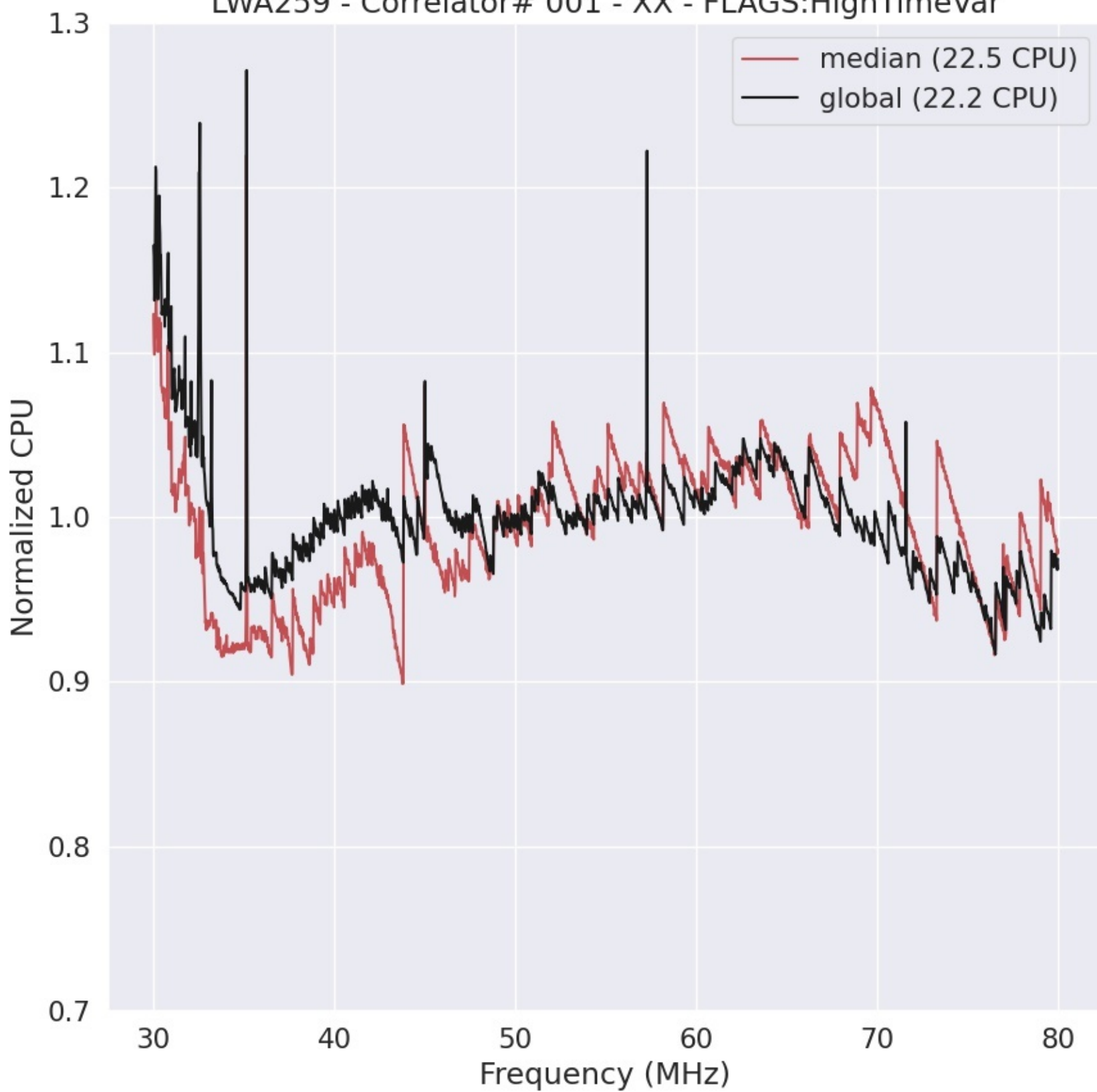
LWA259 - Correlator# 001 - XX - FLAGS:HighTimeVar
