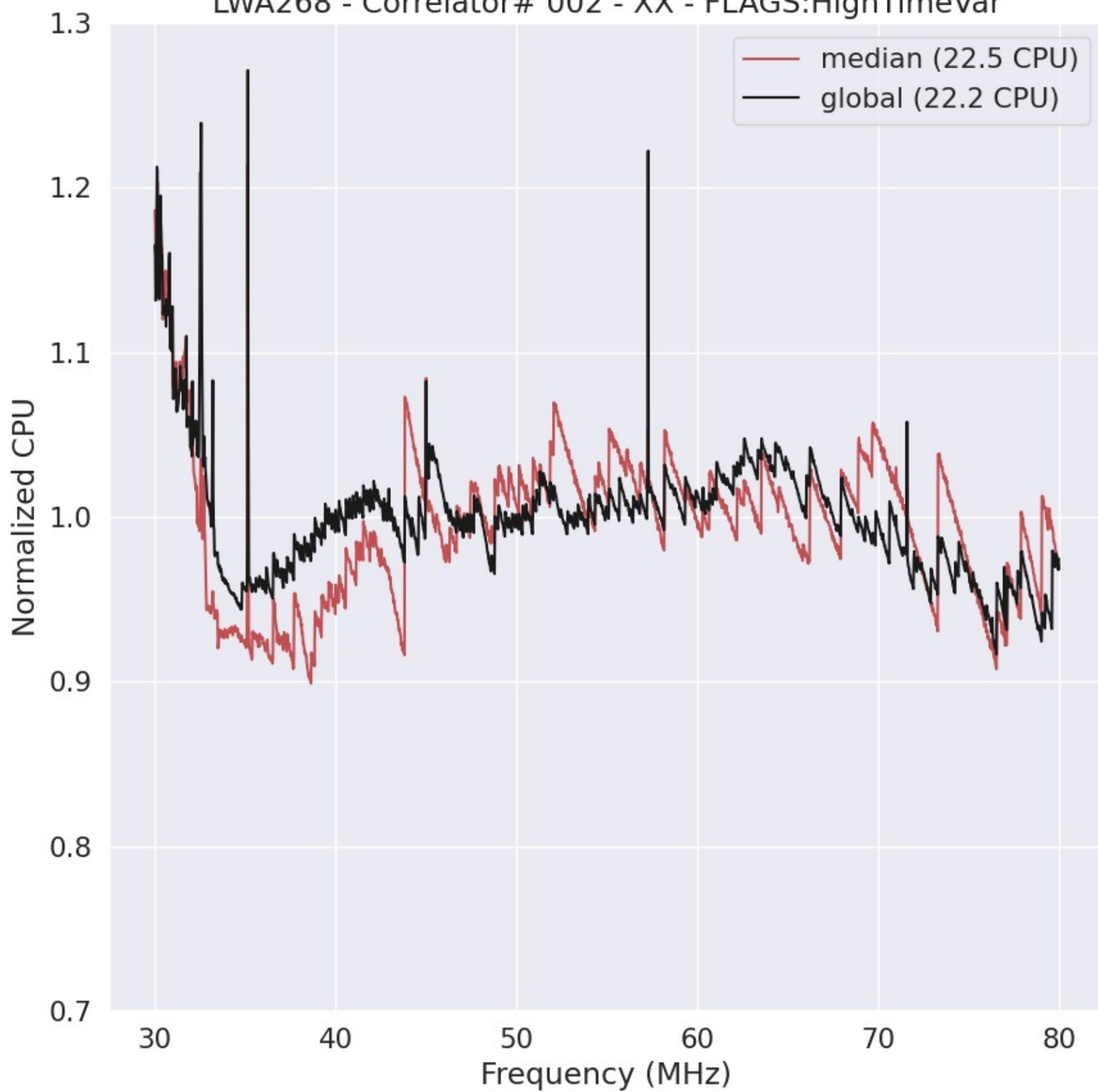
LWA268 - Correlator# 002 - XX - FLAGS:HighTimeVar
