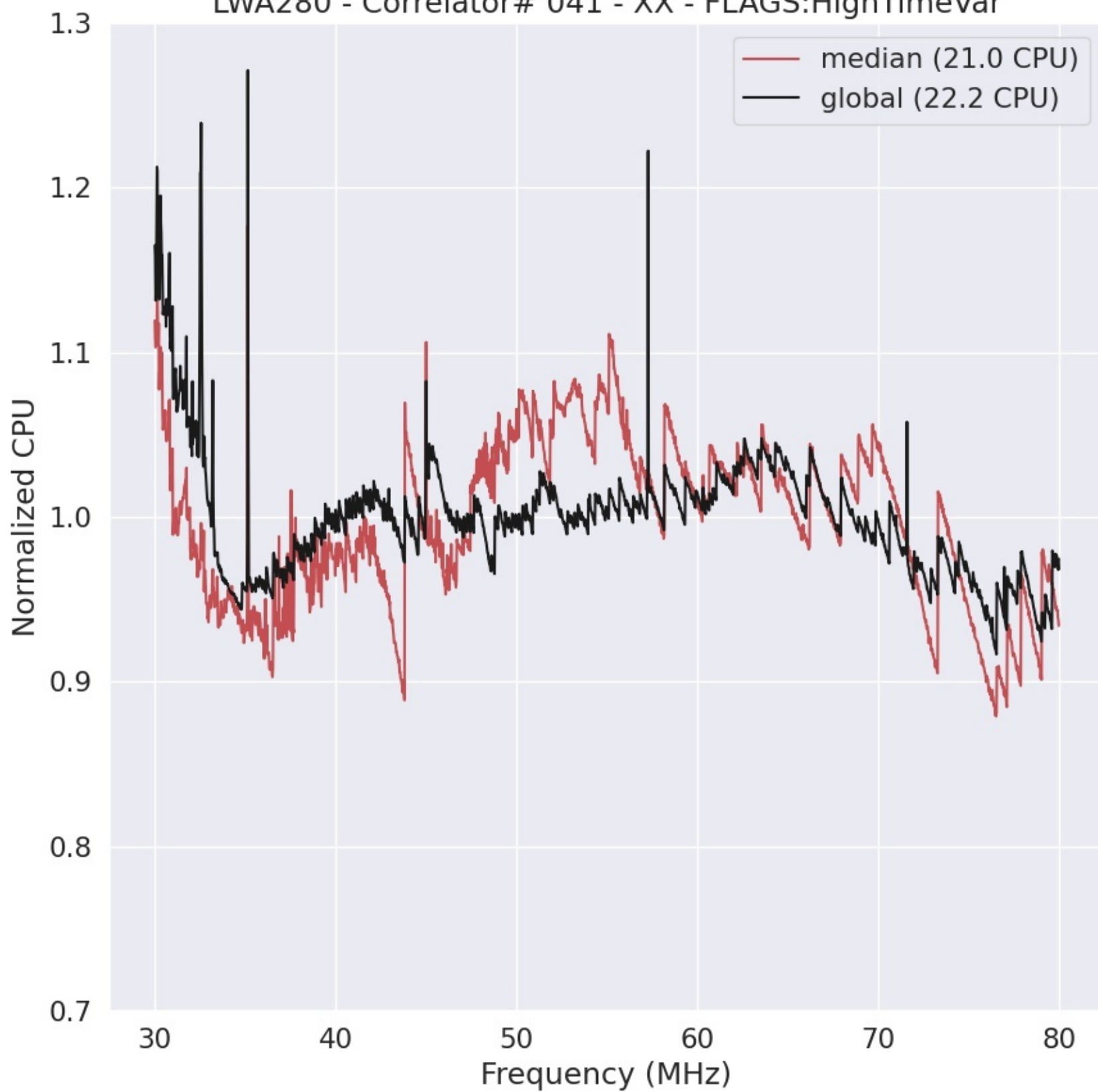
LWA280 - Correlator# 041 - XX - FLAGS:HighTimeVar
