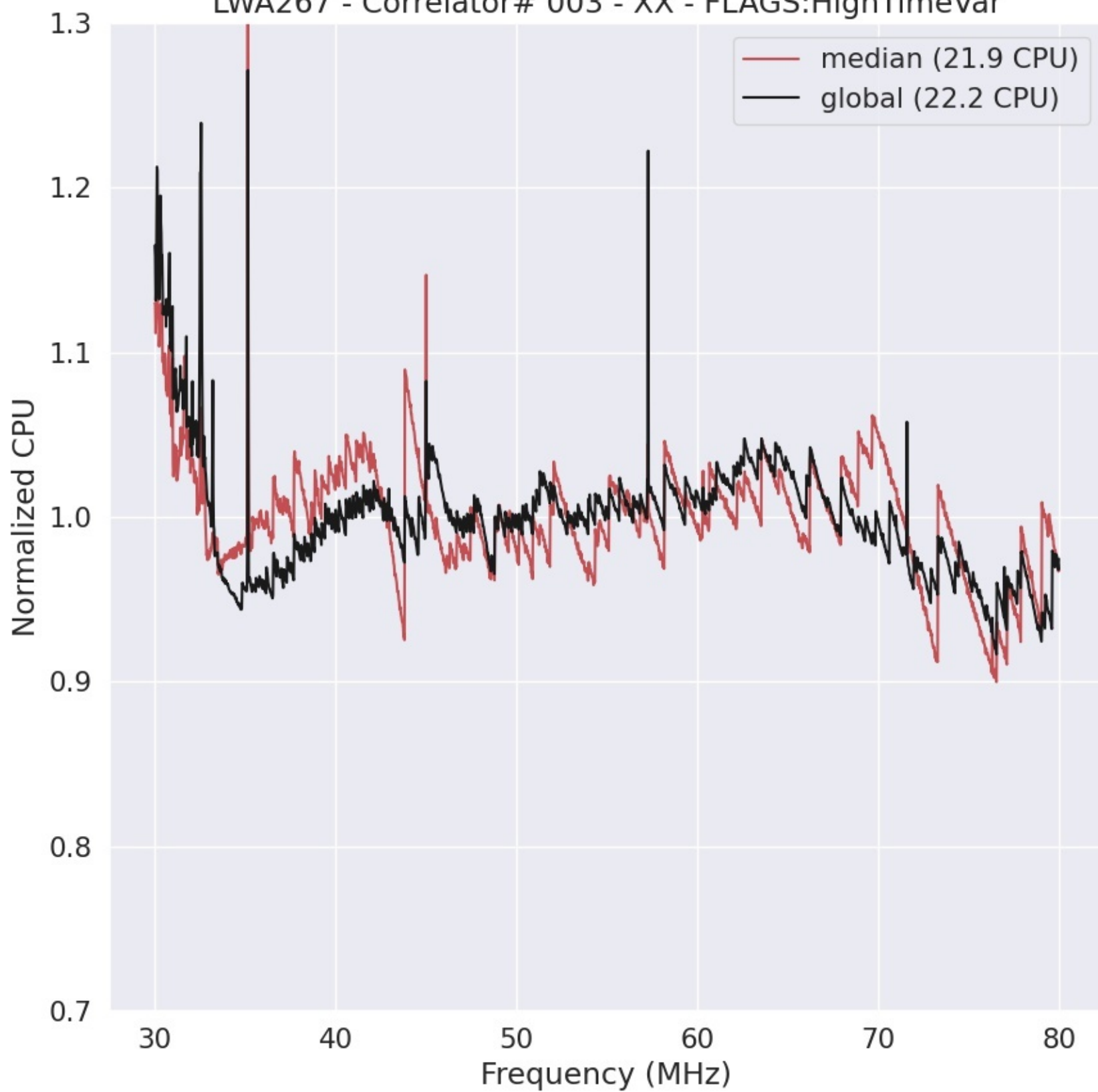
LWA267 - Correlator# 003 - XX - FLAGS:HighTimeVar
