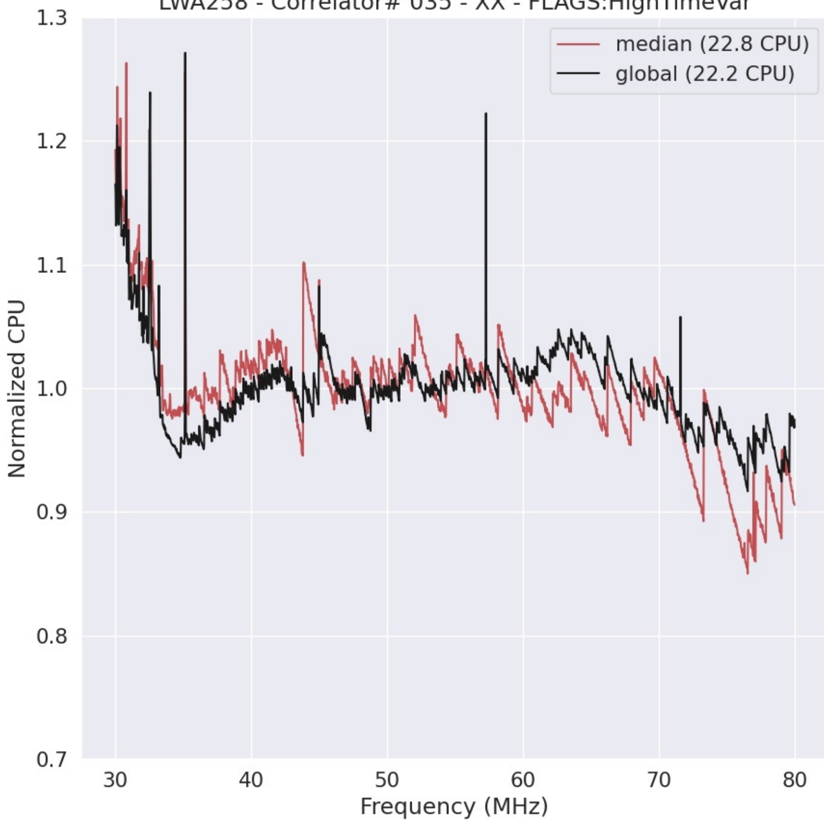
LWA258 - Correlator# 035 - XX - FLAGS:HighTimeVar
