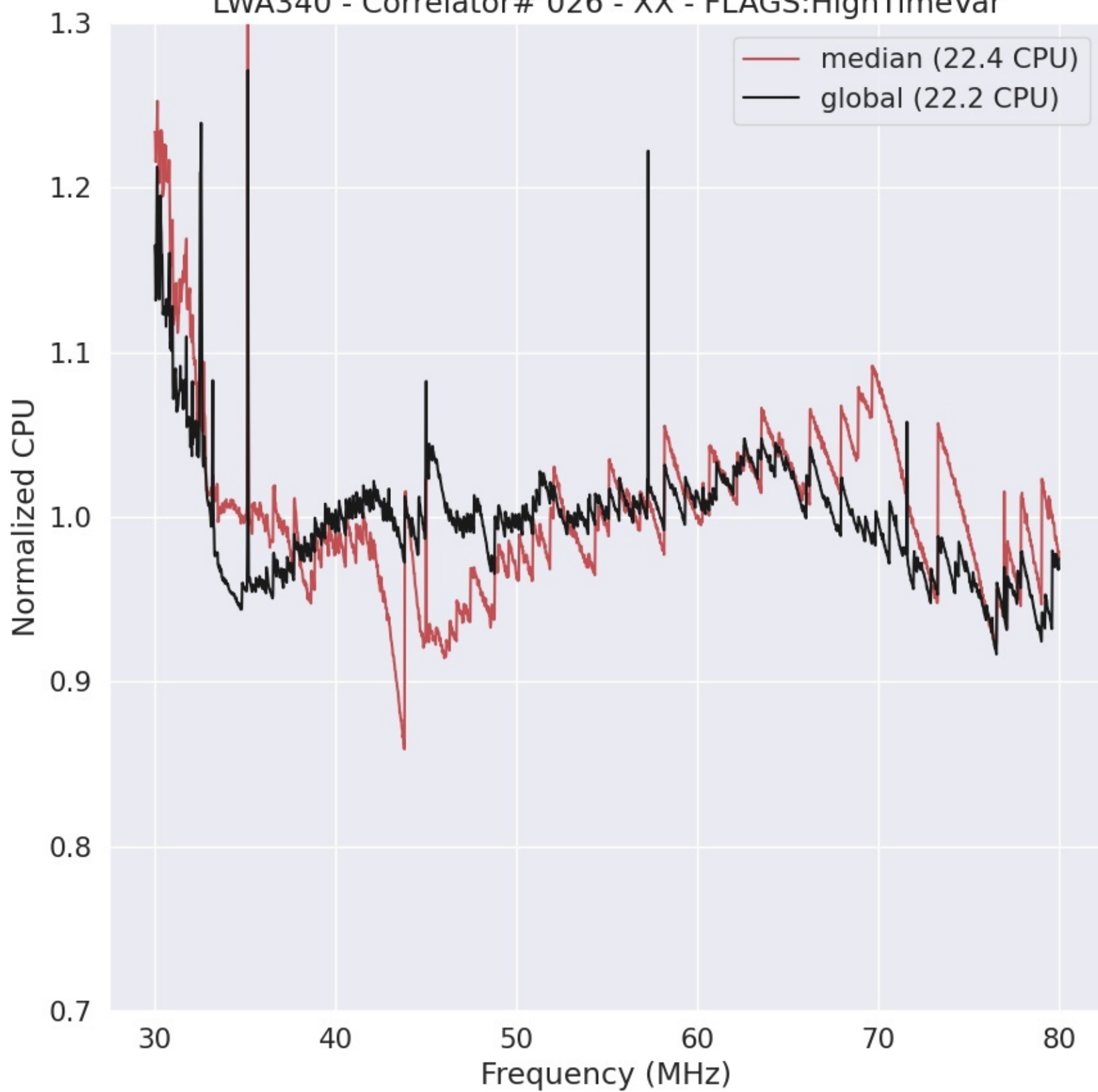
LWA340 - Correlator# 026 - XX - FLAGS:HighTimeVar
