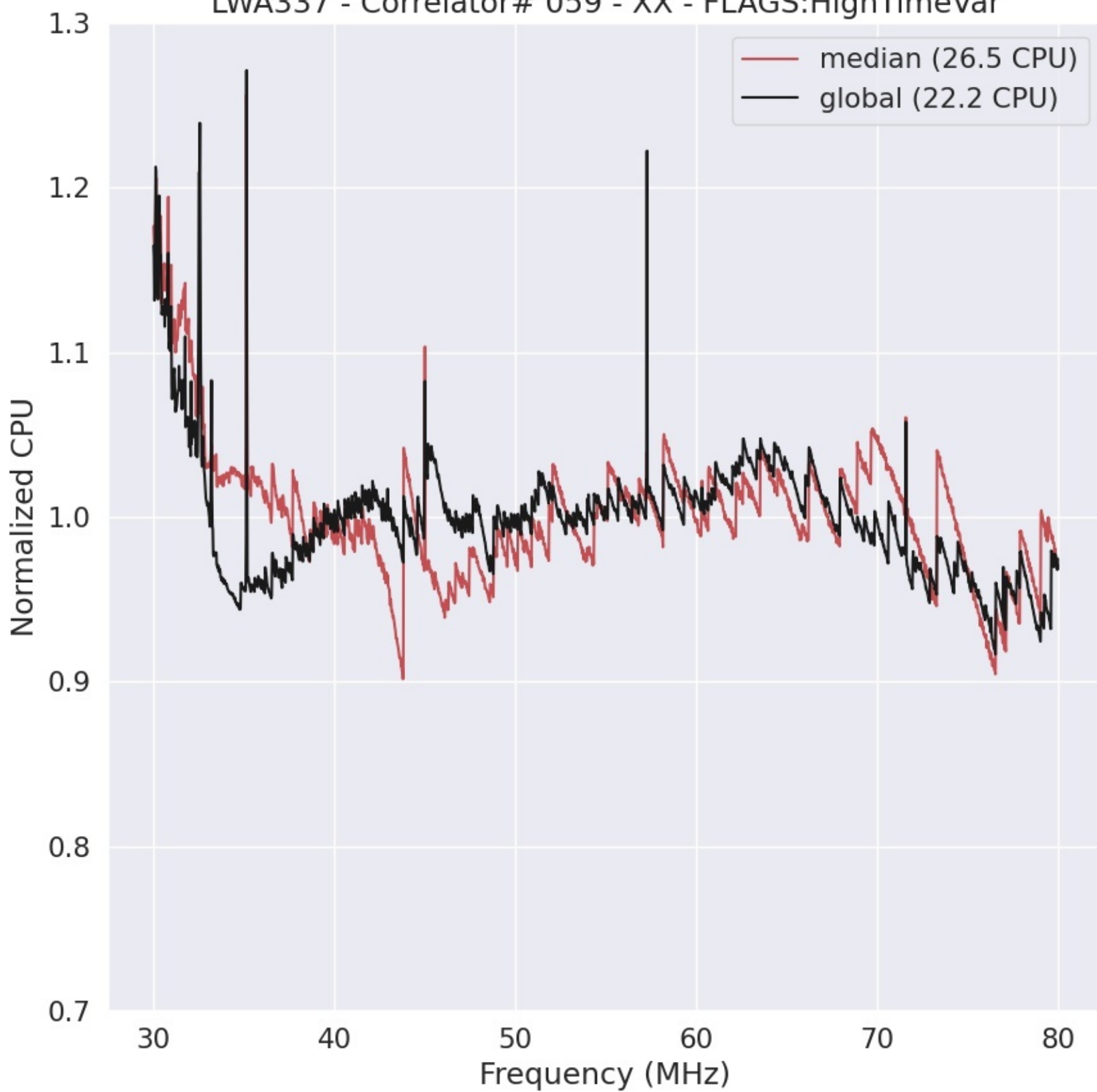
LWA337 - Correlator# 059 - XX - FLAGS:HighTimeVar
