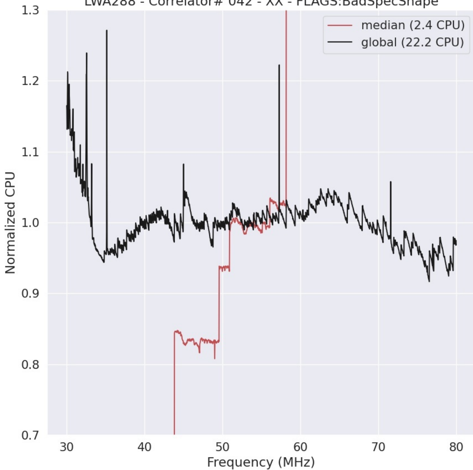
LWA288 - Correlator# 042 - XX - FLAGS:BadSpecShape
