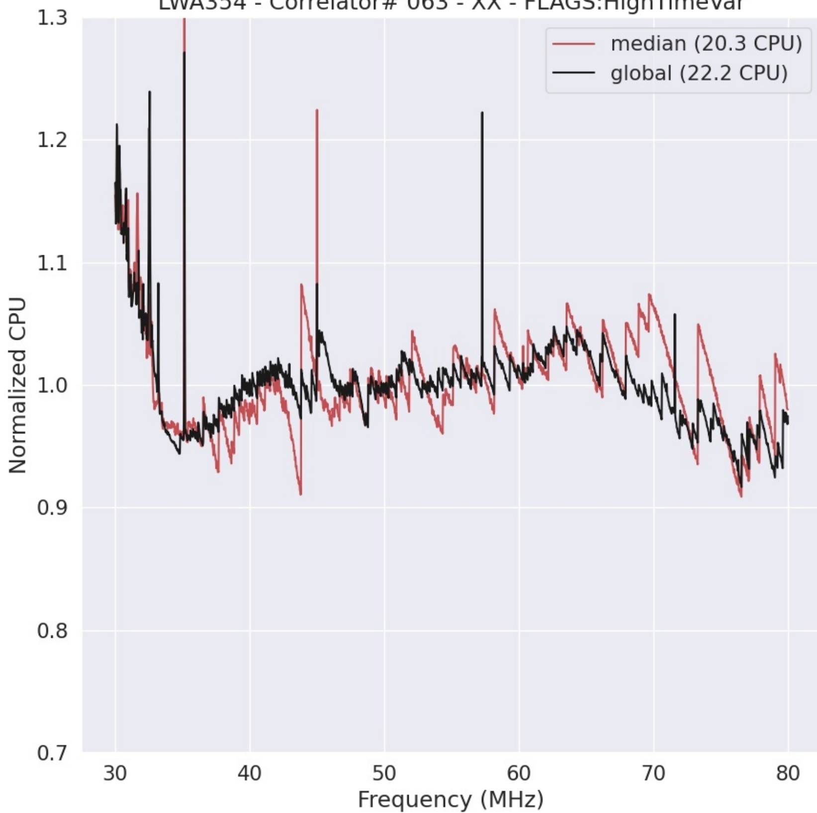
LWA354 - Correlator# 063 - XX - FLAGS:HighTimeVar
