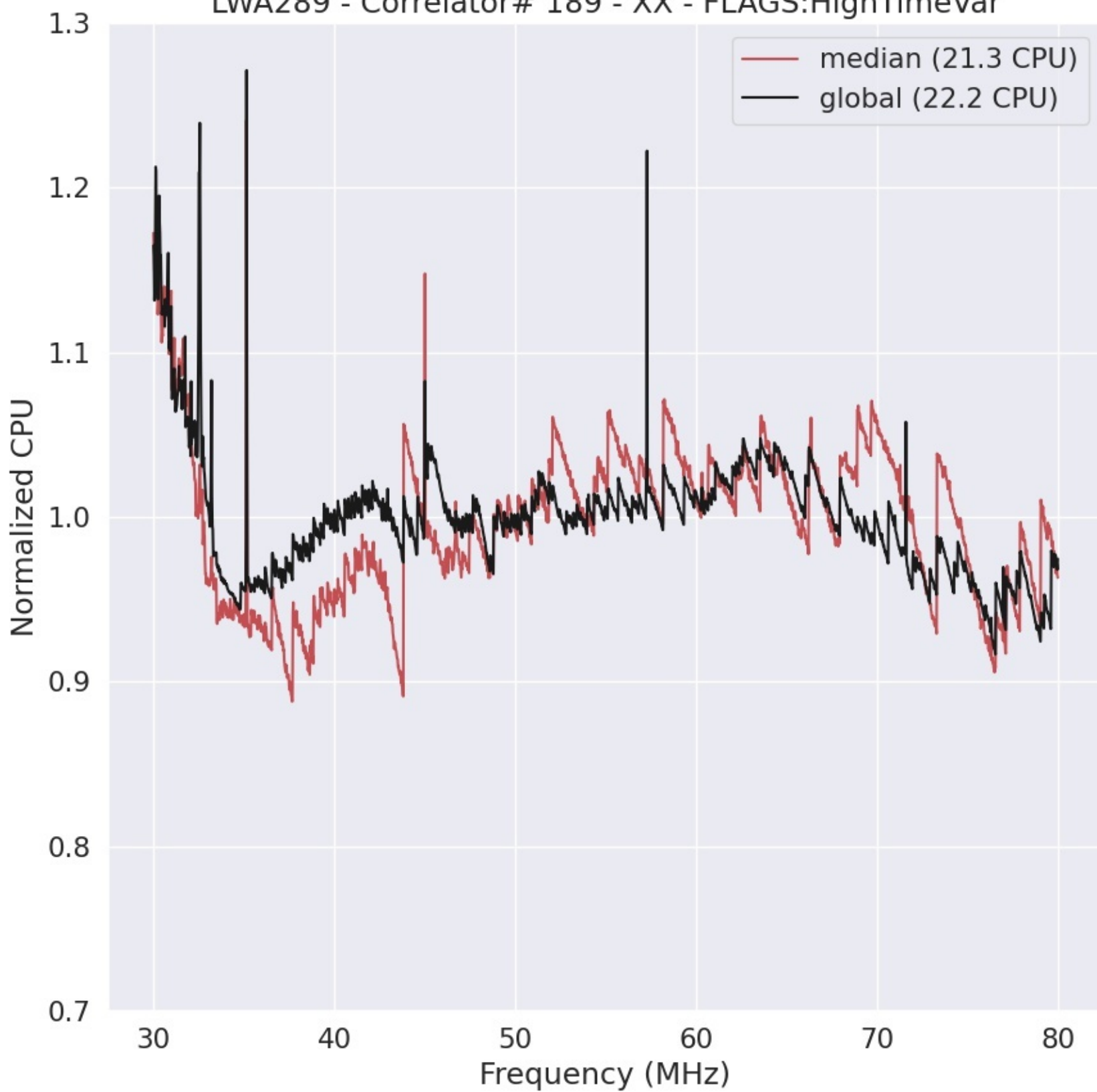
LWA289 - Correlator# 189 - XX - FLAGS:HighTimeVar
