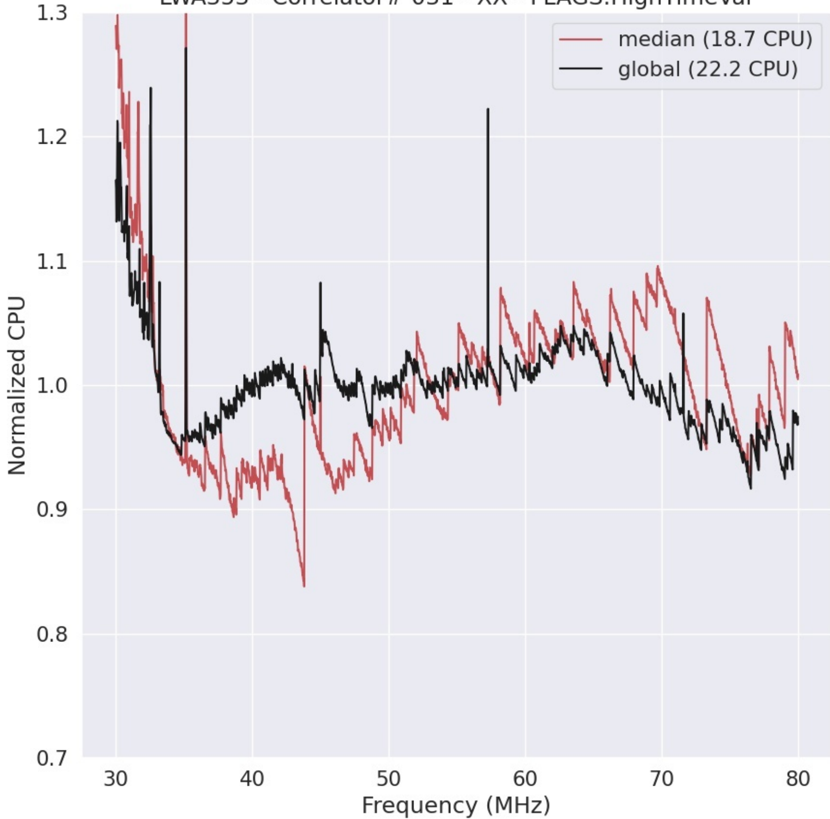
LWA353 - Correlator# 031 - XX - FLAGS:HighTimeVar
