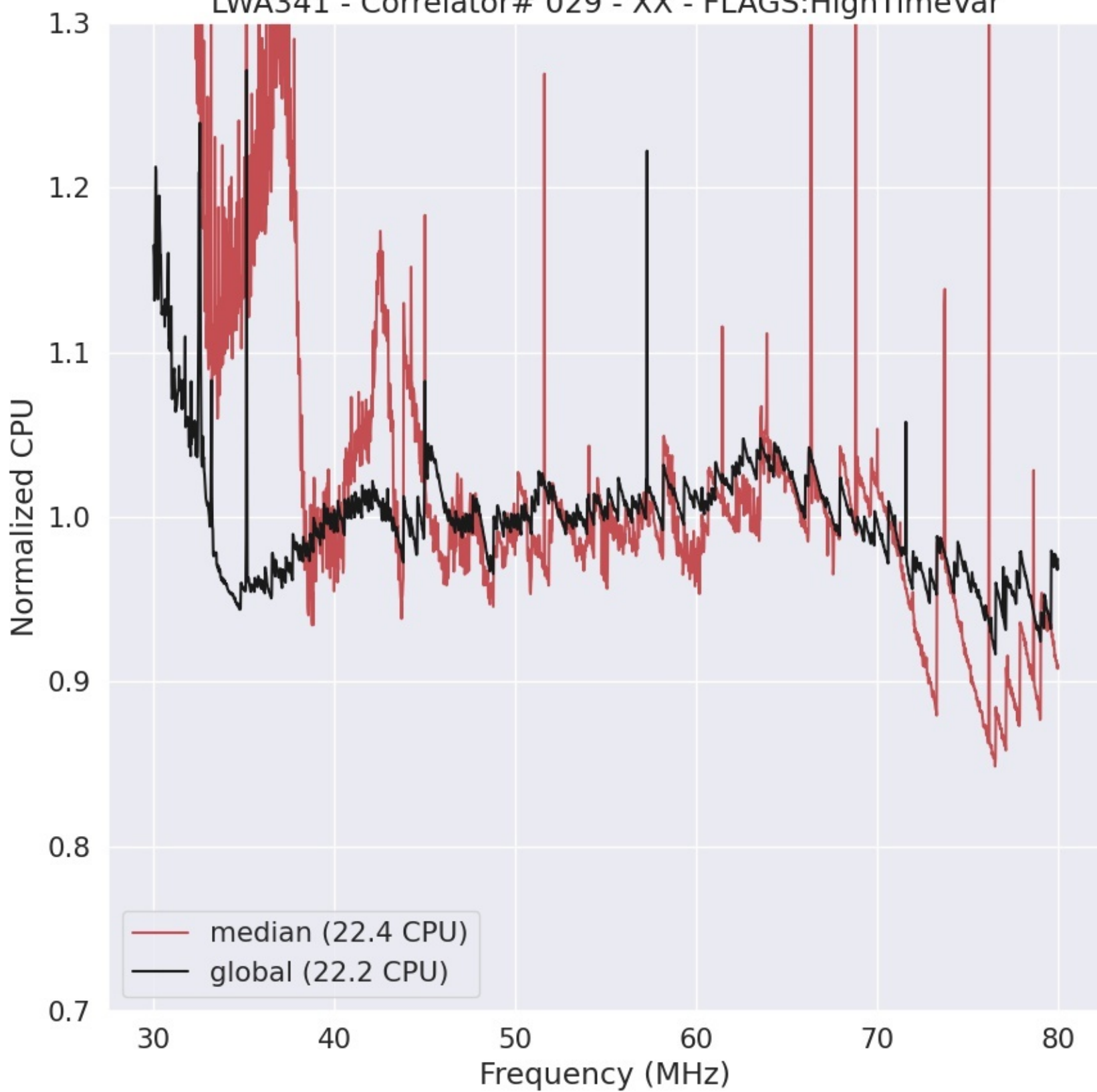
LWA341 - Correlator# 029 - XX - FLAGS:HighTimeVar
