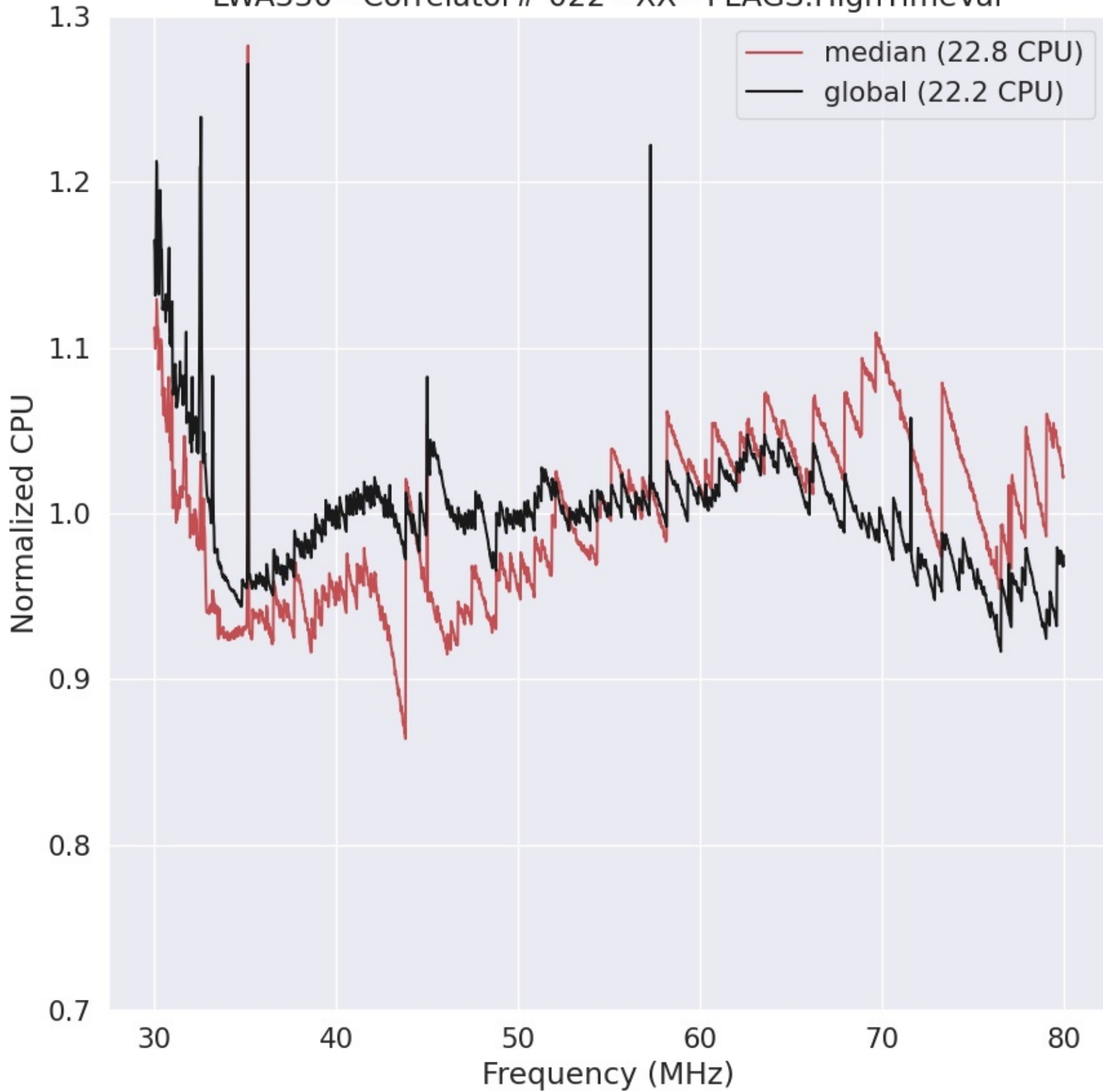
LWA330 - Correlator# 022 - XX - FLAGS:HighTimeVar
