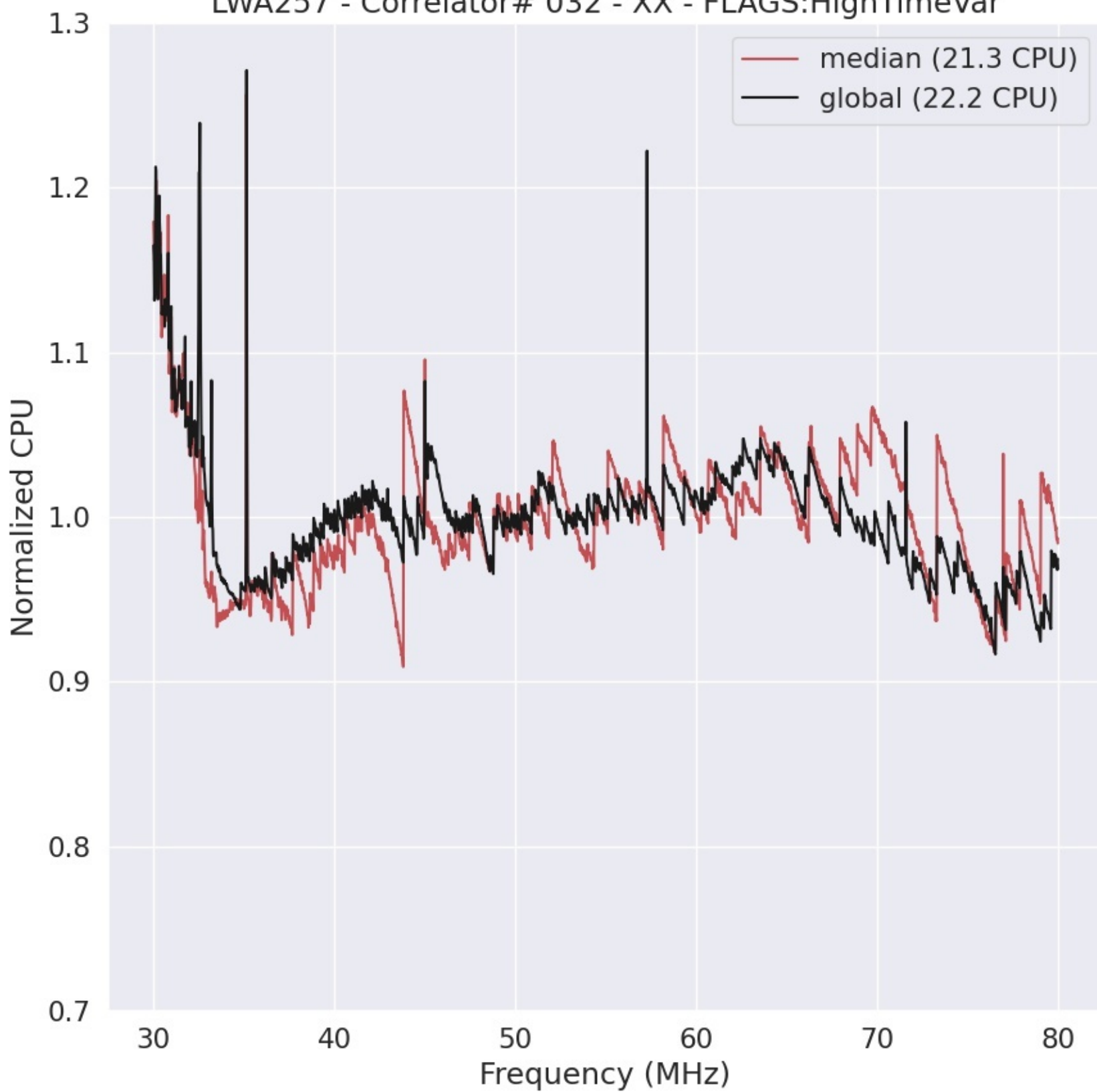
LWA257 - Correlator# 032 - XX - FLAGS:HighTimeVar
