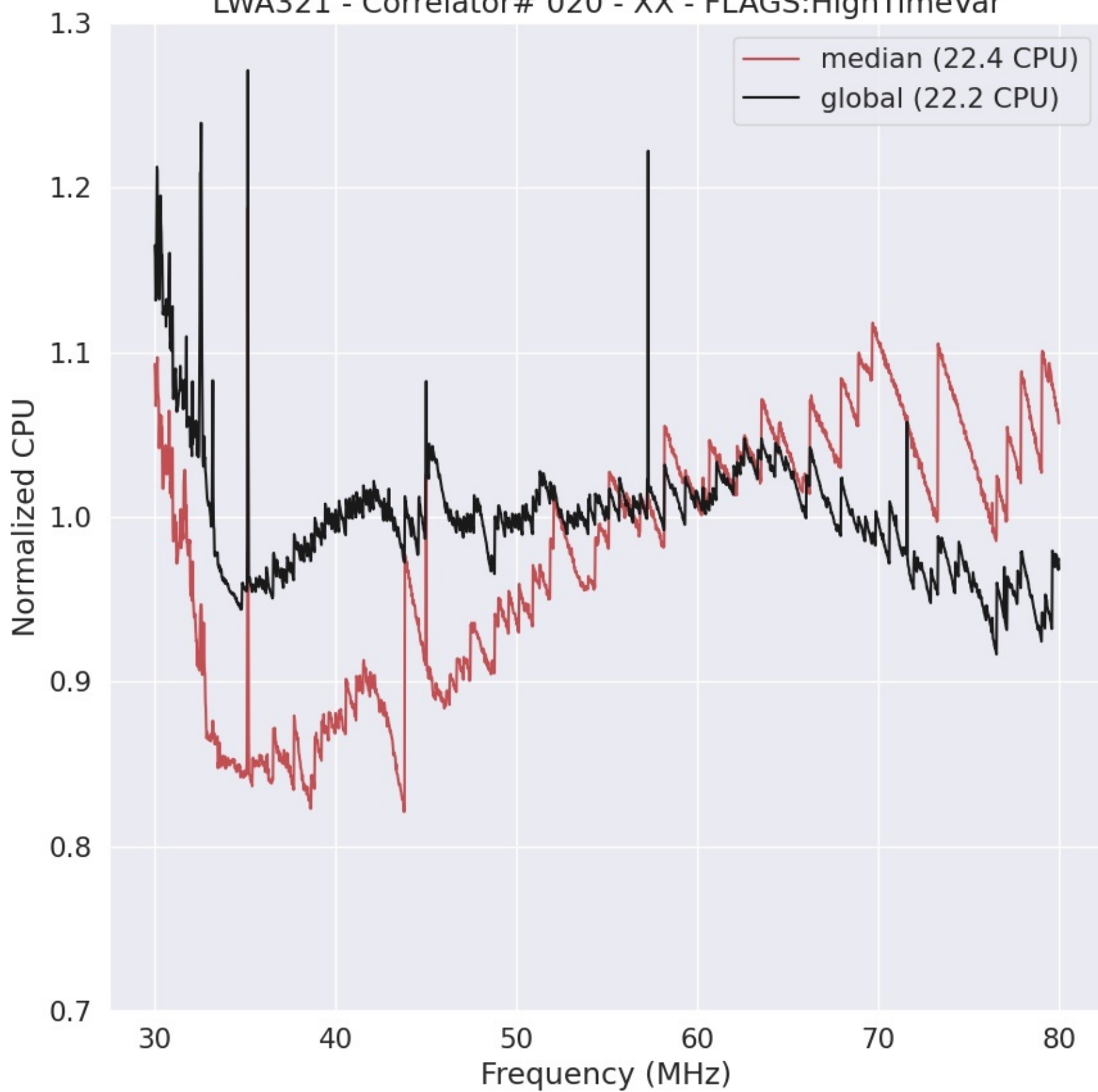
LWA321 - Correlator# 020 - XX - FLAGS:HighTimeVar
