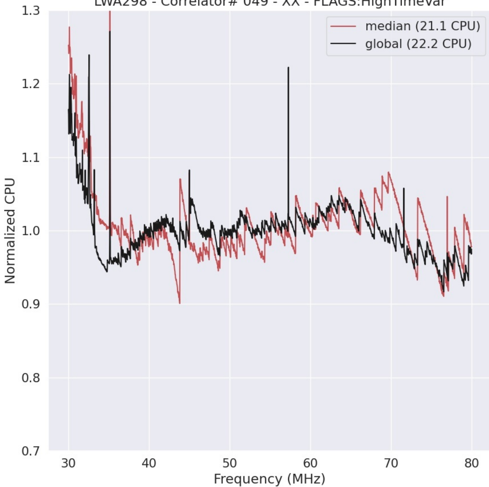
LWA298 - Correlator# 049 - XX - FLAGS:HighTimeVar
