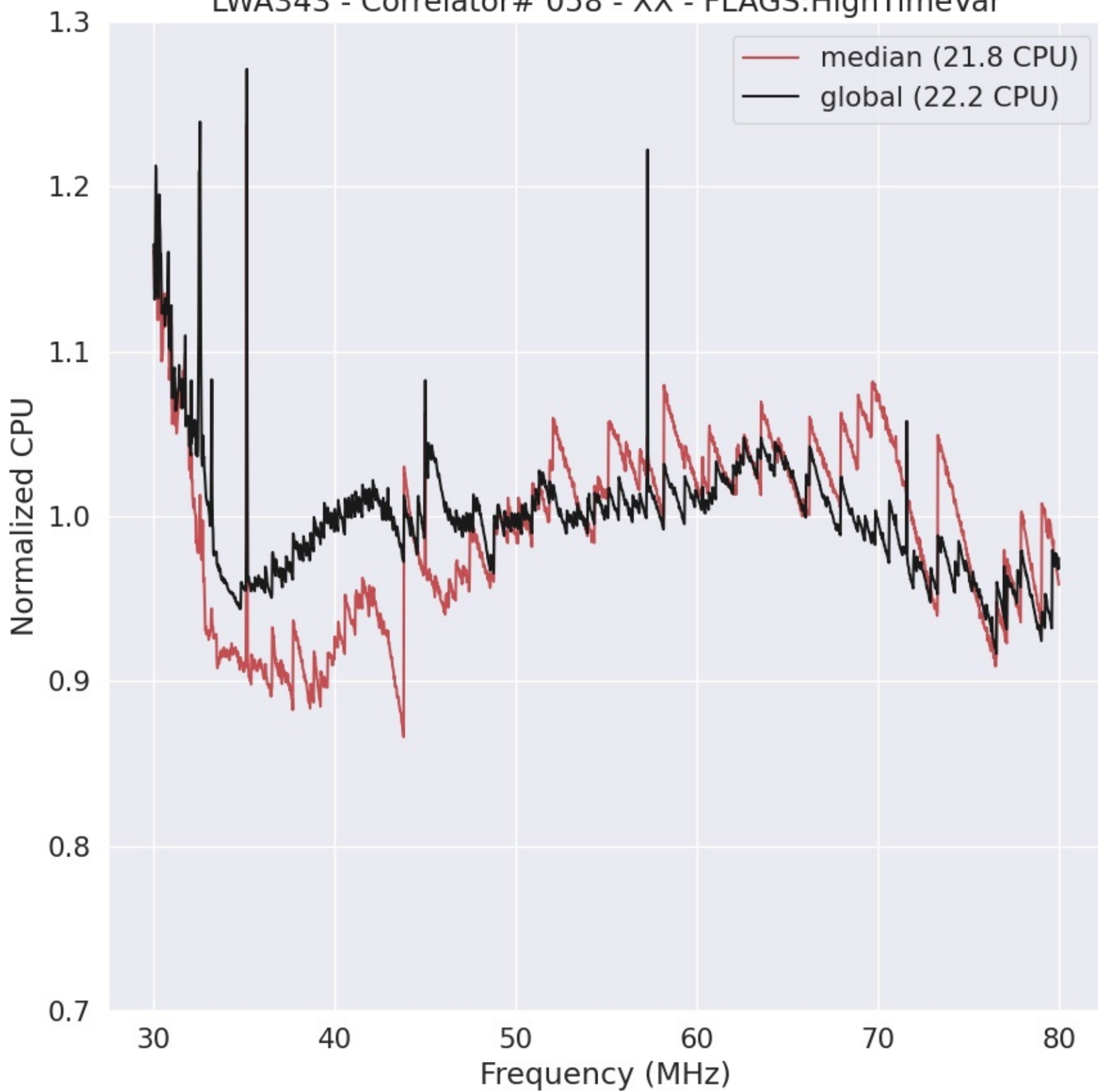
LWA343 - Correlator# 058 - XX - FLAGS:HighTimeVar
