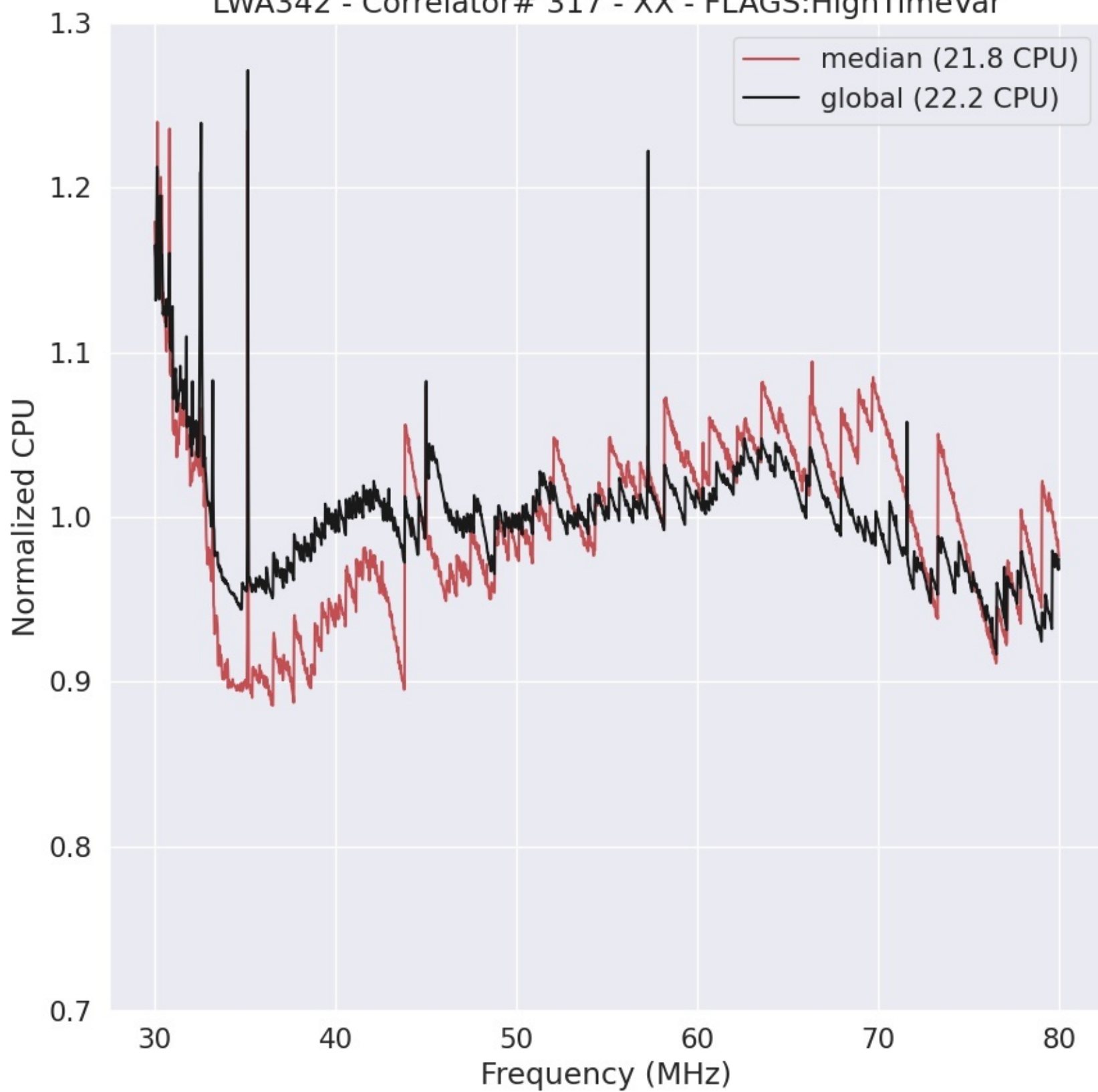
LWA342 - Correlator# 317 - XX - FLAGS:HighTimeVar
