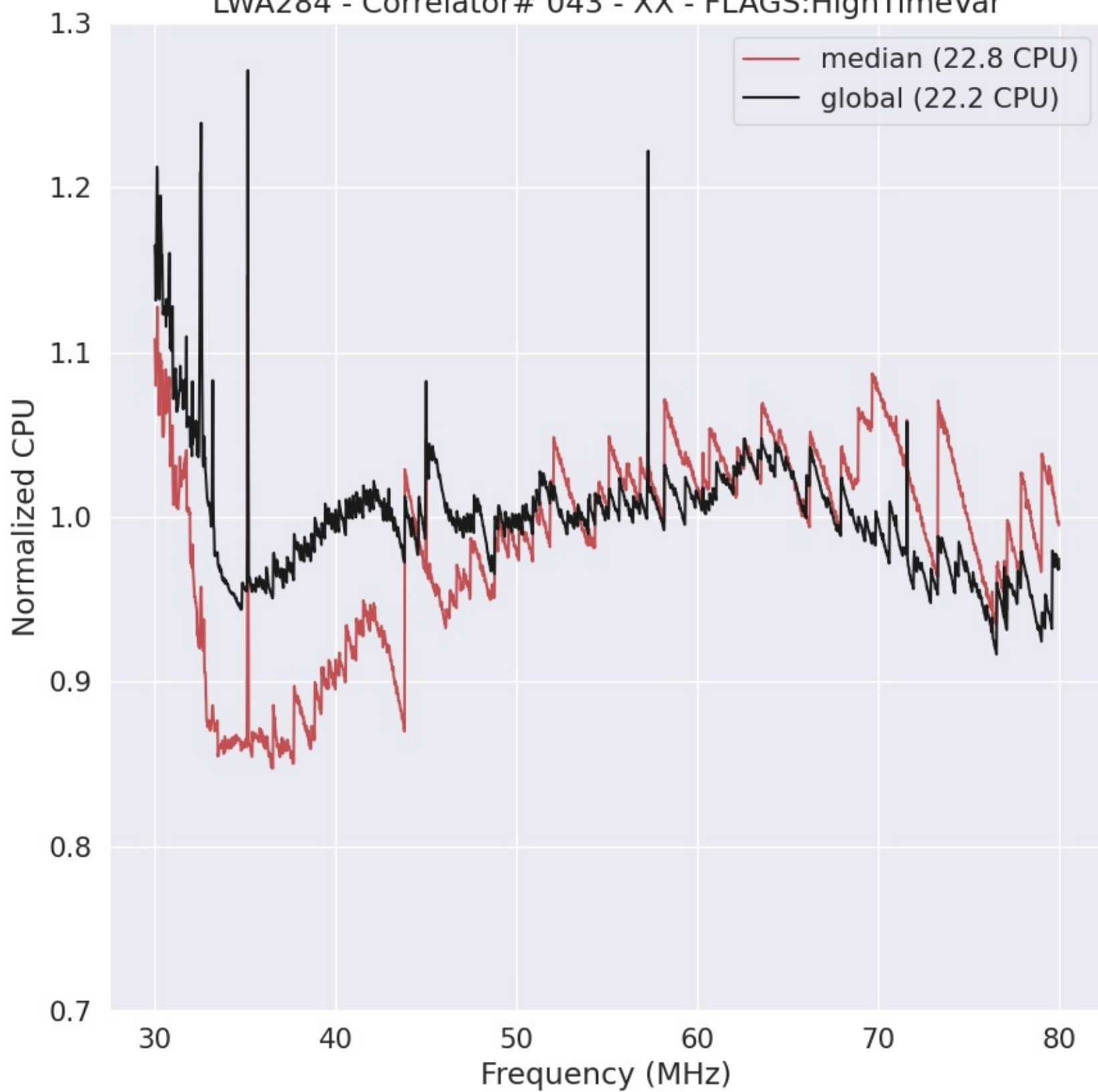
LWA284 - Correlator# 043 - XX - FLAGS:HighTimeVar
