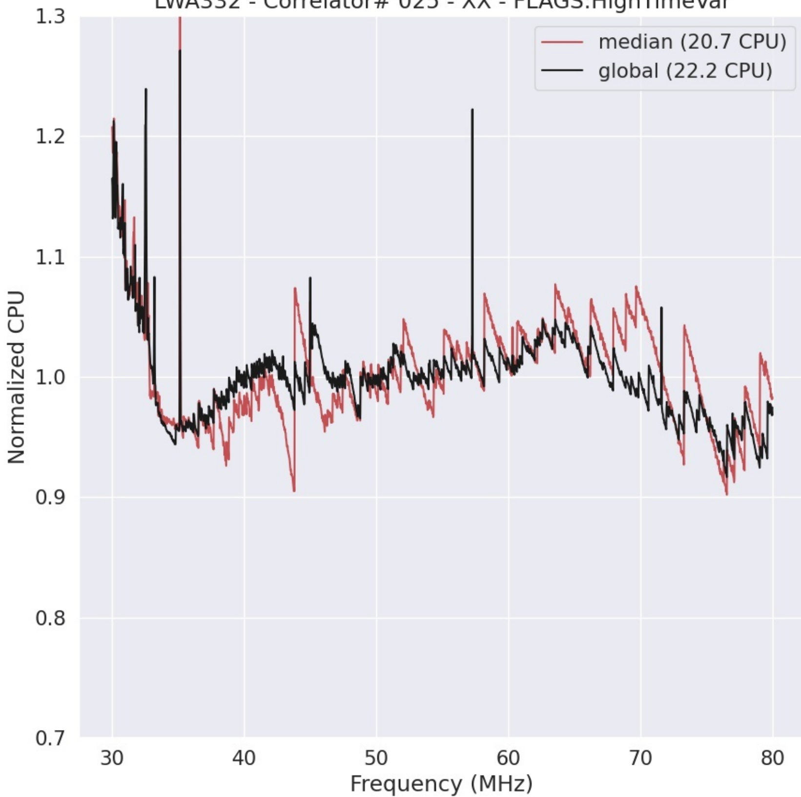
LWA332 - Correlator# 025 - XX - FLAGS:HighTimeVar
