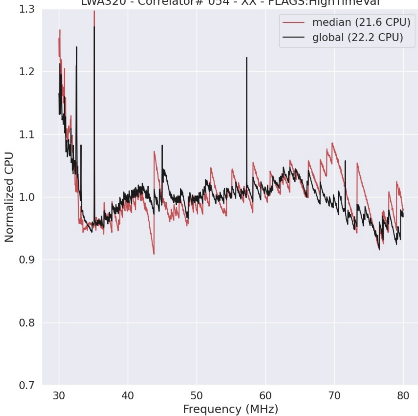
LWA320 - Correlator# 054 - XX - FLAGS:HighTimeVar
