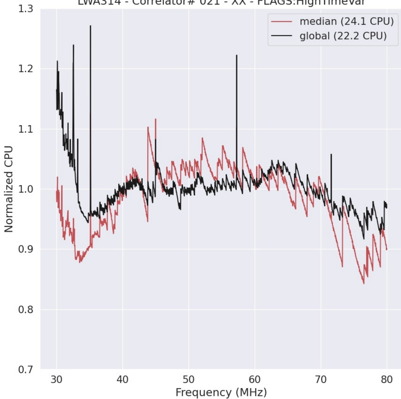
LWA314 - Correlator# 021 - XX - FLAGS:HighTimeVar
