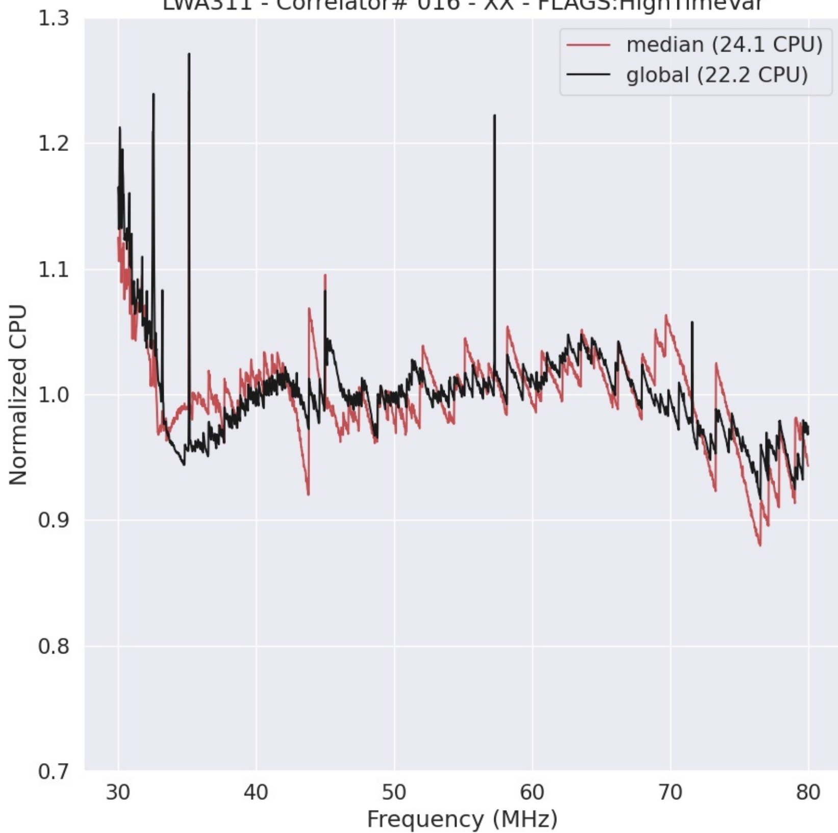
LWA311 - Correlator# 016 - XX - FLAGS:HighTimeVar
