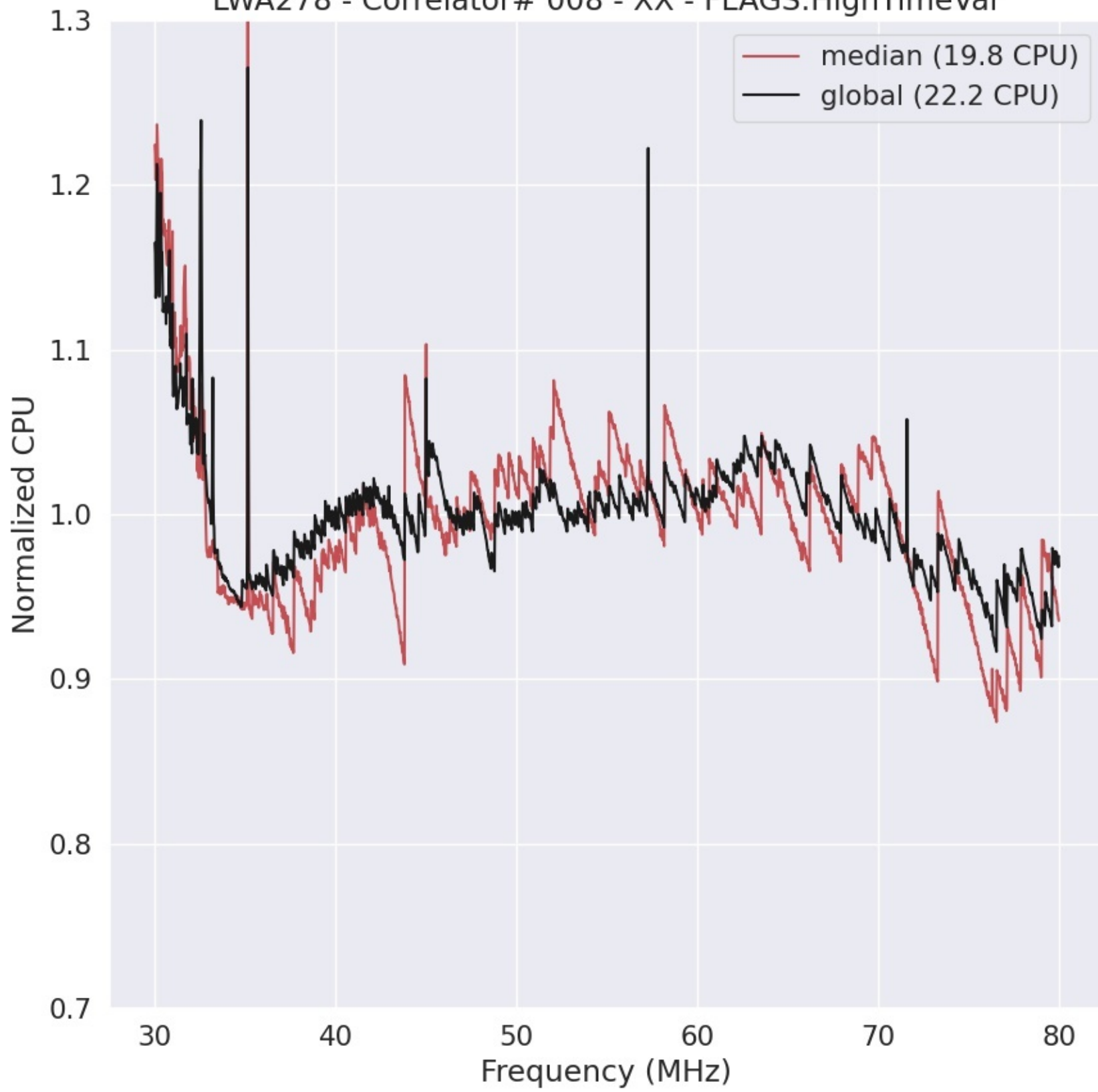
LWA278 - Correlator# 008 - XX - FLAGS:HighTimeVar
