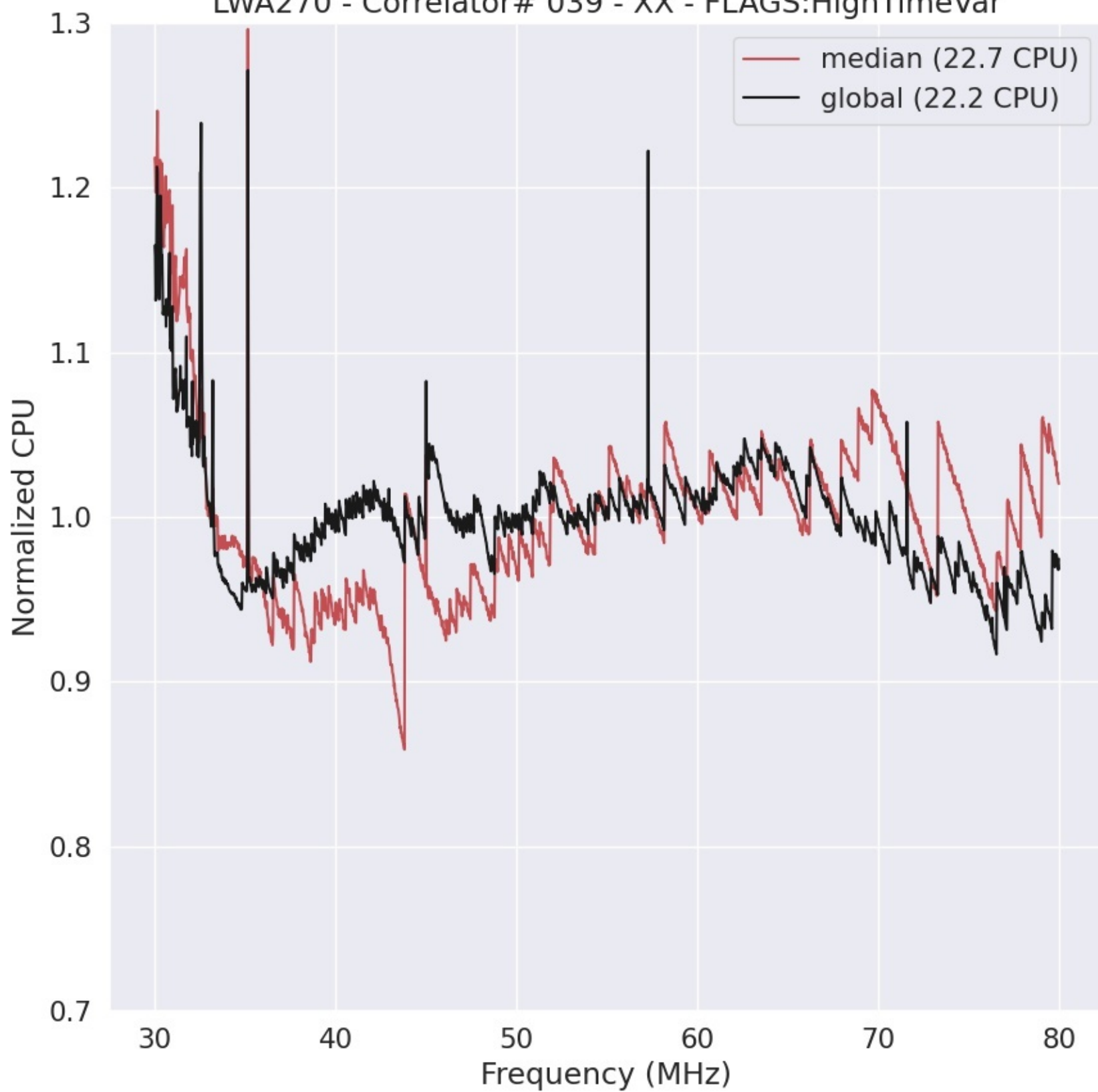
LWA270 - Correlator# 039 - XX - FLAGS:HighTimeVar
