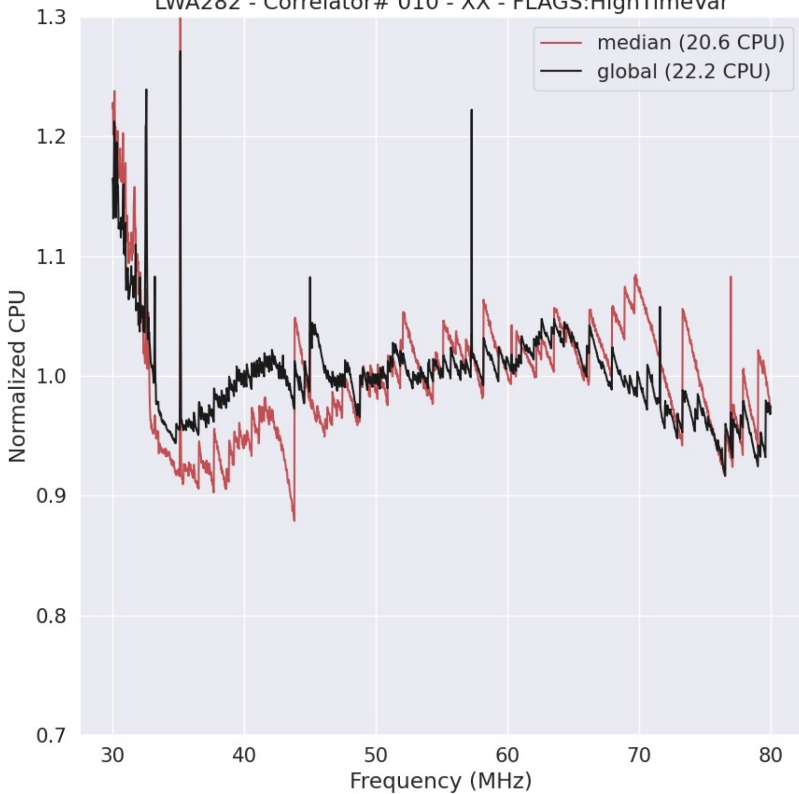
LWA282 - Correlator# 010 - XX - FLAGS:HighTimeVar
