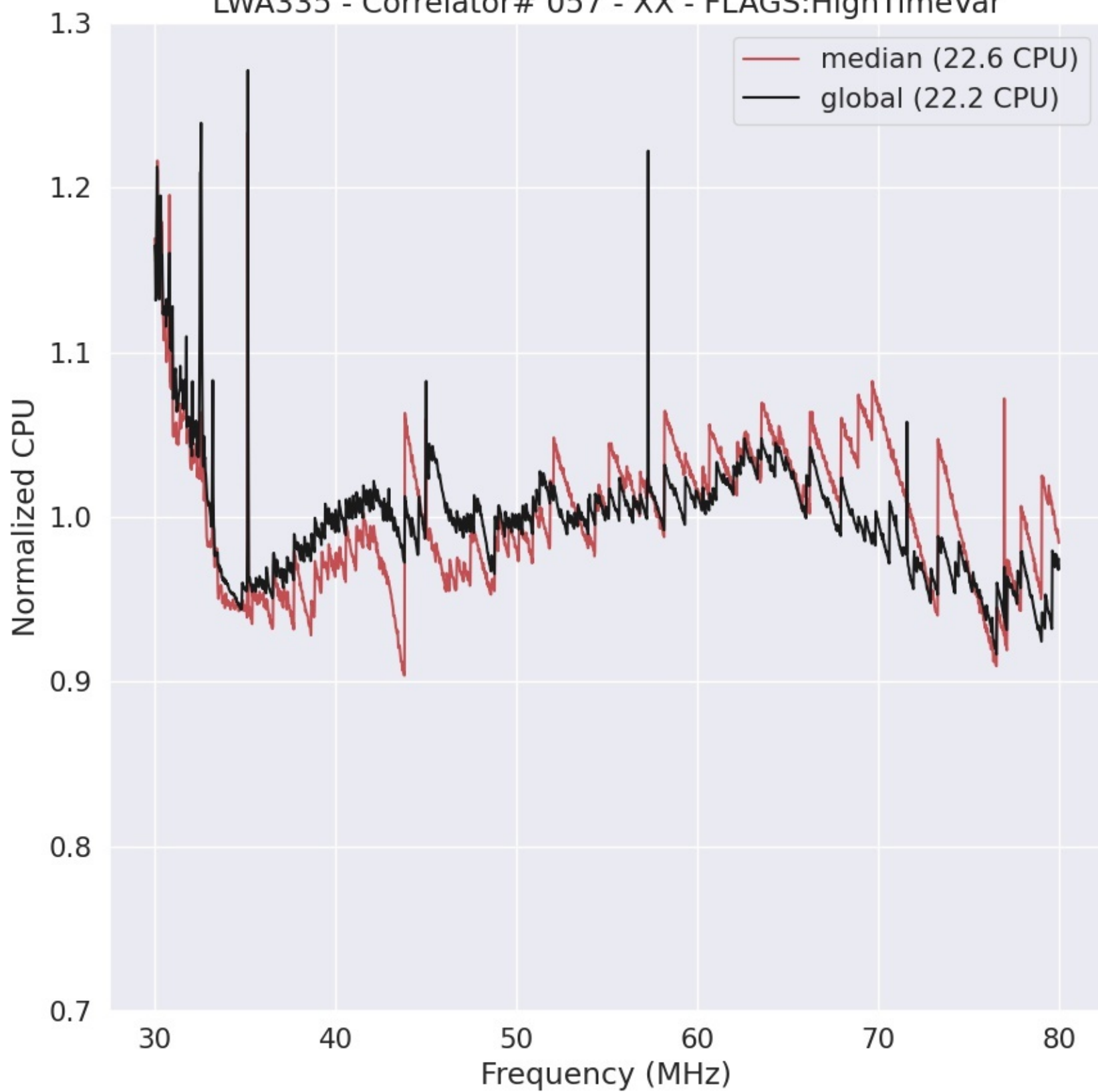
LWA335 - Correlator# 057 - XX - FLAGS:HighTimeVar
