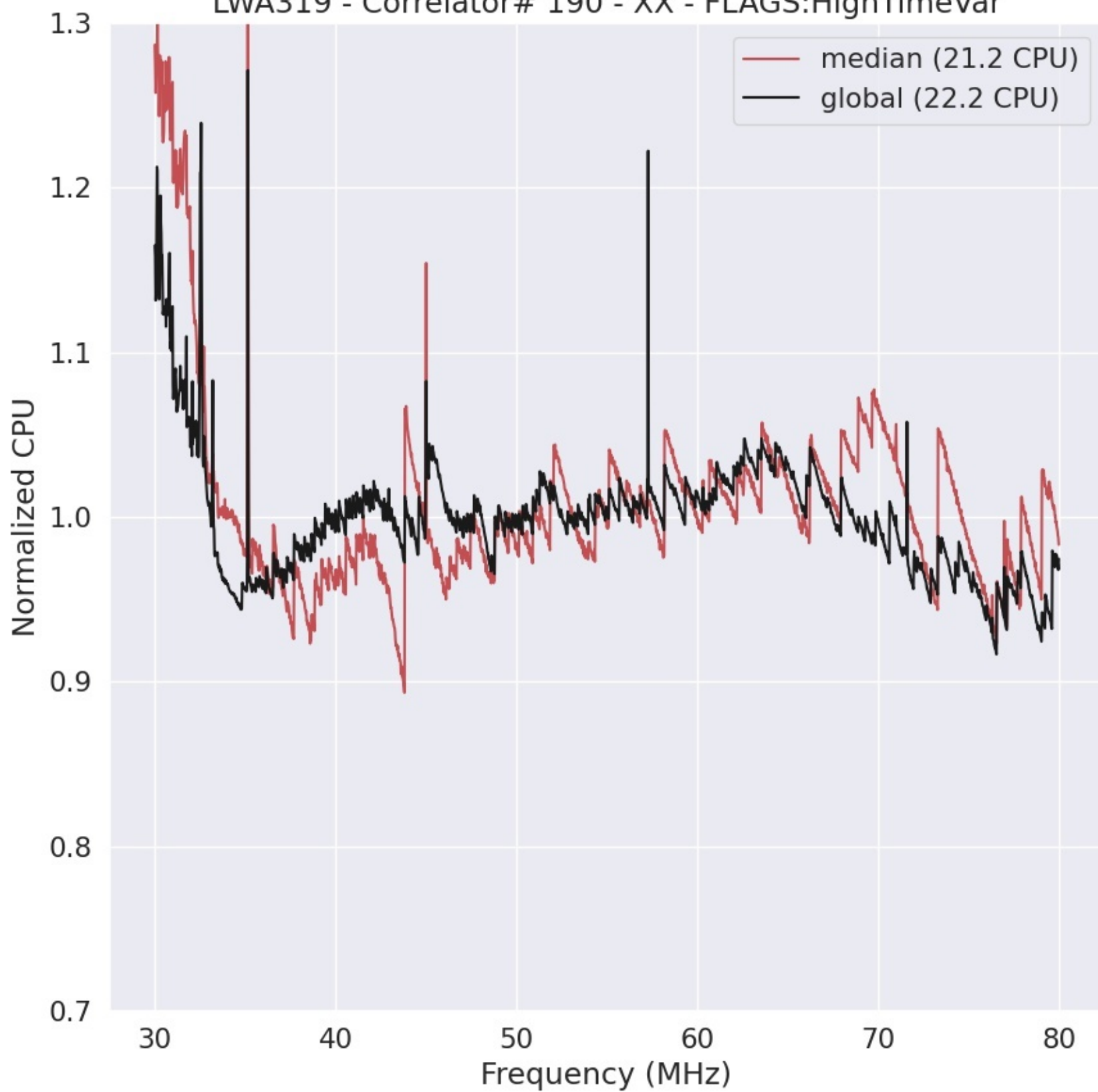
LWA319 - Correlator# 190 - XX - FLAGS:HighTimeVar
