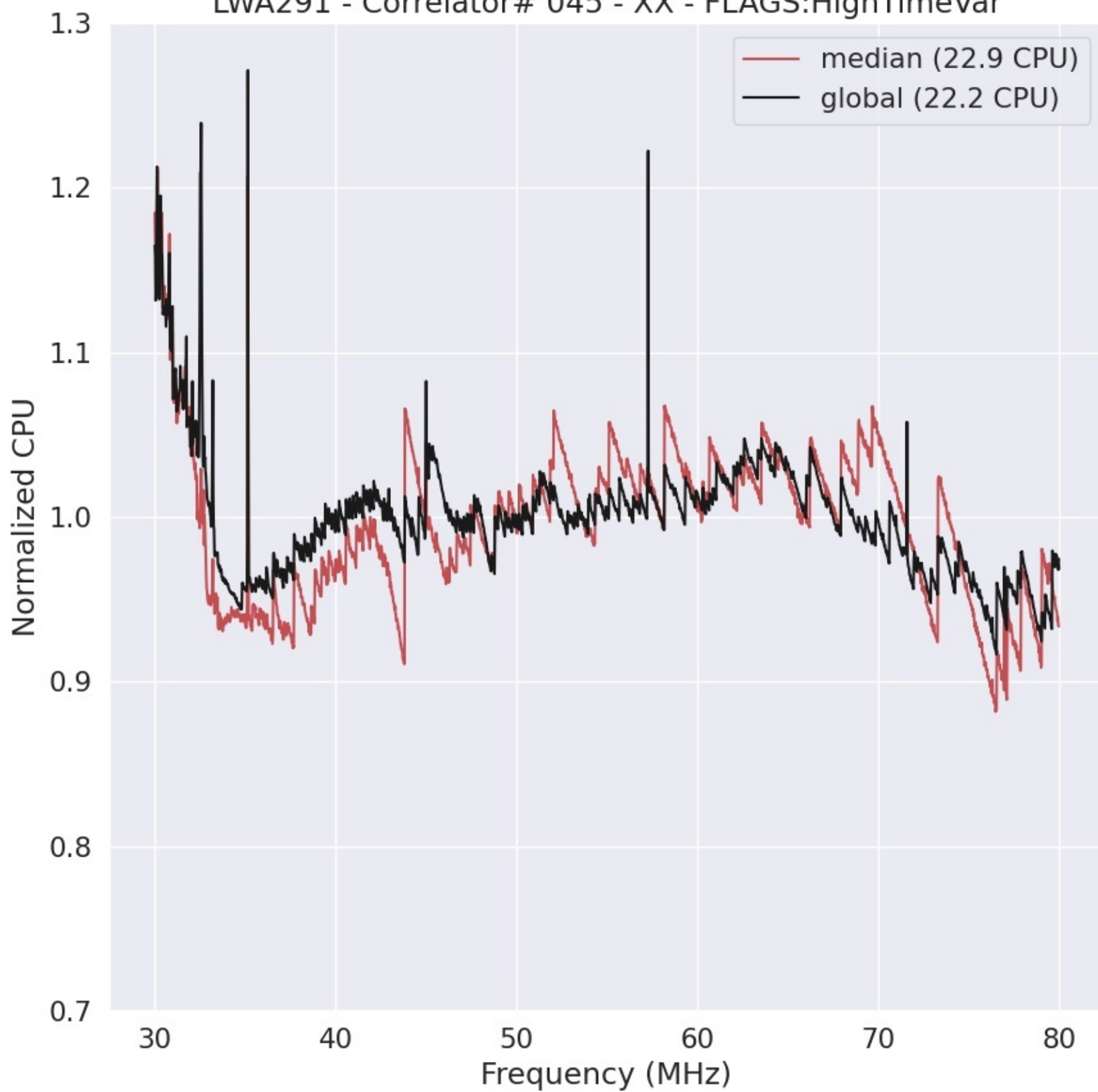
LWA291 - Correlator# 045 - XX - FLAGS:HighTimeVar
