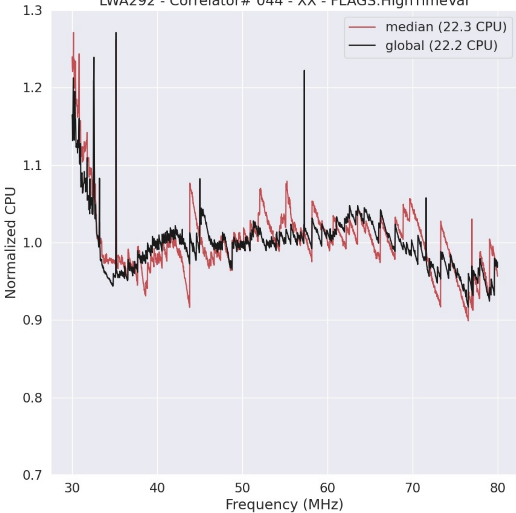
LWA292 - Correlator# 044 - XX - FLAGS:HighTimeVar
