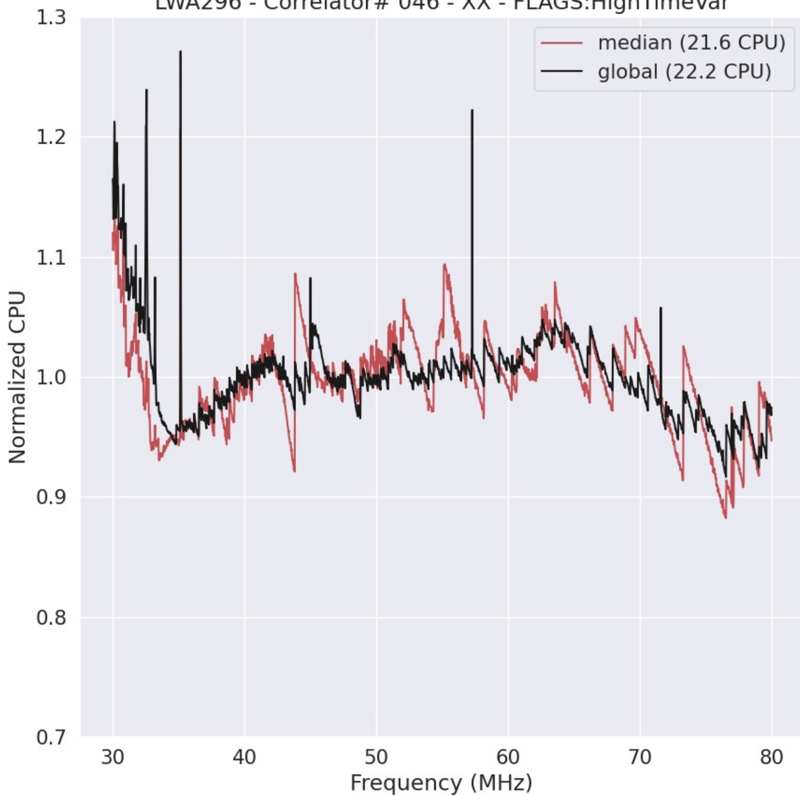
LWA296 - Correlator# 046 - XX - FLAGS:HighTimeVar
