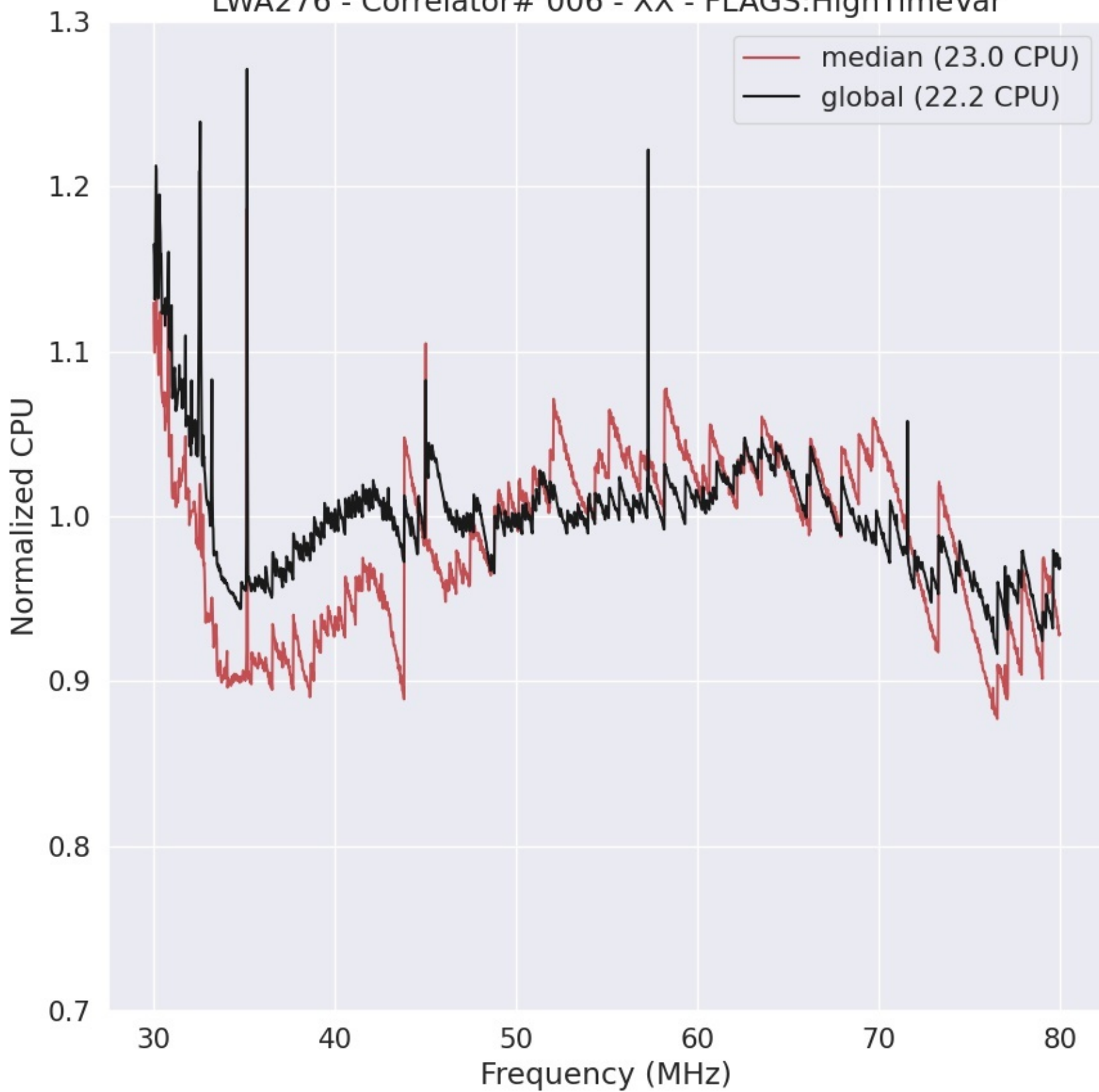
LWA276 - Correlator# 006 - XX - FLAGS:HighTimeVar
