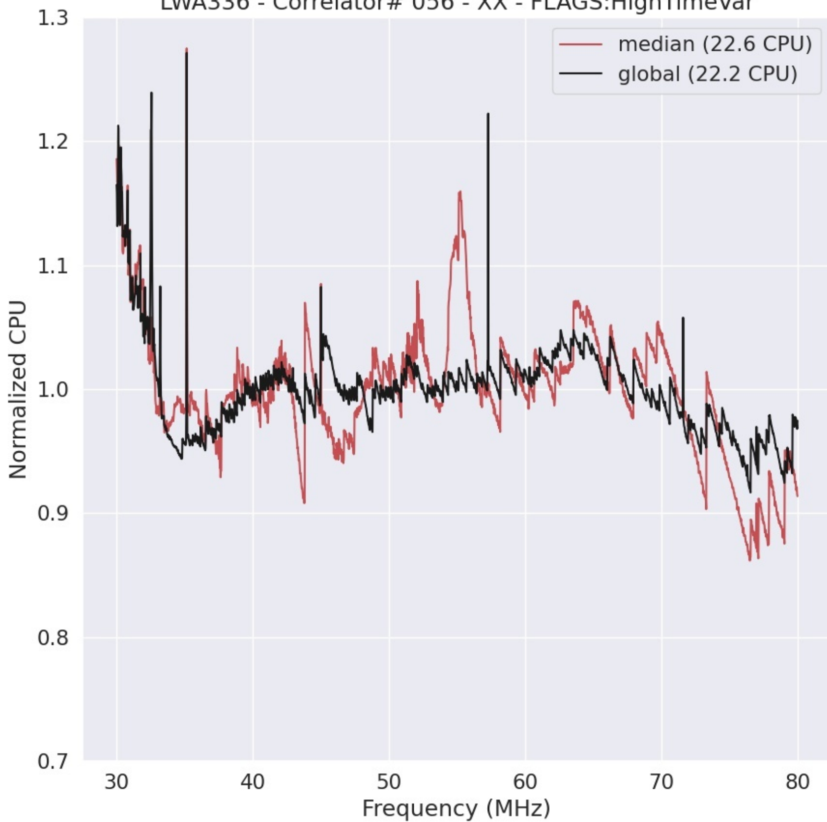
LWA336 - Correlator# 056 - XX - FLAGS:HighTimeVar
