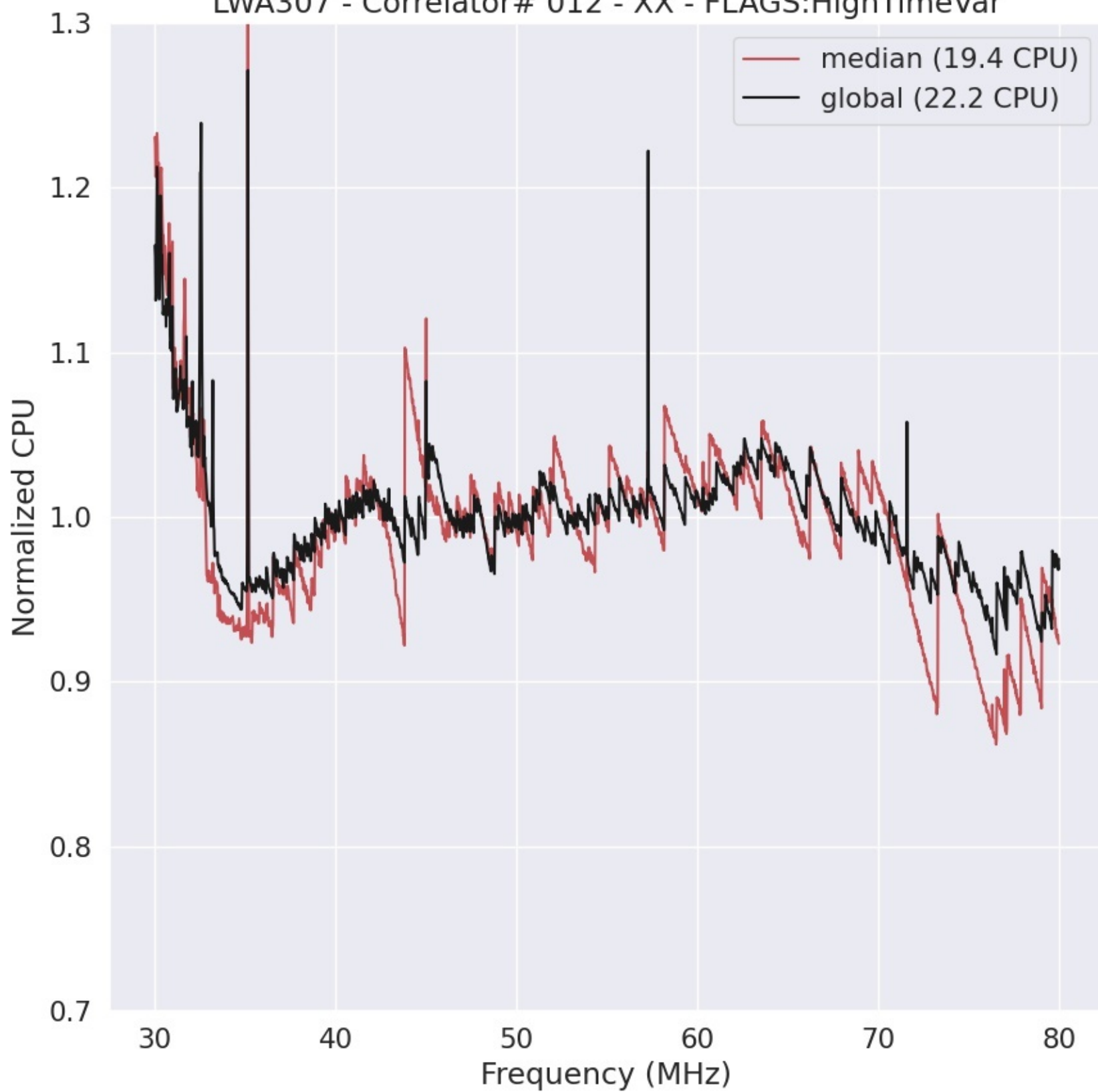
LWA307 - Correlator# 012 - XX - FLAGS:HighTimeVar
