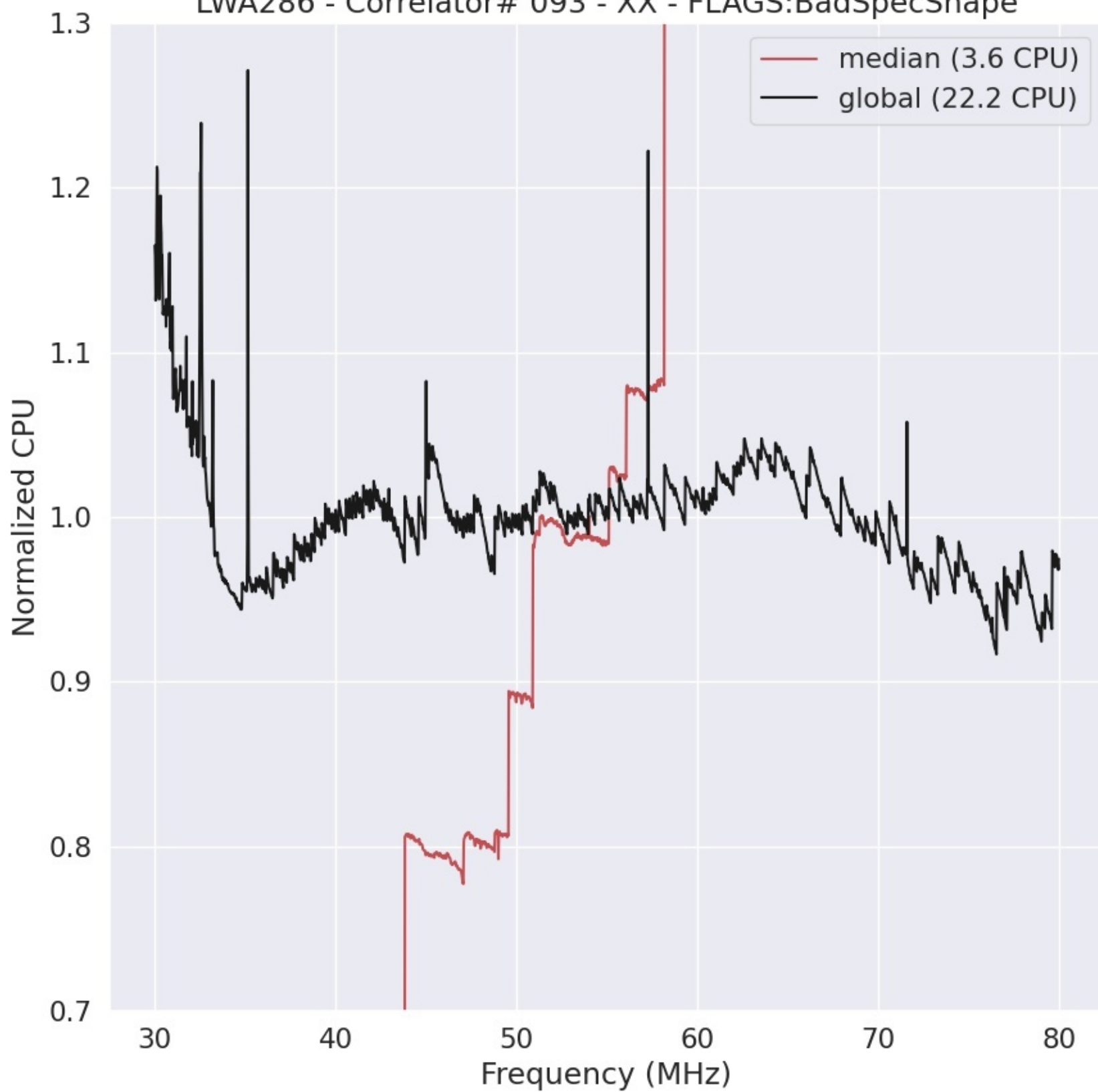
LWA286 - Correlator# 093 - XX - FLAGS:BadSpecShape
