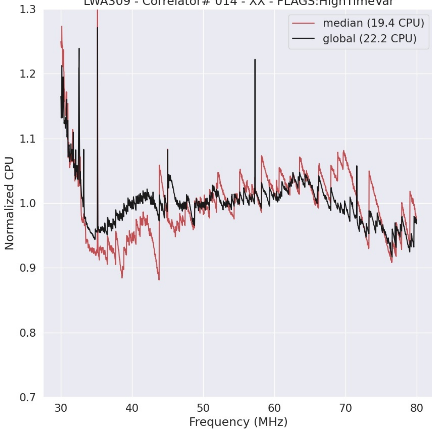
LWA309 - Correlator# 014 - XX - FLAGS:HighTimeVar
