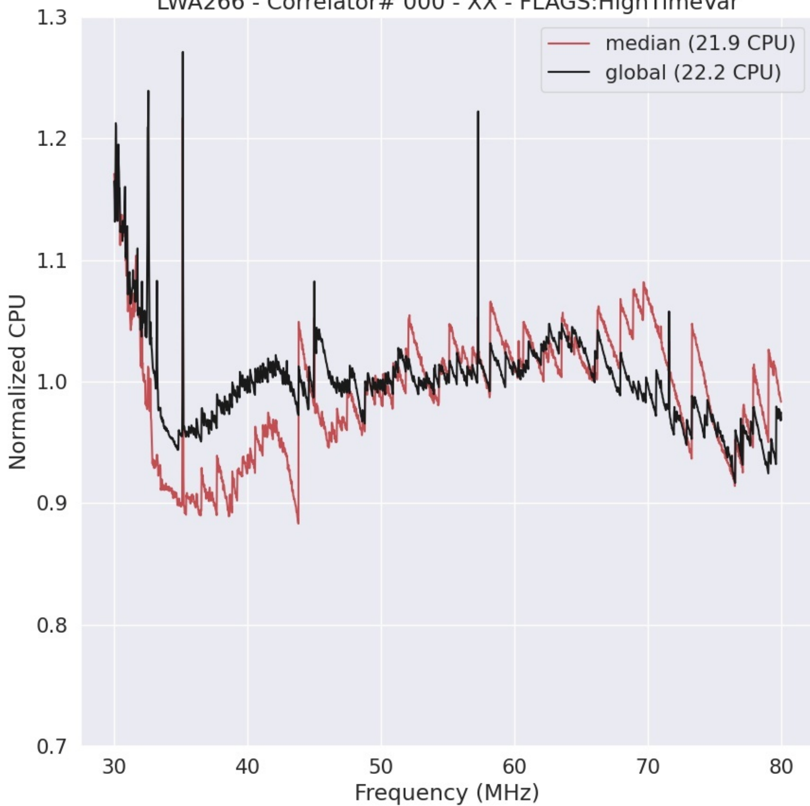
LWA266 - Correlator# 000 - XX - FLAGS:HighTimeVar
