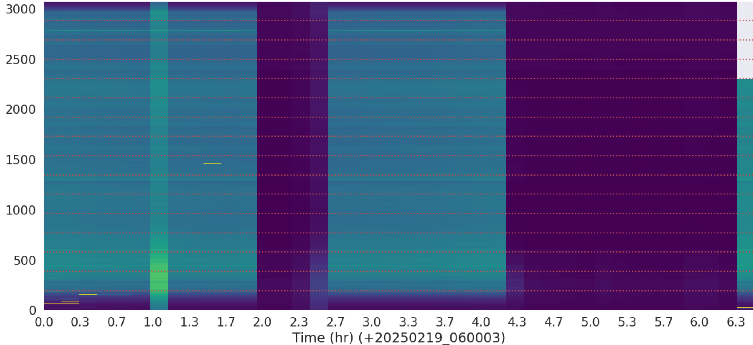
LWA124 - Correlator# 224 - YY - FLAGS: HighTimeVar
