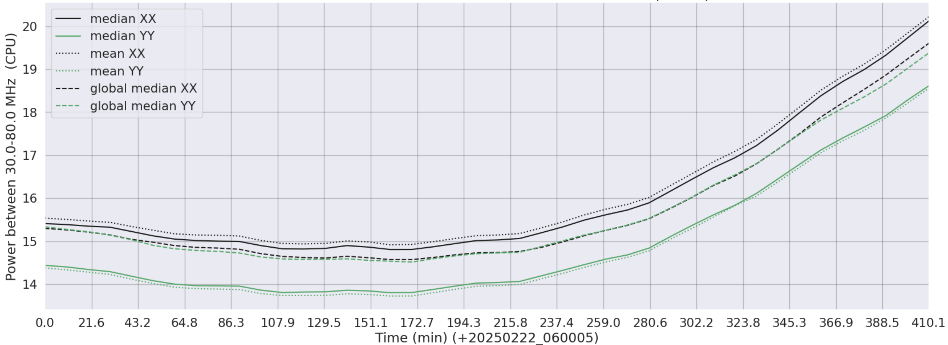
LWA240 - Correlator# 312 - XX FLAGS:Good - YY FLAGS:BadSpecShape
