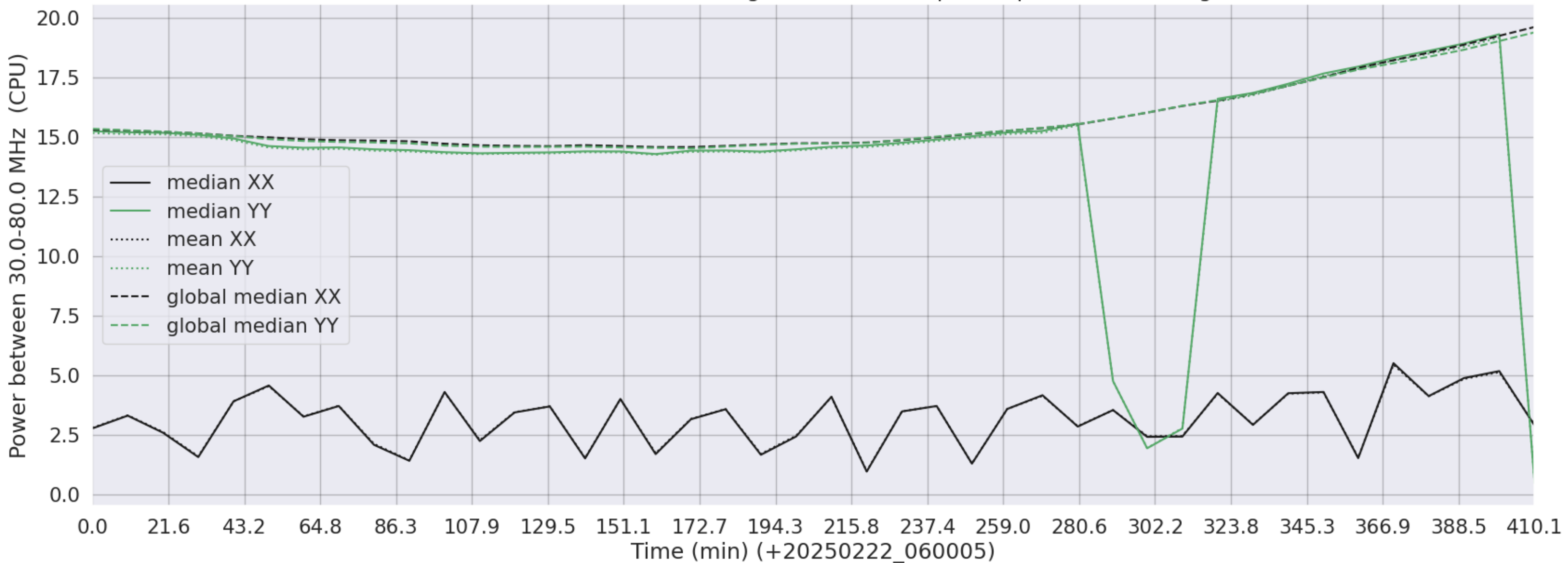
LWA124 - Correlator# 224 - XX FLAGS:HighTimeVar+BadSpecShape - YY FLAGS:HighTimeVar
