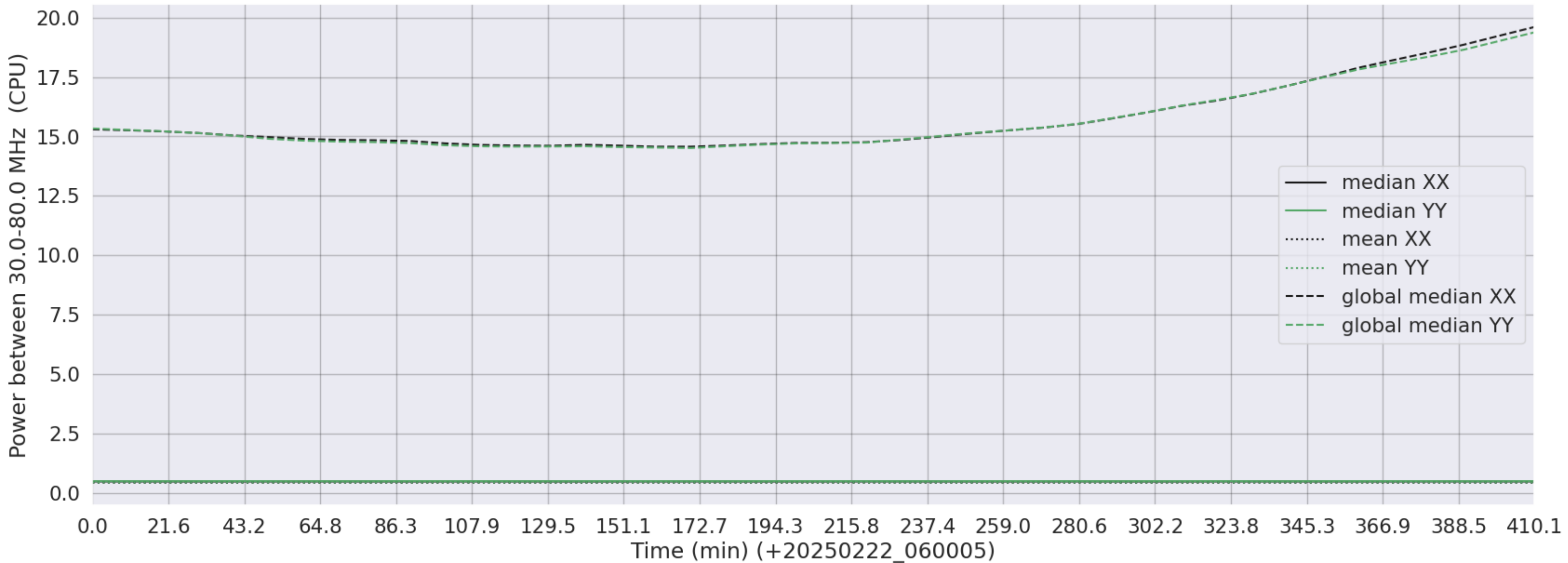
LWA127 - Correlator# 225 - XX FLAGS:LowPower - YY FLAGS:LowPower
