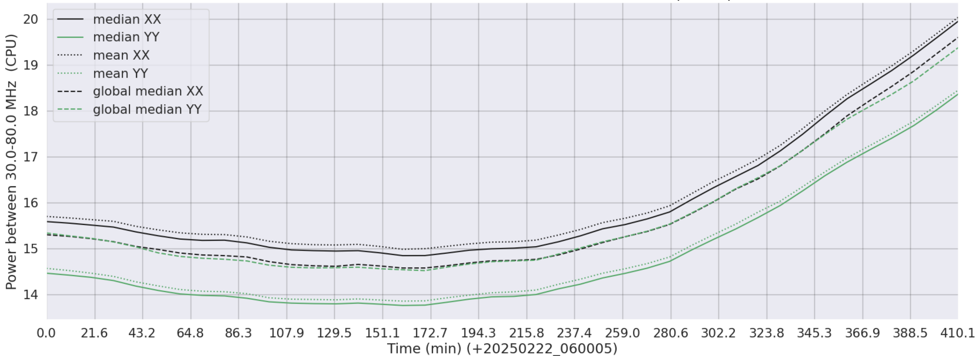
LWA014 - Correlator# 099 - XX FLAGS:Good - YY FLAGS:BadSpecShape
