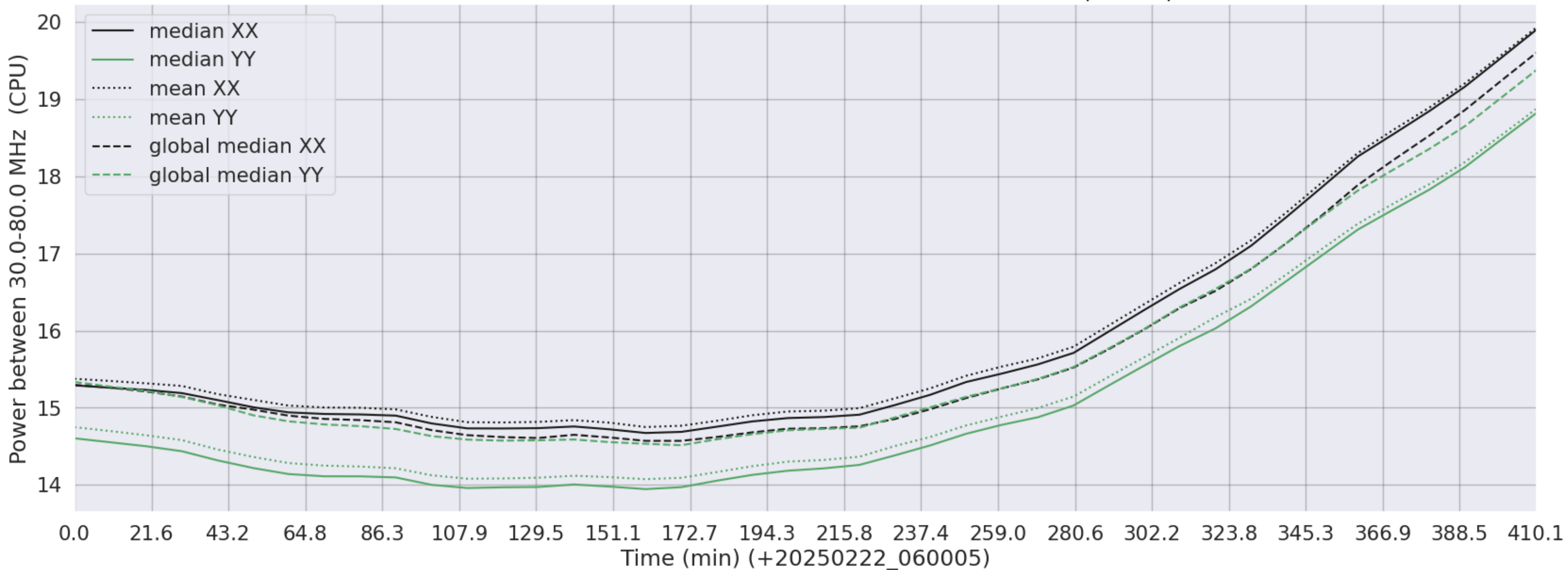
LWA167 - Correlator# 268 - XX FLAGS:Good - YY FLAGS:BadSpecShape
