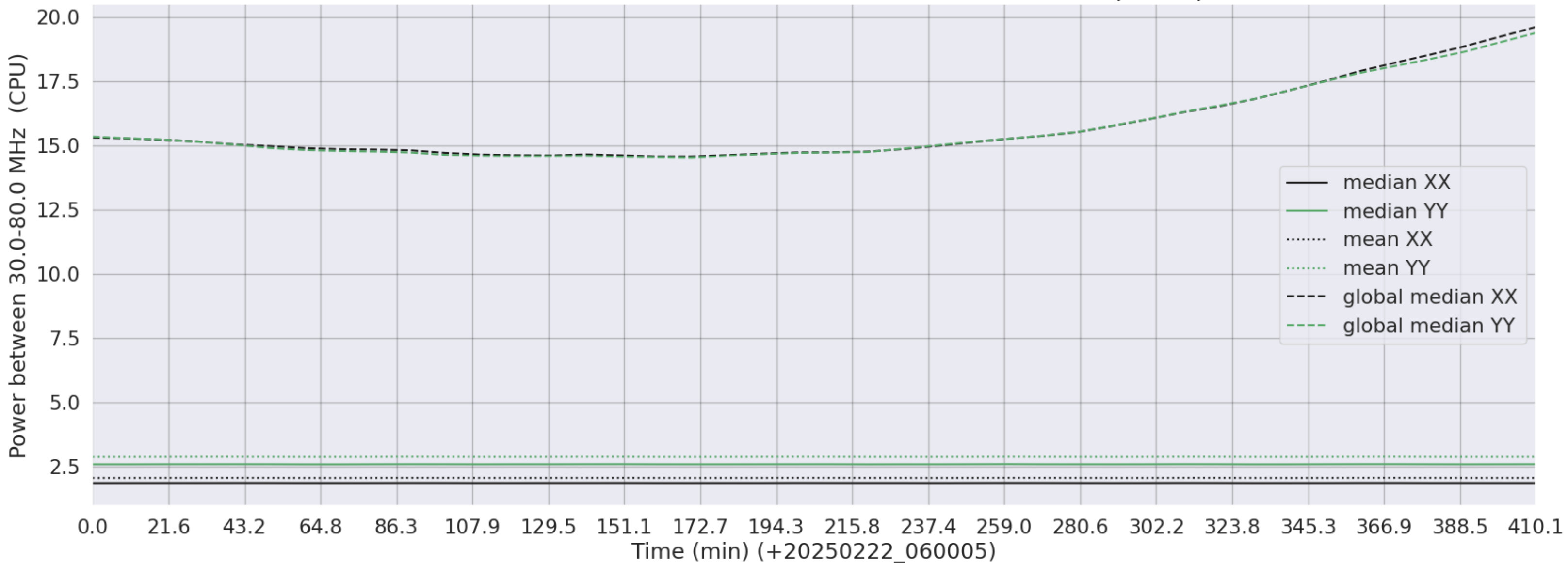
LWA297 - Correlator# 314 - XX FLAGS:LowPower - YY FLAGS:BadSpecShape
