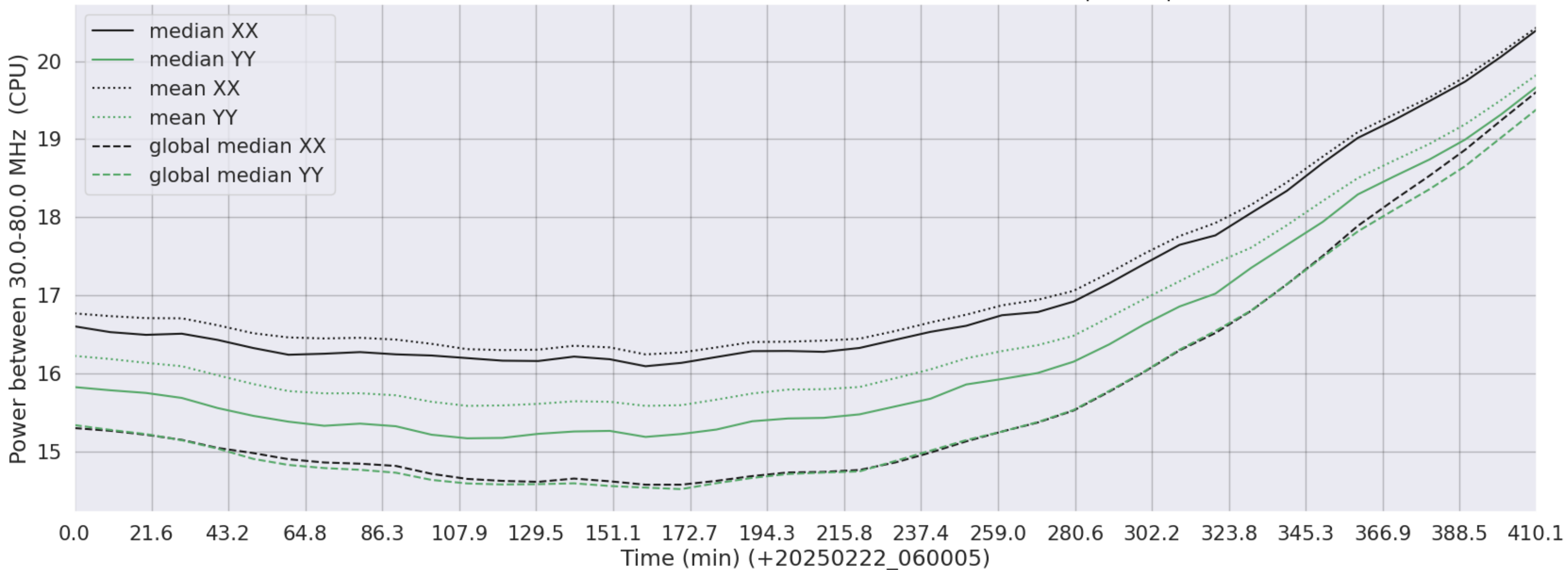
LWA129 - Correlator# 180 - XX FLAGS:Good - YY FLAGS:BadSpecShape
