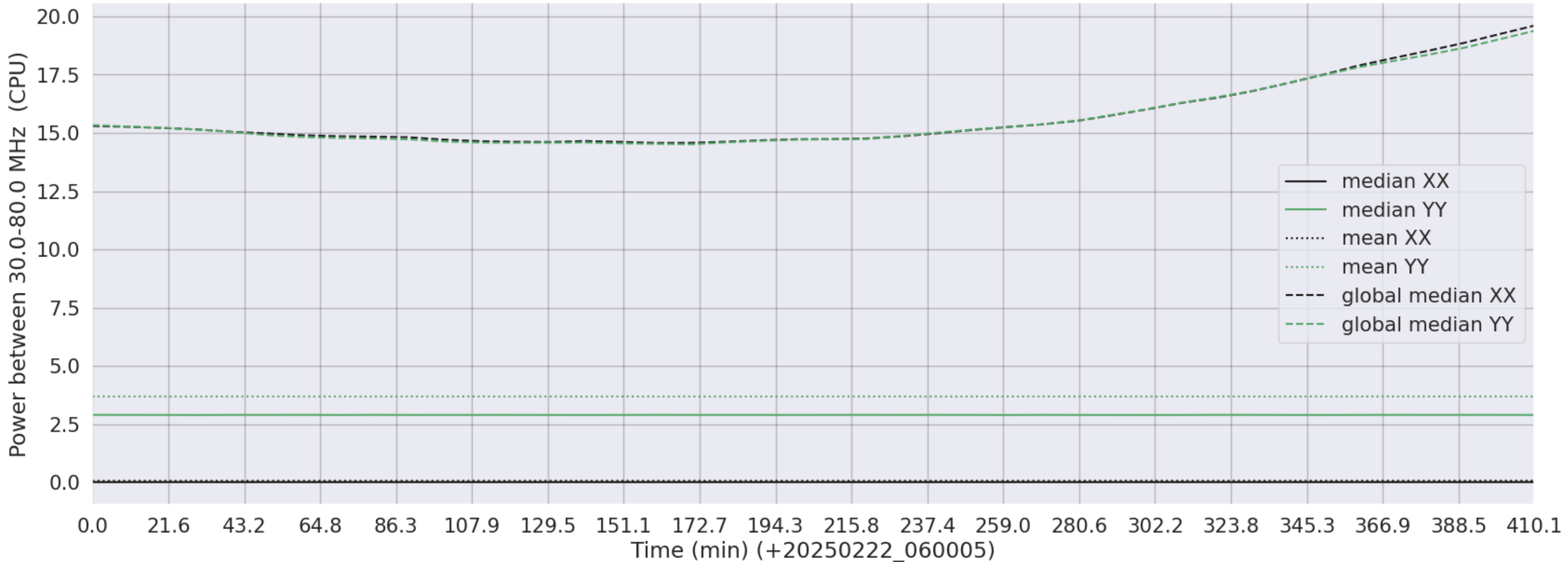
LWA209 - Correlator# 301 - XX FLAGS:LowPower - YY FLAGS:BadSpecShape
