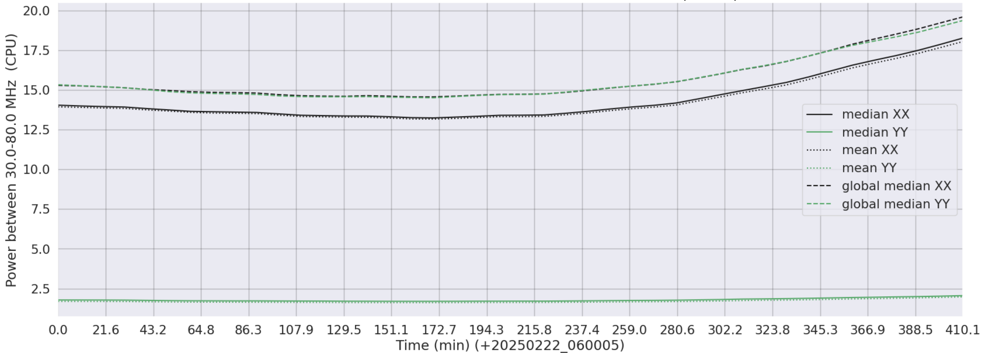
LWA186 - Correlator# 243 - XX FLAGS:Good - YY FLAGS:BadSpecShape
