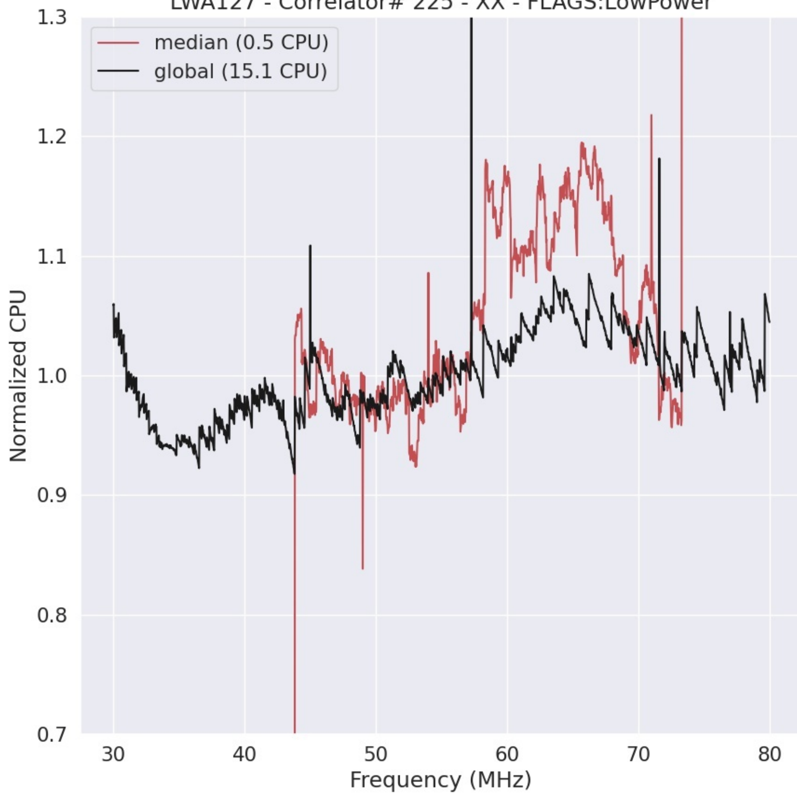
LWA127 - Correlator# 225 - XX - FLAGS:LowPower
