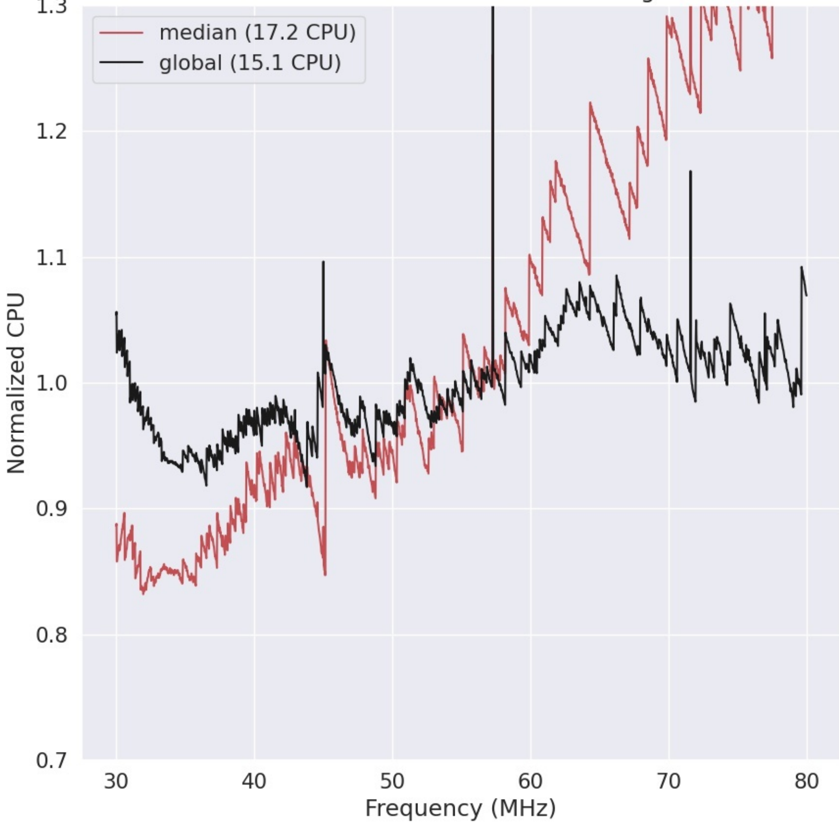
LWA131 - Correlator# 182 - XX - FLAGS:HighTimeVar
