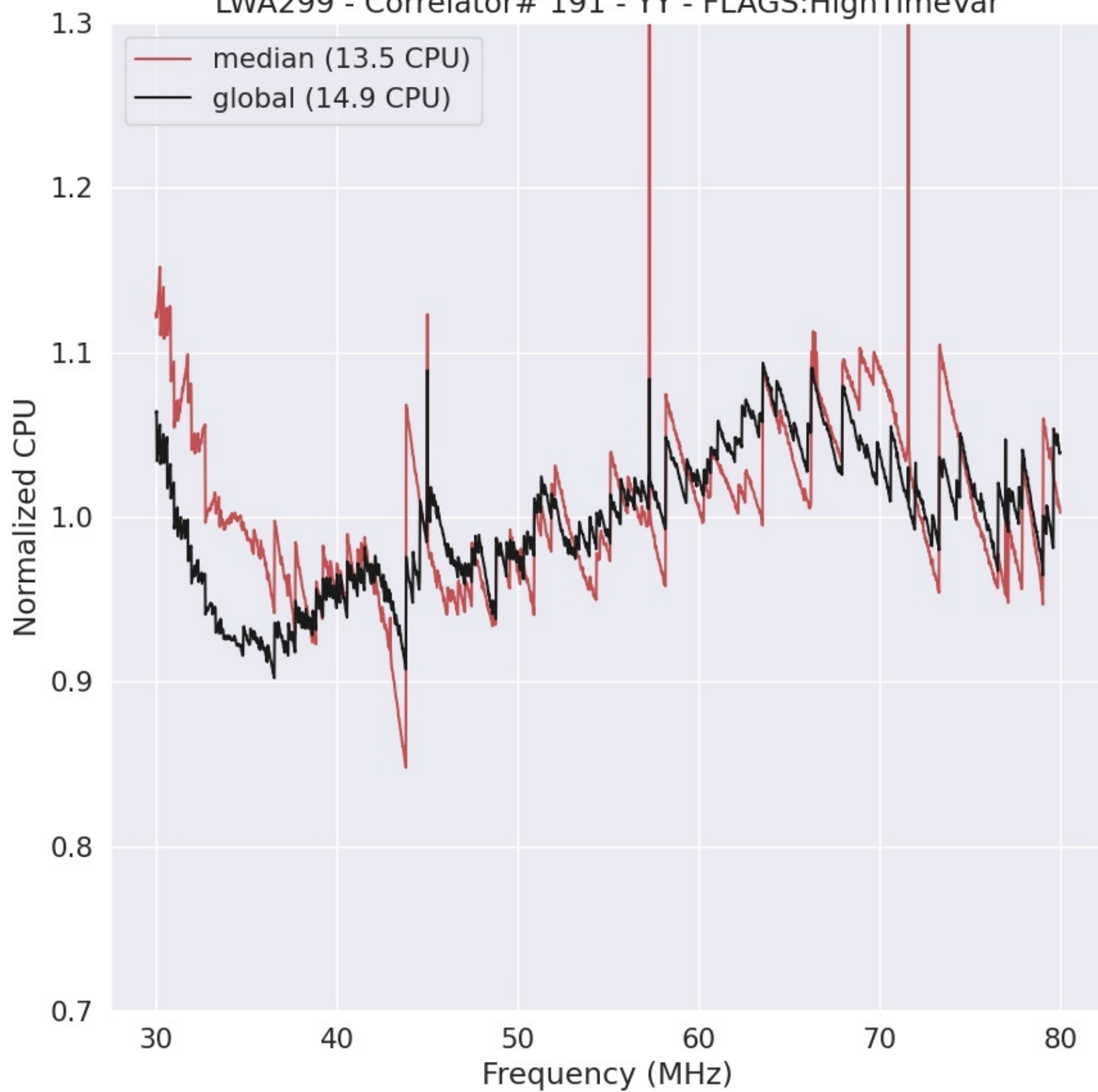
LWA299 - Correlator# 191 - YY - FLAGS:HighTimeVar
