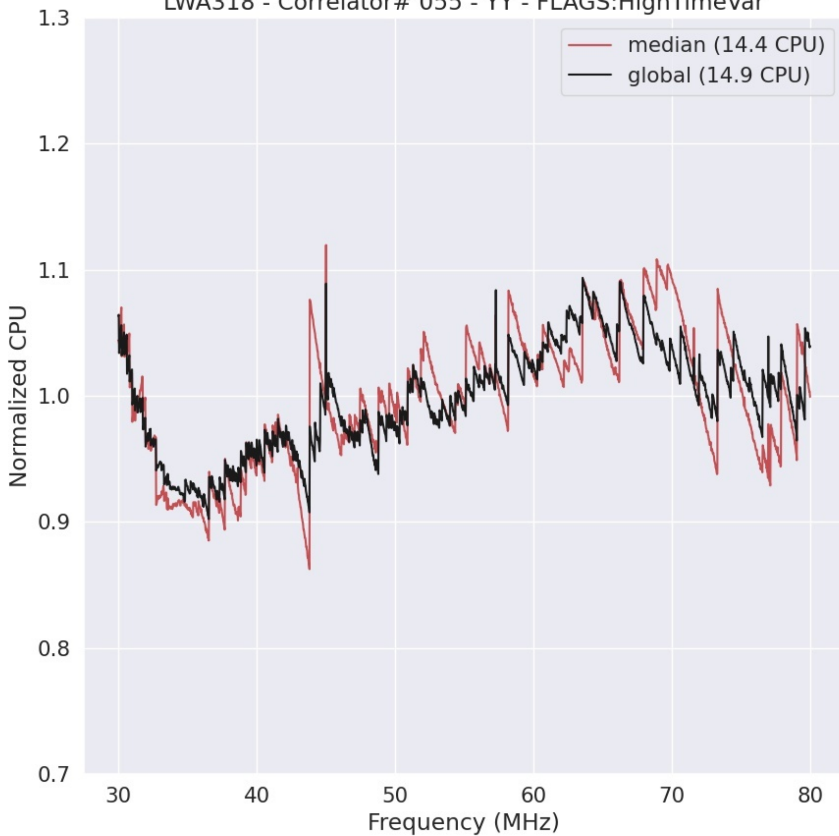
LWA318 - Correlator# 055 - YY - FLAGS:HighTimeVar
