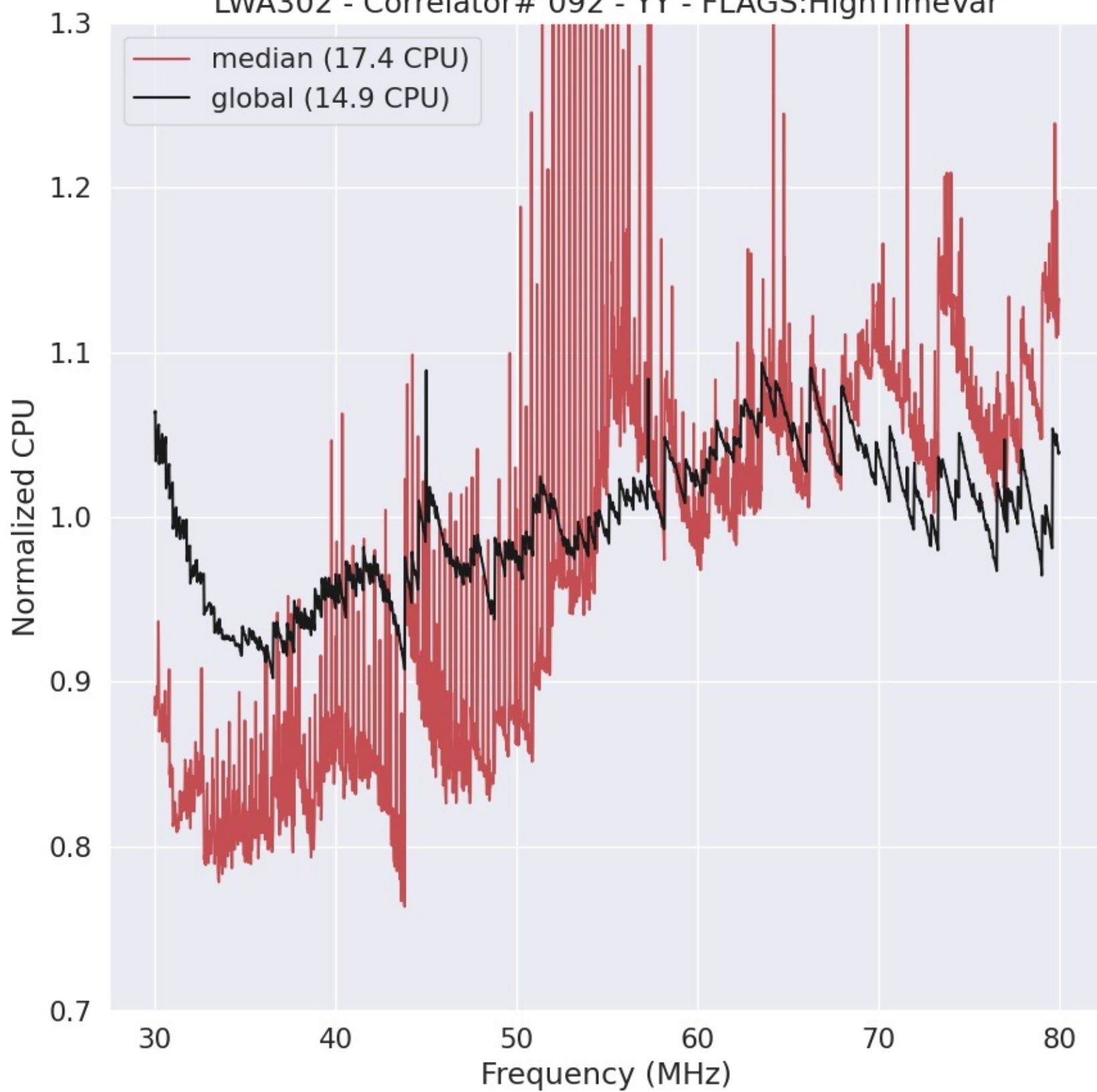
LWA302 - Correlator# 092 - YY - FLAGS:HighTimeVar
