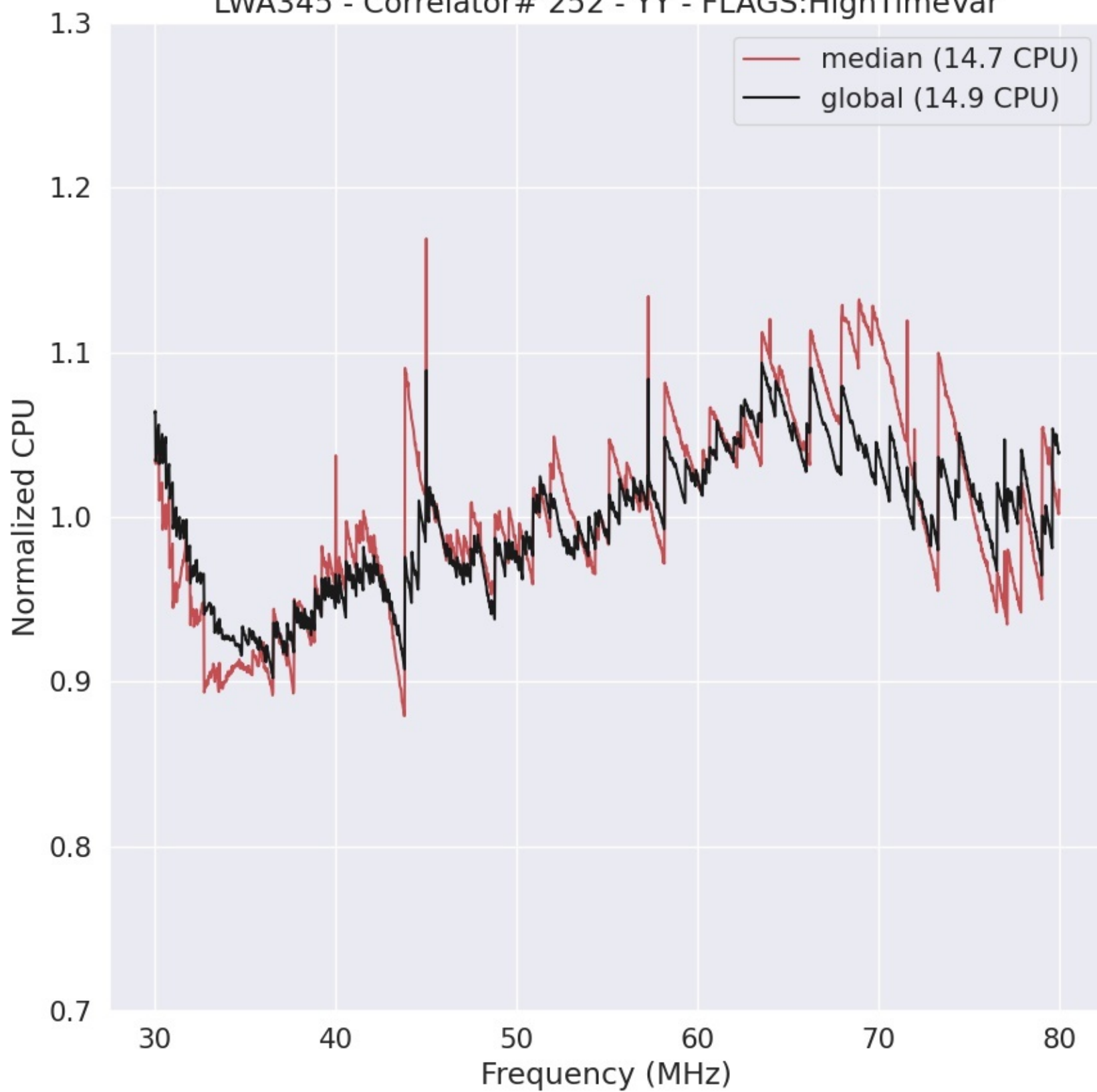
LWA345 - Correlator# 252 - YY - FLAGS:HighTimeVar
