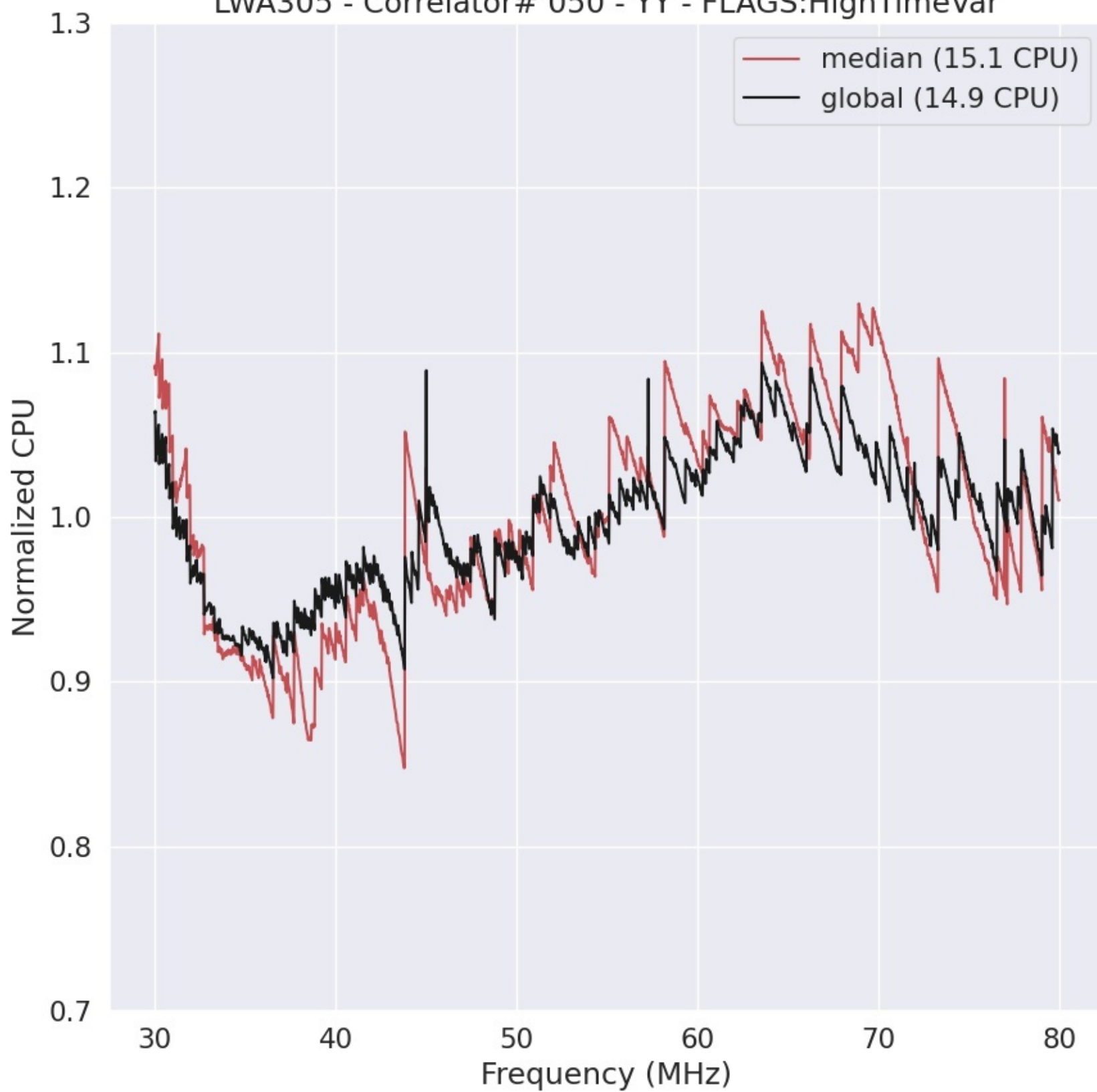
LWA305 - Correlator# 050 - YY - FLAGS:HighTimeVar
