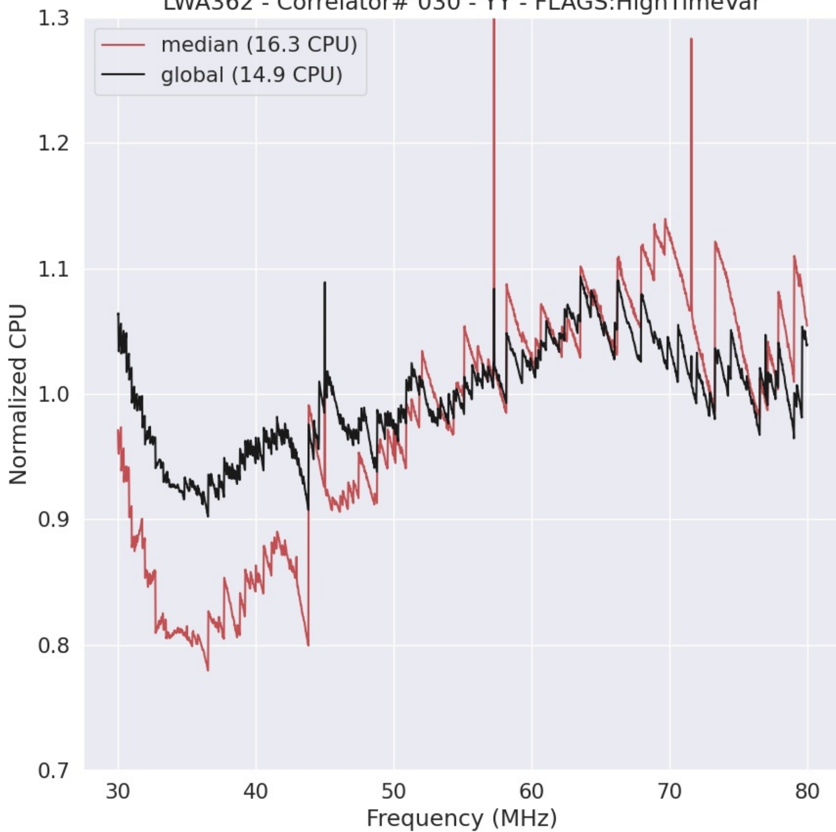
LWA362 - Correlator# 030 - YY - FLAGS:HighTimeVar
