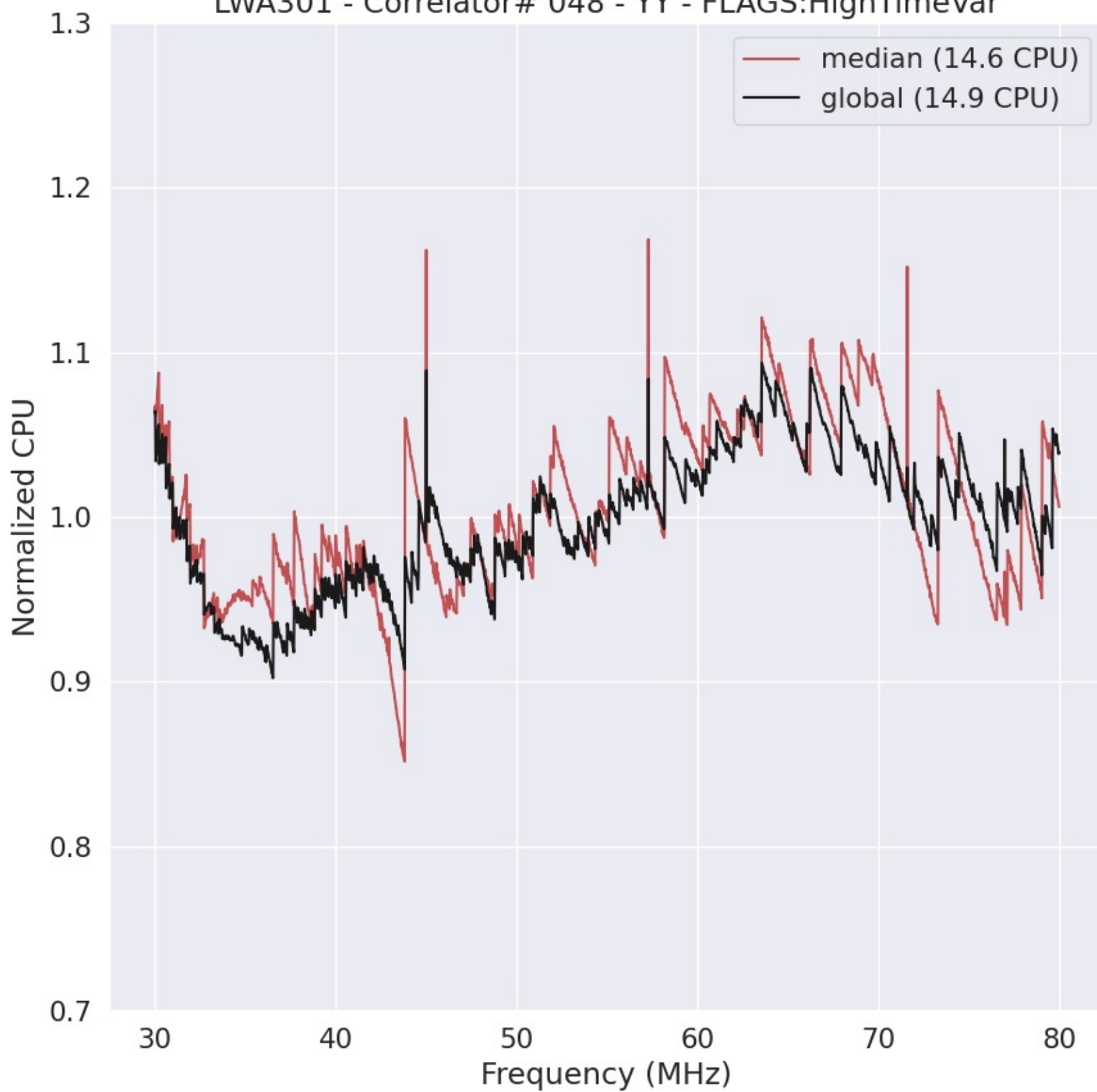
LWA301 - Correlator# 048 - YY - FLAGS:HighTimeVar
