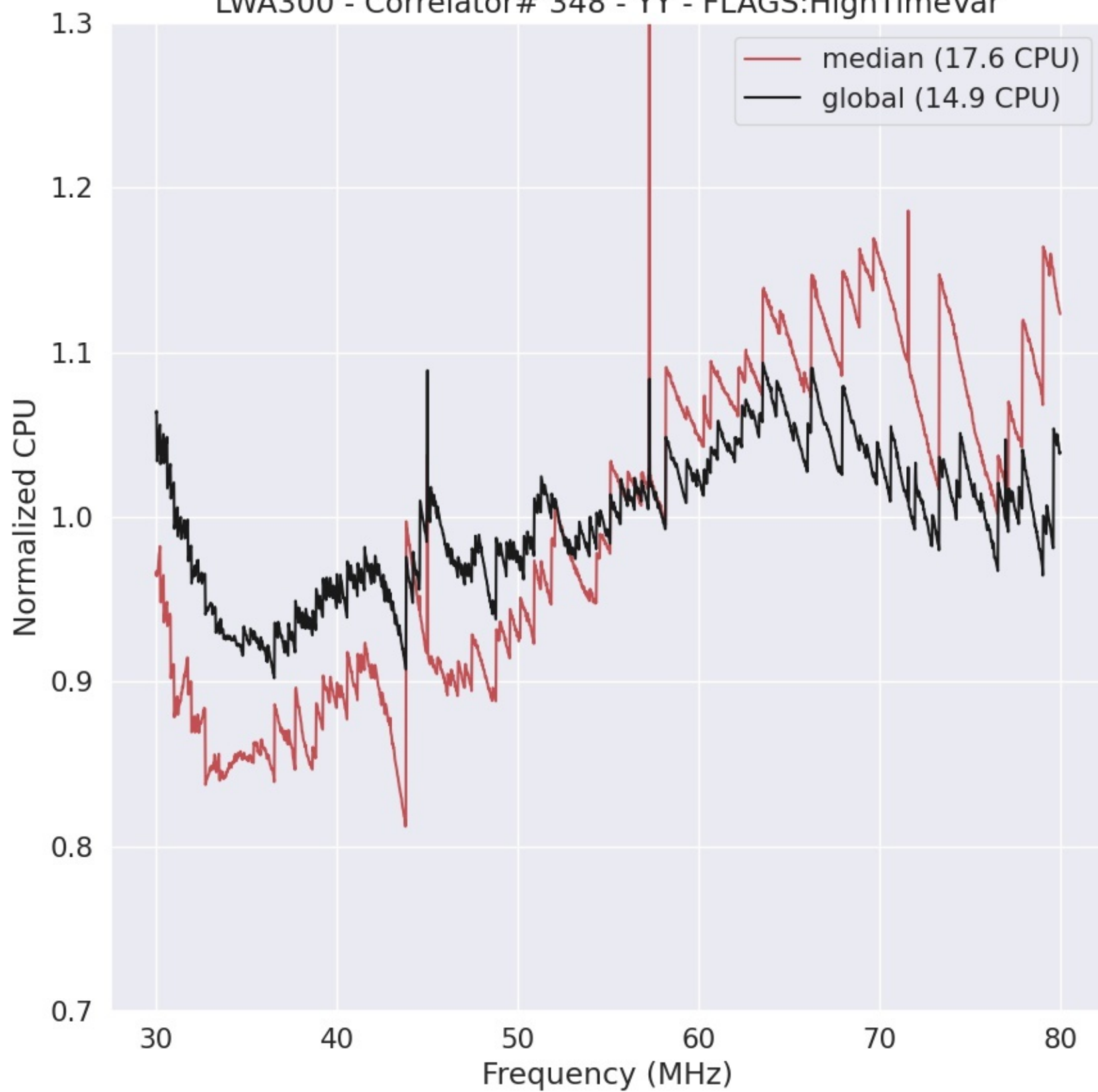
LWA300 - Correlator# 348 - YY - FLAGS:HighTimeVar
