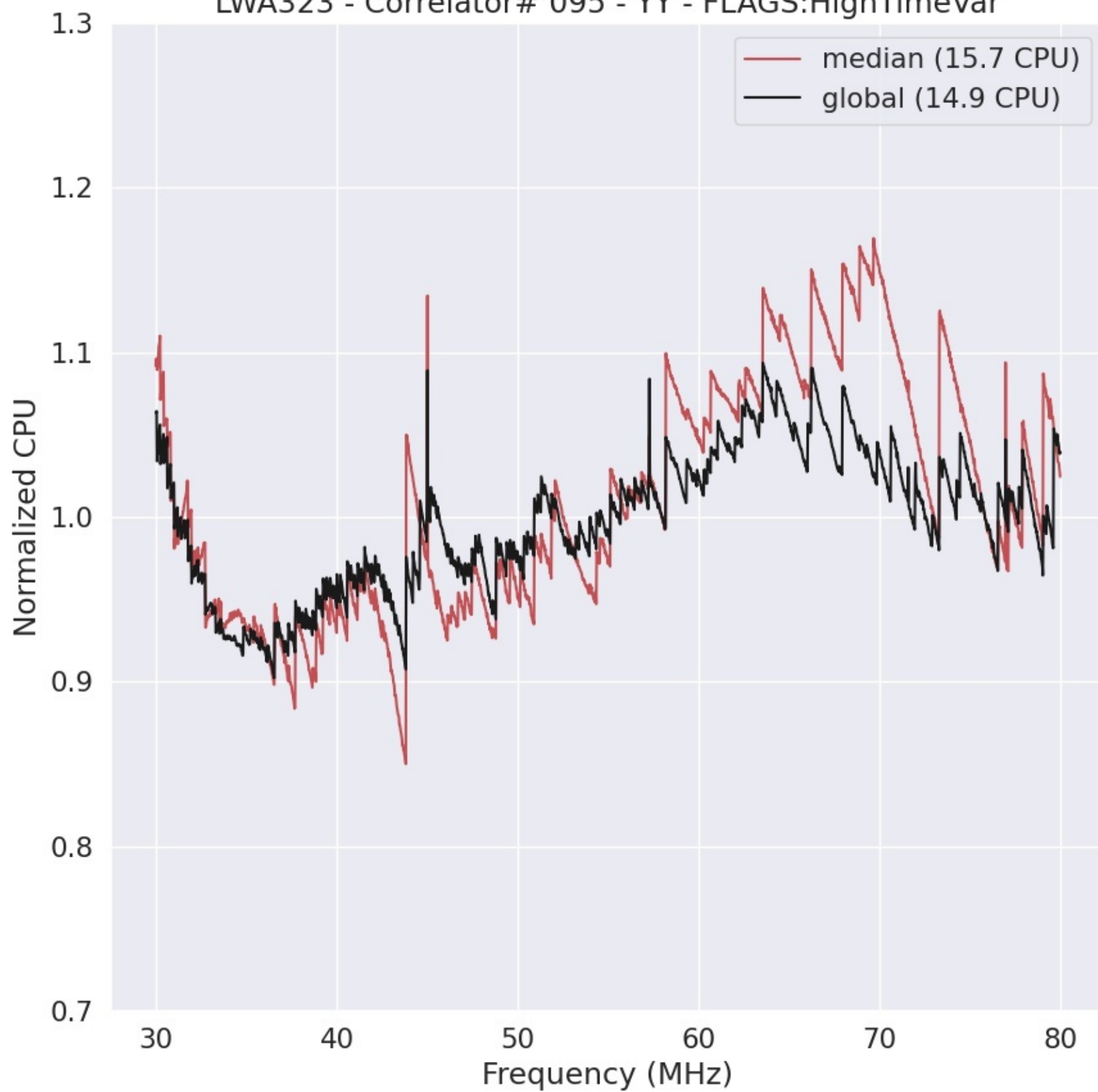
LWA323 - Correlator# 095 - YY - FLAGS:HighTimeVar
