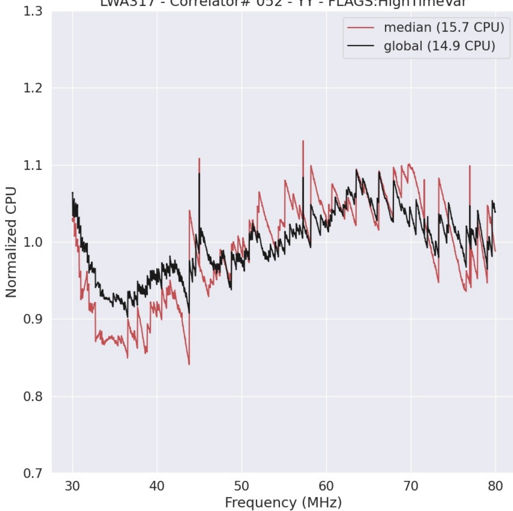
LWA317 - Correlator# 052 - YY - FLAGS:HighTimeVar
