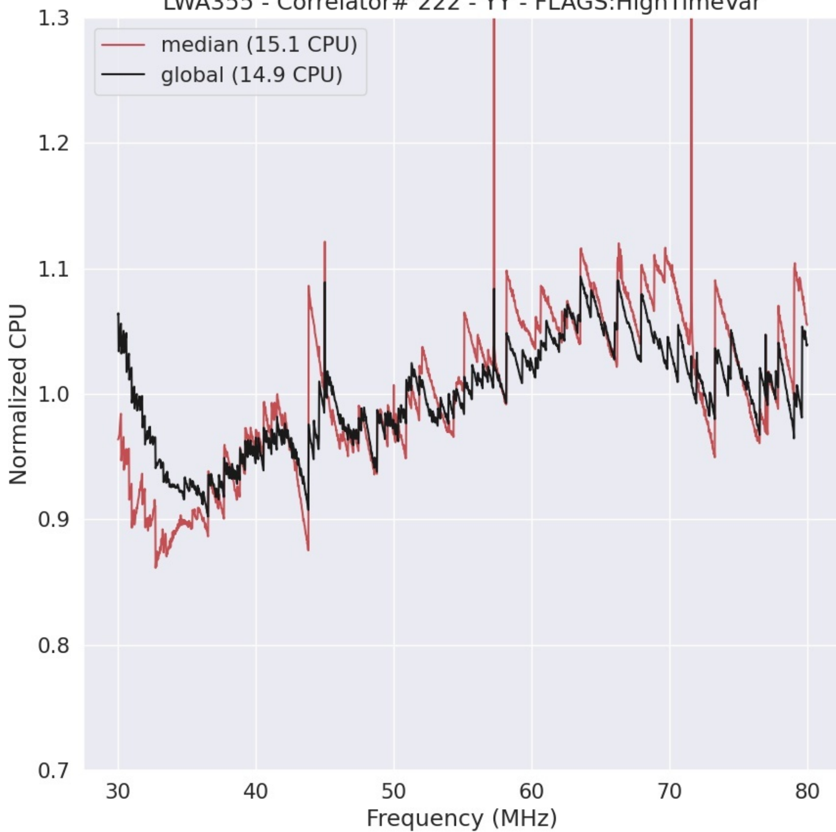
LWA355 - Correlator# 222 - YY - FLAGS:HighTimeVar
