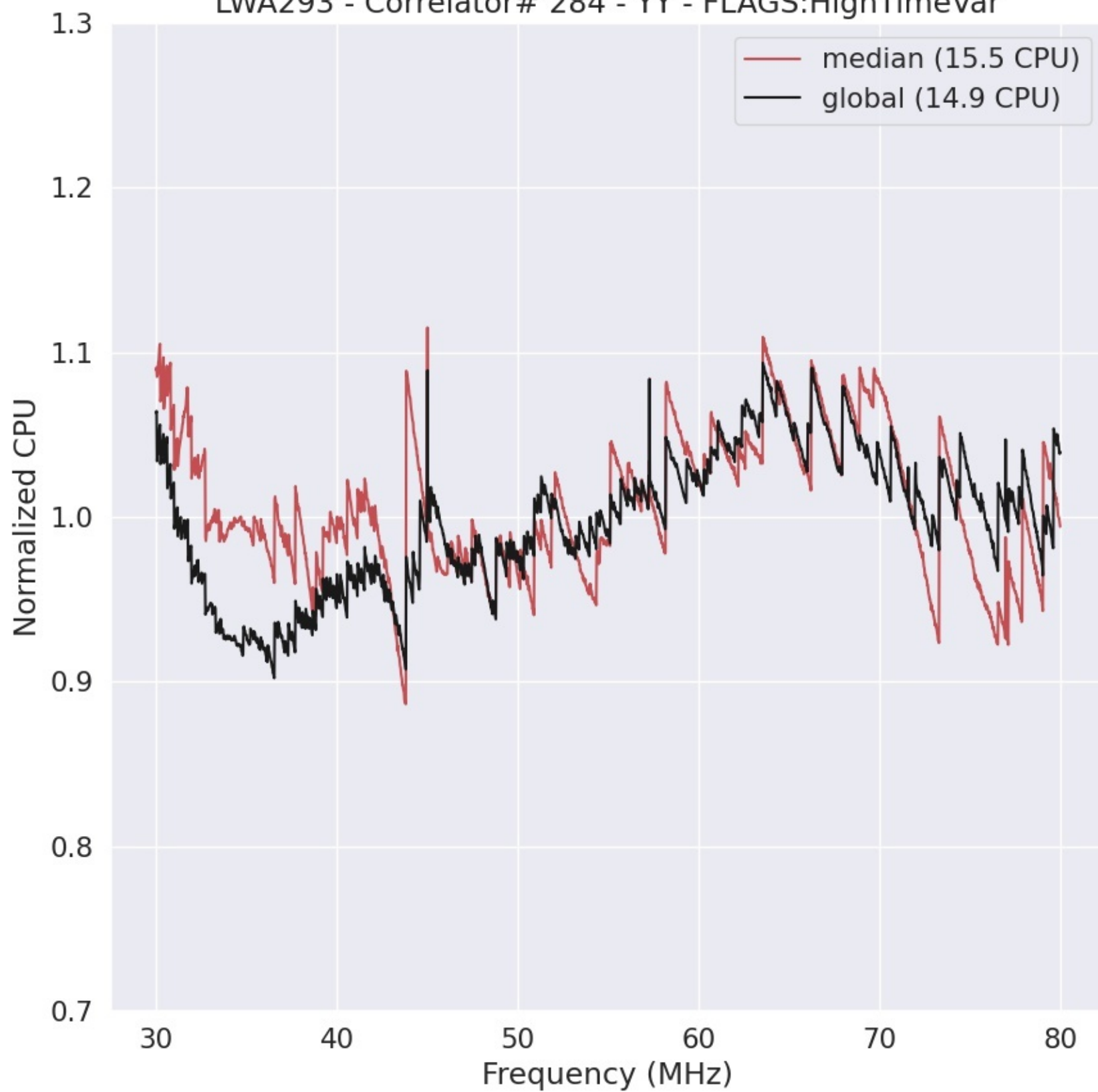
LWA293 - Correlator# 284 - YY - FLAGS:HighTimeVar
