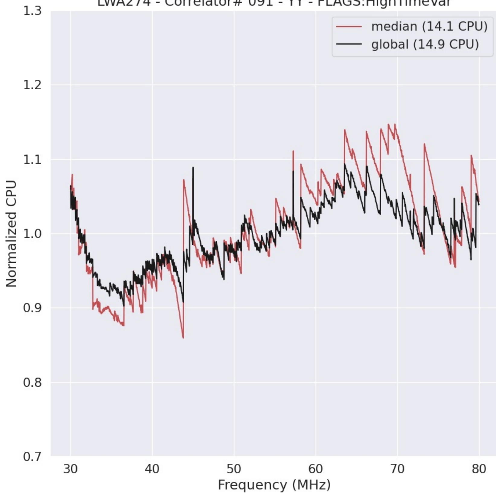
LWA274 - Correlator# 091 - YY - FLAGS:HighTimeVar
