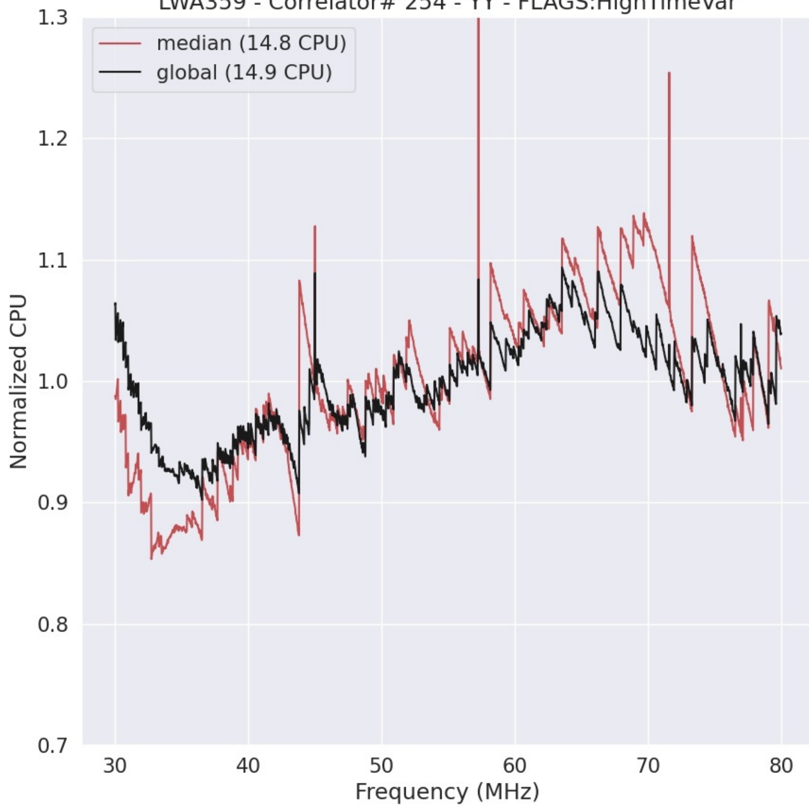
LWA359 - Correlator# 254 - YY - FLAGS:HighTimeVar
