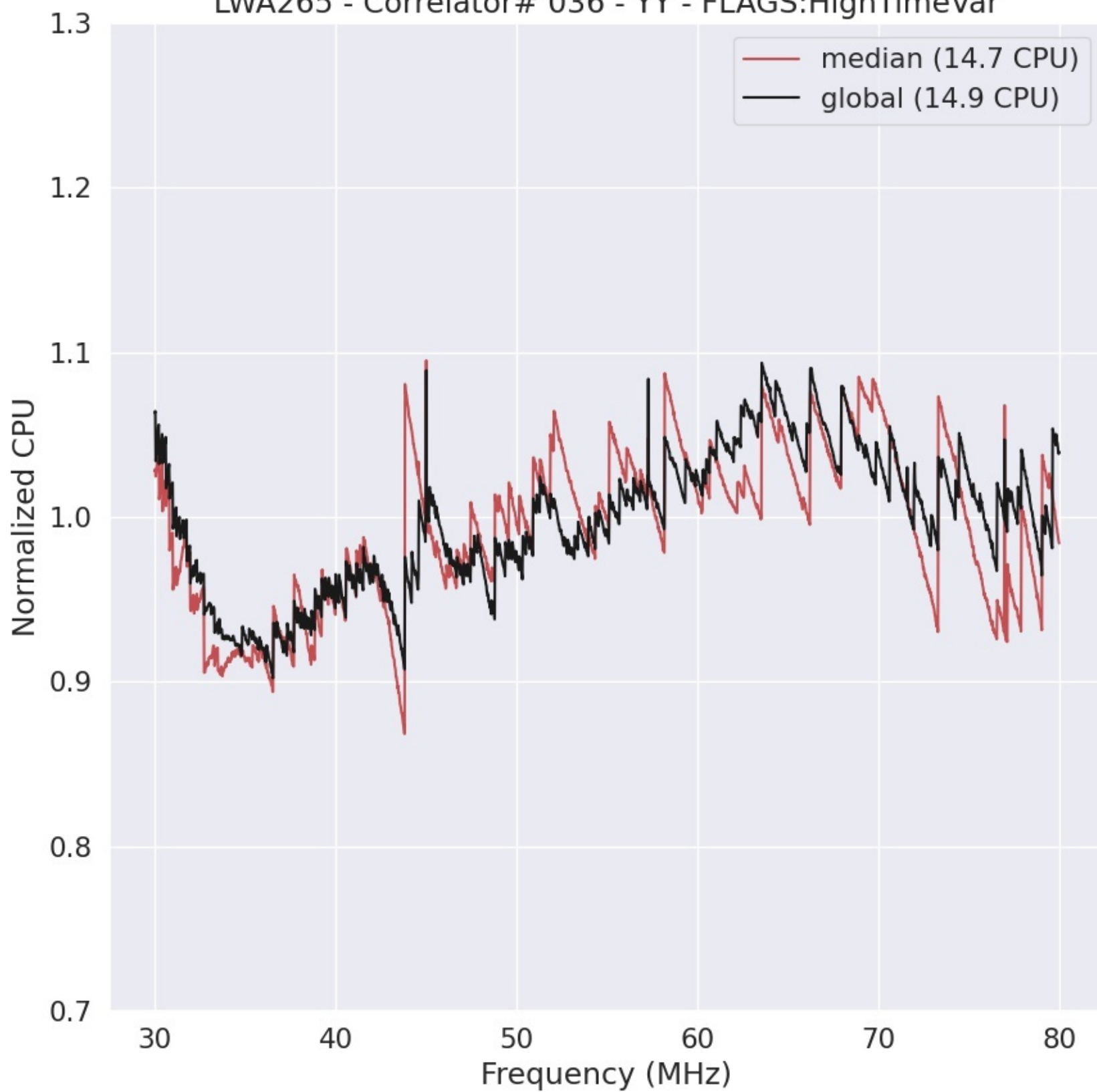
LWA265 - Correlator# 036 - YY - FLAGS:HighTimeVar
