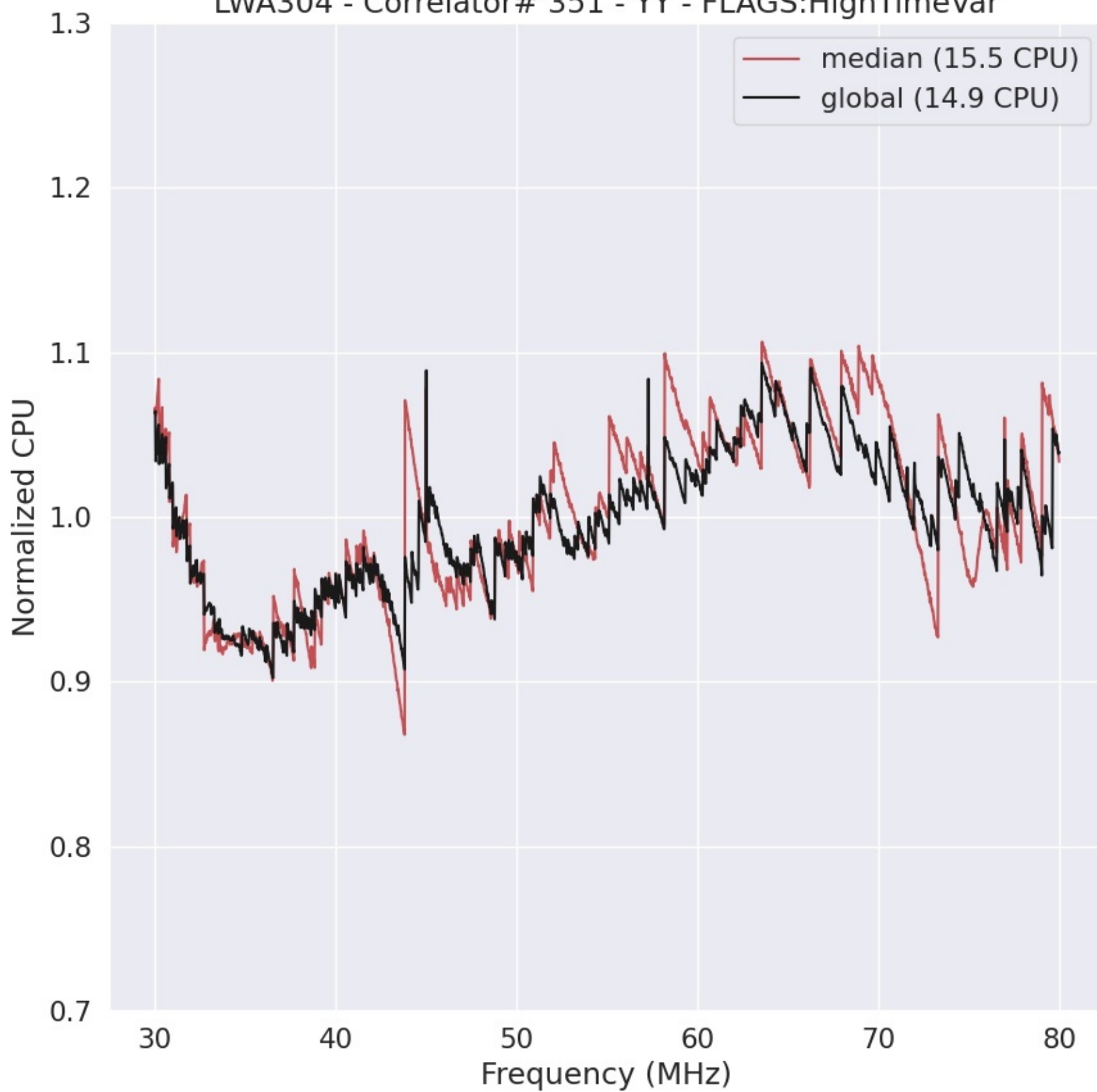
LWA304 - Correlator# 351 - YY - FLAGS:HighTimeVar
