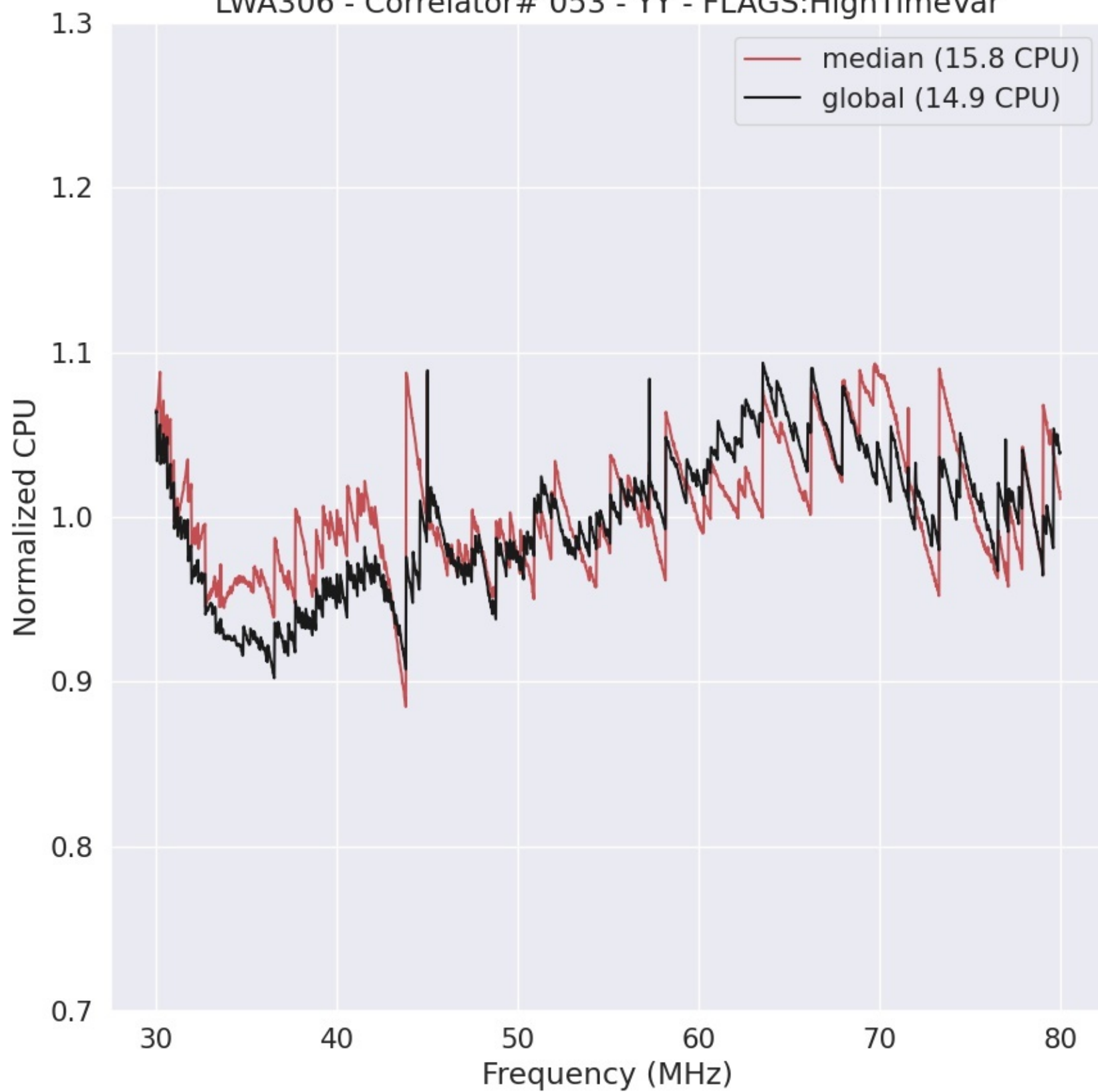
LWA306 - Correlator# 053 - YY - FLAGS:HighTimeVar
