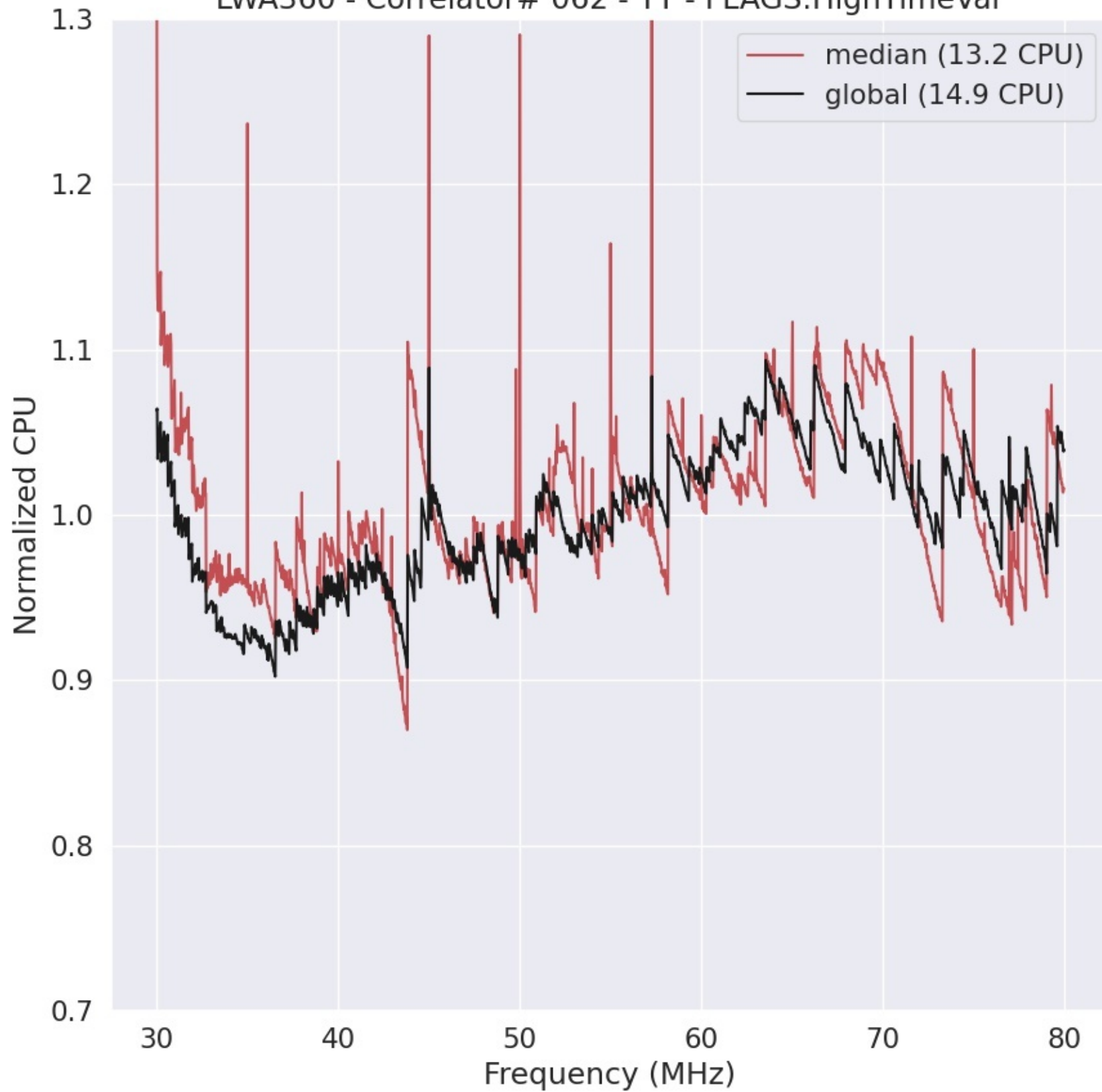
LWA360 - Correlator# 062 - YY - FLAGS:HighTimeVar
