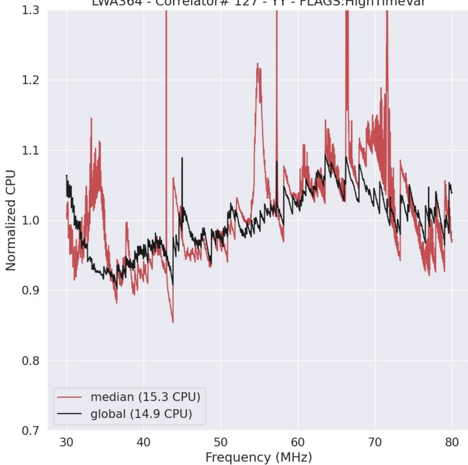
LWA364 - Correlator# 127 - YY - FLAGS:HighTimeVar
