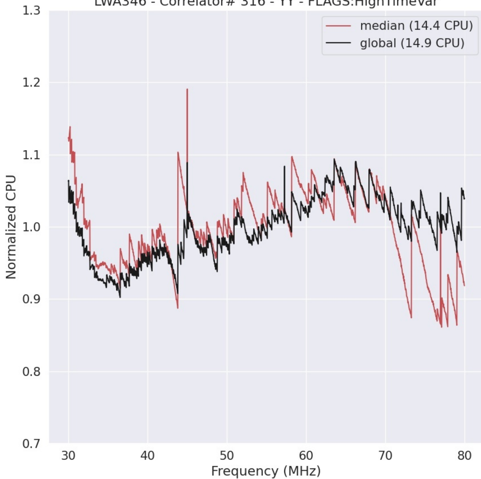
LWA346 - Correlator# 316 - YY - FLAGS:HighTimeVar
