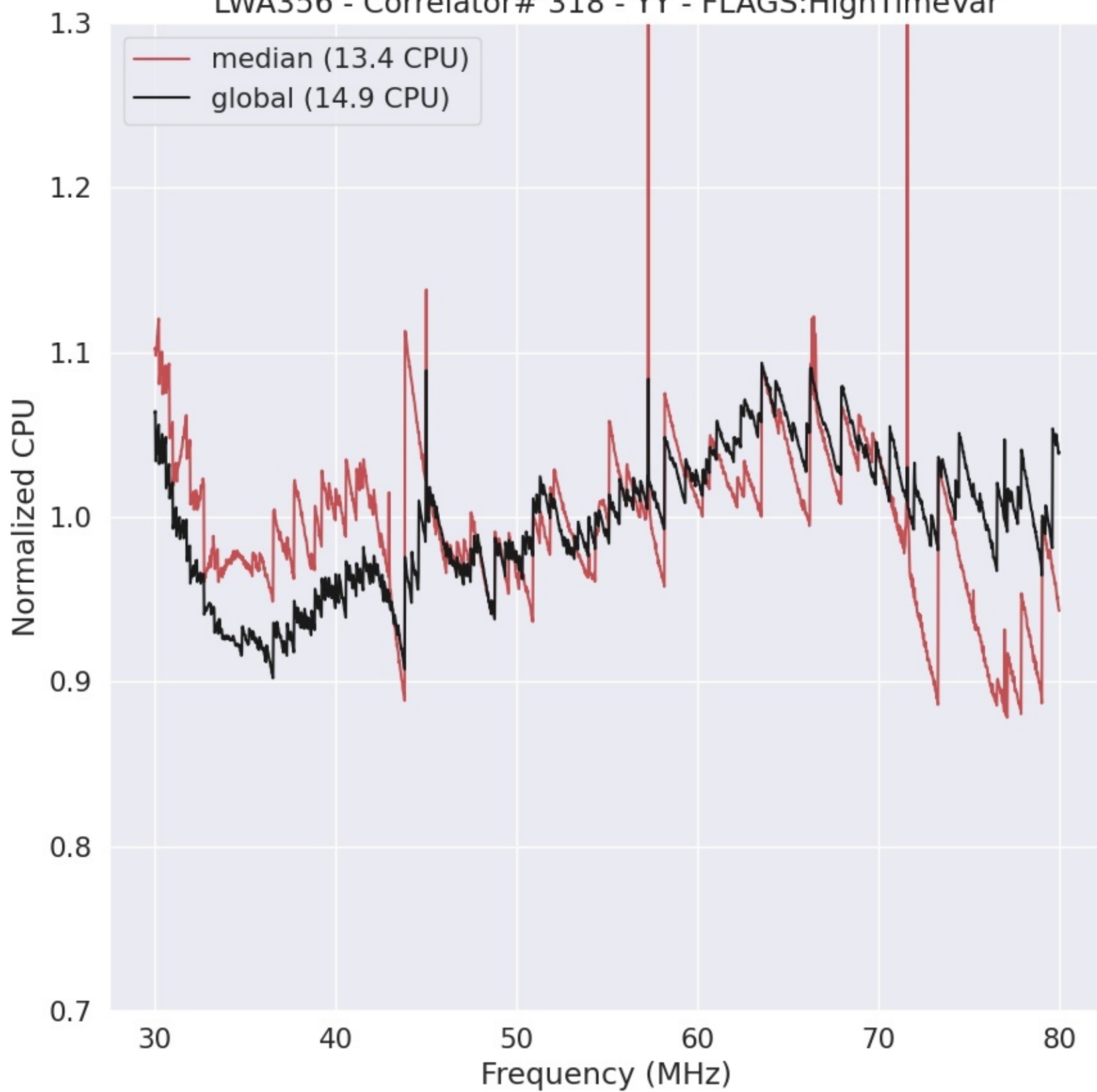
LWA356 - Correlator# 318 - YY - FLAGS:HighTimeVar
