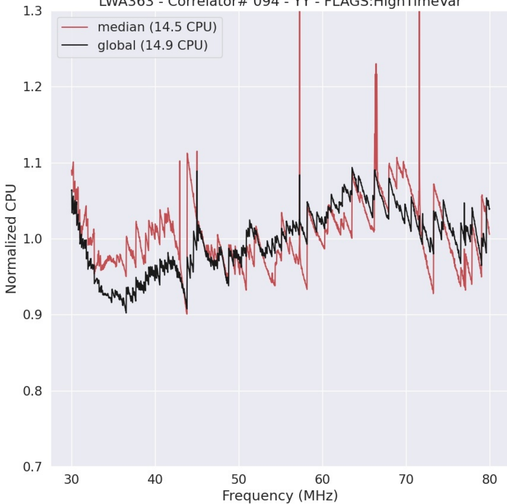
LWA363 - Correlator# 094 - YY - FLAGS:HighTimeVar
