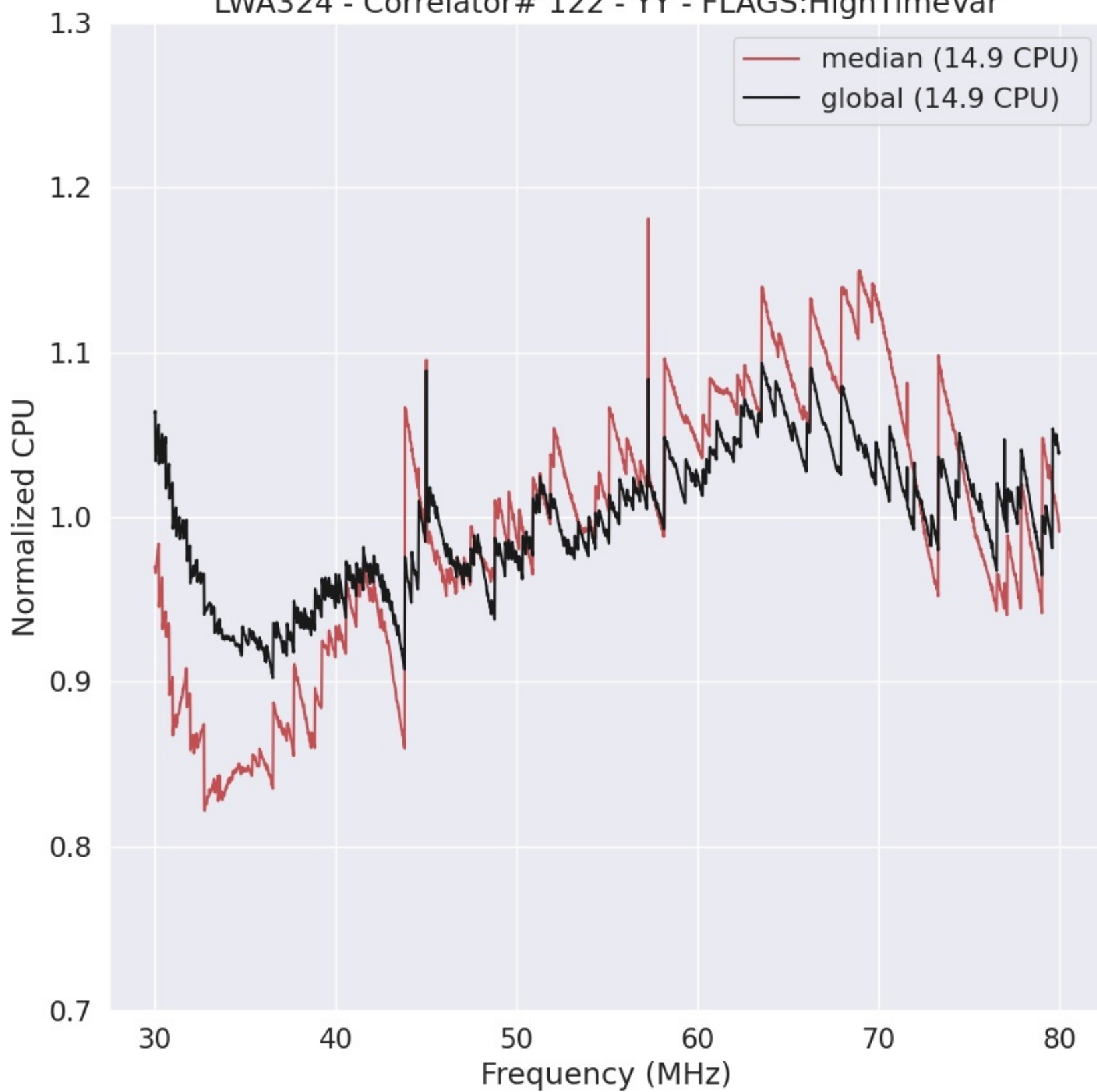
LWA324 - Correlator# 122 - YY - FLAGS:HighTimeVar
