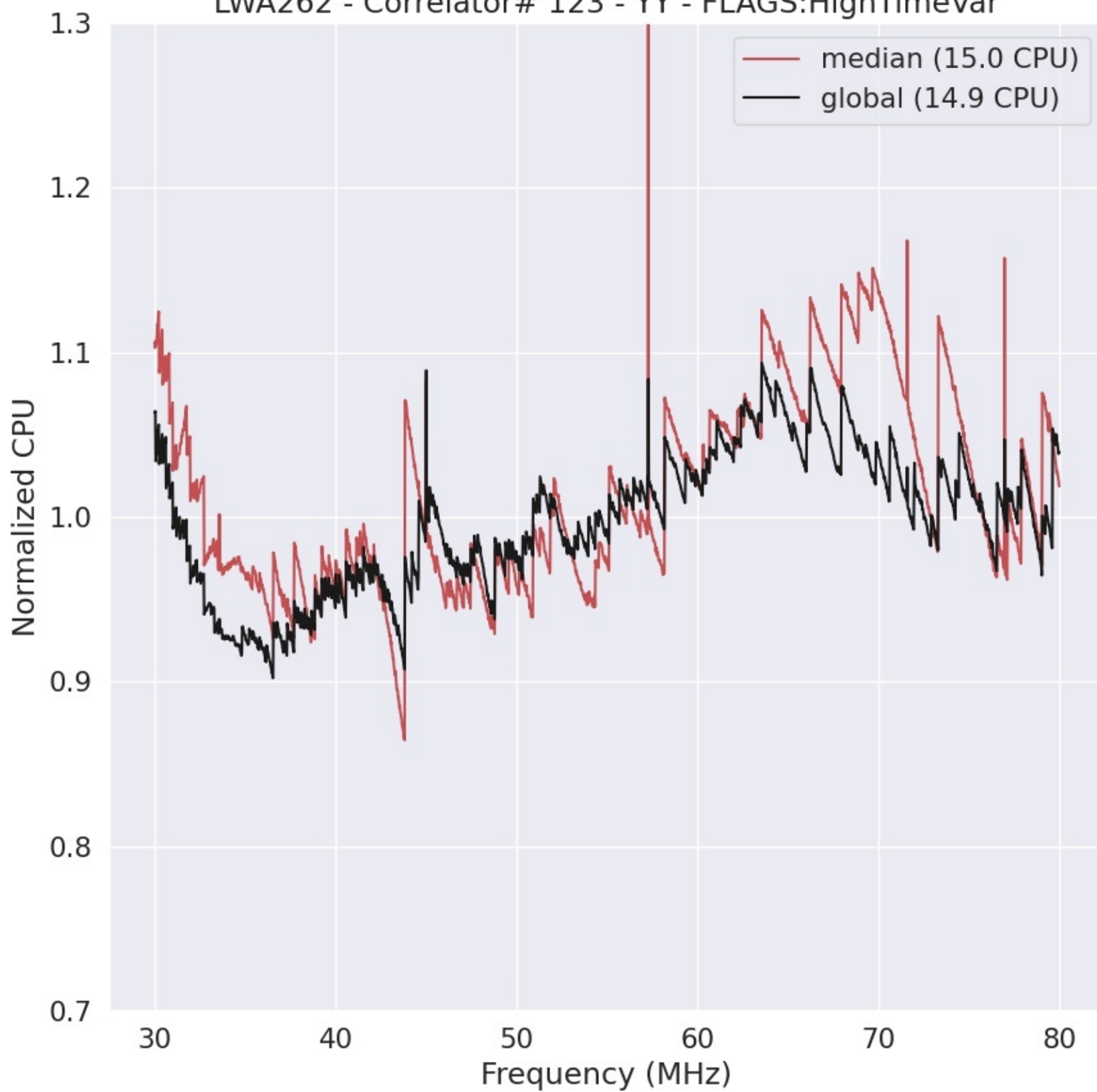
LWA262 - Correlator# 123 - YY - FLAGS:HighTimeVar
