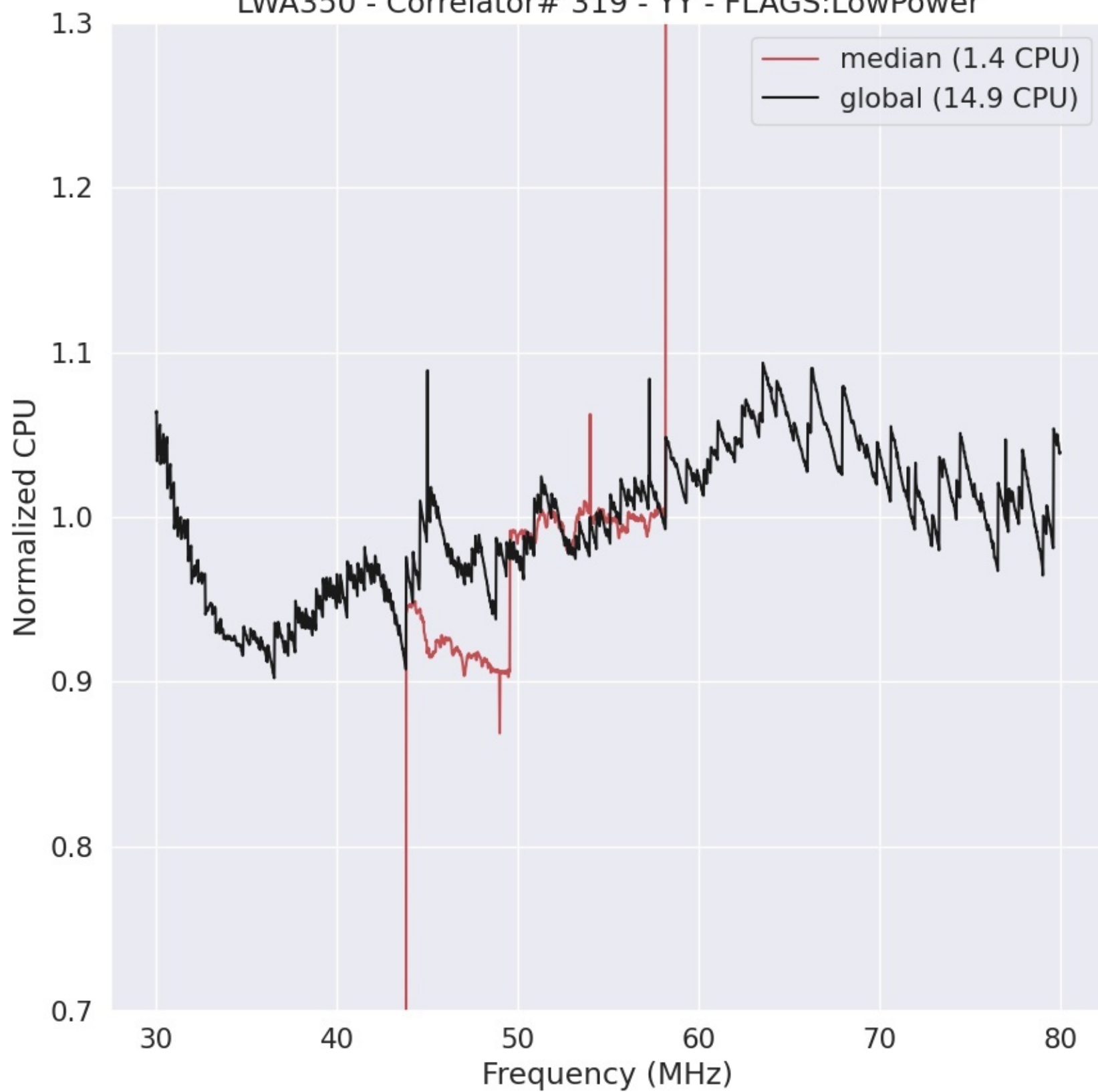
LWA350 - Correlator# 319 - YY - FLAGS:LowPower
