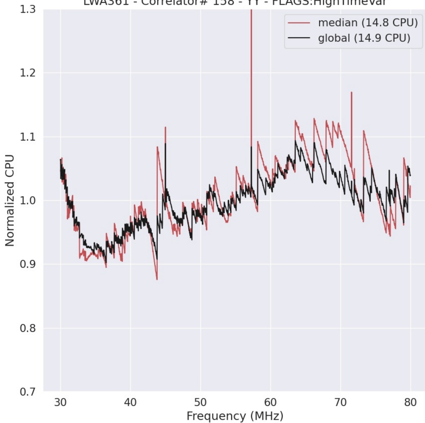
LWA361 - Correlator# 158 - YY - FLAGS:HighTimeVar
