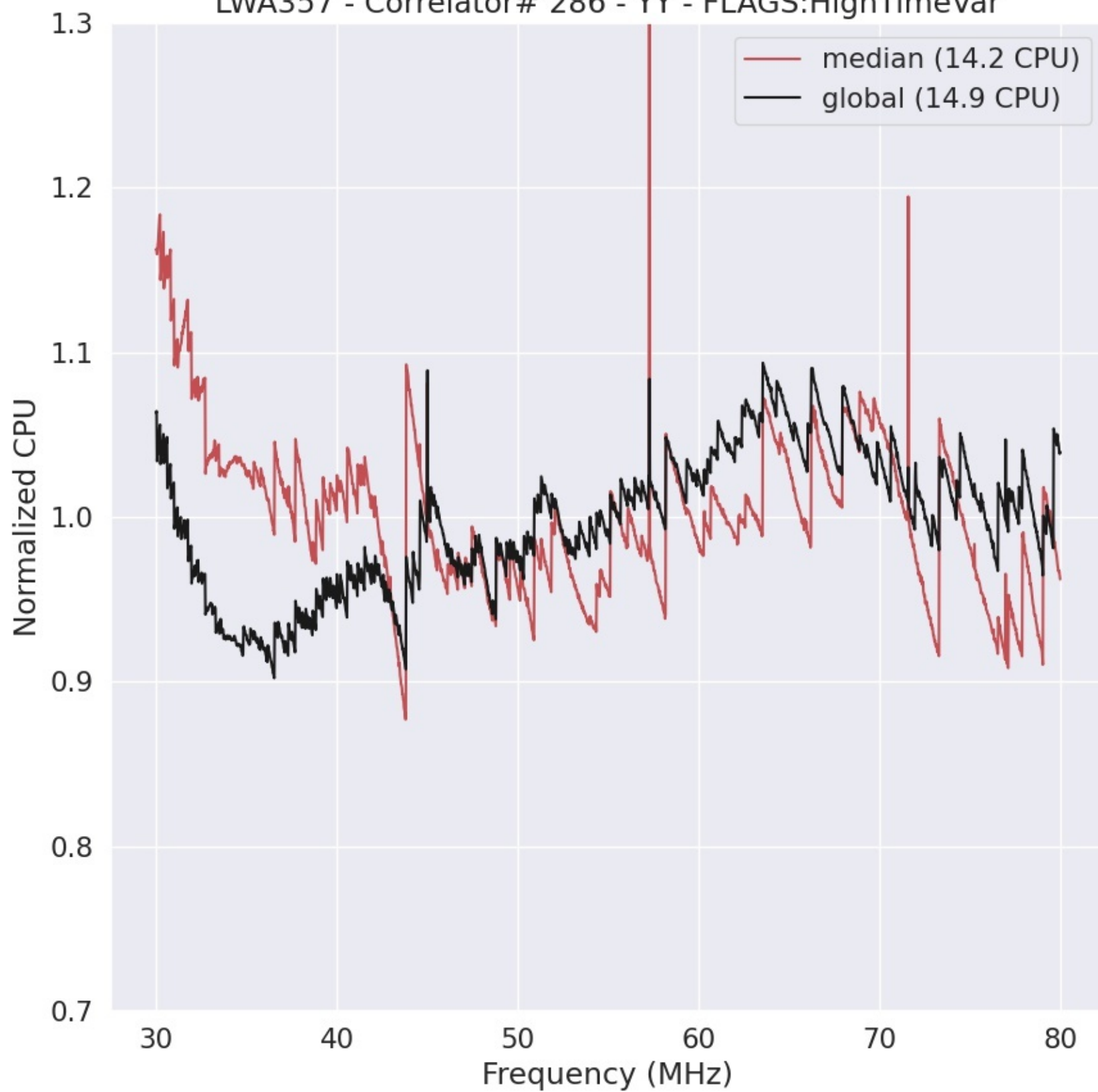
LWA357 - Correlator# 286 - YY - FLAGS:HighTimeVar
