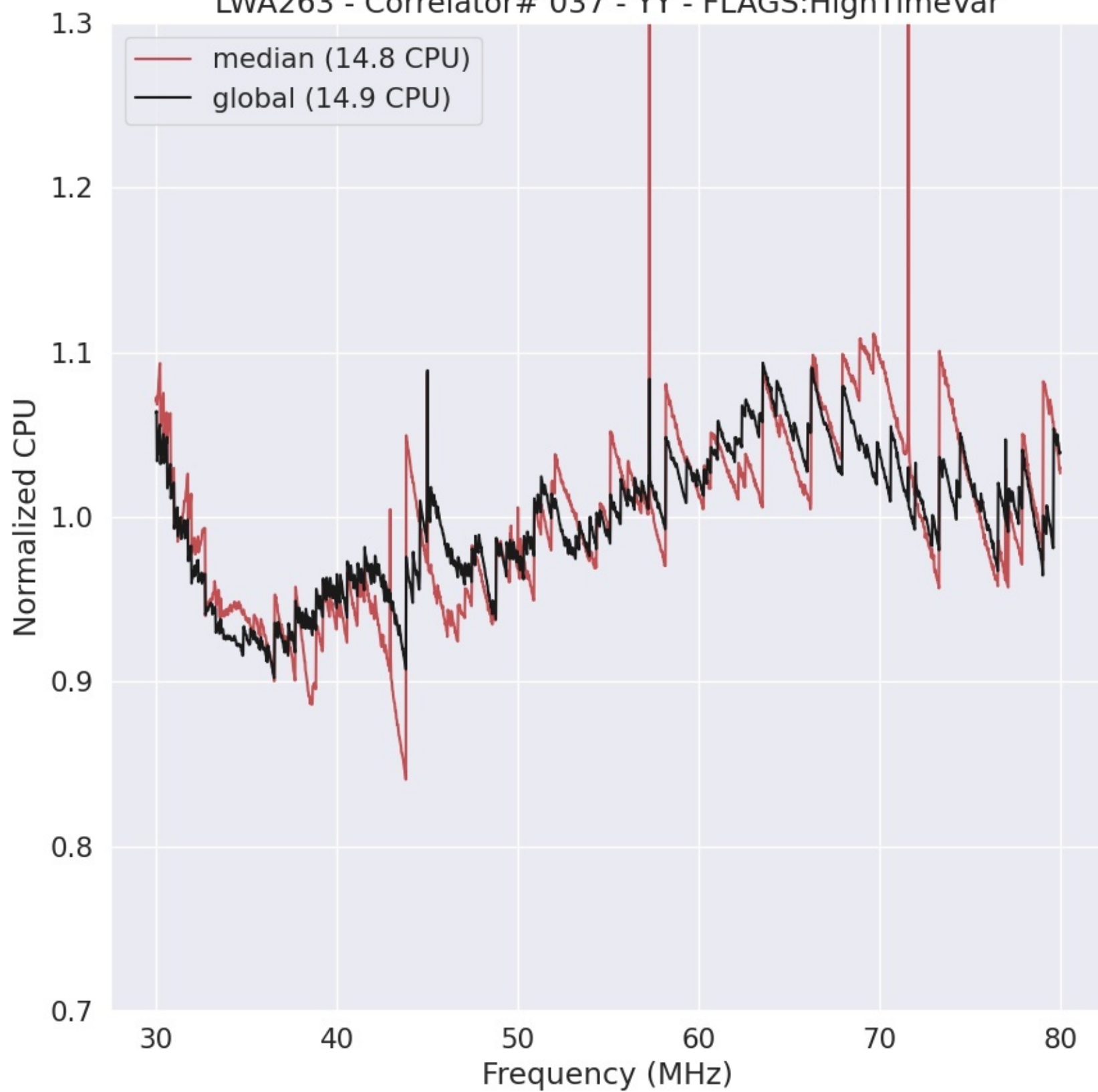
LWA263 - Correlator# 037 - YY - FLAGS:HighTimeVar
