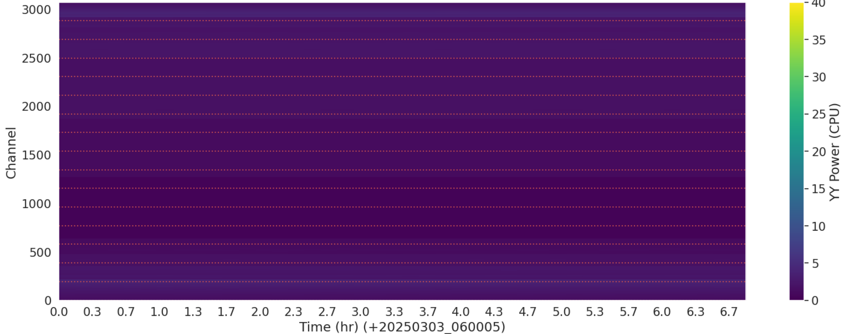
LWA363 - Correlator# 094 - YY - FLAGS: LowPower
