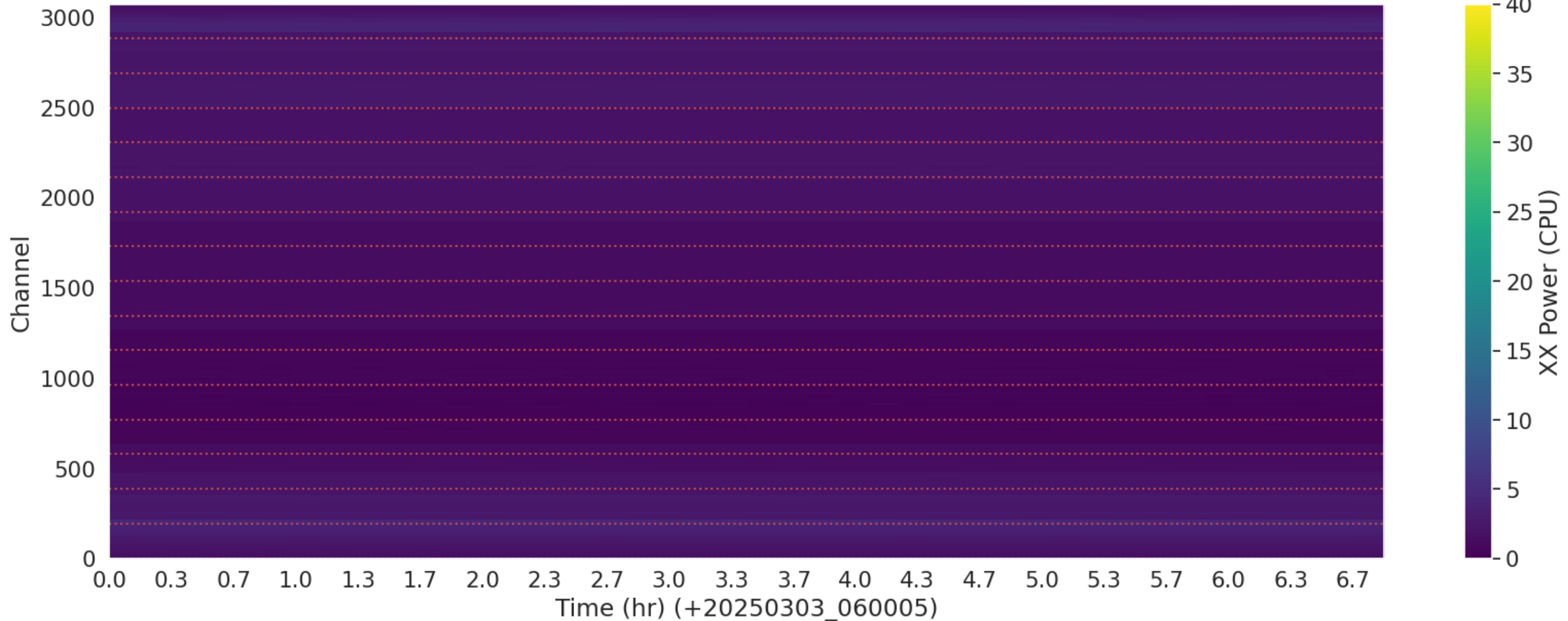
LWA362 - Correlator# 030 - XX - FLAGS: LowPower
