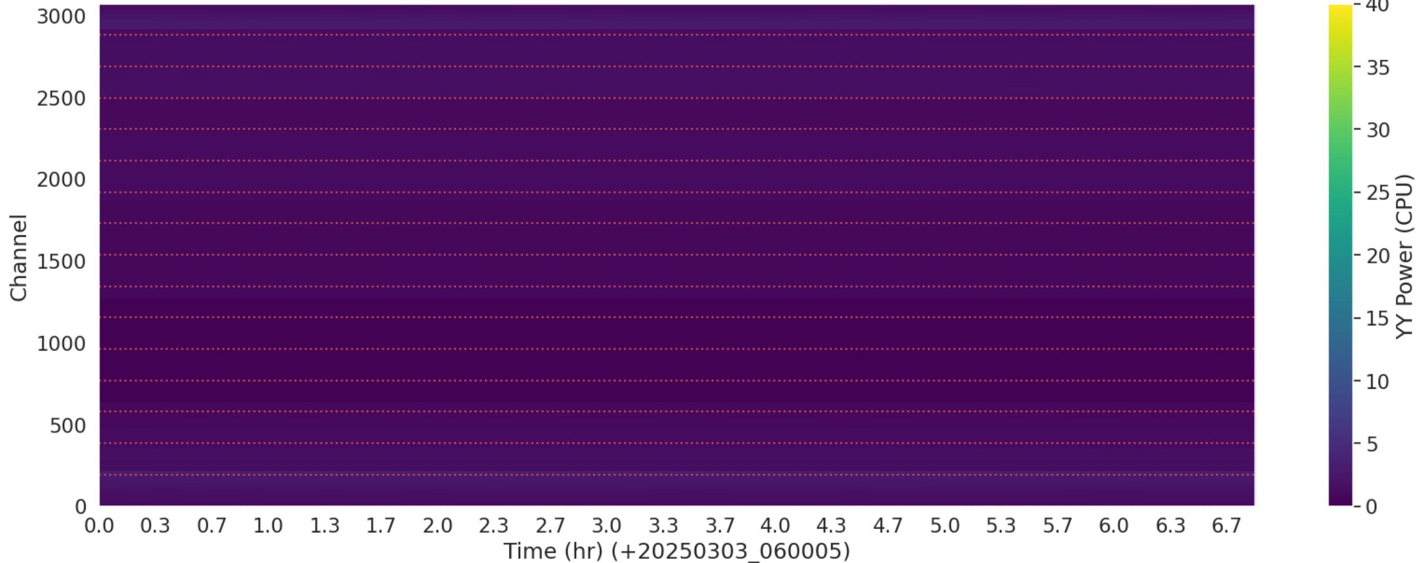
LWA356 - Correlator# 318 - YY - FLAGS: LowPower
