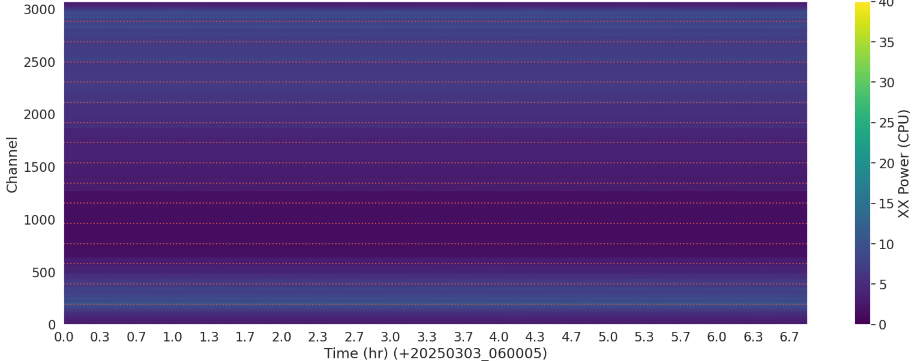
LWA318 - Correlator# 055 - XX - FLAGS: HighTimeVar+BadSpecShape
