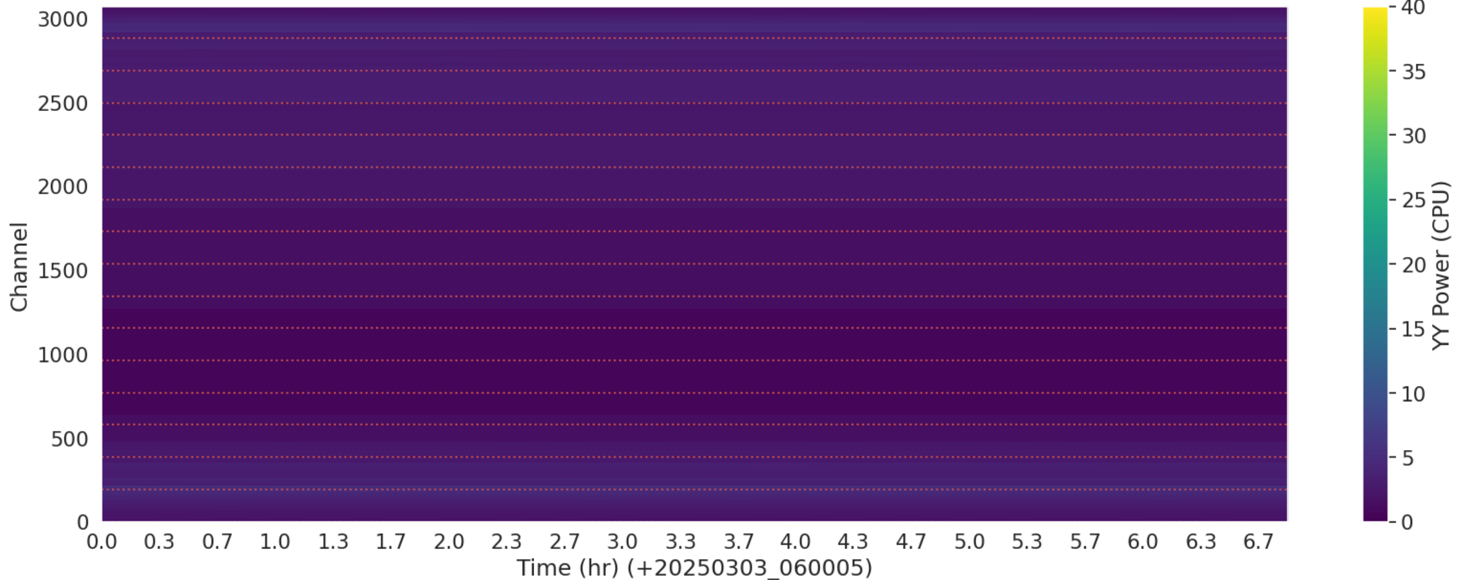
LWA364 - Correlator# 127 - YY - FLAGS: LowPower
