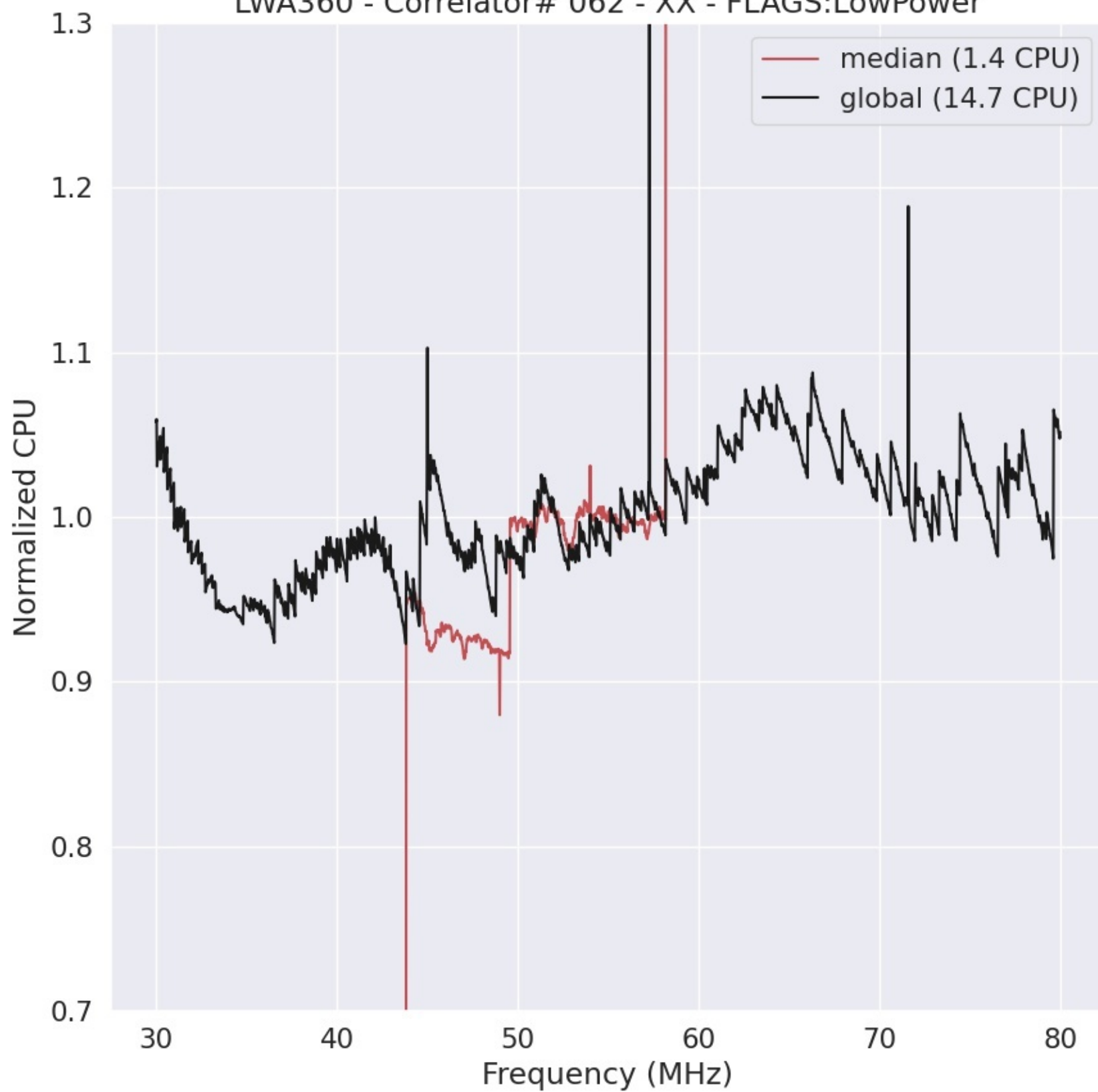
LWA360 - Correlator# 062 - XX - FLAGS:LowPower
