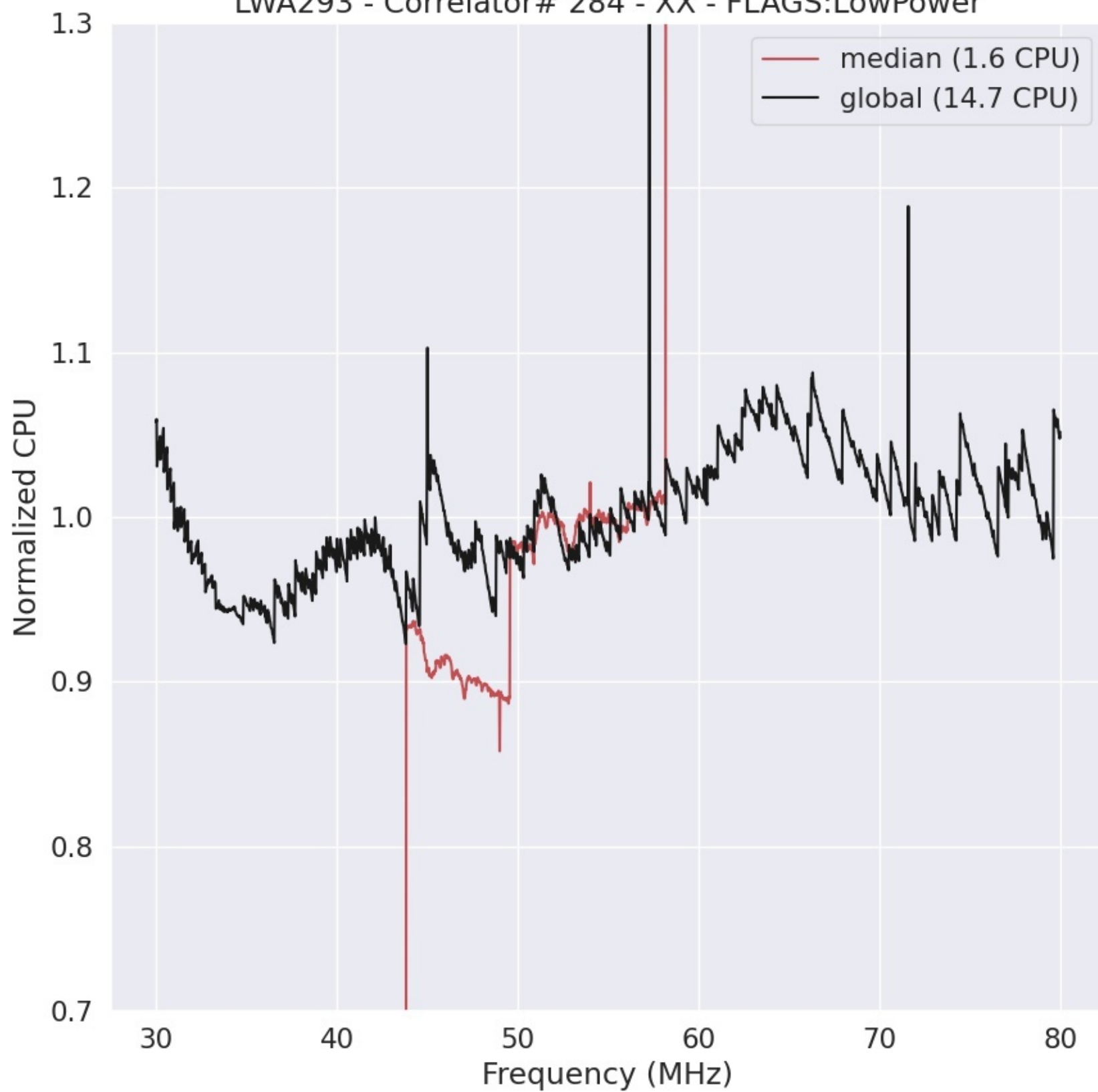
LWA293 - Correlator# 284 - XX - FLAGS:LowPower
