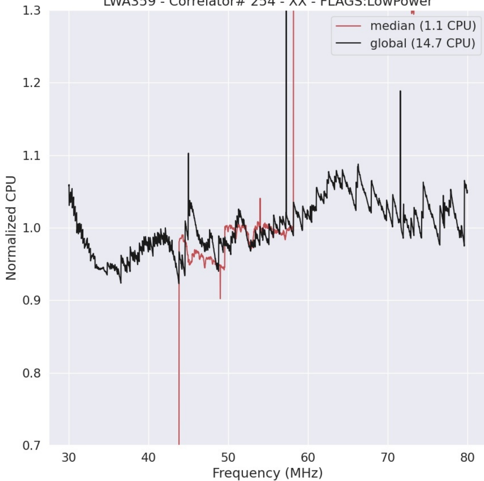
LWA359 - Correlator# 254 - XX - FLAGS:LowPower
