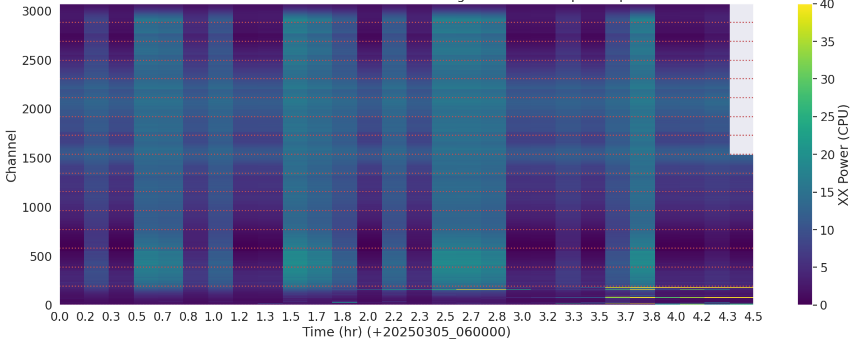
LWA103 - Correlator# 176 - XX - FLAGS: HighTimeVar+BadSpecShape
