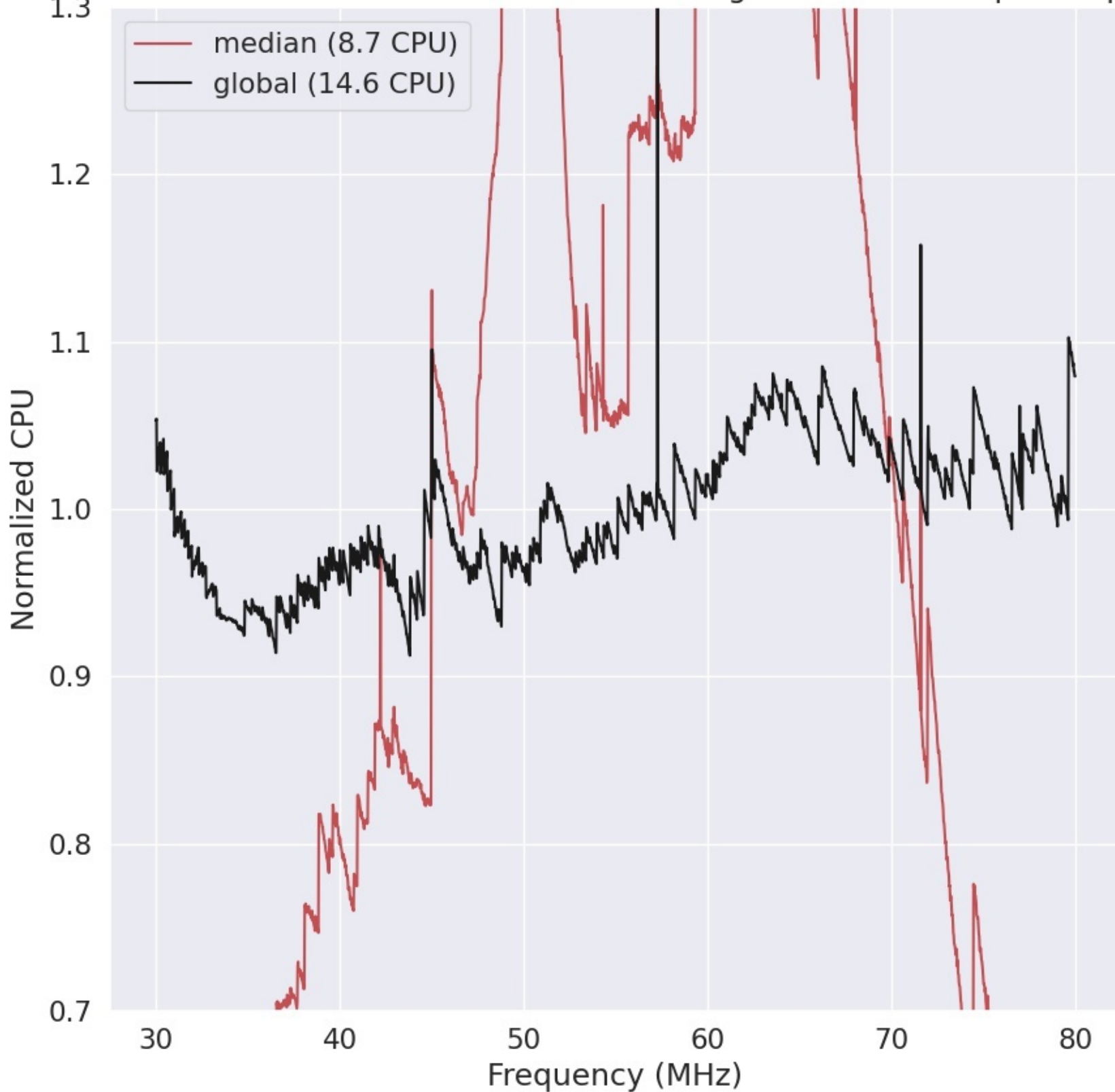
LWA103 - Correlator# 176 - XX - FLAGS:HighTimeVar+BadSpecShape
