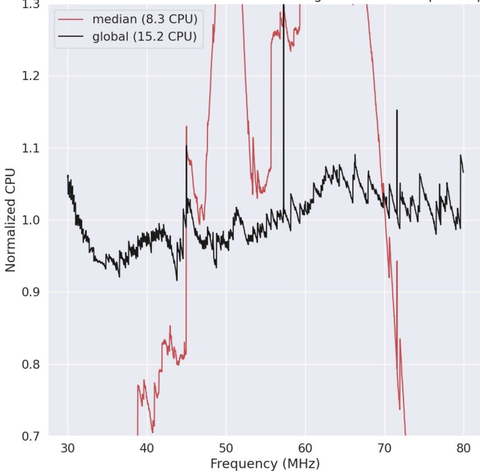
LWA103 - Correlator# 176 - XX - FLAGS:HighTimeVar+BadSpecShape
