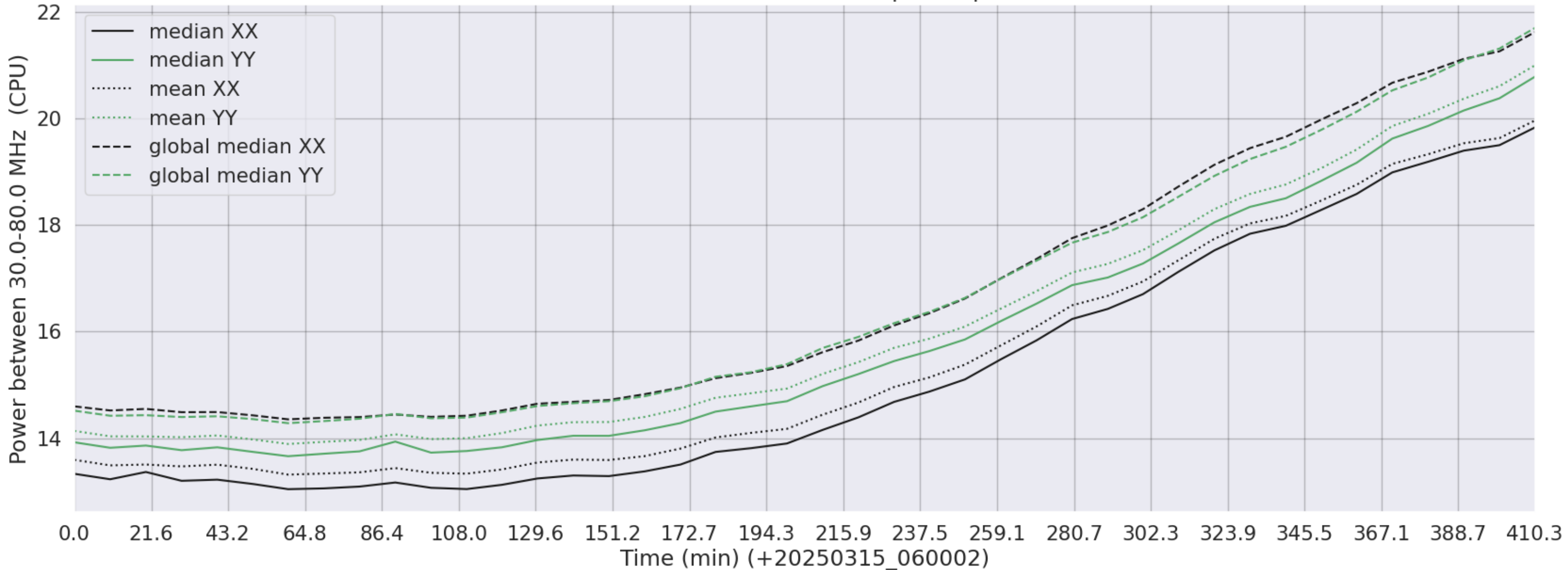
LWA042 - Correlator# 078 - XX FLAGS:BadSpecShape - YY FLAGS:Good
