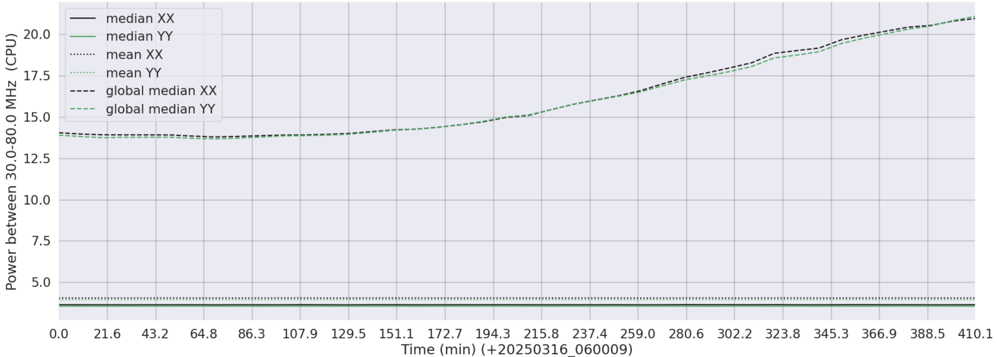
LWA286 - Correlator# 093 - XX FLAGS:HighTimeVar+BadSpecShape - YY FLAGS:HighTimeVar+BadSpecShape
