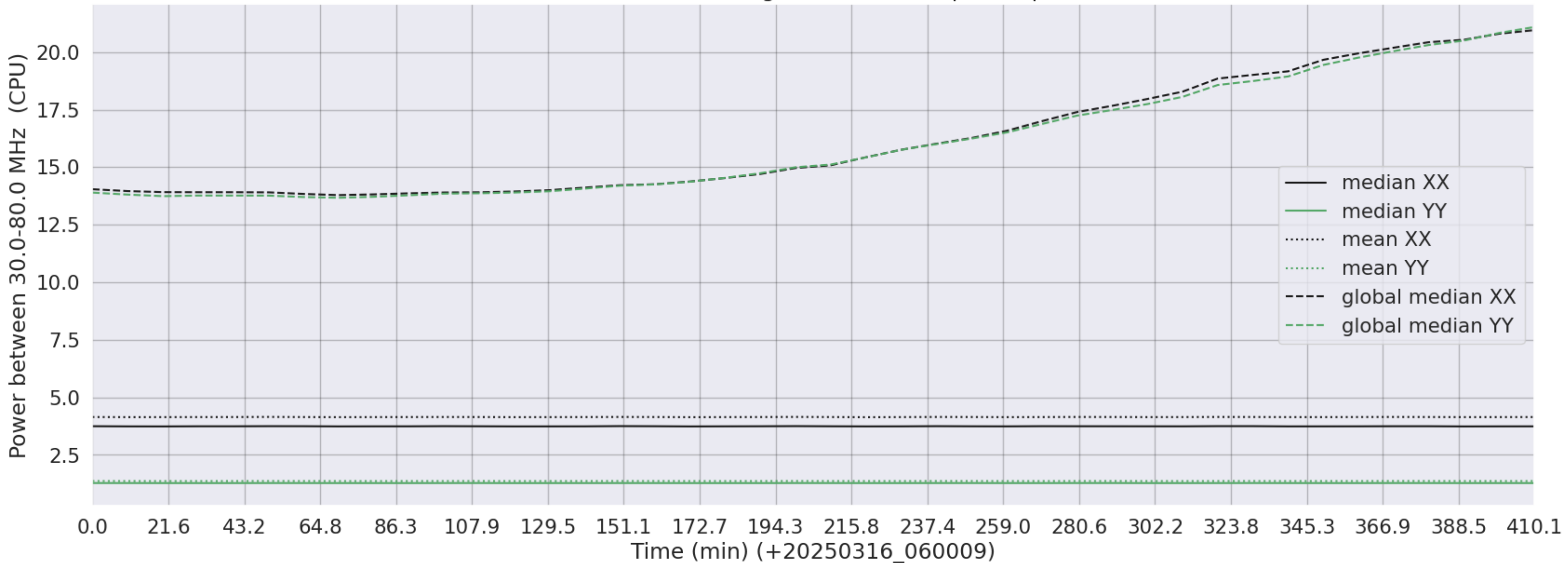
LWA315 - Correlator# 350 - XX FLAGS:HighTimeVar+BadSpecShape - YY FLAGS:LowPower
