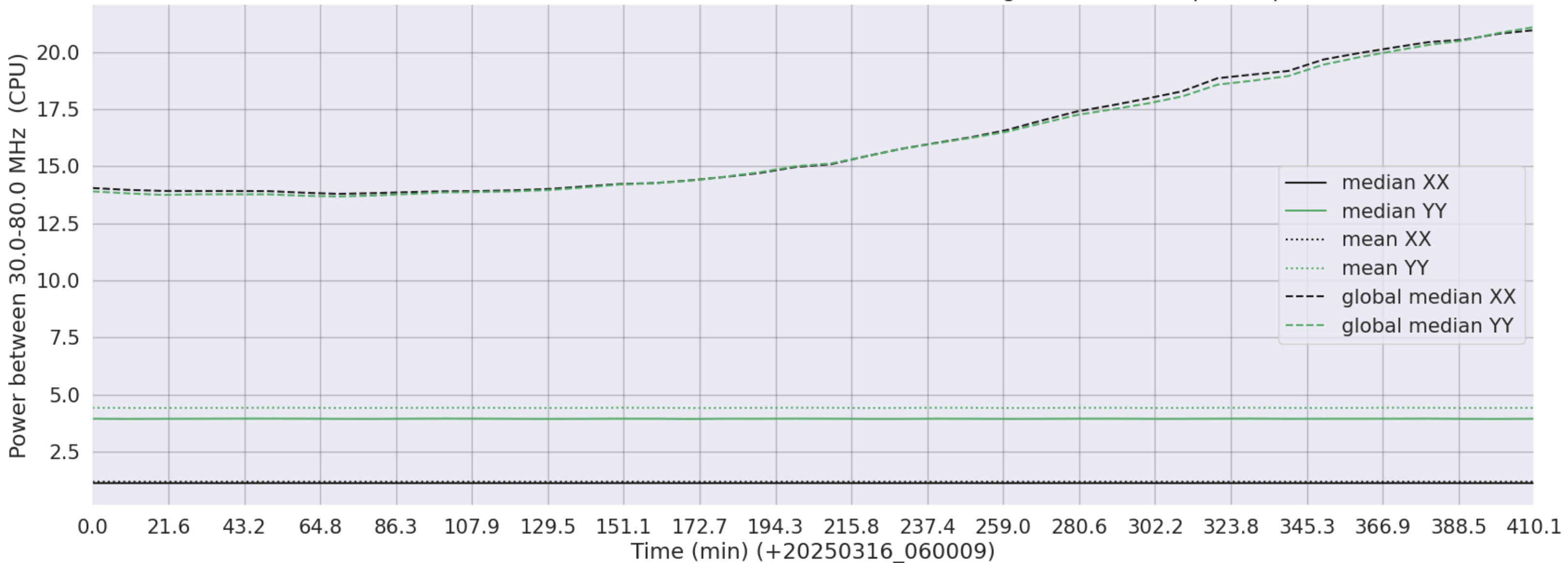
LWA326 - Correlator# 250 - XX FLAGS:LowPower - YY FLAGS:HighTimeVar+BadSpecShape
