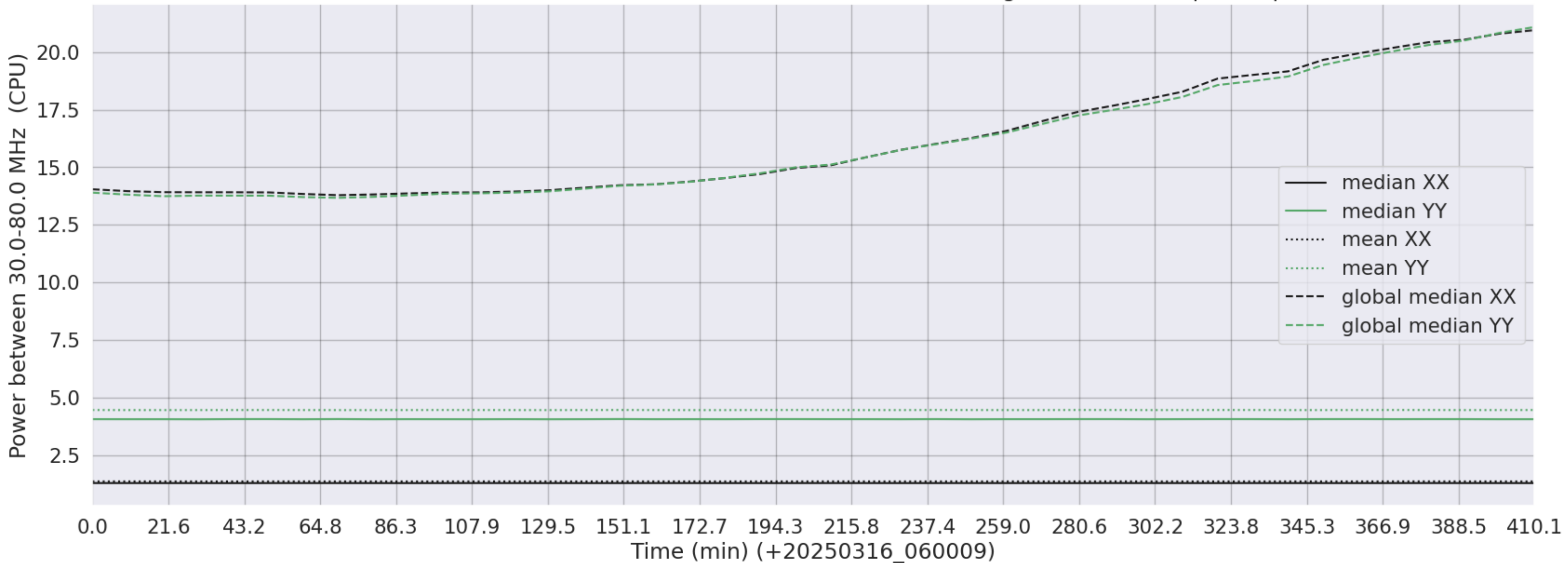
LWA354 - Correlator# 063 - XX FLAGS:LowPower - YY FLAGS:HighTimeVar+BadSpecShape
