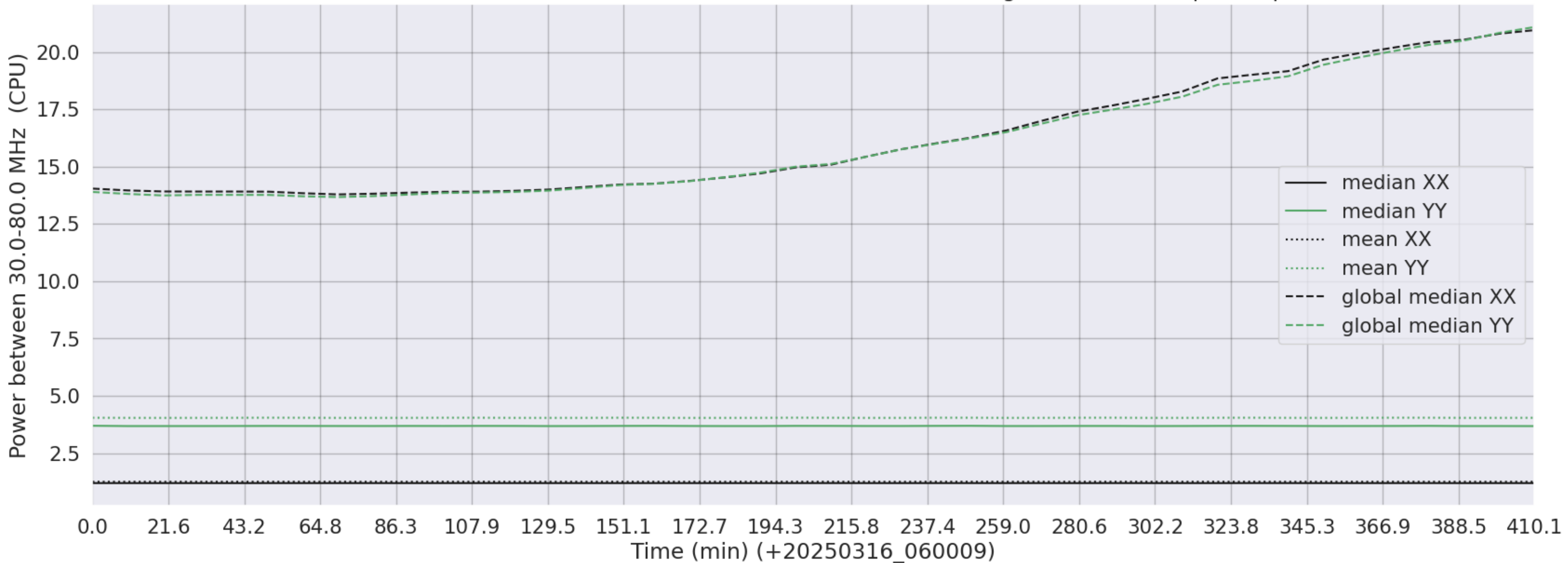
LWA269 - Correlator# 005 - XX FLAGS:LowPower - YY FLAGS:HighTimeVar+BadSpecShape
