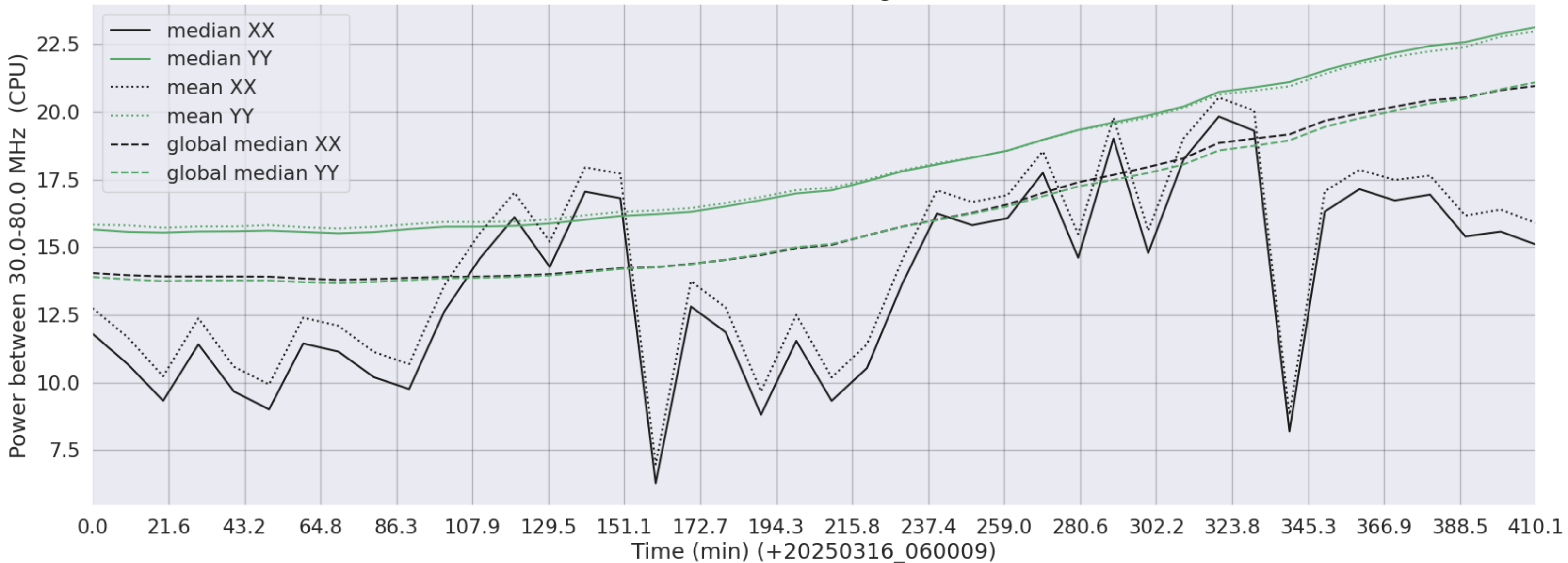
LWA131 - Correlator# 182 - XX FLAGS:HighTimeVar - YY FLAGS:Good
