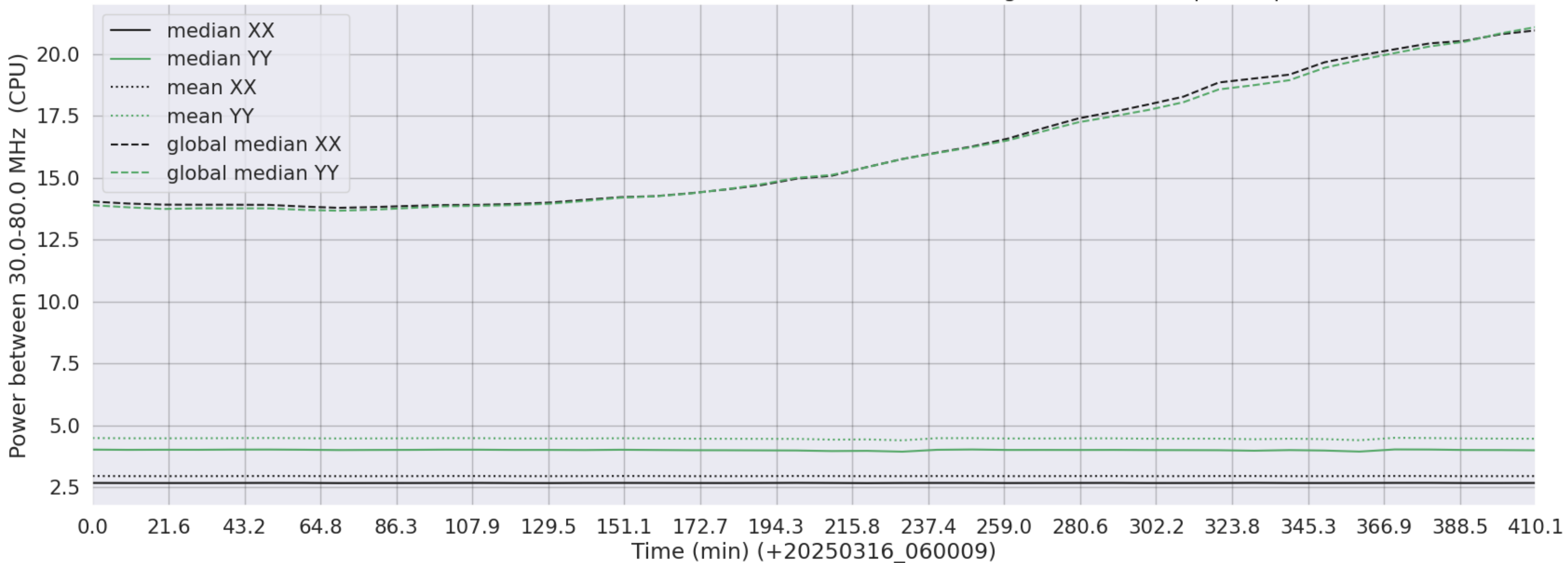
LWA335 - Correlator# 057 - XX FLAGS:LowPower - YY FLAGS:HighTimeVar+BadSpecShape
