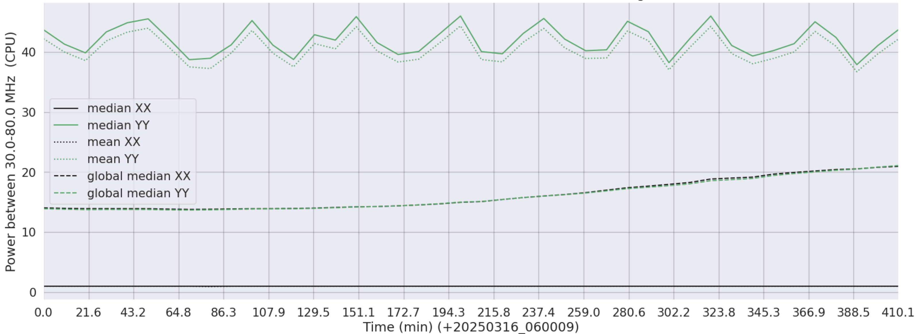
LWA280 - Correlator# 041 - XX FLAGS:LowPower - YY FLAGS:HighTimeVar
