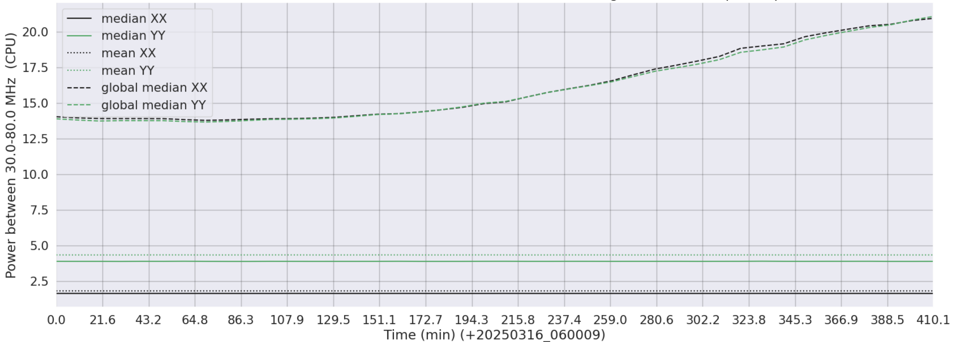
LWA328 - Correlator# 157 - XX FLAGS:LowPower - YY FLAGS:HighTimeVar+BadSpecShape
