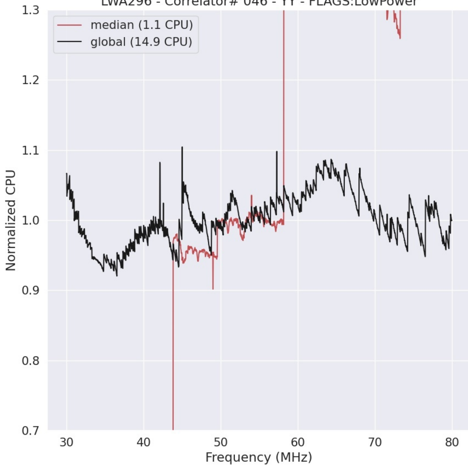
LWA296 - Correlator# 046 - YY - FLAGS:LowPower
