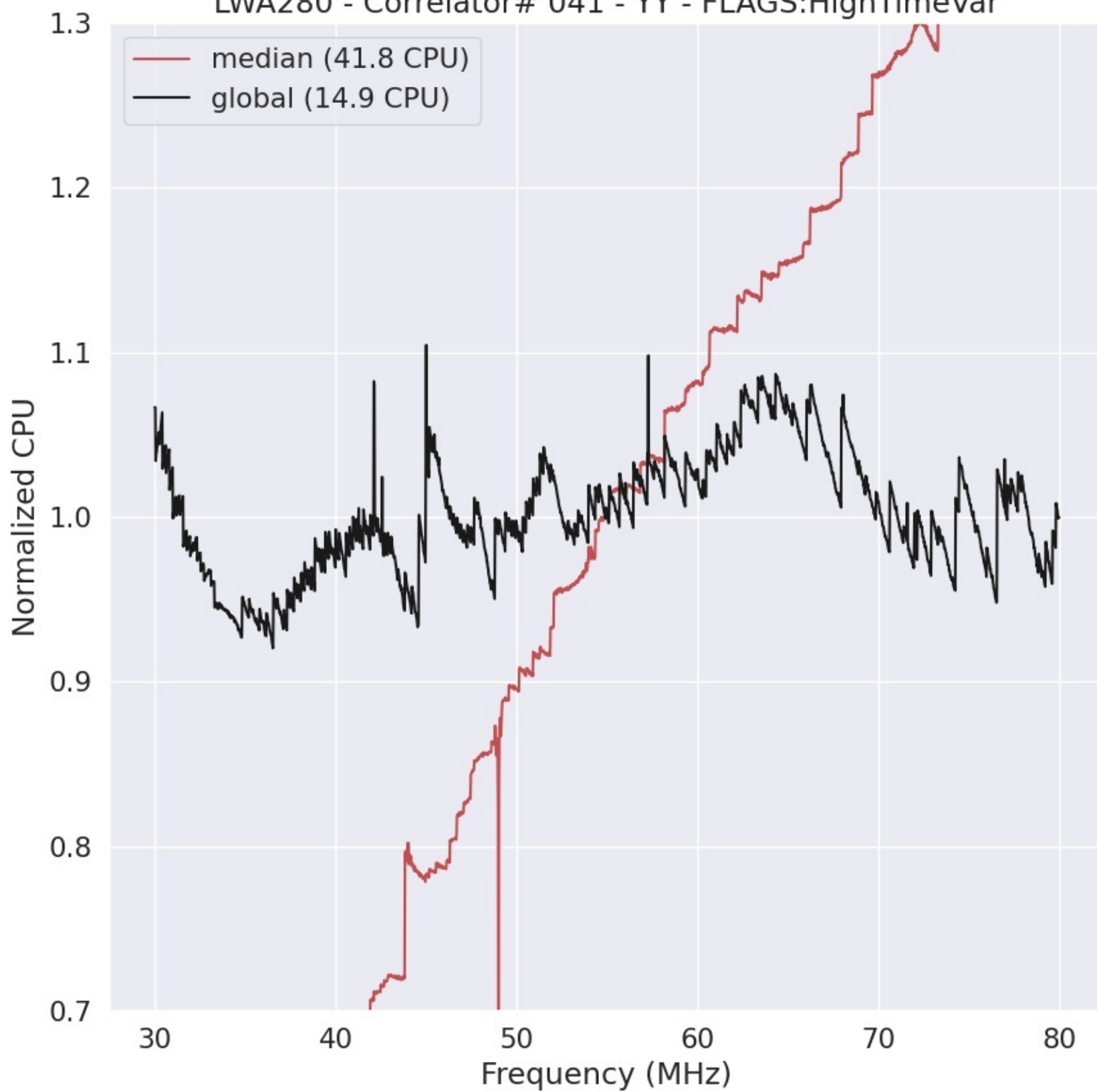
LWA280 - Correlator# 041 - YY - FLAGS:HighTimeVar
