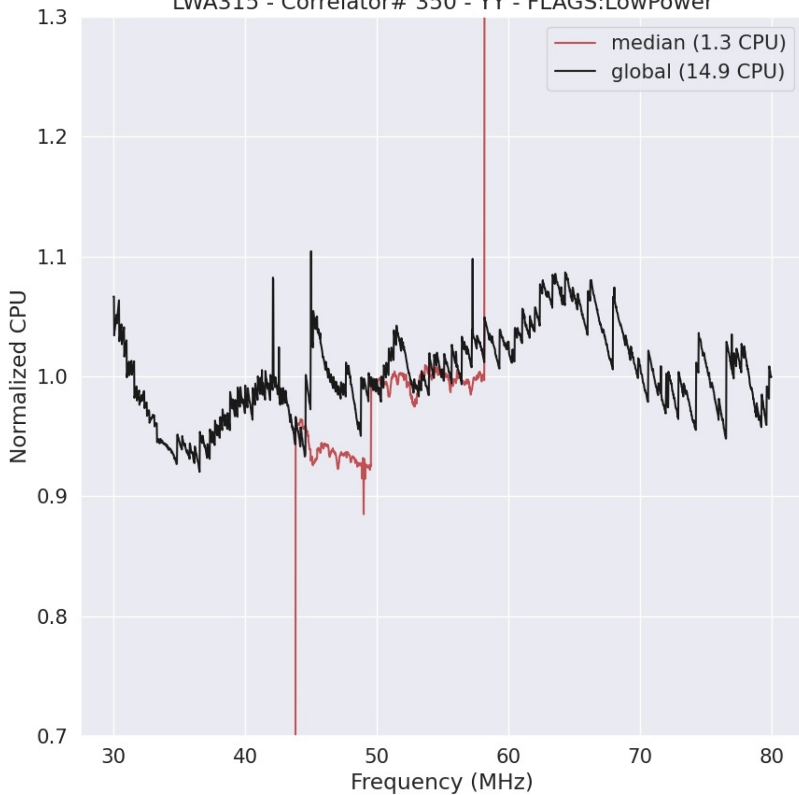
LWA315 - Correlator# 350 - YY - FLAGS:LowPower
