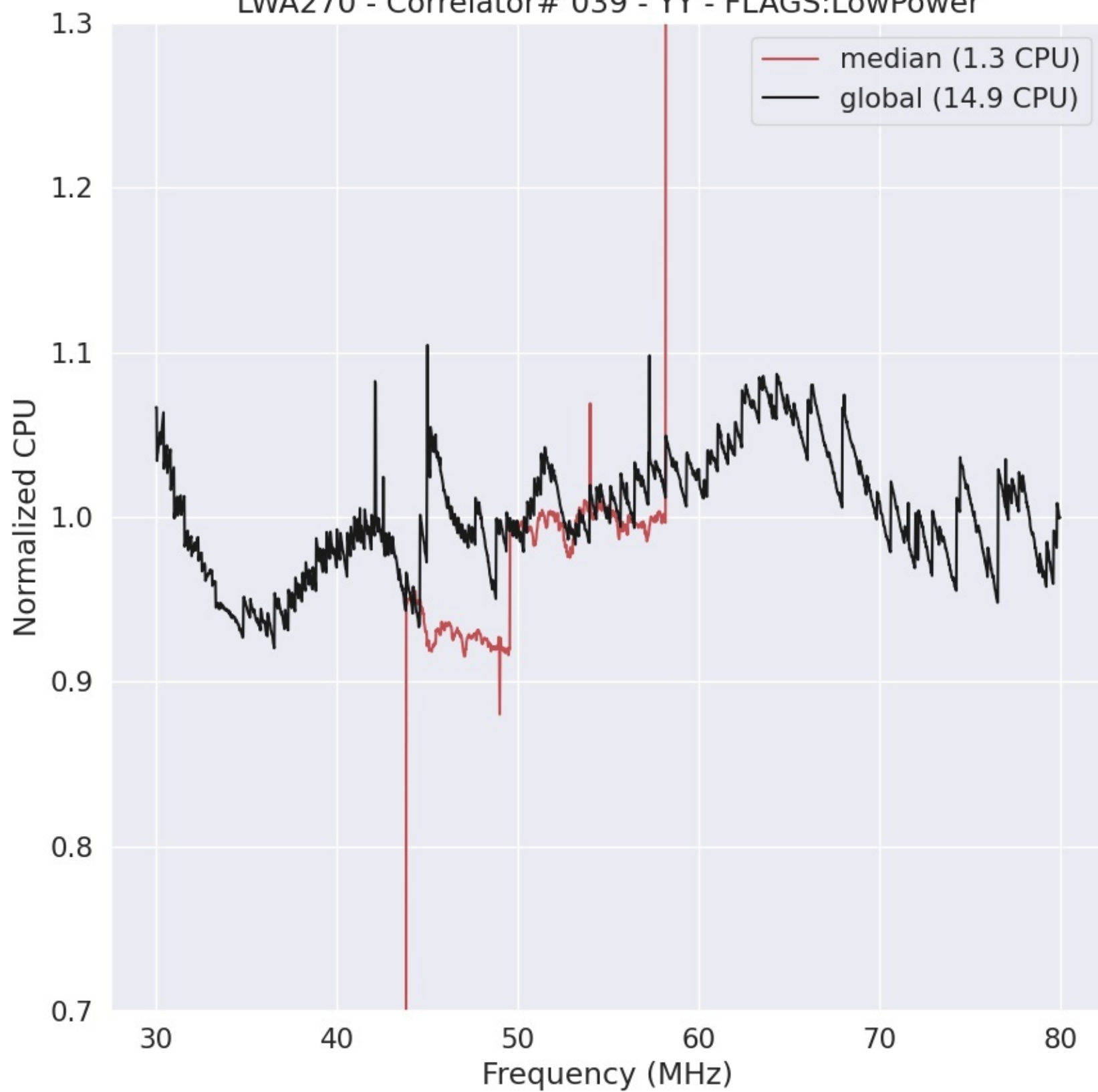
LWA270 - Correlator# 039 - YY - FLAGS:LowPower
