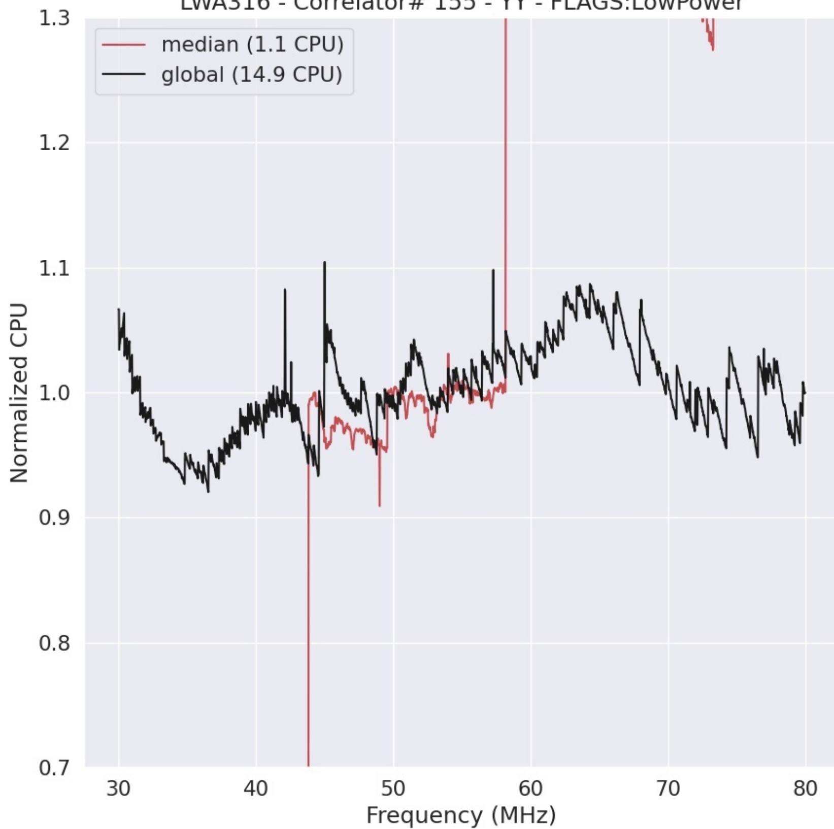
LWA316 - Correlator# 155 - YY - FLAGS:LowPower
