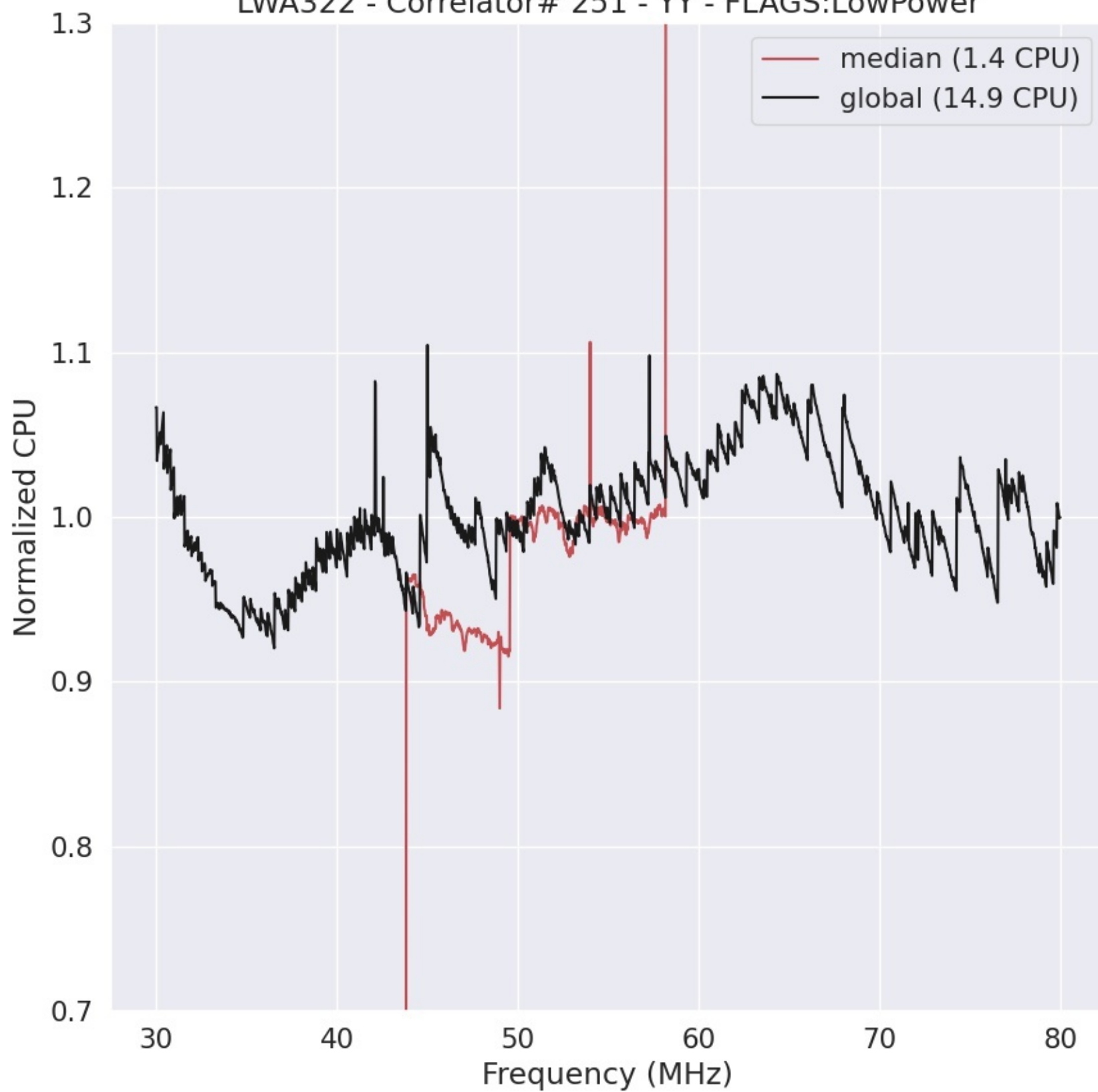
LWA322 - Correlator# 251 - YY - FLAGS:LowPower
