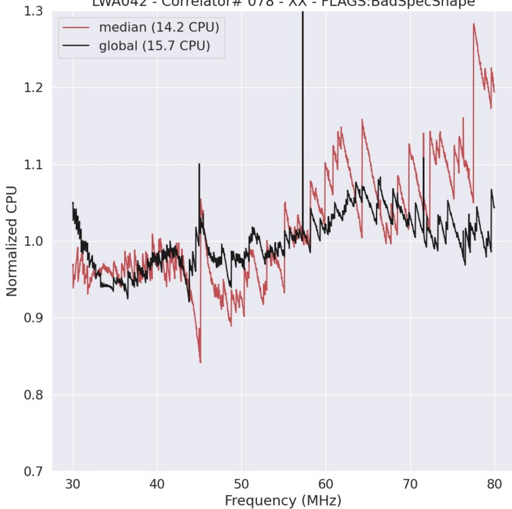
LWA042 - Correlator# 078 - XX - FLAGS:BadSpecShape
