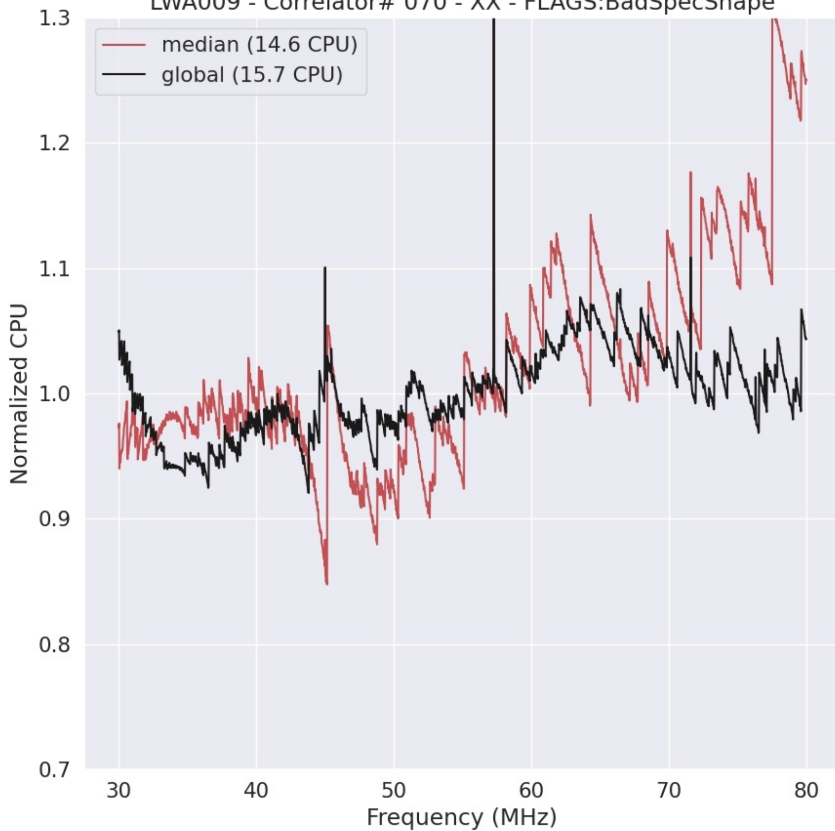
LWA009 - Correlator# 070 - XX - FLAGS:BadSpecShape
