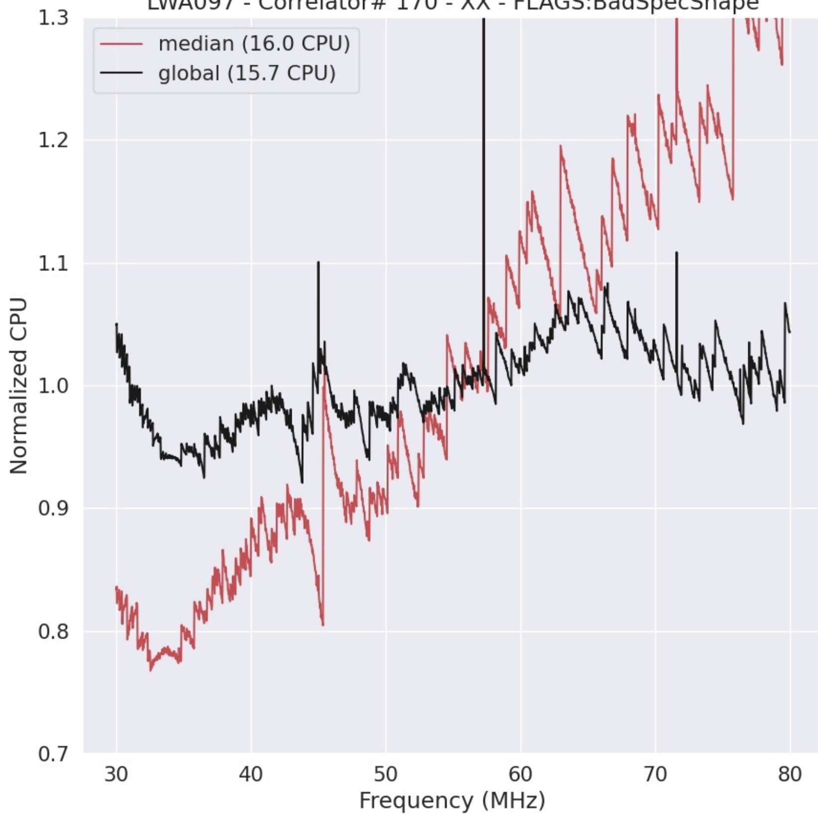
LWA097 - Correlator# 170 - XX - FLAGS:BadSpecShape
