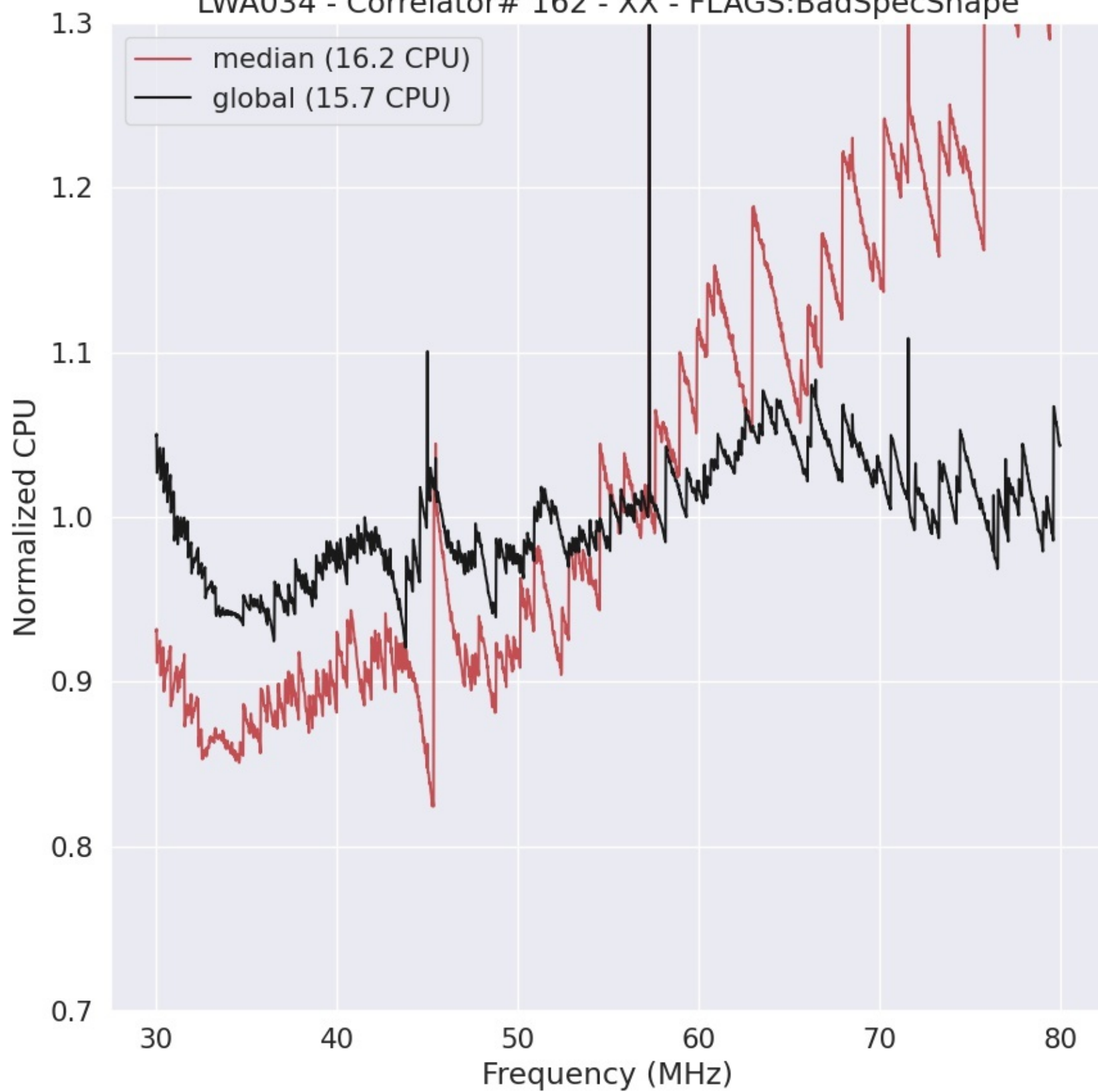
LWA034 - Correlator# 162 - XX - FLAGS:BadSpecShape
