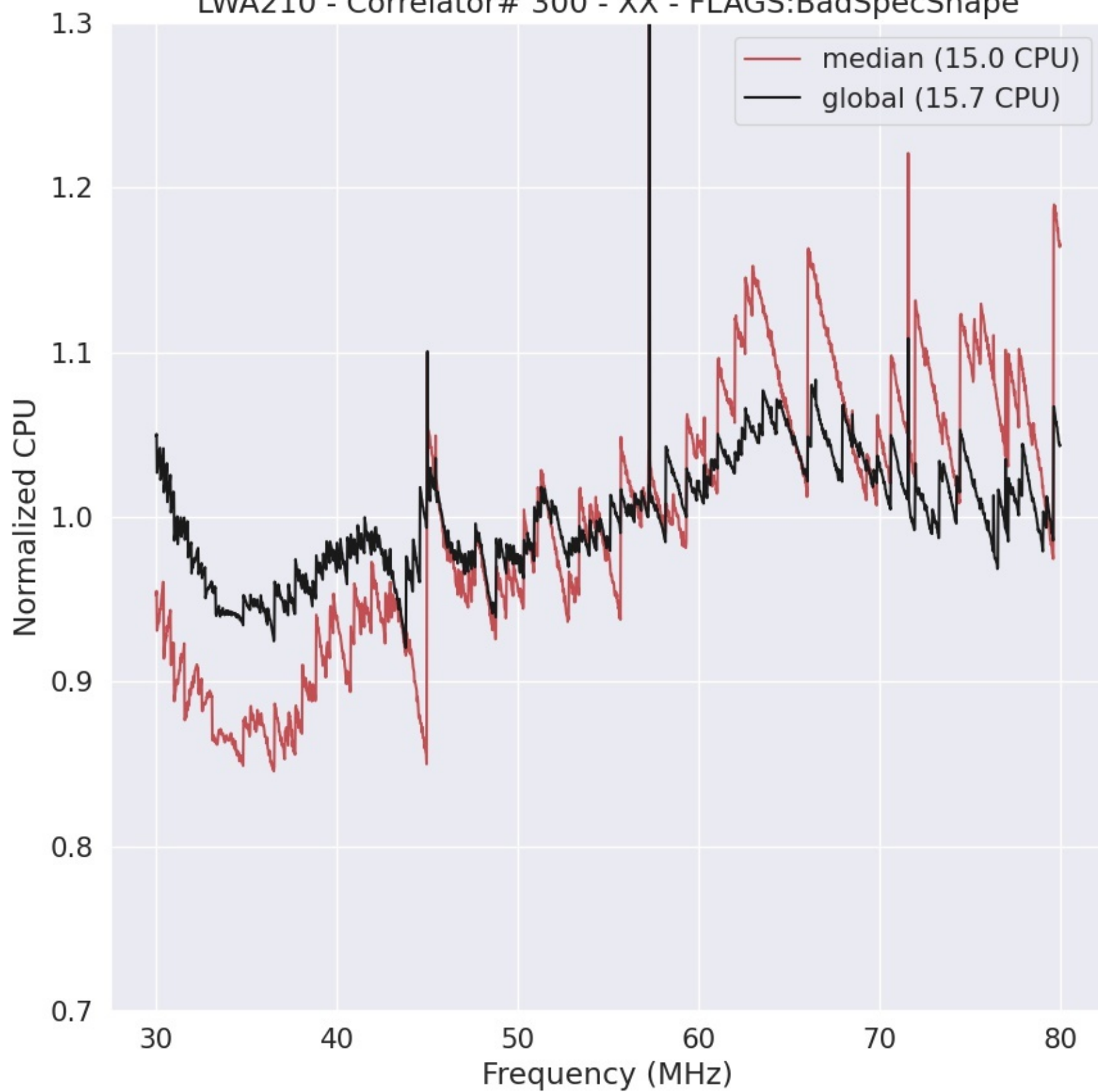
LWA210 - Correlator# 300 - XX - FLAGS:BadSpecShape
