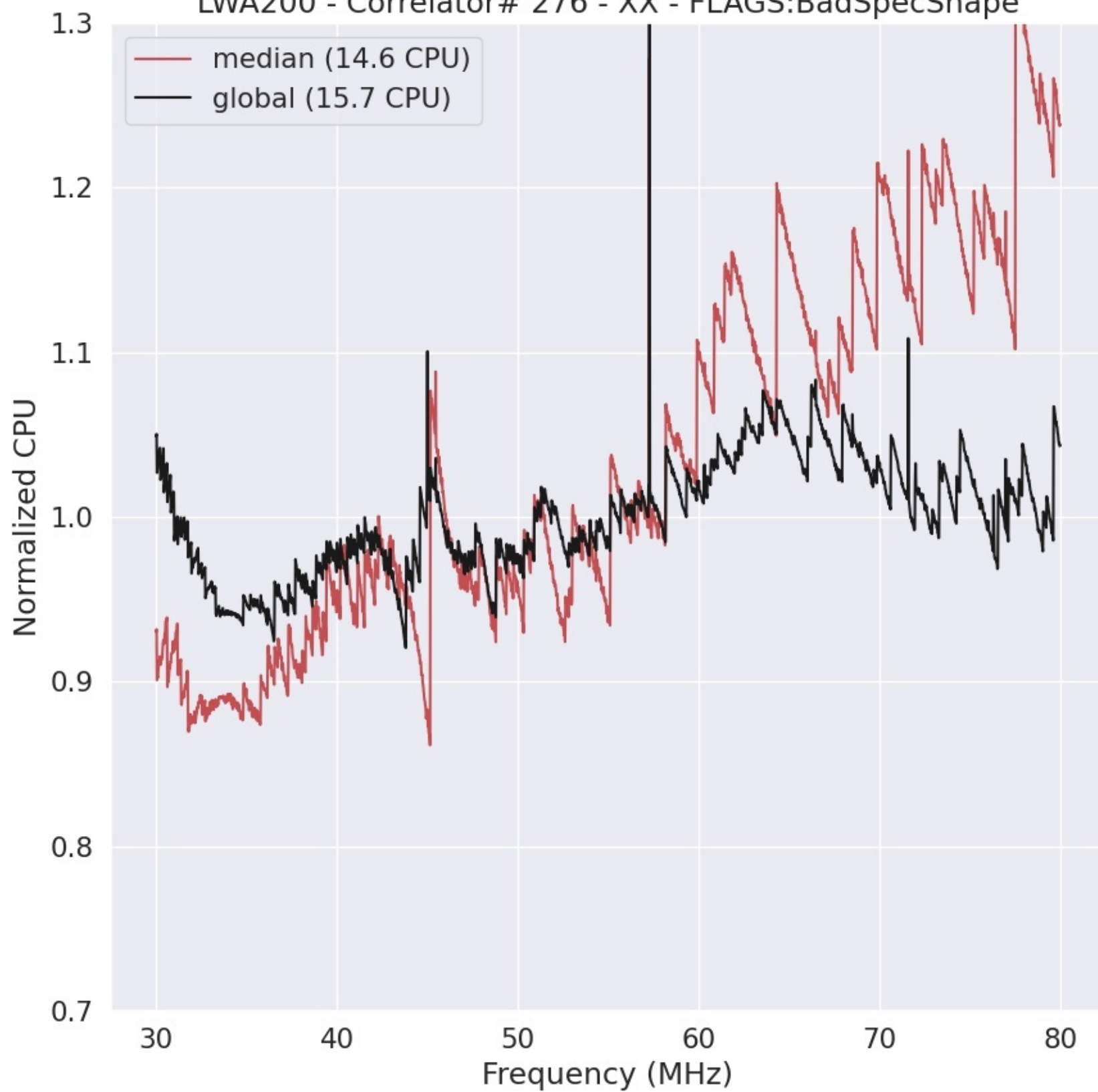
LWA200 - Correlator# 276 - XX - FLAGS:BadSpecShape
