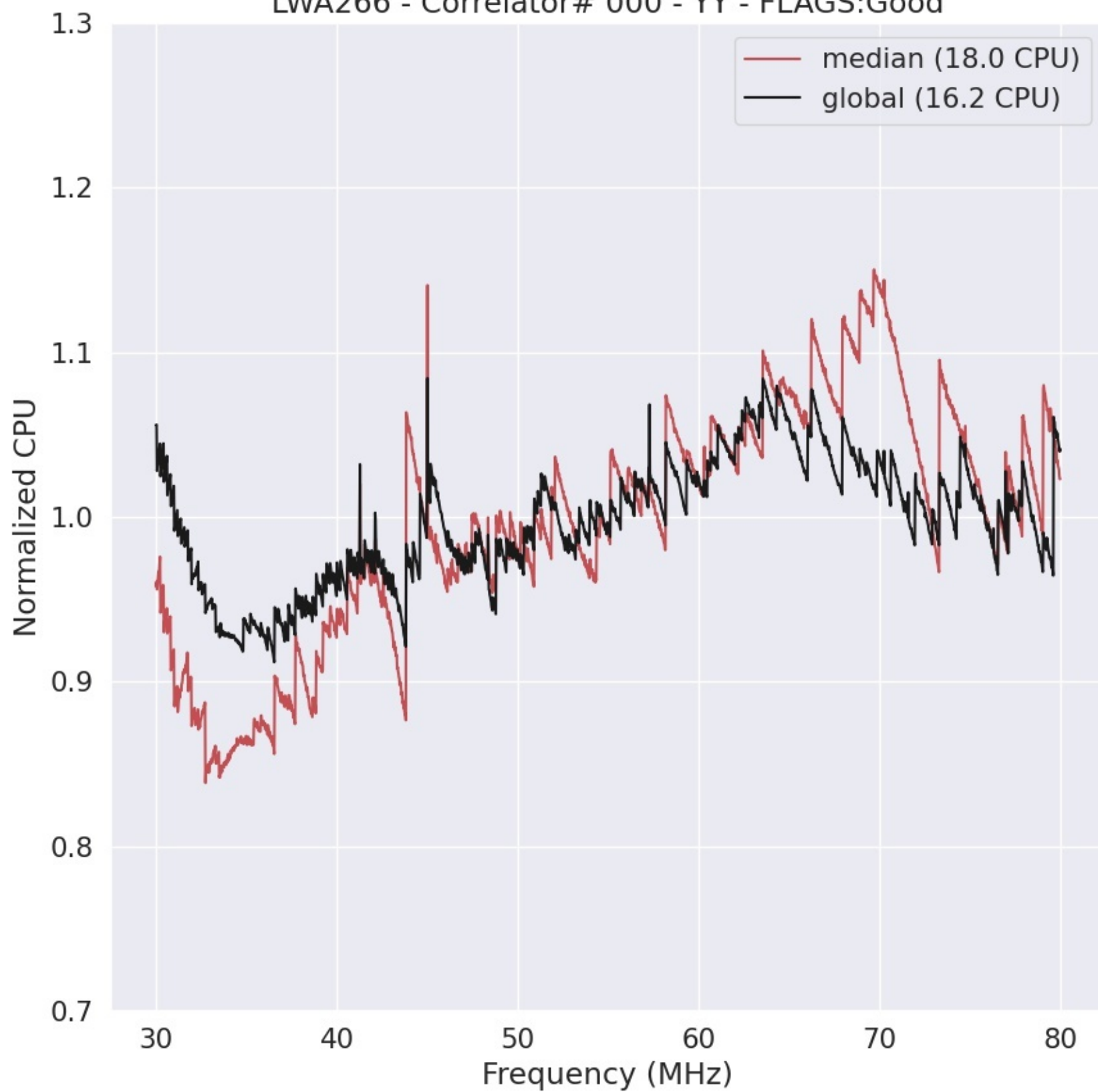
LWA266 - Correlator# 000 - YY - FLAGS:Good
