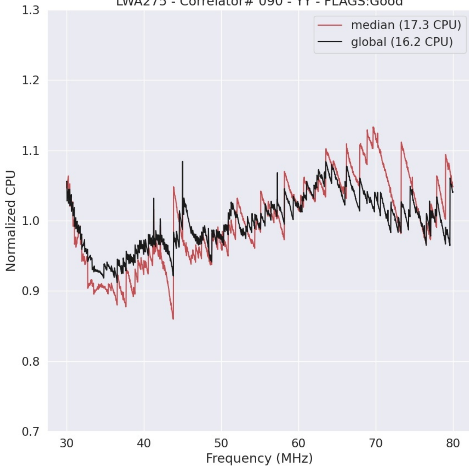
LWA275 - Correlator# 090 - YY - FLAGS:Good
