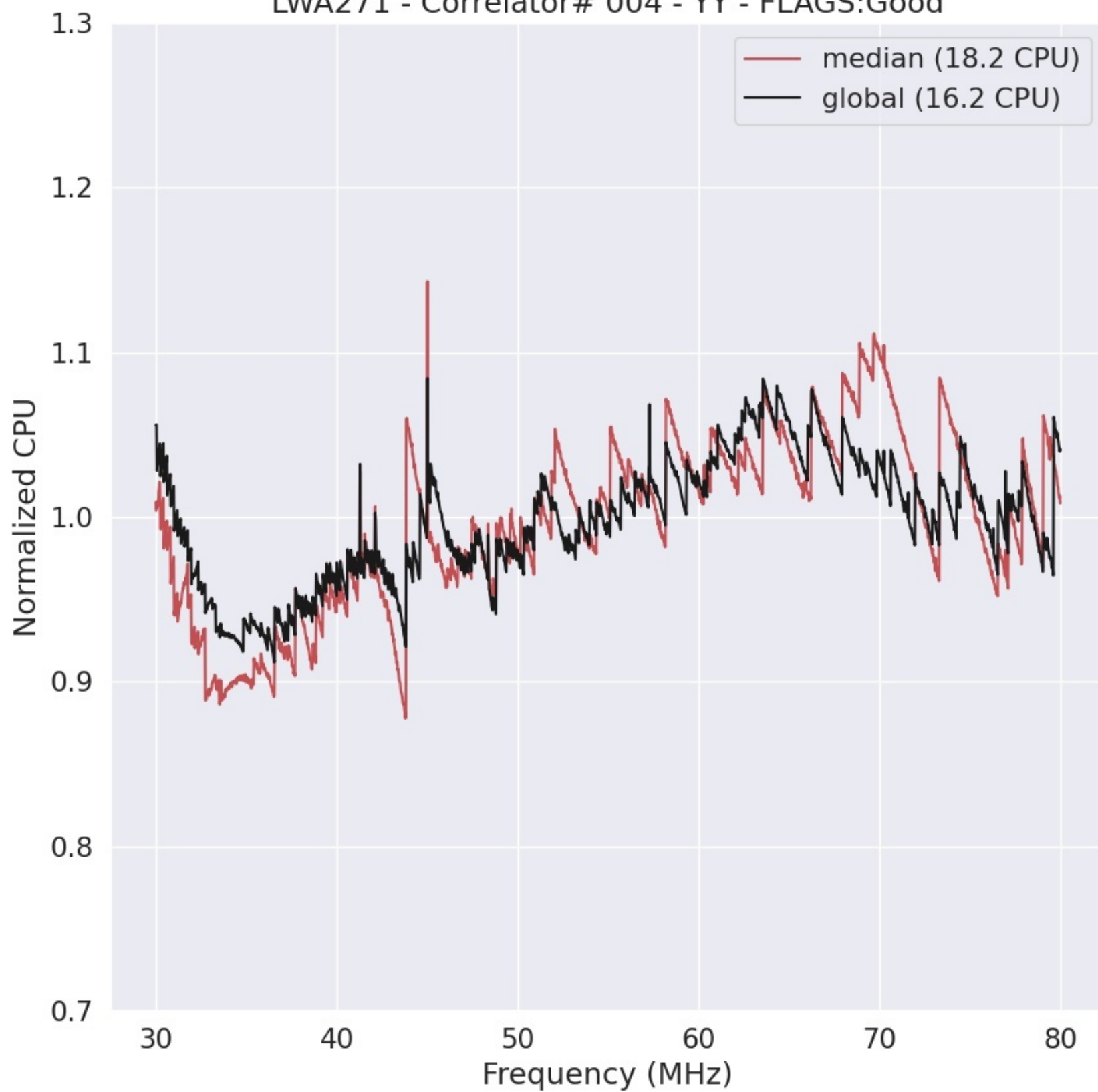
LWA271 - Correlator# 004 - YY - FLAGS:Good
