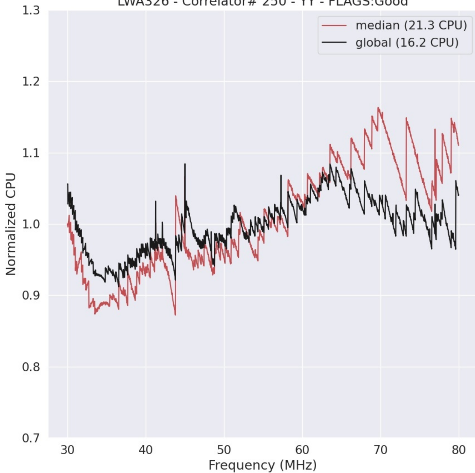
LWA326 - Correlator# 250 - YY - FLAGS:Good
