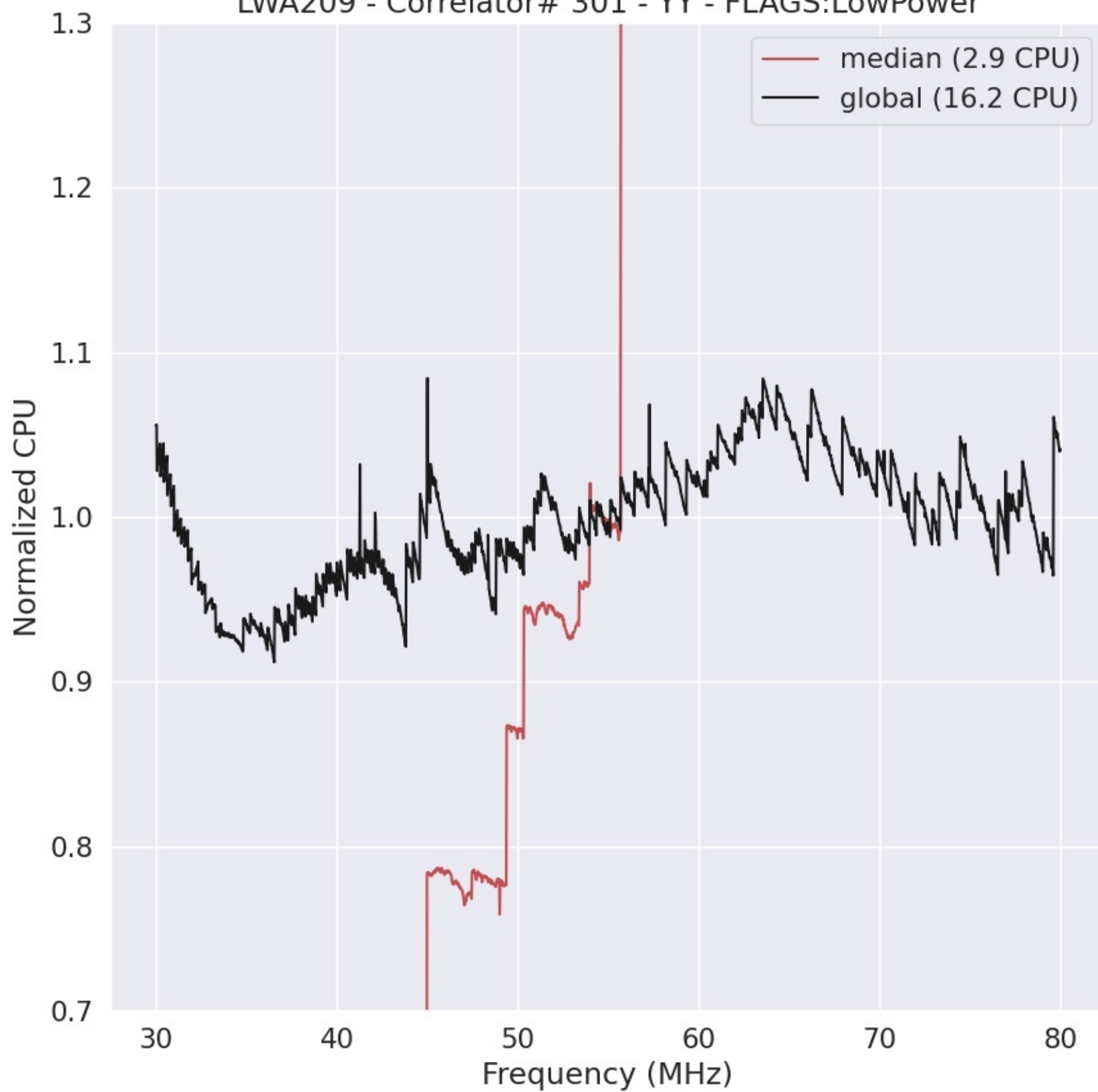
LWA209 - Correlator# 301 - YY - FLAGS:LowPower
