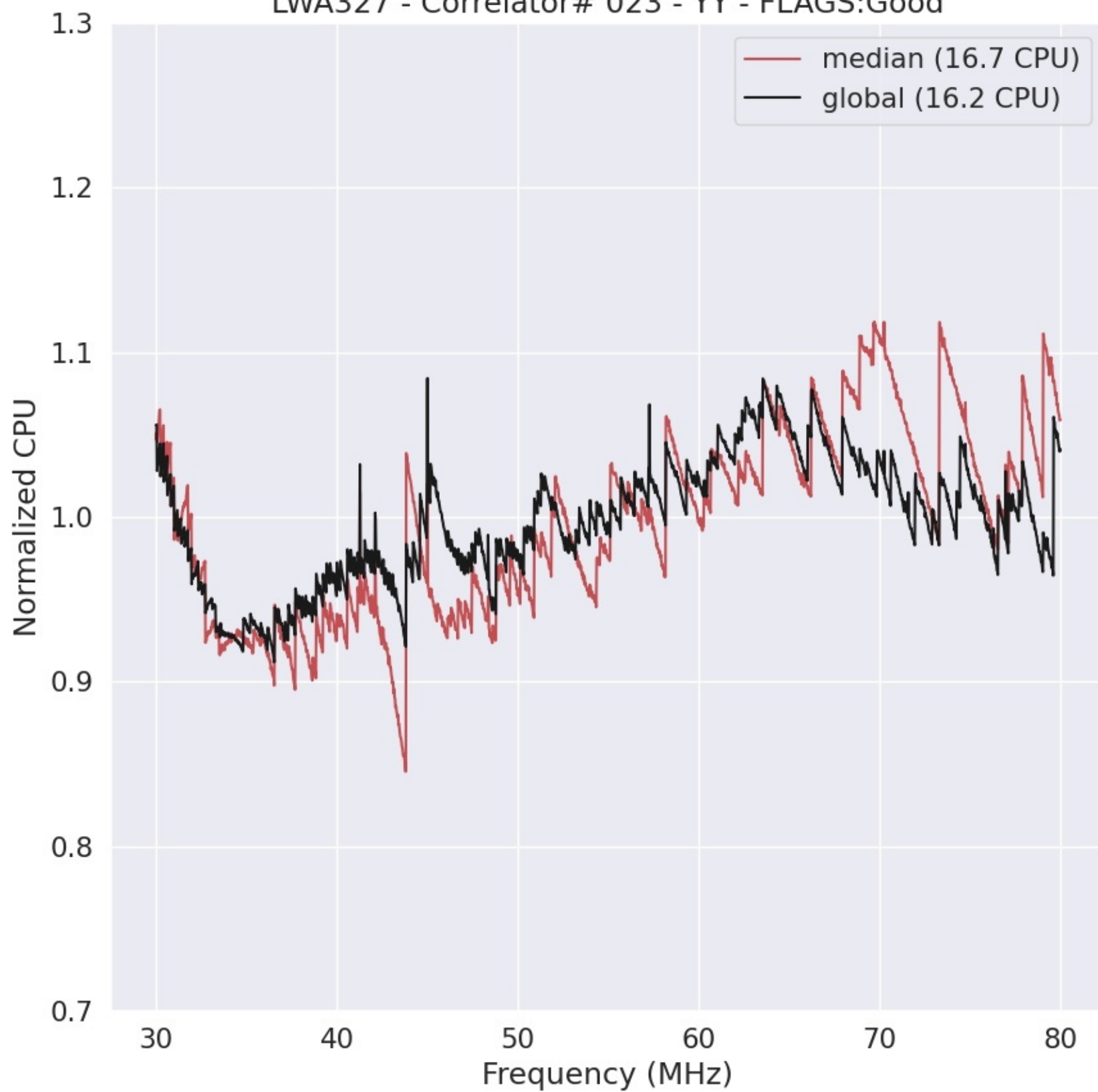
LWA327 - Correlator# 023 - YY - FLAGS:Good
