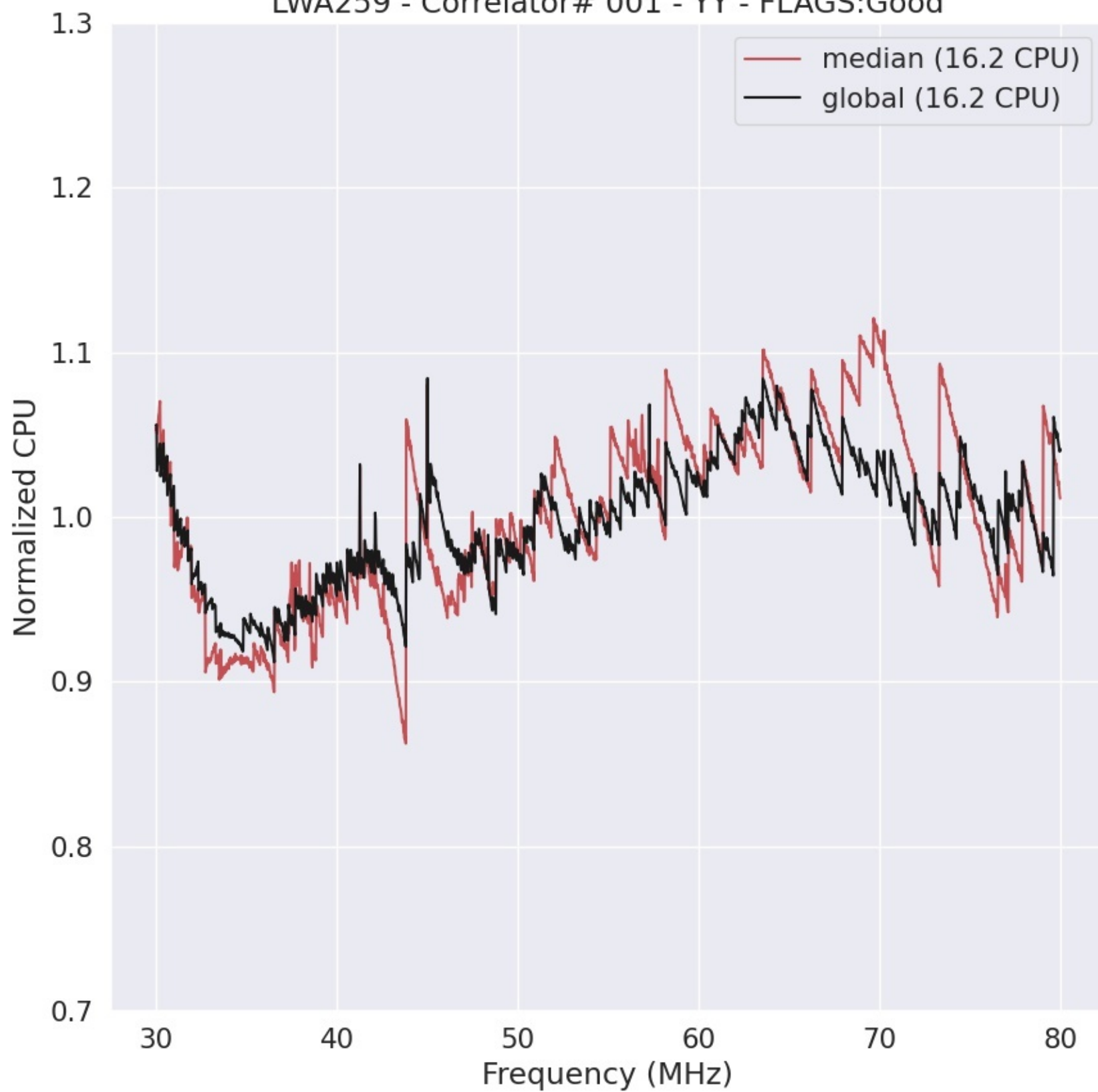
LWA259 - Correlator# 001 - YY - FLAGS:Good
