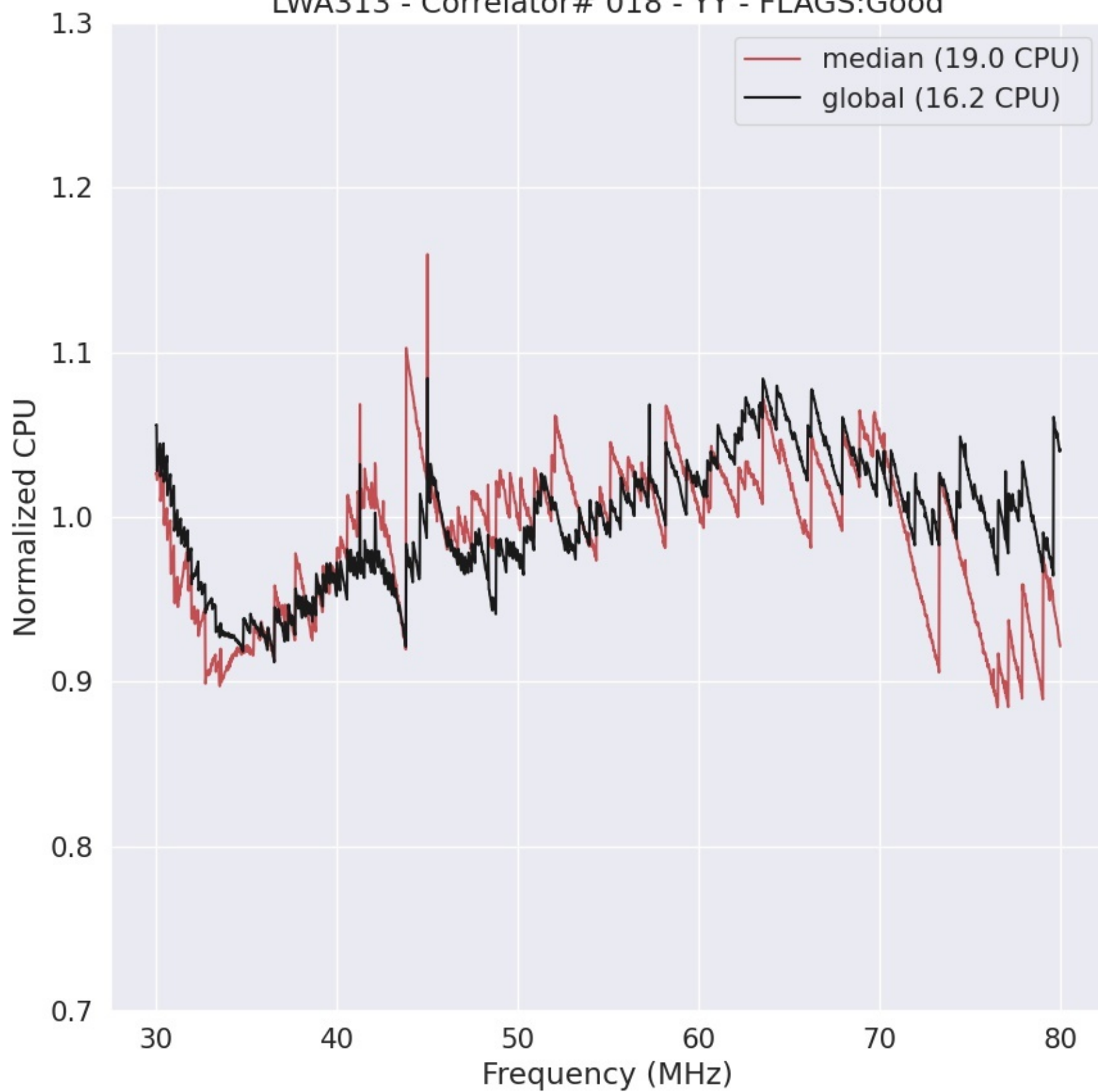
LWA313 - Correlator# 018 - YY - FLAGS:Good
