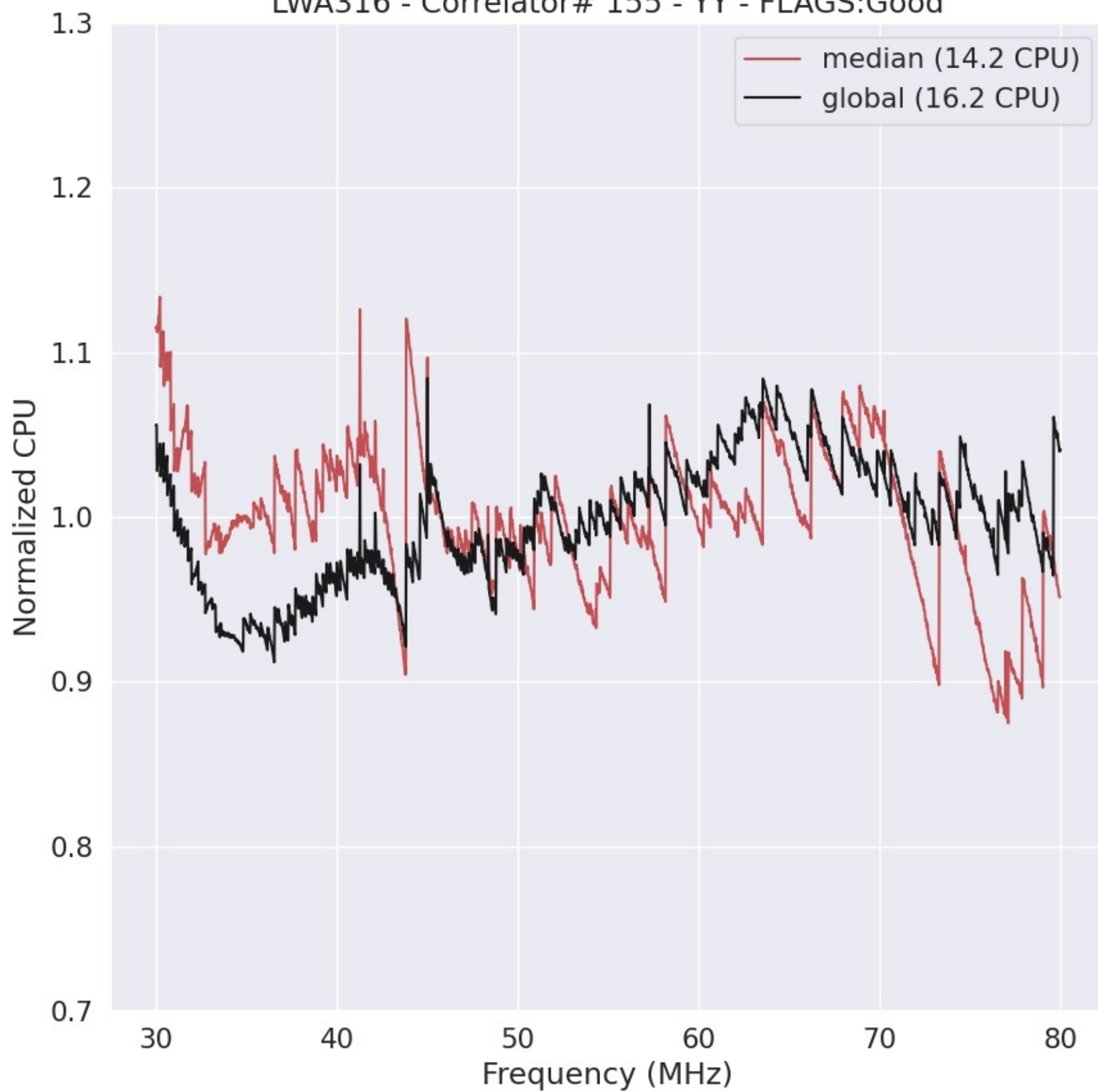
LWA316 - Correlator# 155 - YY - FLAGS:Good
