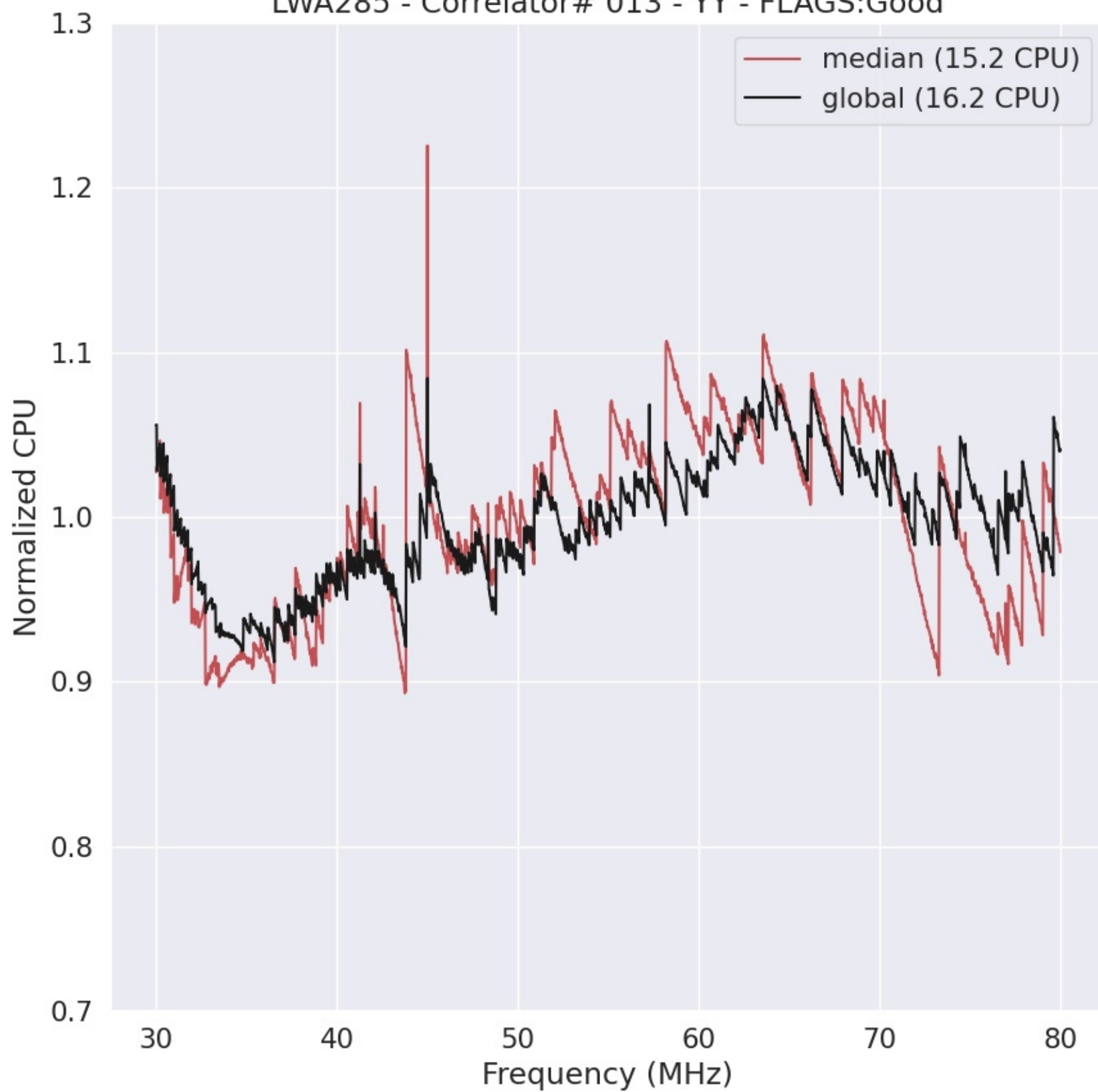
LWA285 - Correlator# 013 - YY - FLAGS:Good
