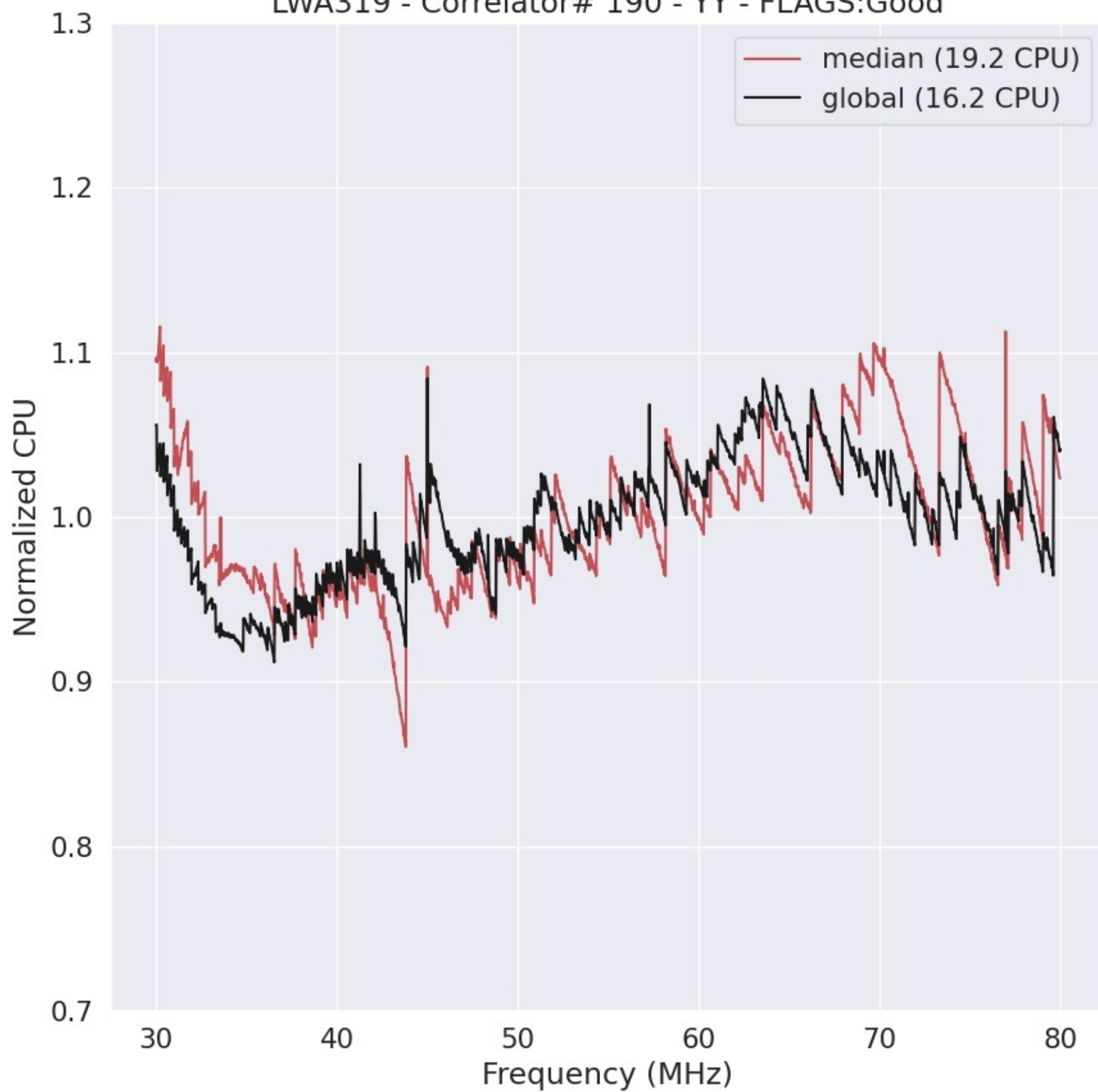
LWA319 - Correlator# 190 - YY - FLAGS:Good
