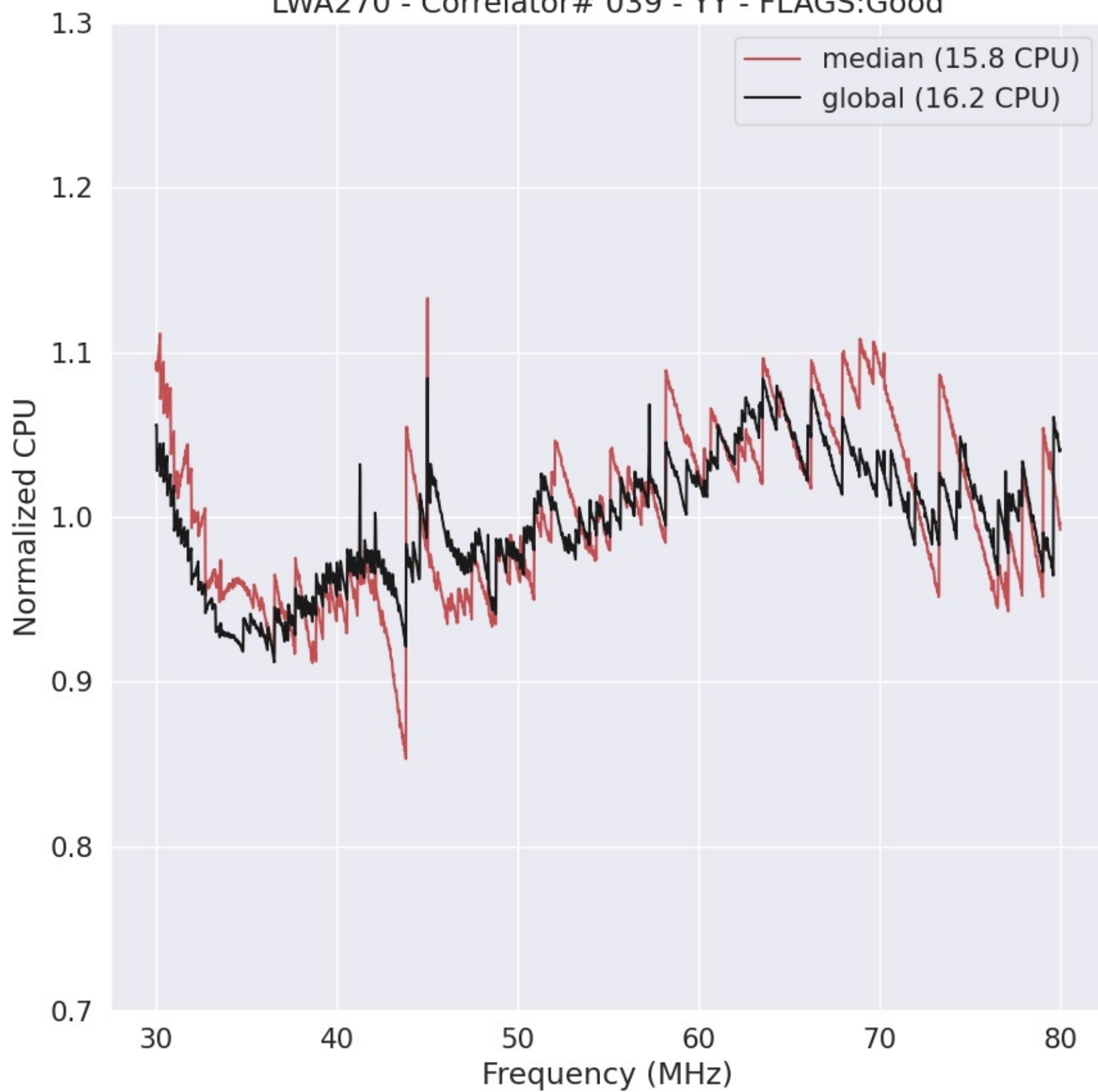
LWA270 - Correlator# 039 - YY - FLAGS:Good
