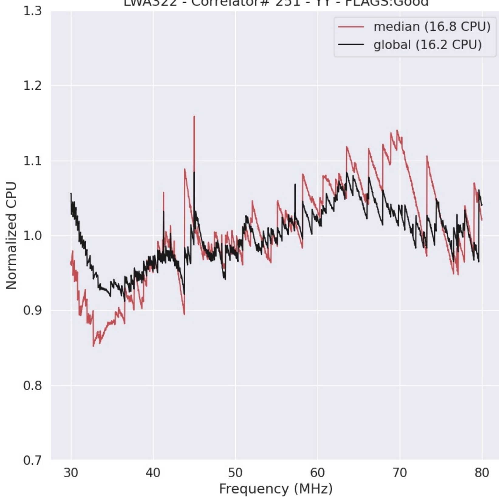
LWA322 - Correlator# 251 - YY - FLAGS:Good
