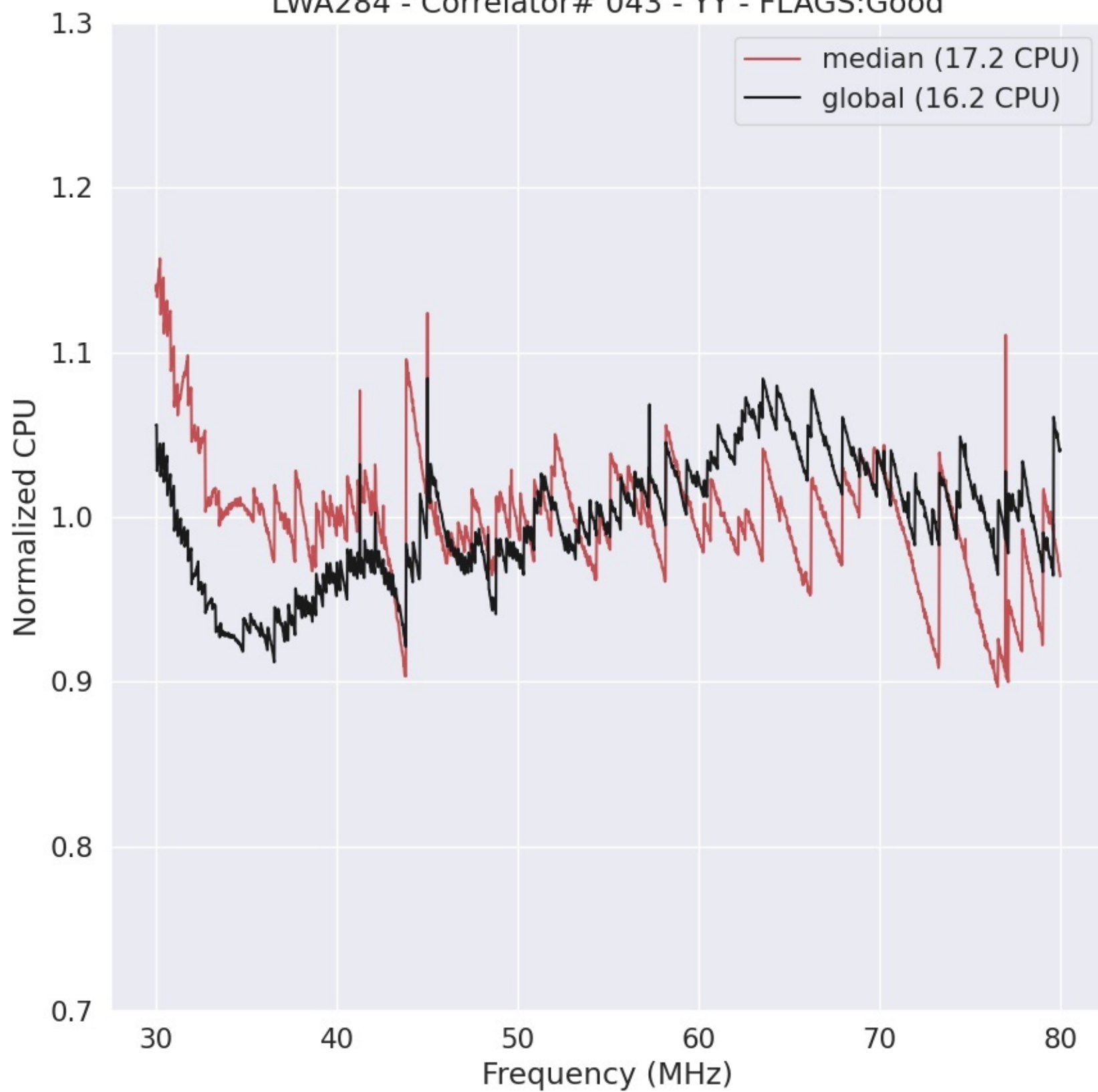
LWA284 - Correlator# 043 - YY - FLAGS:Good
