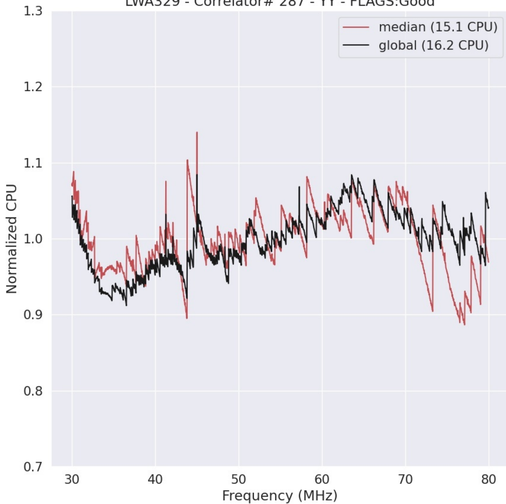
LWA329 - Correlator# 287 - YY - FLAGS:Good
