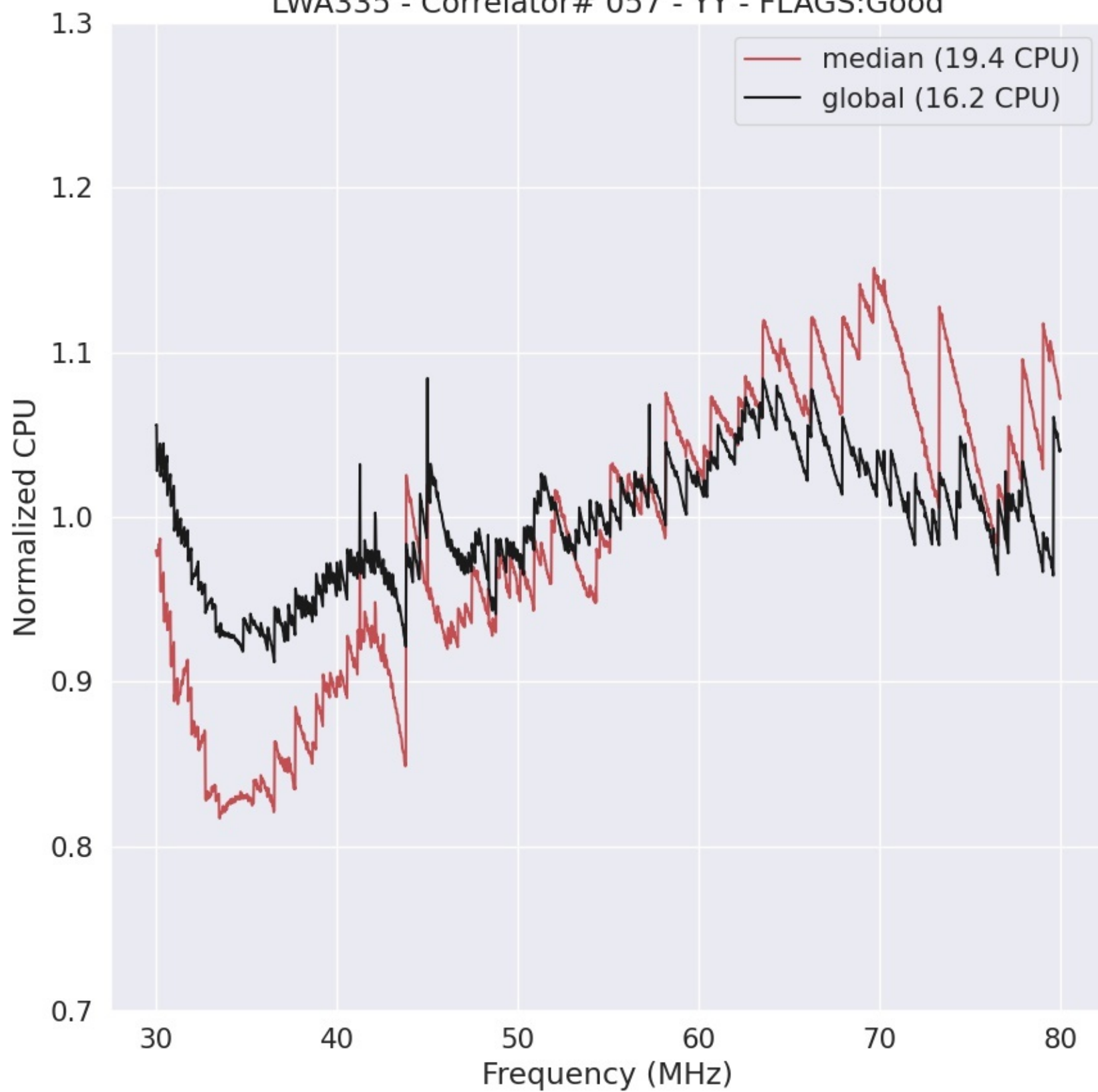
LWA335 - Correlator# 057 - YY - FLAGS:Good
