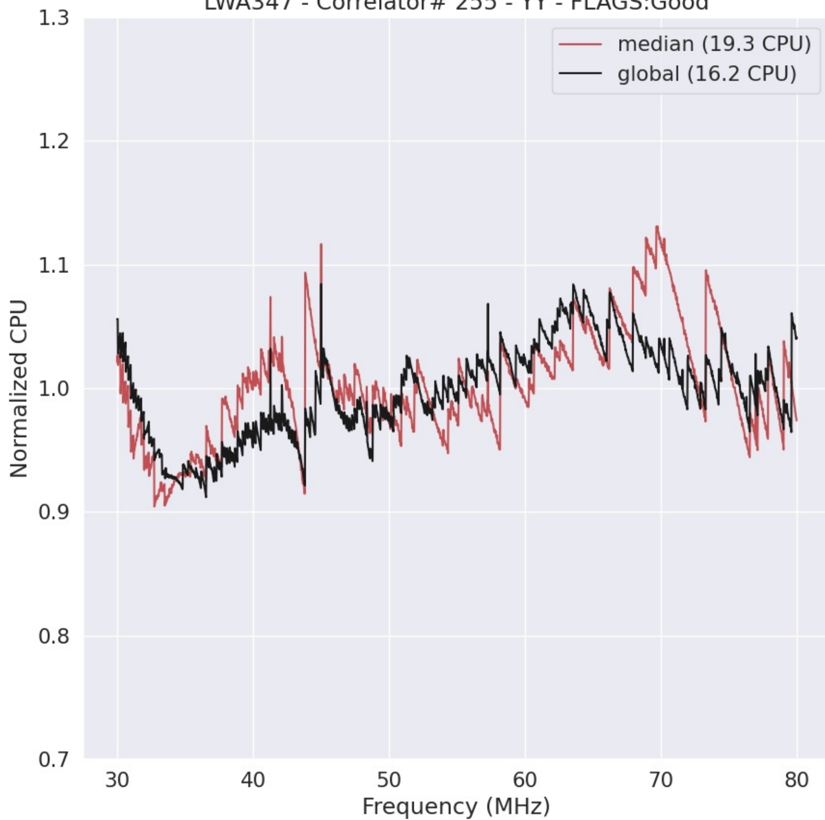
LWA347 - Correlator# 255 - YY - FLAGS:Good
