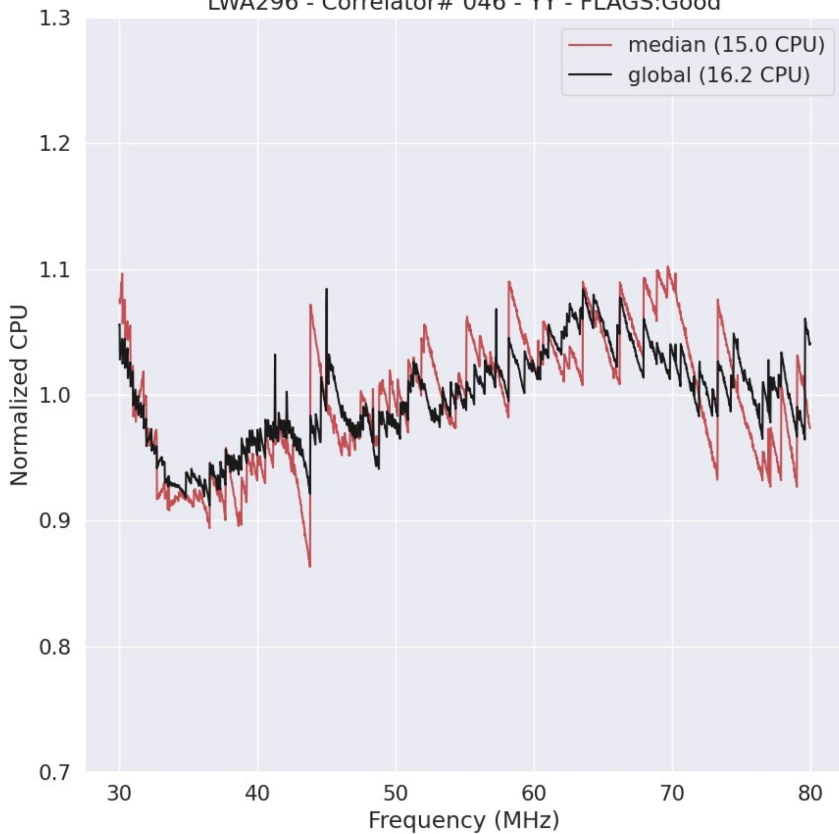
LWA296 - Correlator# 046 - YY - FLAGS:Good
