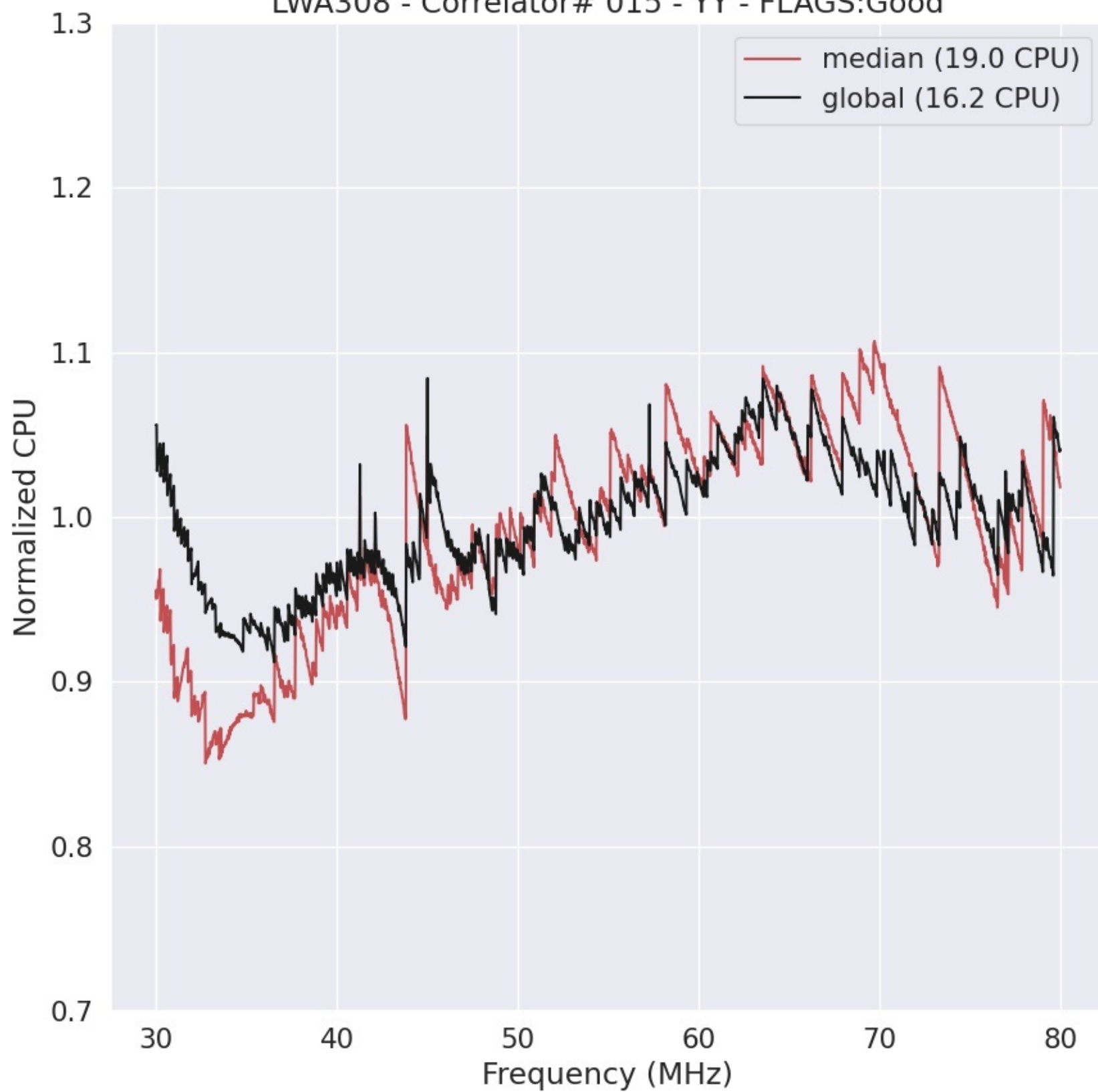
LWA308 - Correlator# 015 - YY - FLAGS:Good
