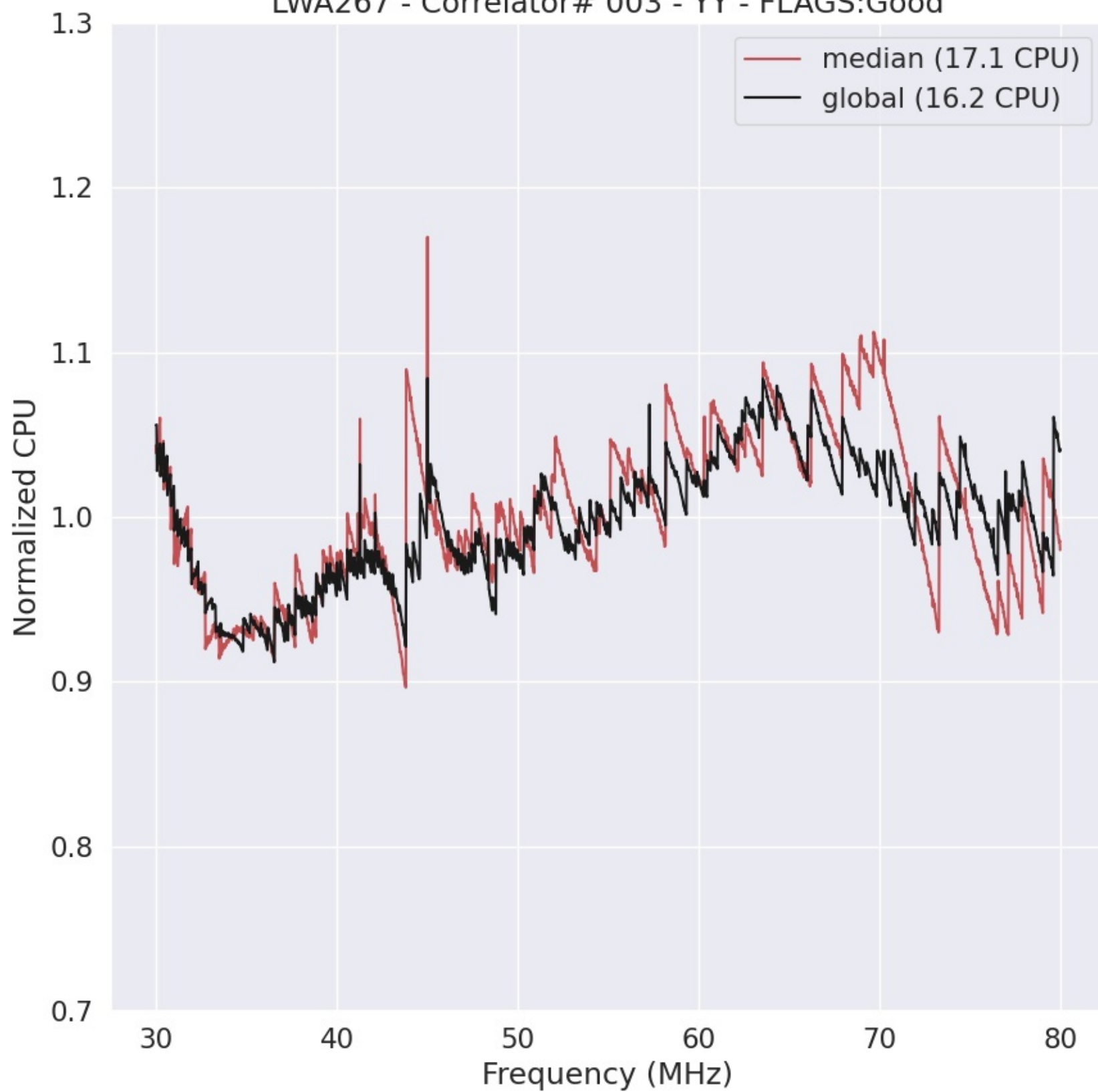
LWA267 - Correlator# 003 - YY - FLAGS:Good
