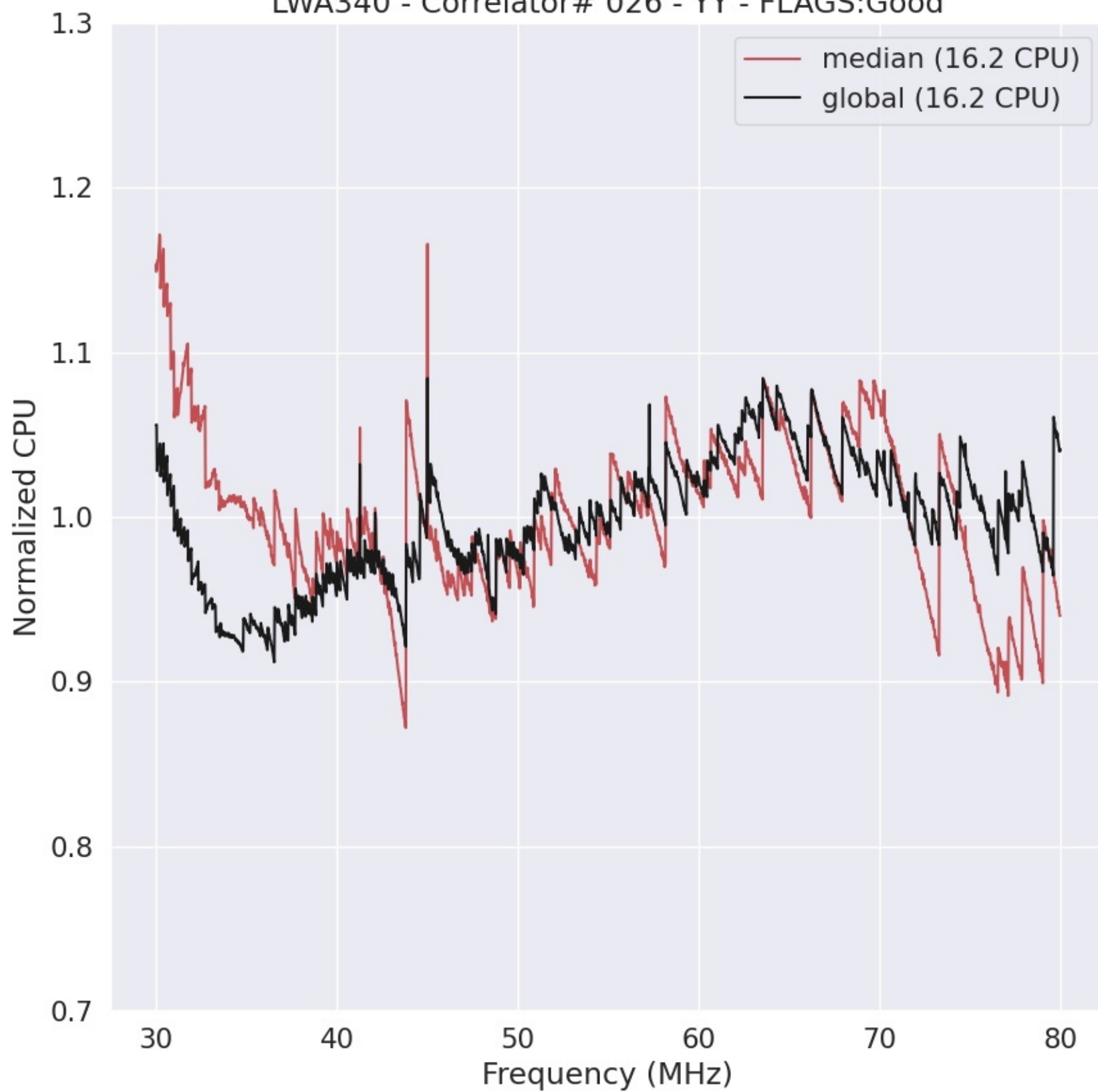
LWA340 - Correlator# 026 - YY - FLAGS:Good
