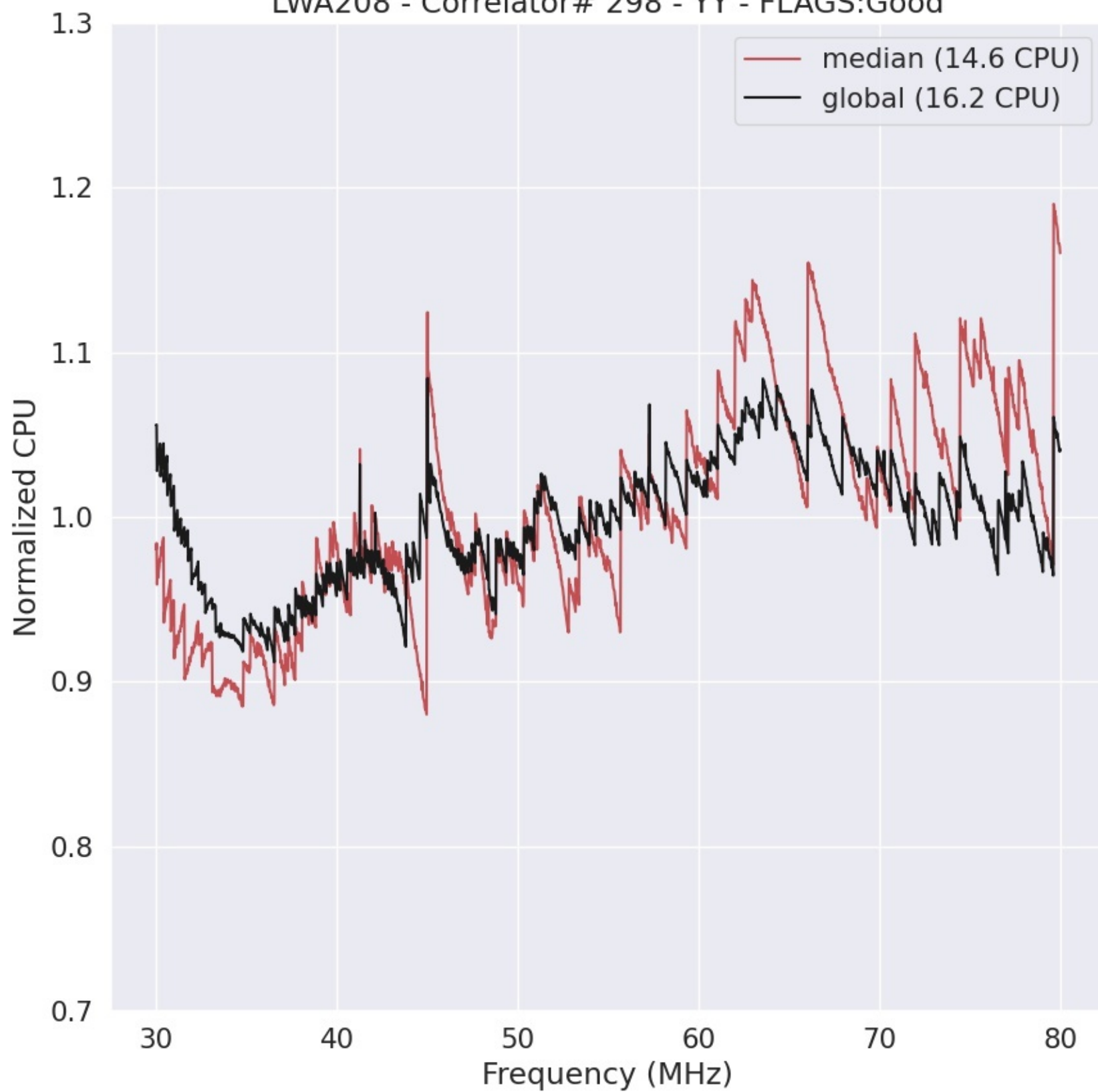
LWA208 - Correlator# 298 - YY - FLAGS:Good
