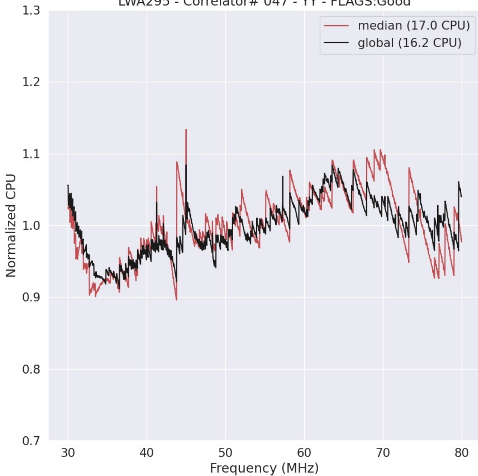
LWA295 - Correlator# 047 - YY - FLAGS:Good
