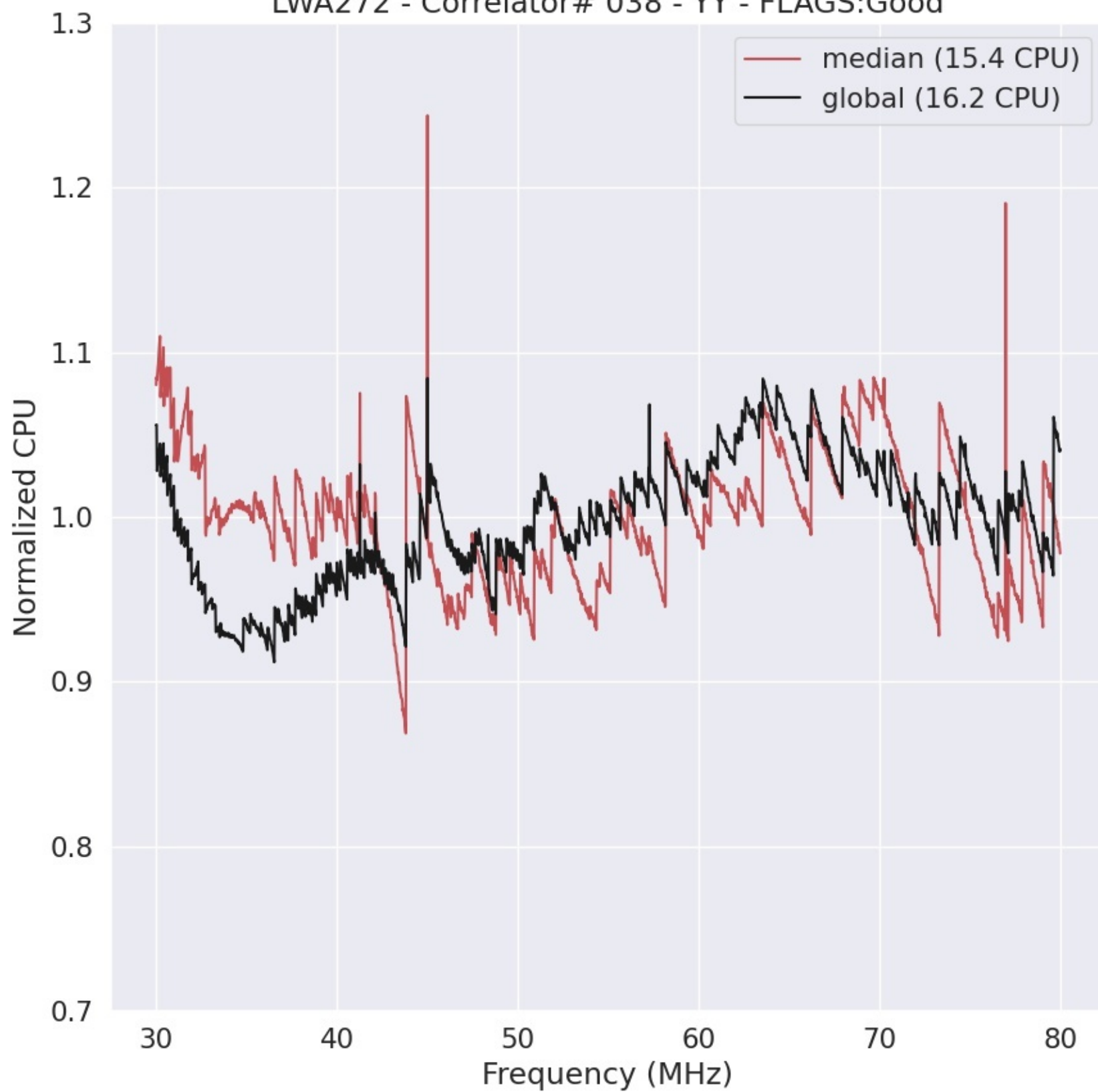
LWA272 - Correlator# 038 - YY - FLAGS:Good
