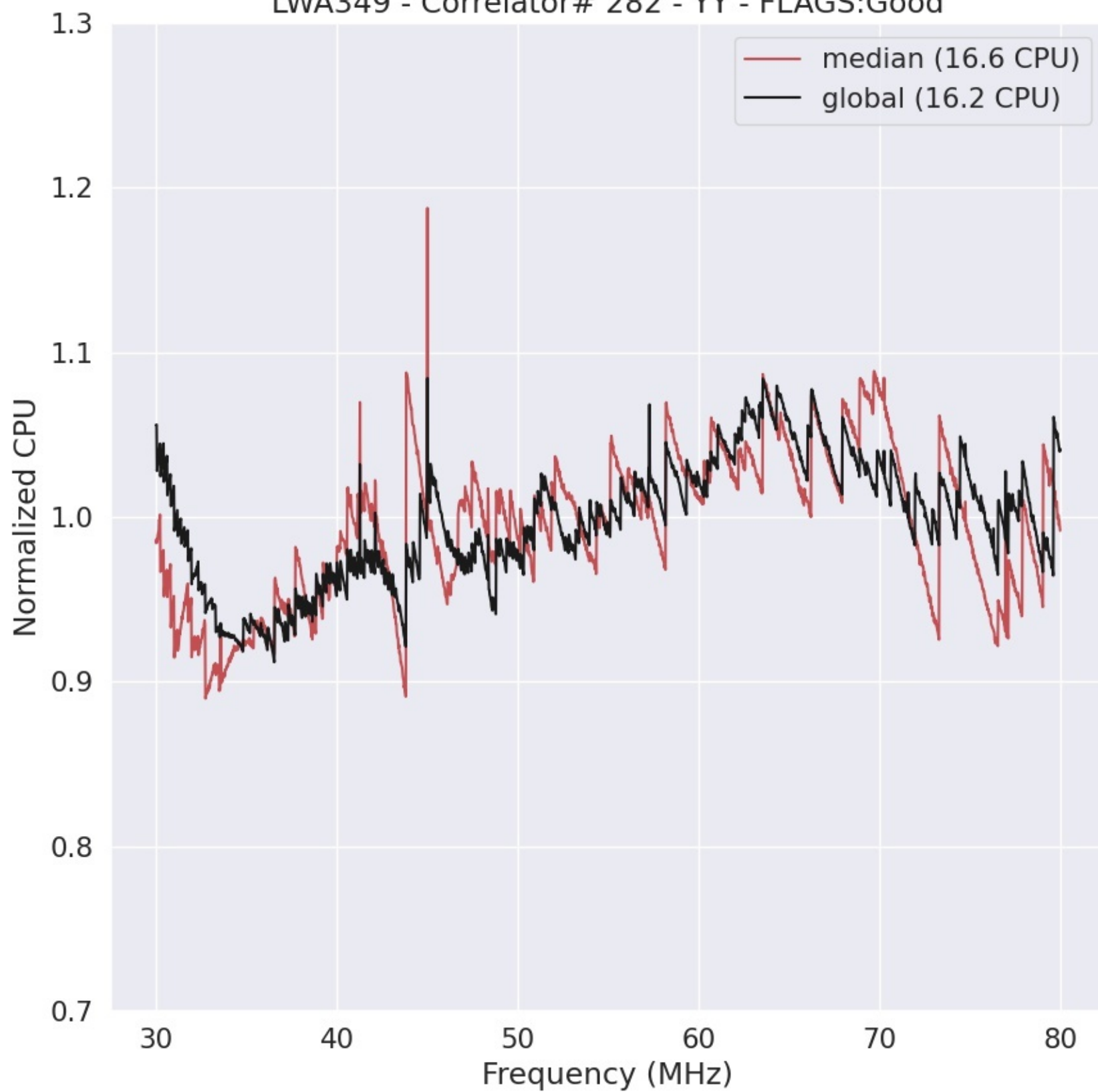
LWA349 - Correlator# 282 - YY - FLAGS:Good
