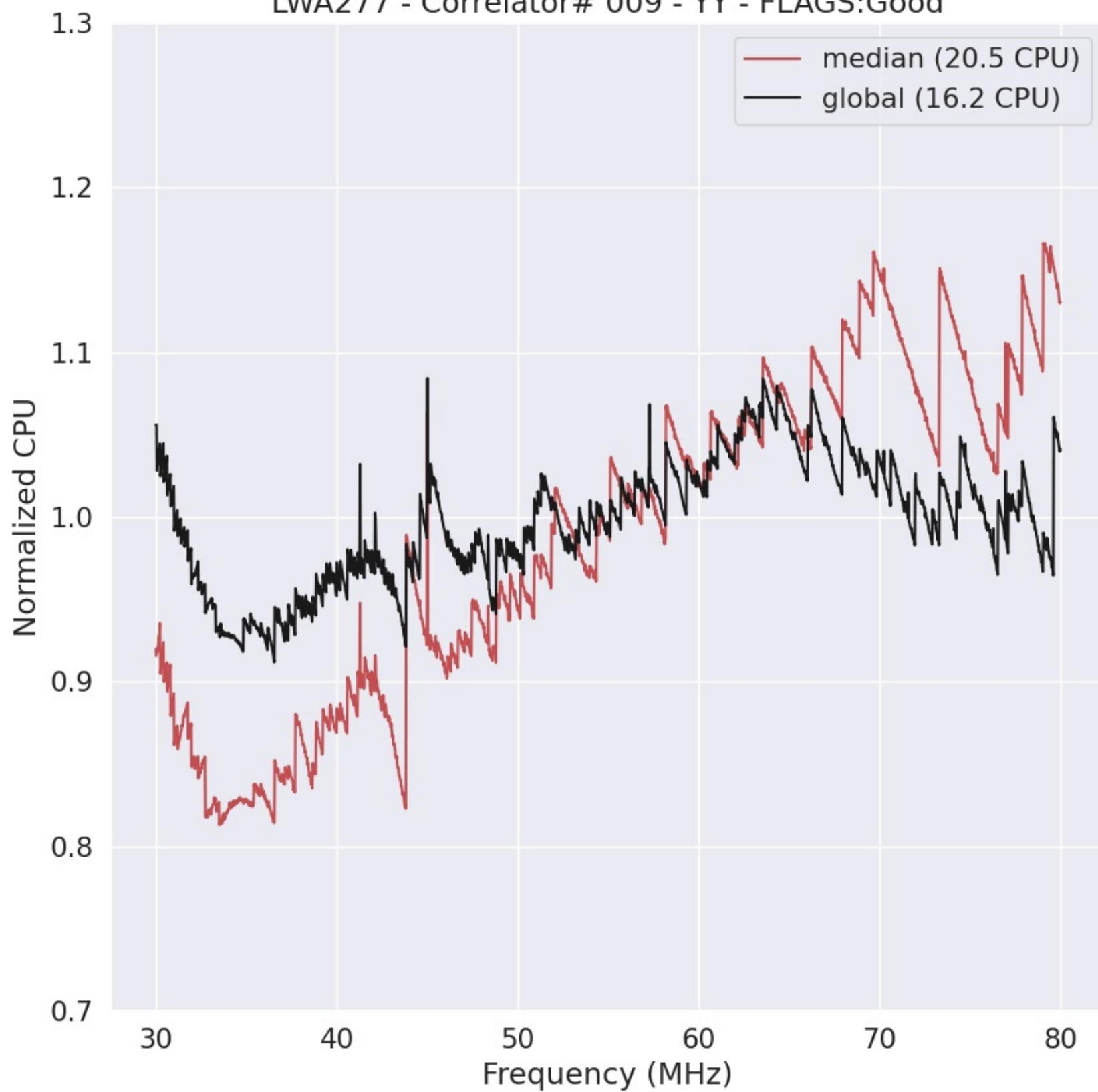
LWA277 - Correlator# 009 - YY - FLAGS:Good
