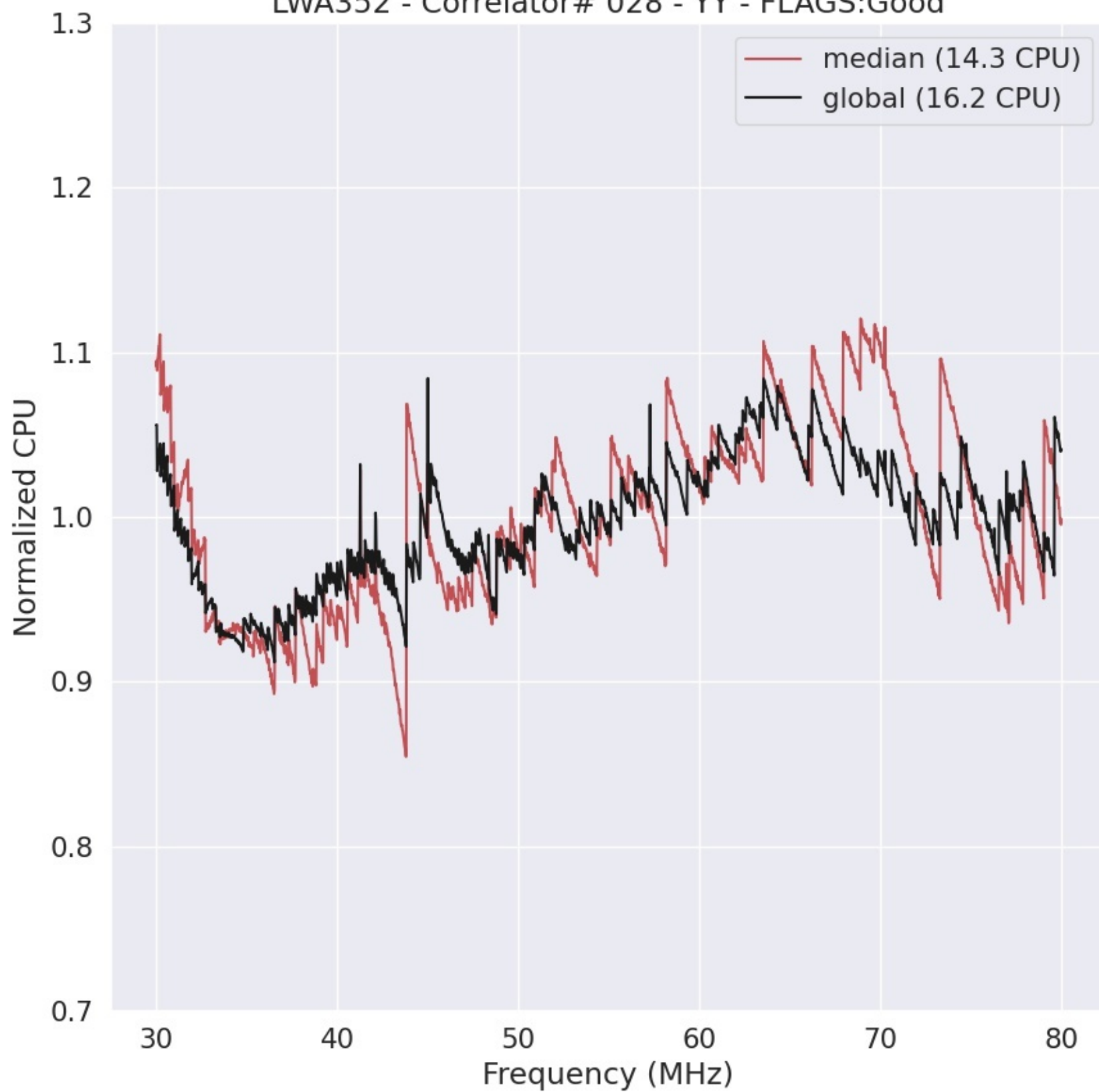
LWA352 - Correlator# 028 - YY - FLAGS:Good
