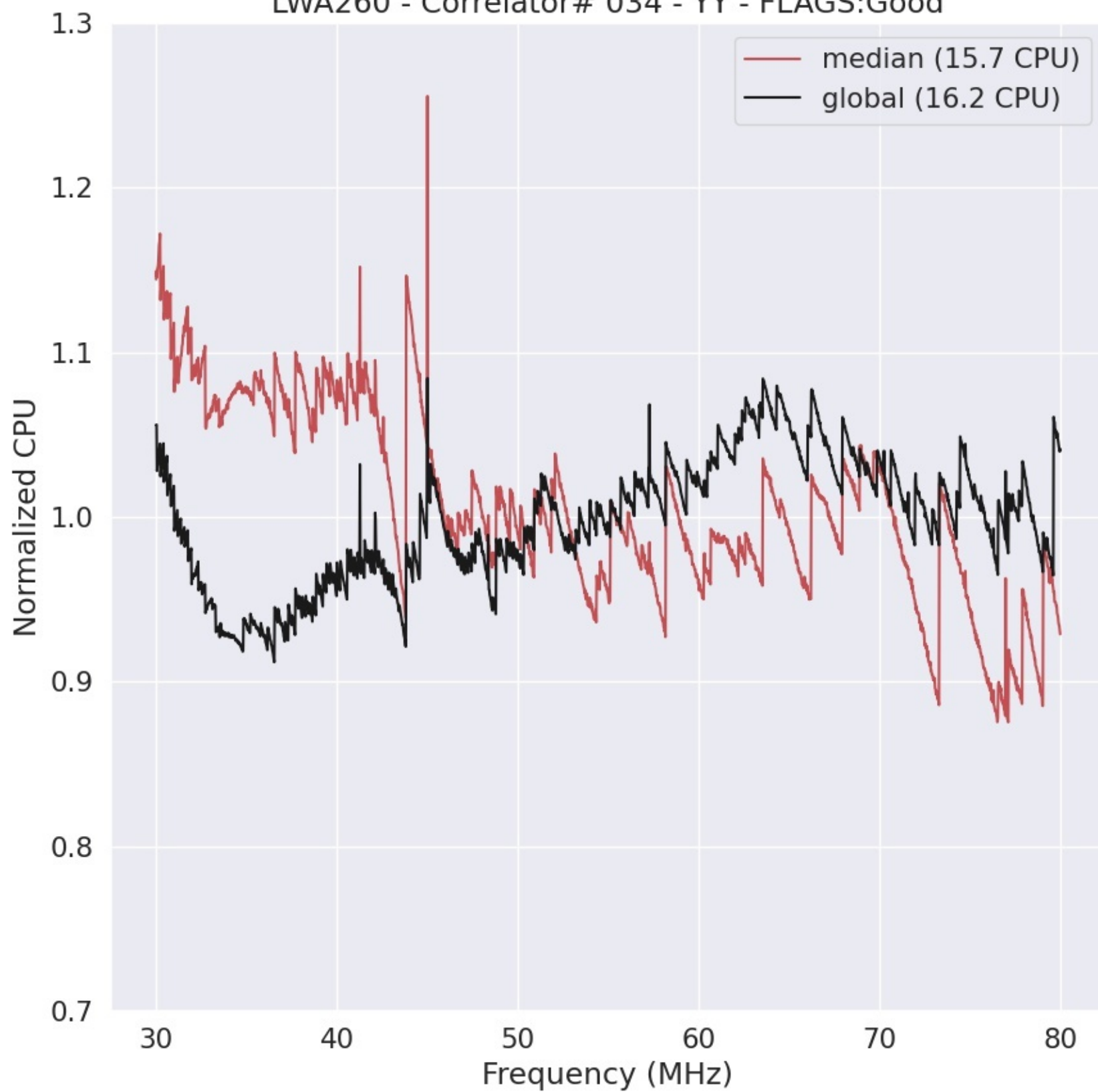
LWA260 - Correlator# 034 - YY - FLAGS:Good
