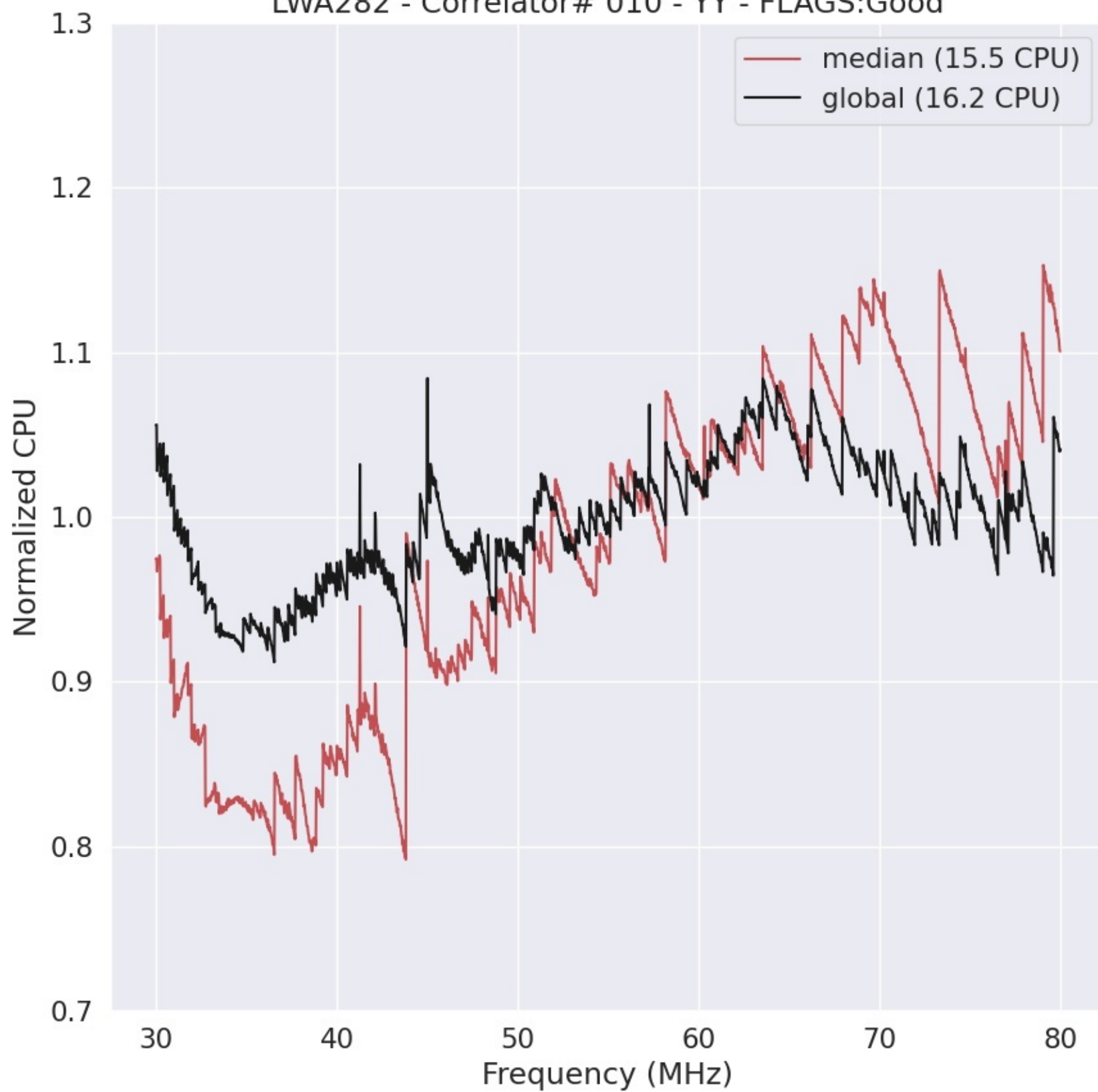
LWA282 - Correlator# 010 - YY - FLAGS:Good
