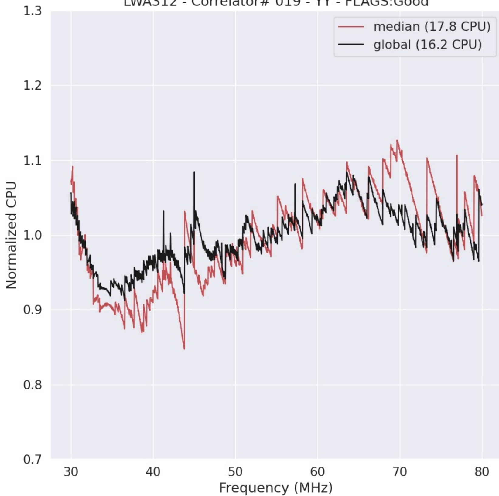
LWA312 - Correlator# 019 - YY - FLAGS:Good
