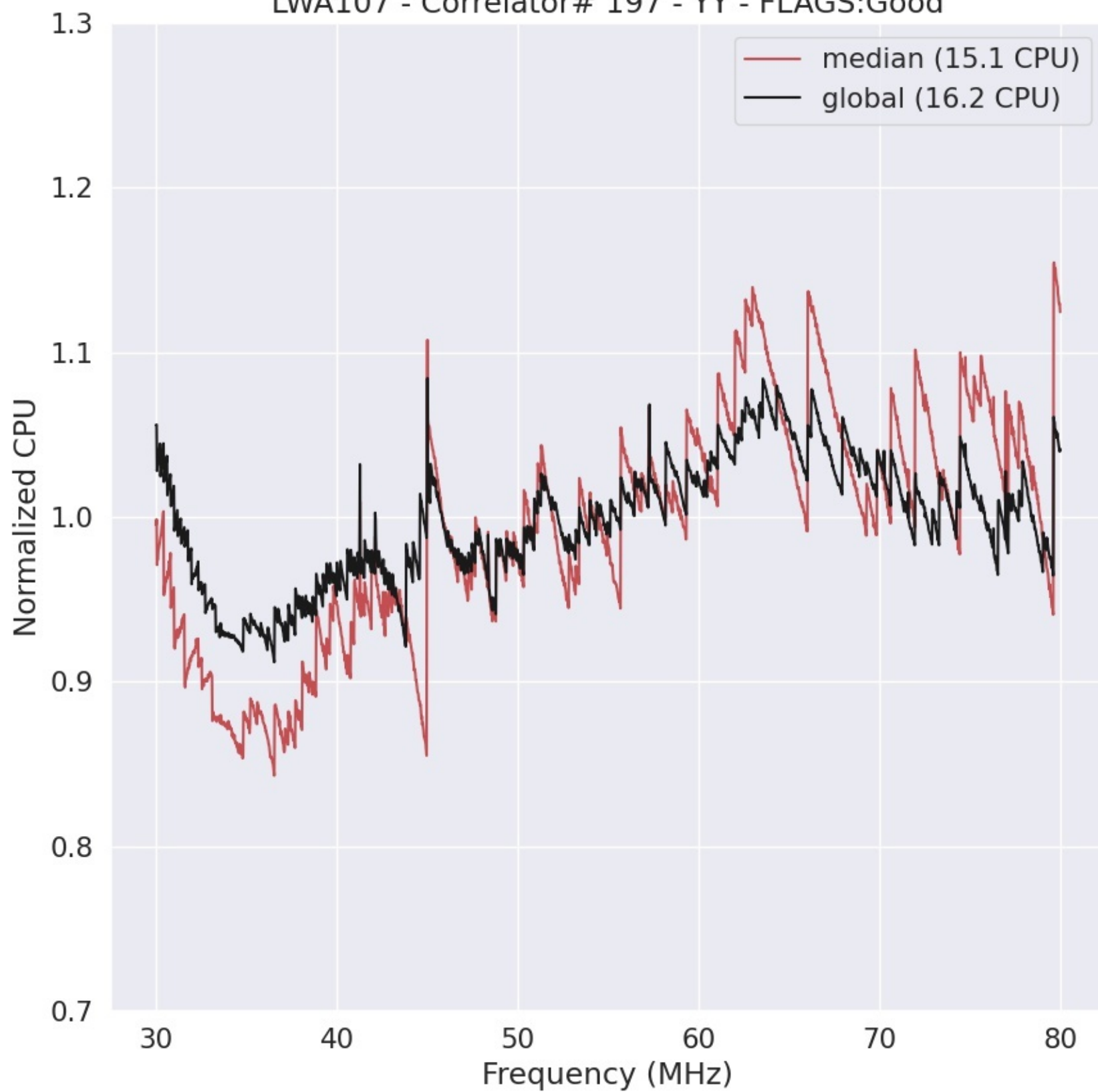
LWA107 - Correlator# 197 - YY - FLAGS:Good
