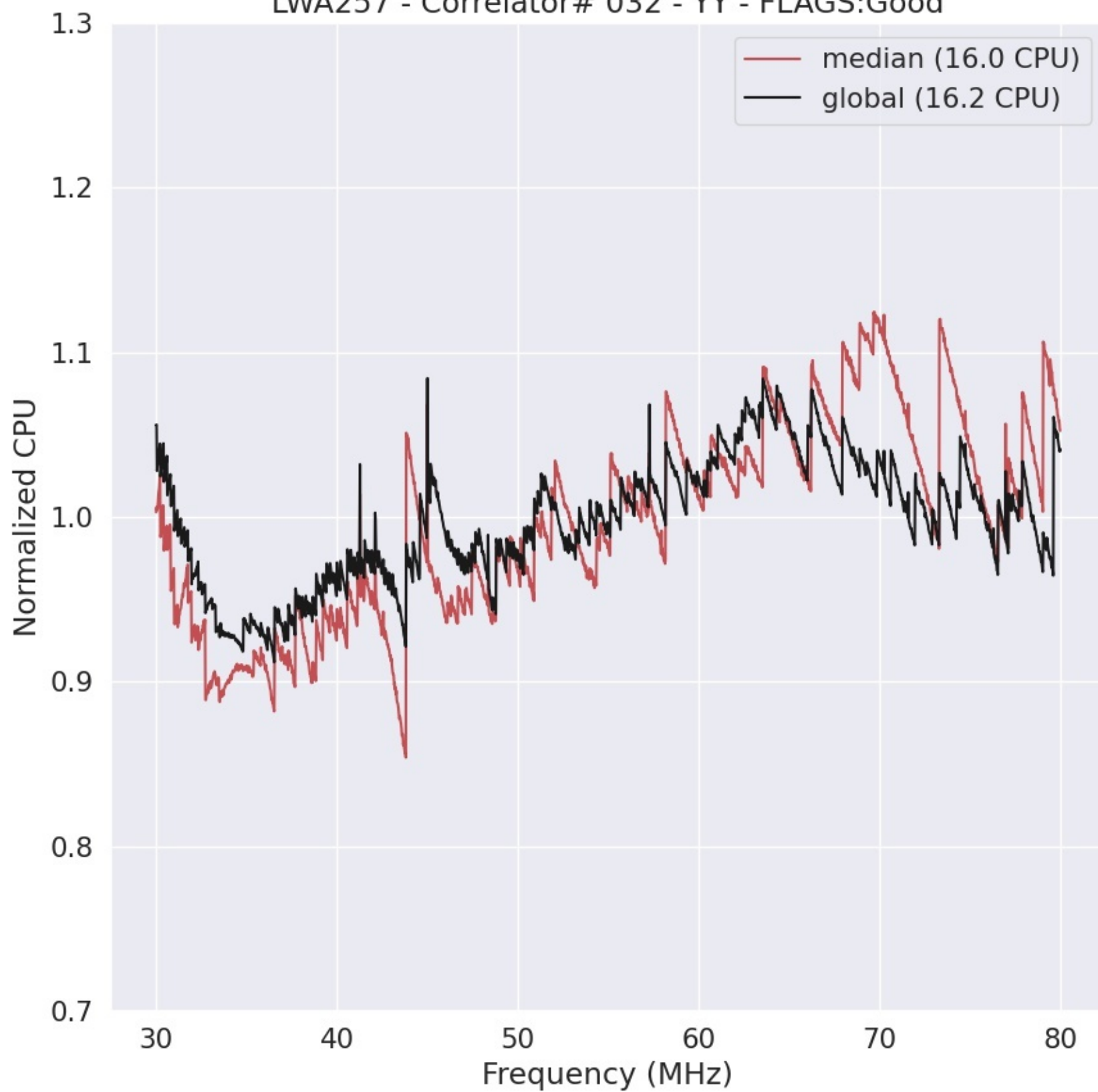
LWA257 - Correlator# 032 - YY - FLAGS:Good
