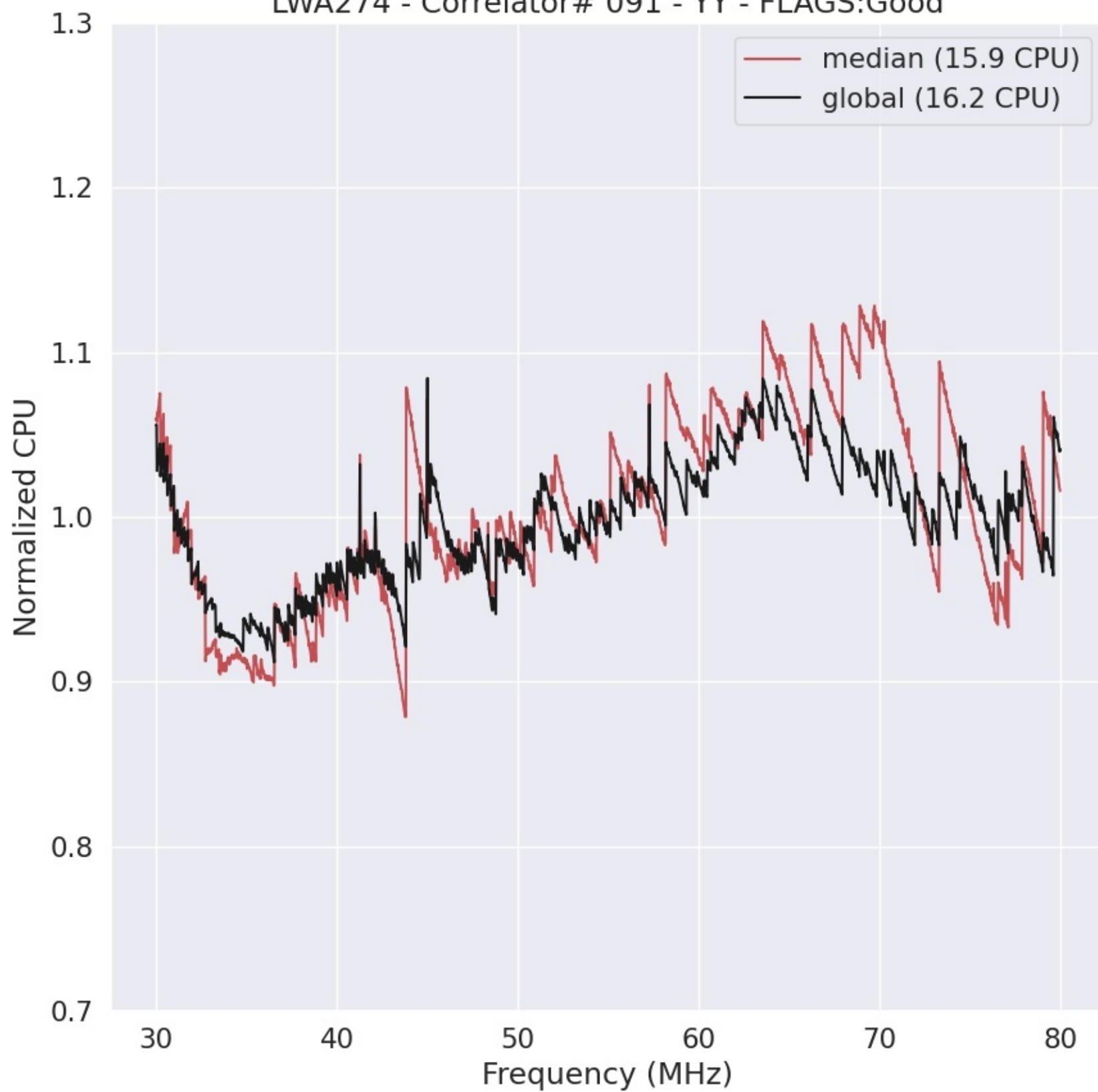
LWA274 - Correlator# 091 - YY - FLAGS:Good
