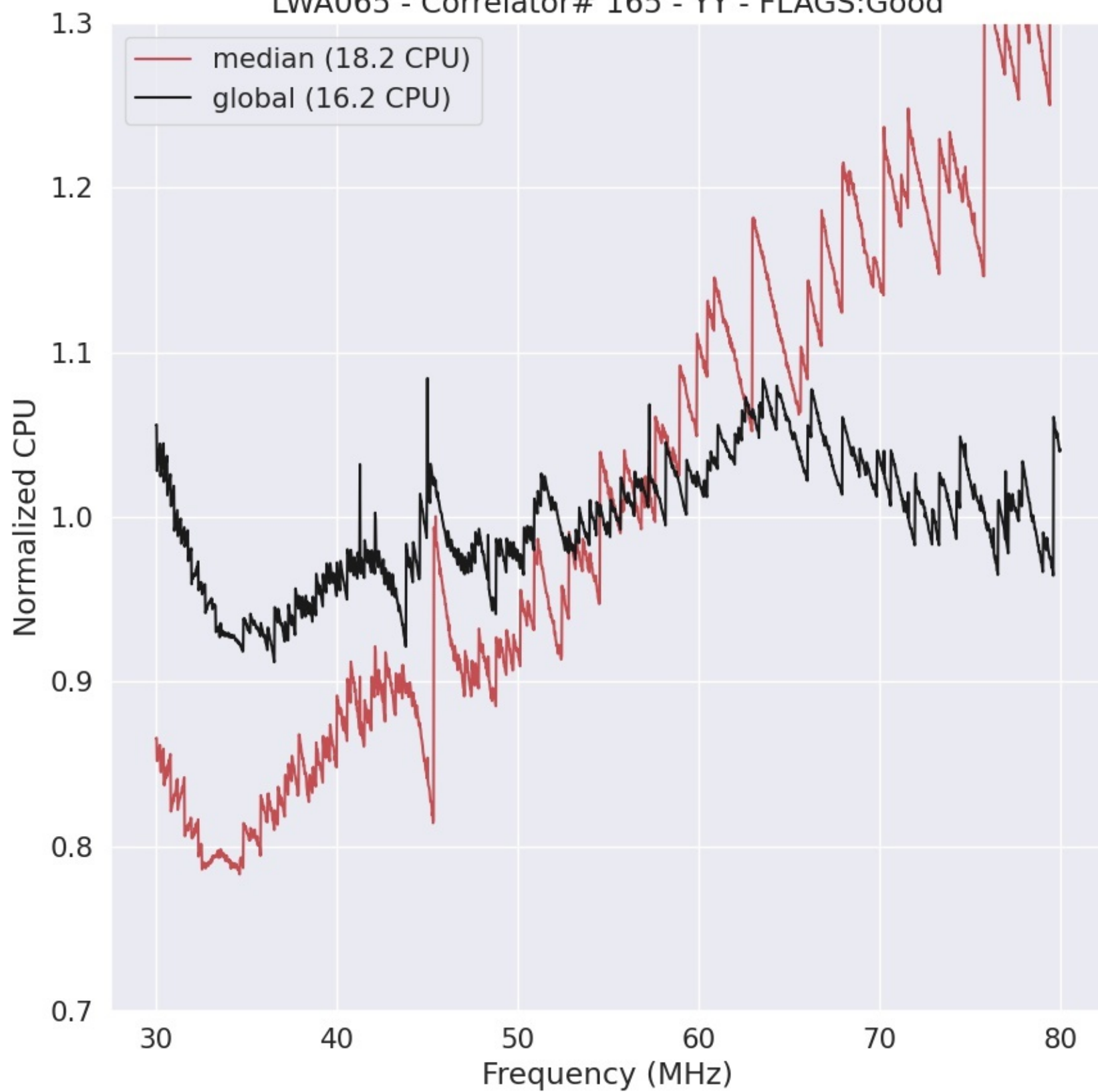
LWA065 - Correlator# 165 - YY - FLAGS:Good
