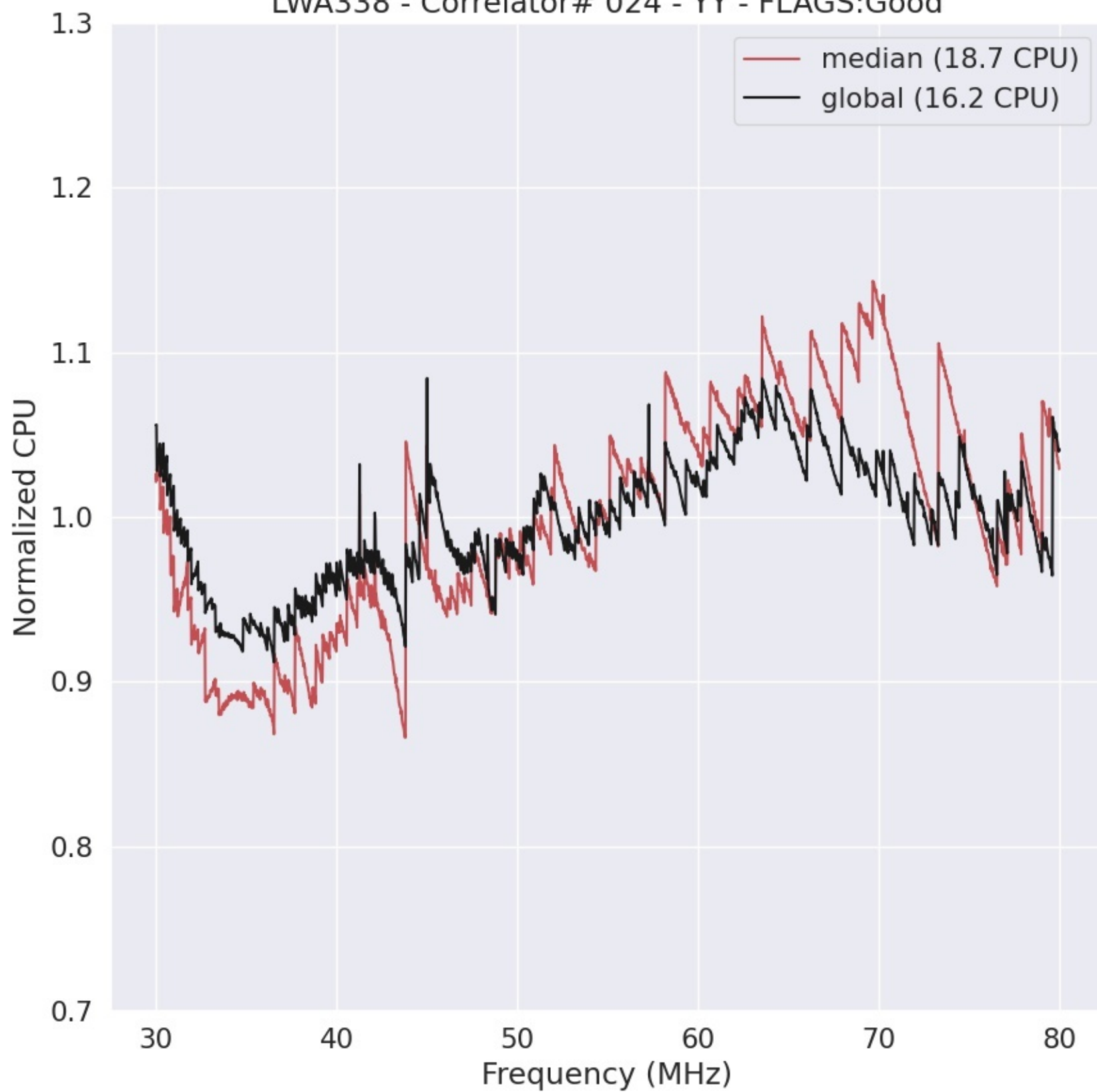
LWA338 - Correlator# 024 - YY - FLAGS:Good
