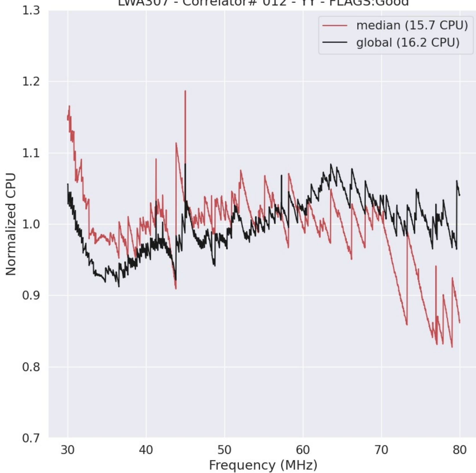
LWA307 - Correlator# 012 - YY - FLAGS:Good
