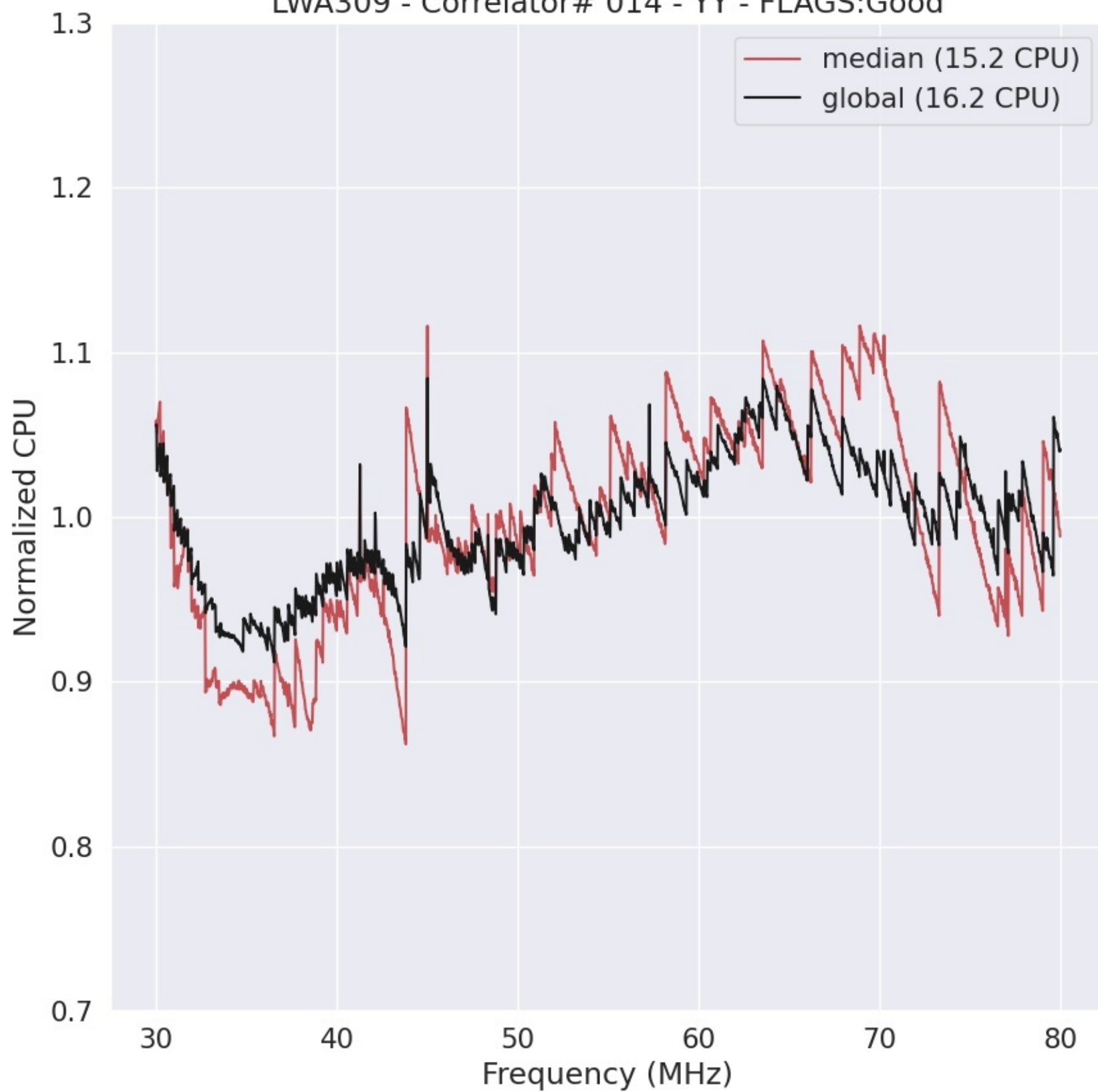
LWA309 - Correlator# 014 - YY - FLAGS:Good
