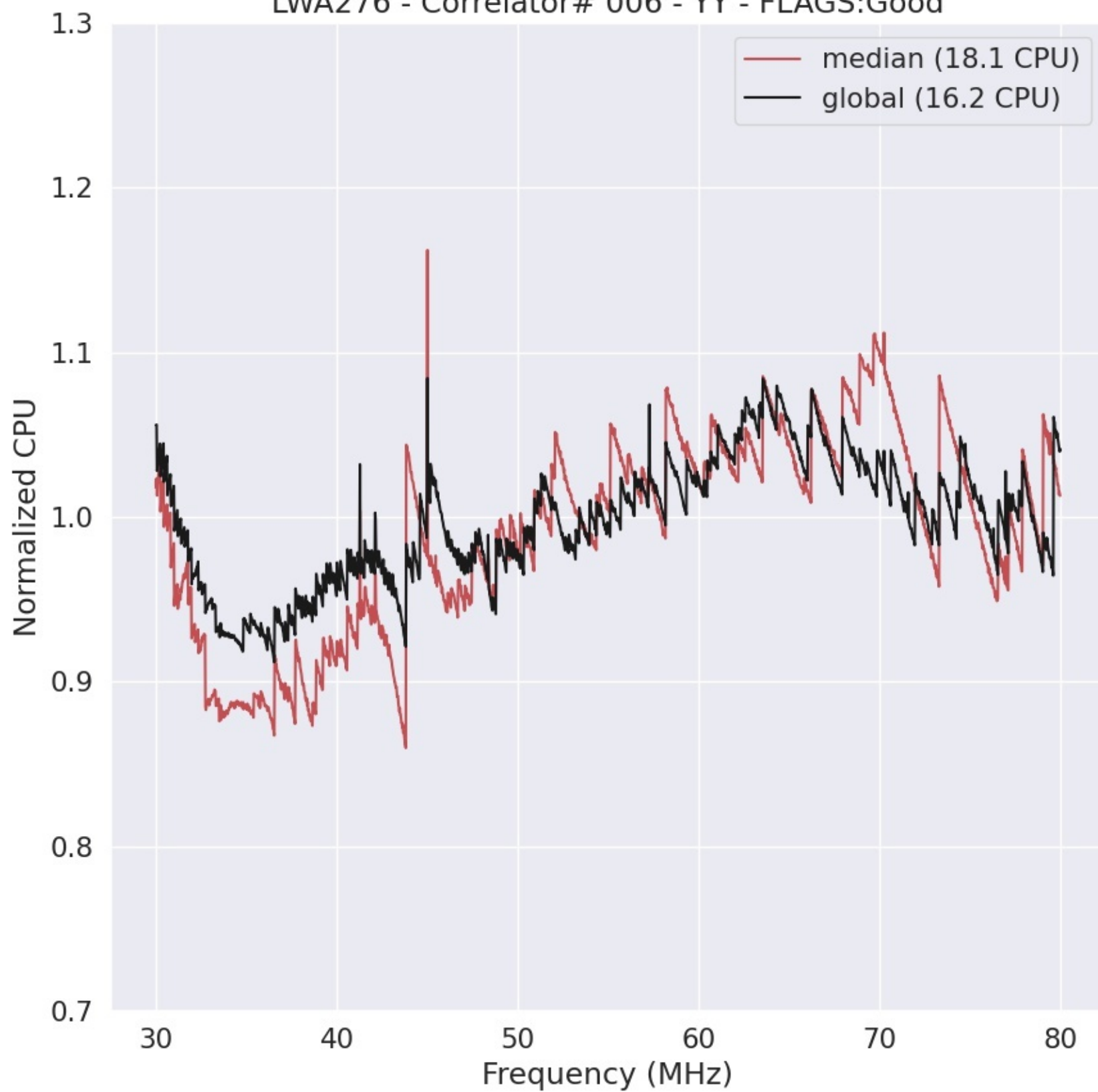
LWA276 - Correlator# 006 - YY - FLAGS:Good
