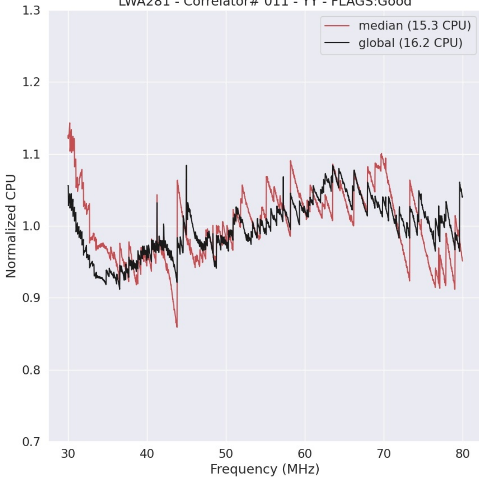
LWA281 - Correlator# 011 - YY - FLAGS:Good
