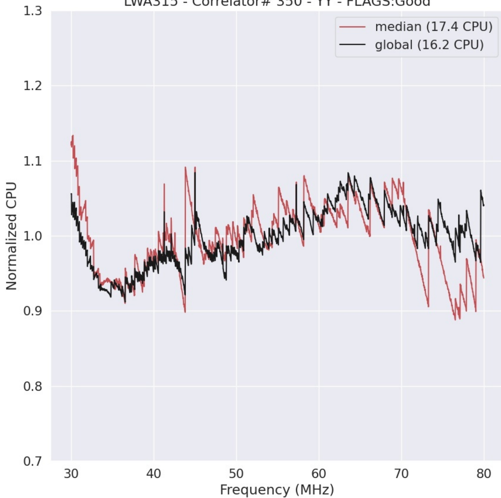
LWA315 - Correlator# 350 - YY - FLAGS:Good
