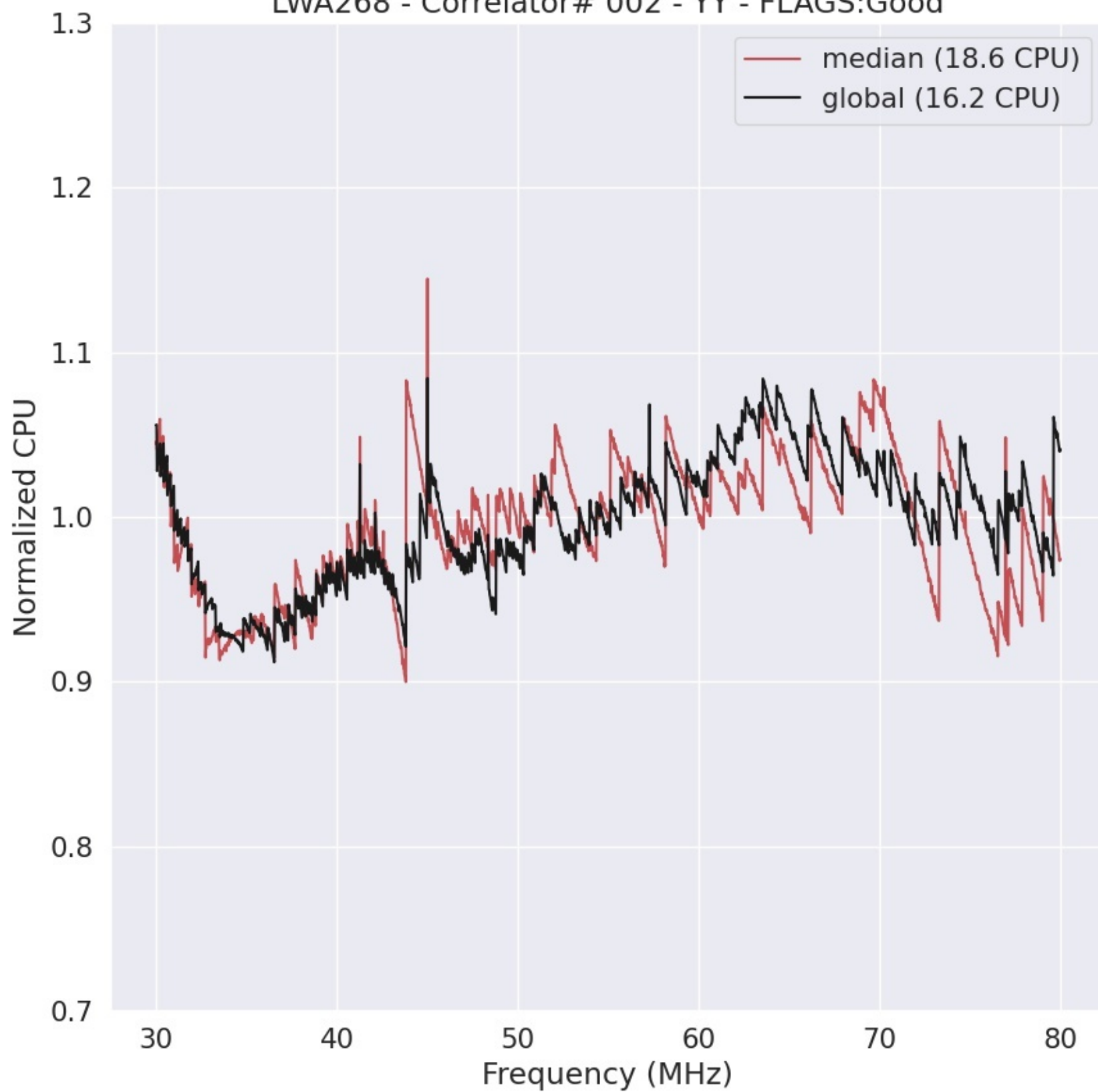
LWA268 - Correlator# 002 - YY - FLAGS:Good
