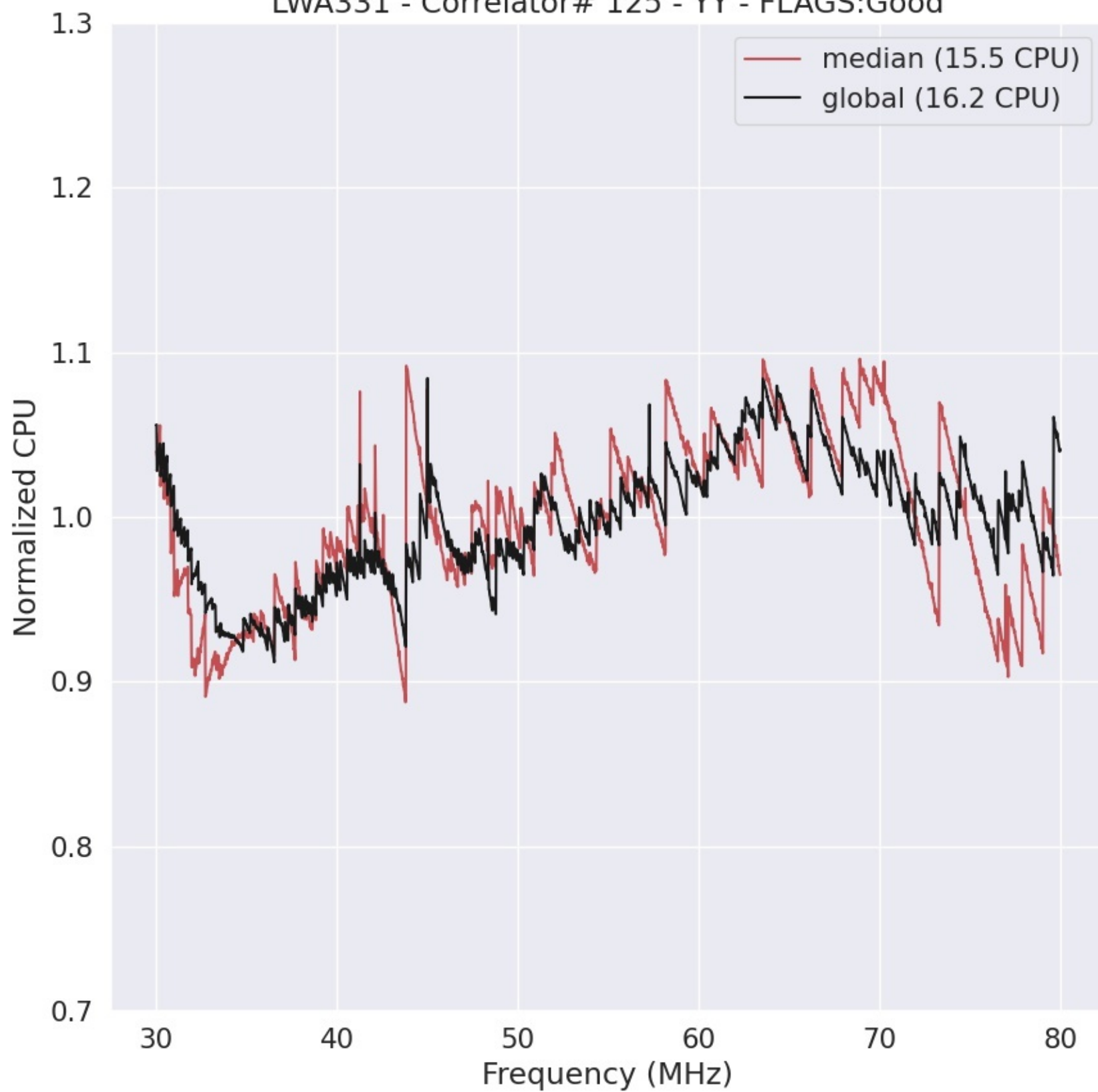
LWA331 - Correlator# 125 - YY - FLAGS:Good
