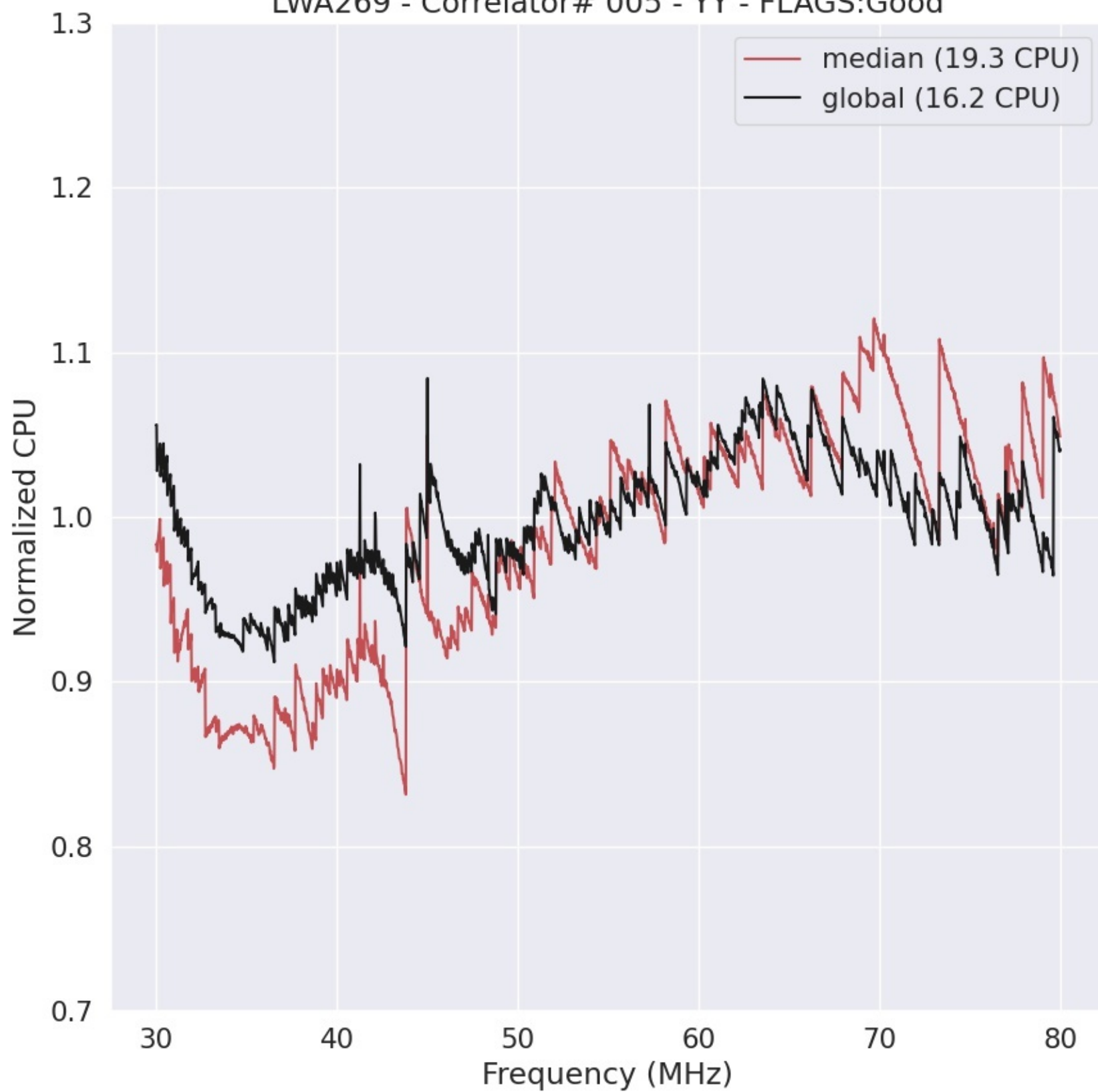
LWA269 - Correlator# 005 - YY - FLAGS:Good
