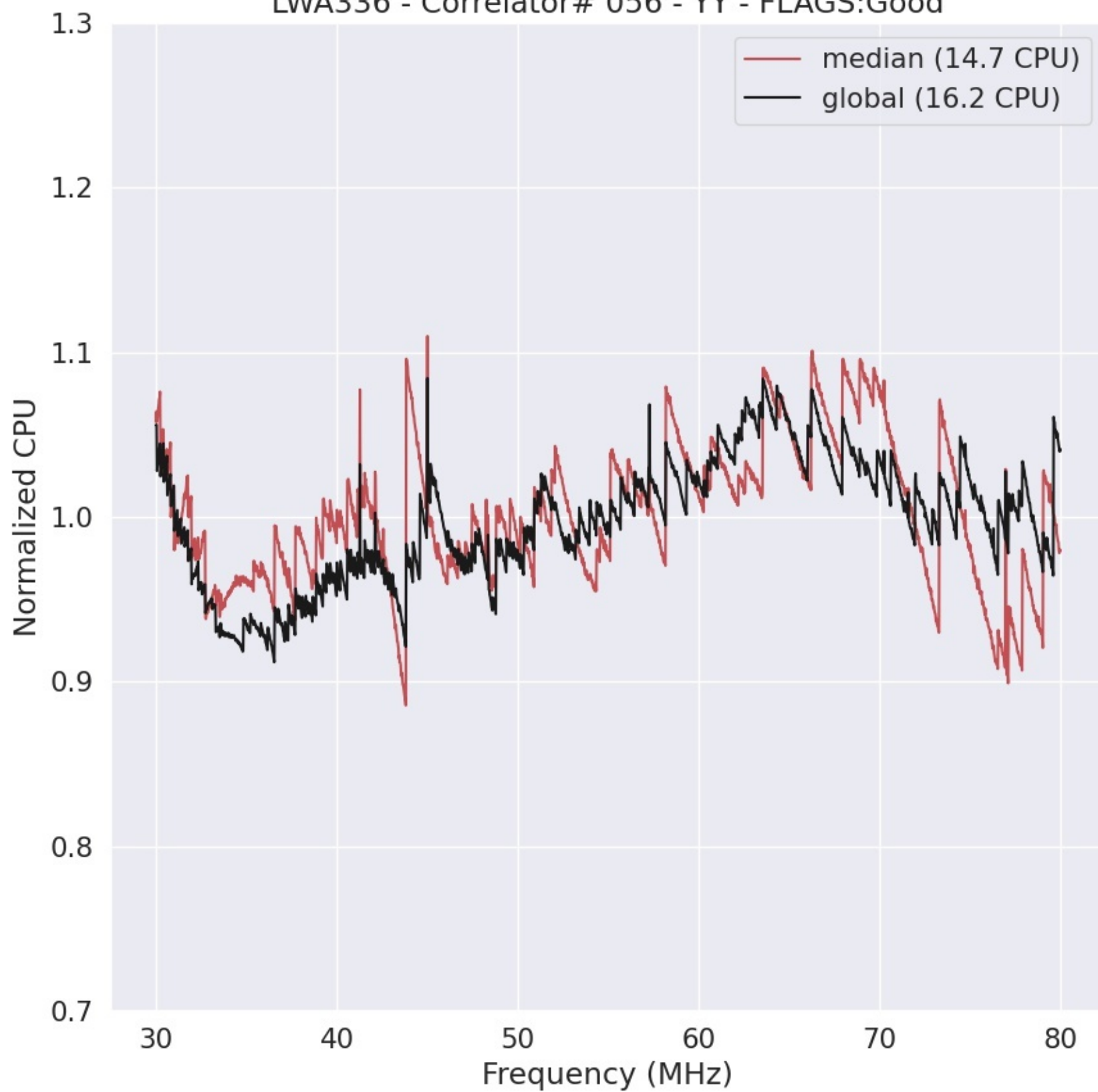
LWA336 - Correlator# 056 - YY - FLAGS:Good
