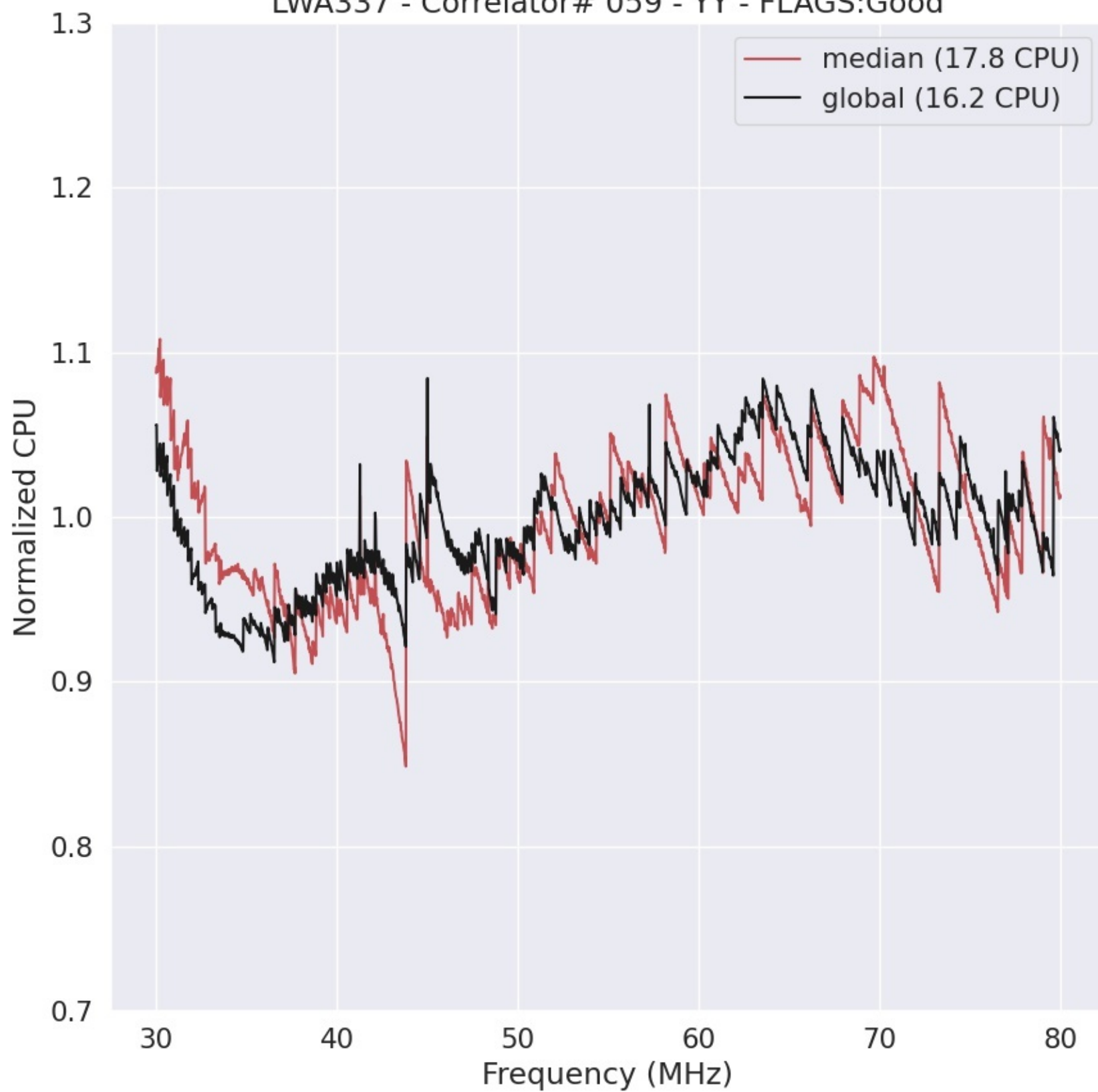
LWA337 - Correlator# 059 - YY - FLAGS:Good
