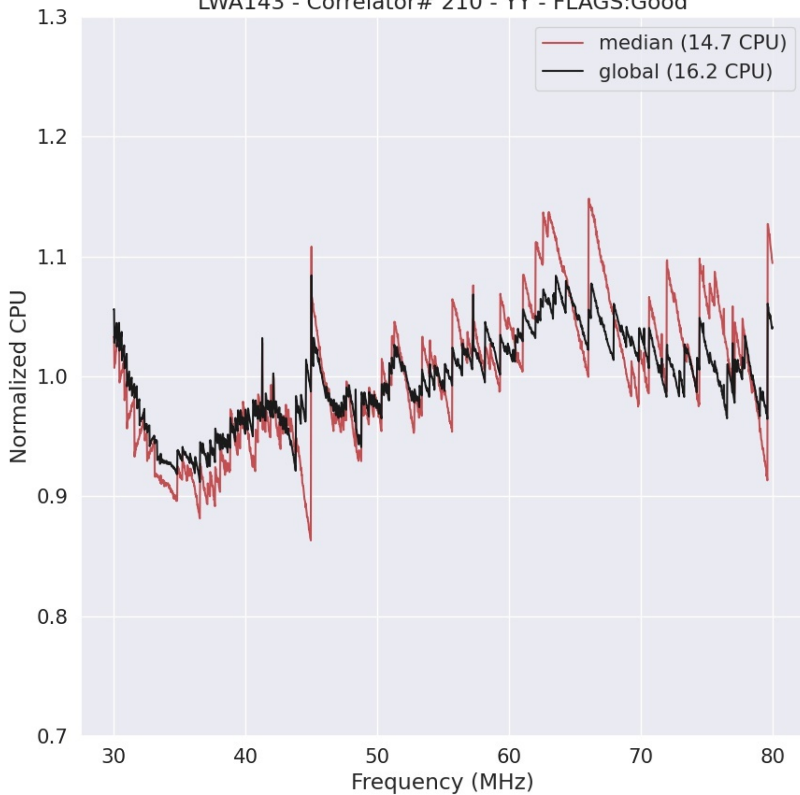
LWA143 - Correlator# 210 - YY - FLAGS:Good
