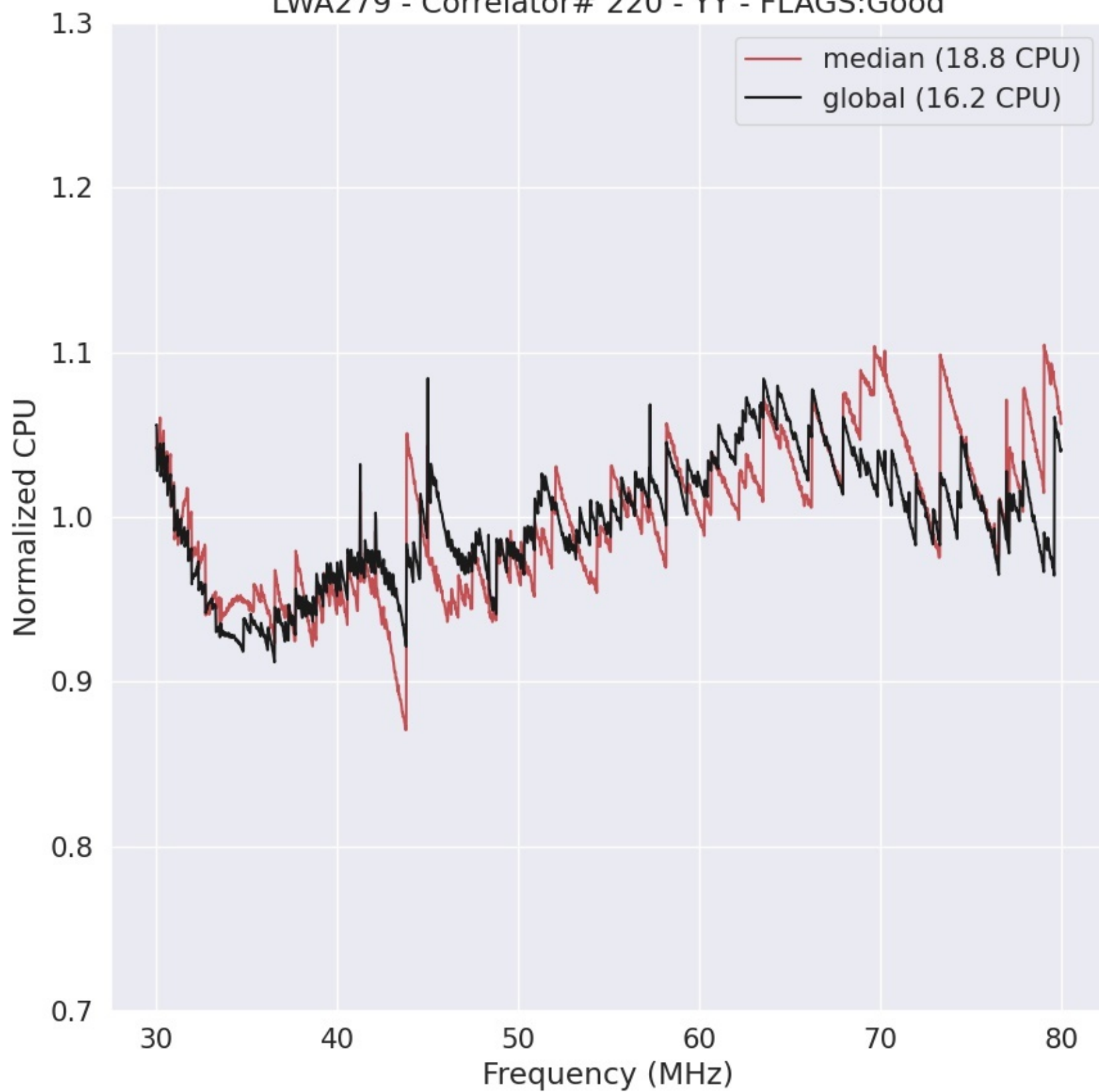
LWA279 - Correlator# 220 - YY - FLAGS:Good
