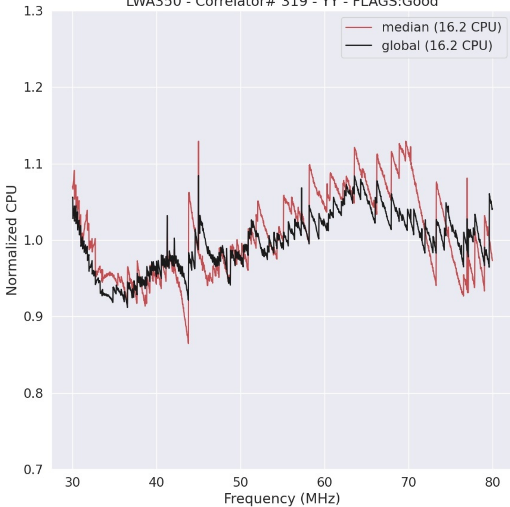
LWA350 - Correlator# 319 - YY - FLAGS:Good
