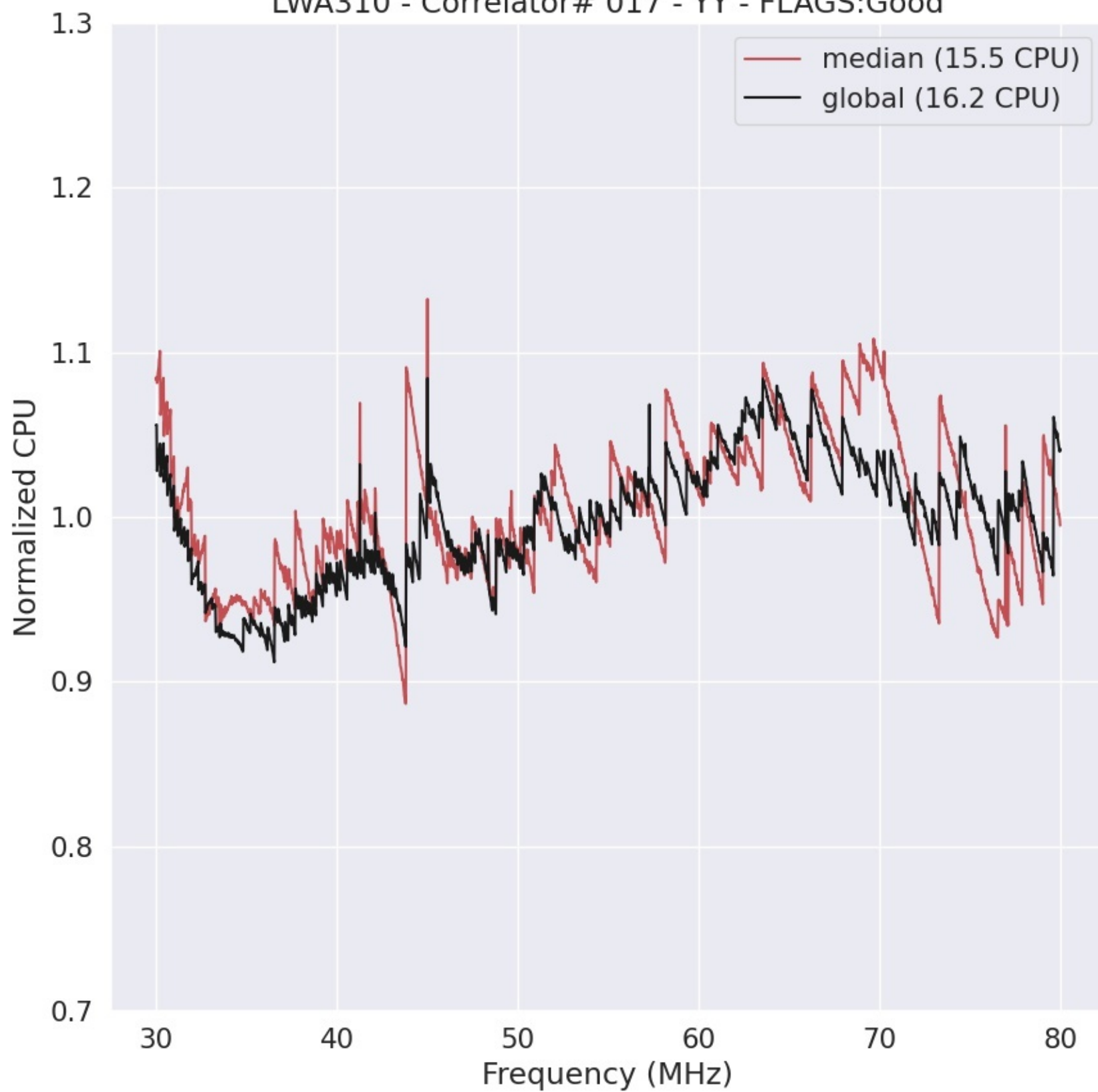
LWA310 - Correlator# 017 - YY - FLAGS:Good
