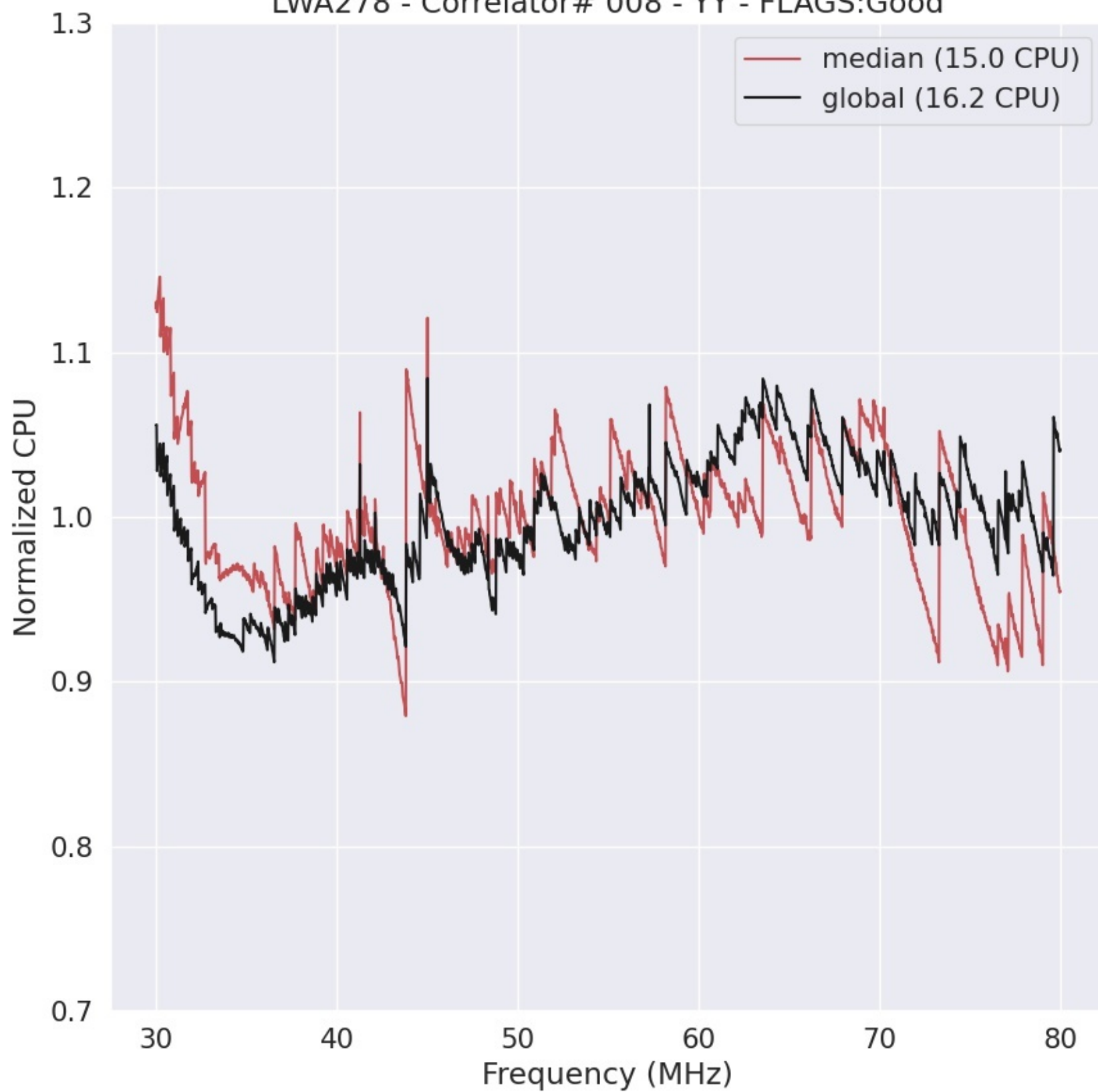
LWA278 - Correlator# 008 - YY - FLAGS:Good
