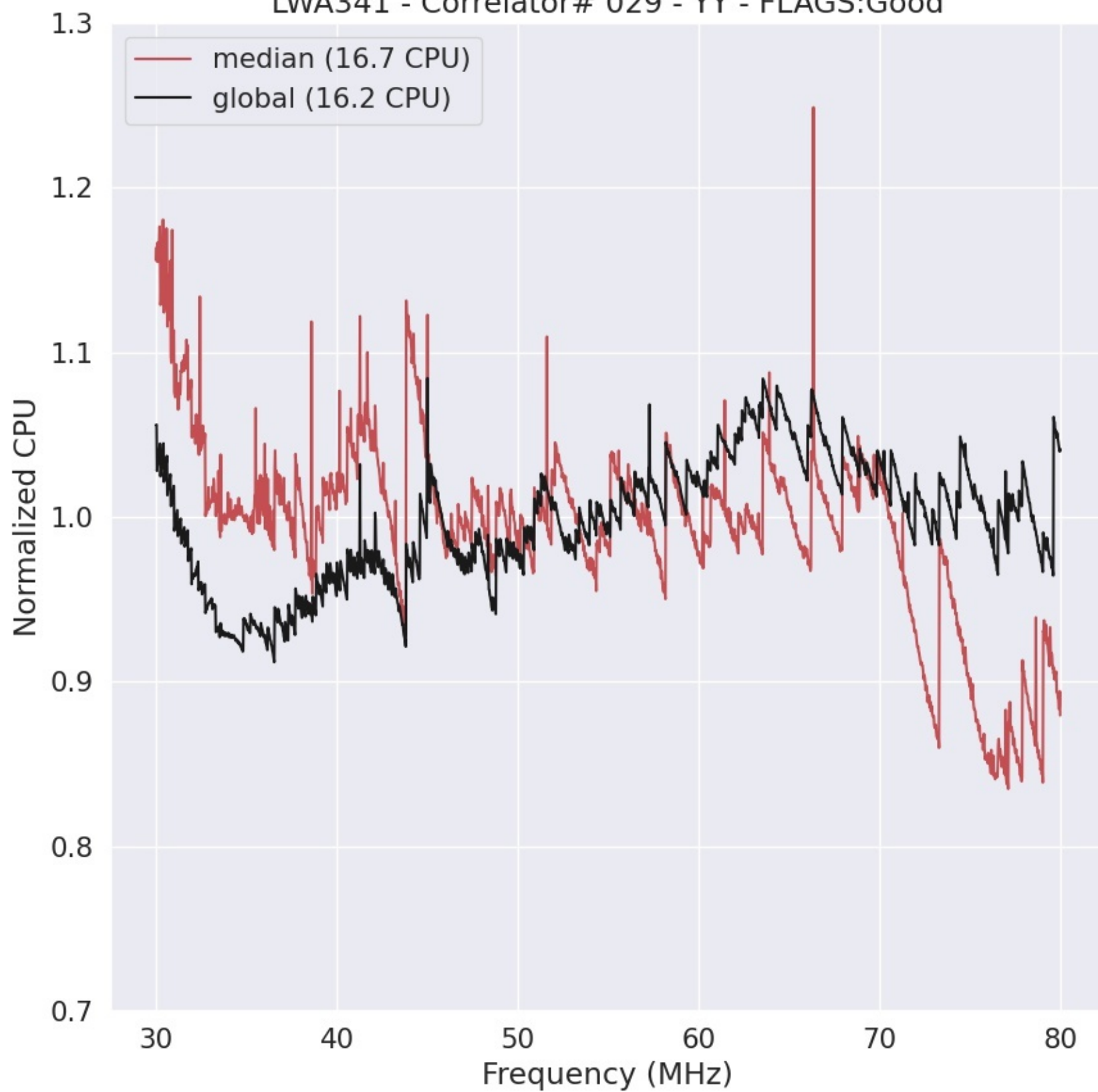
LWA341 - Correlator# 029 - YY - FLAGS:Good
