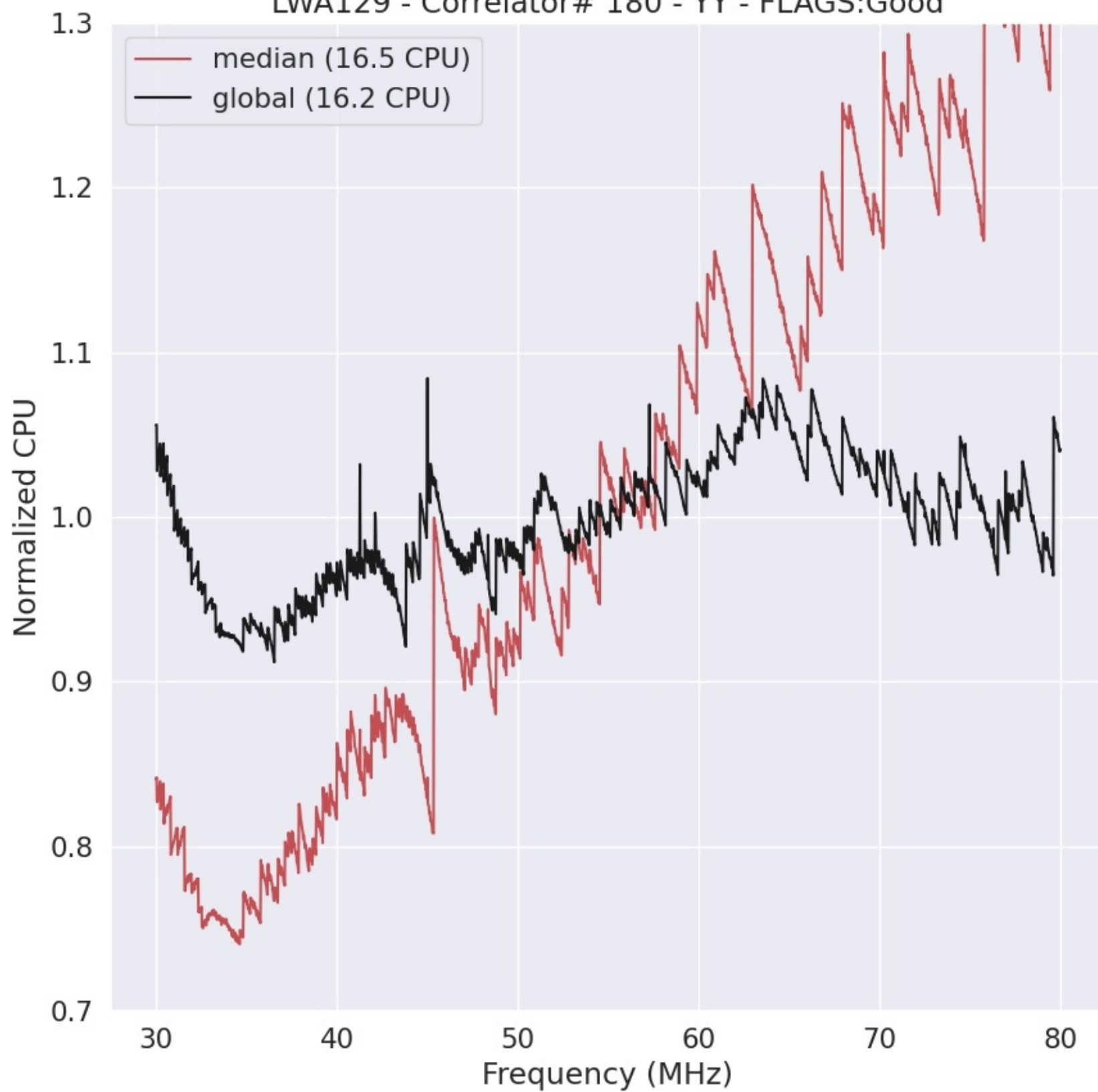
LWA129 - Correlator# 180 - YY - FLAGS:Good
