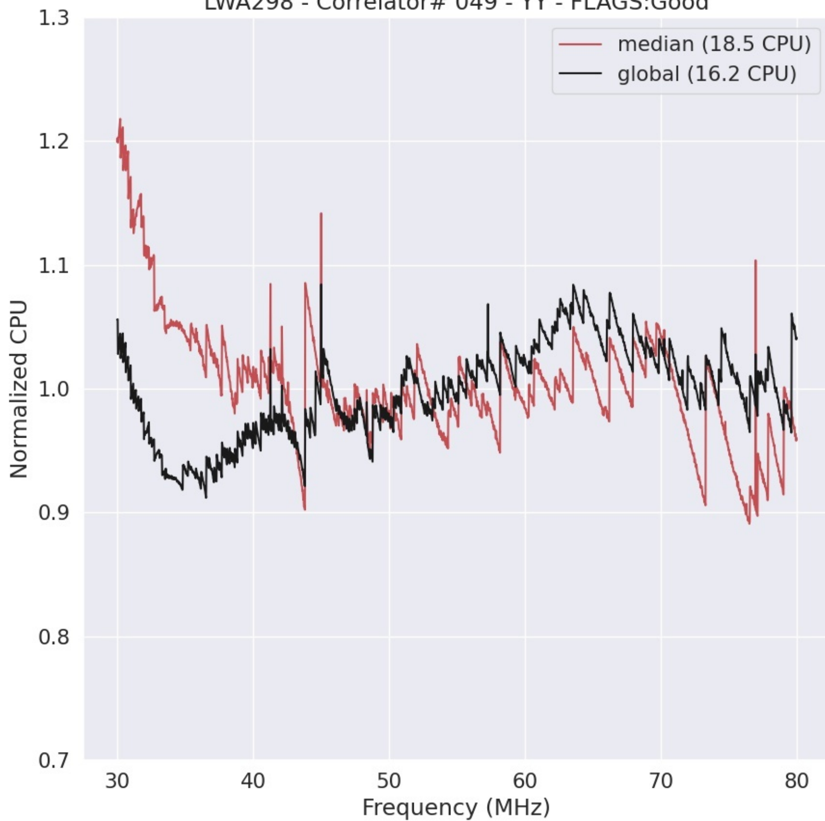
LWA298 - Correlator# 049 - YY - FLAGS:Good
