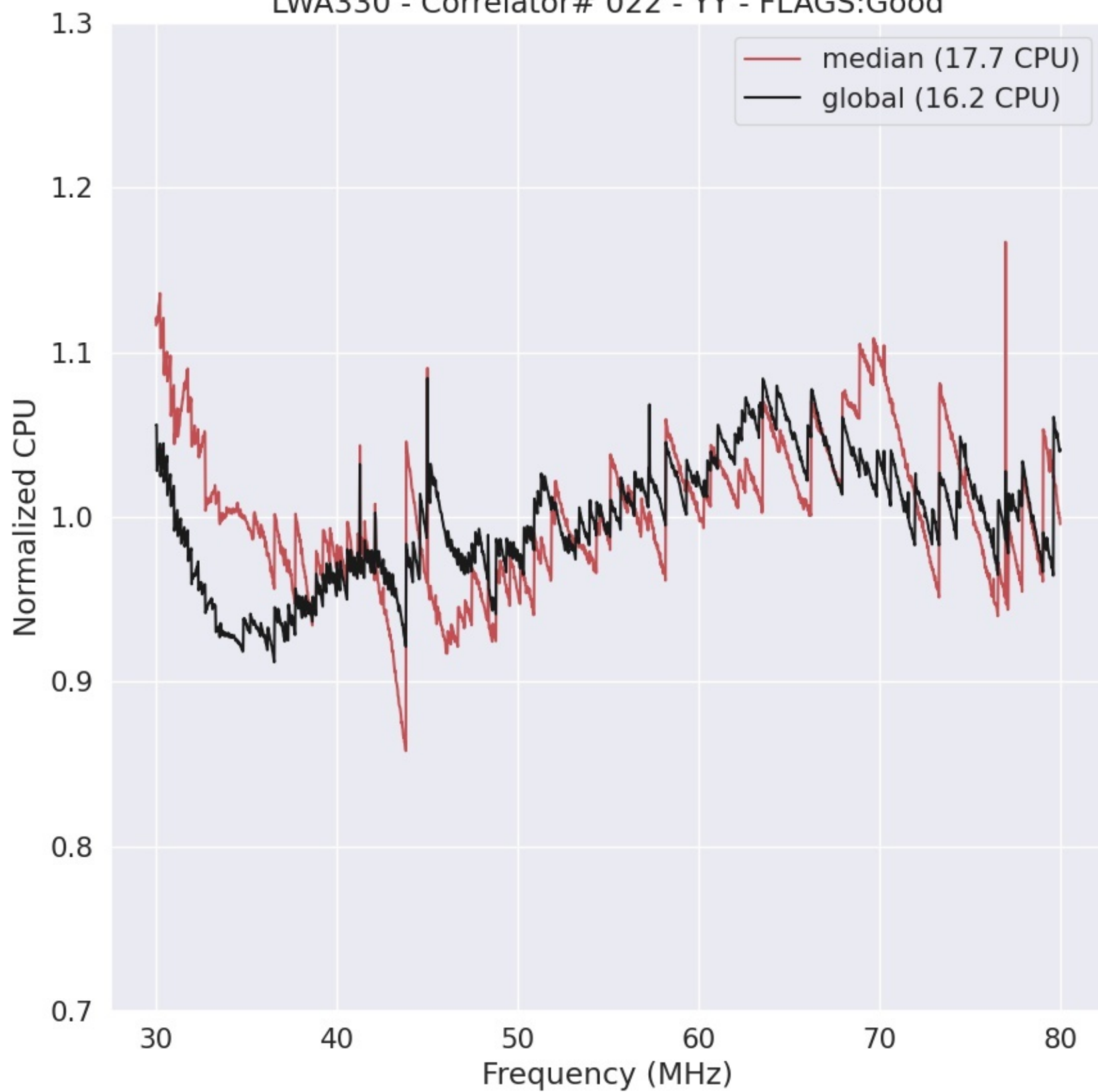
LWA330 - Correlator# 022 - YY - FLAGS:Good
