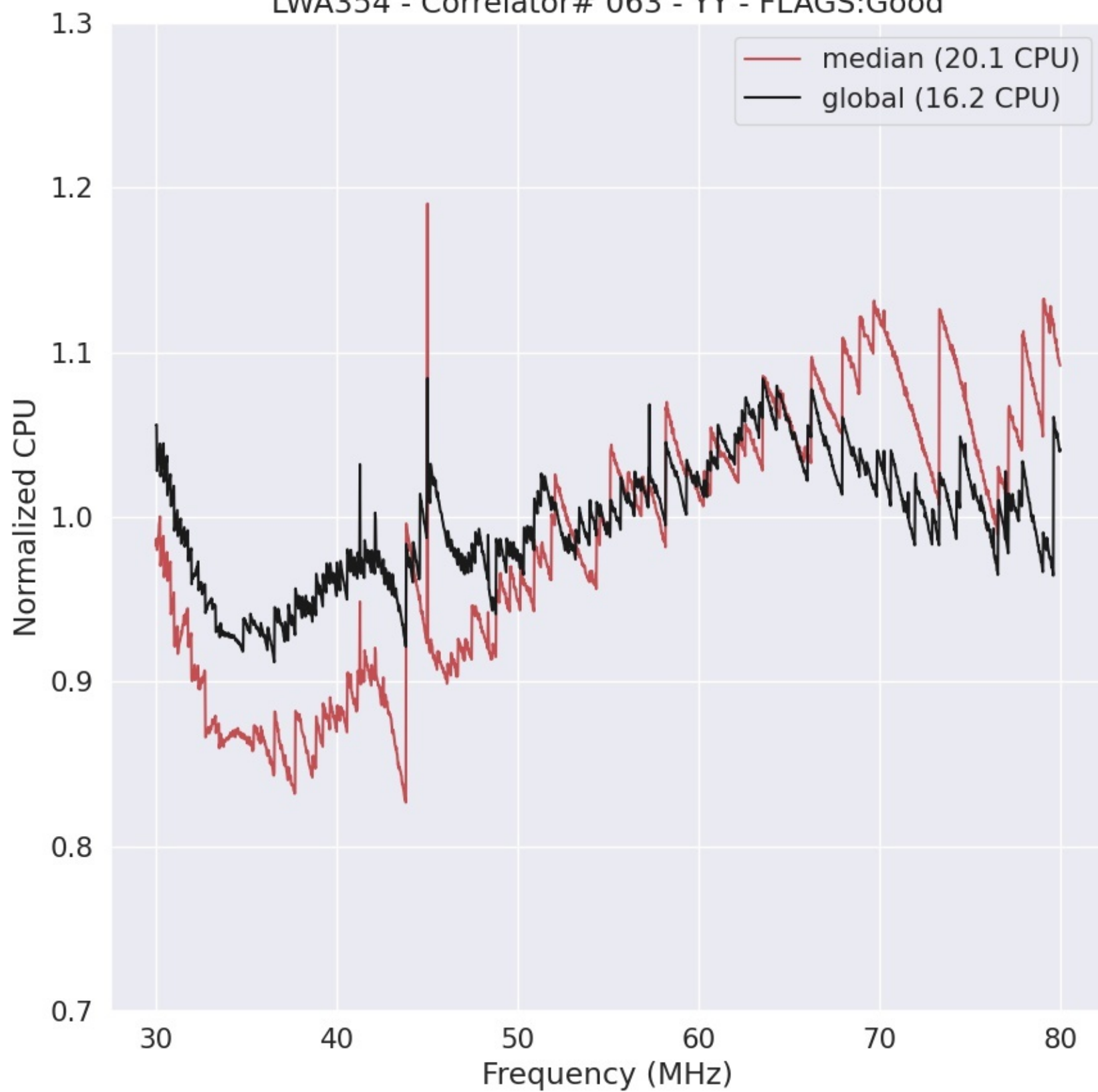
LWA354 - Correlator# 063 - YY - FLAGS:Good
