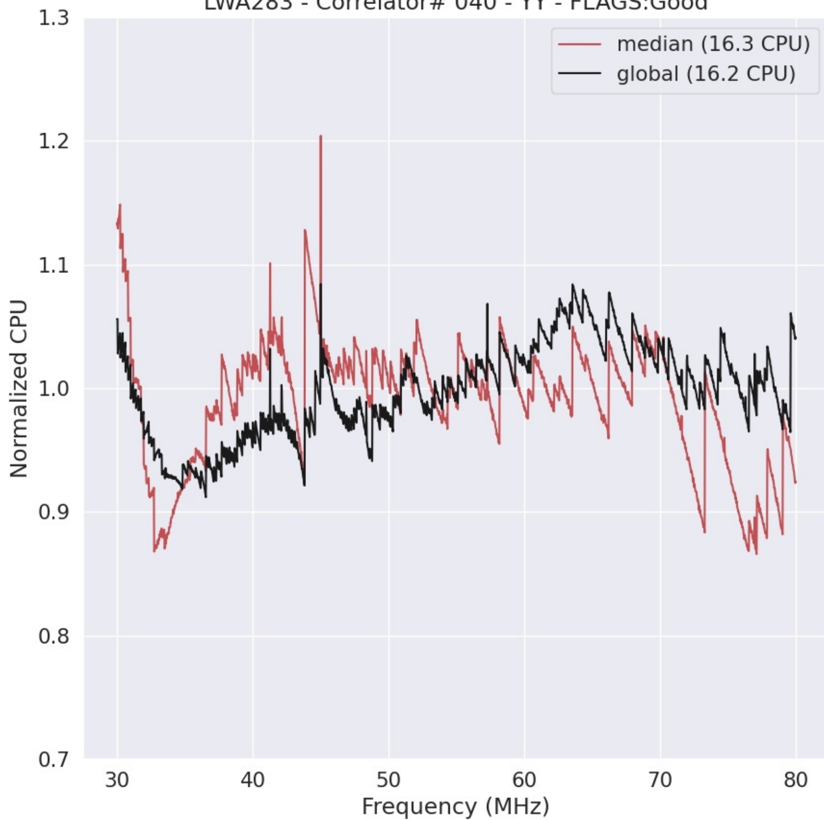
LWA283 - Correlator# 040 - YY - FLAGS:Good
