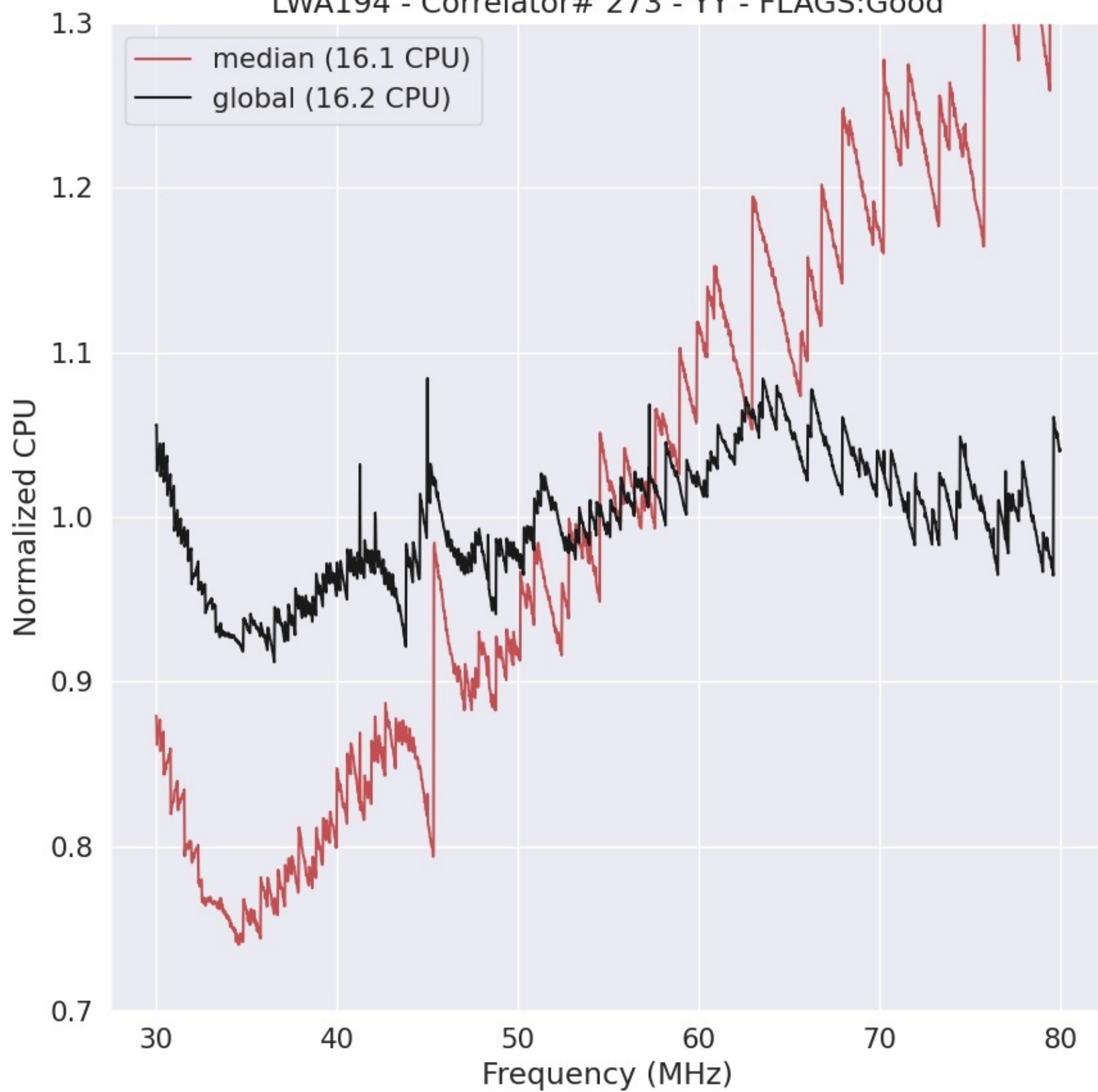
LWA194 - Correlator# 273 - YY - FLAGS:Good
