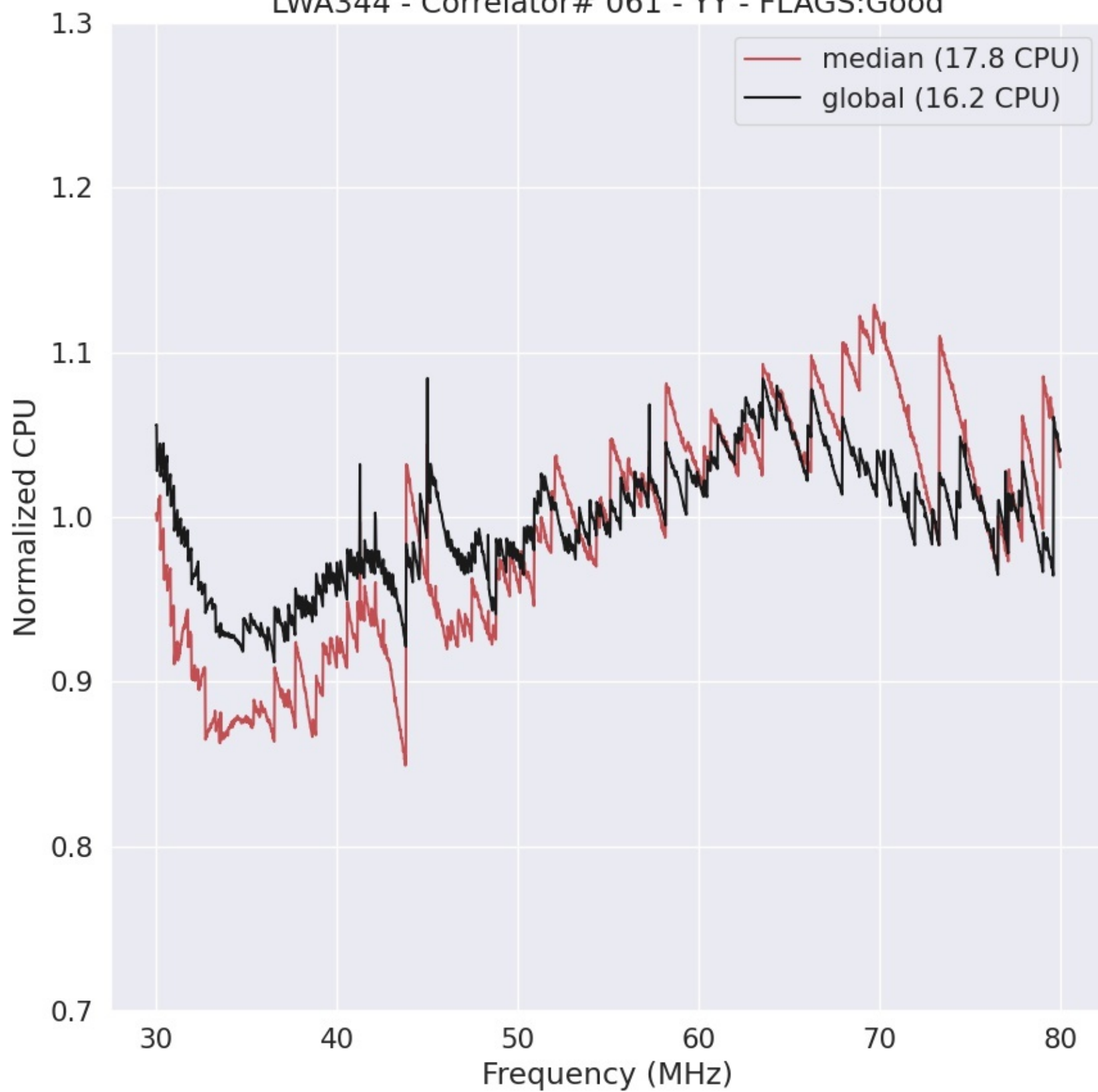
LWA344 - Correlator# 061 - YY - FLAGS:Good
