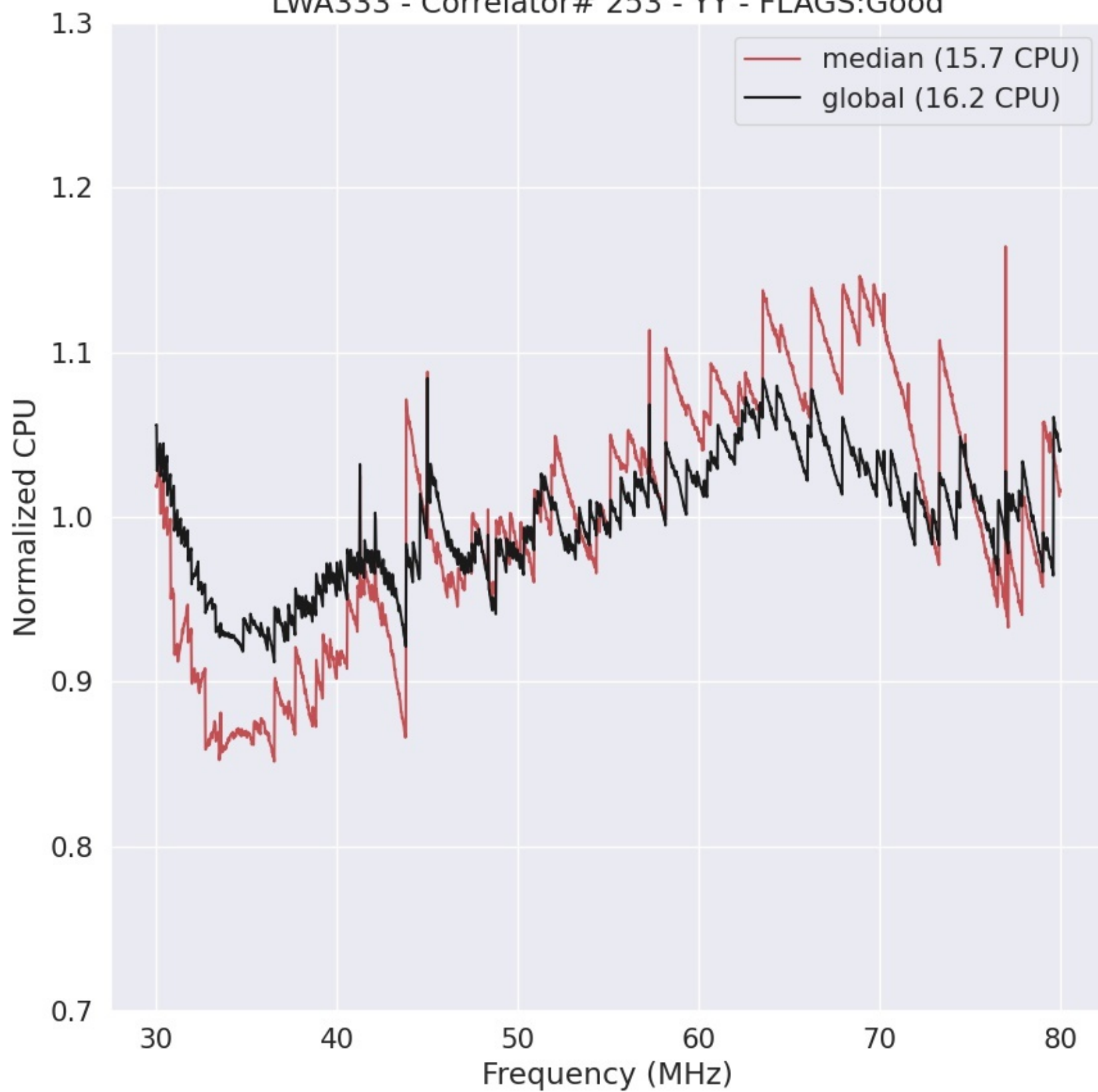
LWA333 - Correlator# 253 - YY - FLAGS:Good
