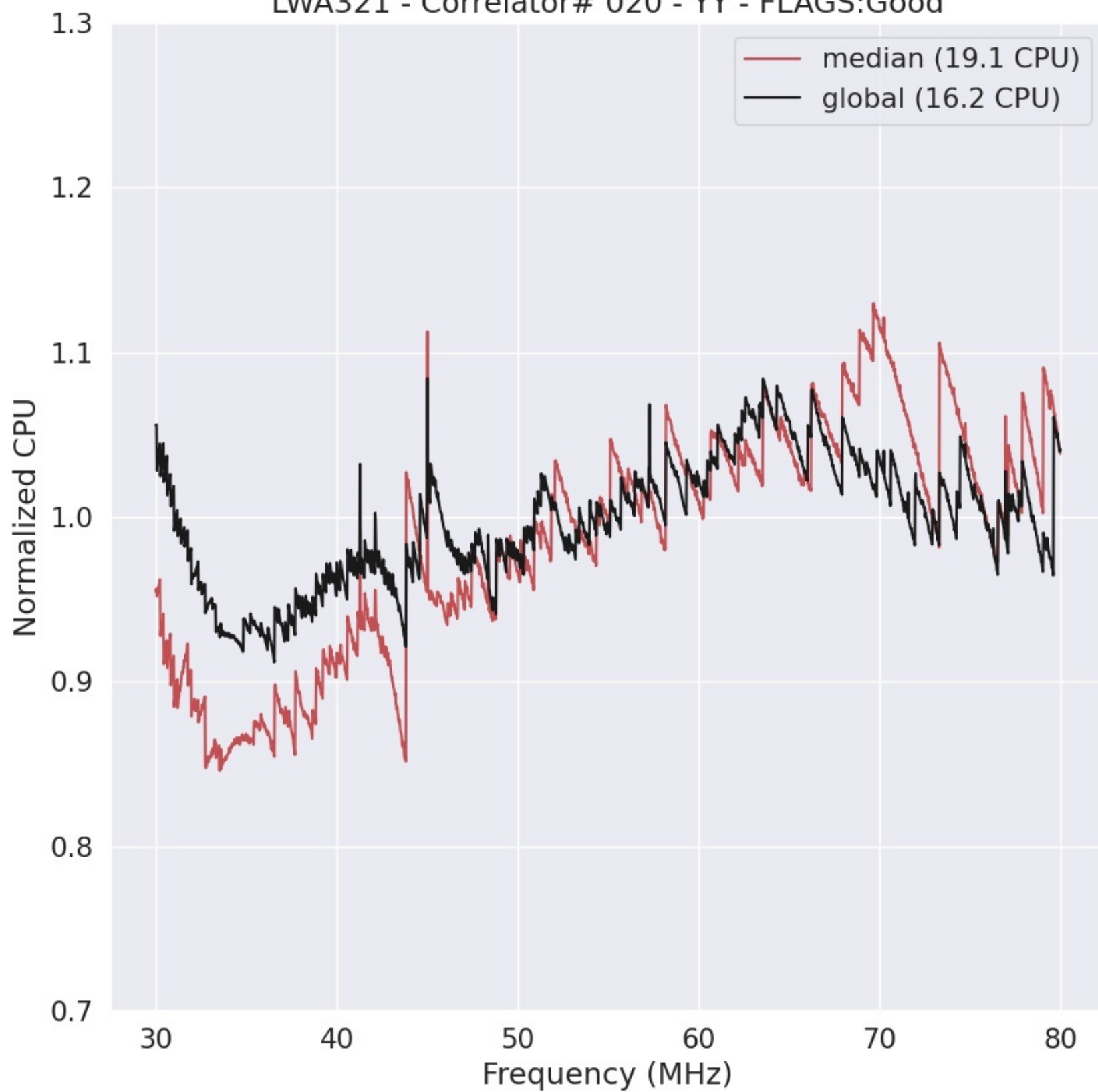
LWA321 - Correlator# 020 - YY - FLAGS:Good
