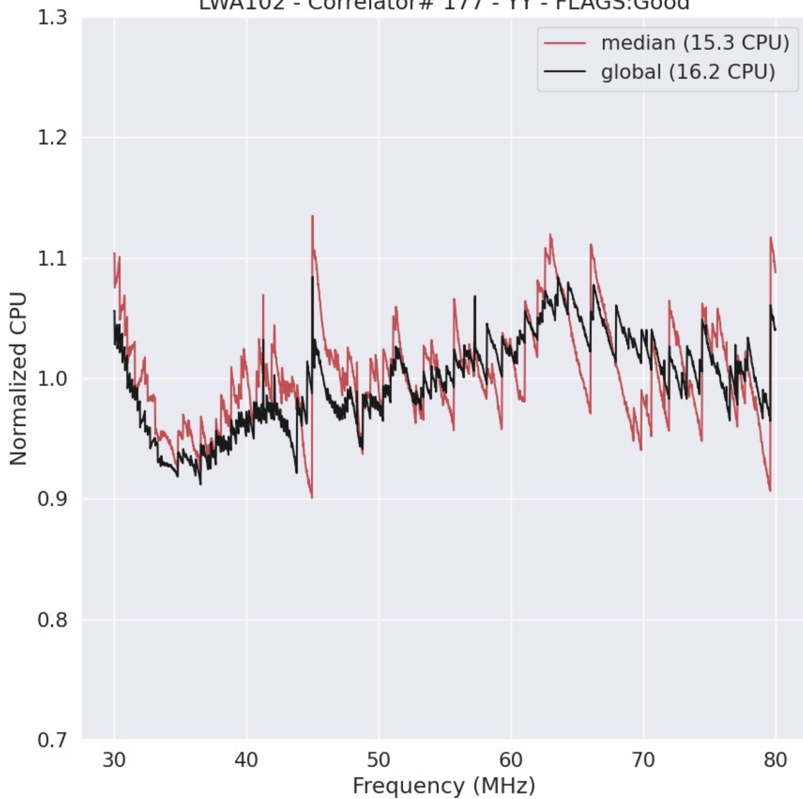
LWA102 - Correlator# 177 - YY - FLAGS:Good
