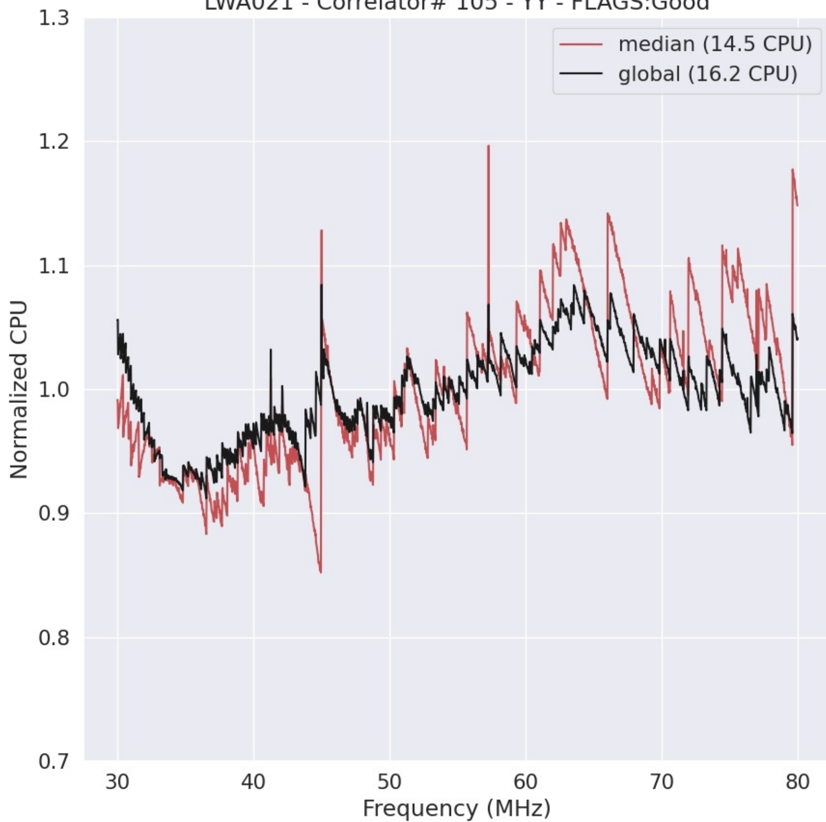
LWA021 - Correlator# 105 - YY - FLAGS:Good
