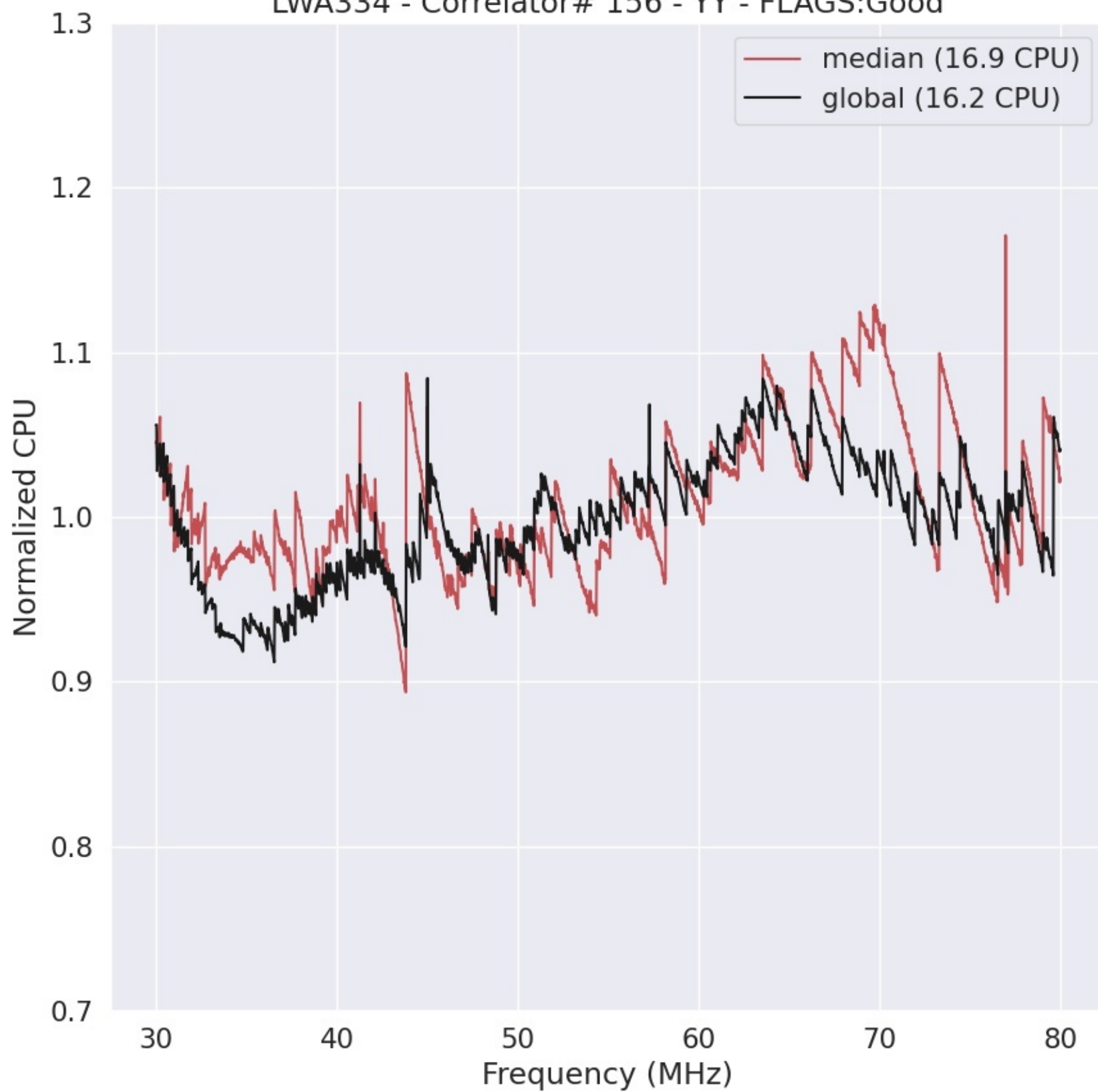
LWA334 - Correlator# 156 - YY - FLAGS:Good
