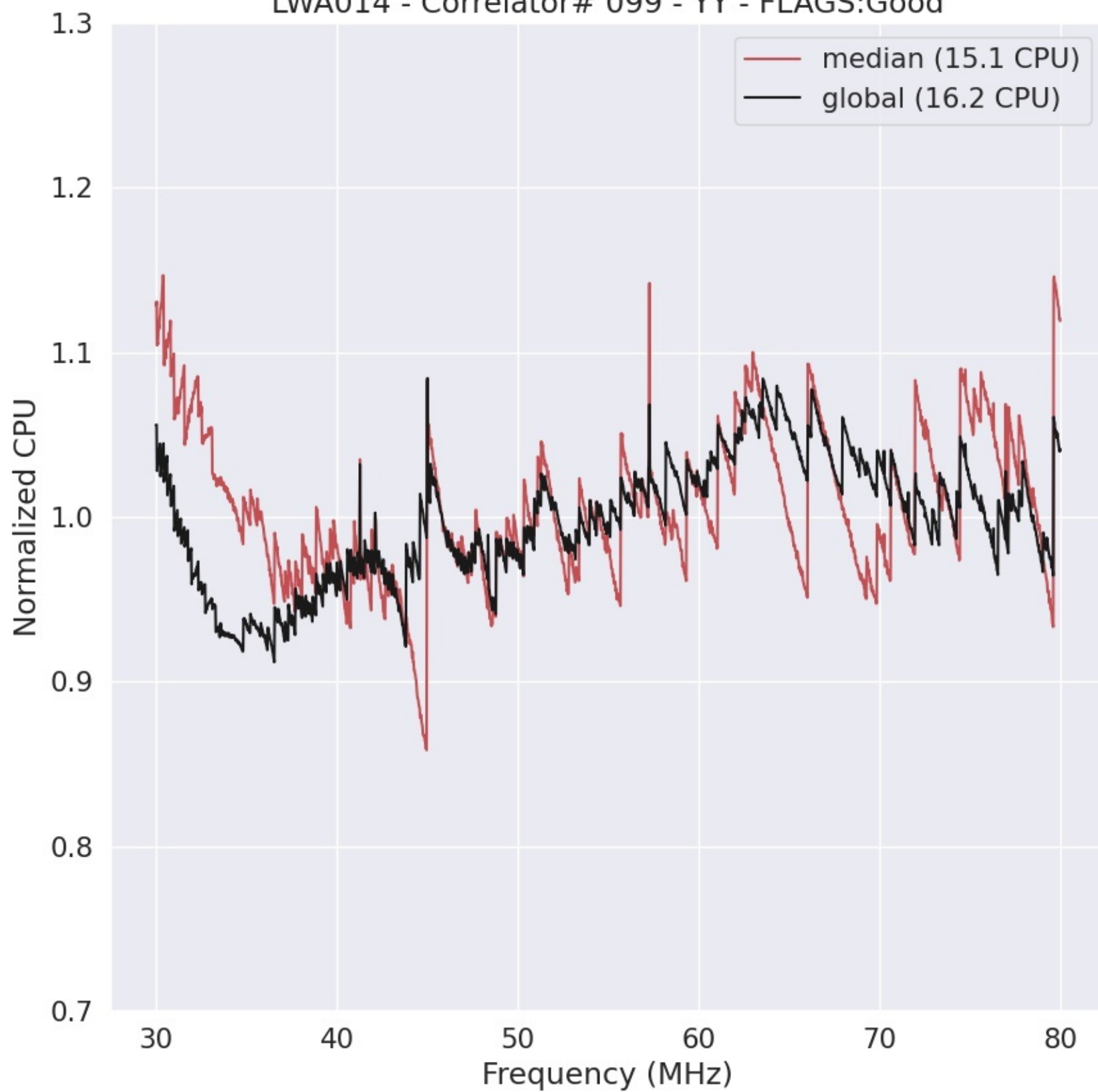
LWA014 - Correlator# 099 - YY - FLAGS:Good
