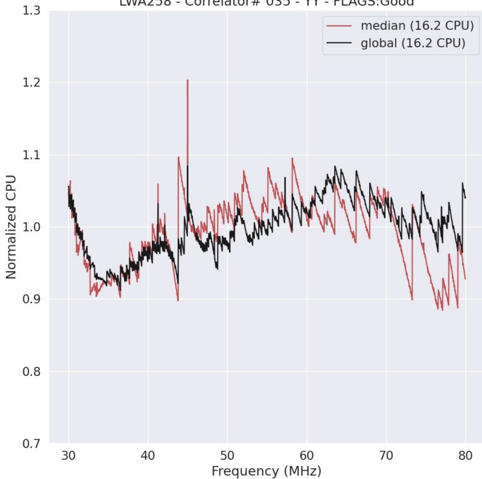
LWA258 - Correlator# 035 - YY - FLAGS:Good
