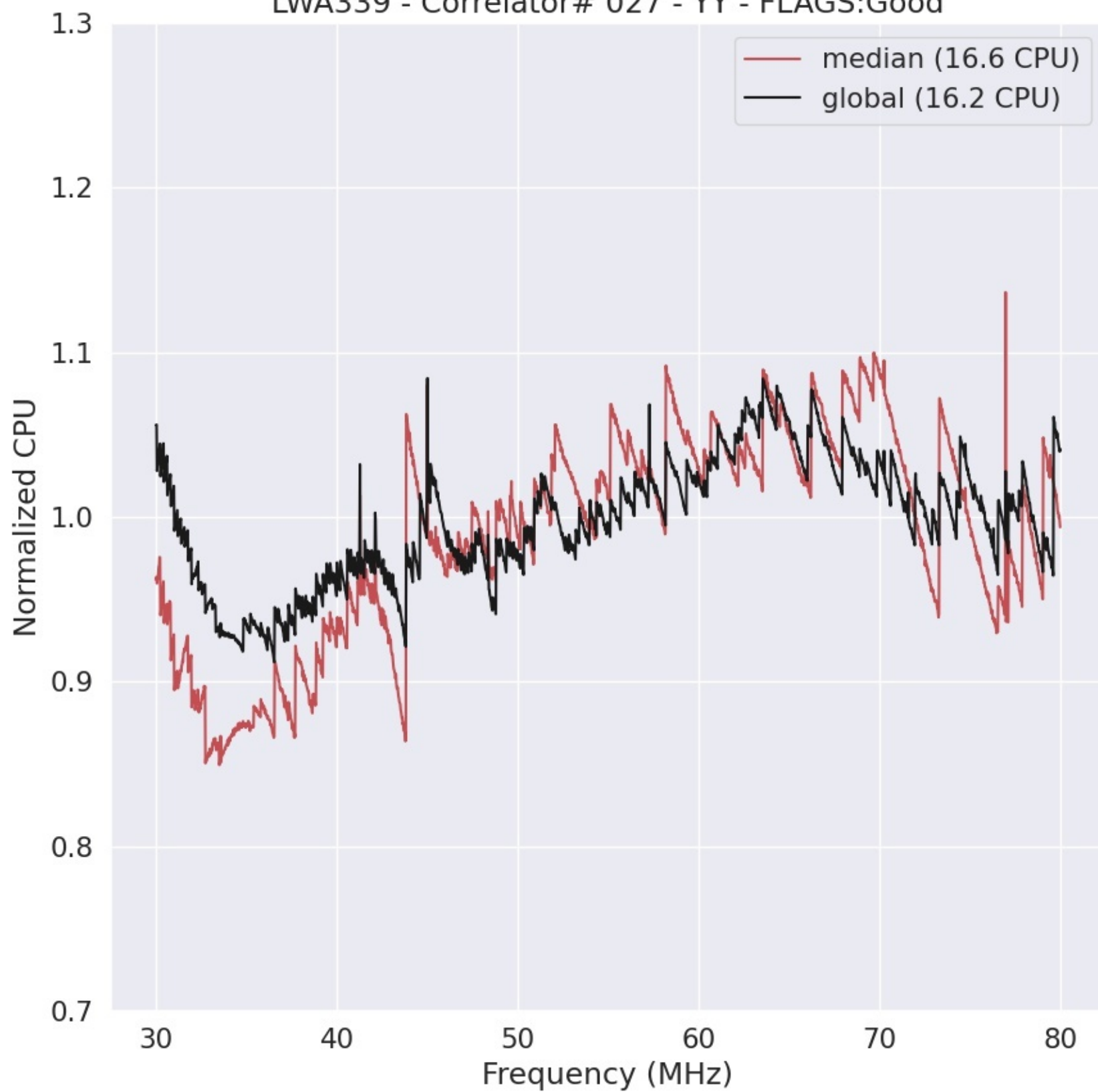
LWA339 - Correlator# 027 - YY - FLAGS:Good
