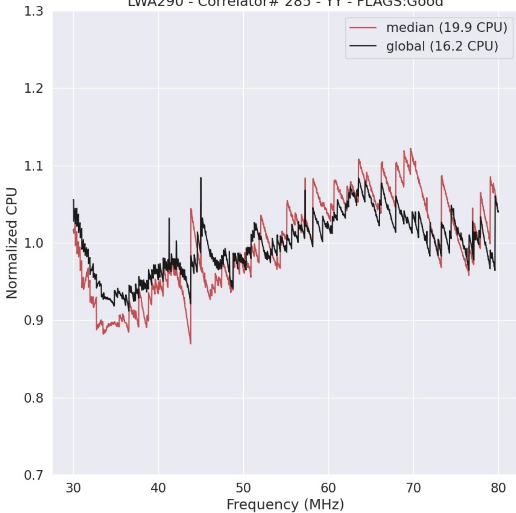
LWA290 - Correlator# 285 - YY - FLAGS:Good
