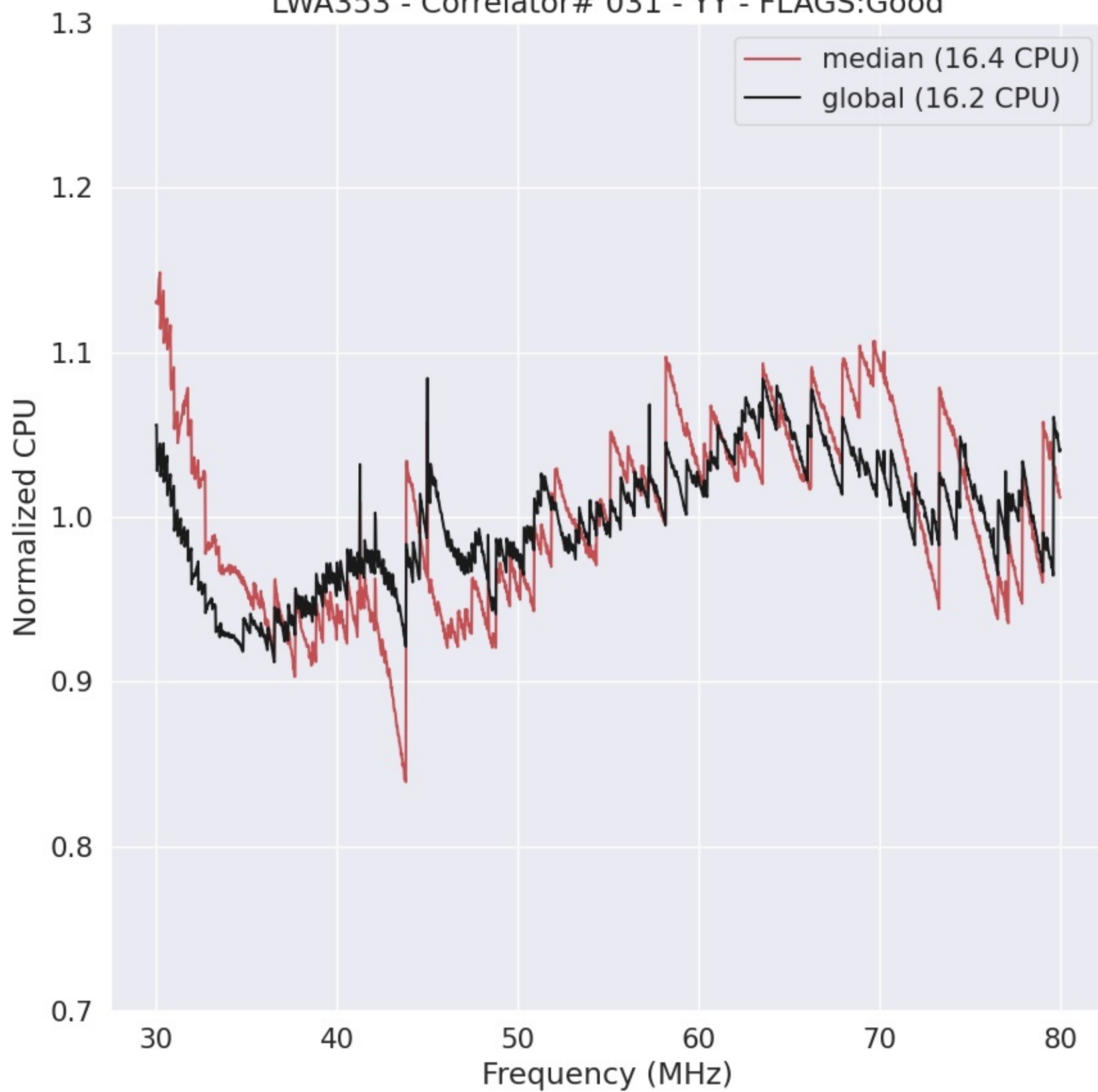
LWA353 - Correlator# 031 - YY - FLAGS:Good
