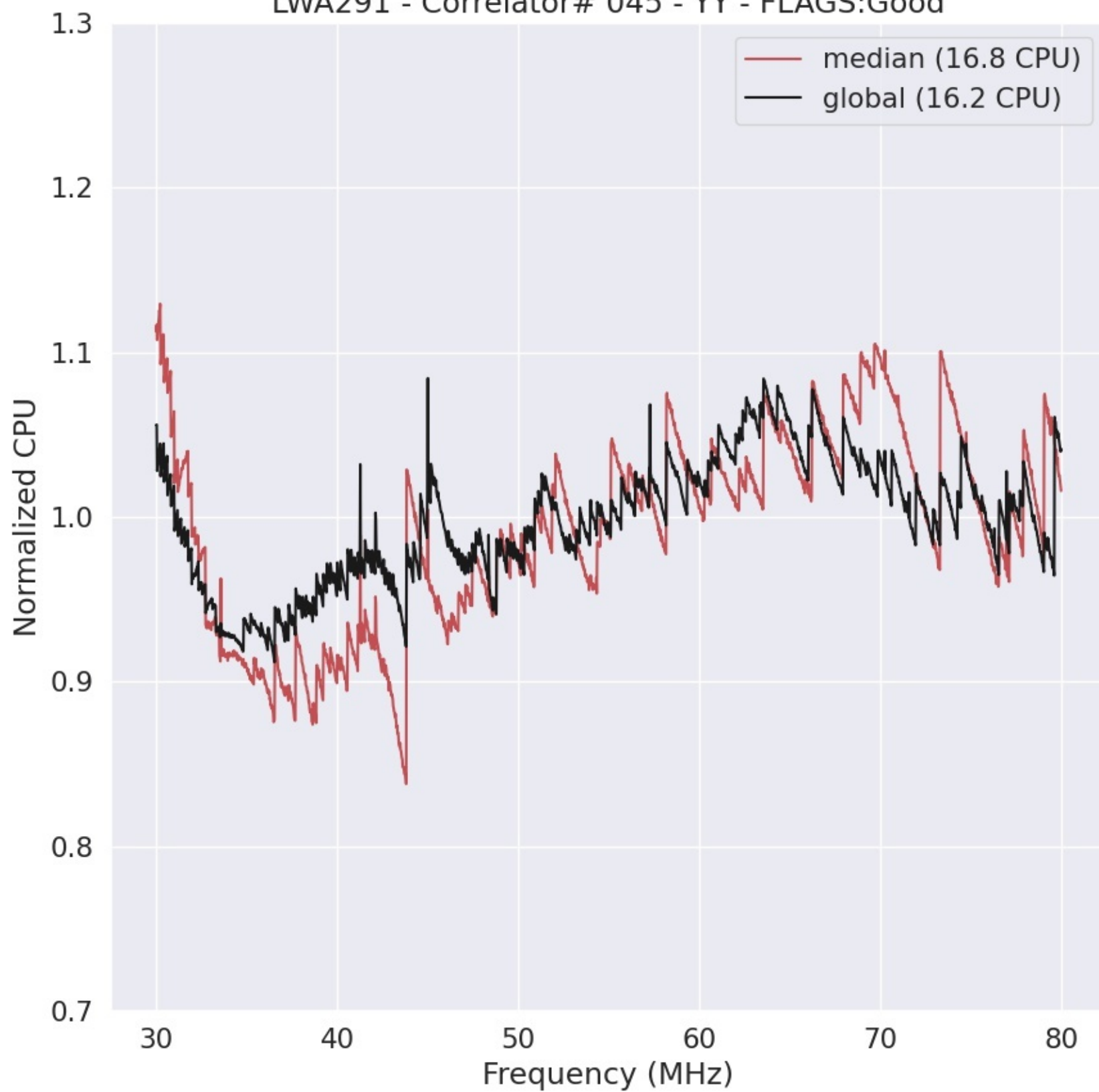
LWA291 - Correlator# 045 - YY - FLAGS:Good
