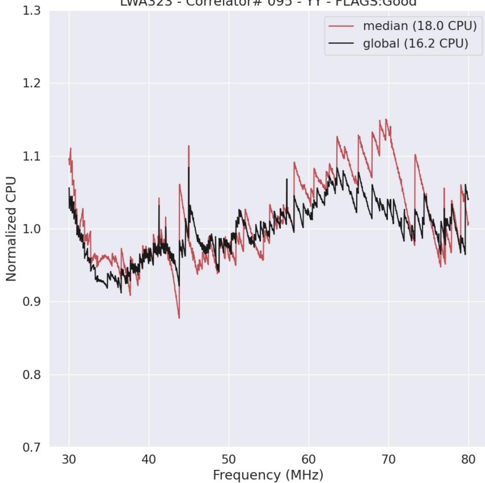
LWA323 - Correlator# 095 - YY - FLAGS:Good
