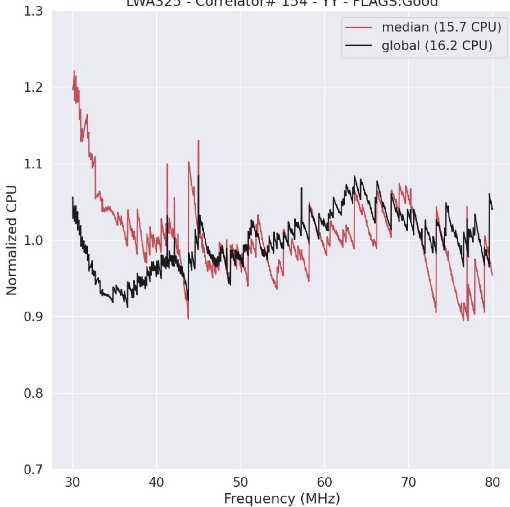
LWA325 - Correlator# 154 - YY - FLAGS:Good
