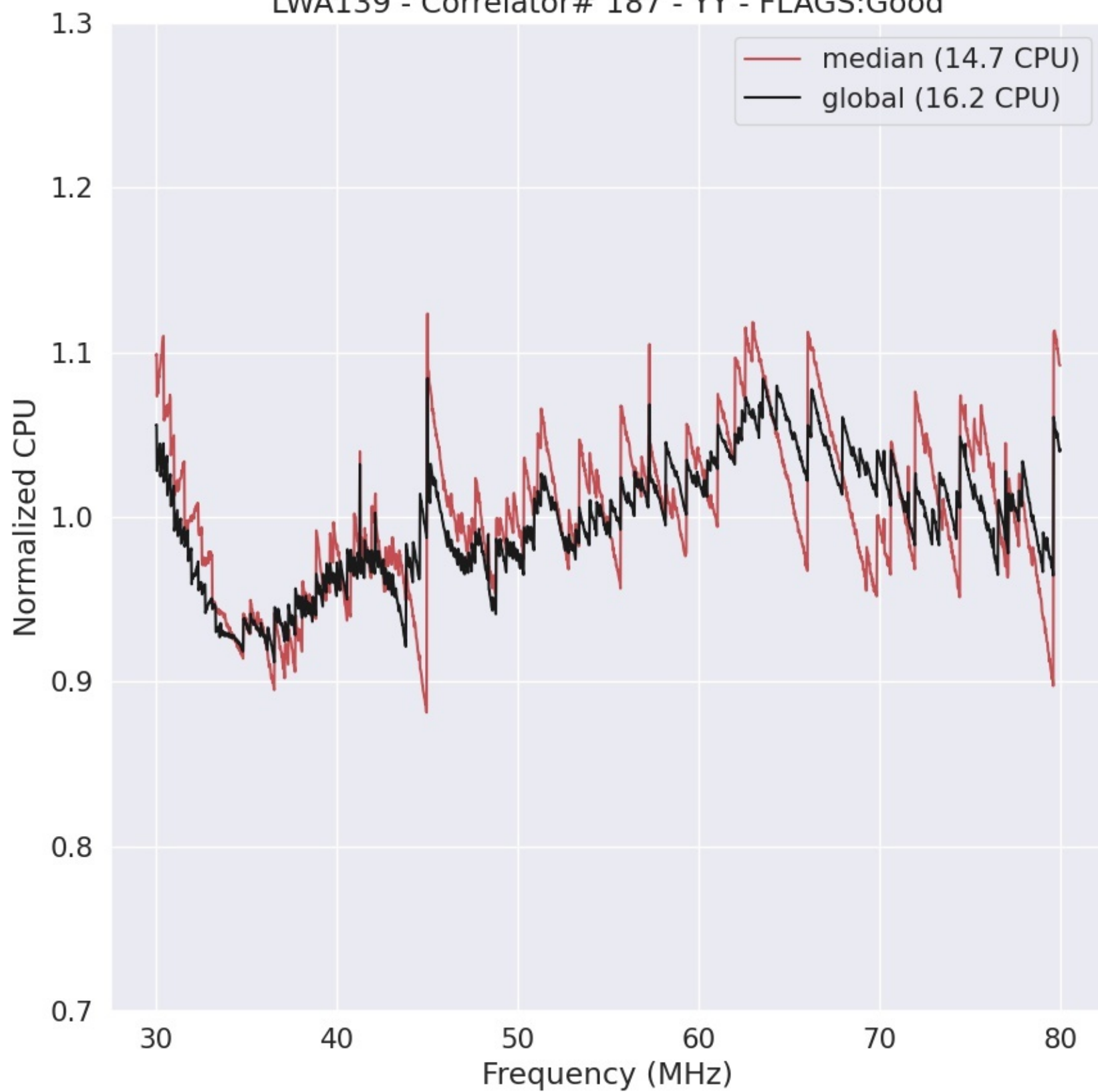
LWA139 - Correlator# 187 - YY - FLAGS:Good
