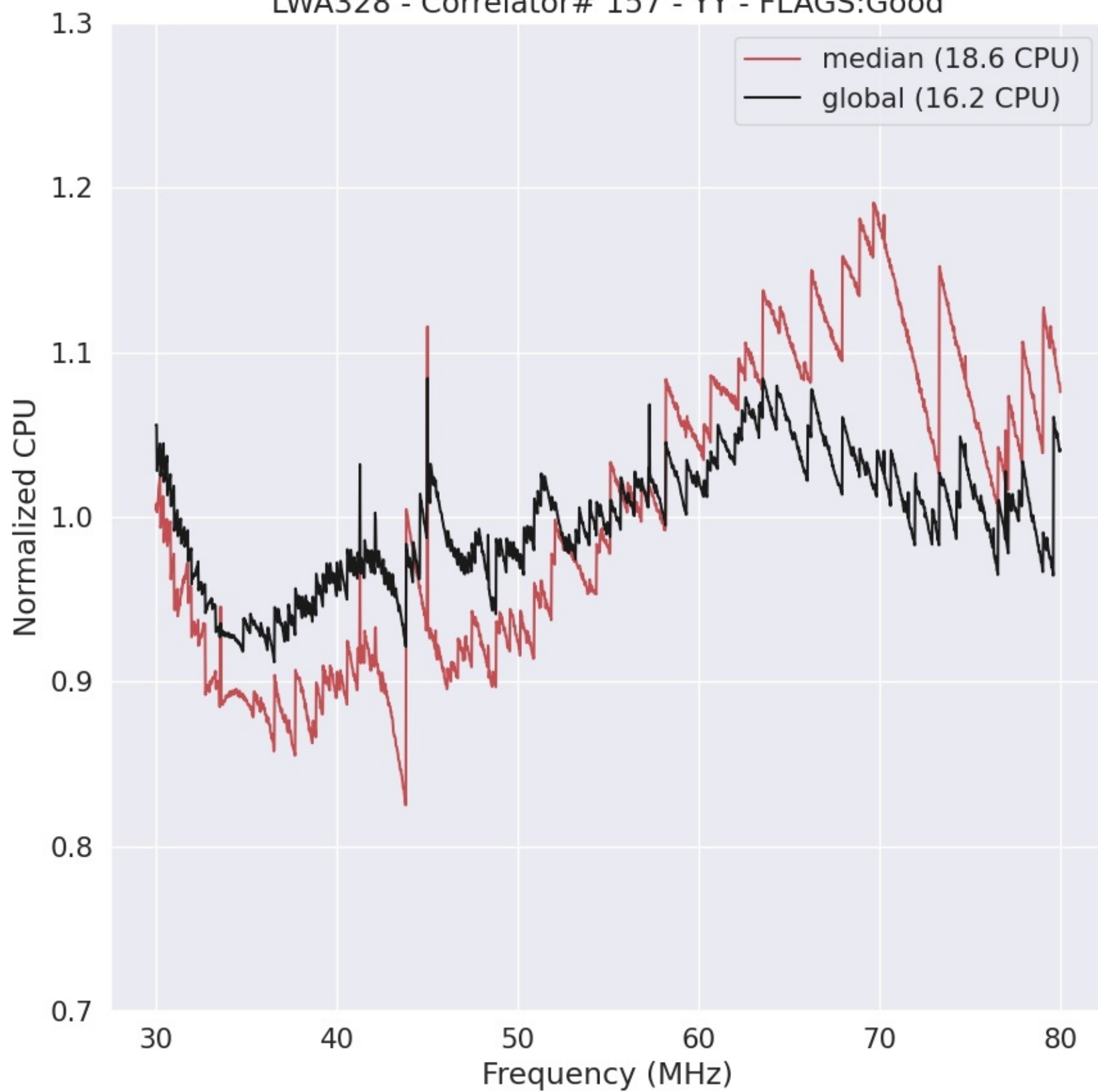
LWA328 - Correlator# 157 - YY - FLAGS:Good
