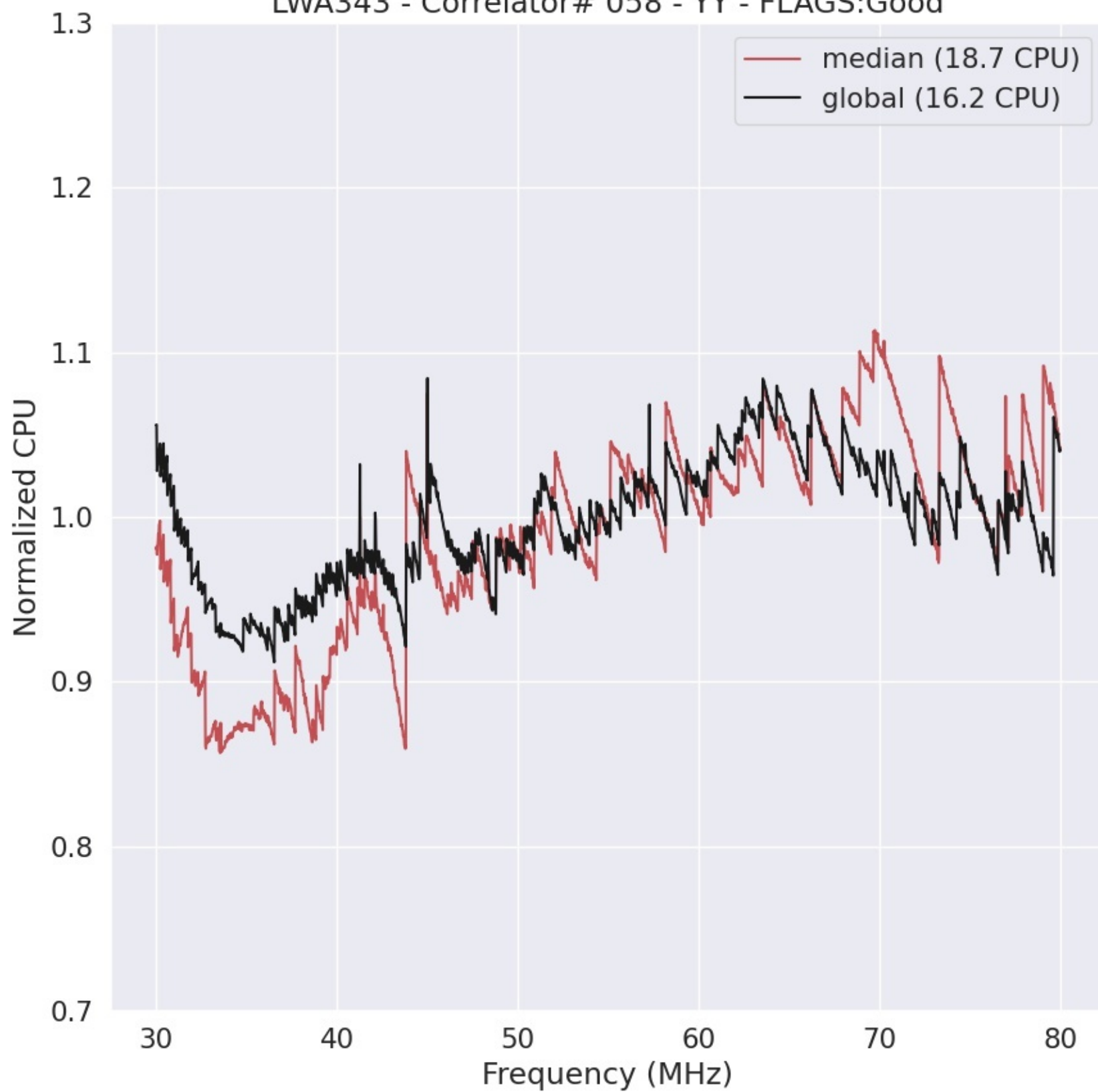
LWA343 - Correlator# 058 - YY - FLAGS:Good
