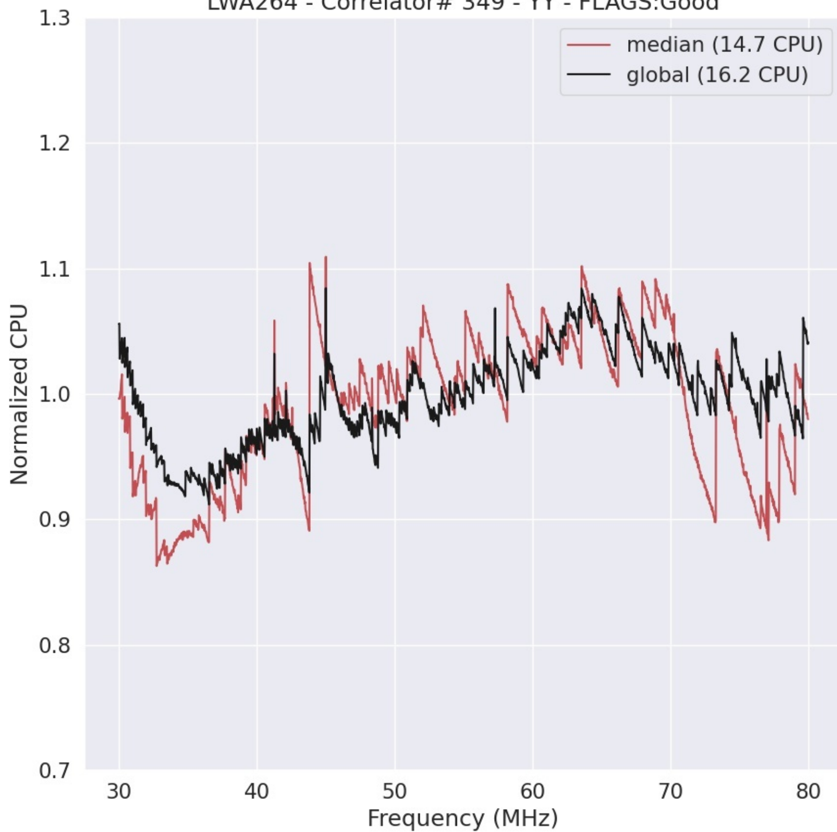
LWA264 - Correlator# 349 - YY - FLAGS:Good
