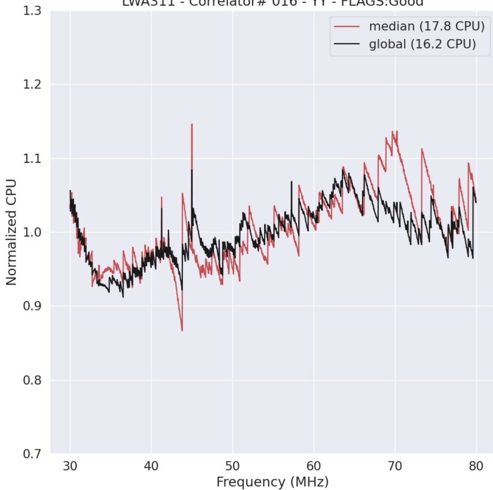
LWA311 - Correlator# 016 - YY - FLAGS:Good
