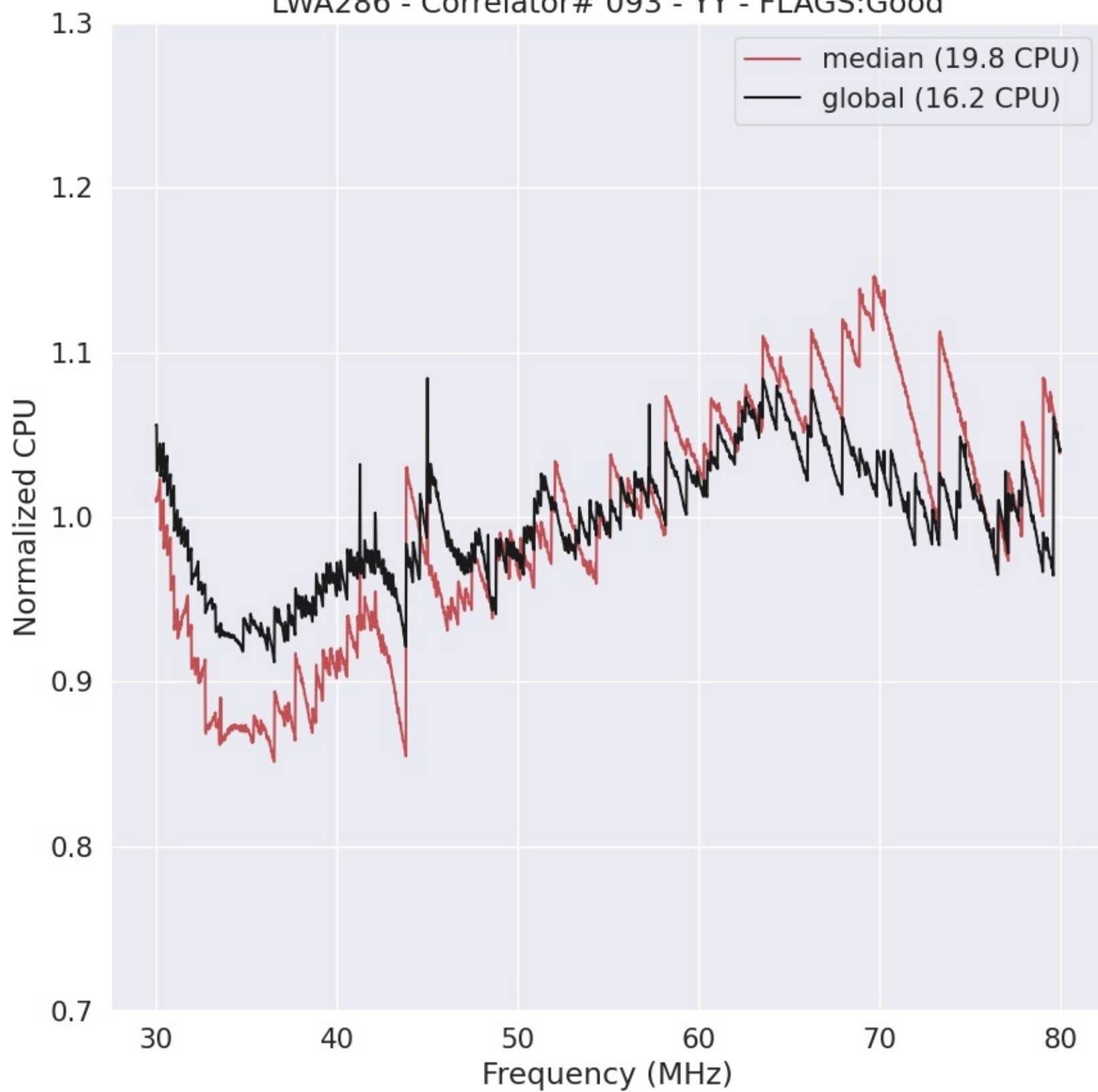
LWA286 - Correlator# 093 - YY - FLAGS:Good
