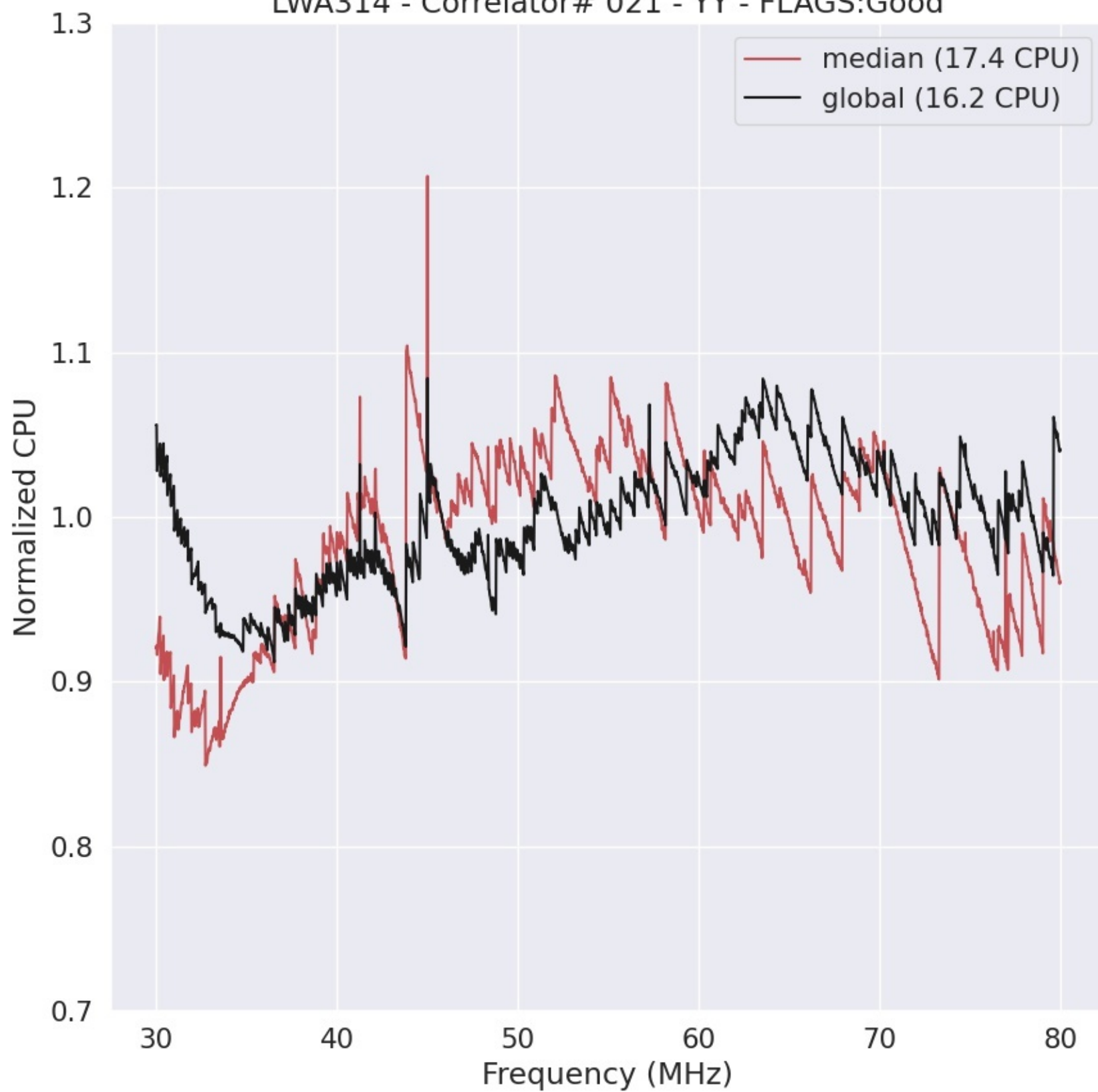
LWA314 - Correlator# 021 - YY - FLAGS:Good
