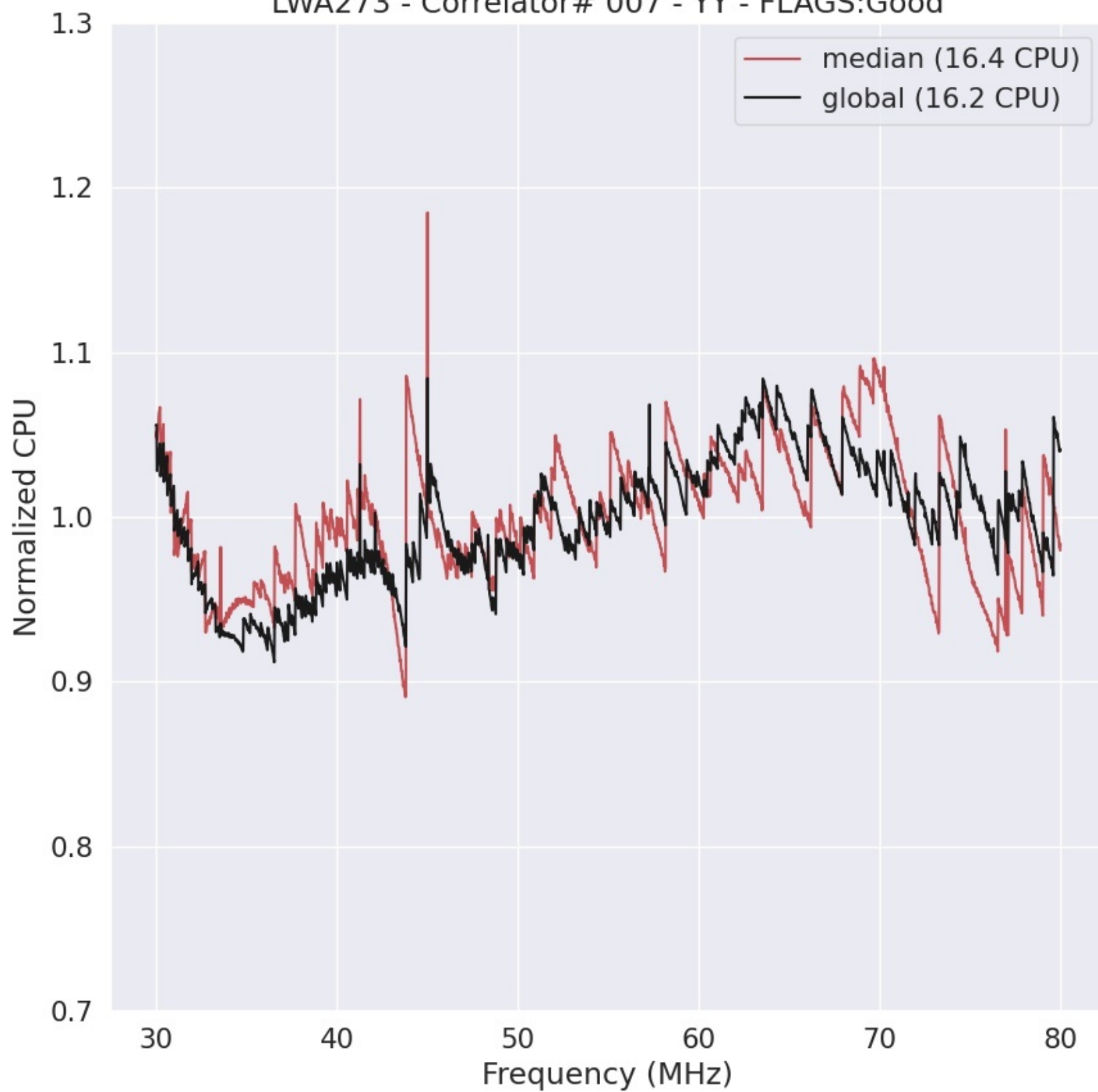
LWA273 - Correlator# 007 - YY - FLAGS:Good
