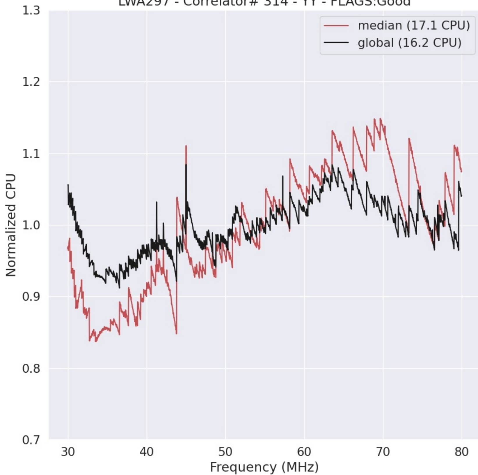
LWA297 - Correlator# 314 - YY - FLAGS:Good
