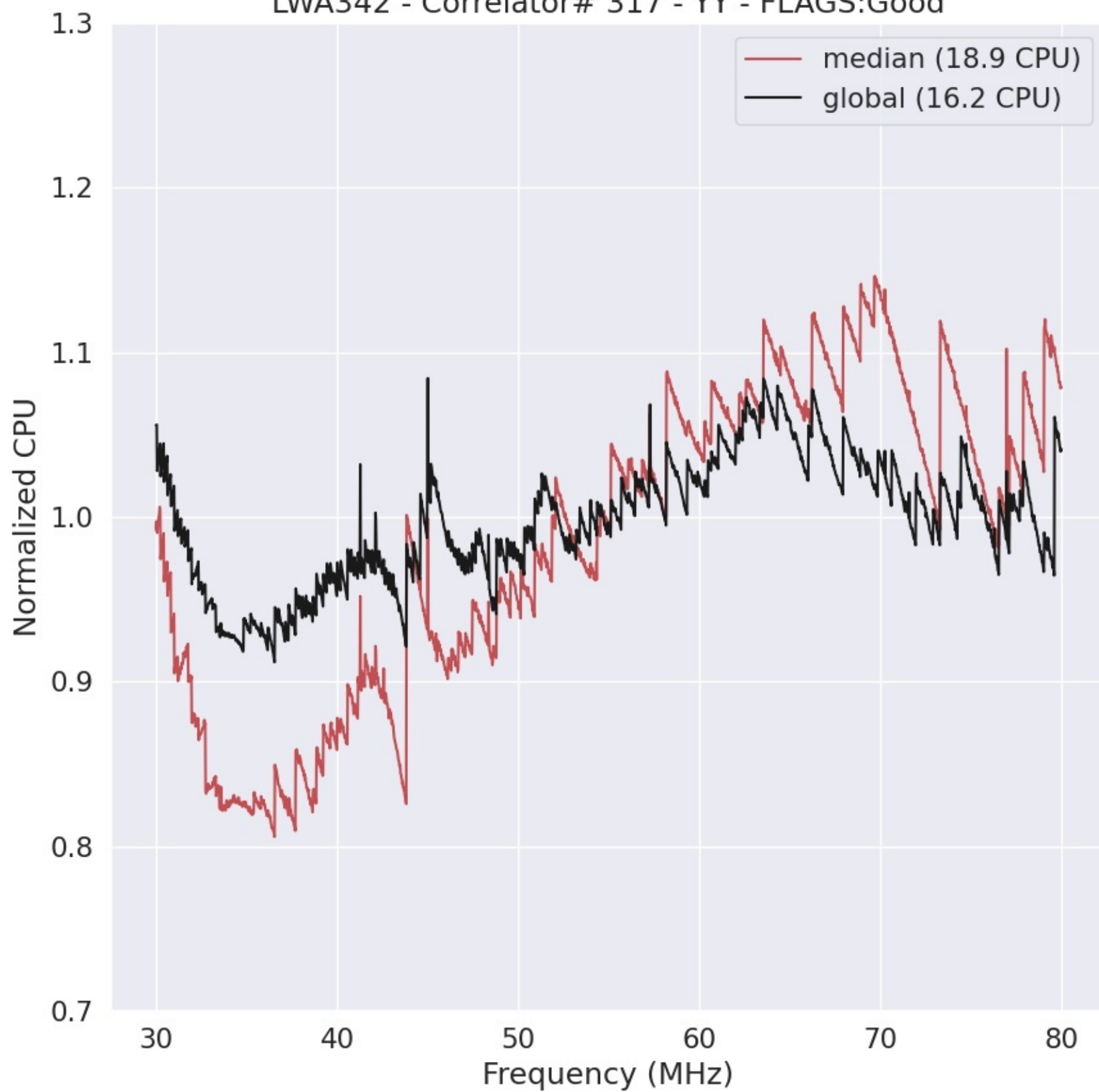
LWA342 - Correlator# 317 - YY - FLAGS:Good
