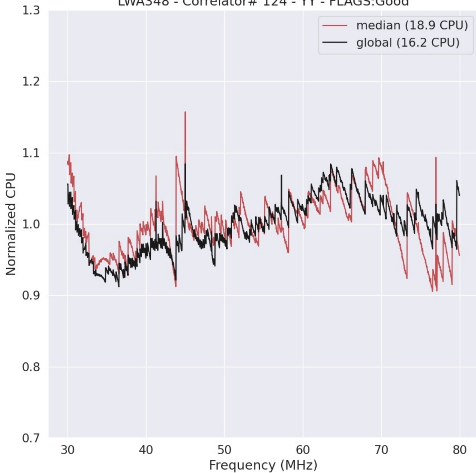
LWA348 - Correlator# 124 - YY - FLAGS:Good
