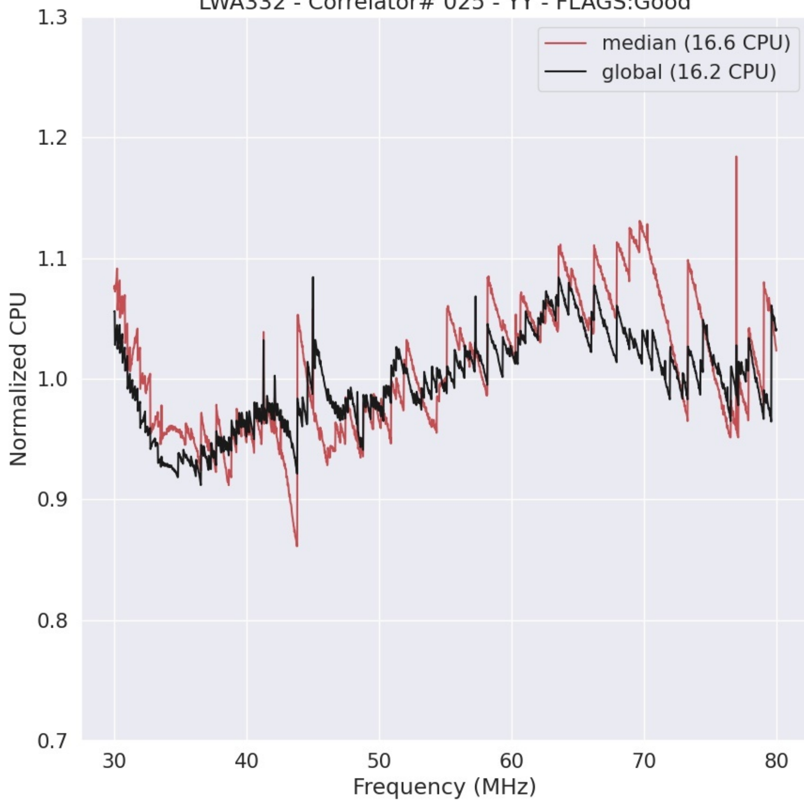
LWA332 - Correlator# 025 - YY - FLAGS:Good
