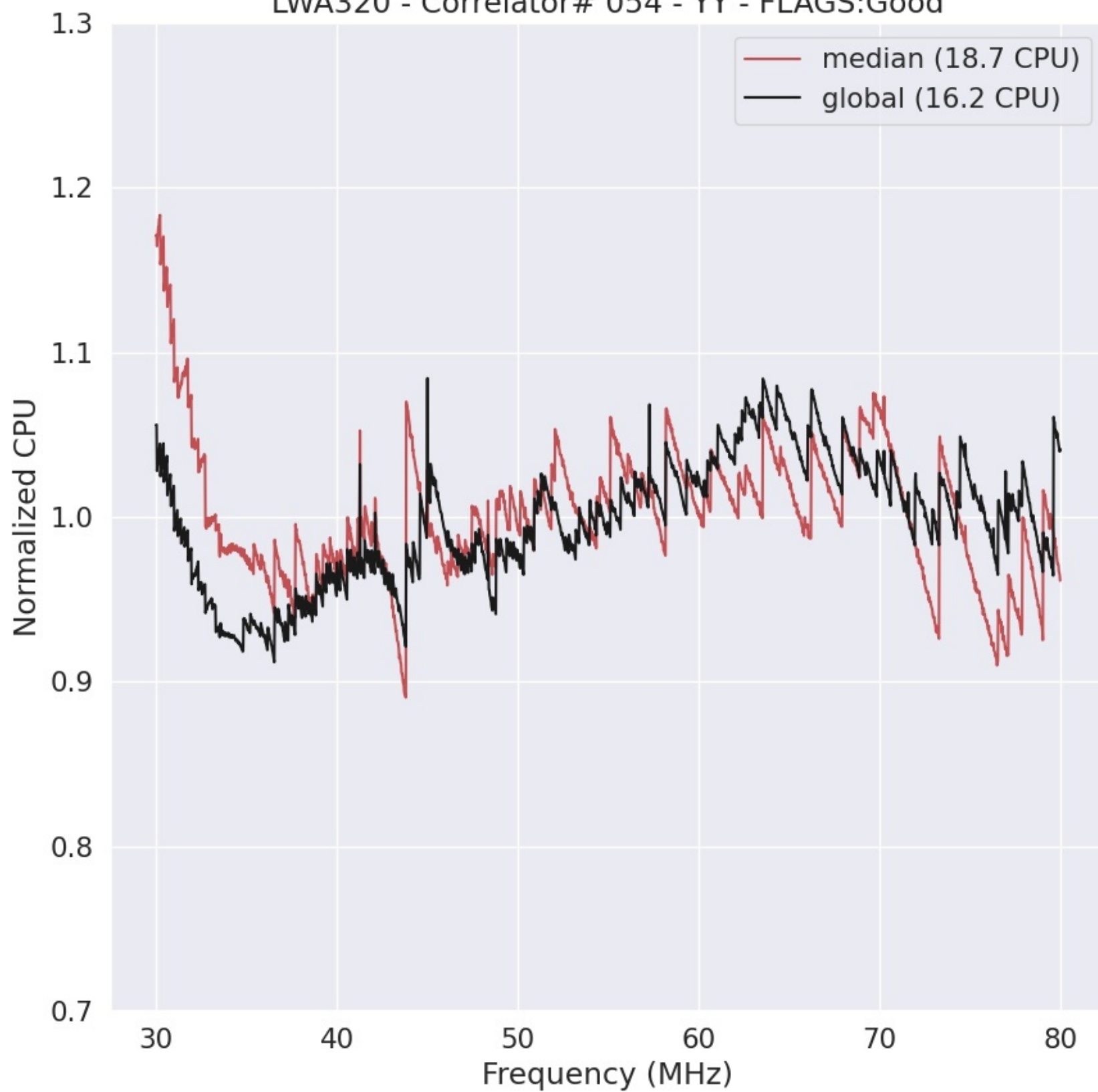
LWA320 - Correlator# 054 - YY - FLAGS:Good
