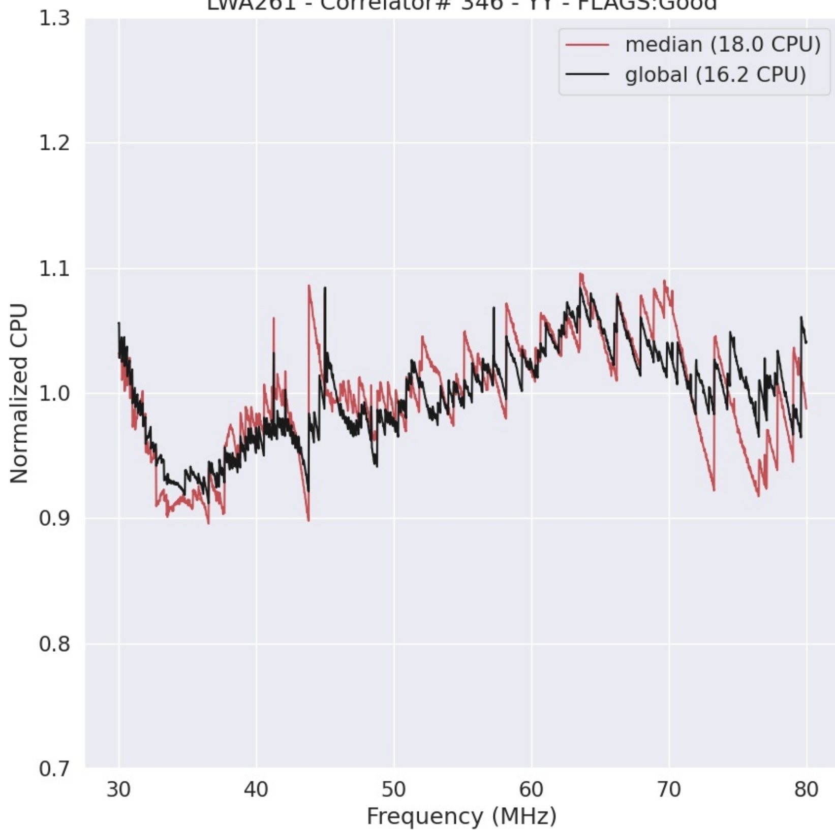
LWA261 - Correlator# 346 - YY - FLAGS:Good
