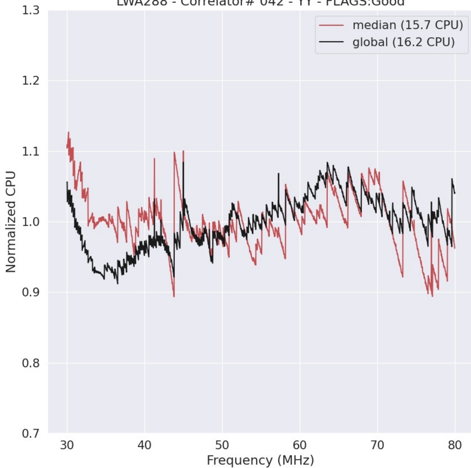
LWA288 - Correlator# 042 - YY - FLAGS:Good
