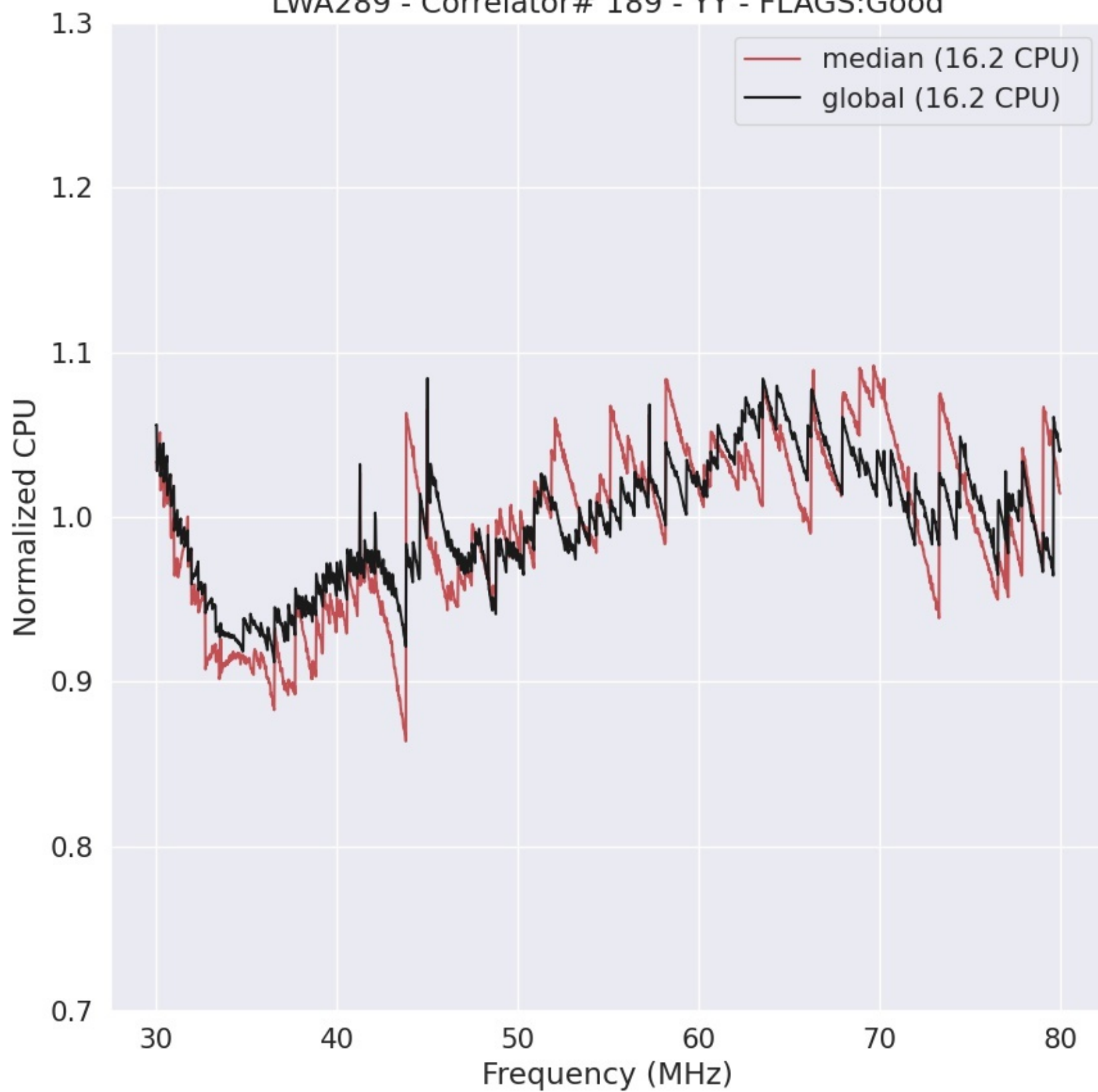
LWA289 - Correlator# 189 - YY - FLAGS:Good
