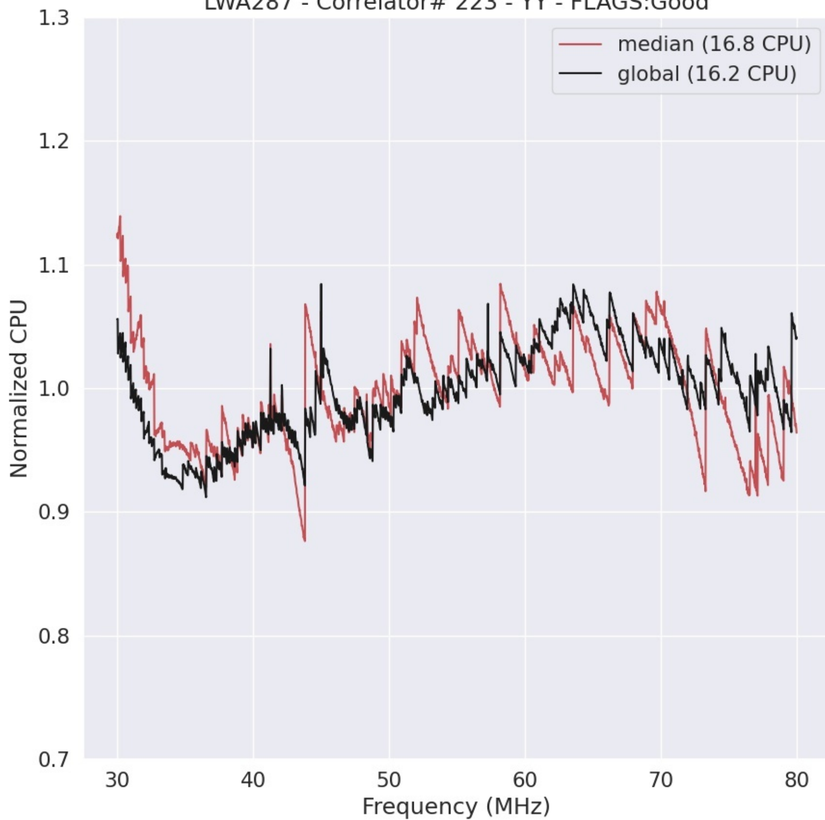
LWA287 - Correlator# 223 - YY - FLAGS:Good
