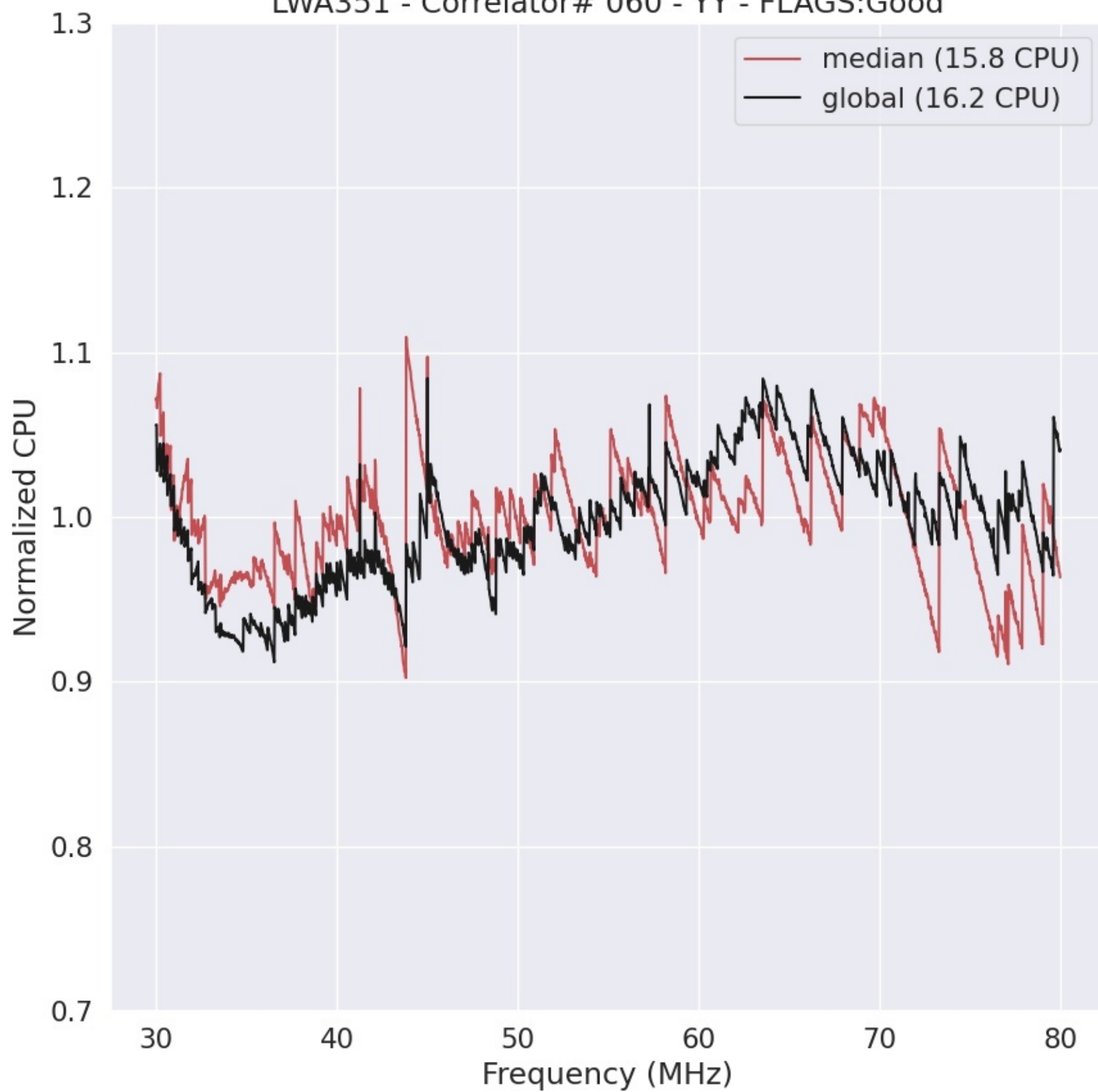
LWA351 - Correlator# 060 - YY - FLAGS:Good
