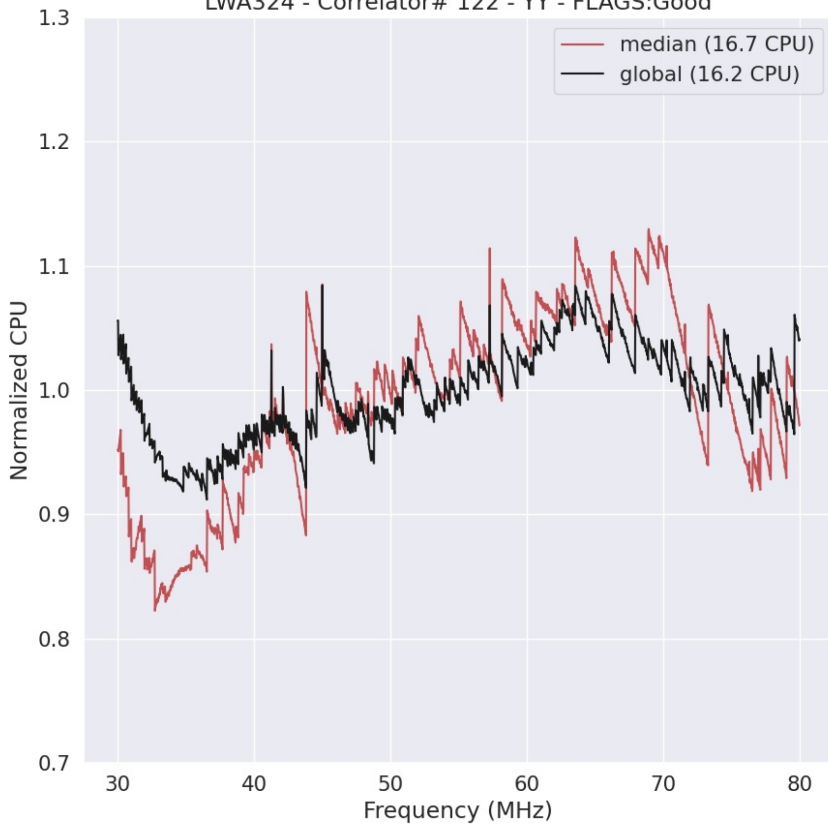
LWA324 - Correlator# 122 - YY - FLAGS:Good
