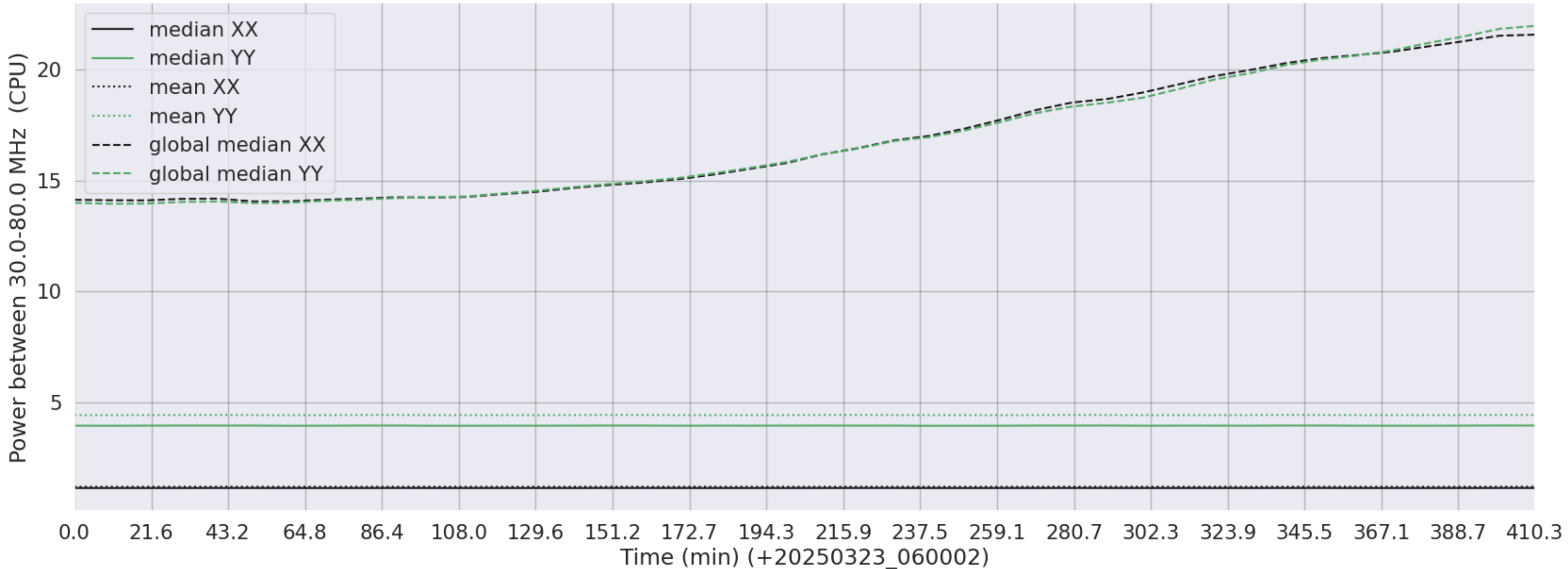
LWA326 - Correlator# 250 - XX FLAGS:LowPower - YY FLAGS:HighTimeVar+BadSpecShape
