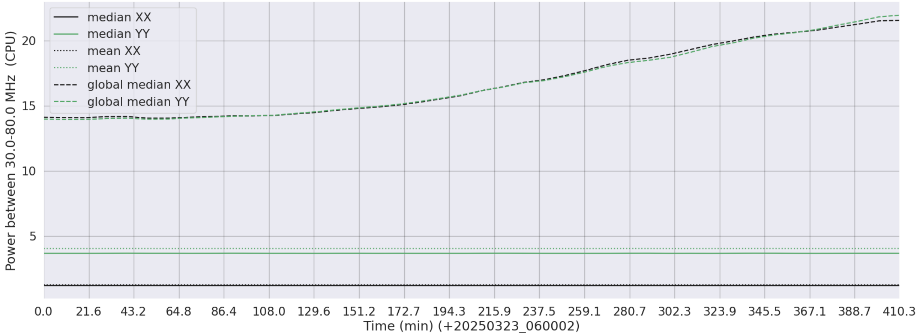
LWA269 - Correlator# 005 - XX FLAGS:LowPower - YY FLAGS:HighTimeVar+BadSpecShape
