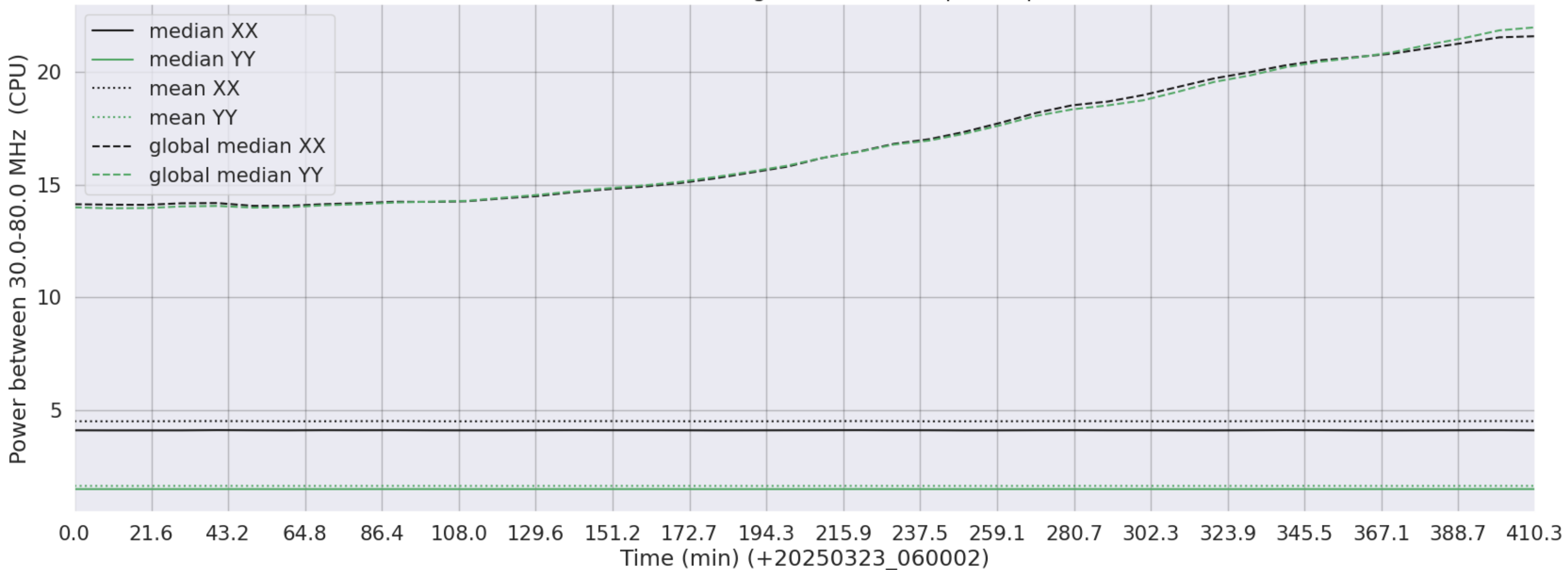
LWA313 - Correlator# 018 - XX FLAGS:HighTimeVar+BadSpecShape - YY FLAGS:LowPower
