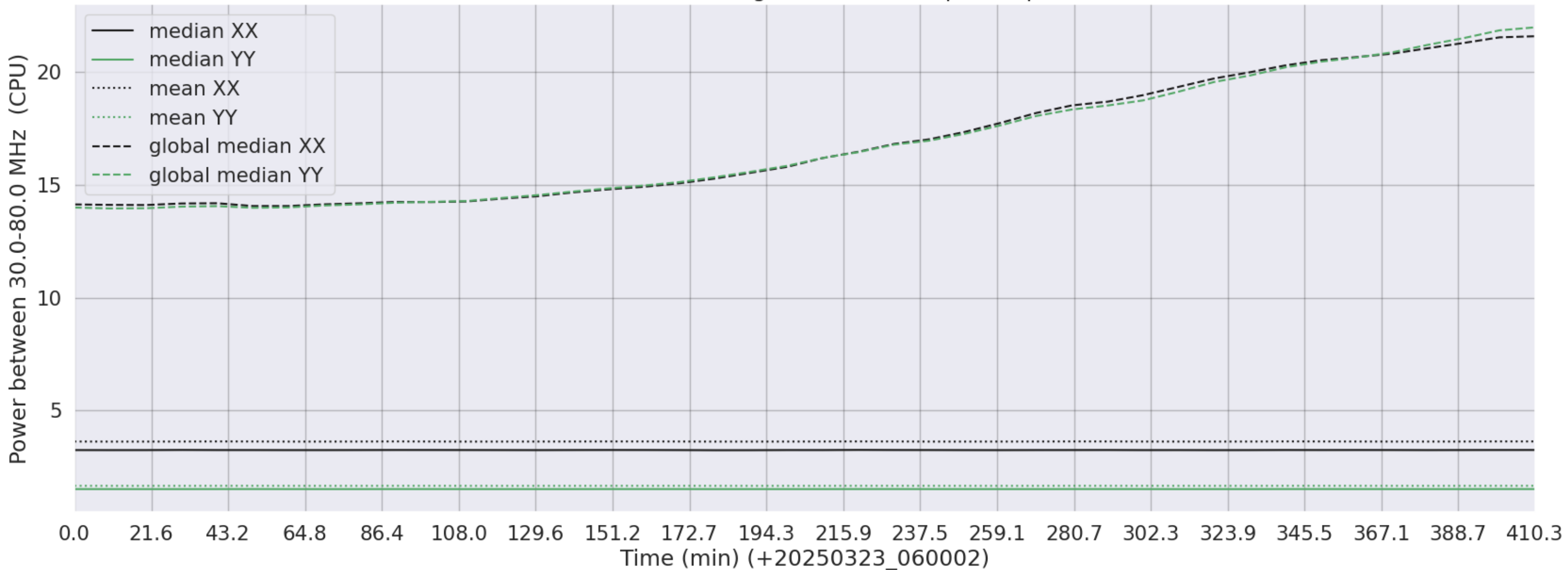
LWA339 - Correlator# 027 - XX FLAGS:HighTimeVar+BadSpecShape - YY FLAGS:LowPower
