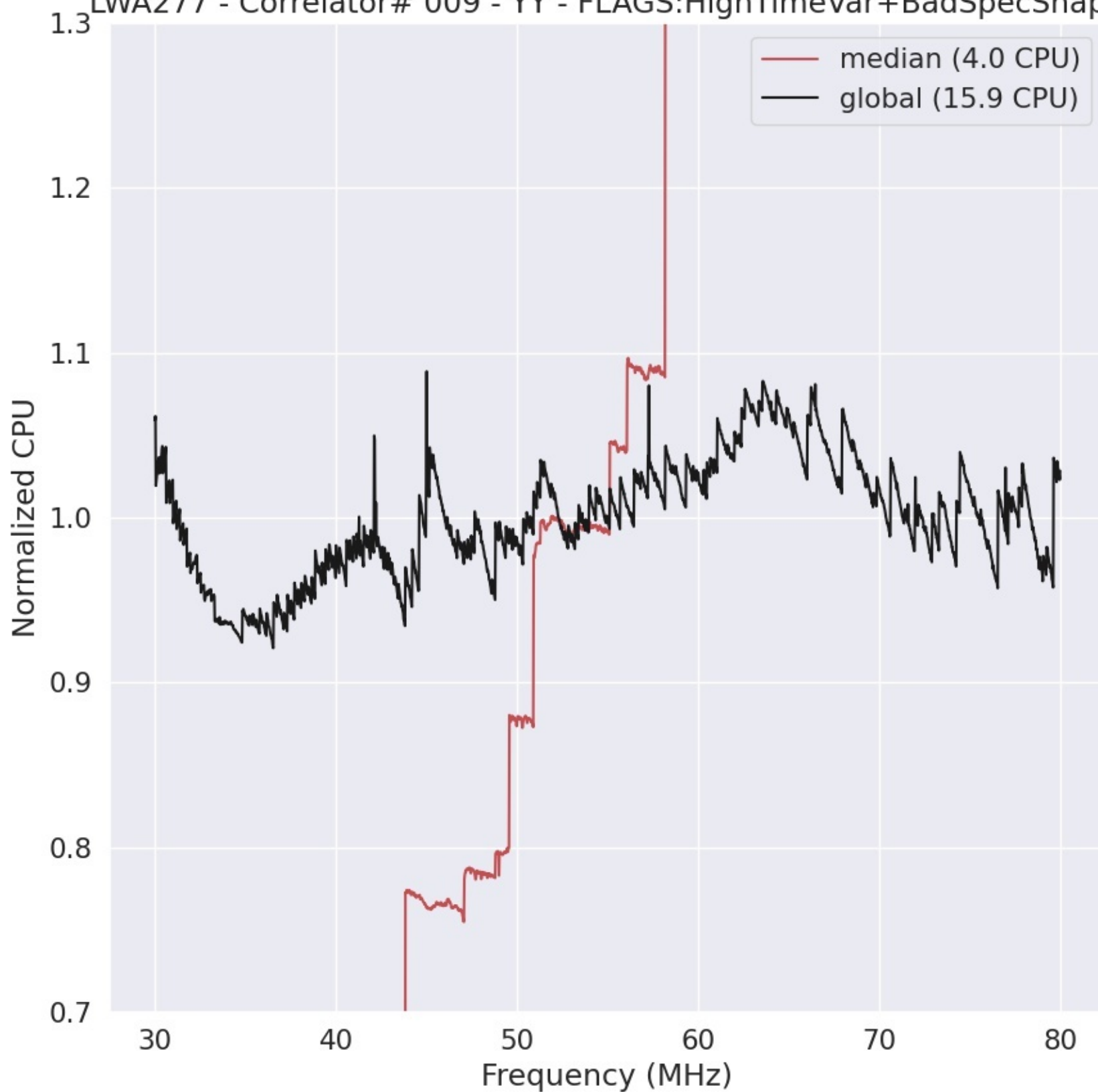
LWA277 - Correlator# 009 - YY - FLAGS:HighTimeVar+BadSpecShape
