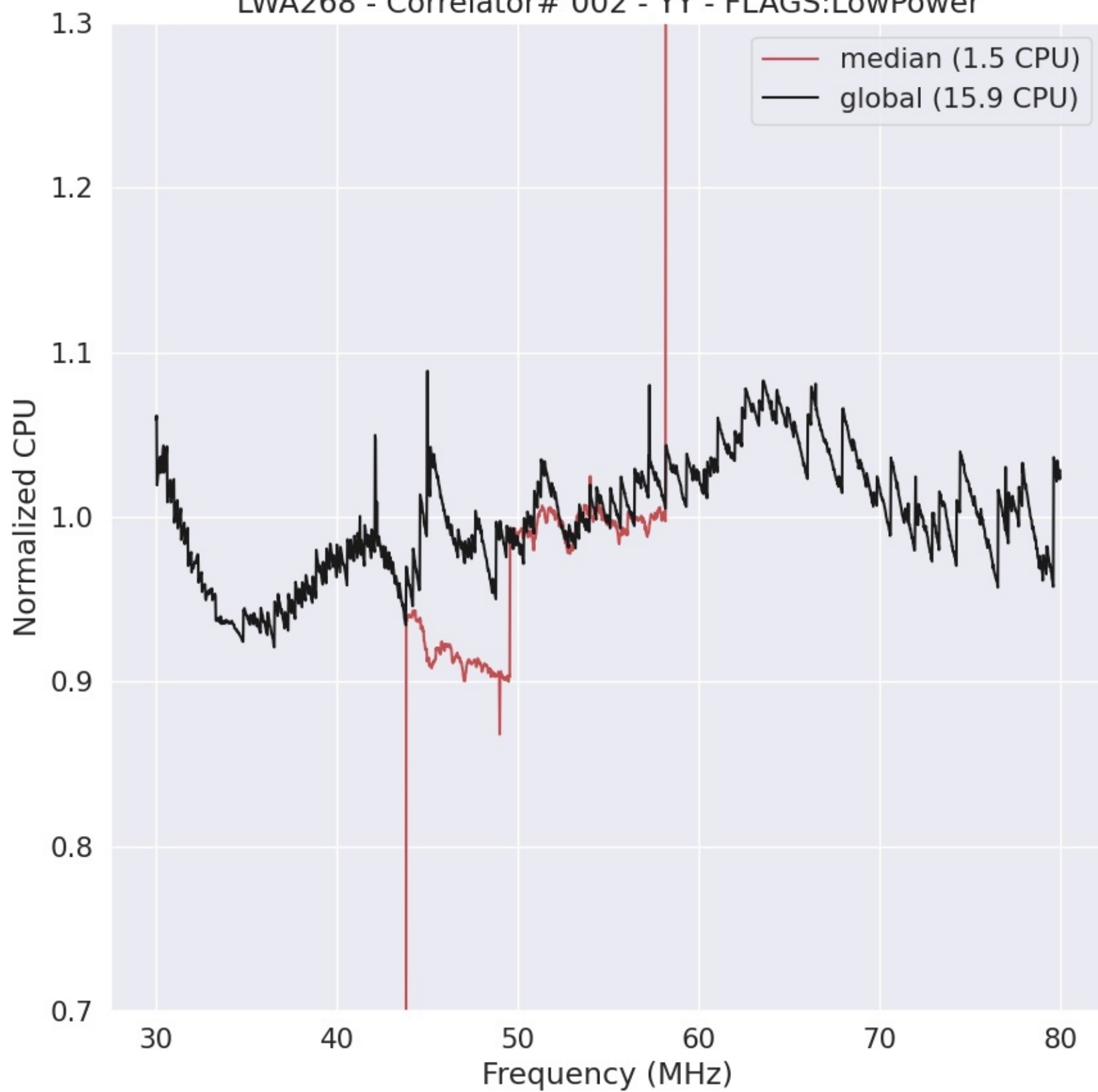
LWA268 - Correlator# 002 - YY - FLAGS:LowPower
