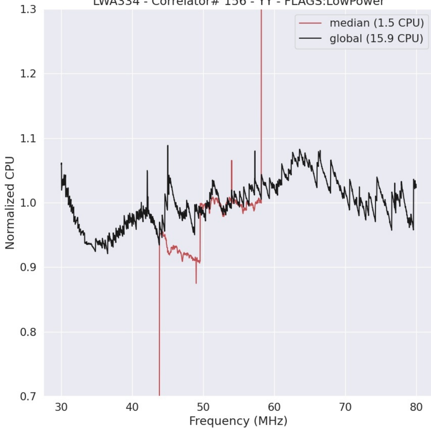
LWA334 - Correlator# 156 - YY - FLAGS:LowPower
