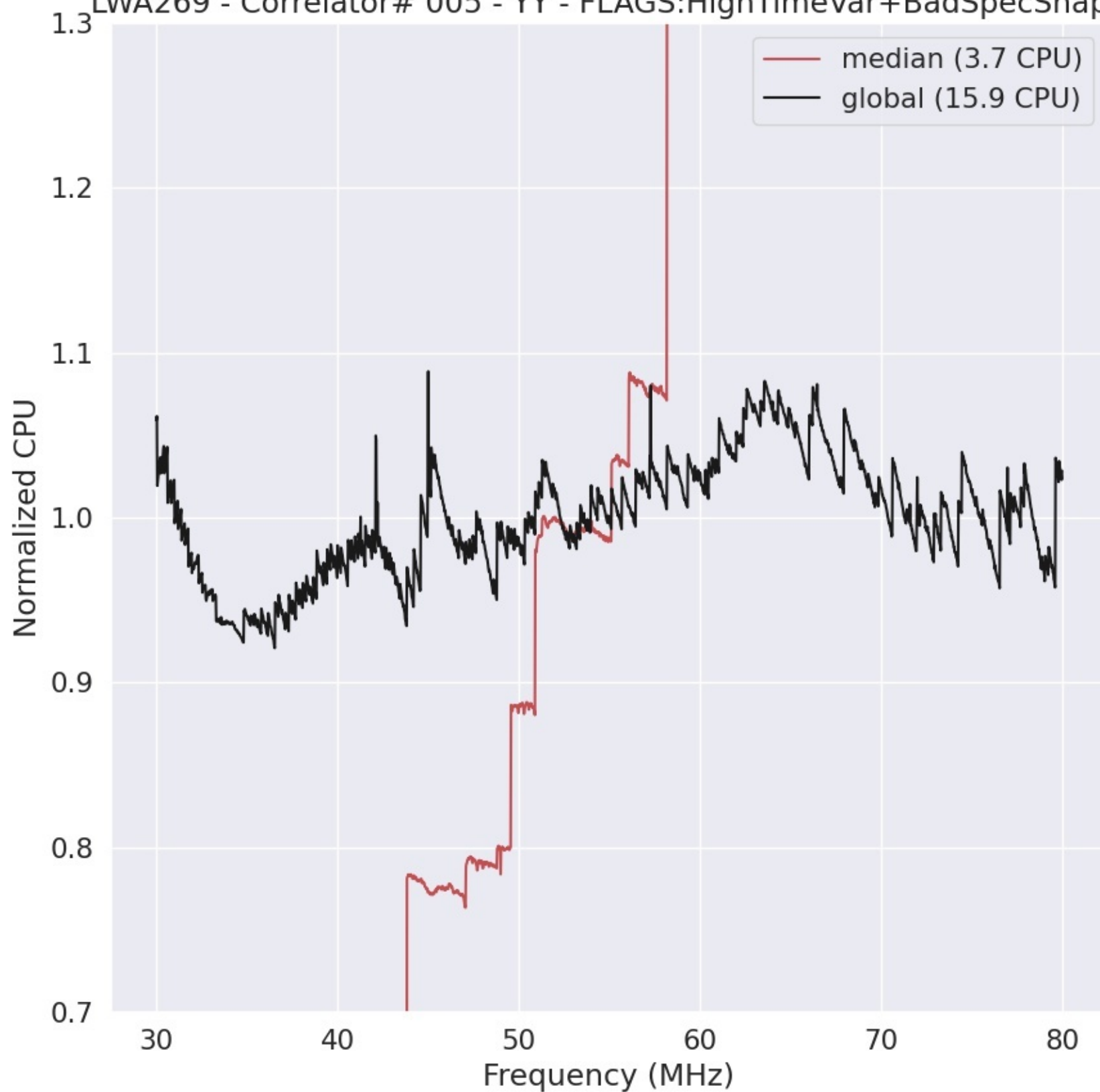
LWA269 - Correlator# 005 - YY - FLAGS:HighTimeVar+BadSpecShape
