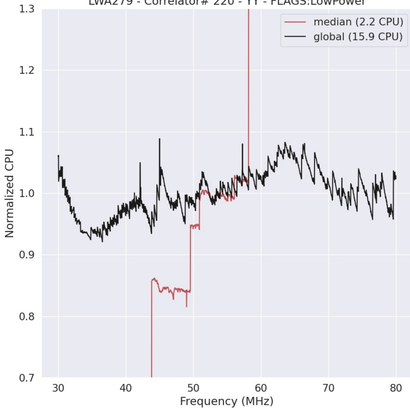
LWA279 - Correlator# 220 - YY - FLAGS:LowPower
