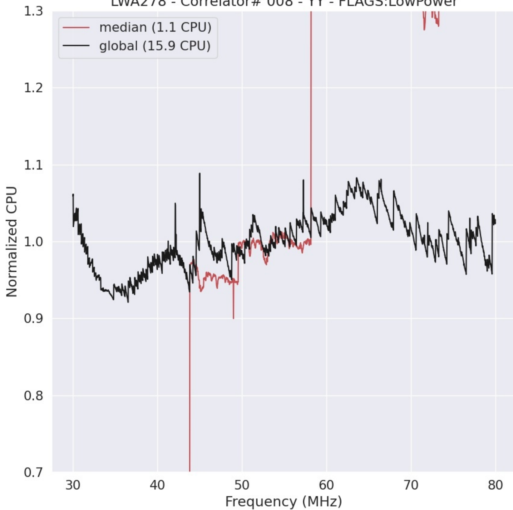
LWA278 - Correlator# 008 - YY - FLAGS:LowPower
