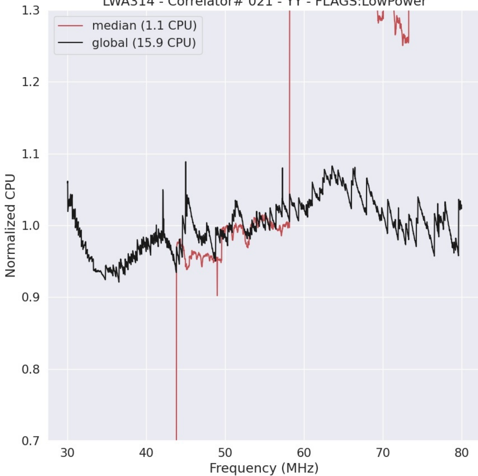
LWA314 - Correlator# 021 - YY - FLAGS:LowPower
