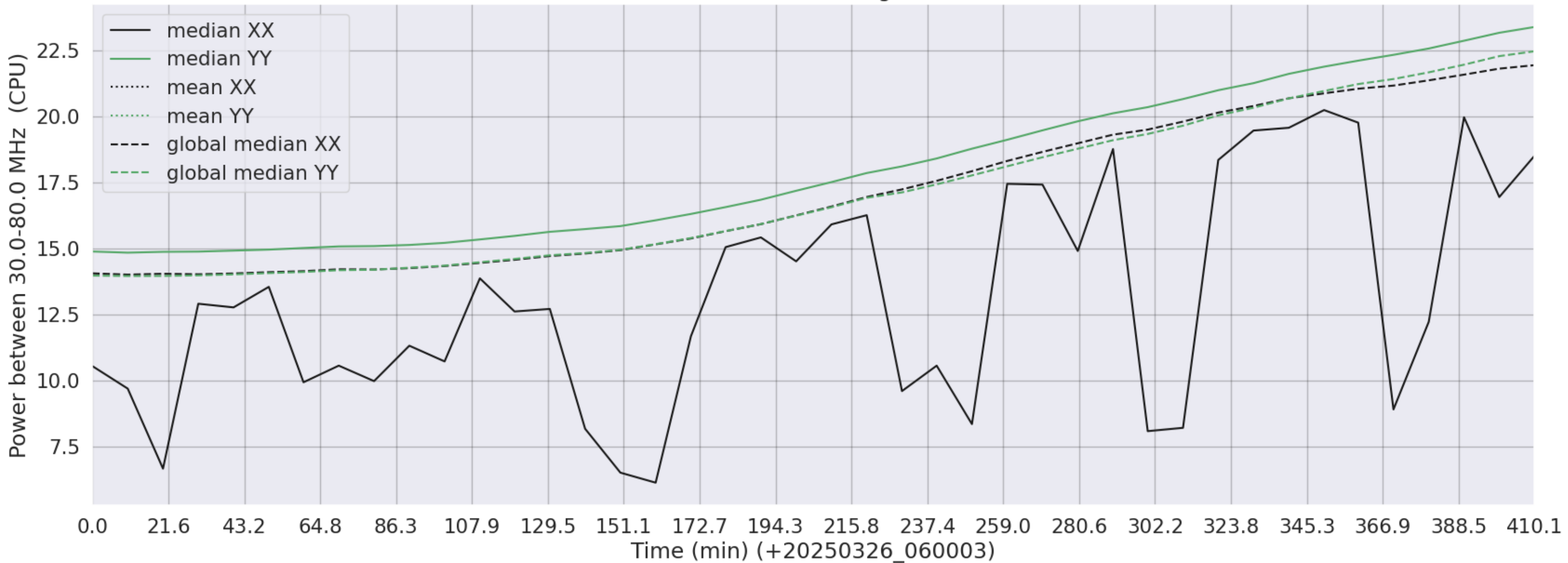
LWA105 - Correlator# 178 - XX FLAGS:HighTimeVar - YY FLAGS:Good
