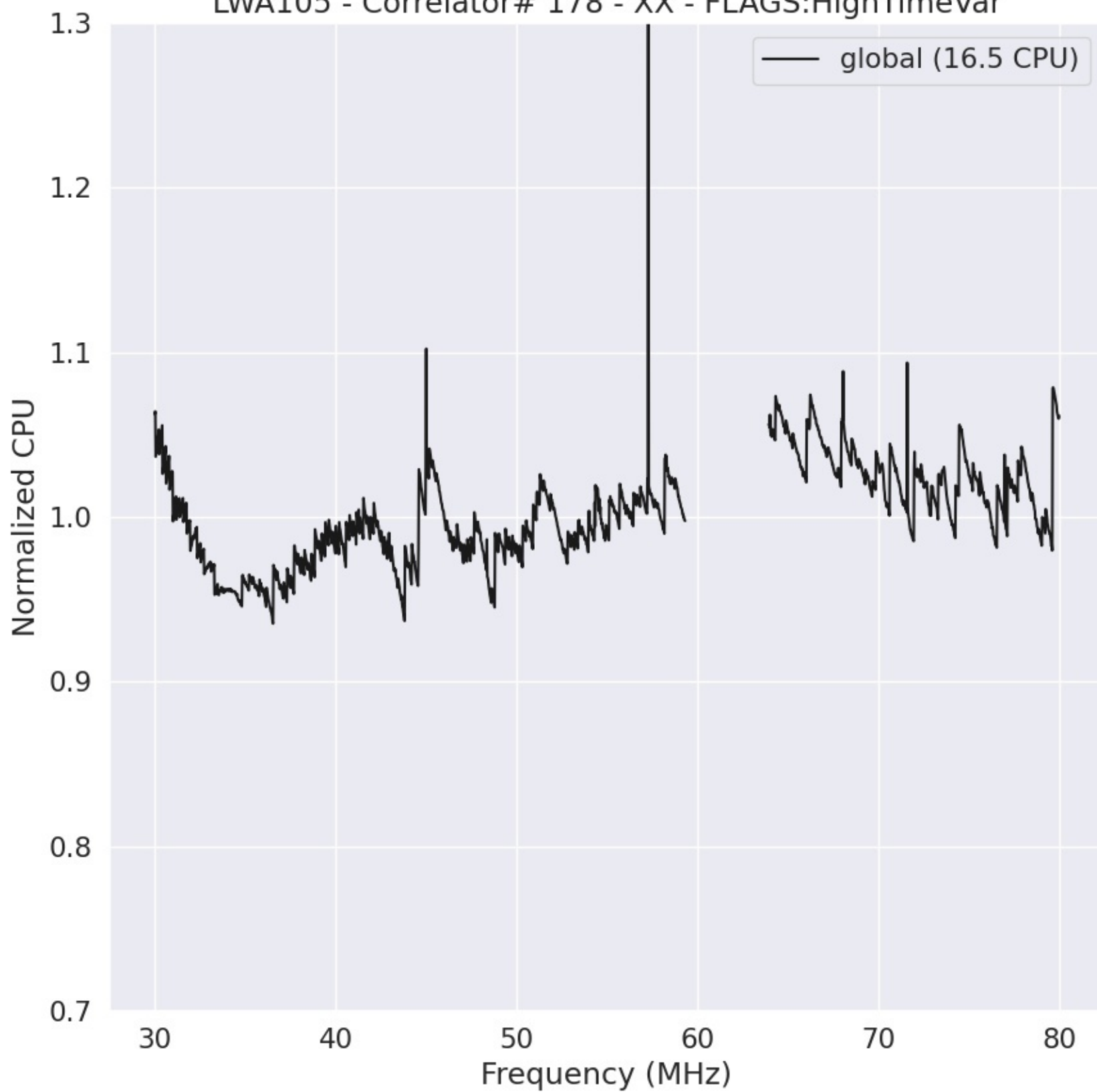
LWA105 - Correlator# 178 - XX - FLAGS:HighTimeVar
