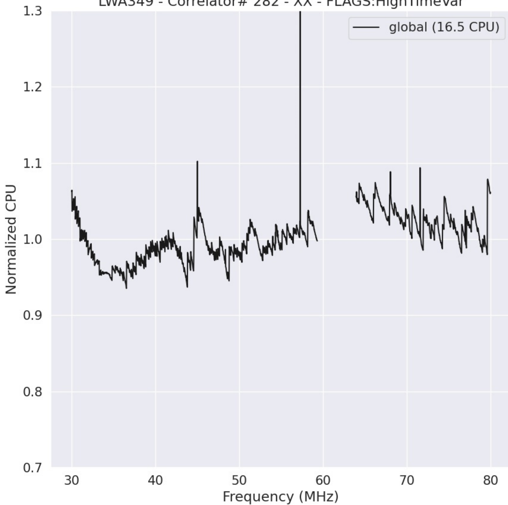
LWA349 - Correlator# 282 - XX - FLAGS:HighTimeVar
