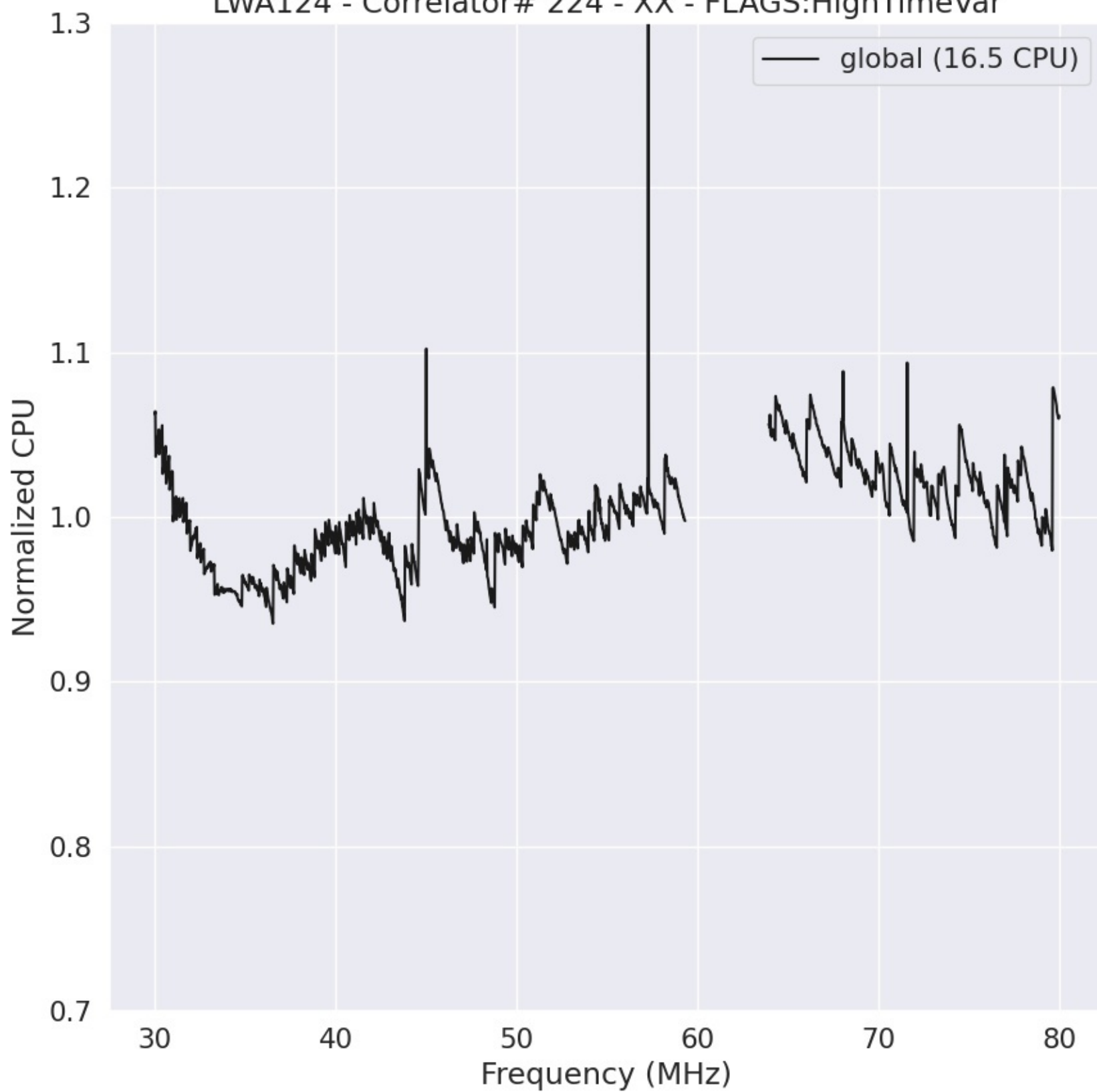
LWA124 - Correlator# 224 - XX - FLAGS:HighTimeVar
