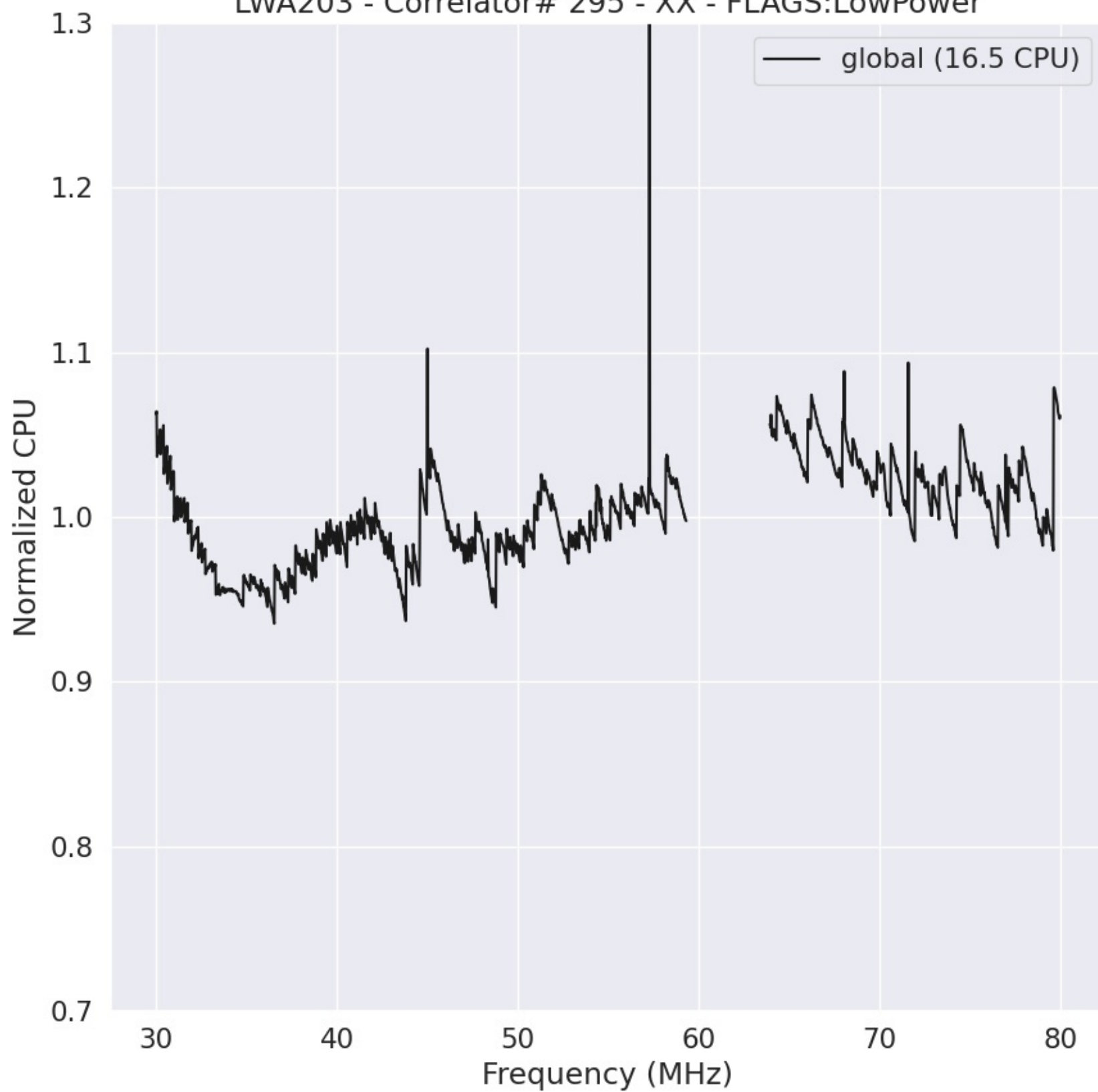
LWA203 - Correlator# 295 - XX - FLAGS:LowPower
