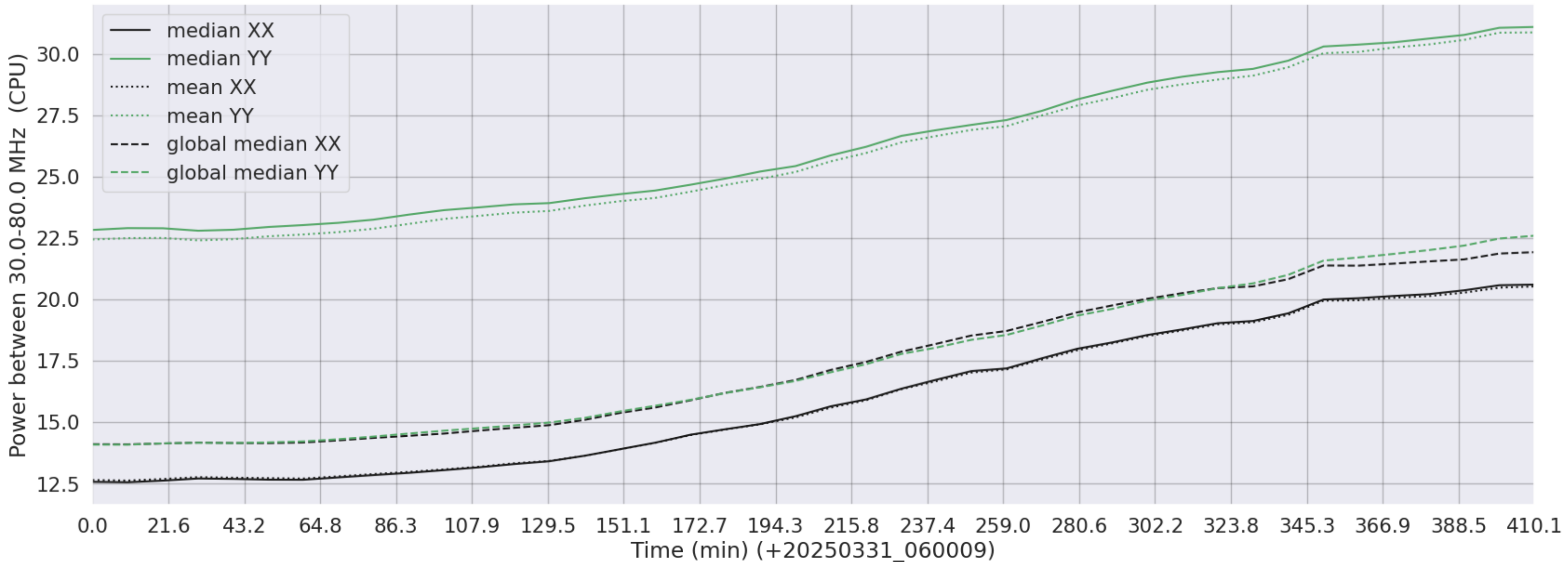
LWA303 - Correlator# 051 - XX FLAGS:Good - YY FLAGS:Good
