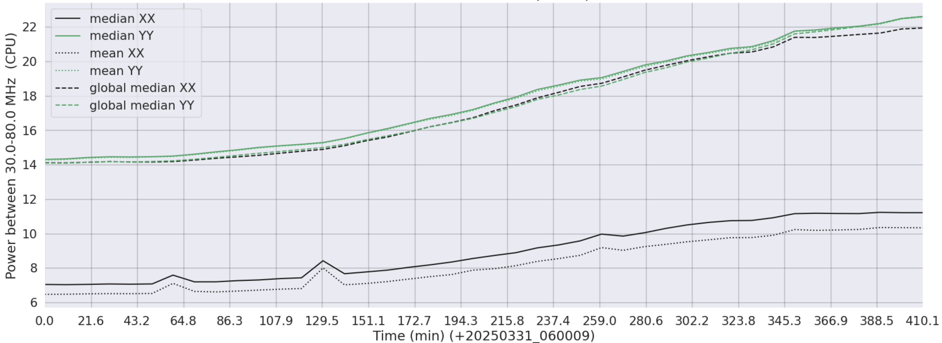
LWA103 - Correlator# 176 - XX FLAGS:BadSpecShape - YY FLAGS:Good
