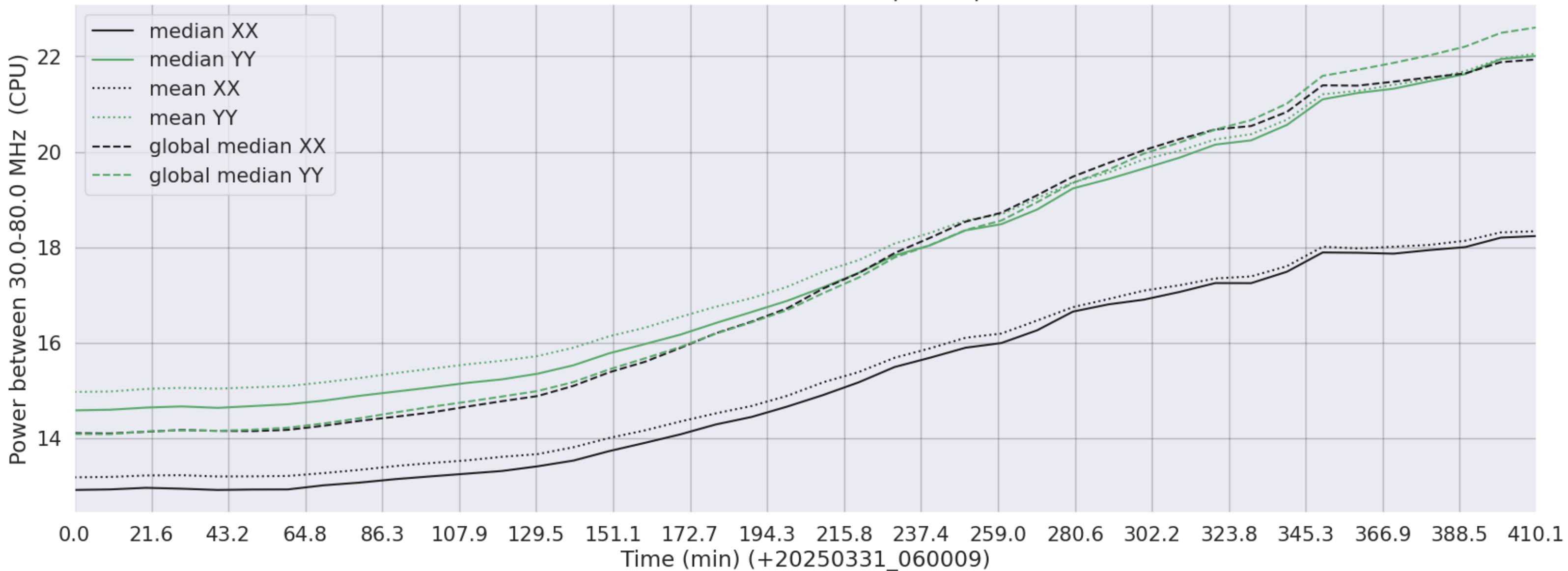
LWA129 - Correlator# 180 - XX FLAGS:BadSpecShape - YY FLAGS:Good
