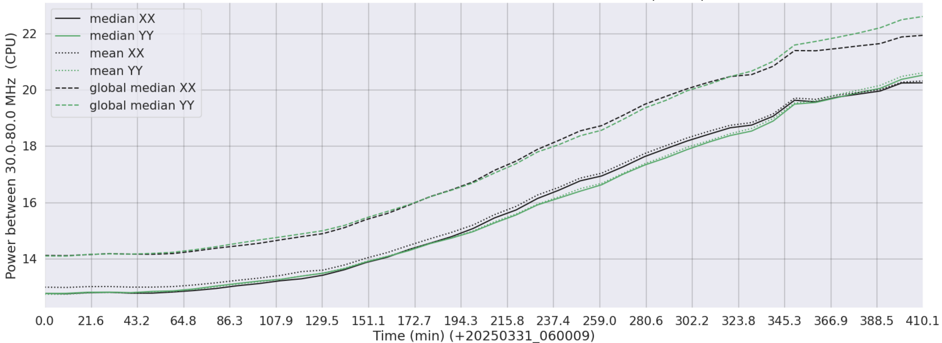
LWA021 - Correlator# 105 - XX FLAGS:Good - YY FLAGS:BadSpecShape
