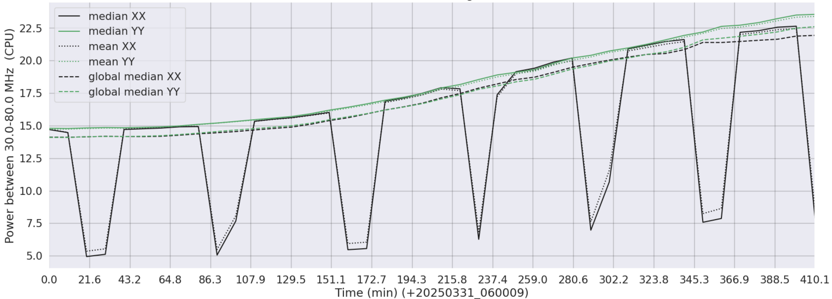
LWA349 - Correlator# 282 - XX FLAGS:HighTimeVar - YY FLAGS:Good
