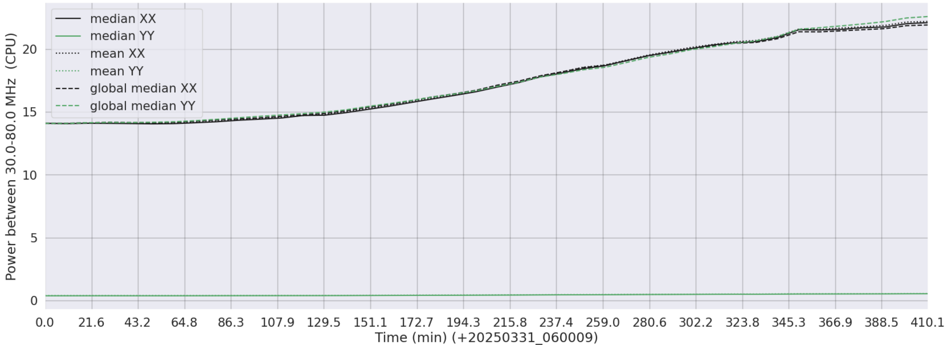
LWA185 - Correlator# 240 - XX FLAGS:Good - YY FLAGS:LowPower
