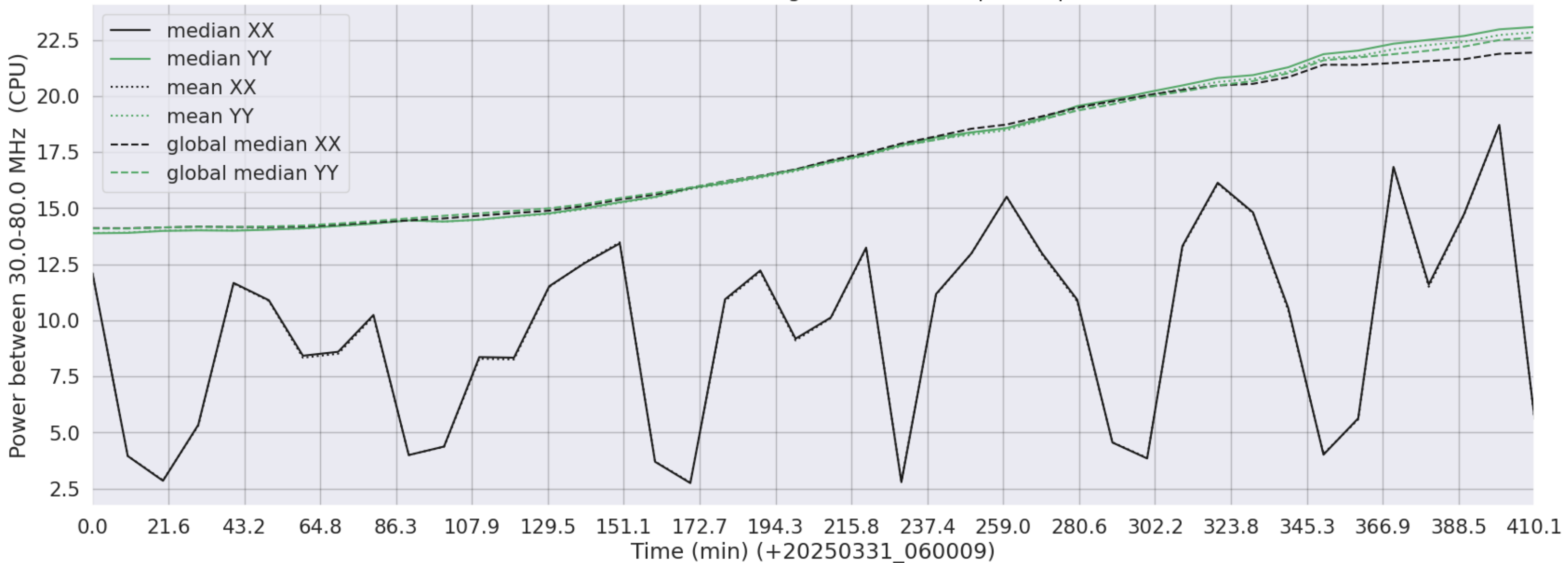
LWA124 - Correlator# 224 - XX FLAGS:HighTimeVar+BadSpecShape - YY FLAGS:Good
